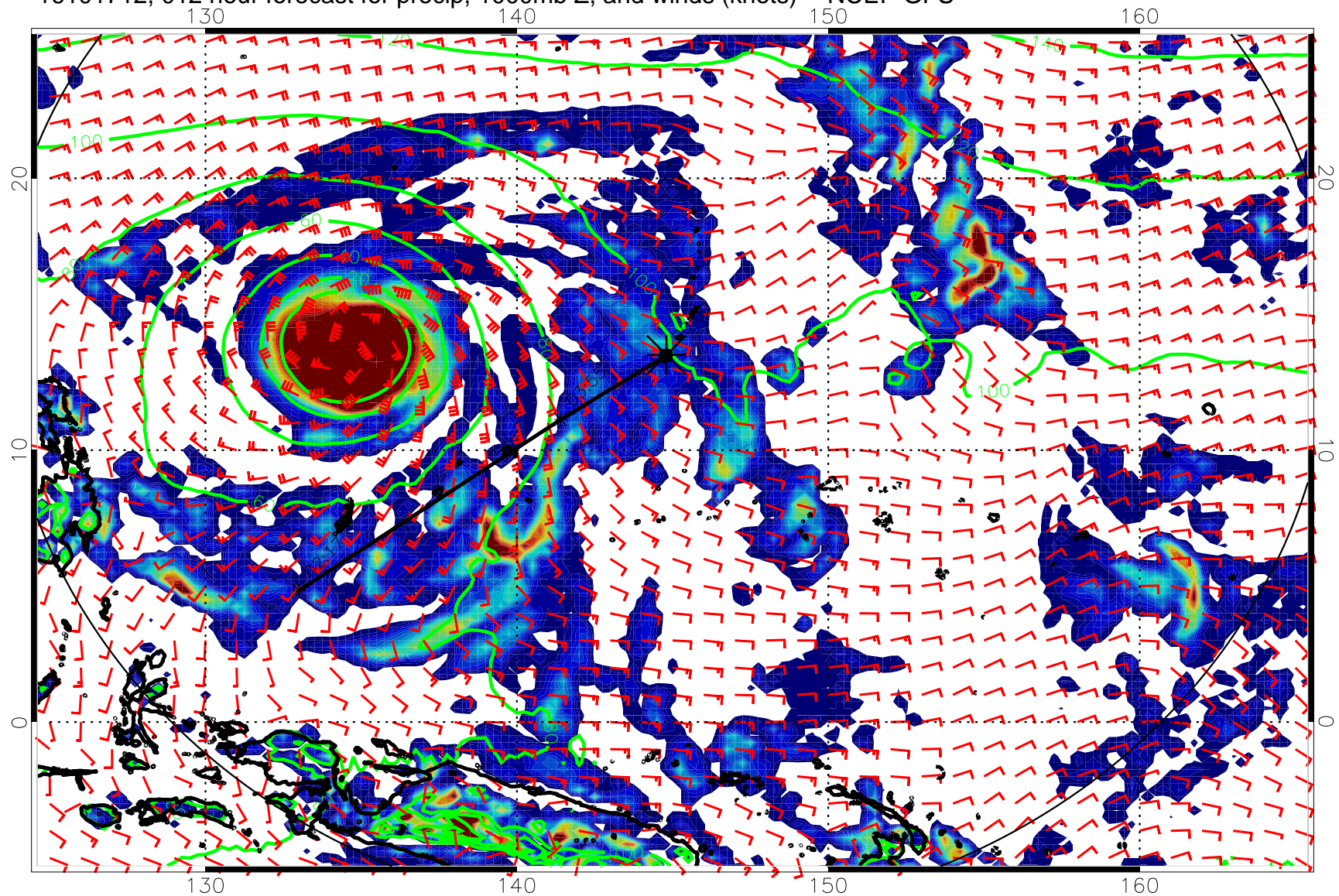
16101712, 012 hour forecast for precip, 1000mb Z, and winds (knots) -- NCEP GFS
