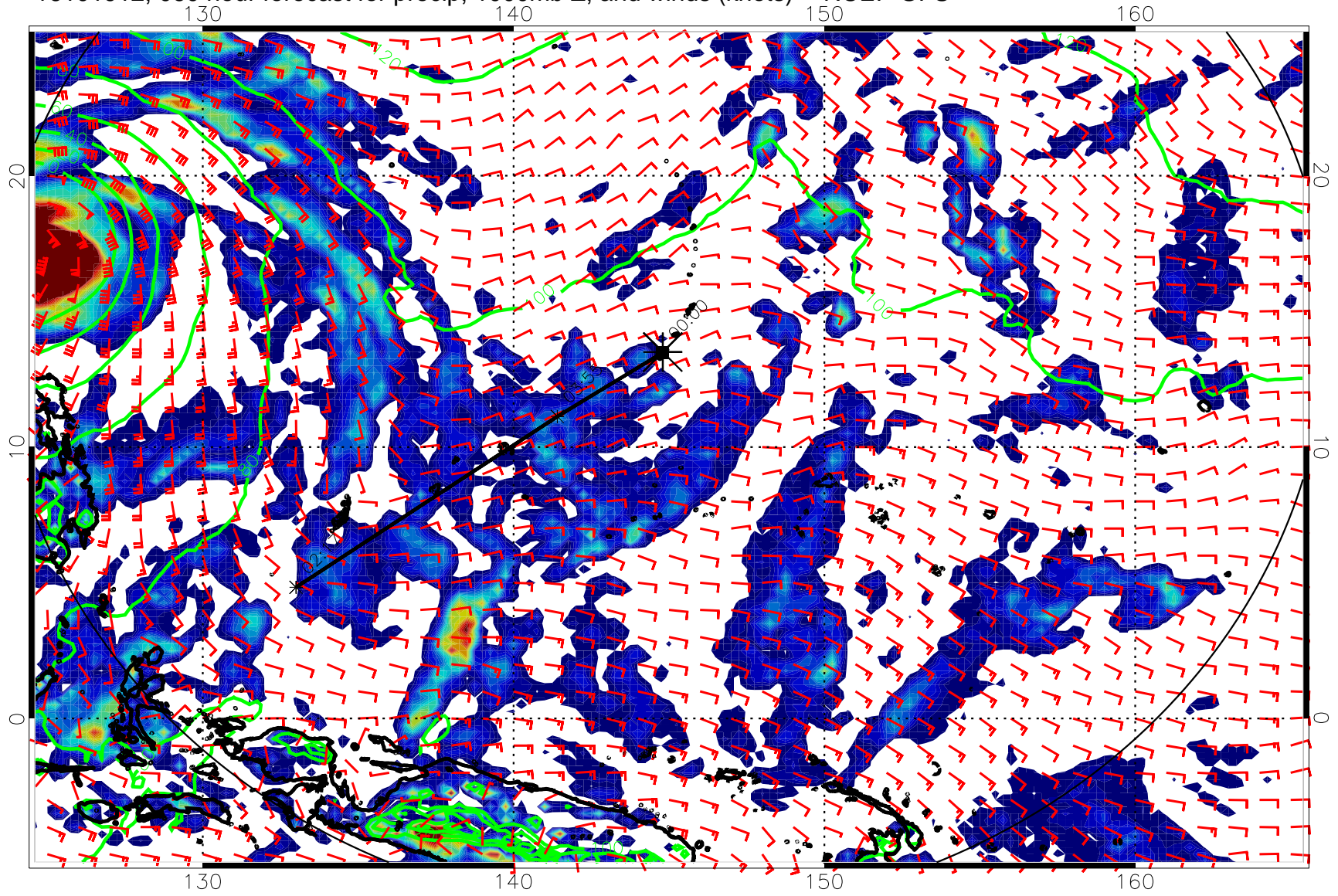
16101912, 060 hour forecast for precip, 1000mb Z, and winds (knots) -- NCEP GFS
