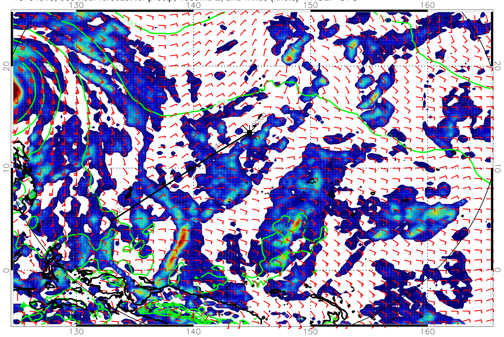
16101918, 066 hour forecast for precip, 1000mb Z, and winds (knots) -- NCEP GFS
