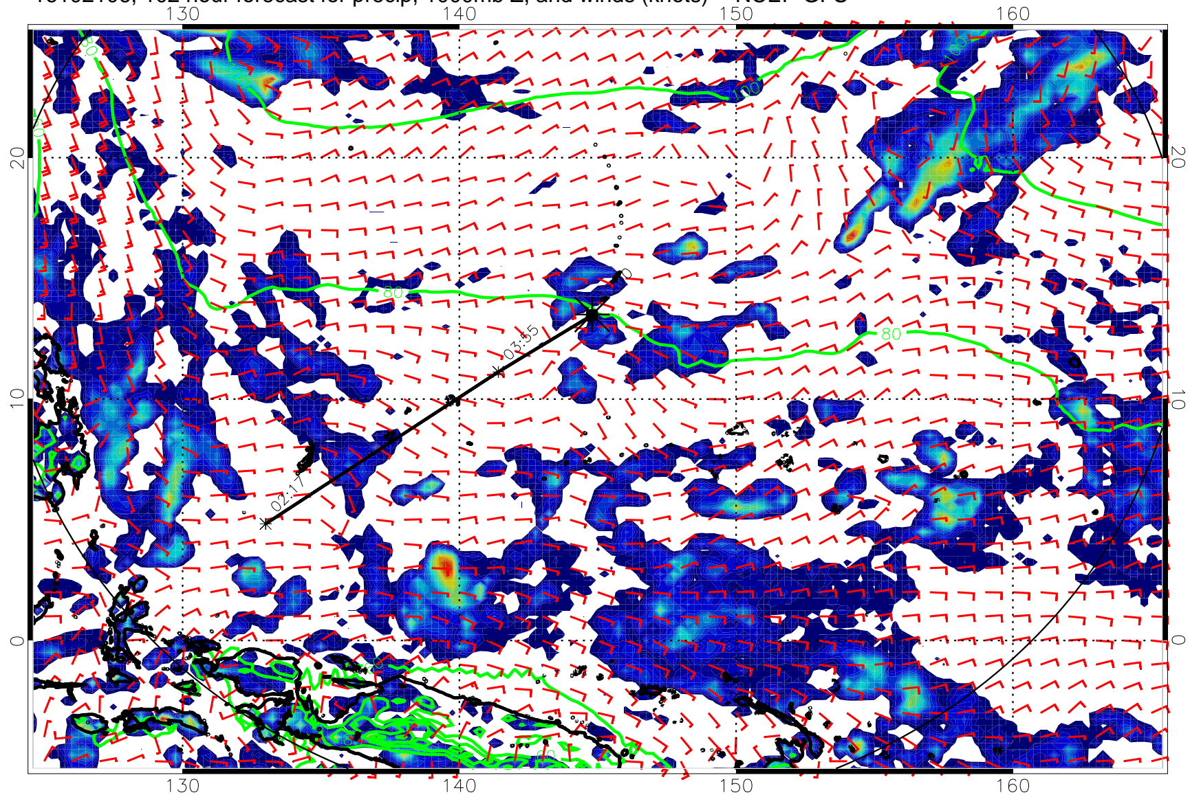
16102106, 102 hour forecast for precip, 1000mb Z, and winds (knots) -- NCEP GFS
