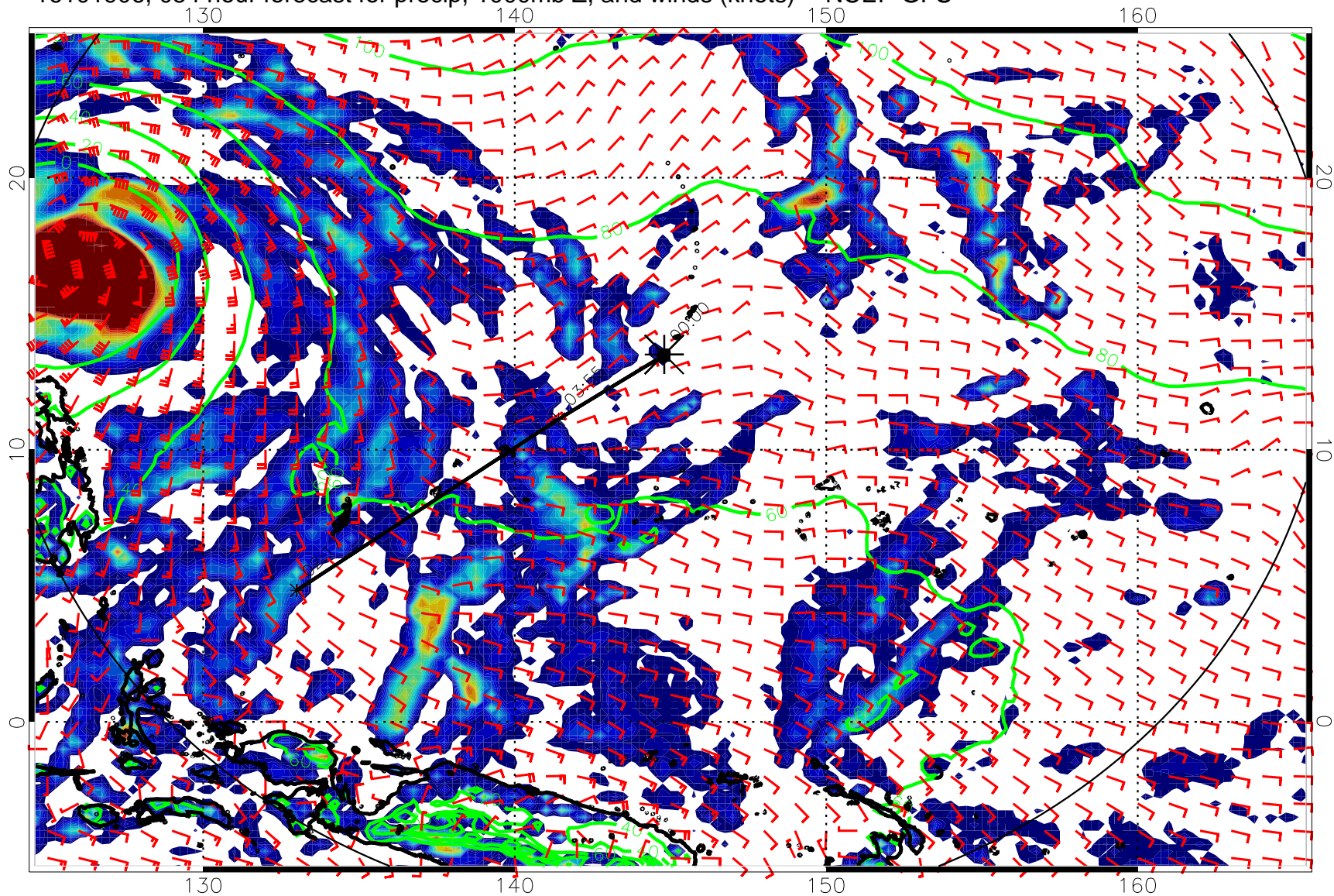
16101906, 054 hour forecast for precip, 1000mb Z, and winds (knots) -- NCEP GFS
