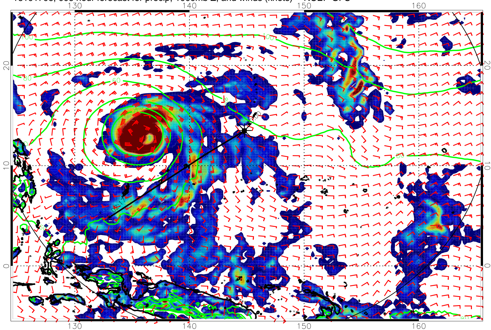
16101706, 006 hour forecast for precip, 1000mb Z, and winds (knots) -- NCEP GFS
