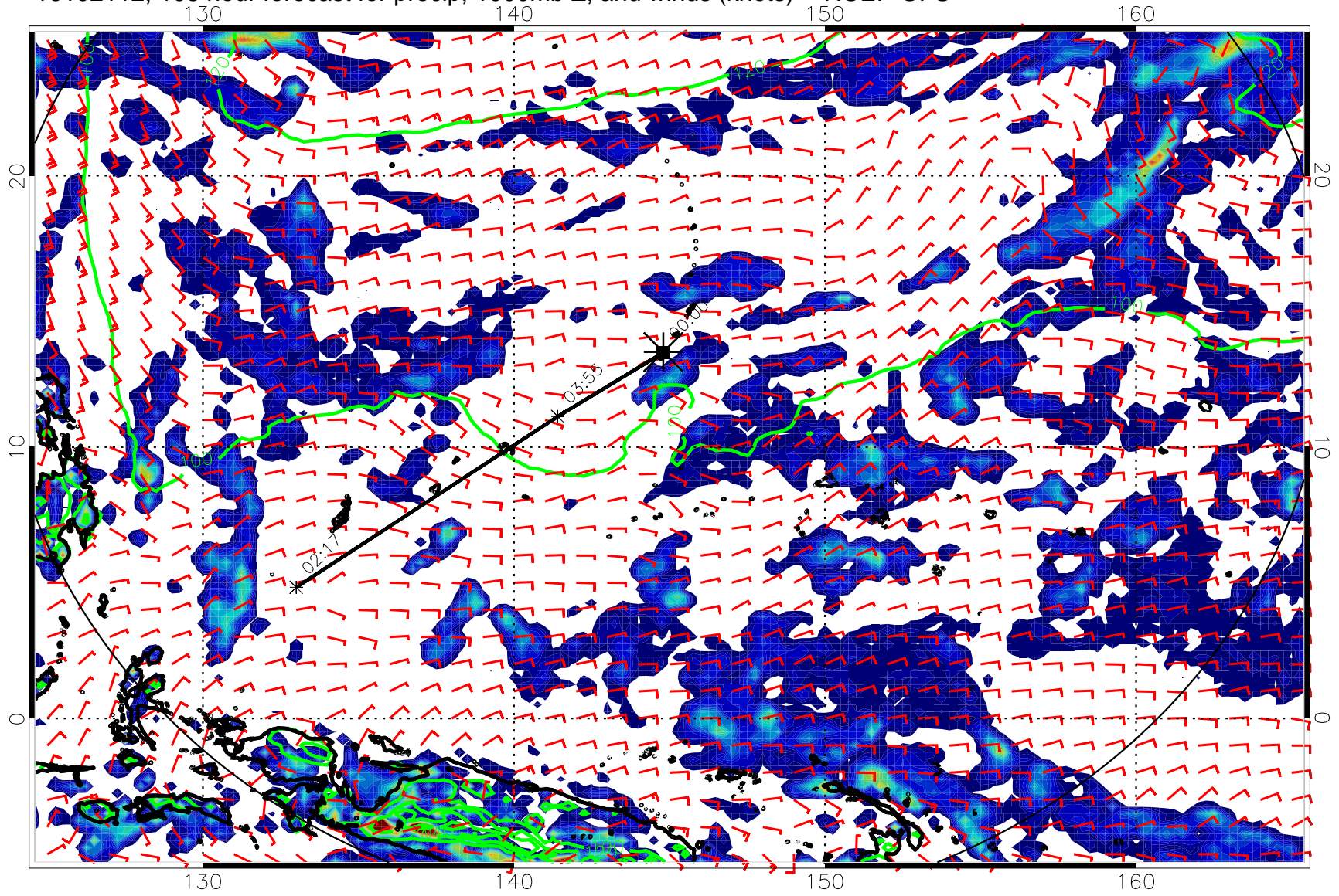
16102112, 108 hour forecast for precip, 1000mb Z, and winds (knots) -- NCEP GFS
