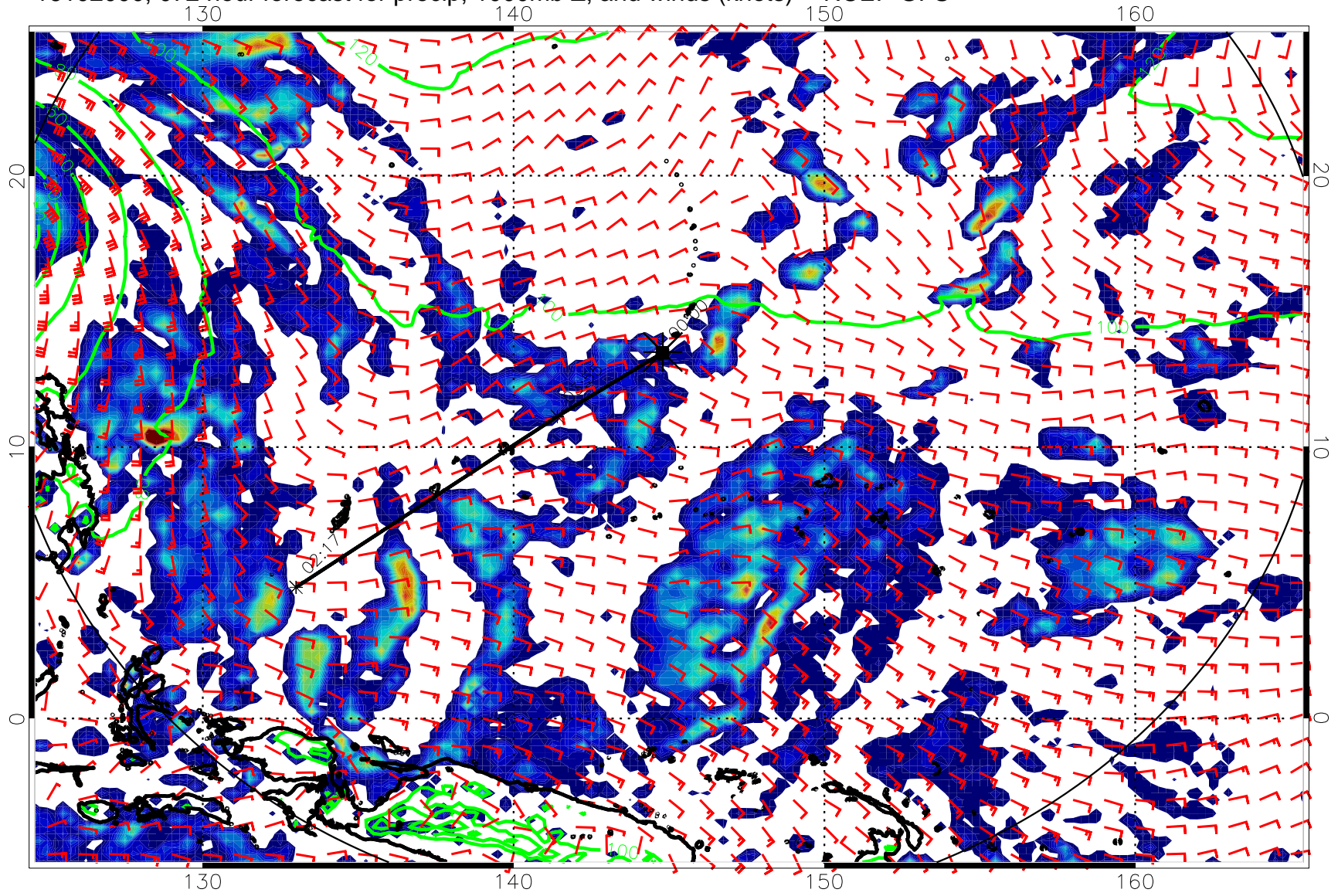
16102000, 072 hour forecast for precip, 1000mb Z, and winds (knots) -- NCEP GFS
