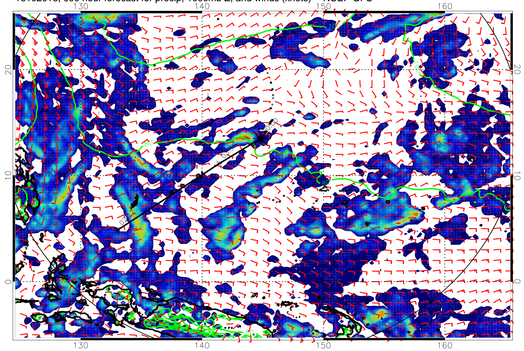
16102018, 090 hour forecast for precip, 1000mb Z, and winds (knots) -- NCEP GFS
