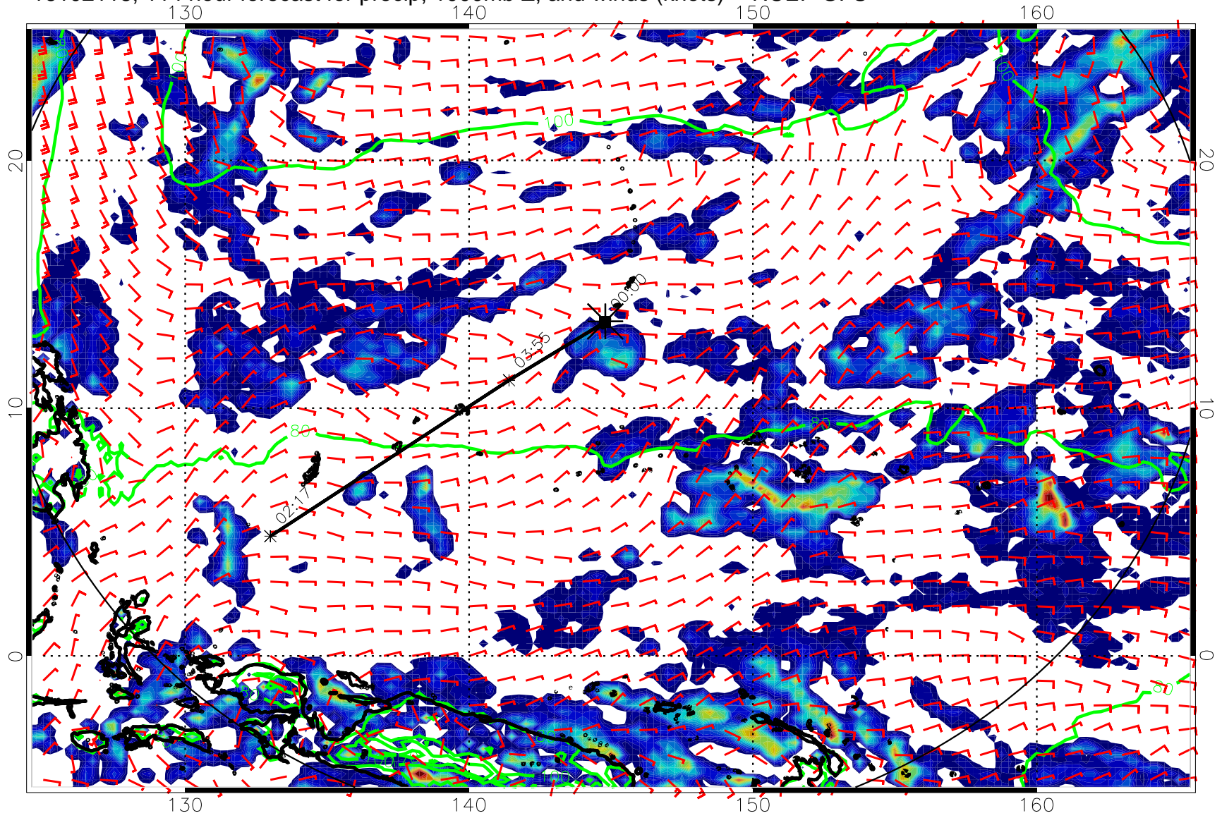
16102118, 114 hour forecast for precip, 1000mb Z, and winds (knots) -- NCEP GFS
