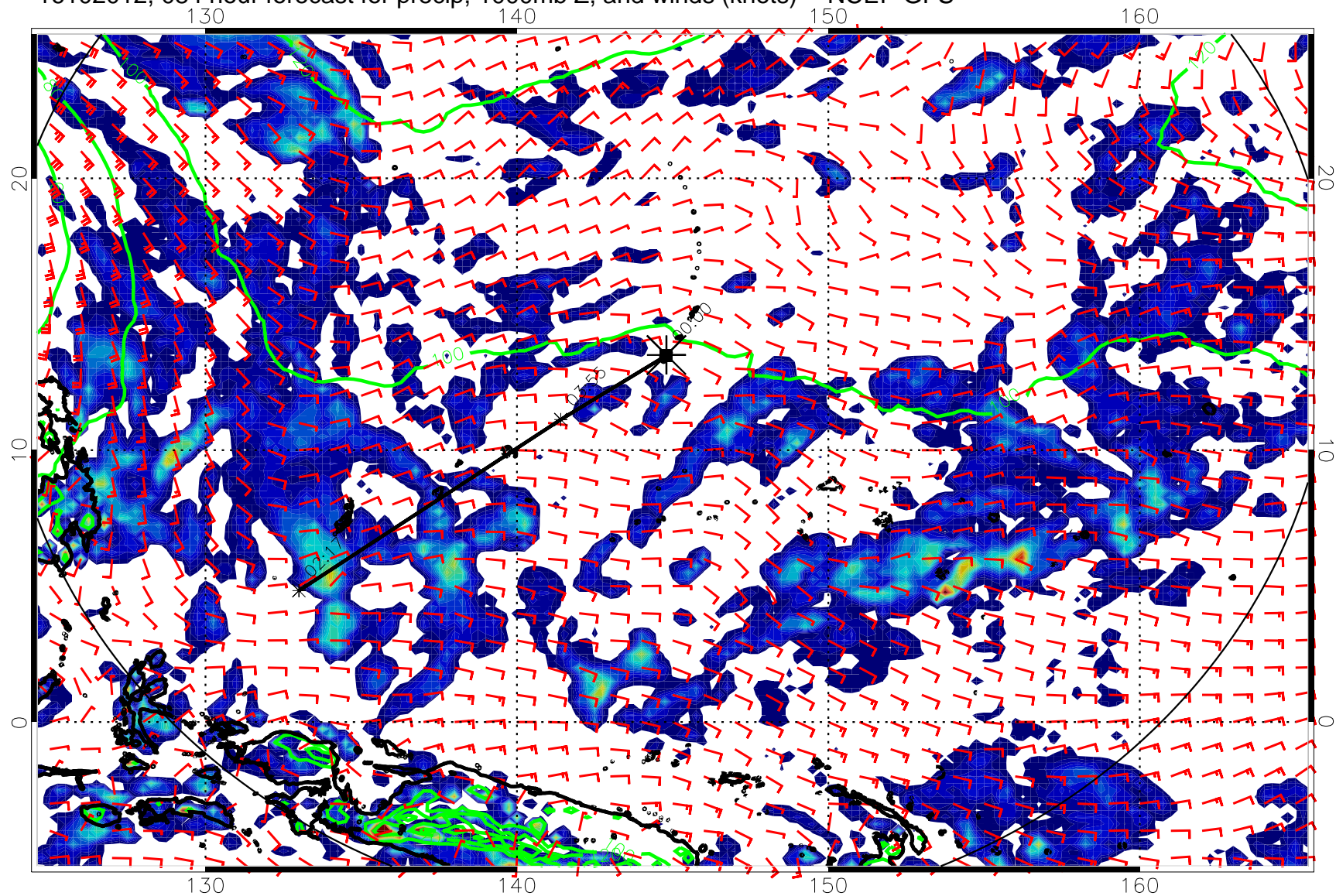
16102012, 084 hour forecast for precip, 1000mb Z, and winds (knots) -- NCEP GFS
