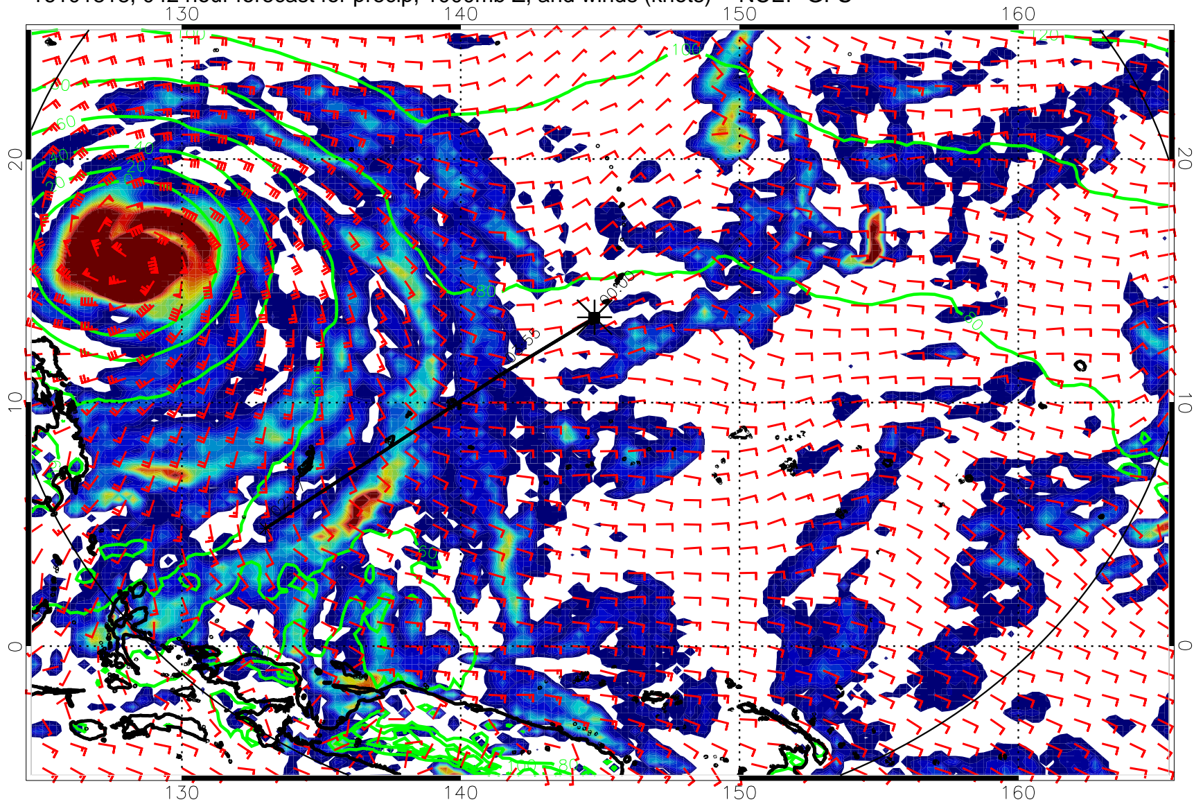
16101818, 042 hour forecast for precip, 1000mb Z, and winds (knots) -- NCEP GFS
