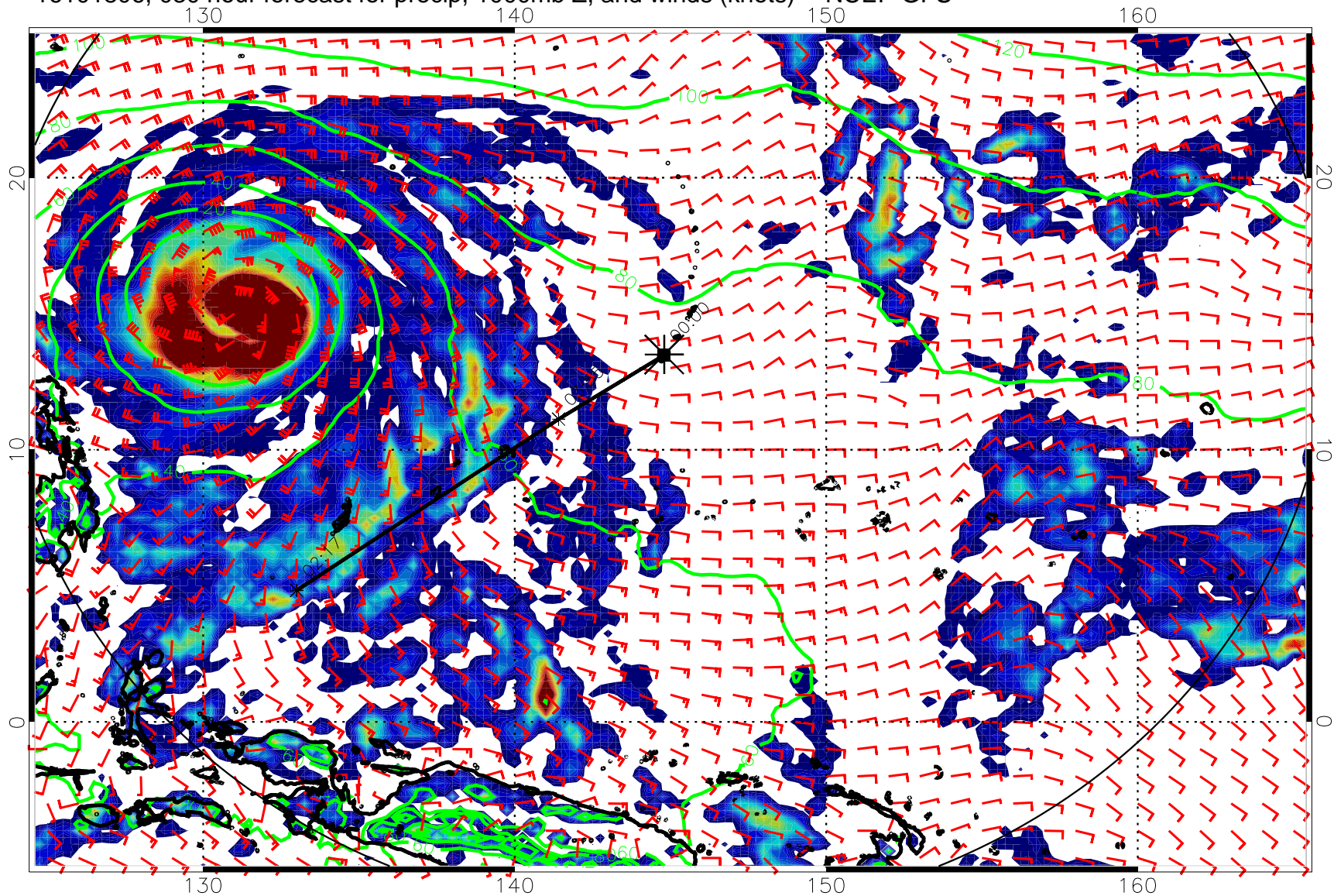
16101806, 030 hour forecast for precip, 1000mb Z, and winds (knots) -- NCEP GFS
