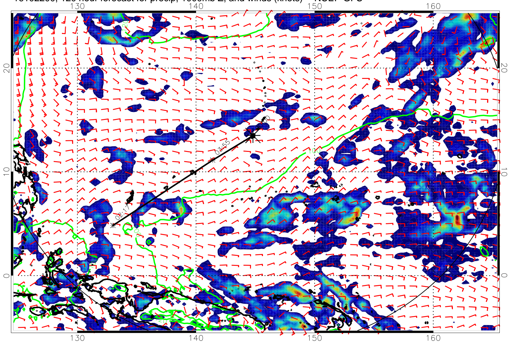
16102200, 120 hour forecast for precip, 1000mb Z, and winds (knots) -- NCEP GFS
