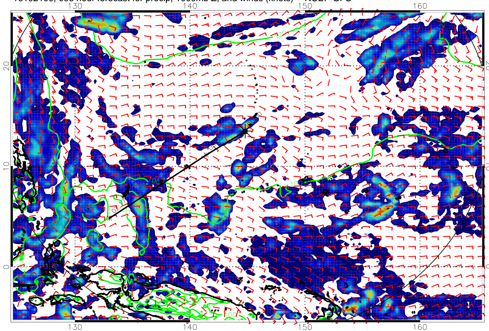
16102100, 096 hour forecast for precip, 1000mb Z, and winds (knots) -- NCEP GFS
