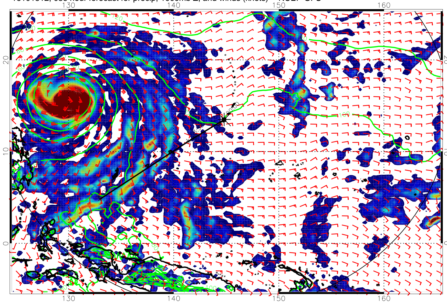
16101812, 036 hour forecast for precip, 1000mb Z, and winds (knots) -- NCEP GFS
