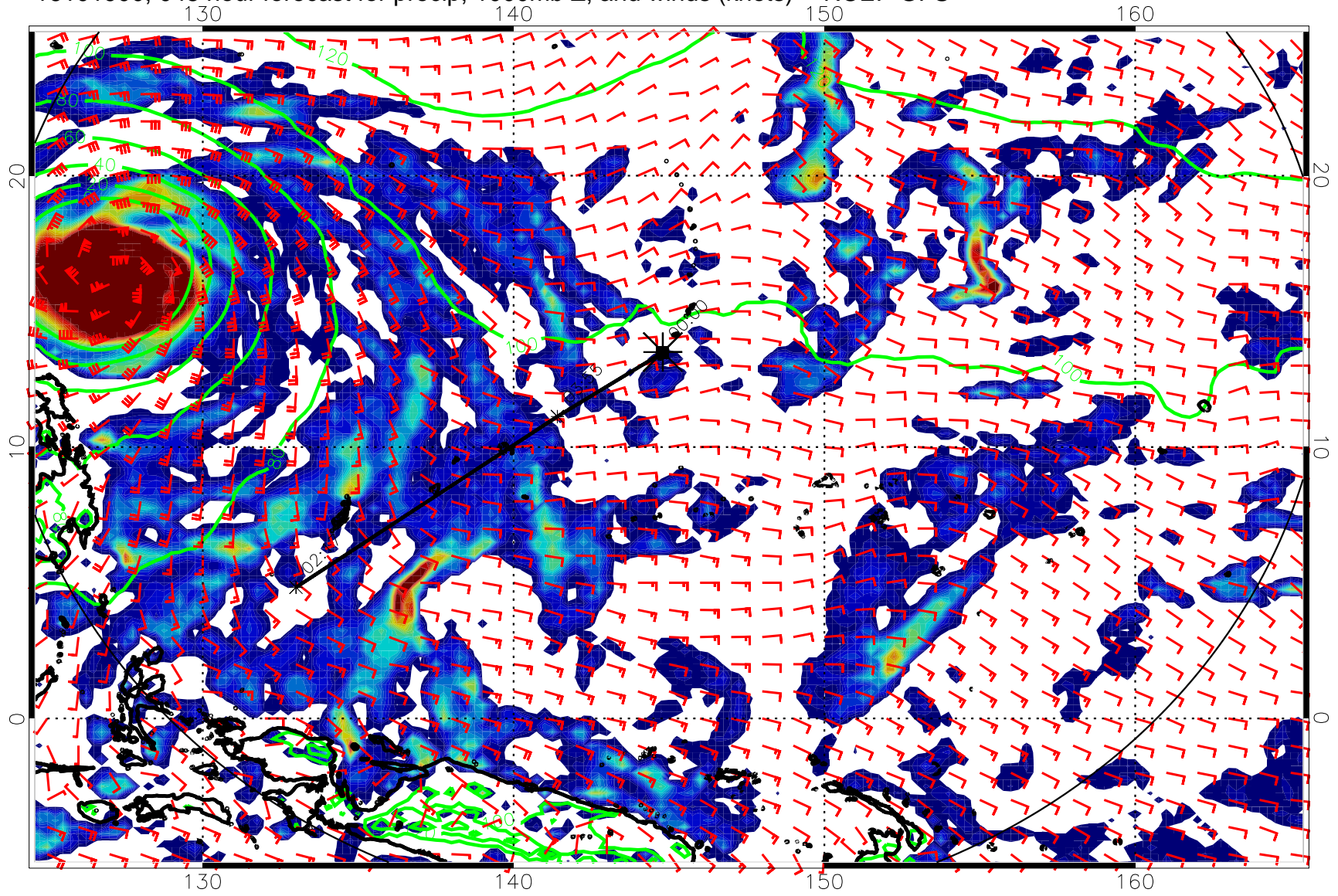
16101900, 048 hour forecast for precip, 1000mb Z, and winds (knots) -- NCEP GFS
