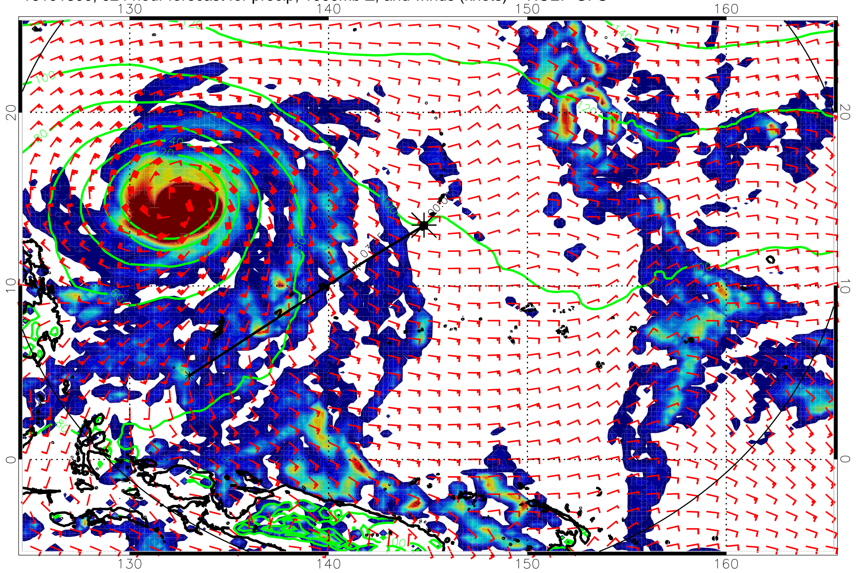
16101800, 024 hour forecast for precip, 1000mb Z, and winds (knots) -- NCEP GFS
