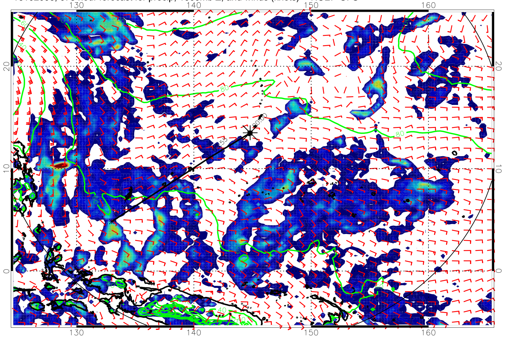
16102006, 078 hour forecast for precip, 1000mb Z, and winds (knots) -- NCEP GFS
