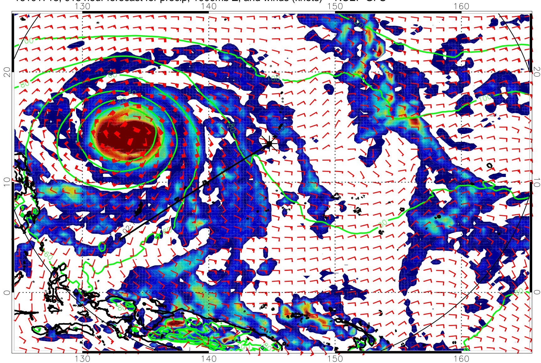
16101718, 018 hour forecast for precip, 1000mb Z, and winds (knots) -- NCEP GFS
