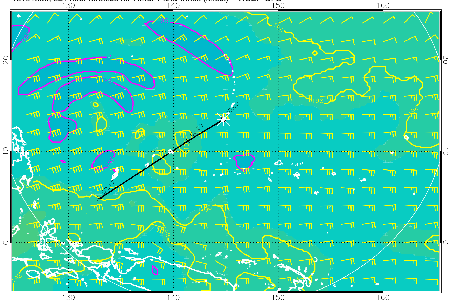
16101800, 024 hour forecast for 70mb T and winds (knots) -- NCEP GFS
