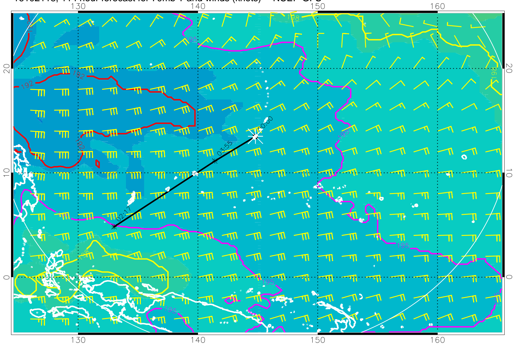
16102118, 114 hour forecast for 70mb T and winds (knots) -- NCEP GFS
