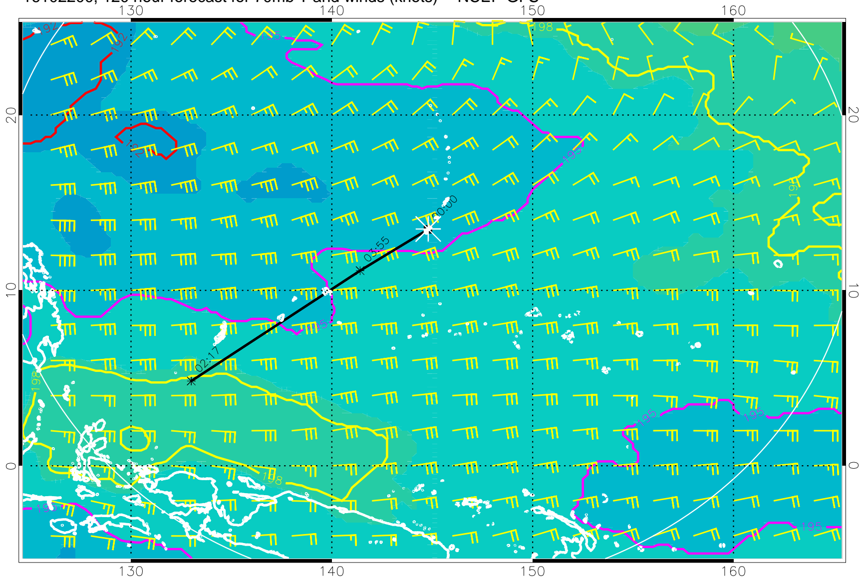
16102200, 120 hour forecast for 70mb T and winds (knots) -- NCEP GFS
