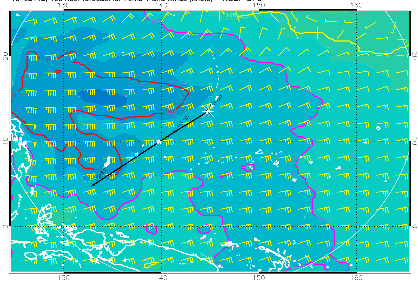
16102112, 108 hour forecast for 70mb T and winds (knots) -- NCEP GFS
