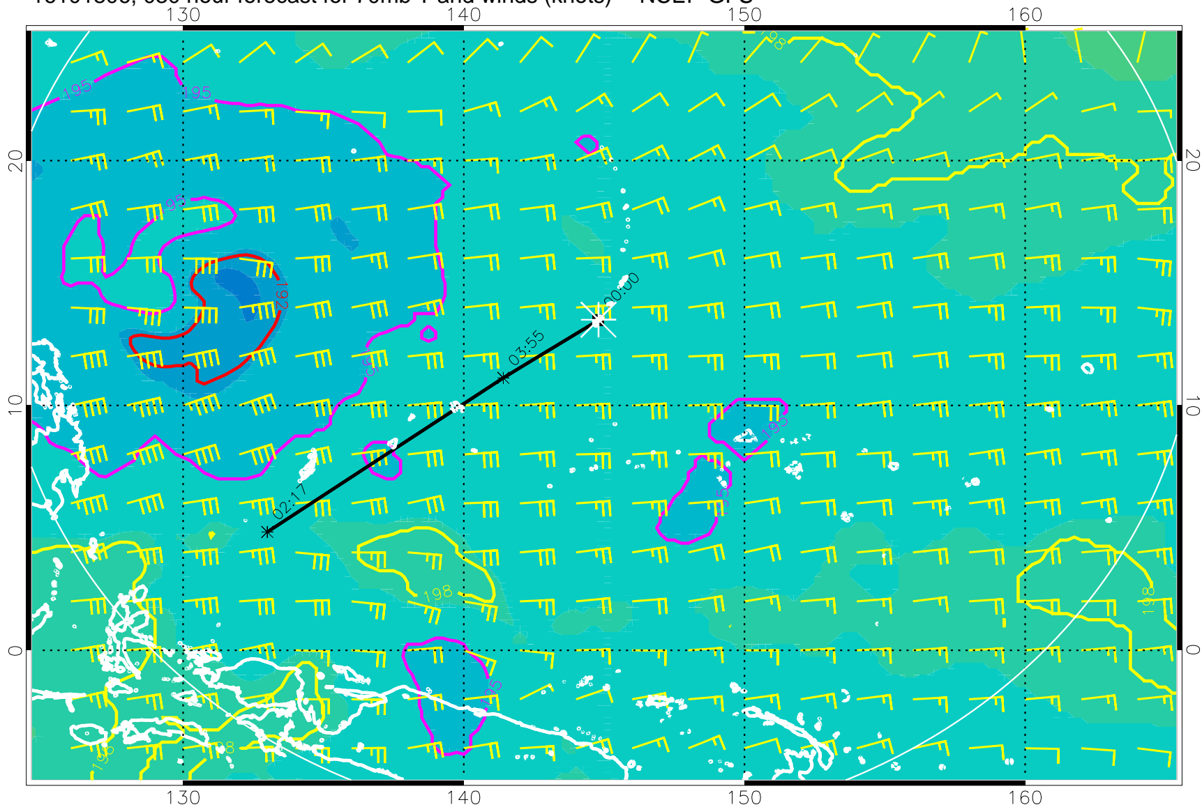
16101806, 030 hour forecast for 70mb T and winds (knots) -- NCEP GFS
