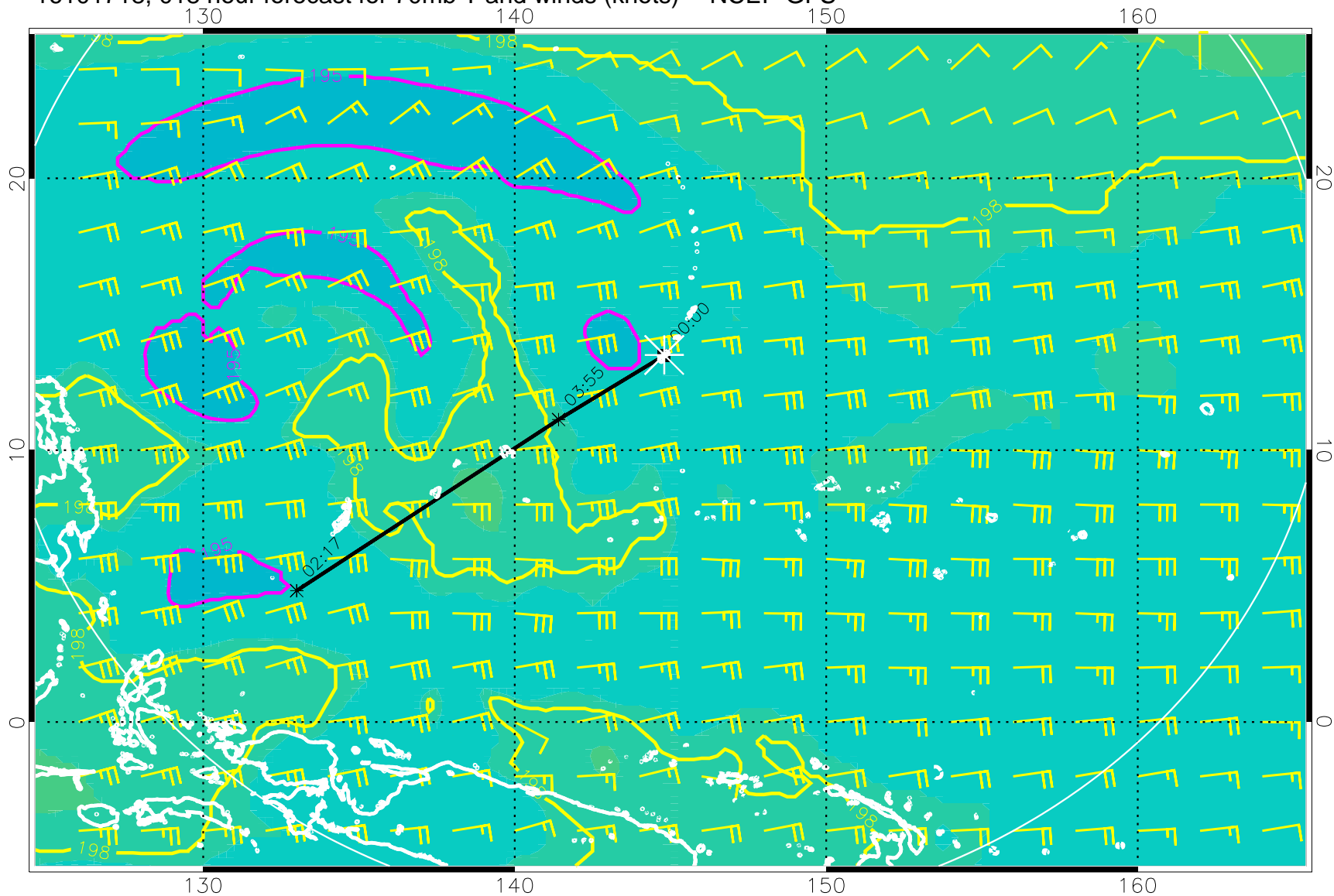
16101718, 018 hour forecast for 70mb T and winds (knots) -- NCEP GFS
