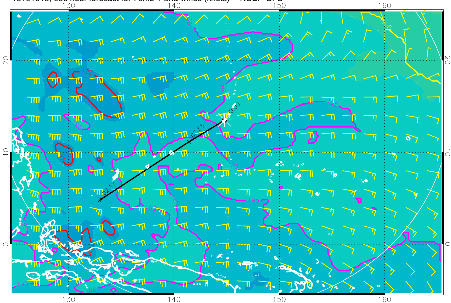
16101918, 066 hour forecast for 70mb T and winds (knots) -- NCEP GFS
