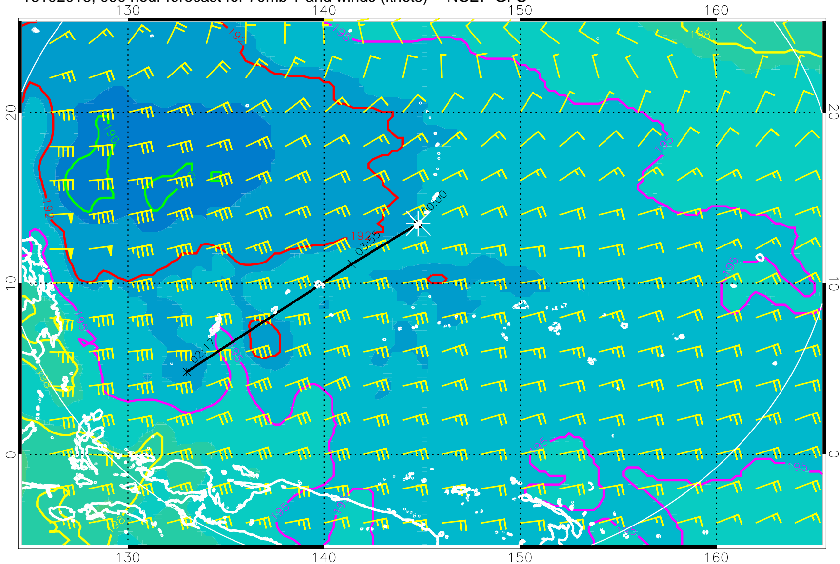
16102018, 090 hour forecast for 70mb T and winds (knots) -- NCEP GFS
