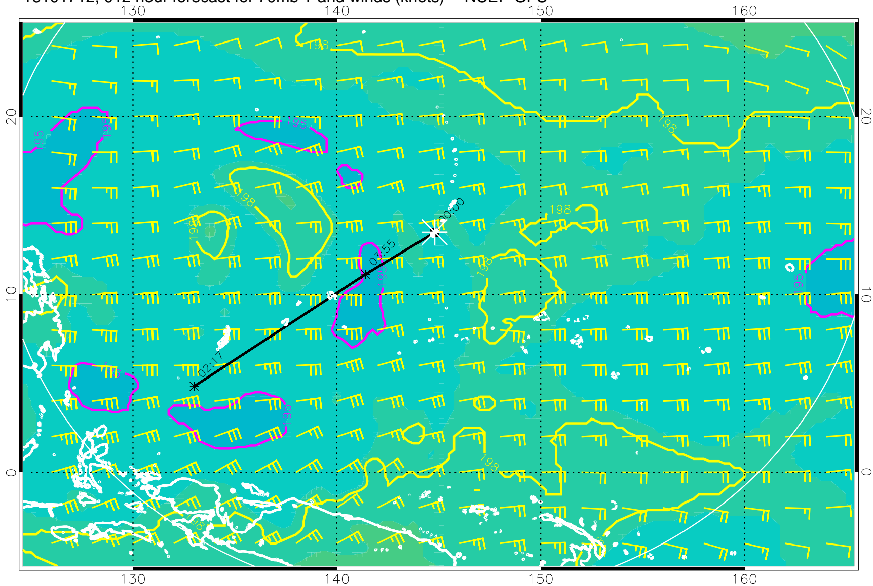
16101712, 012 hour forecast for 70mb T and winds (knots) -- NCEP GFS
