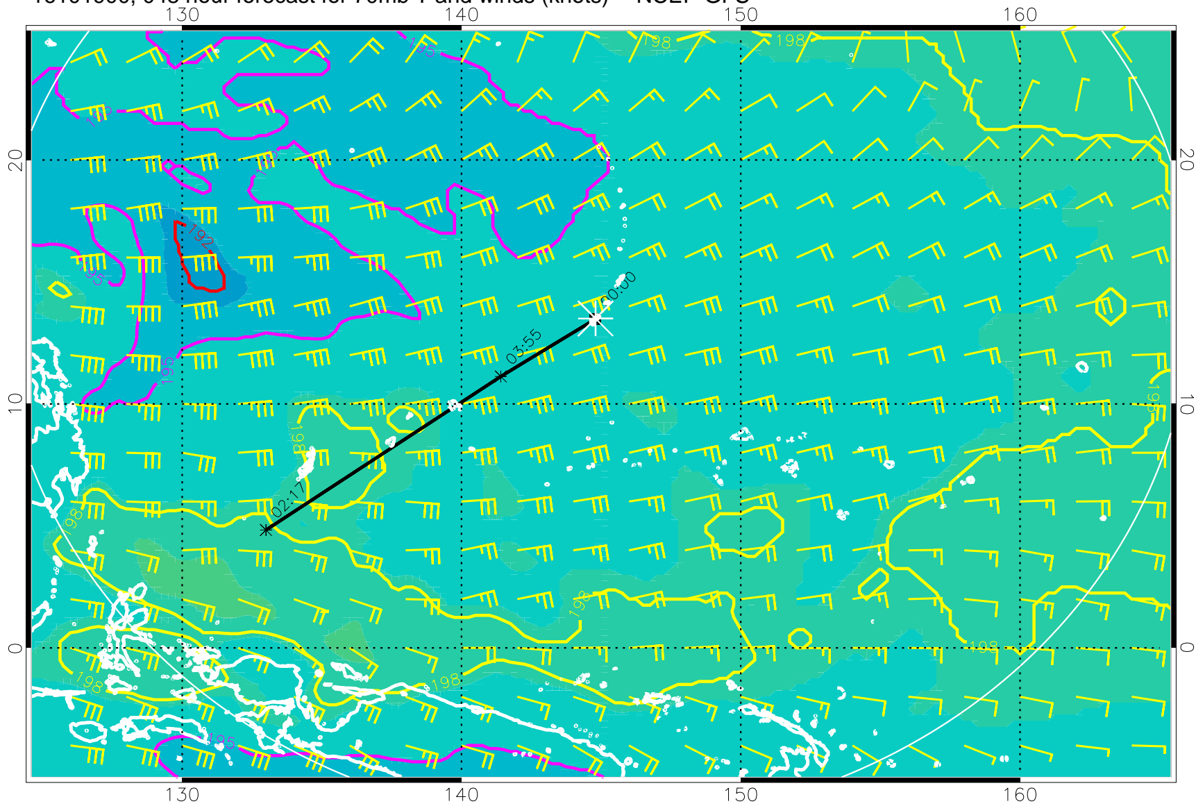
16101900, 048 hour forecast for 70mb T and winds (knots) -- NCEP GFS
