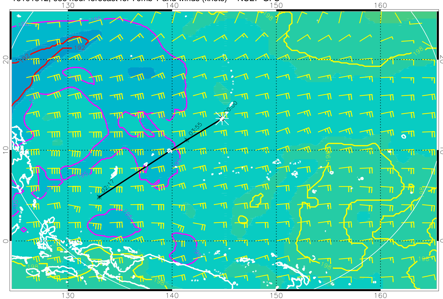
16101812, 036 hour forecast for 70mb T and winds (knots) -- NCEP GFS
