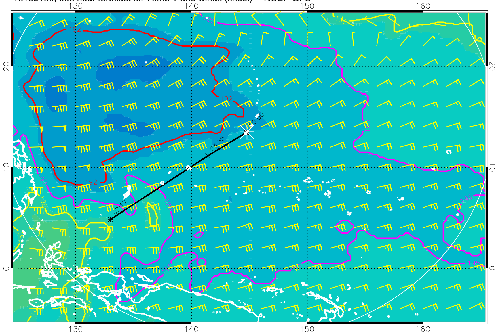
16102100, 096 hour forecast for 70mb T and winds (knots) -- NCEP GFS
