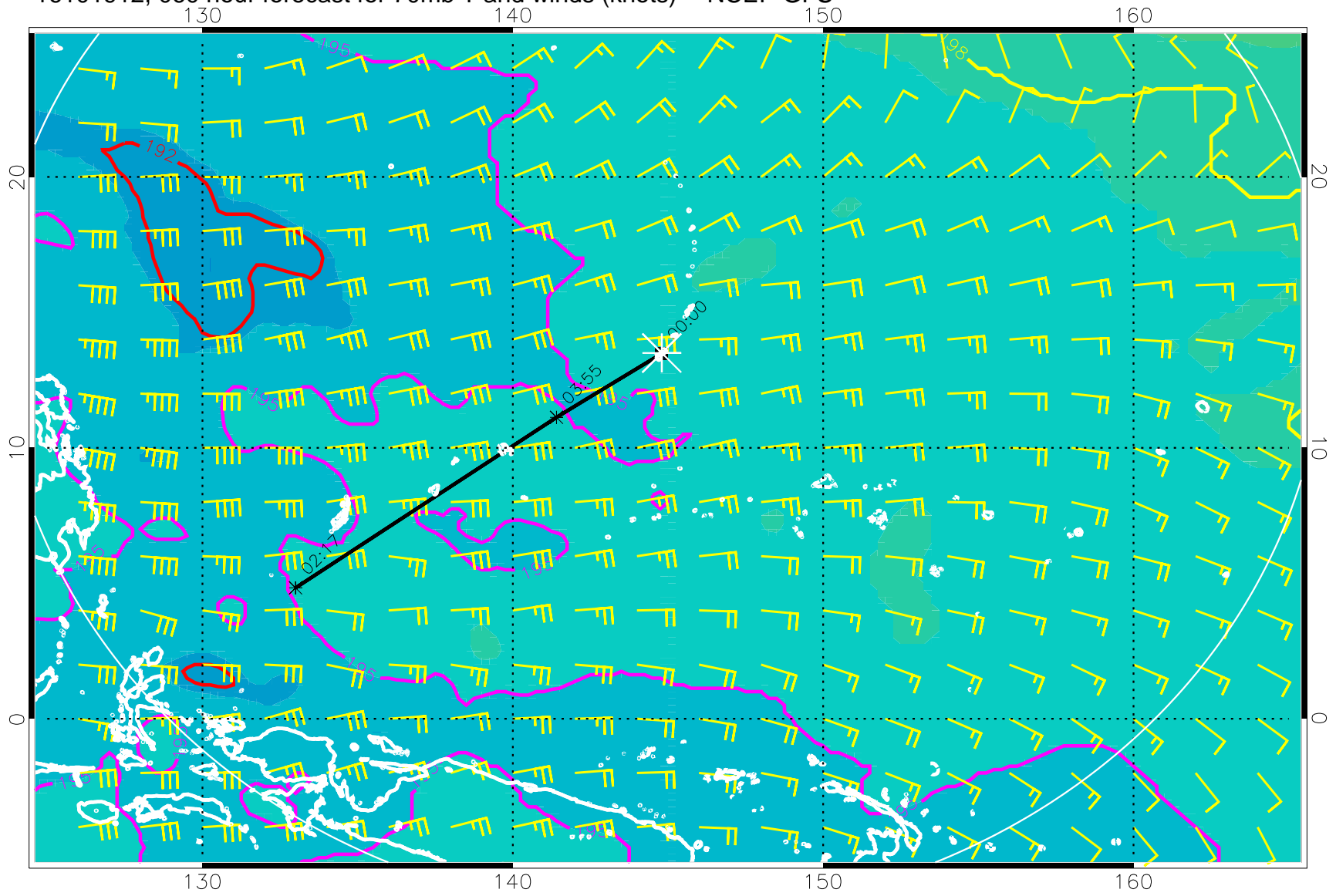
16101912, 060 hour forecast for 70mb T and winds (knots) -- NCEP GFS
