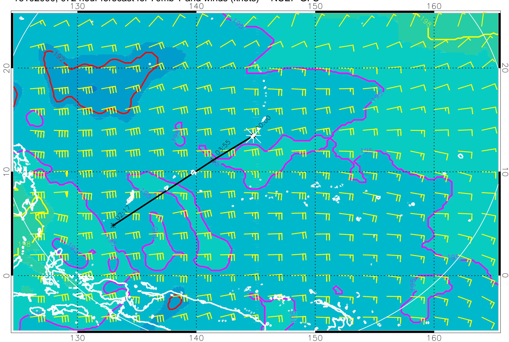
16102000, 072 hour forecast for 70mb T and winds (knots) -- NCEP GFS
