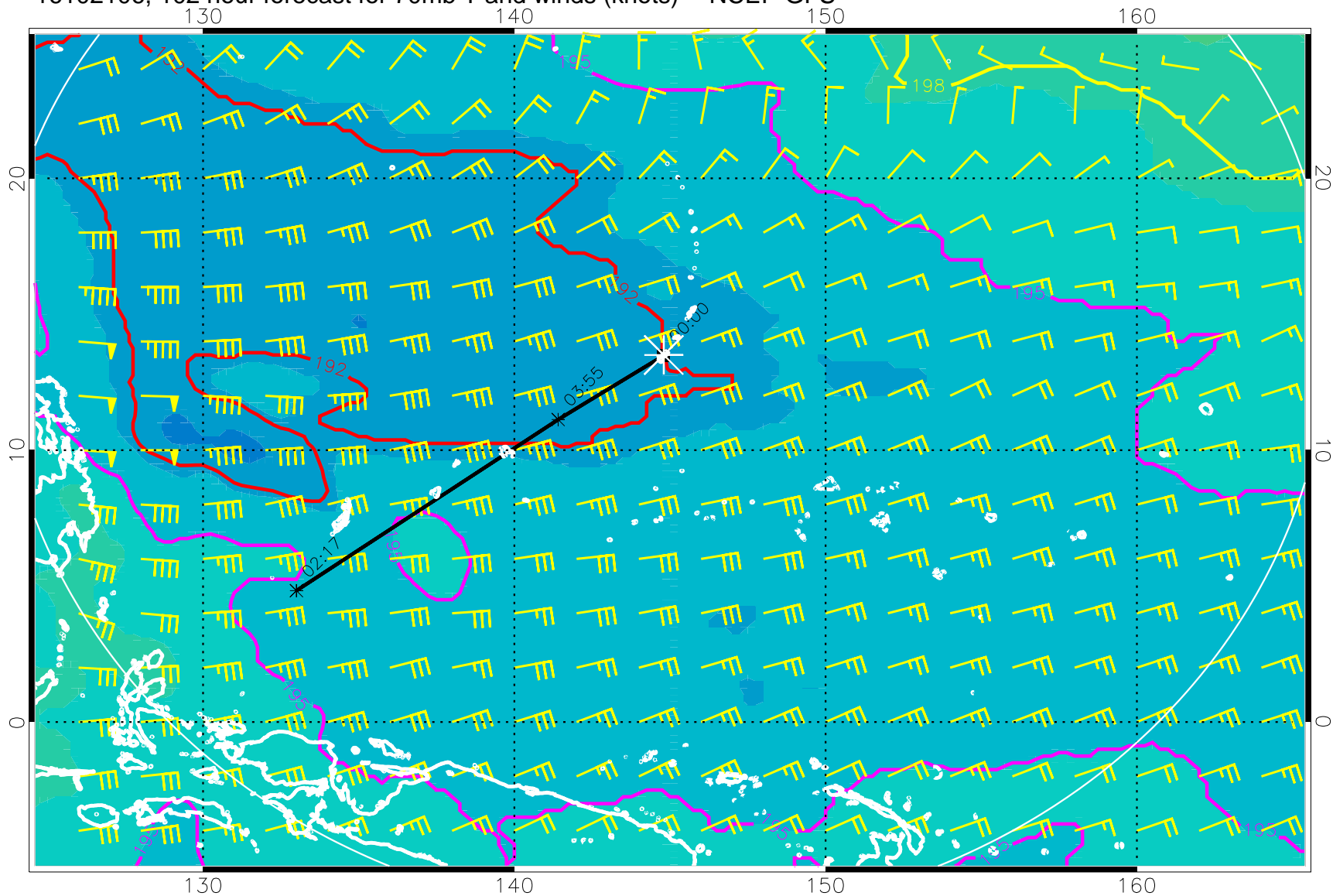
16102106, 102 hour forecast for 70mb T and winds (knots) -- NCEP GFS
