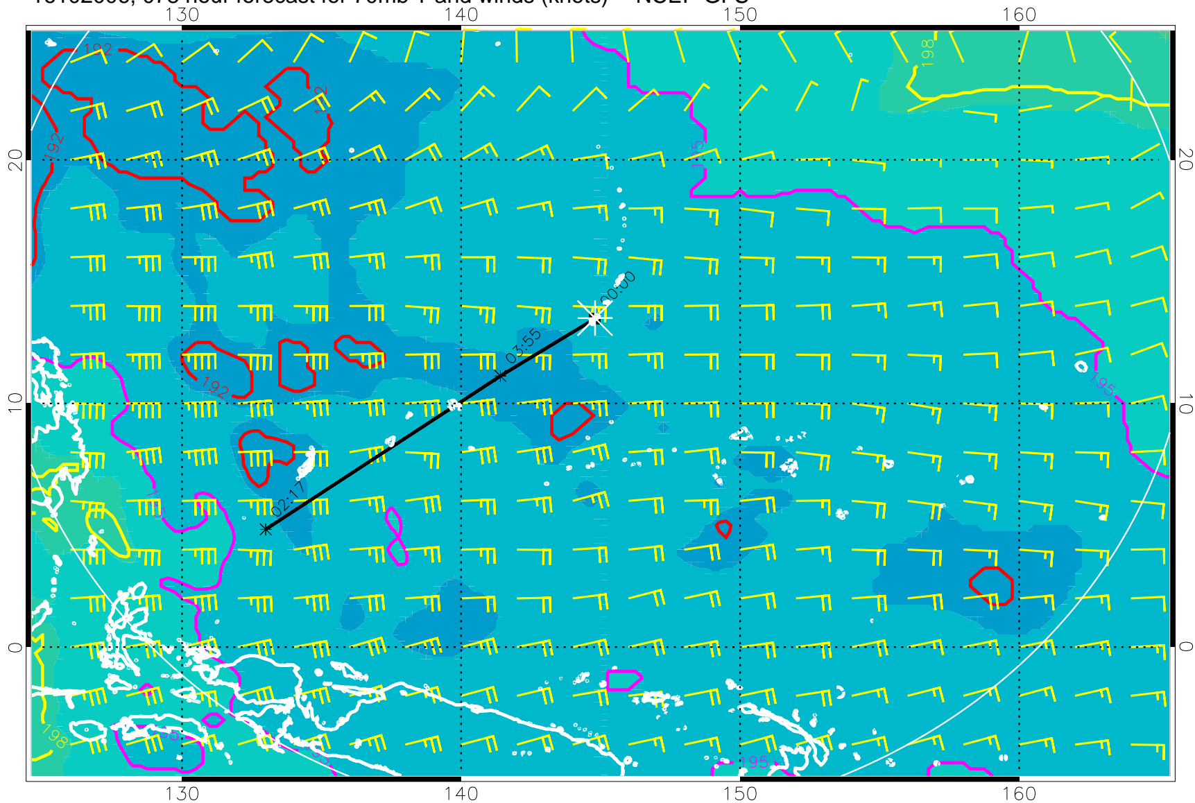
16102006, 078 hour forecast for 70mb T and winds (knots) -- NCEP GFS
