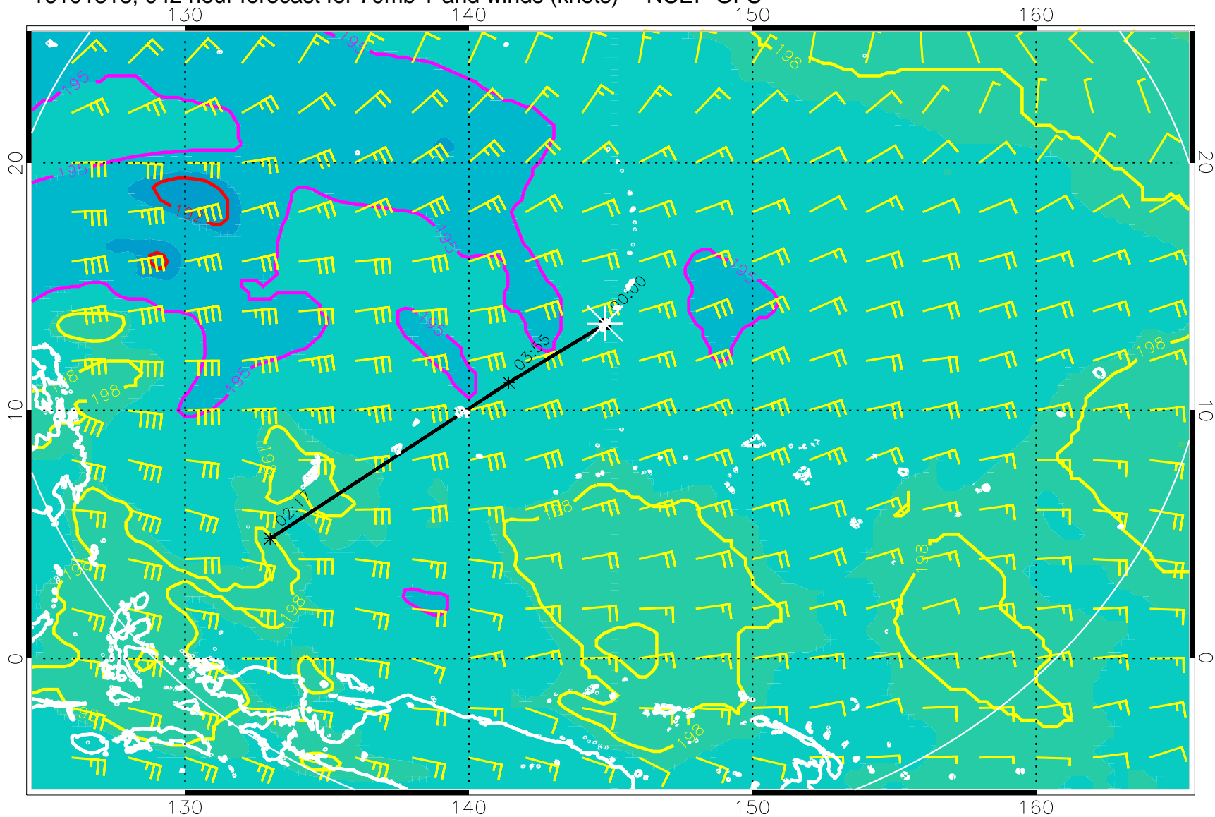
16101818, 042 hour forecast for 70mb T and winds (knots) -- NCEP GFS
