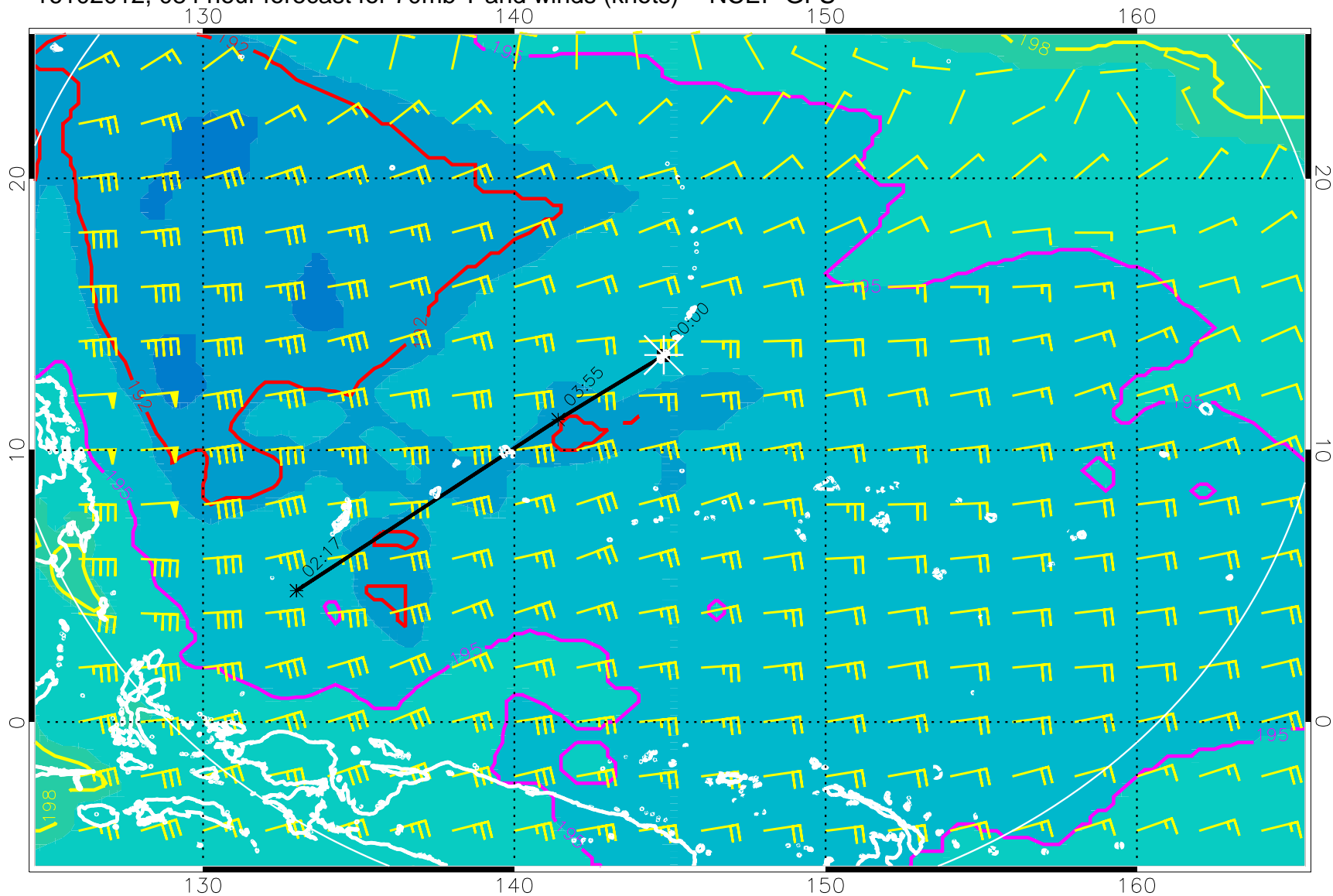
16102012, 084 hour forecast for 70mb T and winds (knots) -- NCEP GFS
