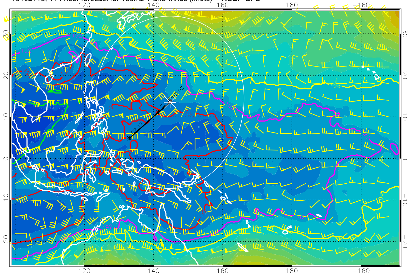
16102118, 114 hour forecast for 100mb T and winds (knots) -- NCEP GFS
