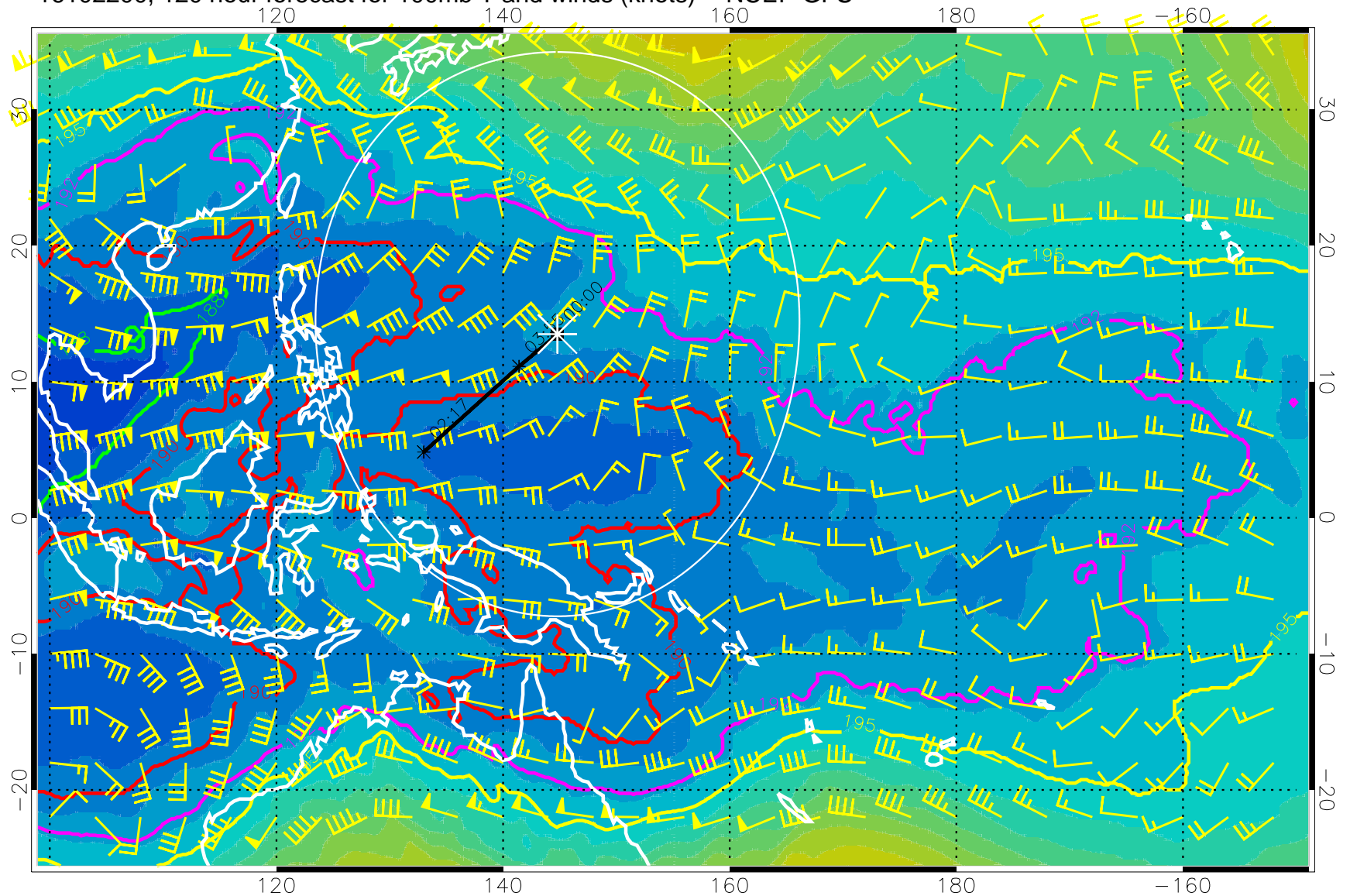
16102200, 120 hour forecast for 100mb T and winds (knots) -- NCEP GFS
