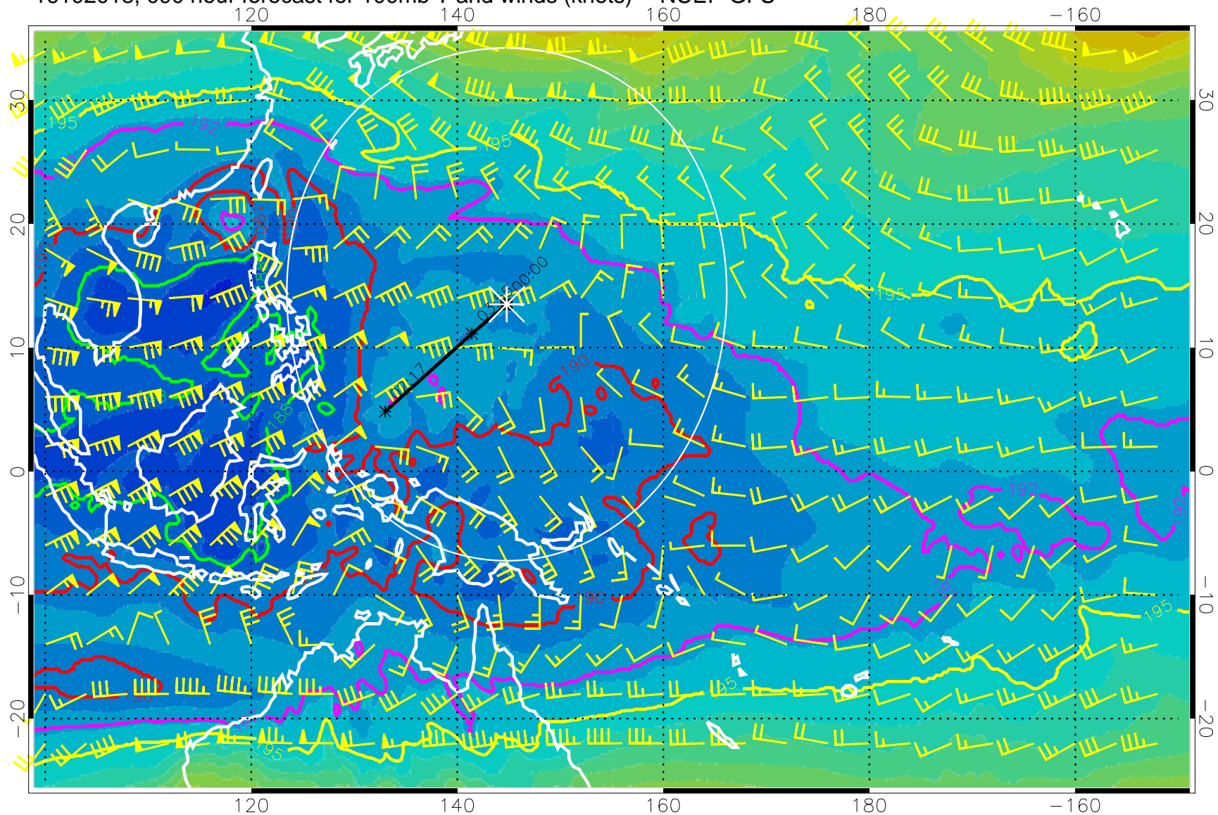
16102018, 090 hour forecast for 100mb T and winds (knots) -- NCEP GFS
