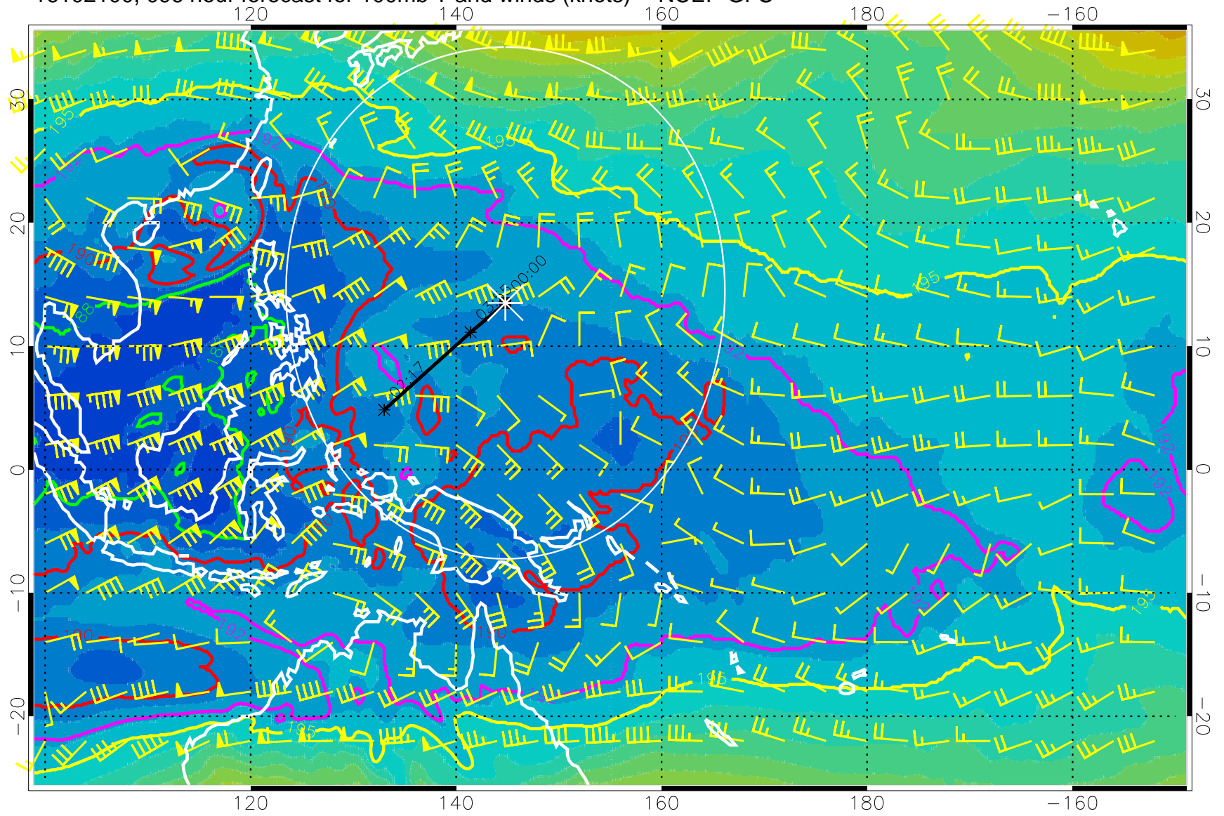
16102100, 096 hour forecast for 100mb T and winds (knots) -- NCEP GFS
