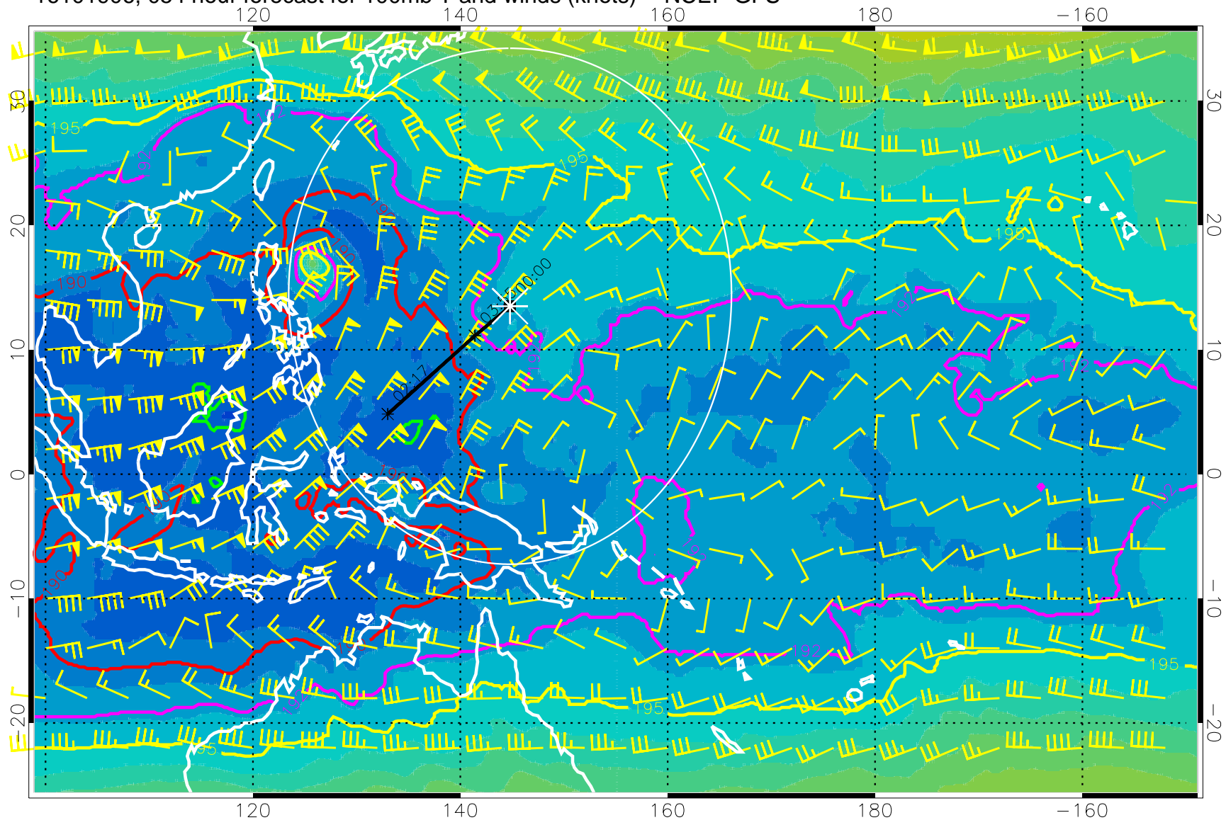
16101906, 054 hour forecast for 100mb T and winds (knots) -- NCEP GFS
