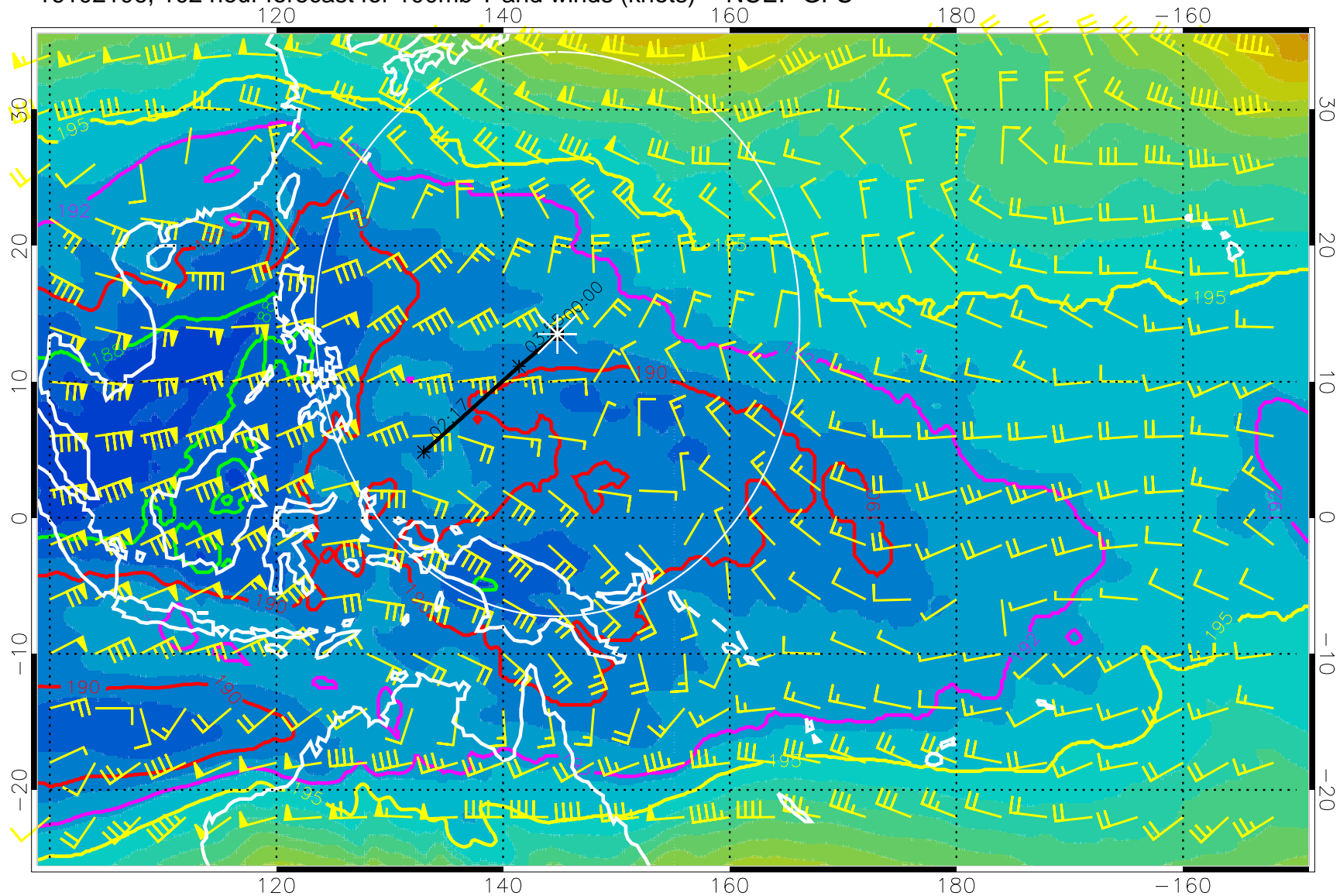
16102106, 102 hour forecast for 100mb T and winds (knots) -- NCEP GFS
