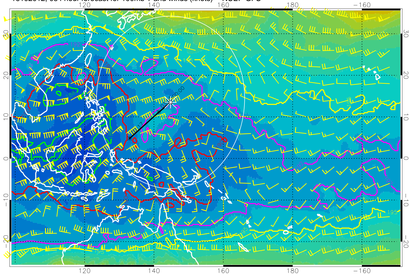
16102012, 084 hour forecast for 100mb T and winds (knots) -- NCEP GFS
