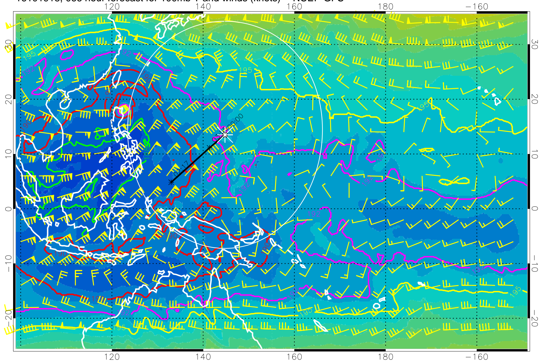
16101918, 066 hour forecast for 100mb T and winds (knots) -- NCEP GFS
