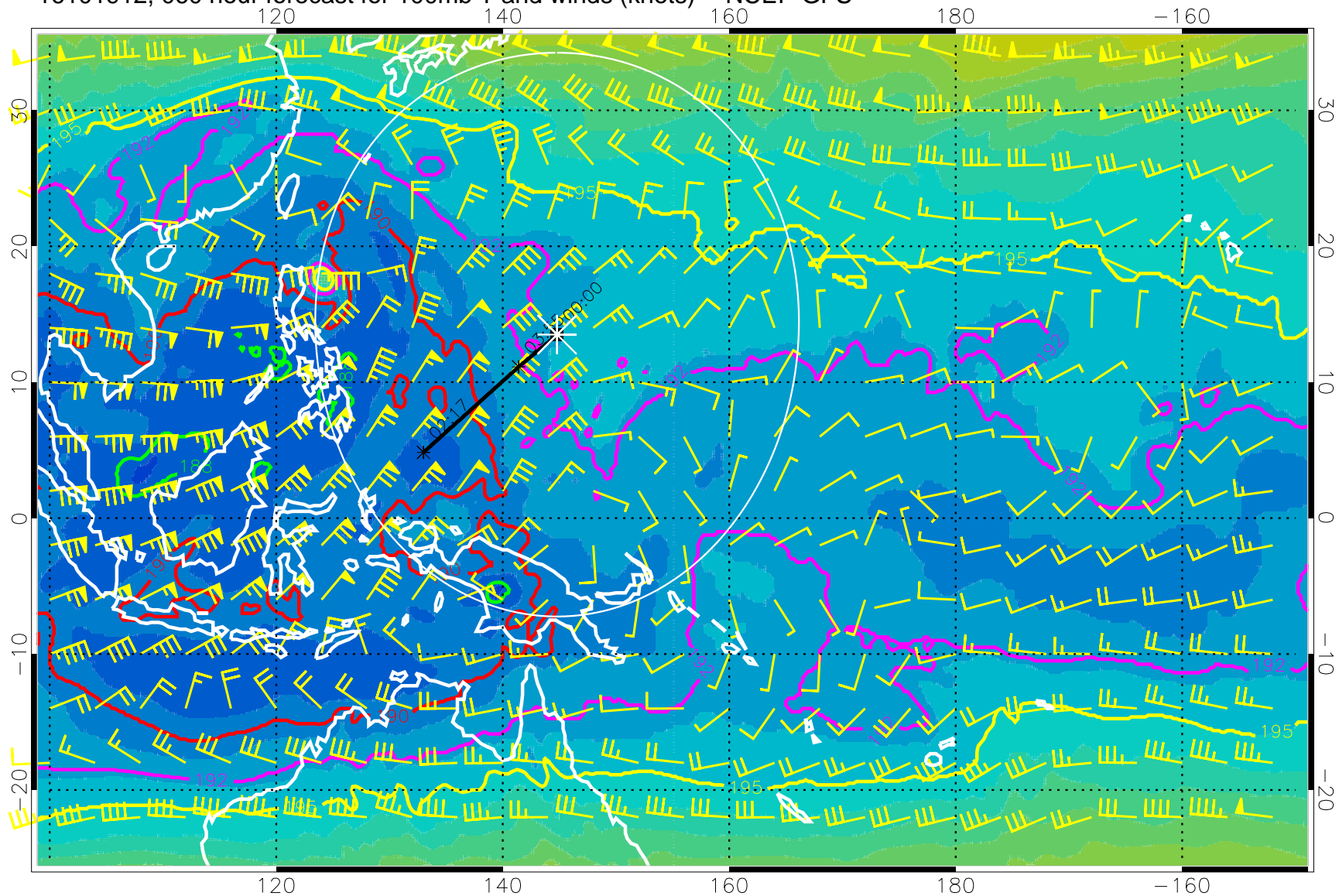
16101912, 060 hour forecast for 100mb T and winds (knots) -- NCEP GFS
