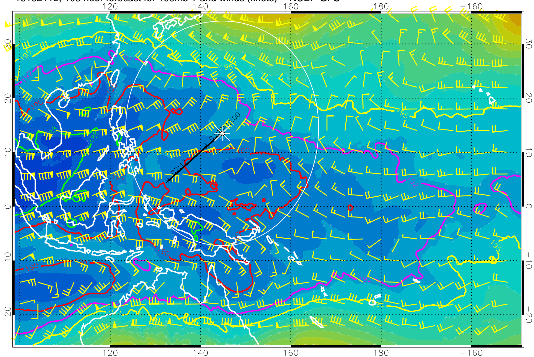
16102112, 108 hour forecast for 100mb T and winds (knots) -- NCEP GFS
