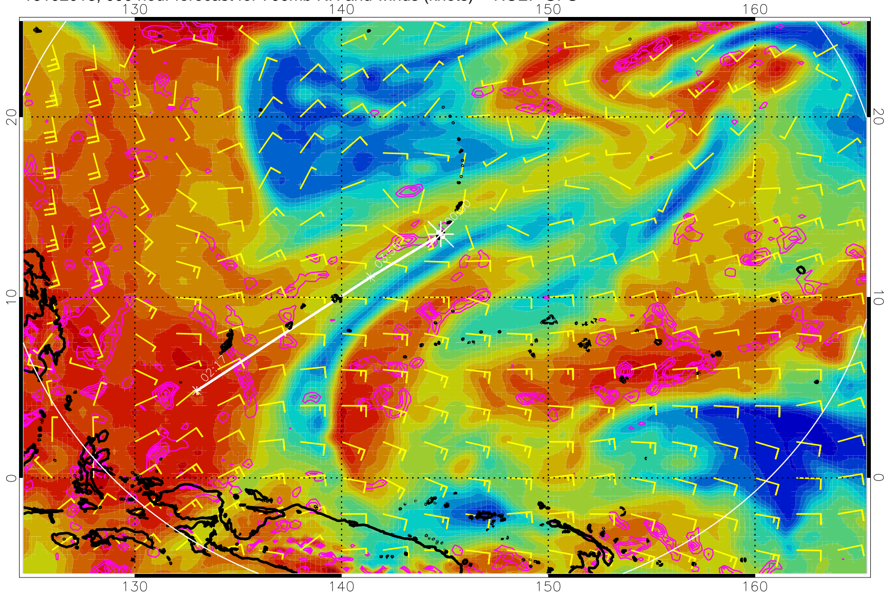
16102018, 090 hour forecast for 700mb RH and winds (knots) -- NCEP GFS
