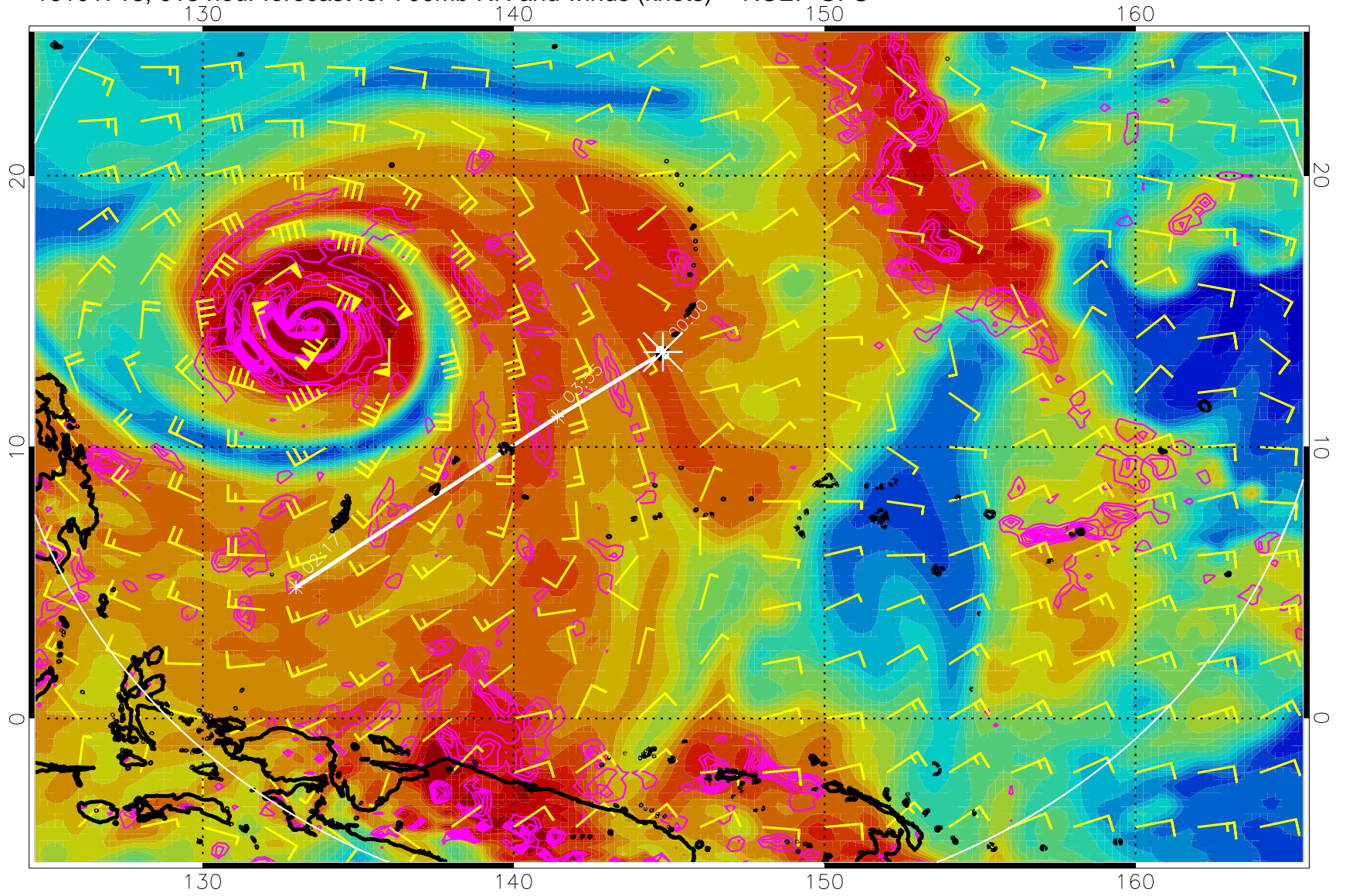
16101718, 018 hour forecast for 700mb RH and winds (knots) -- NCEP GFS
