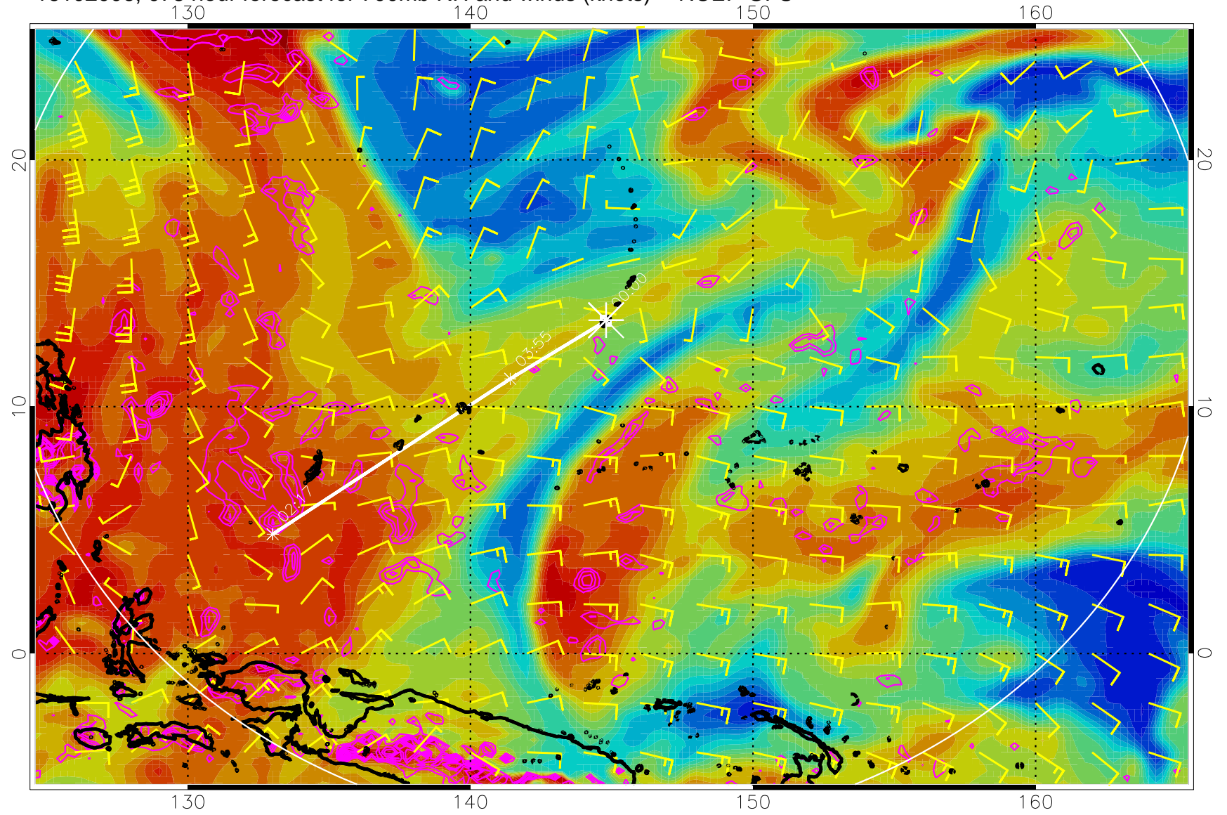
16102006, 078 hour forecast for 700mb RH and winds (knots) -- NCEP GFS
