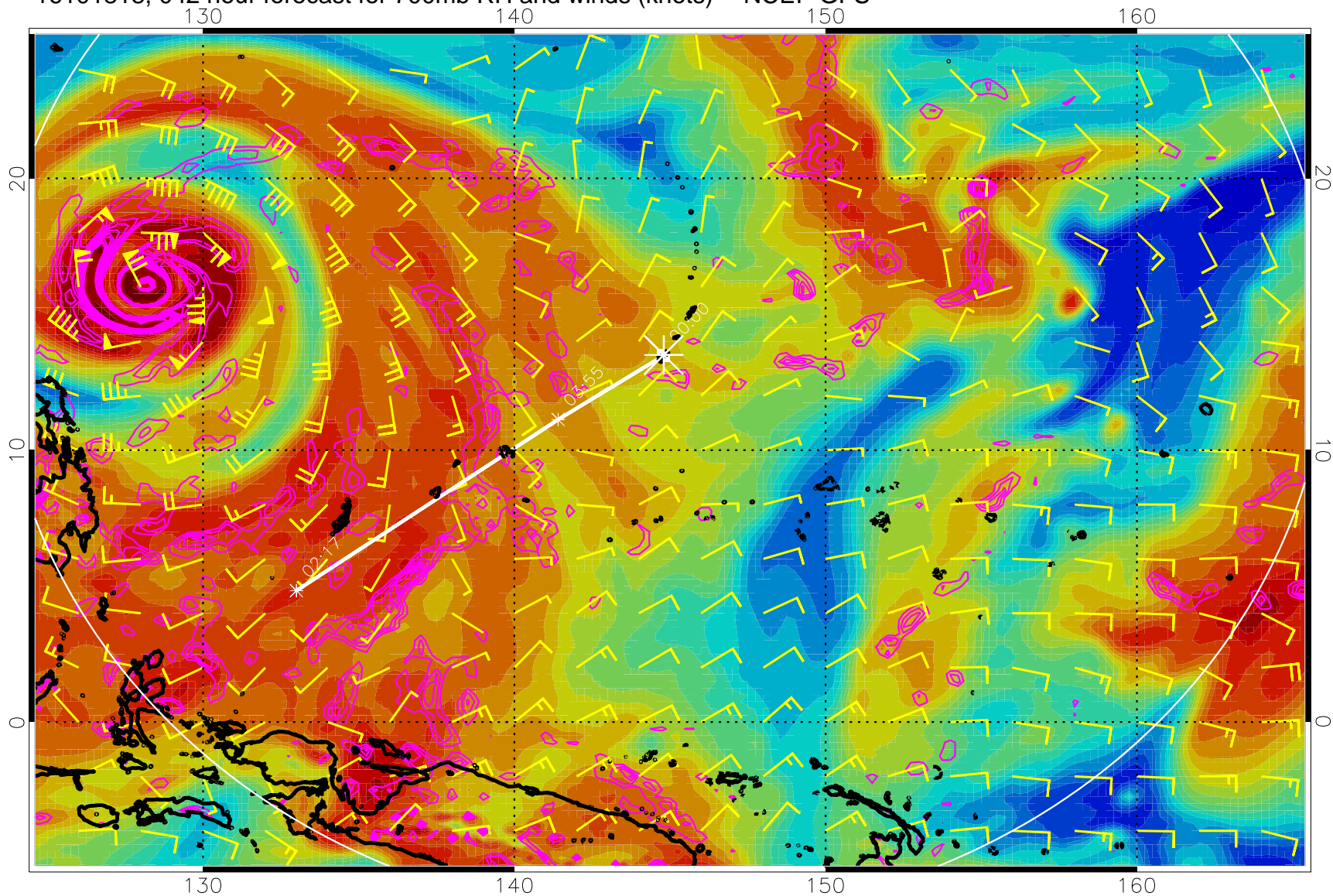
16101818, 042 hour forecast for 700mb RH and winds (knots) -- NCEP GFS
