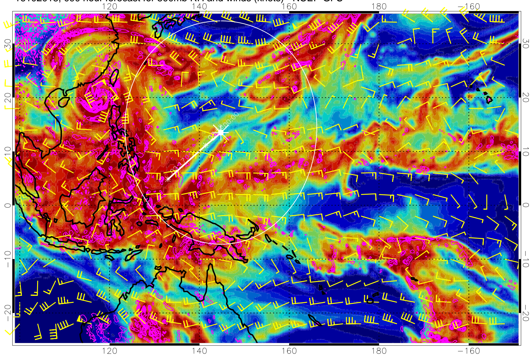
16102018, 090 hour forecast for 500mb RH and winds (knots) - NCEP GFS
