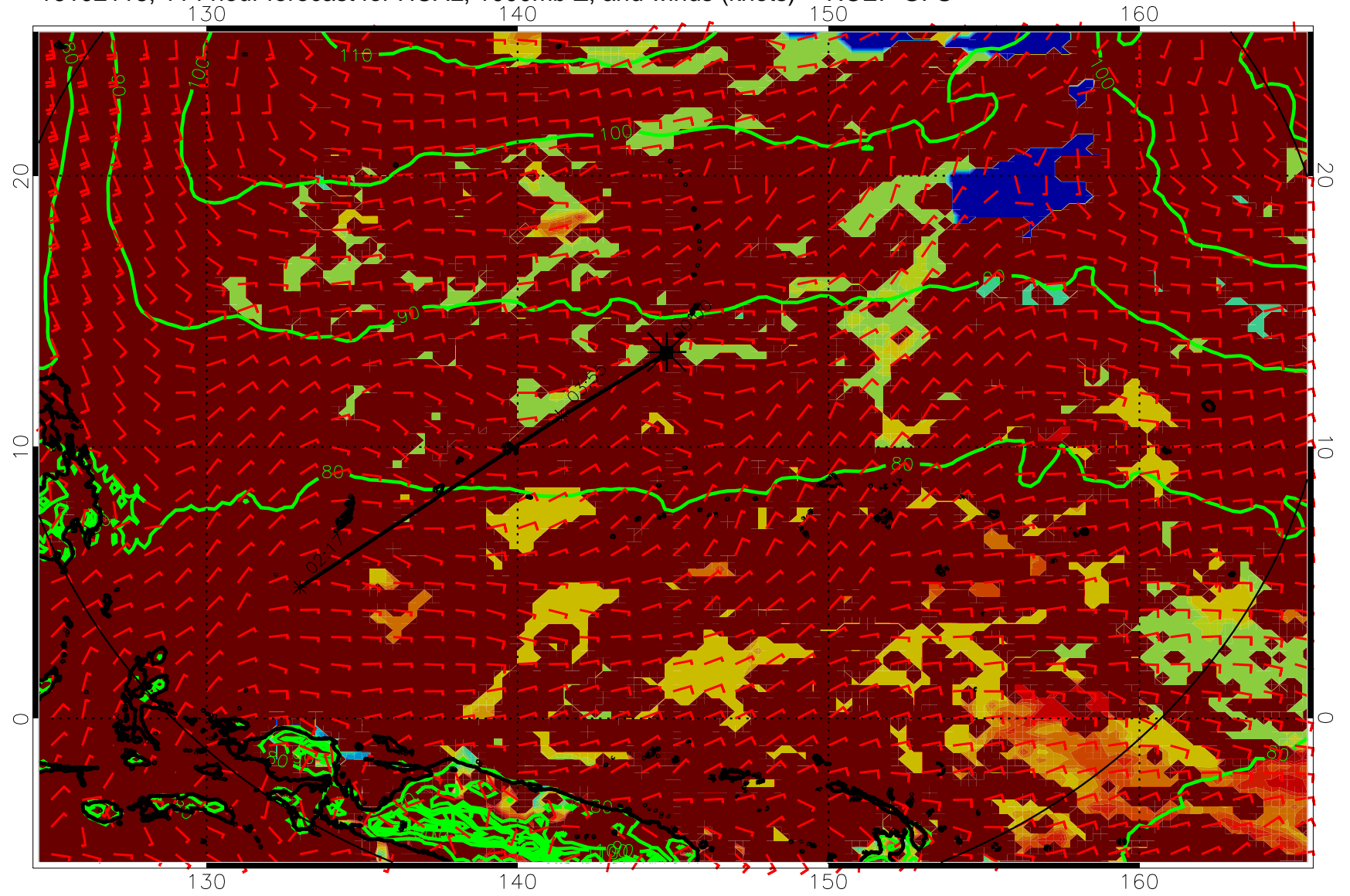
16102118, 114 hour forecast for HCAL, 1000mb Z, and winds (knots) -- NCEP GFS
