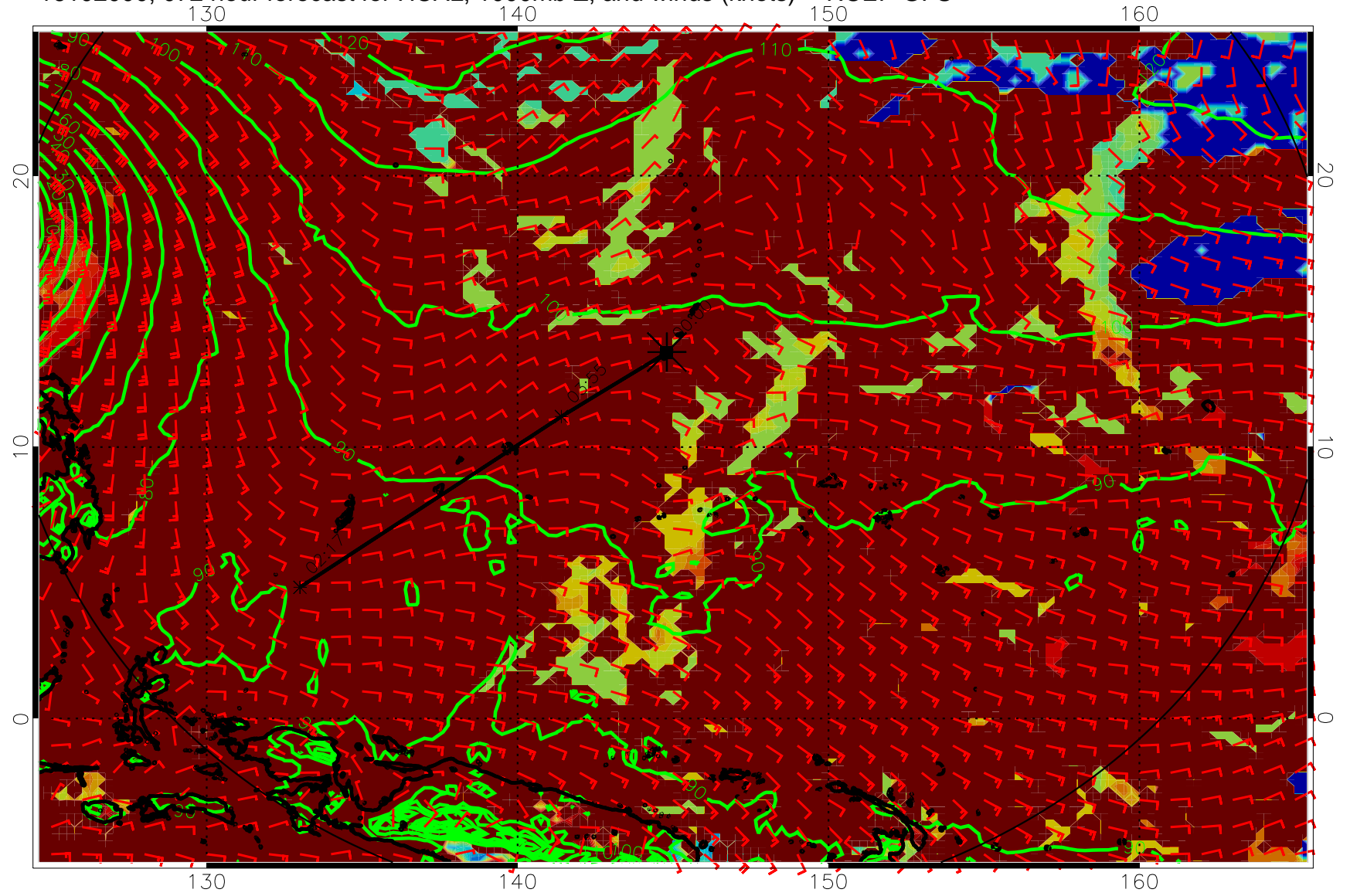
16102000, 072 hour forecast for HCAL, 1000mb Z, and winds (knots) -- NCEP GFS
