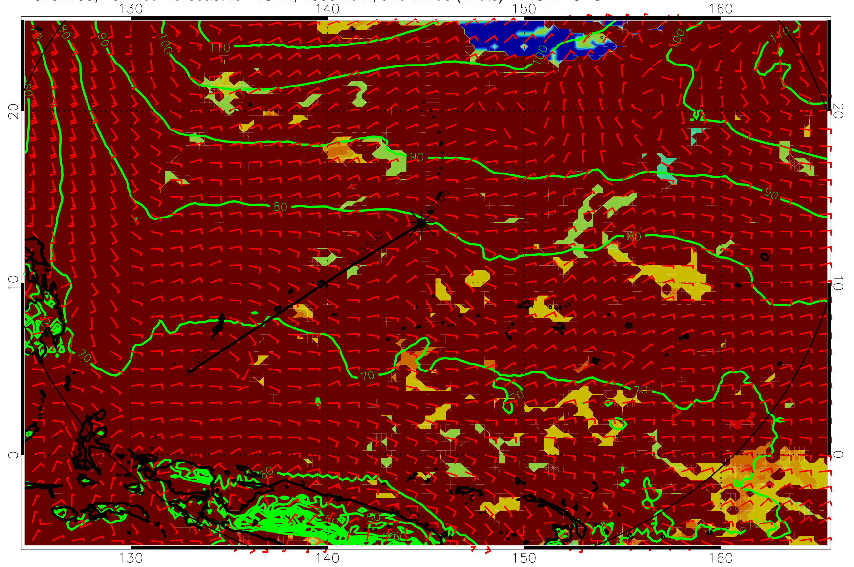
16102106, 102 hour forecast for HCAL, 1000mb Z, and winds (knots) -- NCEP GFS
