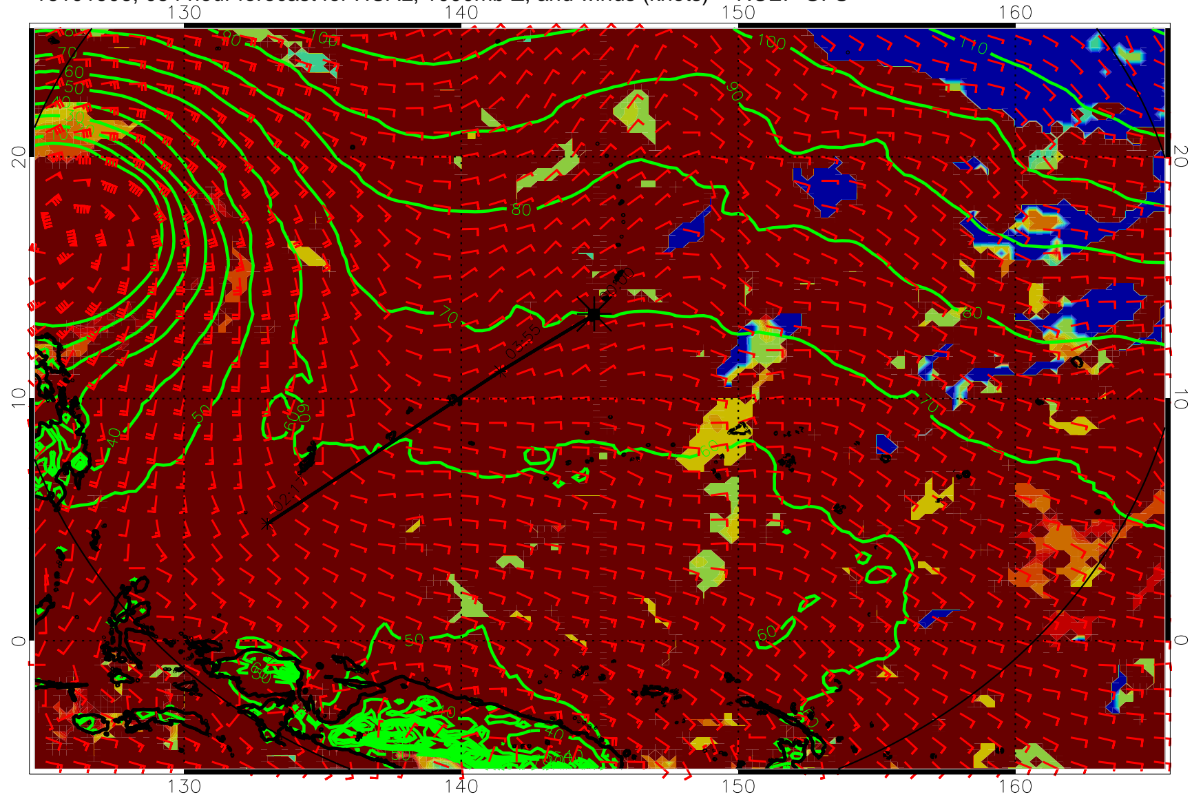
16101906, 054 hour forecast for HCAL, 1000mb Z, and winds (knots) -- NCEP GFS
