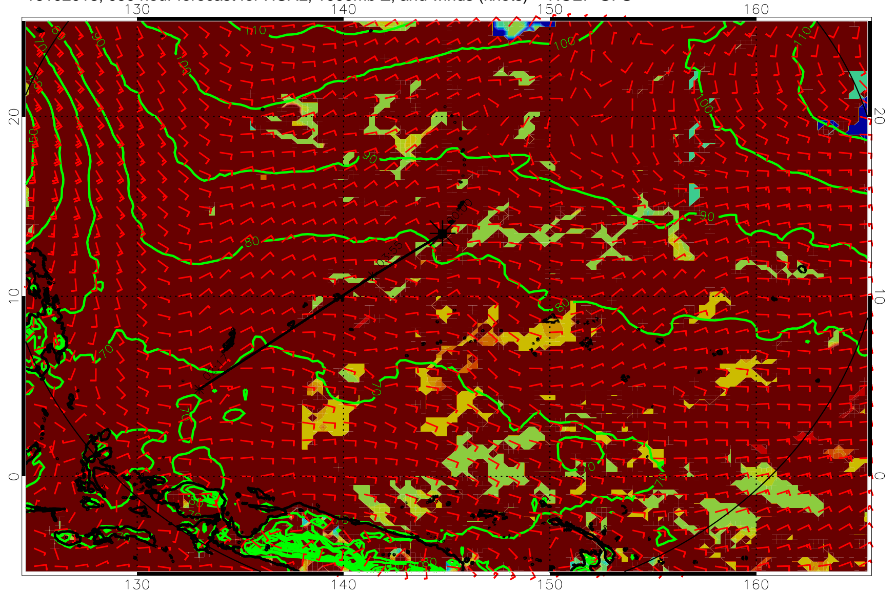
16102018, 090 hour forecast for HCAL, 1000mb Z, and winds (knots) -- NCEP GFS
