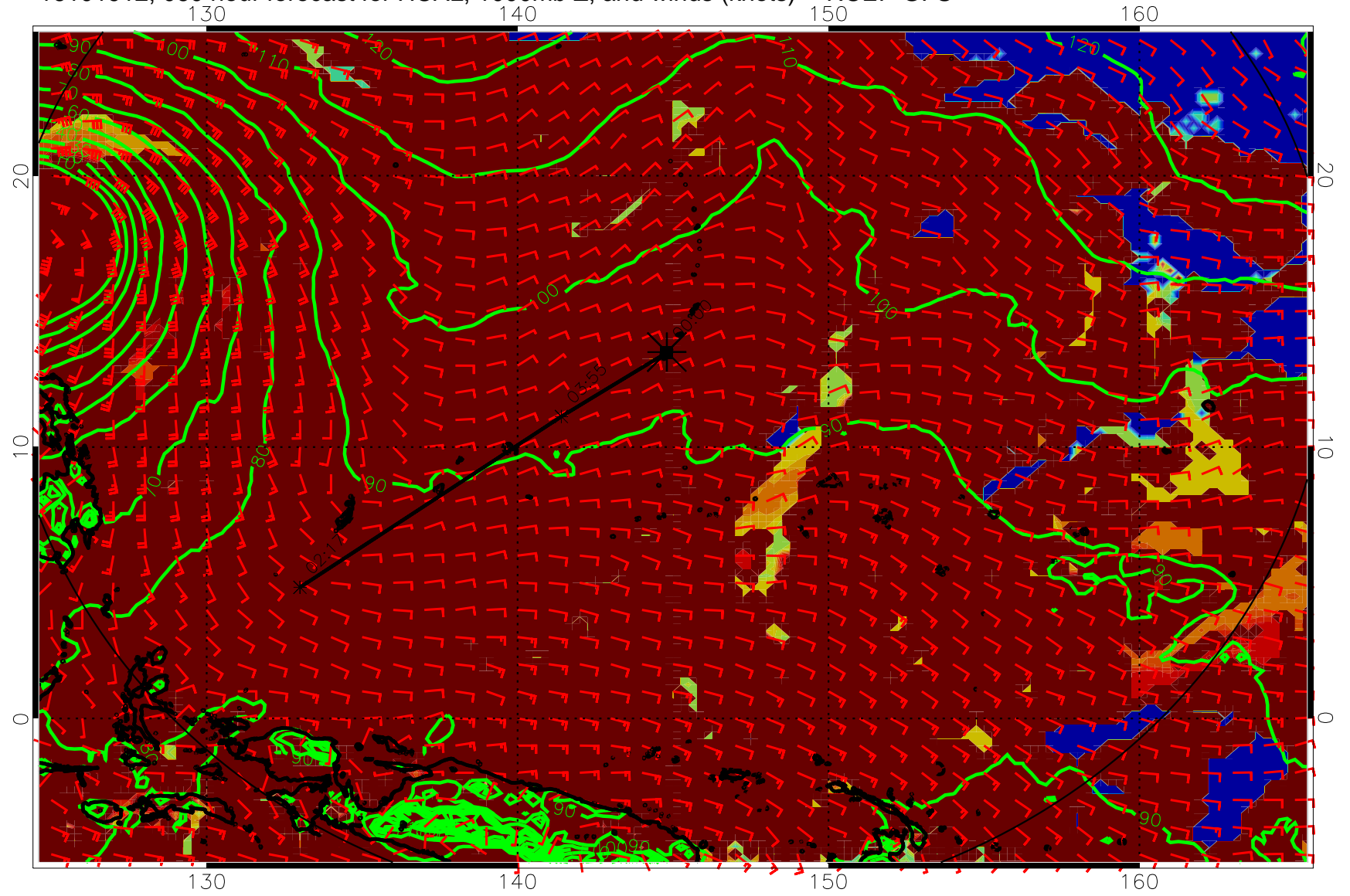
16101912, 060 hour forecast for HCAL, 1000mb Z, and winds (knots) -- NCEP GFS
