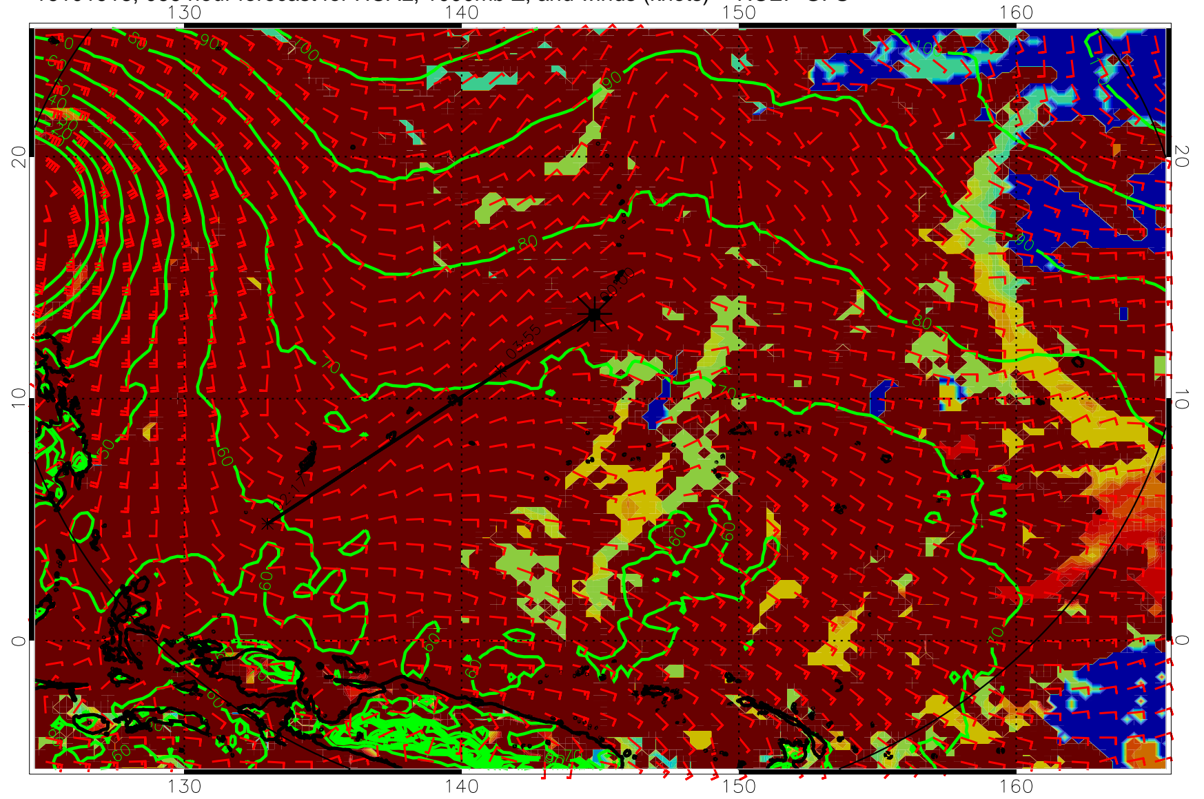
16101918, 066 hour forecast for HCAL, 1000mb Z, and winds (knots) -- NCEP GFS
