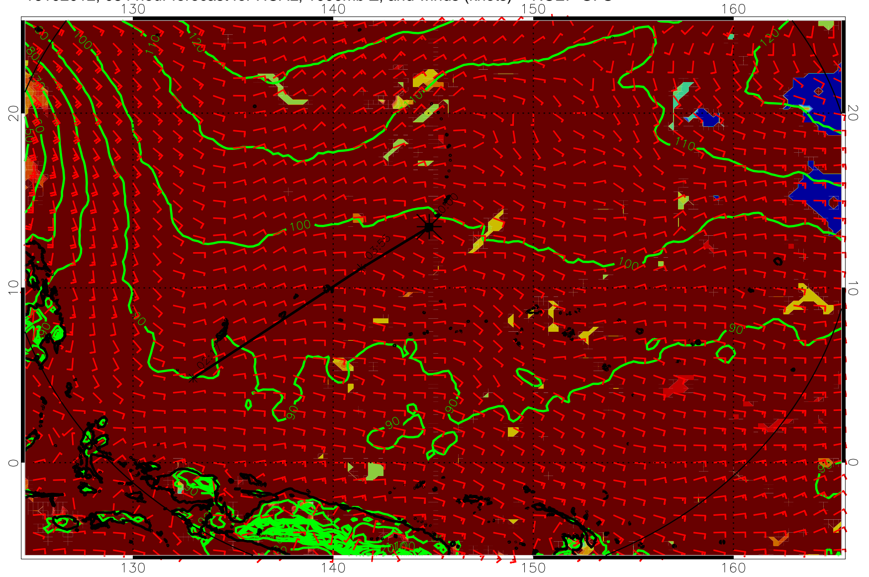
16102012, 084 hour forecast for HCAL, 1000mb Z, and winds (knots) -- NCEP GFS
