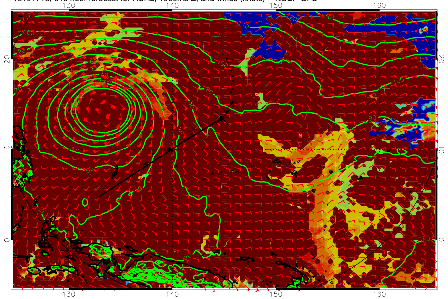
16101718, 018 hour forecast for HCAL, 1000mb Z, and winds (knots) -- NCEP GFS
