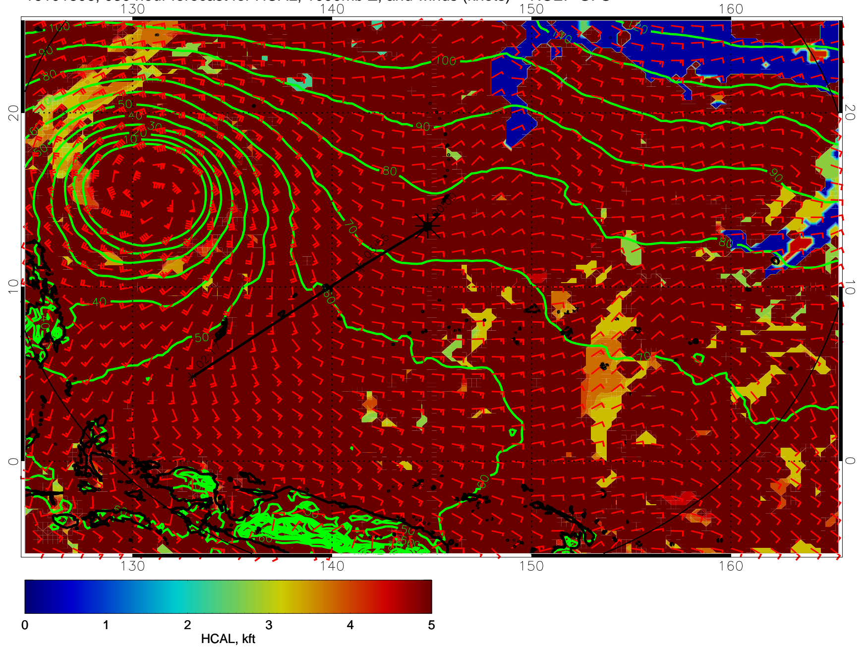
16101806, 030 hour forecast for HCAL, 1000mb Z, and winds (knots) -- NCEP GFS
