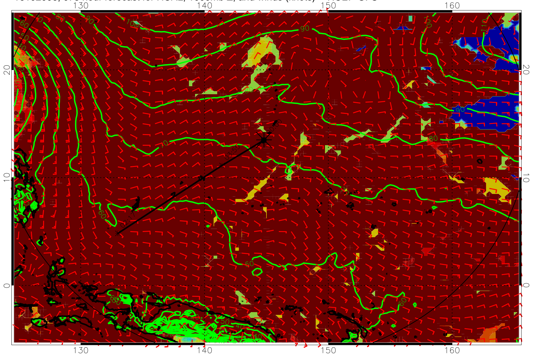
16102006, 078 hour forecast for HCAL, 1000mb Z, and winds (knots) -- NCEP GFS
