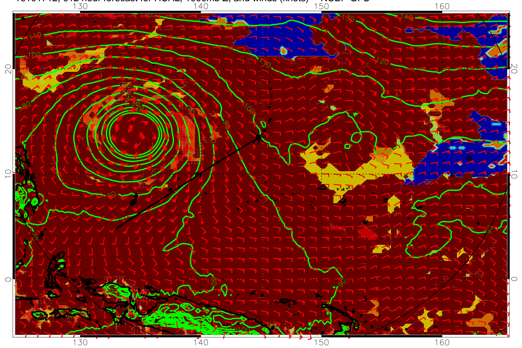
16101712, 012 hour forecast for HCAL, 1000mb Z, and winds (knots) -- NCEP GFS
