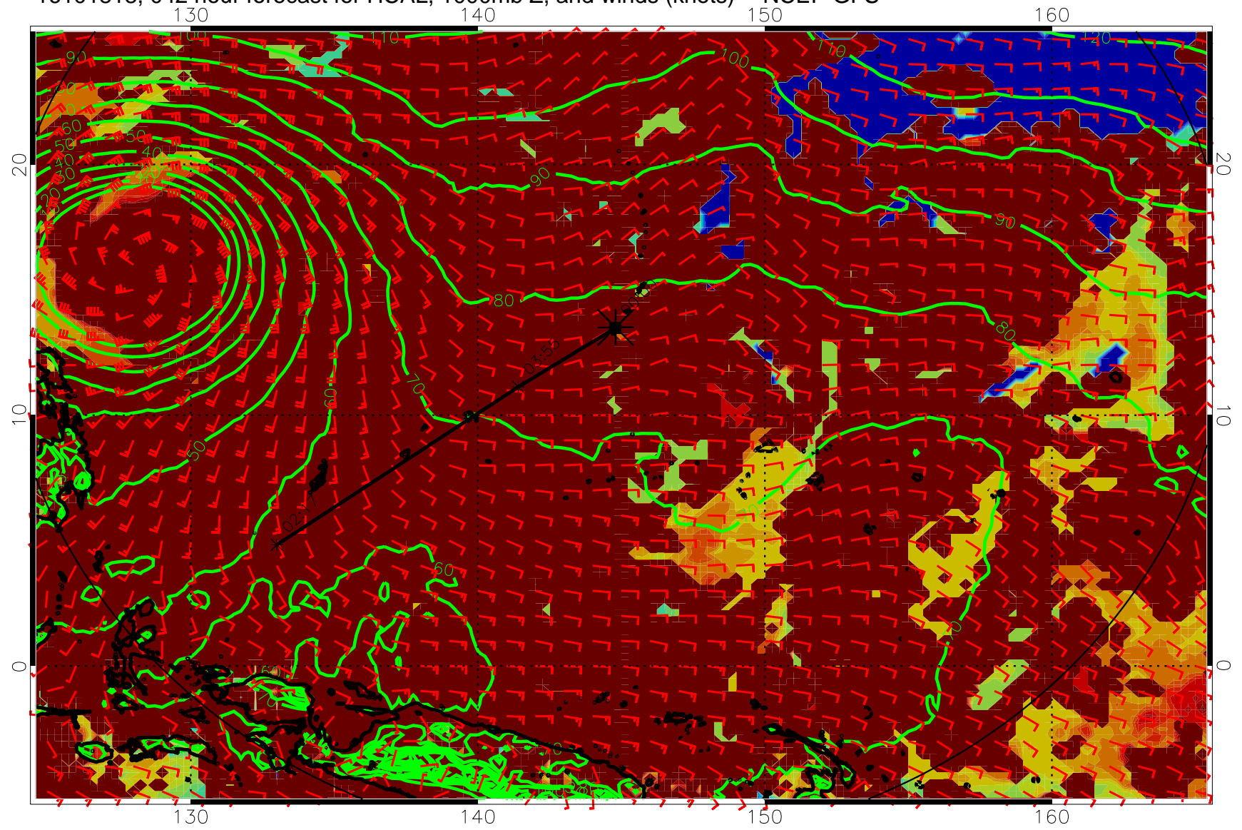
16101818, 042 hour forecast for HCAL, 1000mb Z, and winds (knots) -- NCEP GFS
