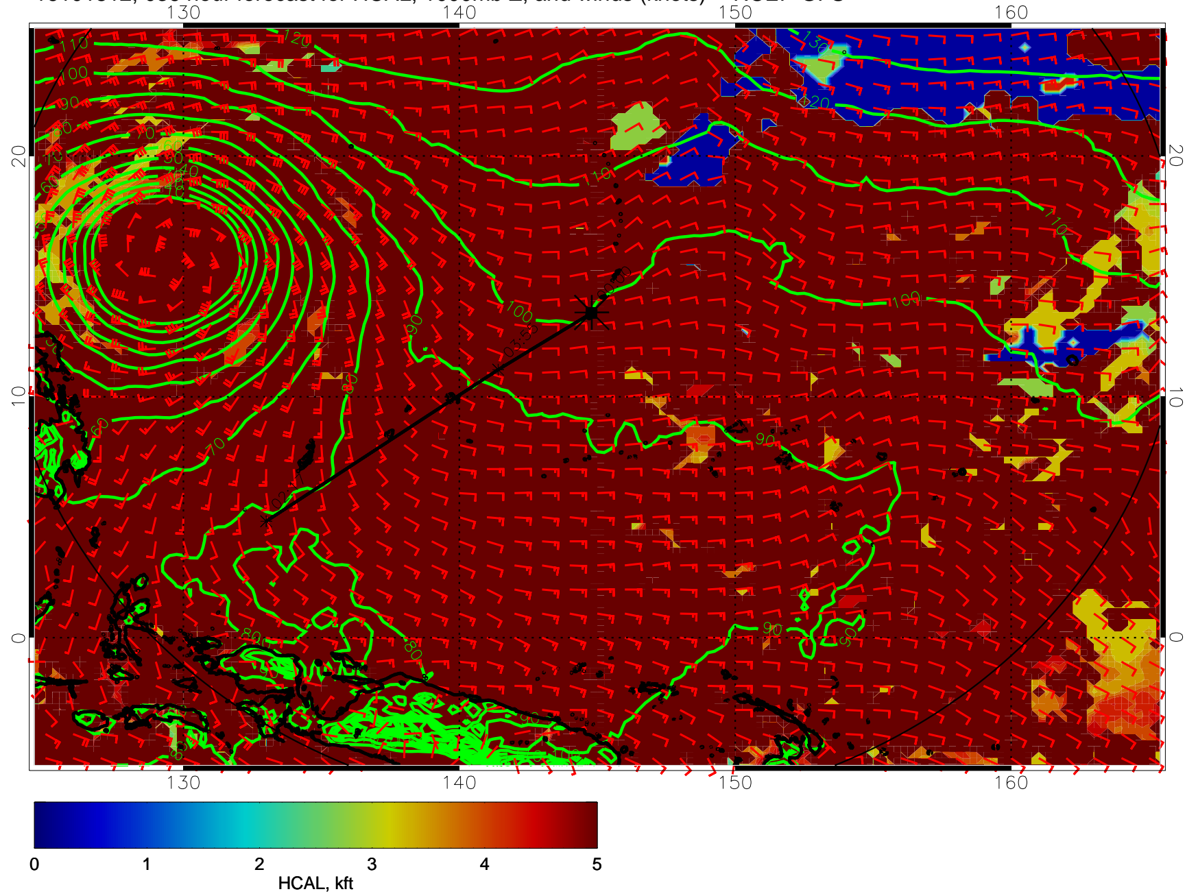
16101812, 036 hour forecast for HCAL, 1000mb Z, and winds (knots) -- NCEP GFS
