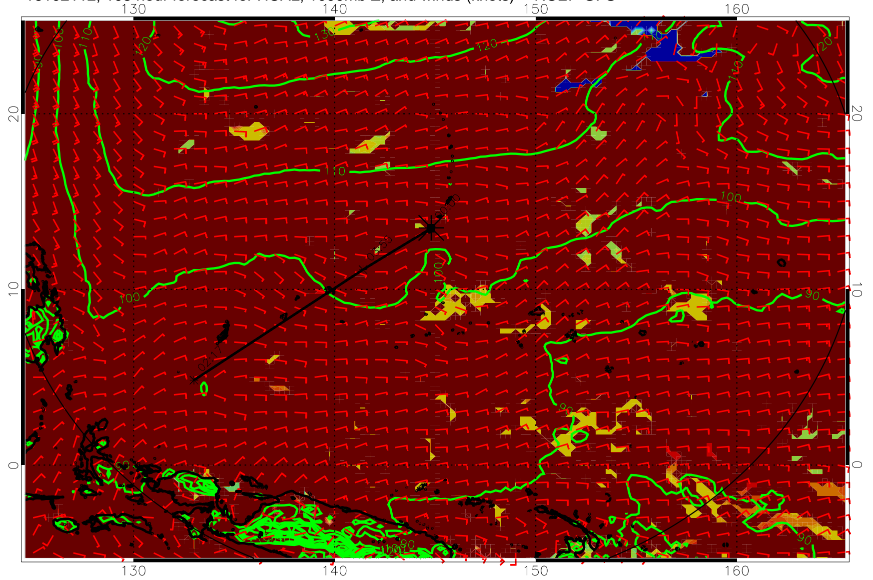
16102112, 108 hour forecast for HCAL, 1000mb Z, and winds (knots) -- NCEP GFS
