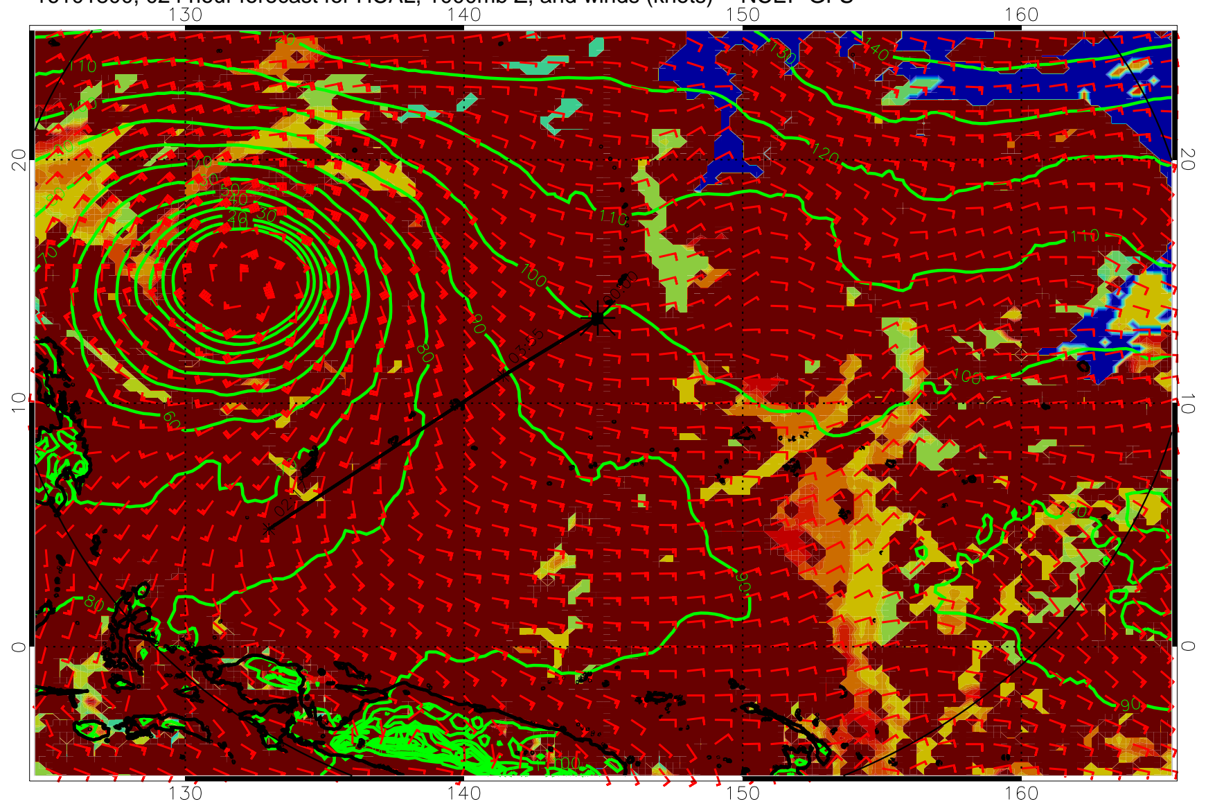
16101800, 024 hour forecast for HCAL, 1000mb Z, and winds (knots) -- NCEP GFS
