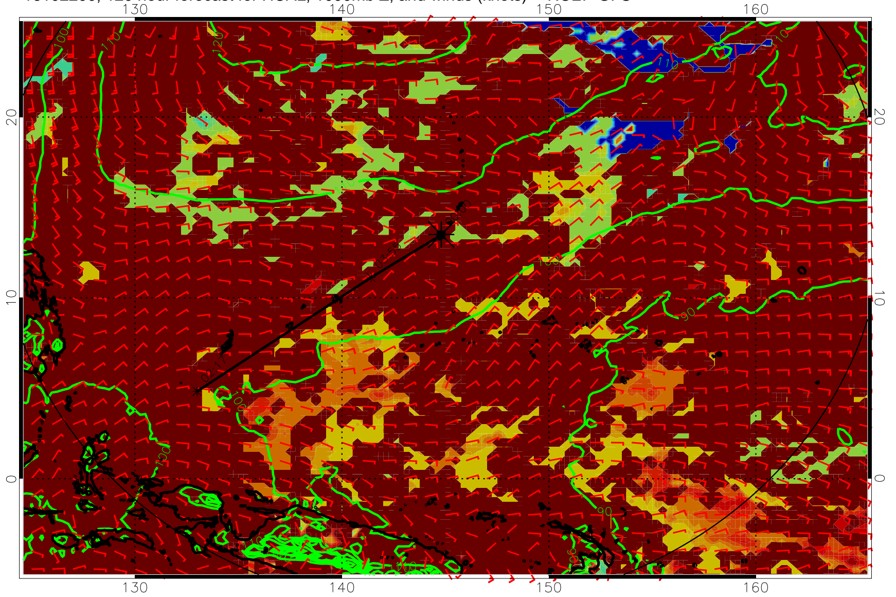
16102200, 120 hour forecast for HCAL, 1000mb Z, and winds (knots) -- NCEP GFS
