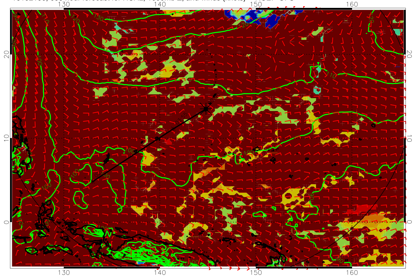
16102100, 096 hour forecast for HCAL, 1000mb Z, and winds (knots) -- NCEP GFS
