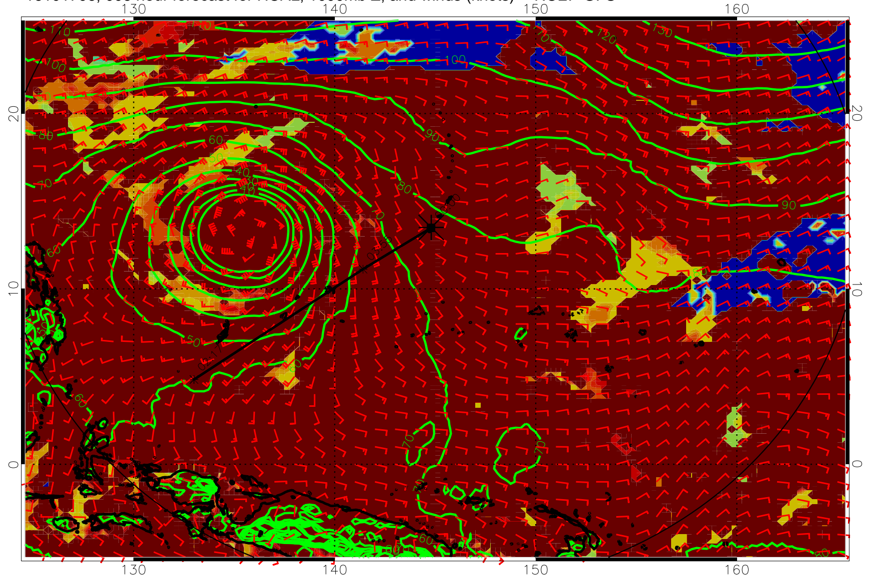
16101706, 006 hour forecast for HCAL, 1000mb Z, and winds (knots) -- NCEP GFS
