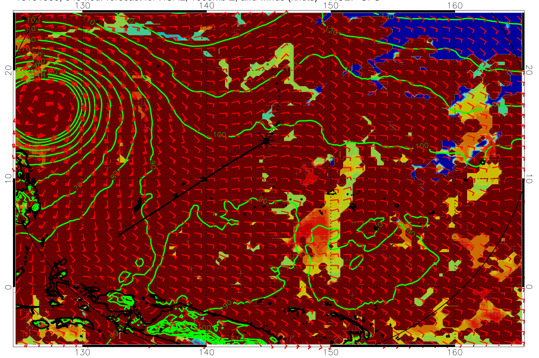
16101900, 048 hour forecast for HCAL, 1000mb Z, and winds (knots) -- NCEP GFS
