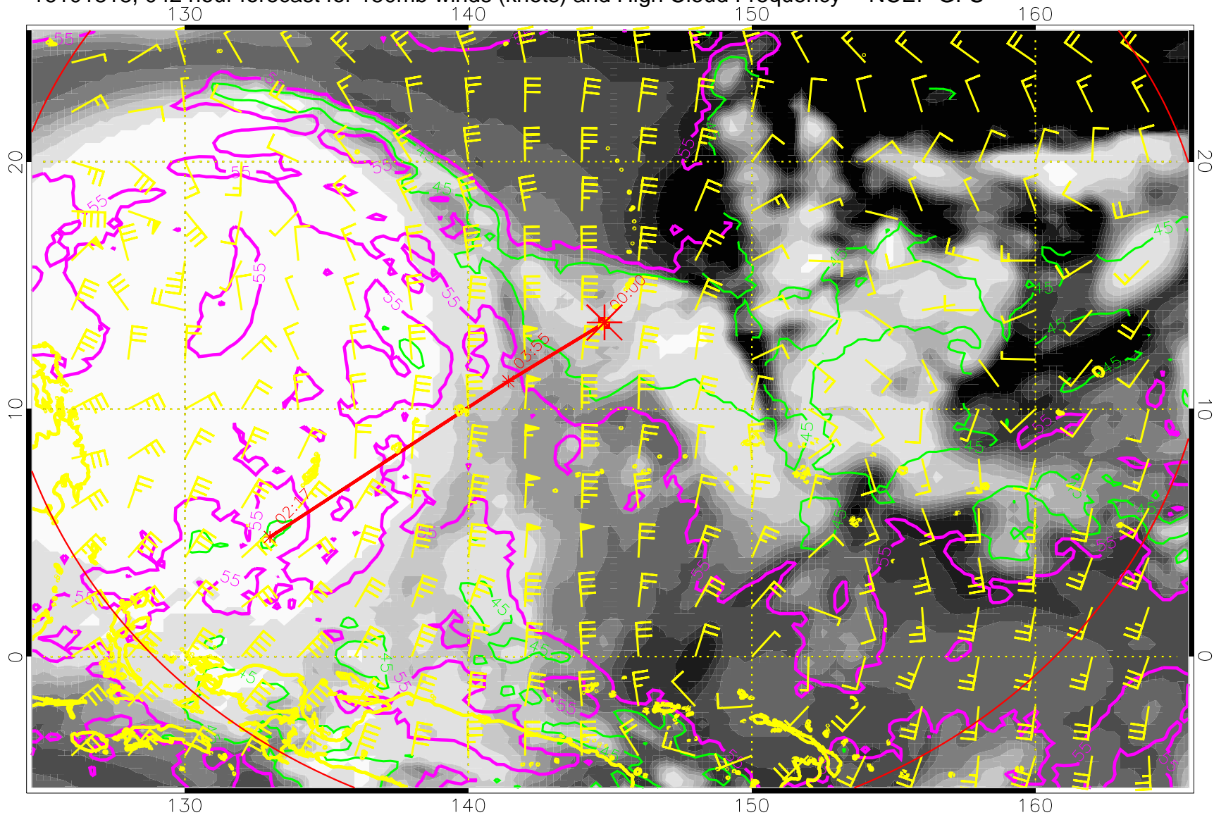
16101818, 042 hour forecast for 150mb winds (knots) and High Cloud Frequency -- NCEP GFS
