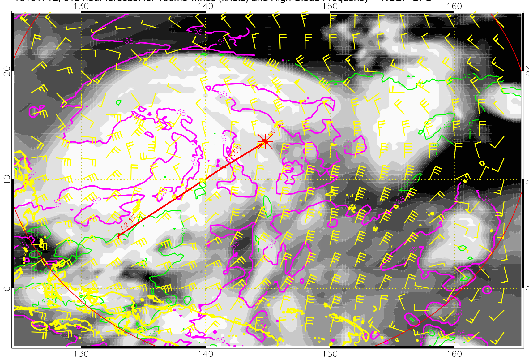
16101712, 012 hour forecast for 150mb winds (knots) and High Cloud Frequency -- NCEP GFS
