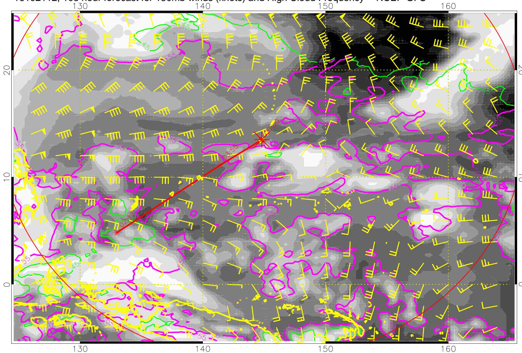
16102112, 108 hour forecast for 150mb winds (knots) and High Cloud Frequency -- NCEP GFS
