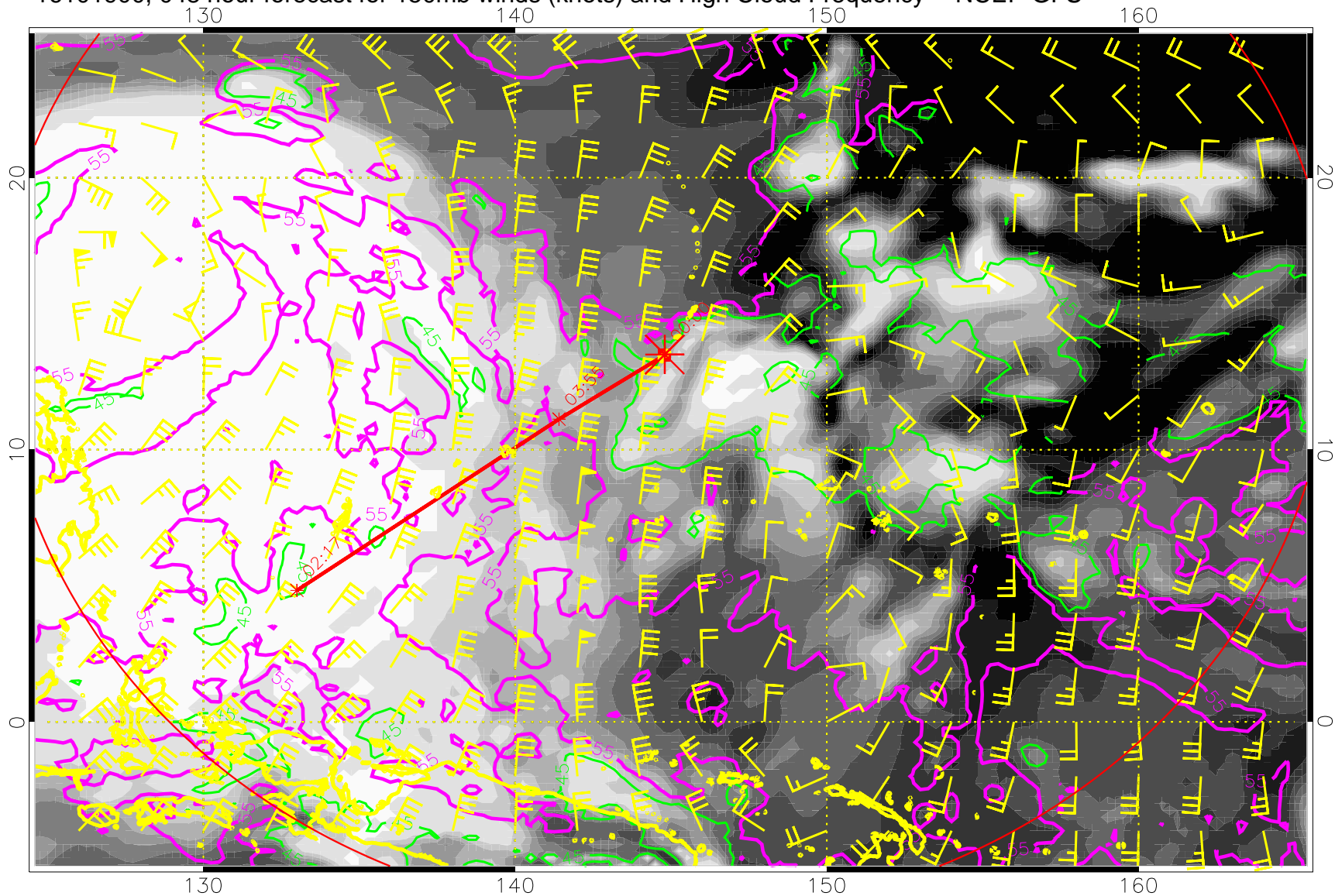
16101900, 048 hour forecast for 150mb winds (knots) and High Cloud Frequency -- NCEP GFS
