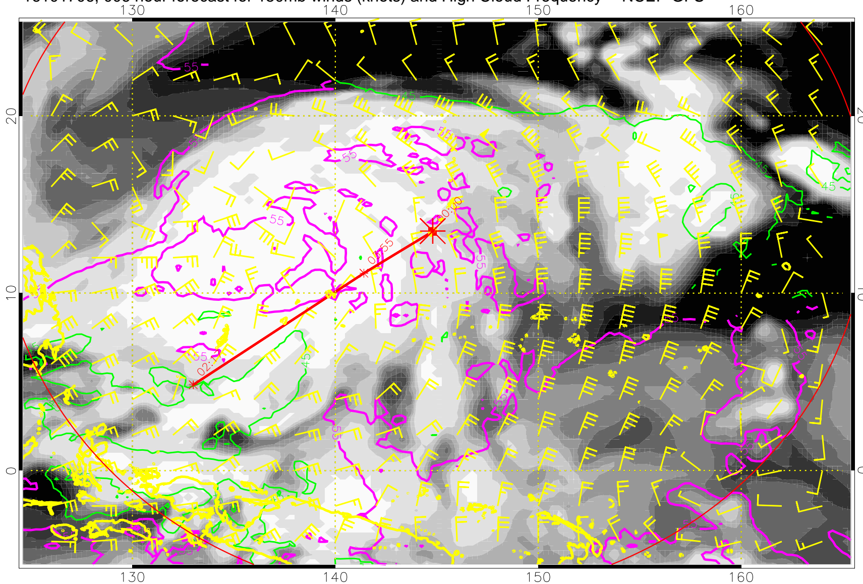
16101706, 006 hour forecast for 150mb winds (knots) and High Cloud Frequency -- NCEP GFS
