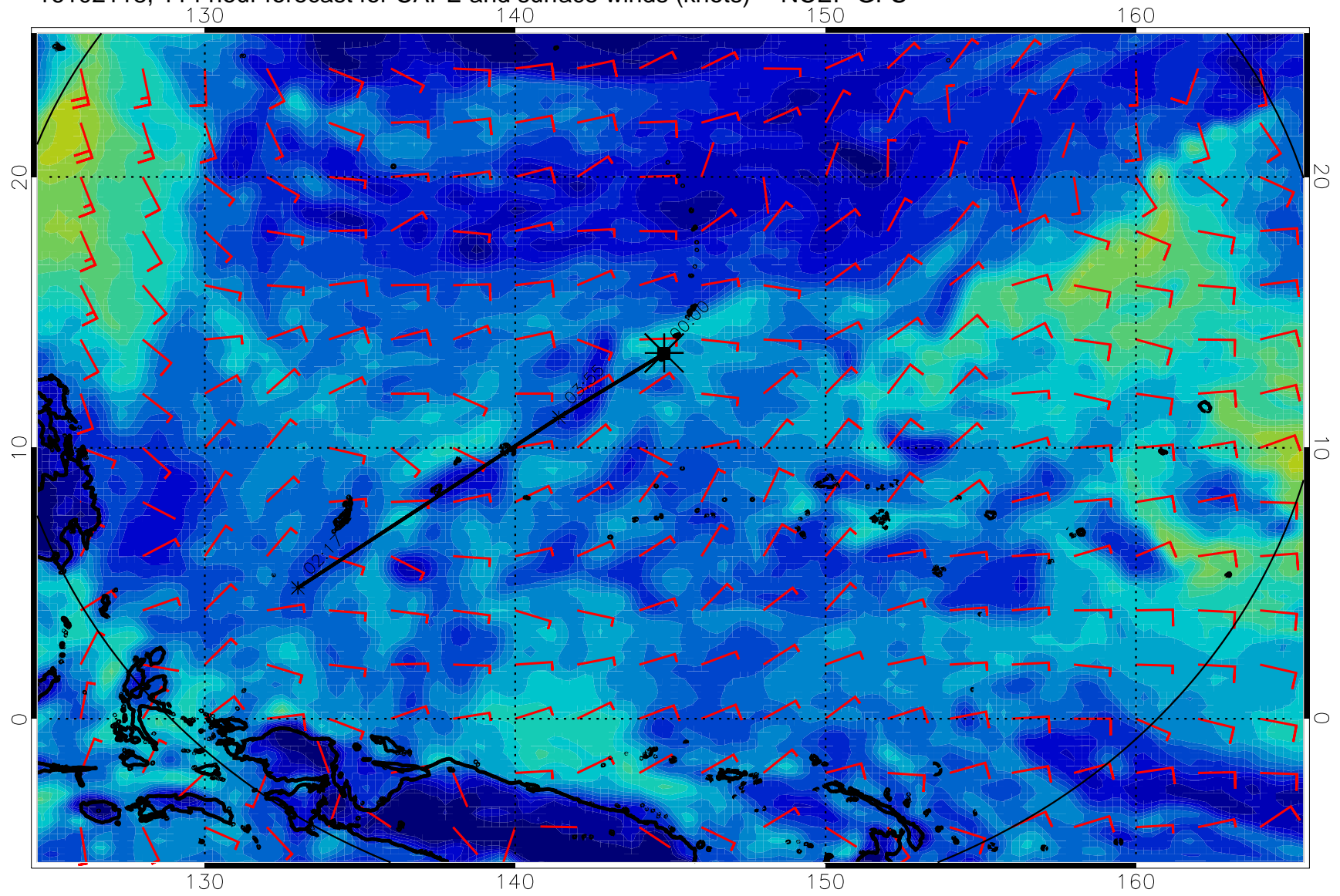
16102118, 114 hour forecast for CAPE and surface winds (knots) -- NCEP GFS
