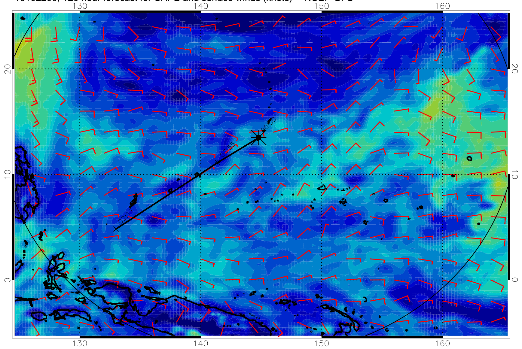
16102200, 120 hour forecast for CAPE and surface winds (knots) -- NCEP GFS
