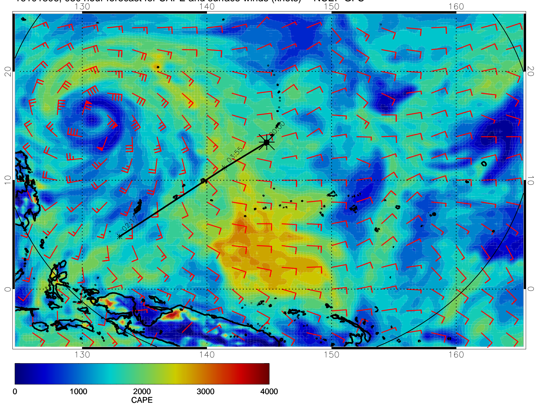
16101806, 030 hour forecast for CAPE and surface winds (knots) -- NCEP GFS
