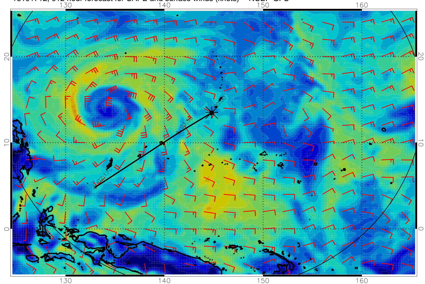
16101712, 012 hour forecast for CAPE and surface winds (knots) -- NCEP GFS
