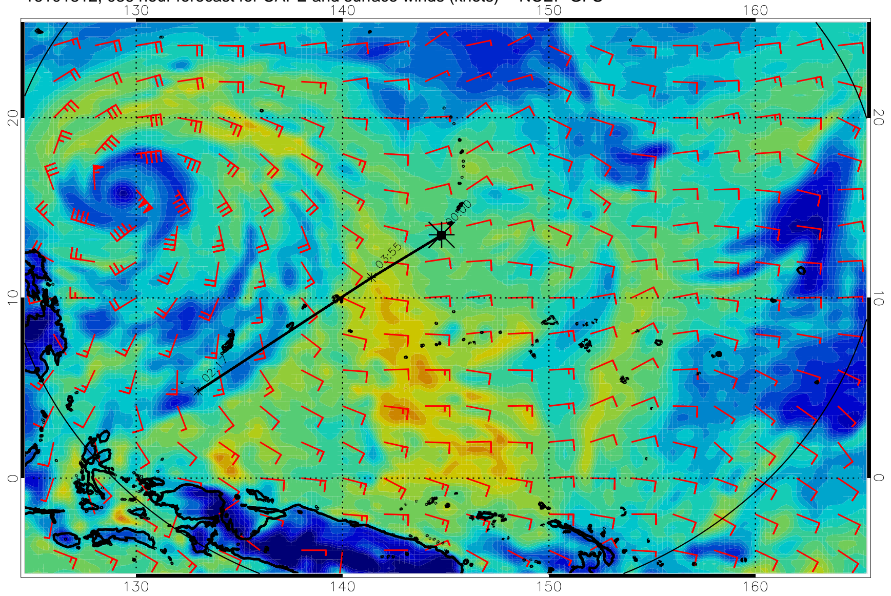
16101812, 036 hour forecast for CAPE and surface winds (knots) -- NCEP GFS
