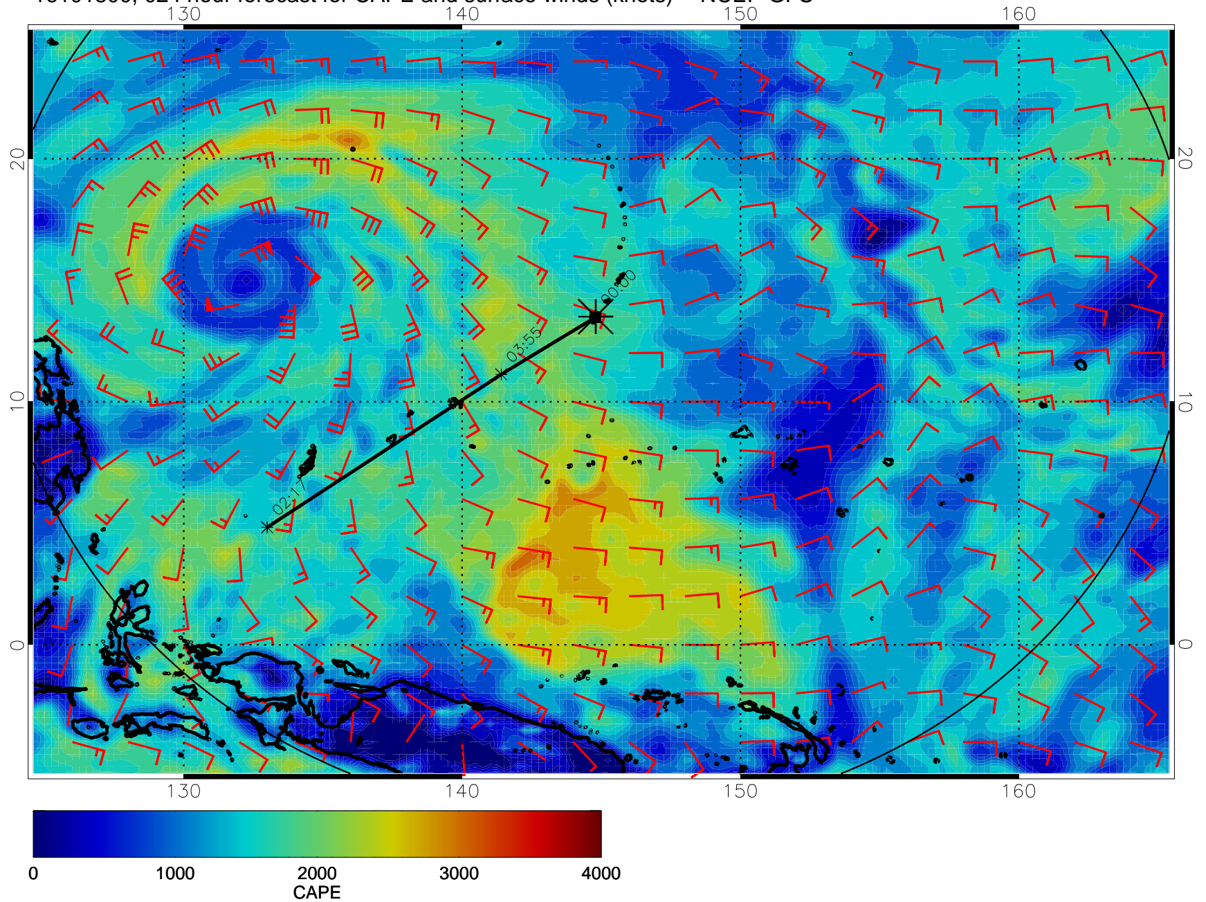
16101800, 024 hour forecast for CAPE and surface winds (knots) -- NCEP GFS
