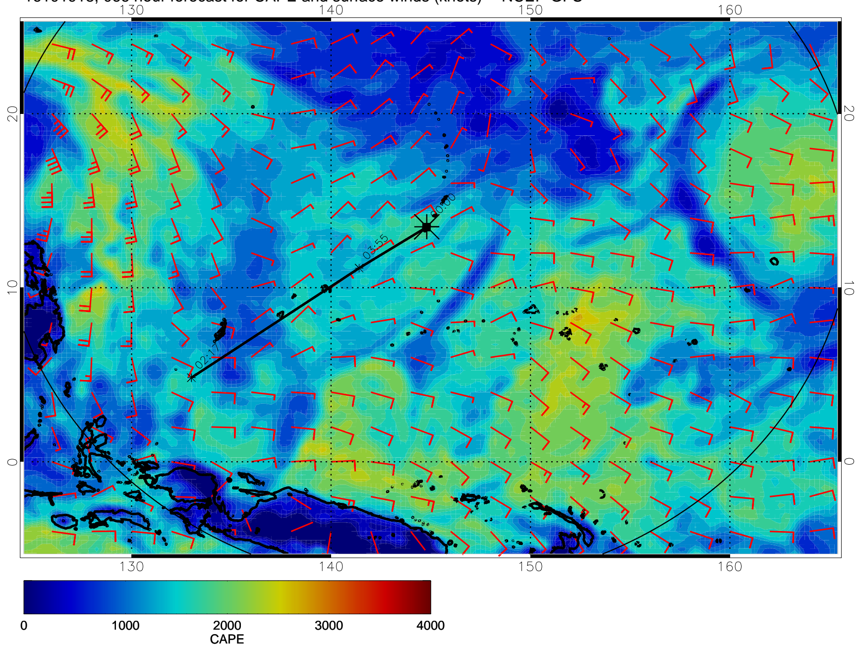
16101918, 066 hour forecast for CAPE and surface winds (knots) -- NCEP GFS
