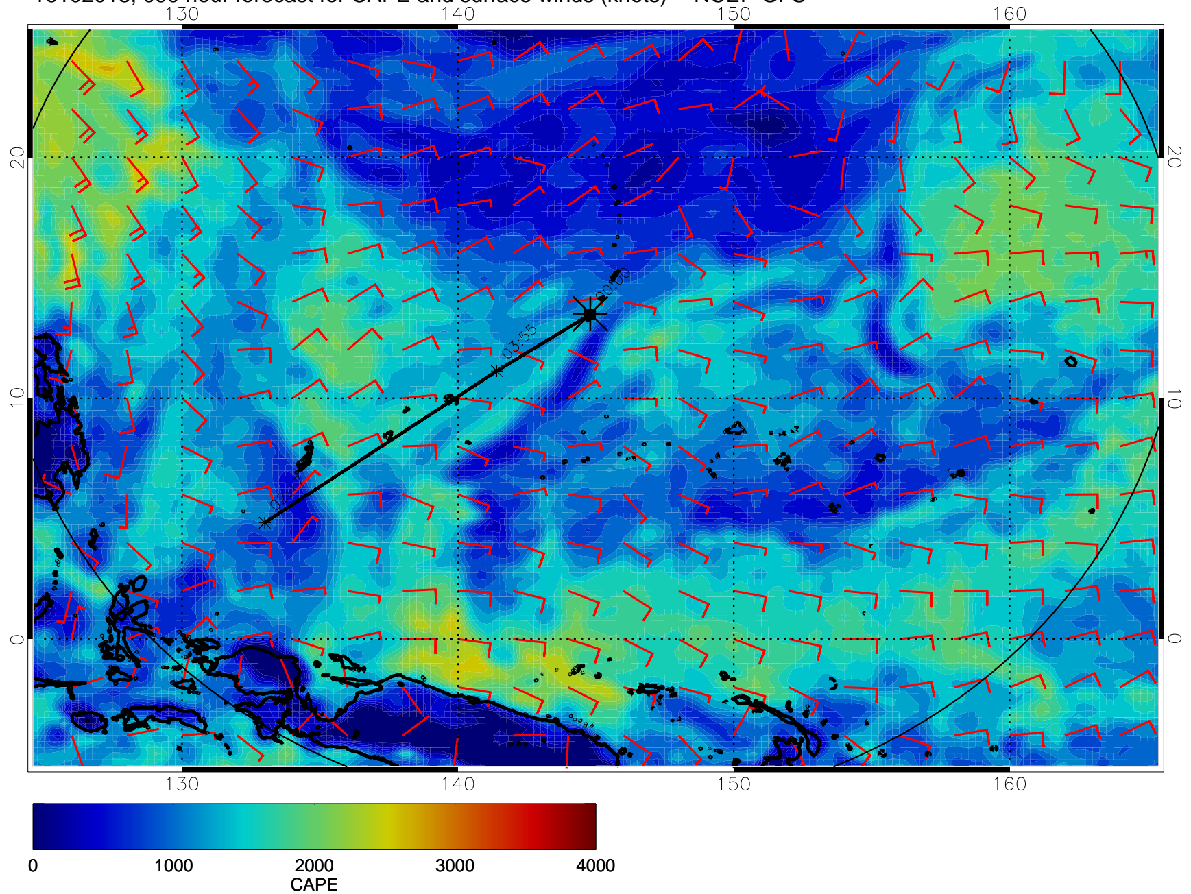
16102018, 090 hour forecast for CAPE and surface winds (knots) -- NCEP GFS
