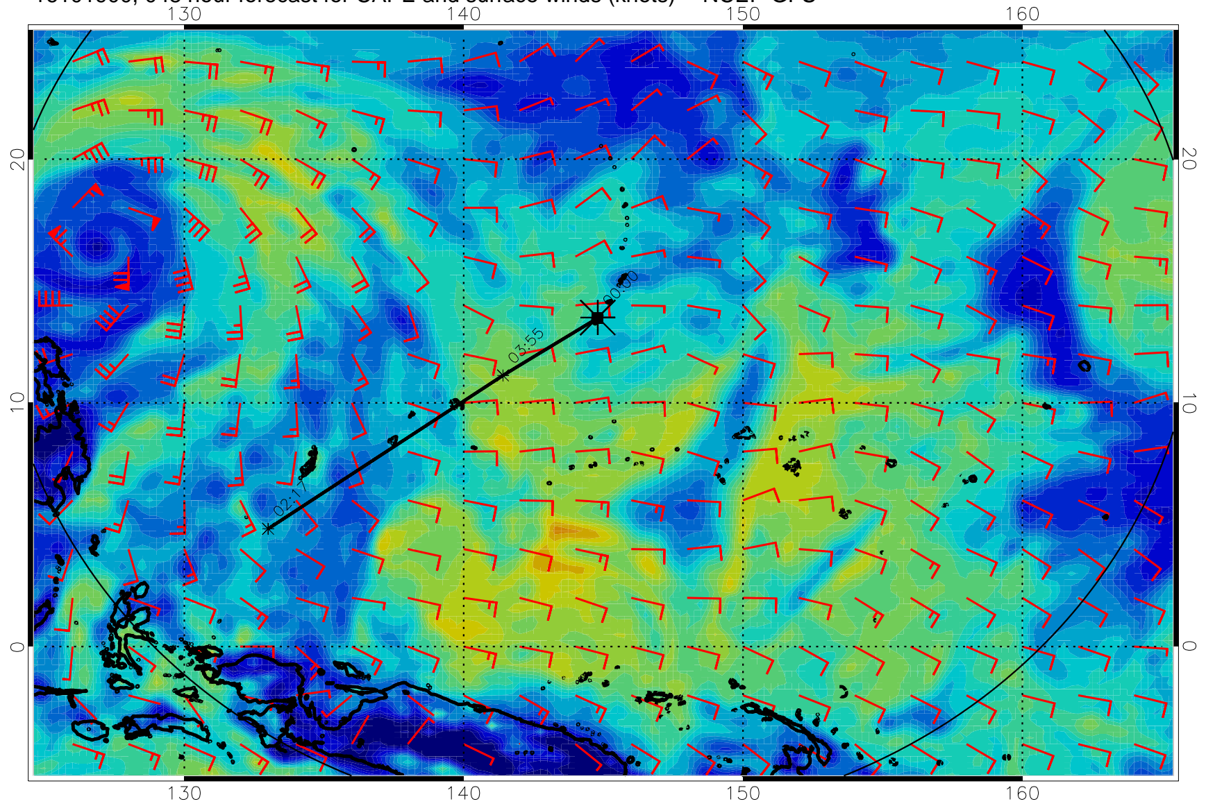
16101900, 048 hour forecast for CAPE and surface winds (knots) -- NCEP GFS
