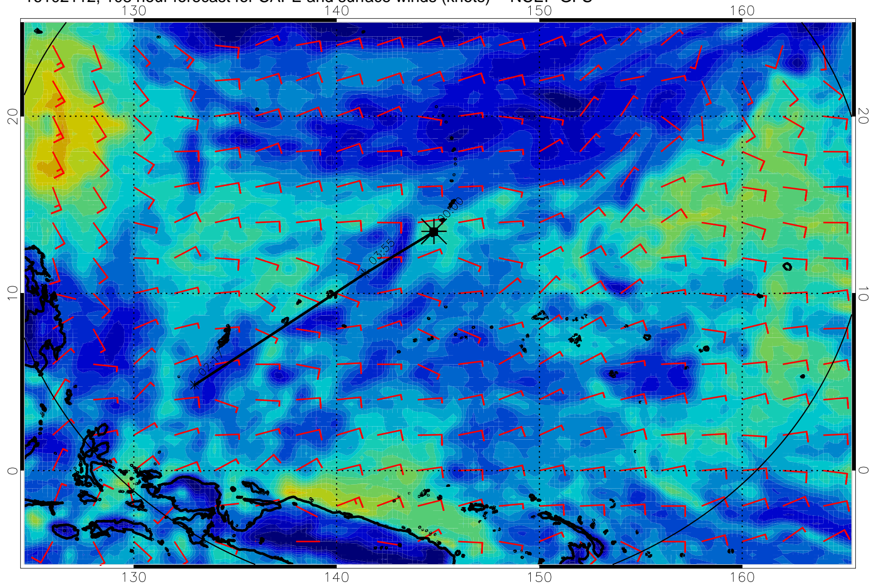
16102112, 108 hour forecast for CAPE and surface winds (knots) -- NCEP GFS
