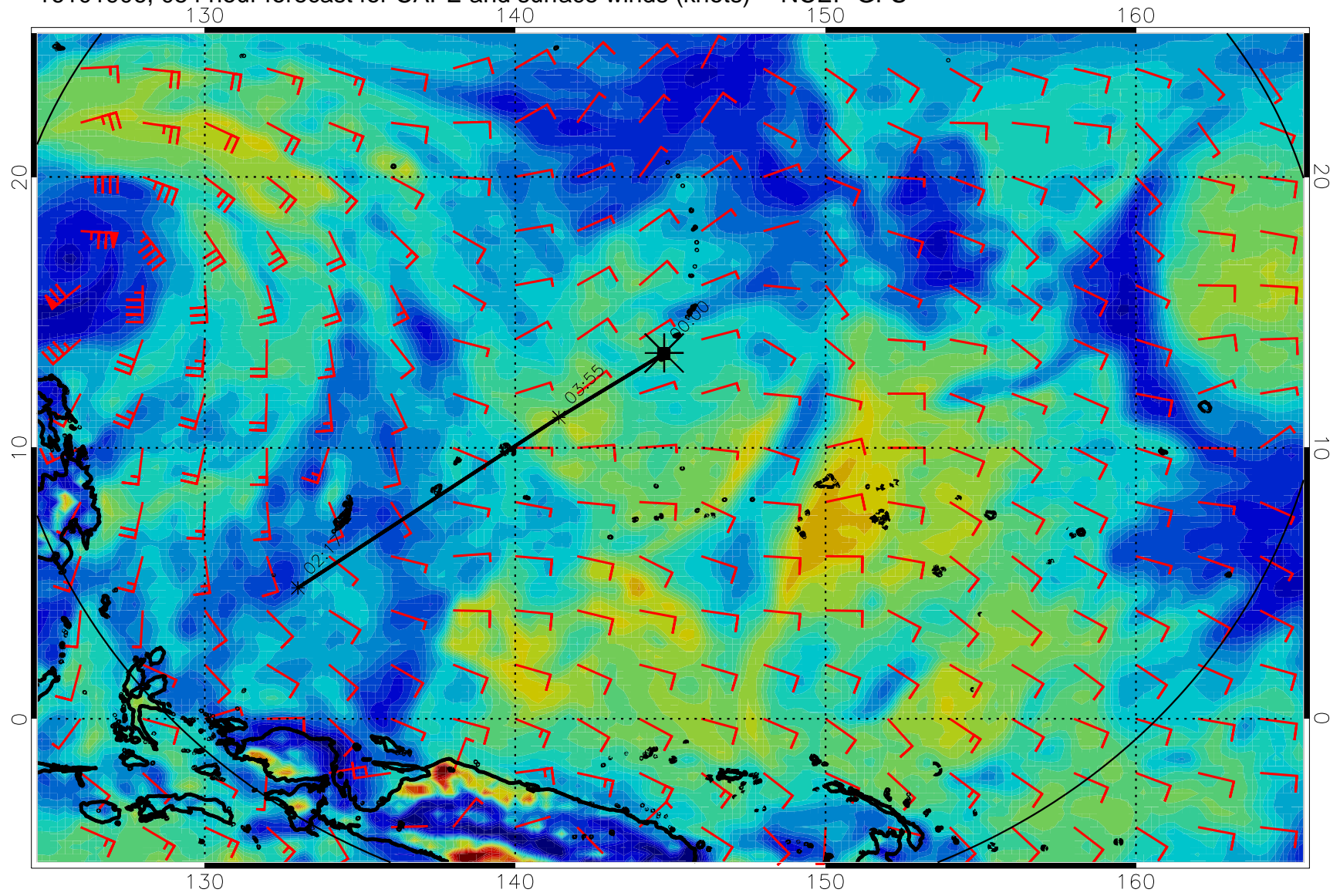
16101906, 054 hour forecast for CAPE and surface winds (knots) -- NCEP GFS
