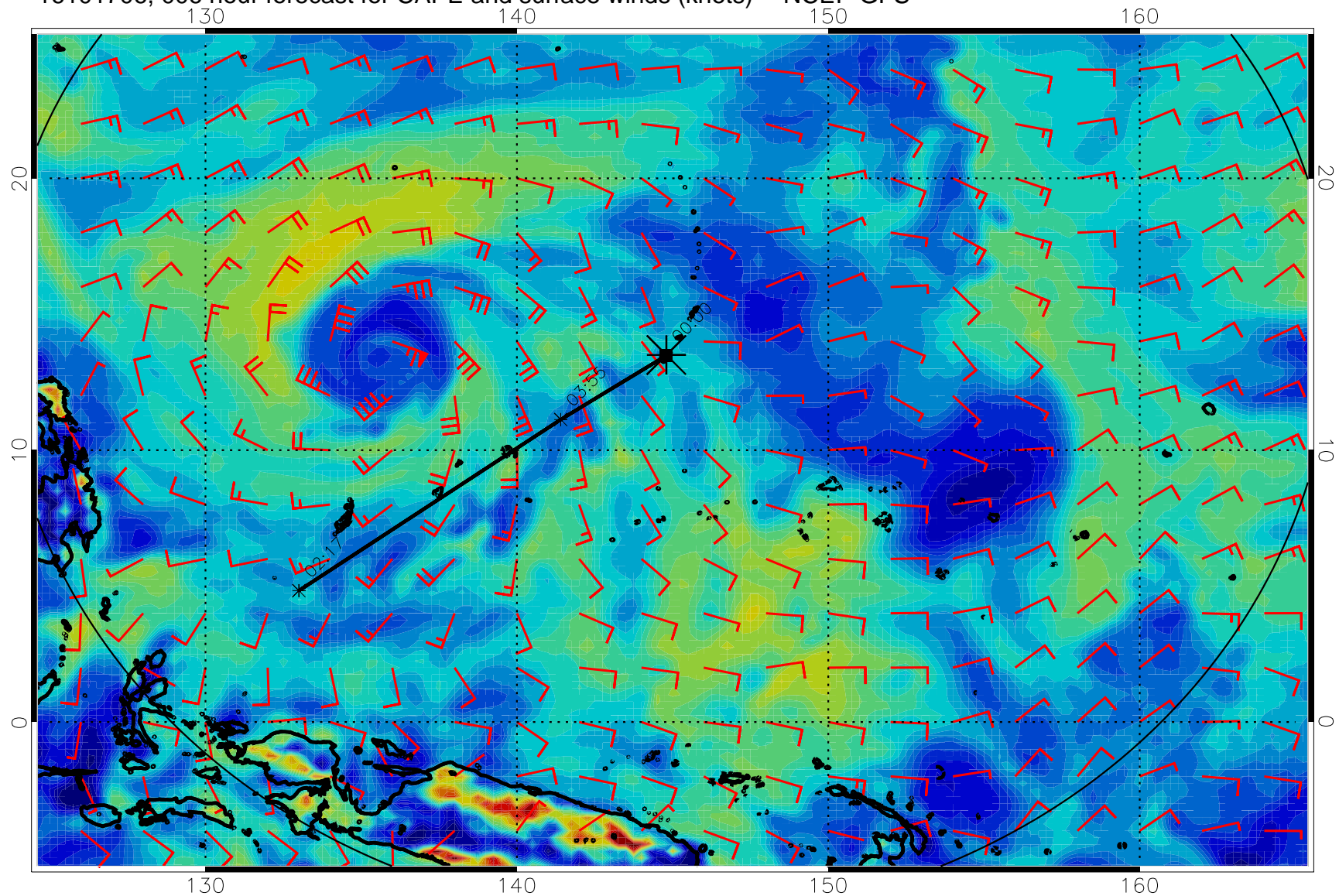
16101706, 006 hour forecast for CAPE and surface winds (knots) -- NCEP GFS
