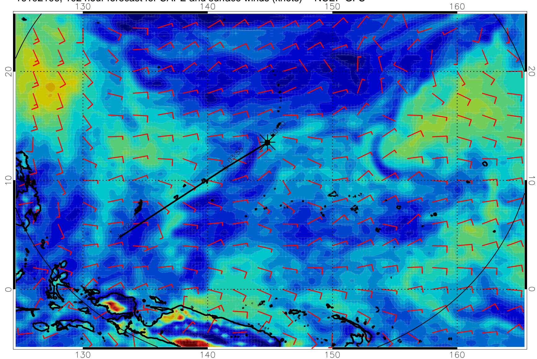
16102106, 102 hour forecast for CAPE and surface winds (knots) -- NCEP GFS
