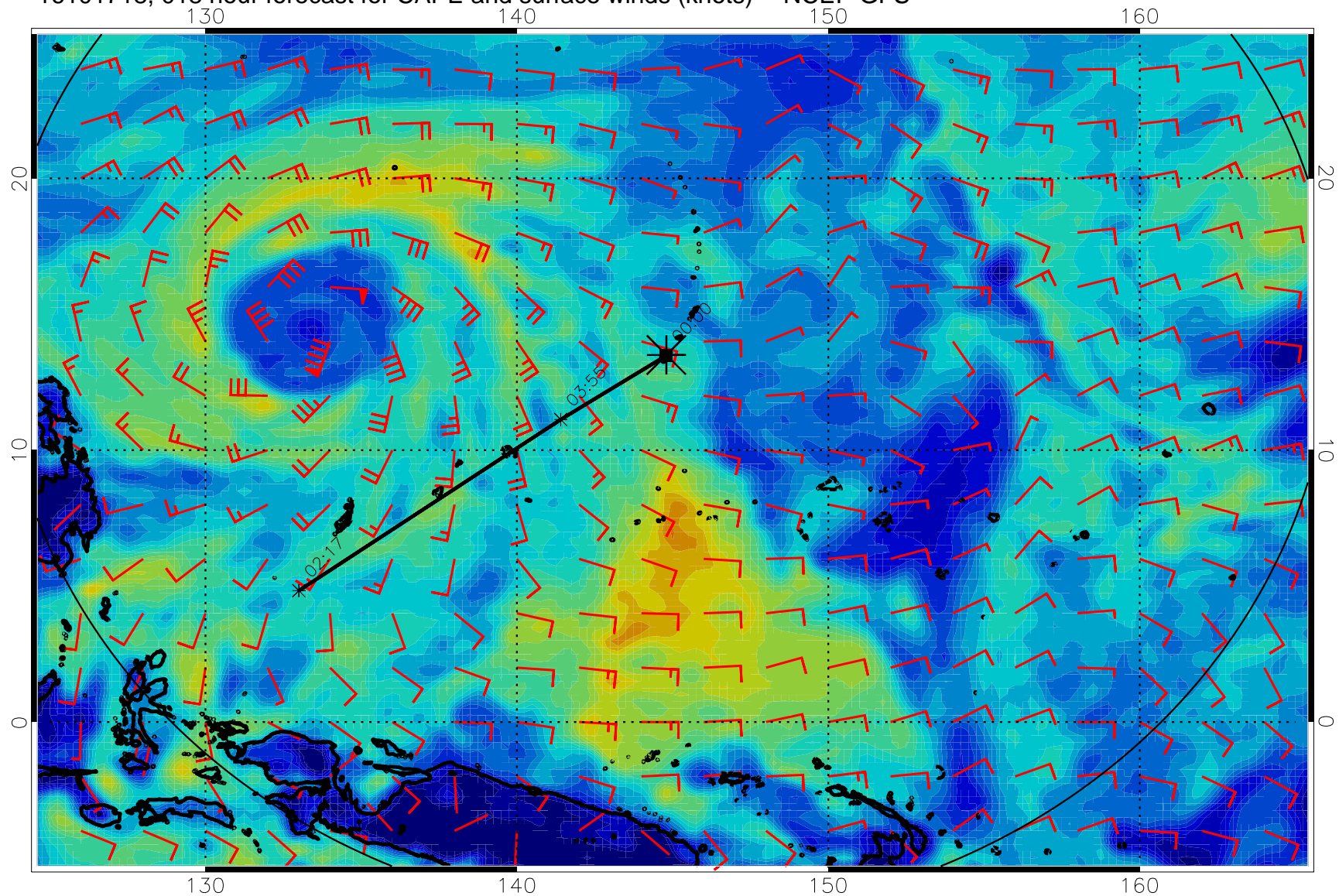
16101718, 018 hour forecast for CAPE and surface winds (knots) -- NCEP GFS
