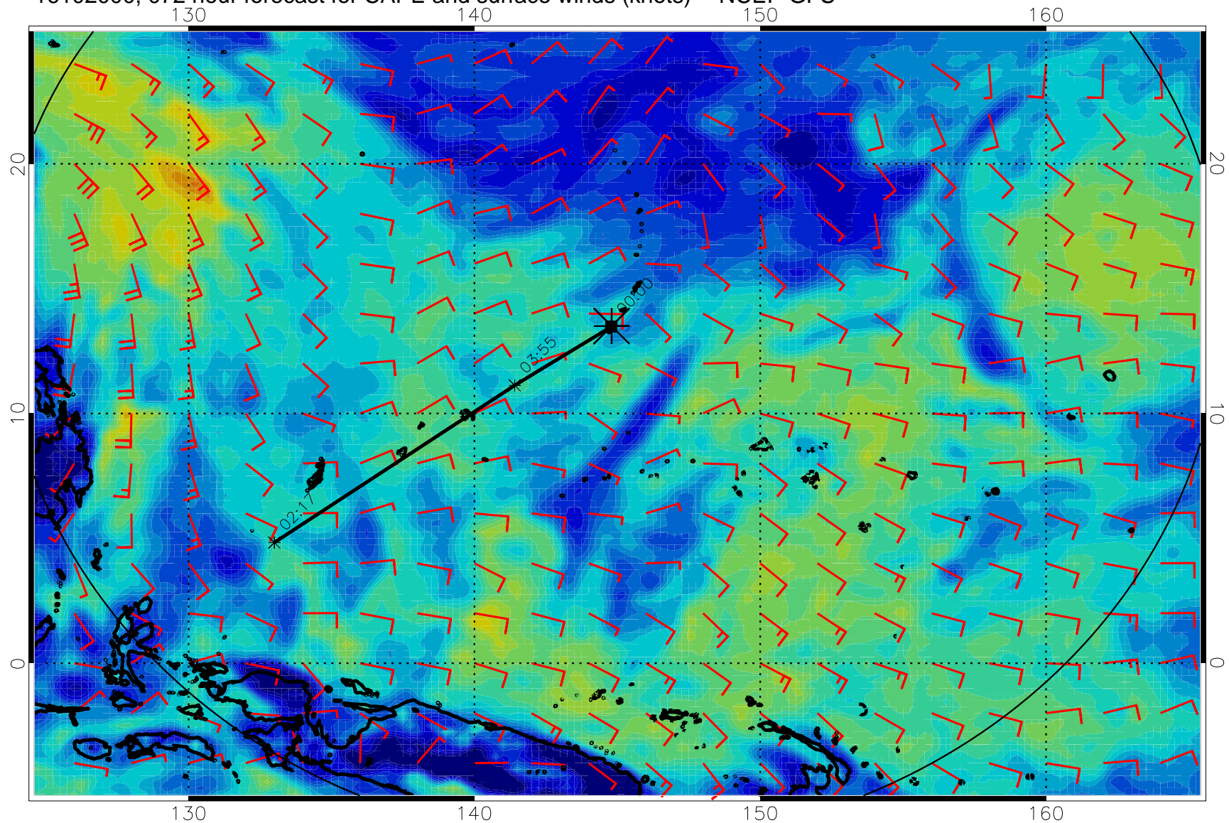
16102000, 072 hour forecast for CAPE and surface winds (knots) -- NCEP GFS
