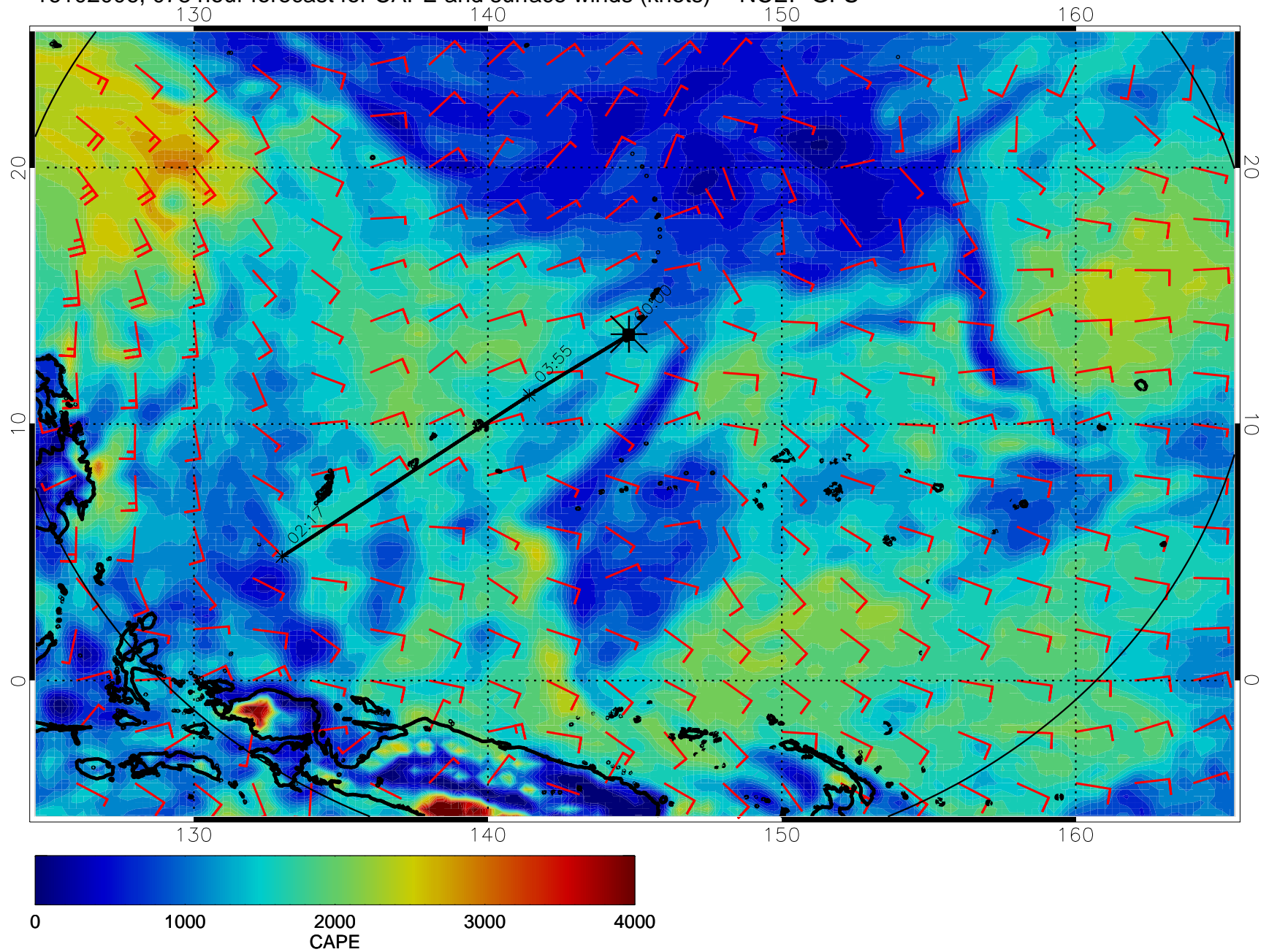
16102006, 078 hour forecast for CAPE and surface winds (knots) -- NCEP GFS
