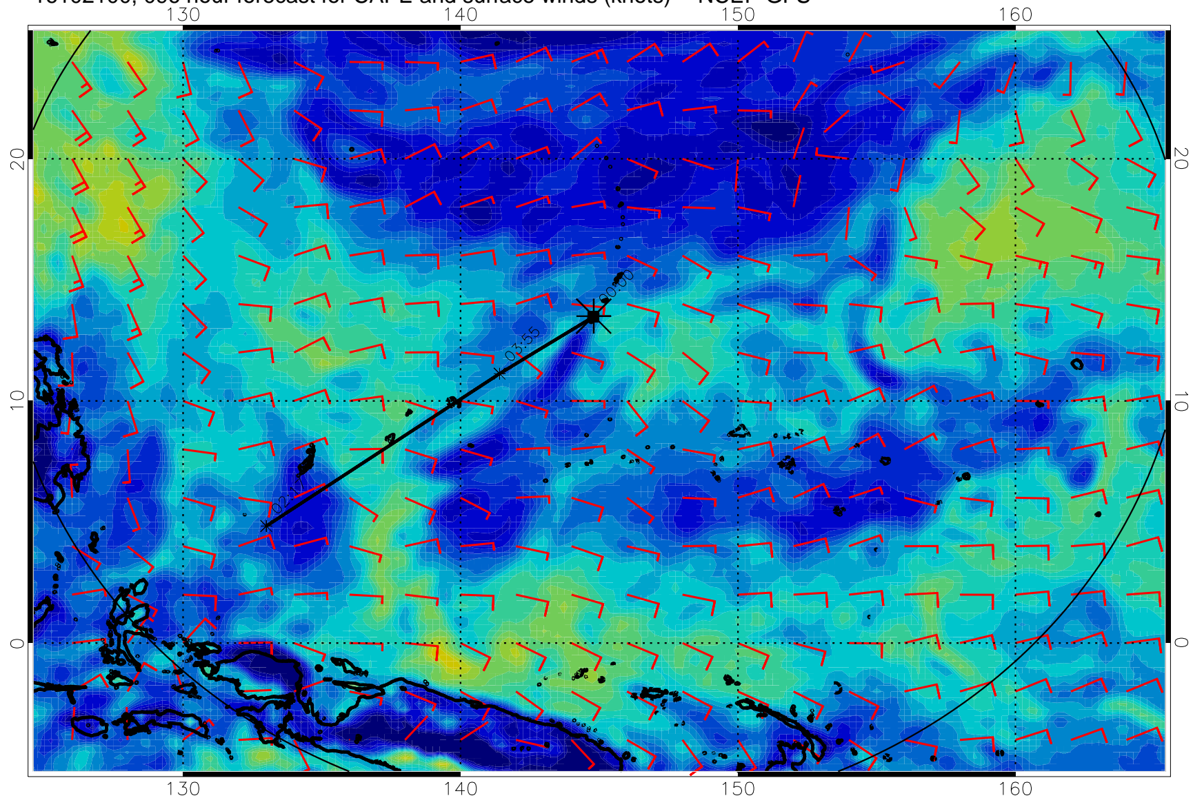
16102100, 096 hour forecast for CAPE and surface winds (knots) -- NCEP GFS
