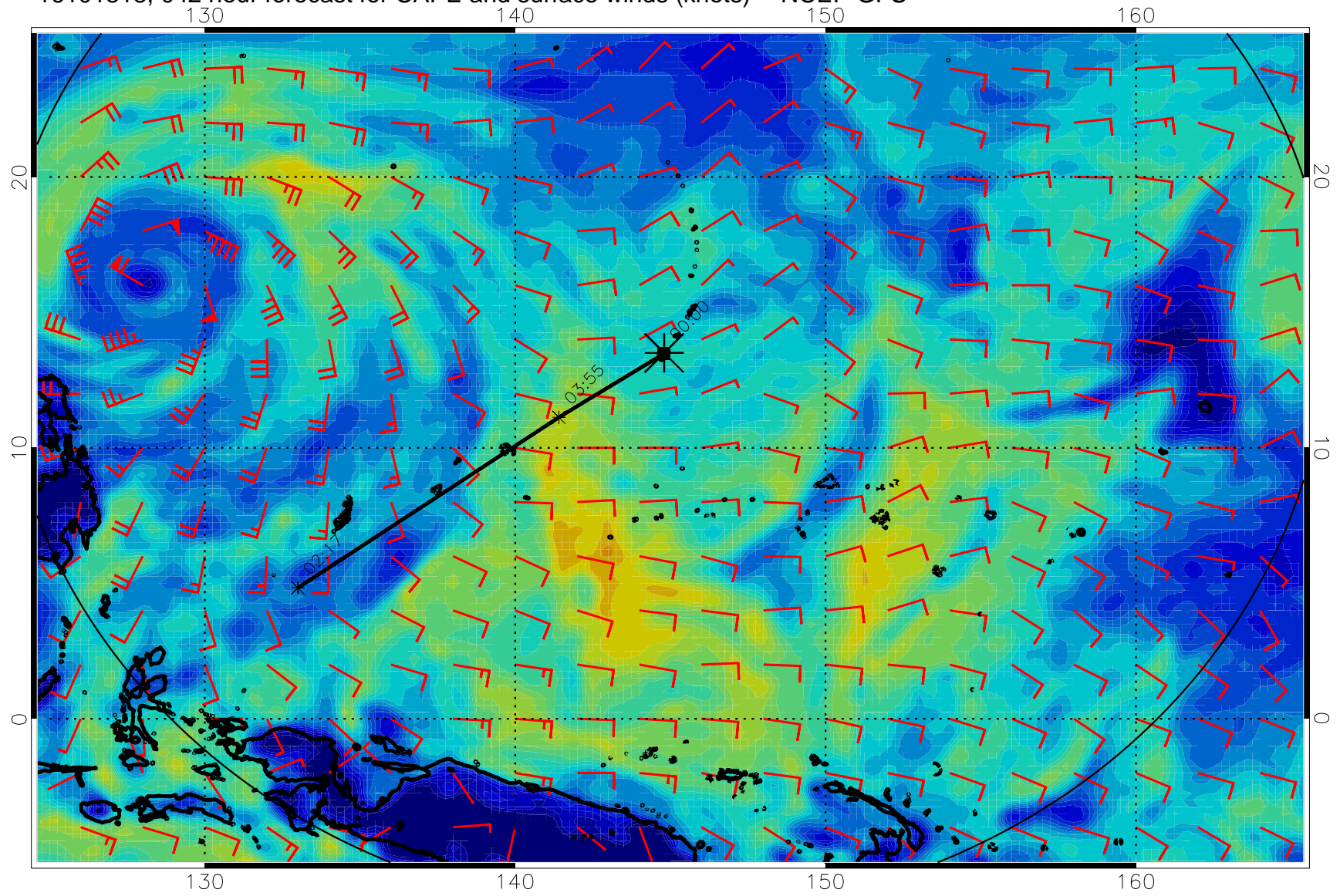
16101818, 042 hour forecast for CAPE and surface winds (knots) -- NCEP GFS
