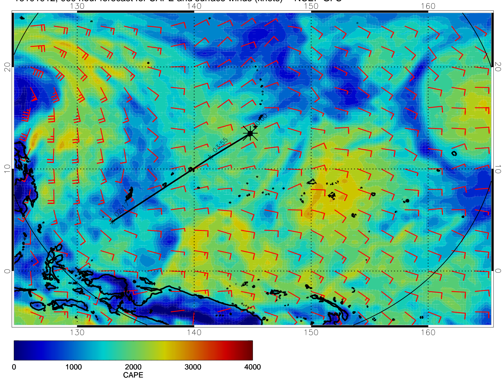
16101912, 060 hour forecast for CAPE and surface winds (knots) -- NCEP GFS
