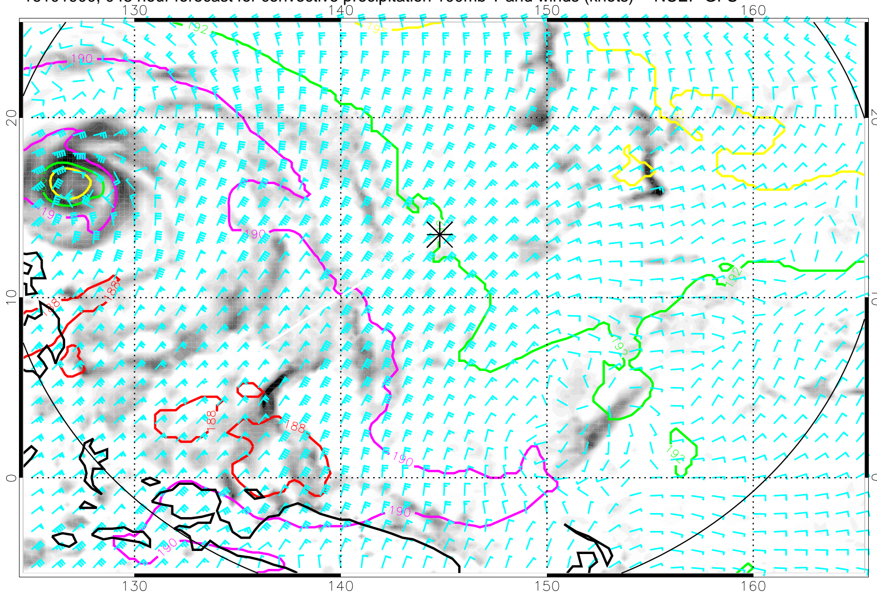
16101900, 048 hour forecast for convective precipitation 100mb T and winds (knots) -- NCEP GFS
