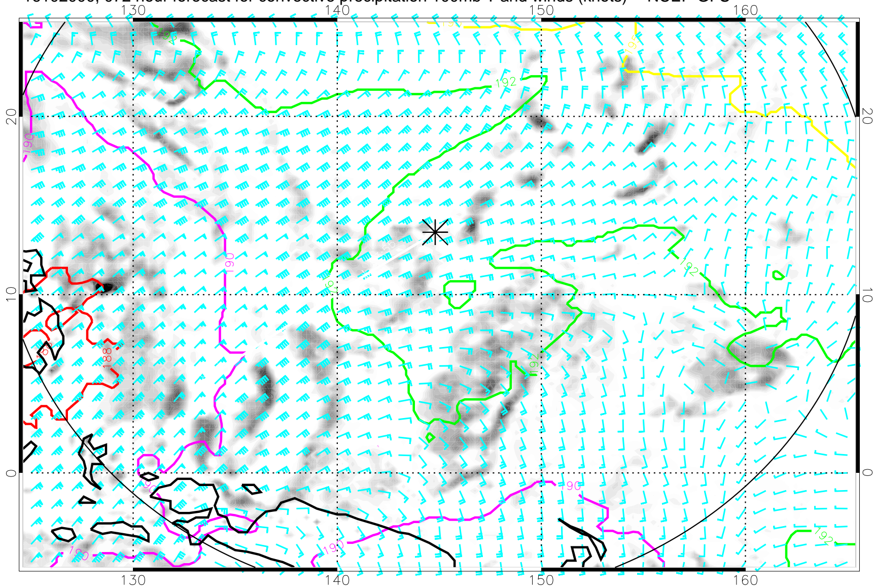
16102000, 072 hour forecast for convective precipitation 100mb T and winds (knots) -- NCEP GFS
