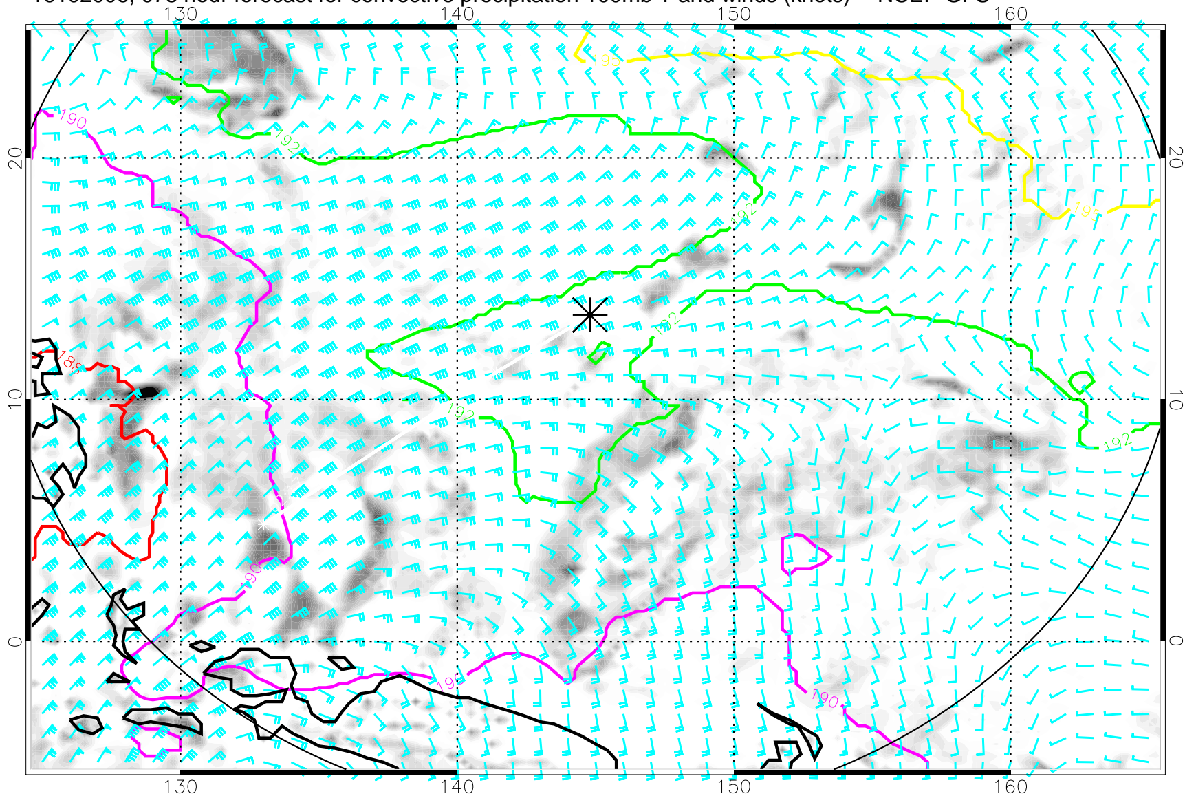
16102006, 078 hour forecast for convective precipitation 100mb T and winds (knots) -- NCEP GFS
