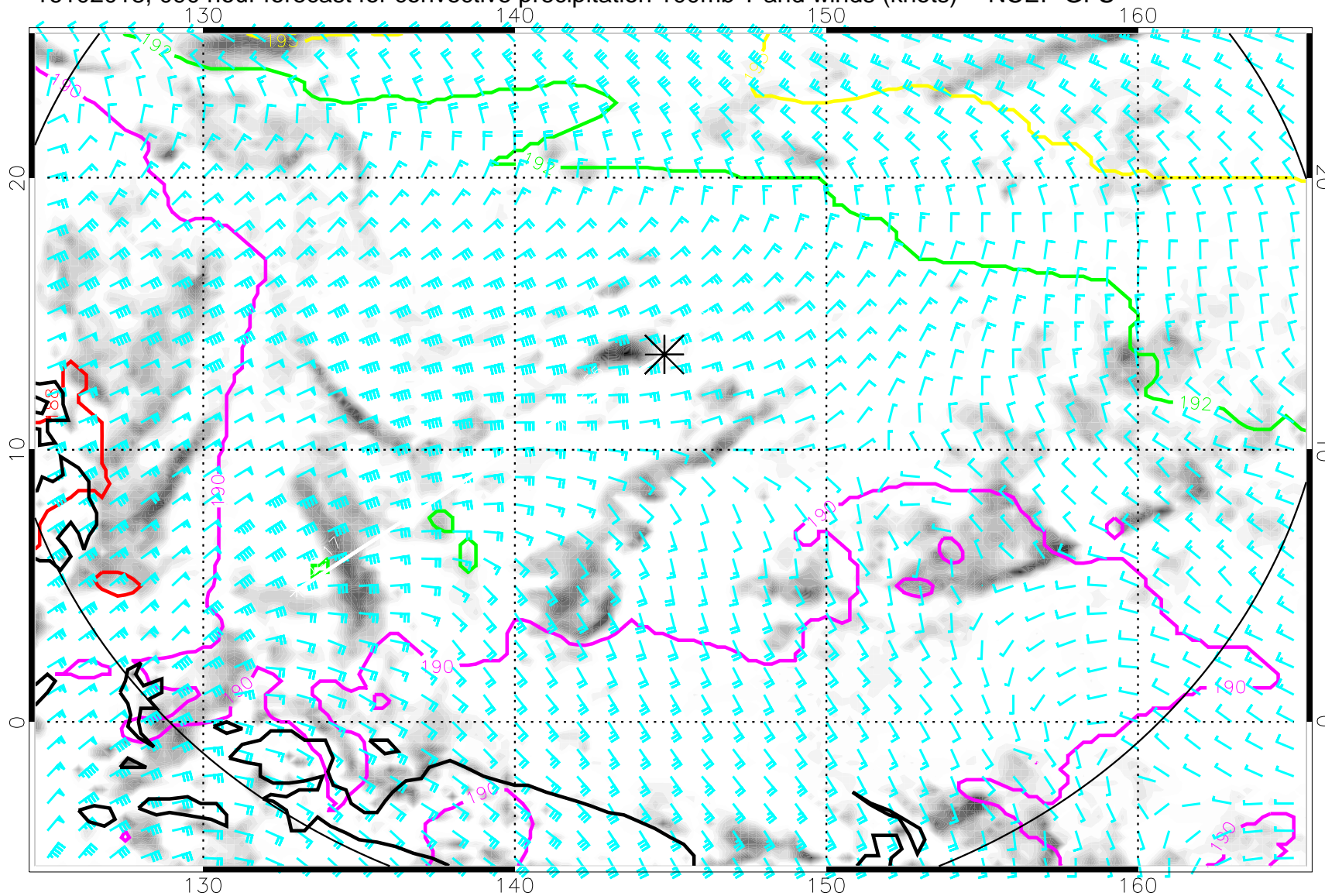
16102018, 090 hour forecast for convective precipitation 100mb T and winds (knots) -- NCEP GFS
