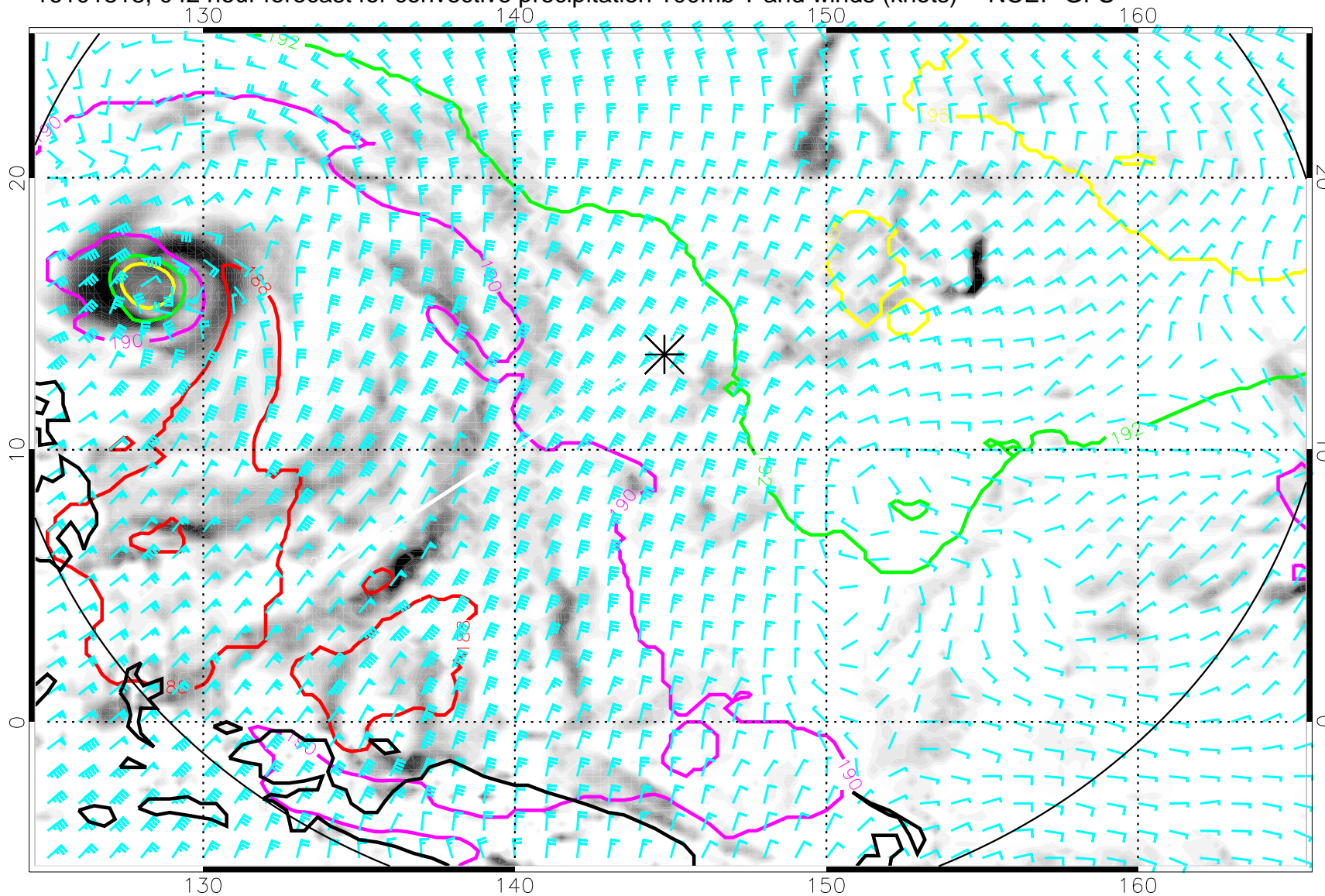
16101818, 042 hour forecast for convective precipitation 100mb T and winds (knots) -- NCEP GFS
