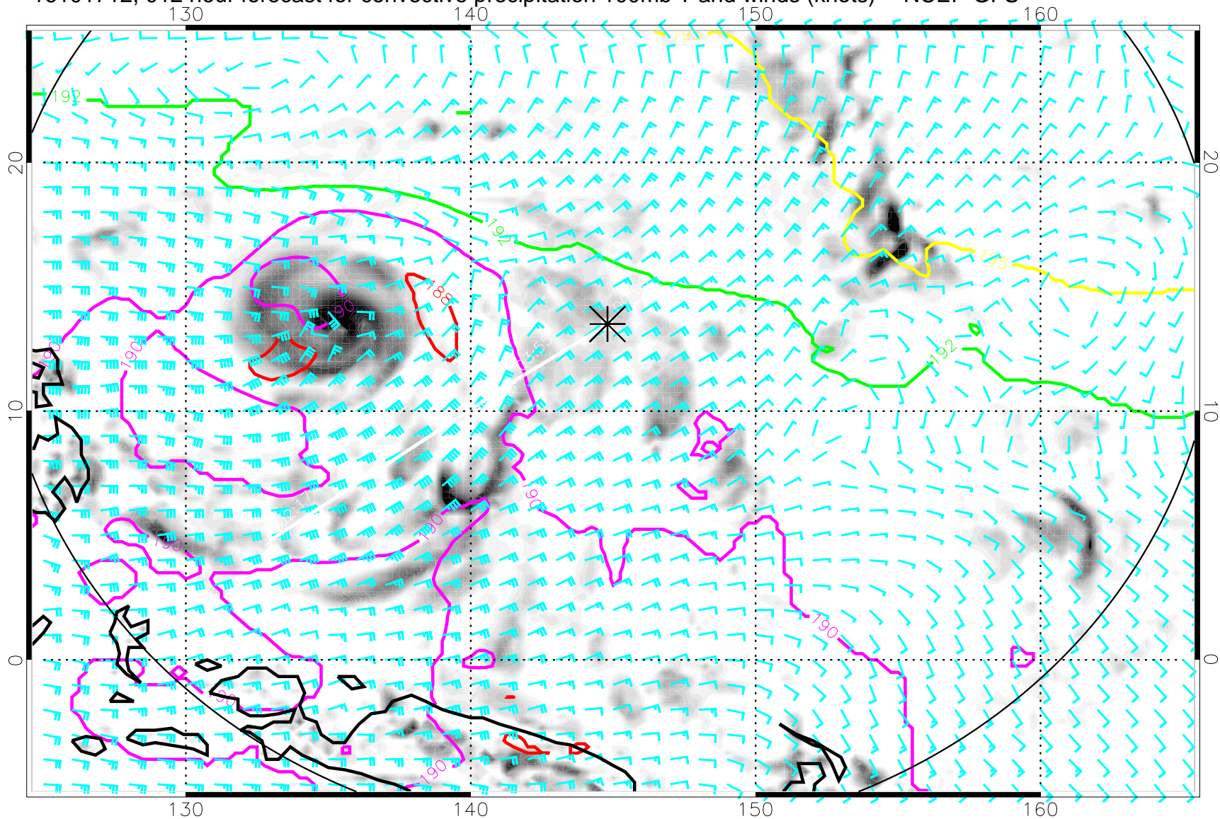
16101712, 012 hour forecast for convective precipitation 100mb T and winds (knots) -- NCEP GFS
