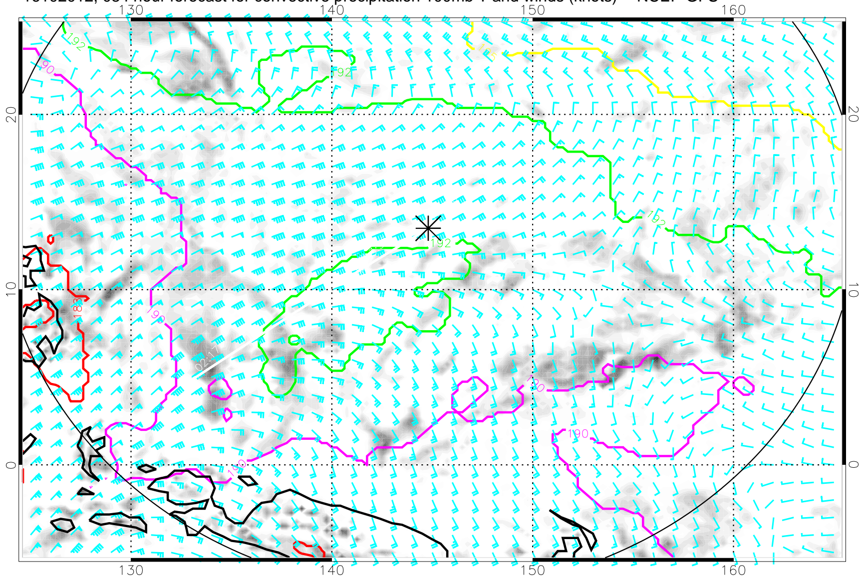
16102012, 084 hour forecast for convective precipitation 100mb T and winds (knots) -- NCEP GFS
