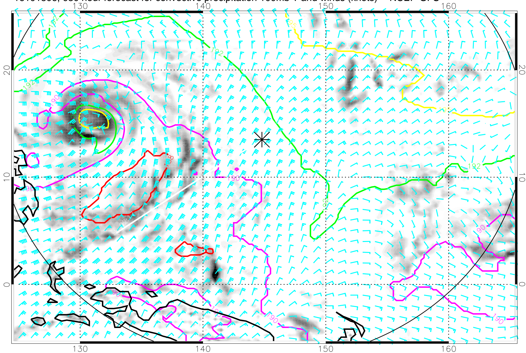
16101806, 030 hour forecast for convective precipitation 100mb T and winds (knots) -- NCEP GFS
