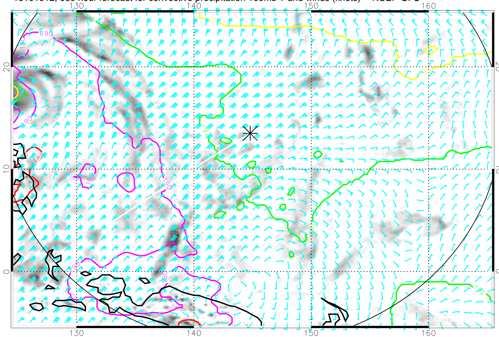
16101912, 060 hour forecast for convective precipitation 100mb T and winds (knots) -- NCEP GFS
