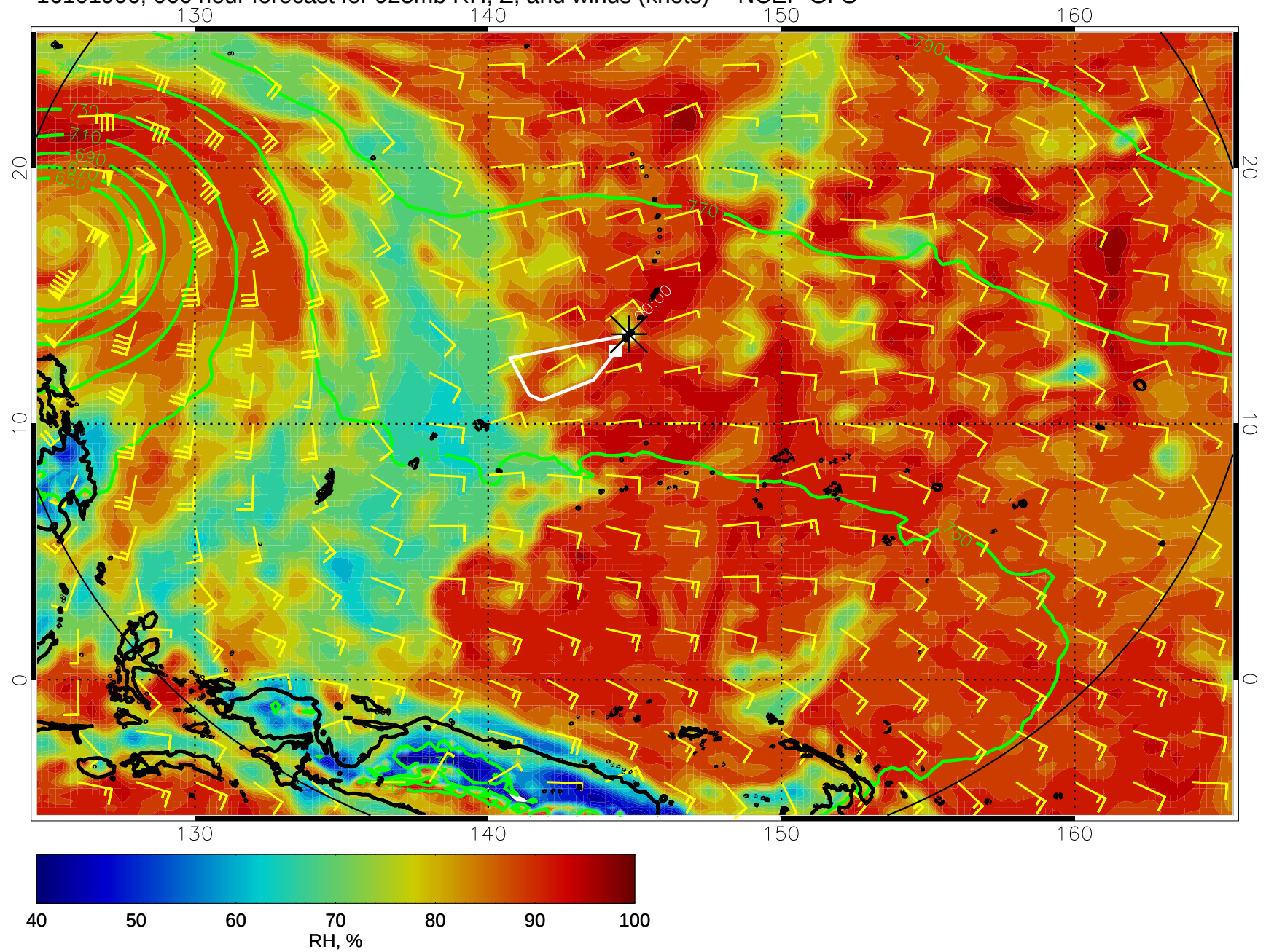
16101906, 066 hour forecast for 925mb RH, Z, and winds (knots) -- NCEP GFS
