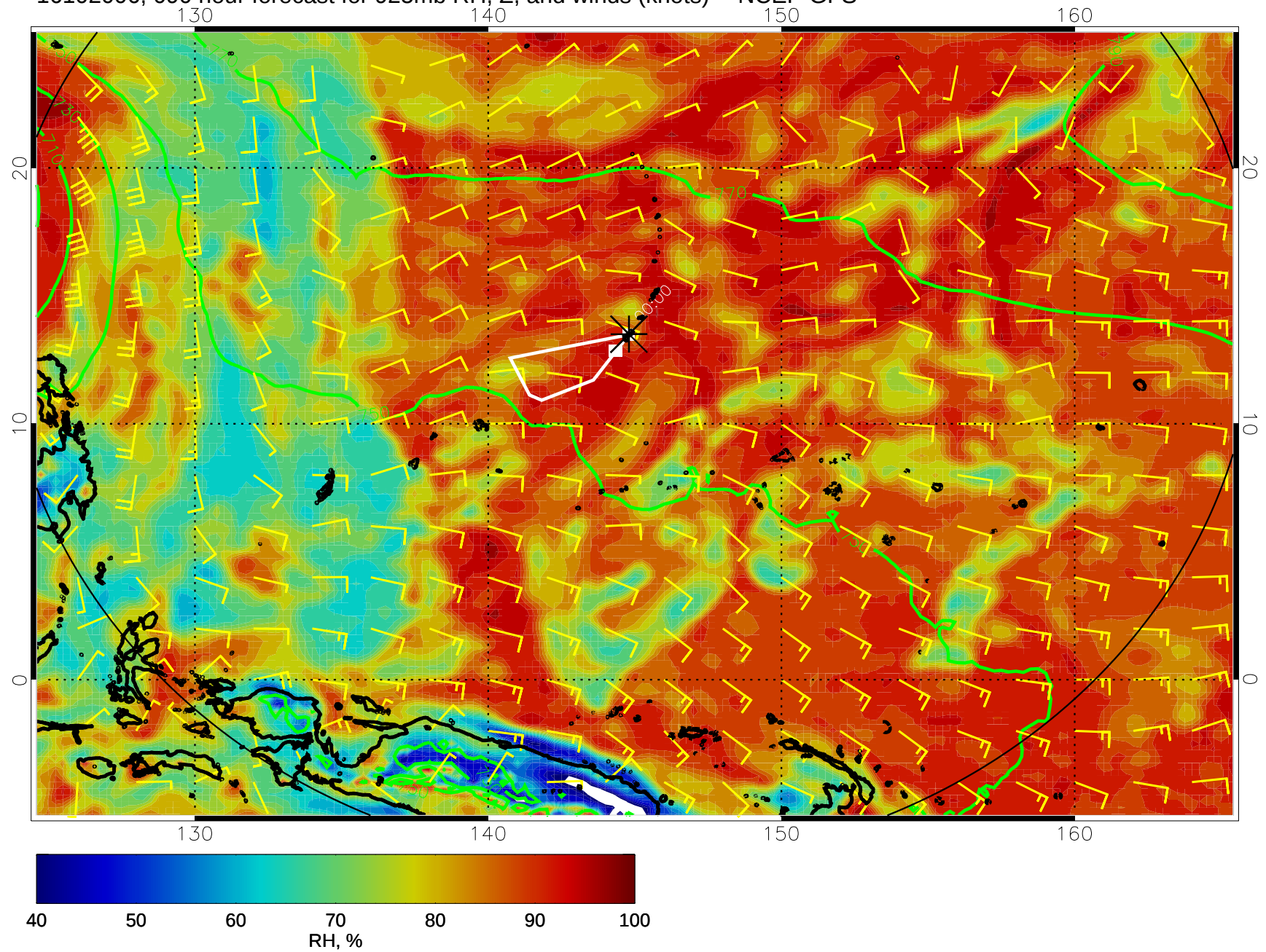
16102006, 090 hour forecast for 925mb RH, Z, and winds (knots) -- NCEP GFS
