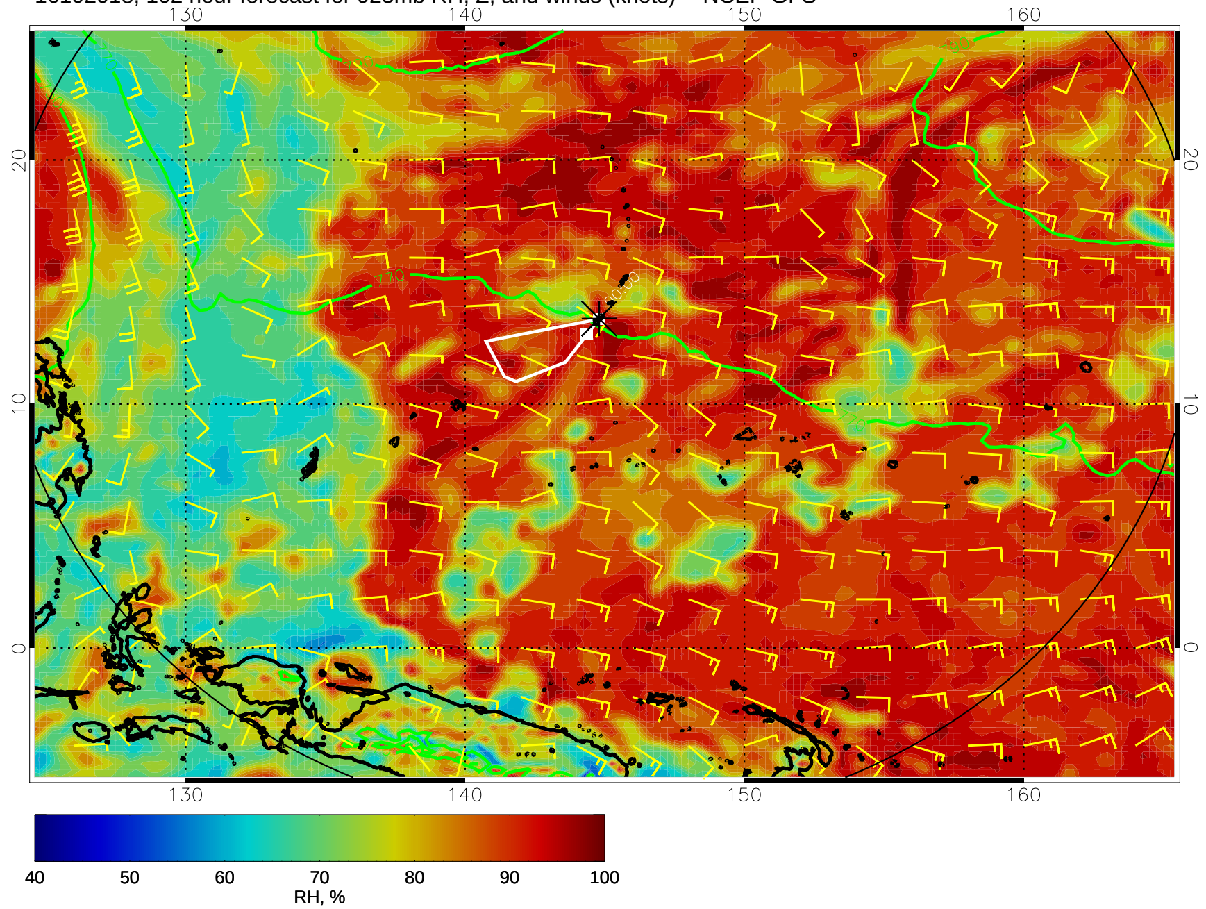
16102018, 102 hour forecast for 925mb RH, Z, and winds (knots) -- NCEP GFS
