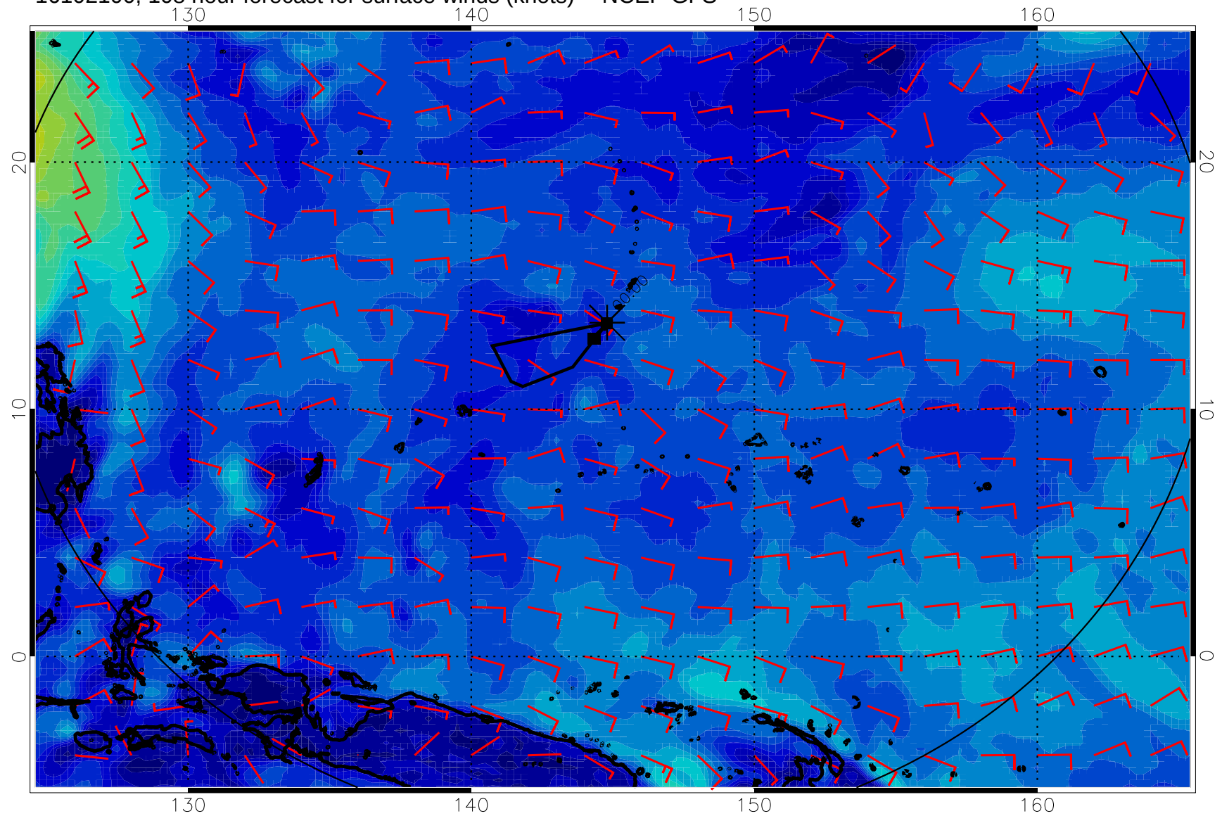
16102100, 108 hour forecast for surface winds (knots) -- NCEP GFS
