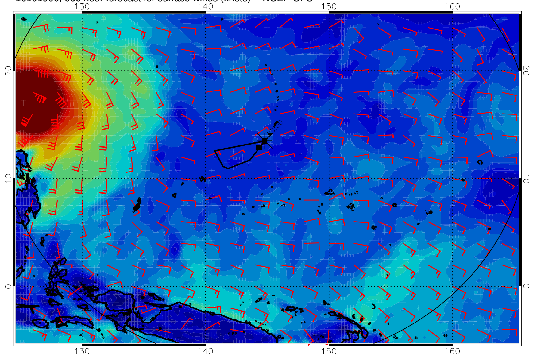
16101906, 066 hour forecast for surface winds (knots) -- NCEP GFS
