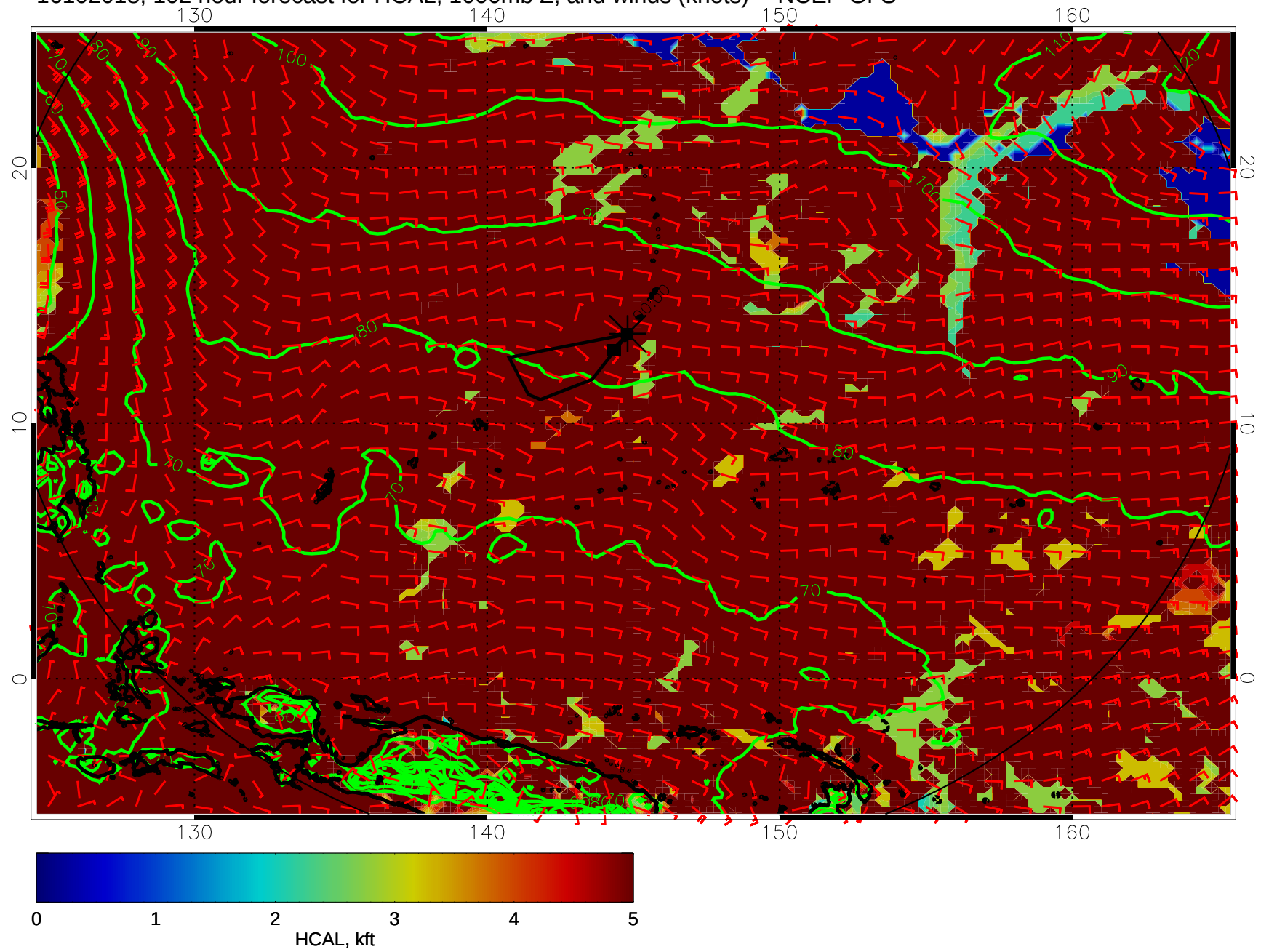
16102018, 102 hour forecast for HCAL, 1000mb Z, and winds (knots) -- NCEP GFS
