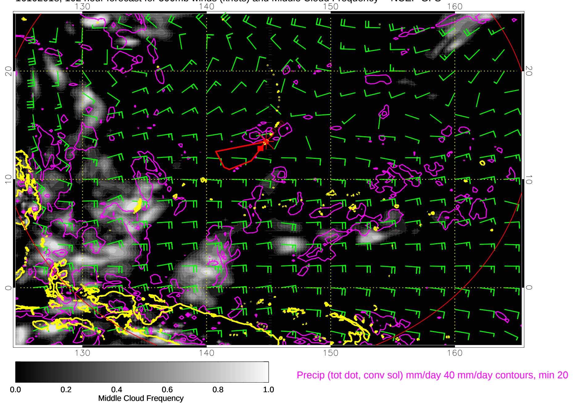
16102018, 102 hour forecast for 500mb winds (knots) and Middle Cloud Frequency -- NCEP GFS
