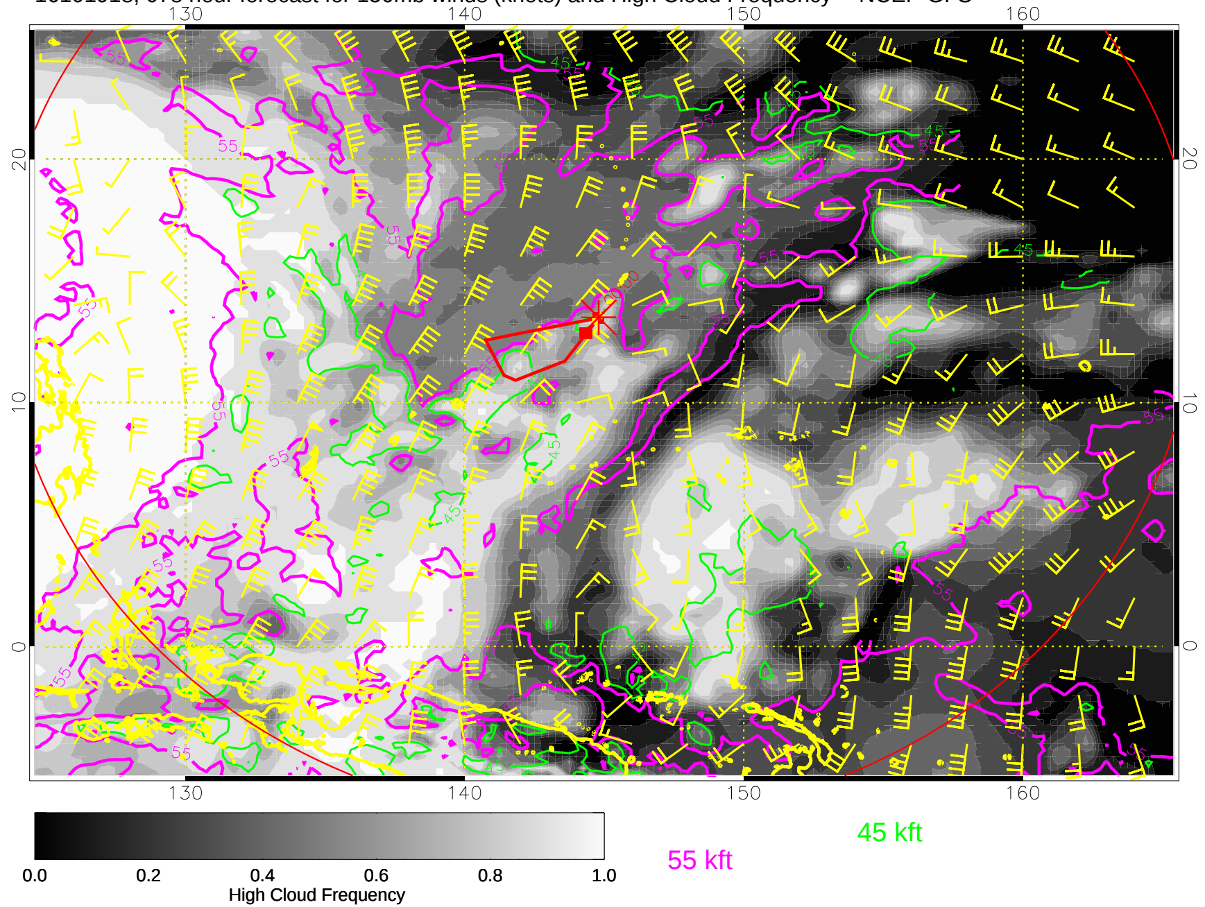
16101918, 078 hour forecast for 150mb winds (knots) and High Cloud Frequency -- NCEP GFS
