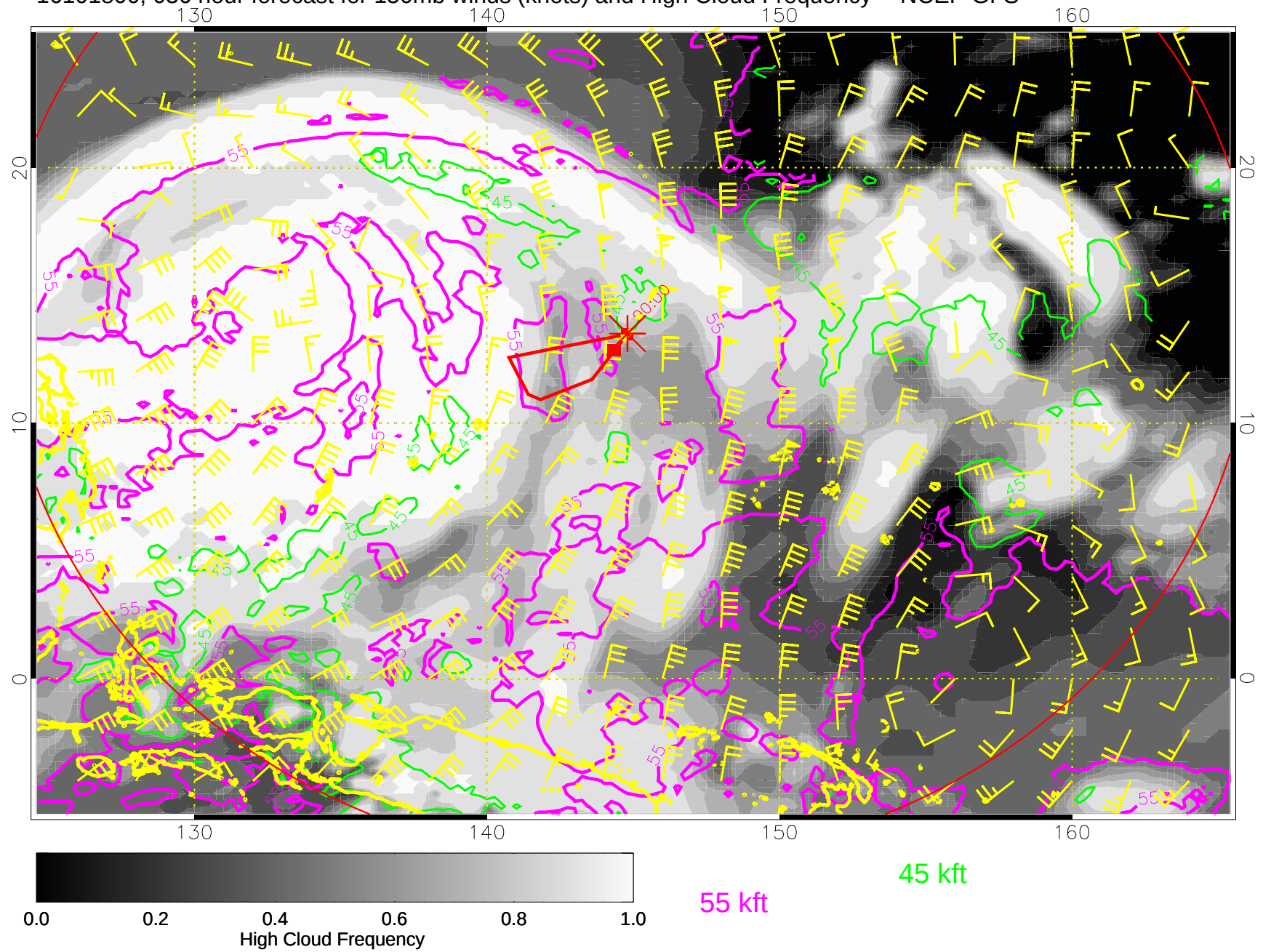
16101800, 036 hour forecast for 150mb winds (knots) and High Cloud Frequency -- NCEP GFS
