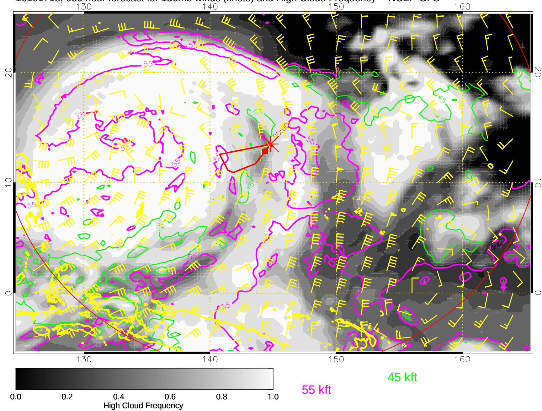
16101718, 0300 hour forecast for 150mb winds (knots) and High Cloud Frequency -- NCEP GFS
