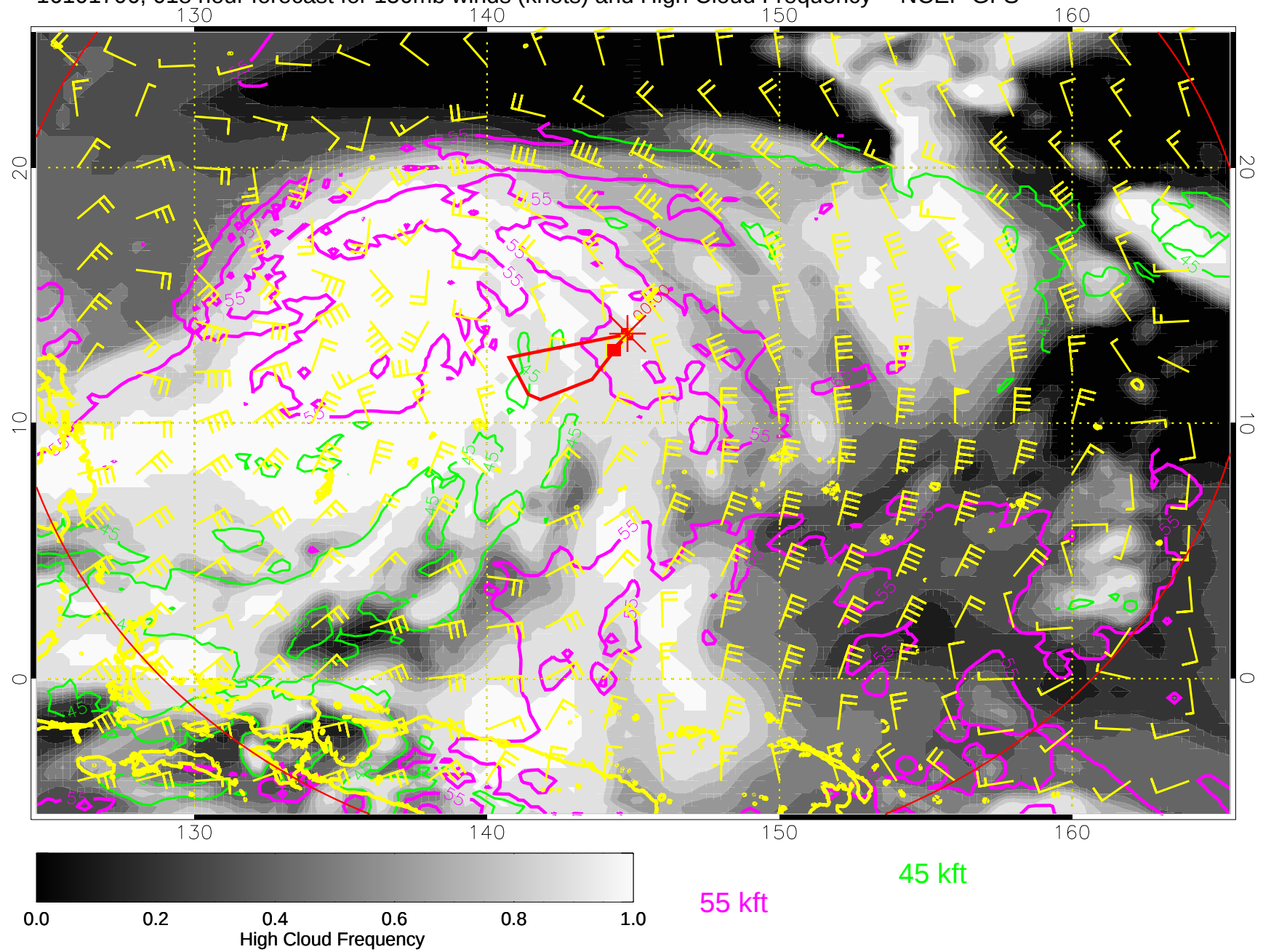
16101706, 018 hour forecast for 150mb winds (knots) and High Cloud Frequency -- NCEP GFS
