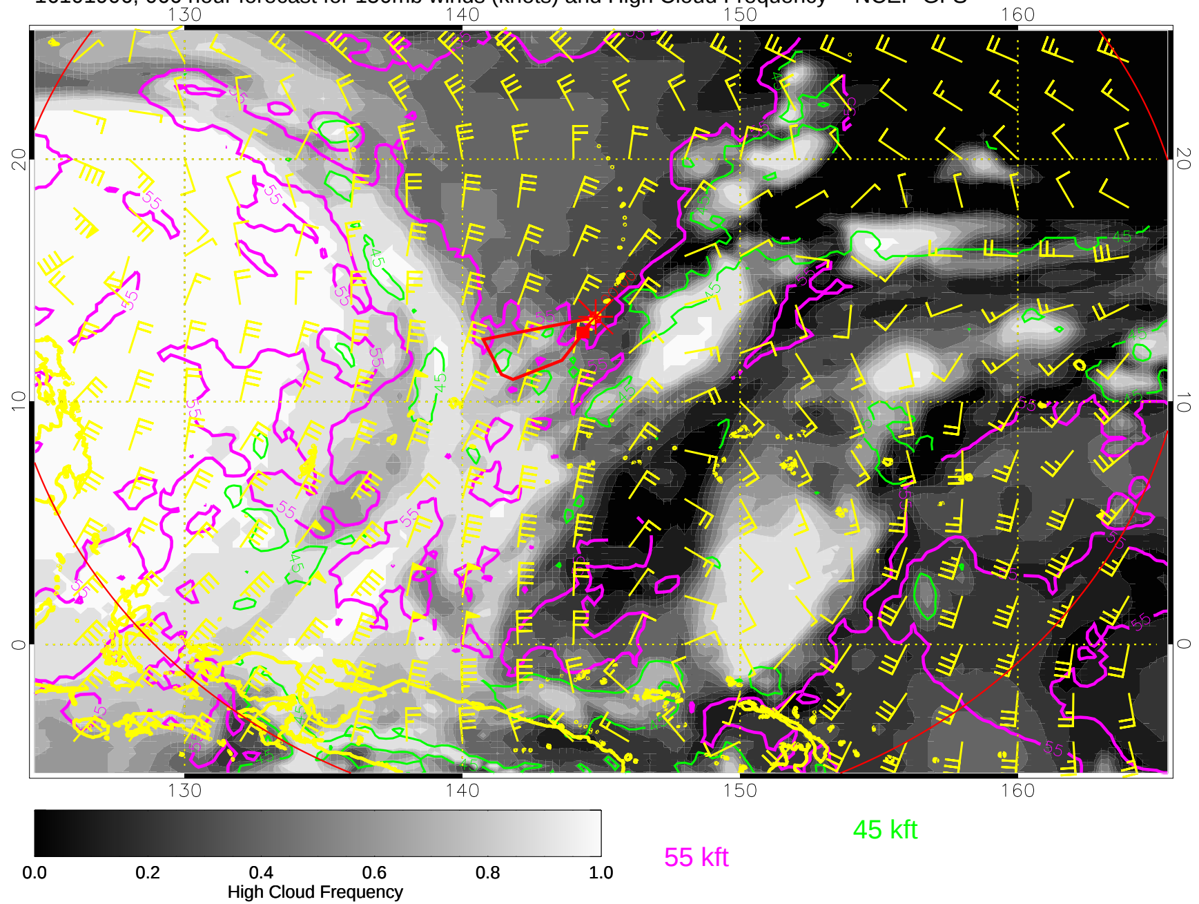
16101906, 066 hour forecast for 150mb winds (knots) and High Cloud Frequency -- NCEP GFS
