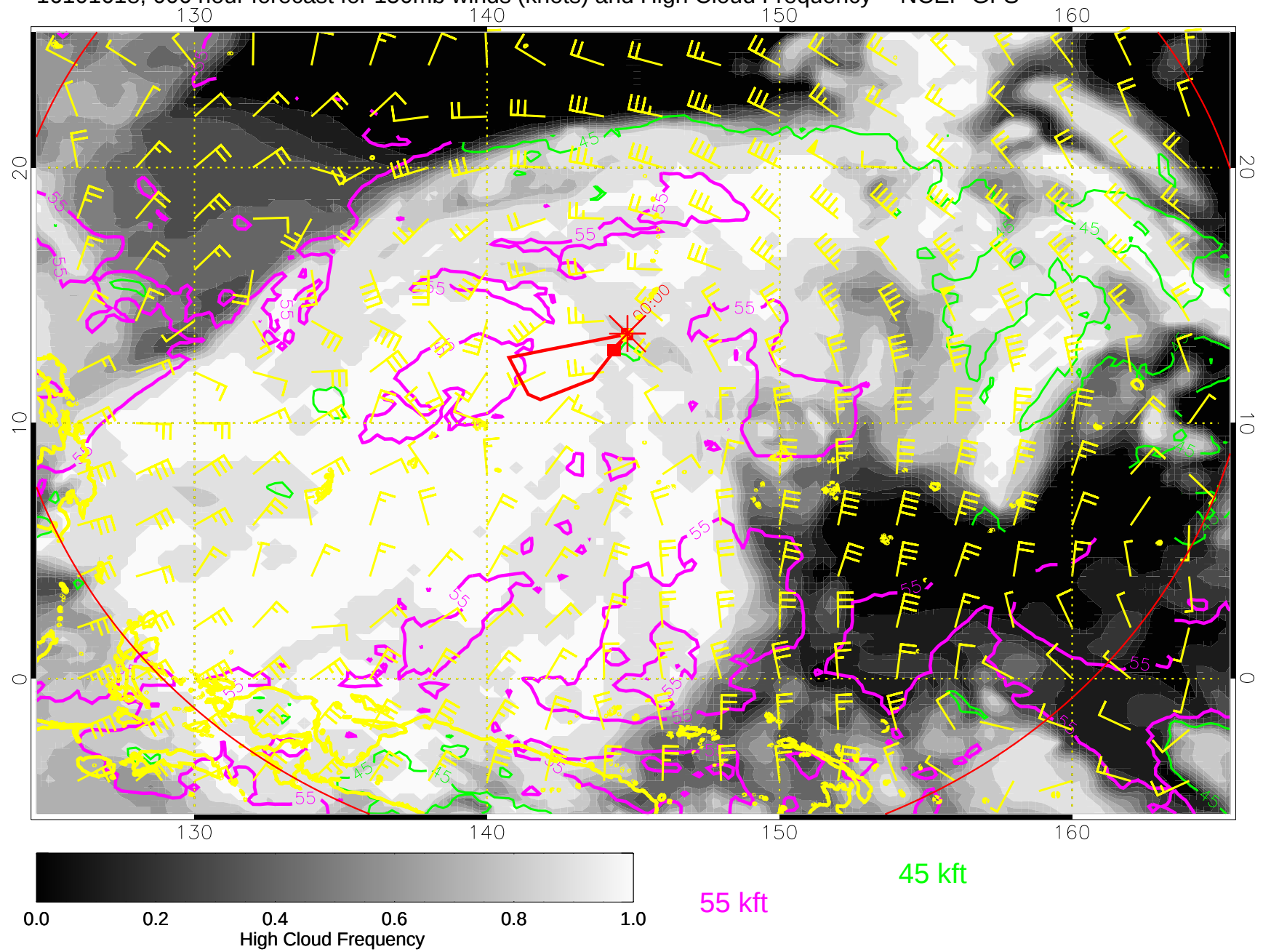
16101618, 006 hour forecast for 150mb winds (knots) and High Cloud Frequency -- NCEP GFS
