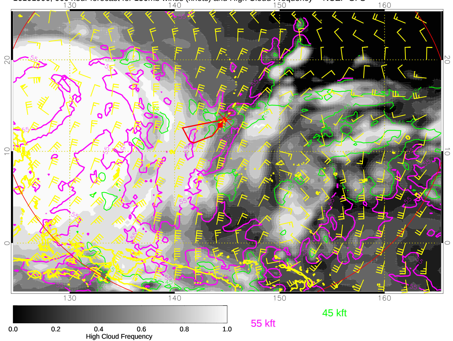
16101900, 060 hour forecast for 150mb winds (knots) and High Cloud Frequency -- NCEP GFS
