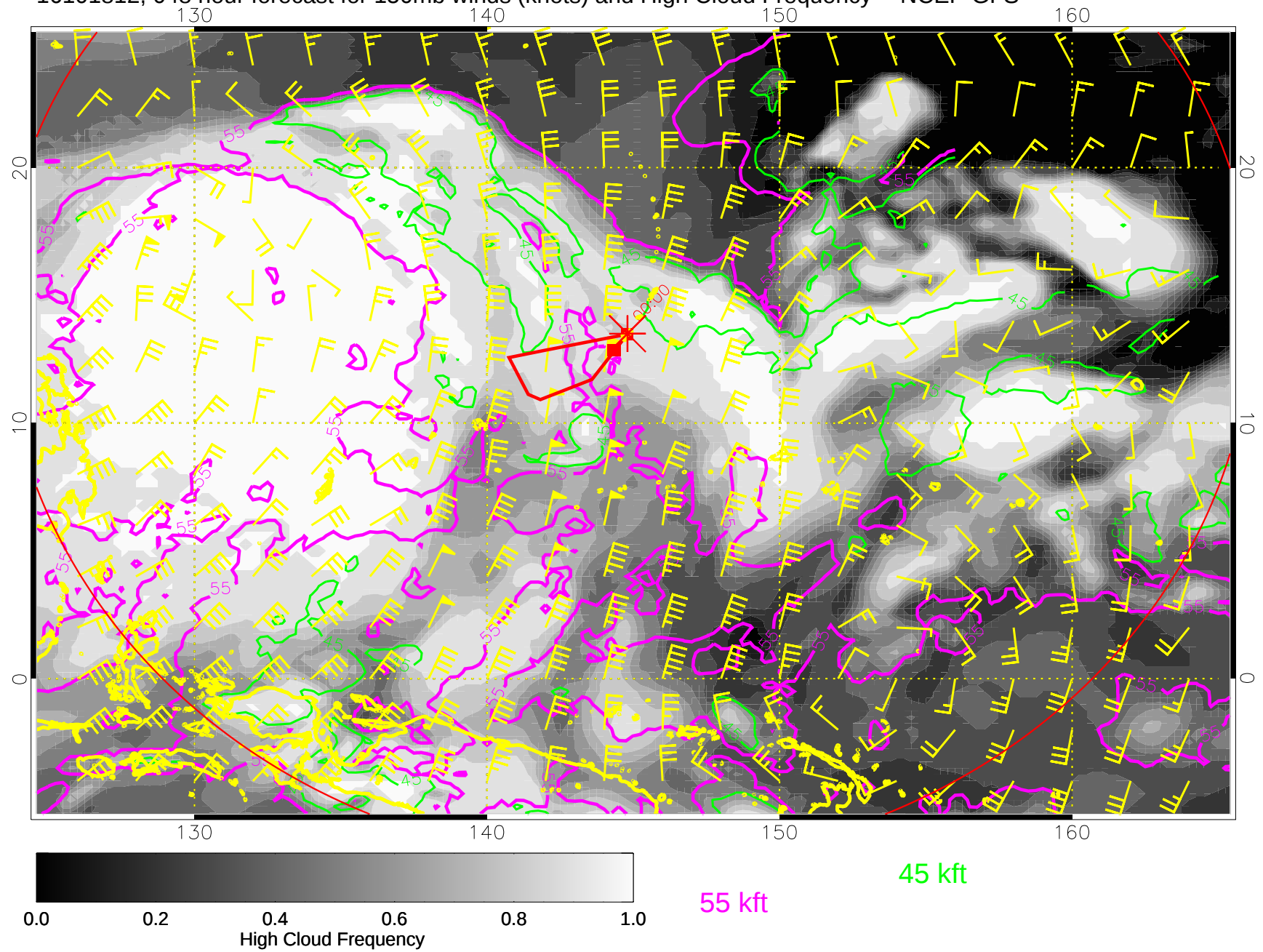
16101812, 048 hour forecast for 150mb winds (knots) and High Cloud Frequency -- NCEP GFS
