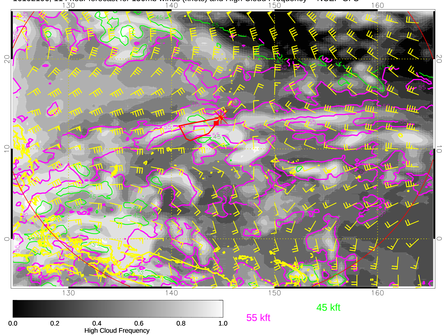
16102106, 114 hour forecast for 150mb winds (knots) and High Cloud Frequency -- NCEP GFS
