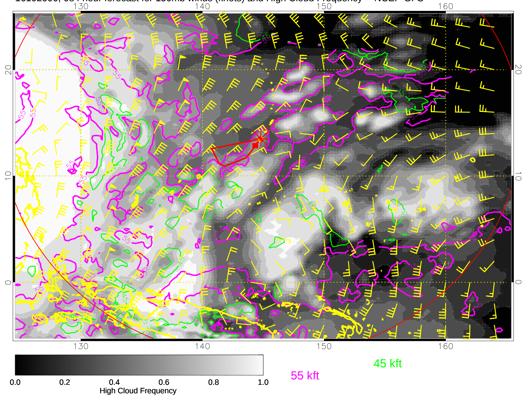
16102000, 084 hour forecast for 150mb winds (knots) and High Cloud Frequency -- NCEP GFS
