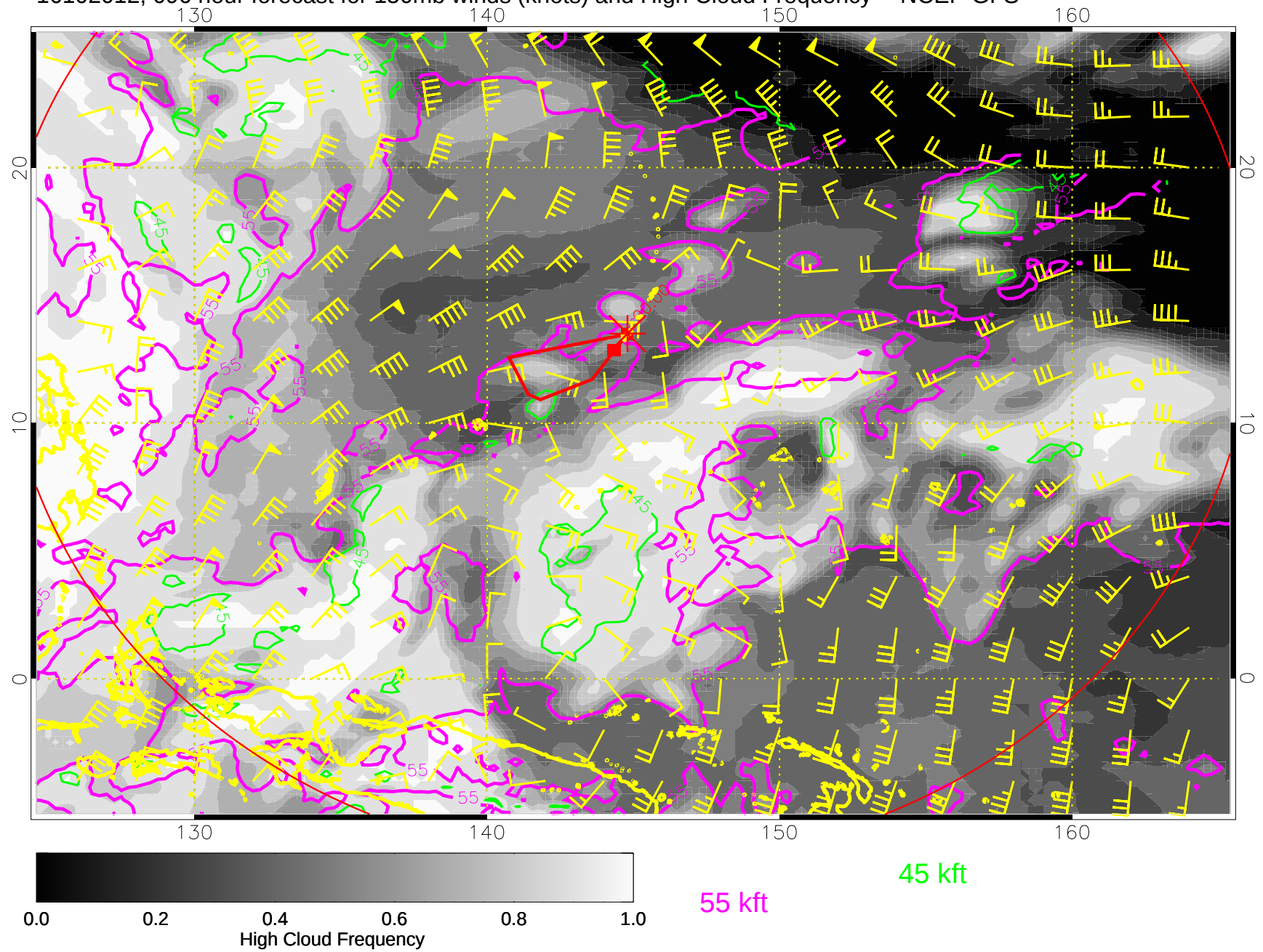
16102012, 096 hour forecast for 150mb winds (knots) and High Cloud Frequency -- NCEP GFS
