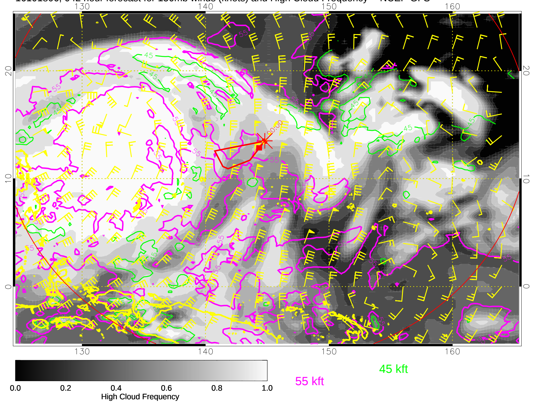
16101806, 042 hour forecast for 150mb winds (knots) and High Cloud Frequency -- NCEP GFS
