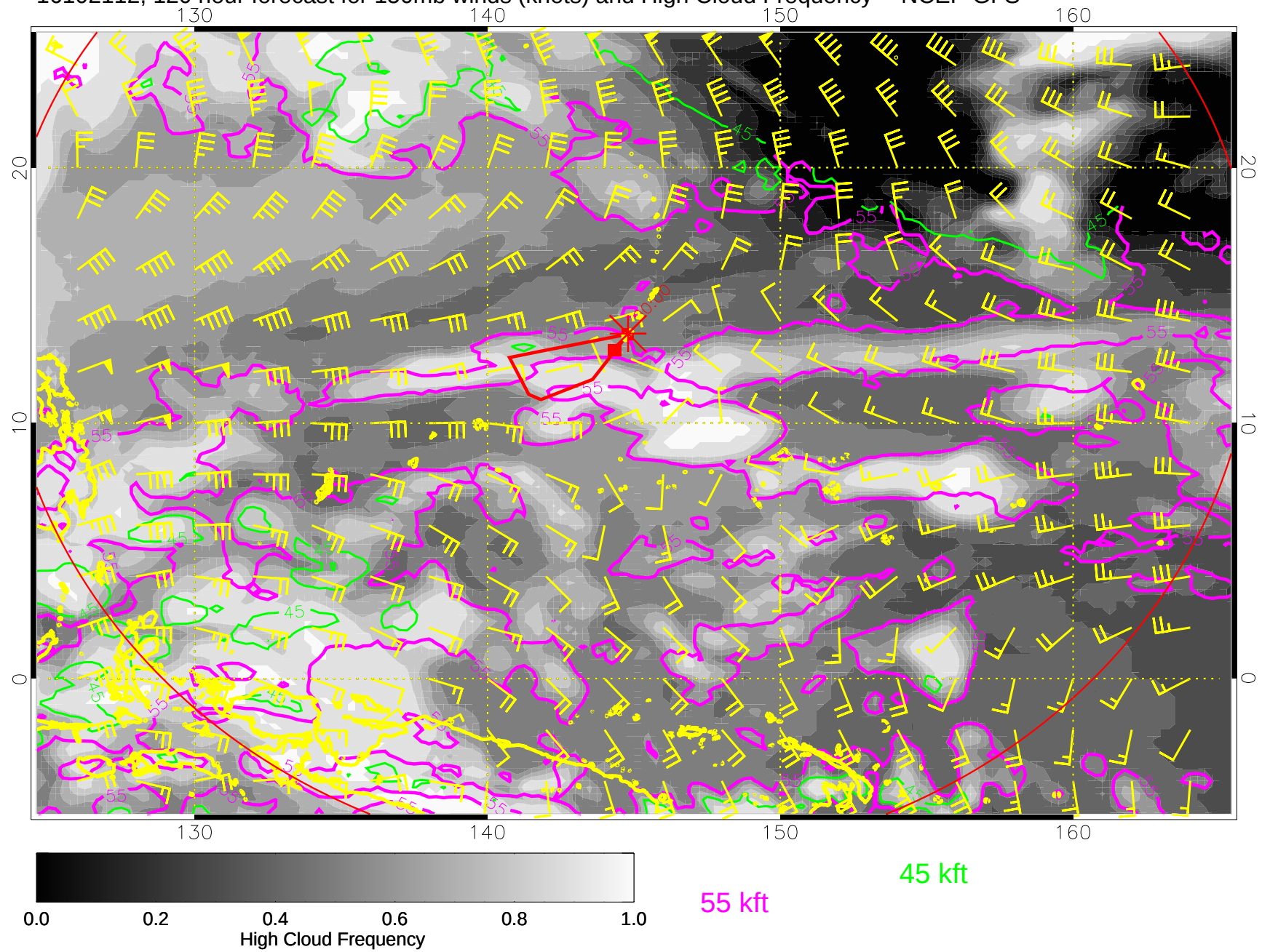
16102112, 120 hour forecast for 150mb winds (knots) and High Cloud Frequency -- NCEP GFS
