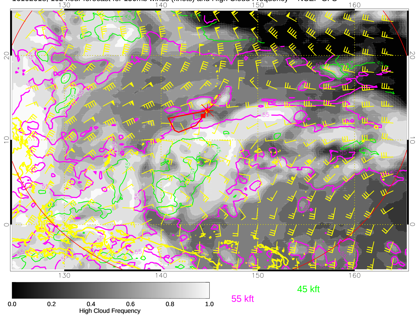
16102018, 102 hour forecast for 150mb winds (knots) and High Cloud Frequency -- NCEP GFS
