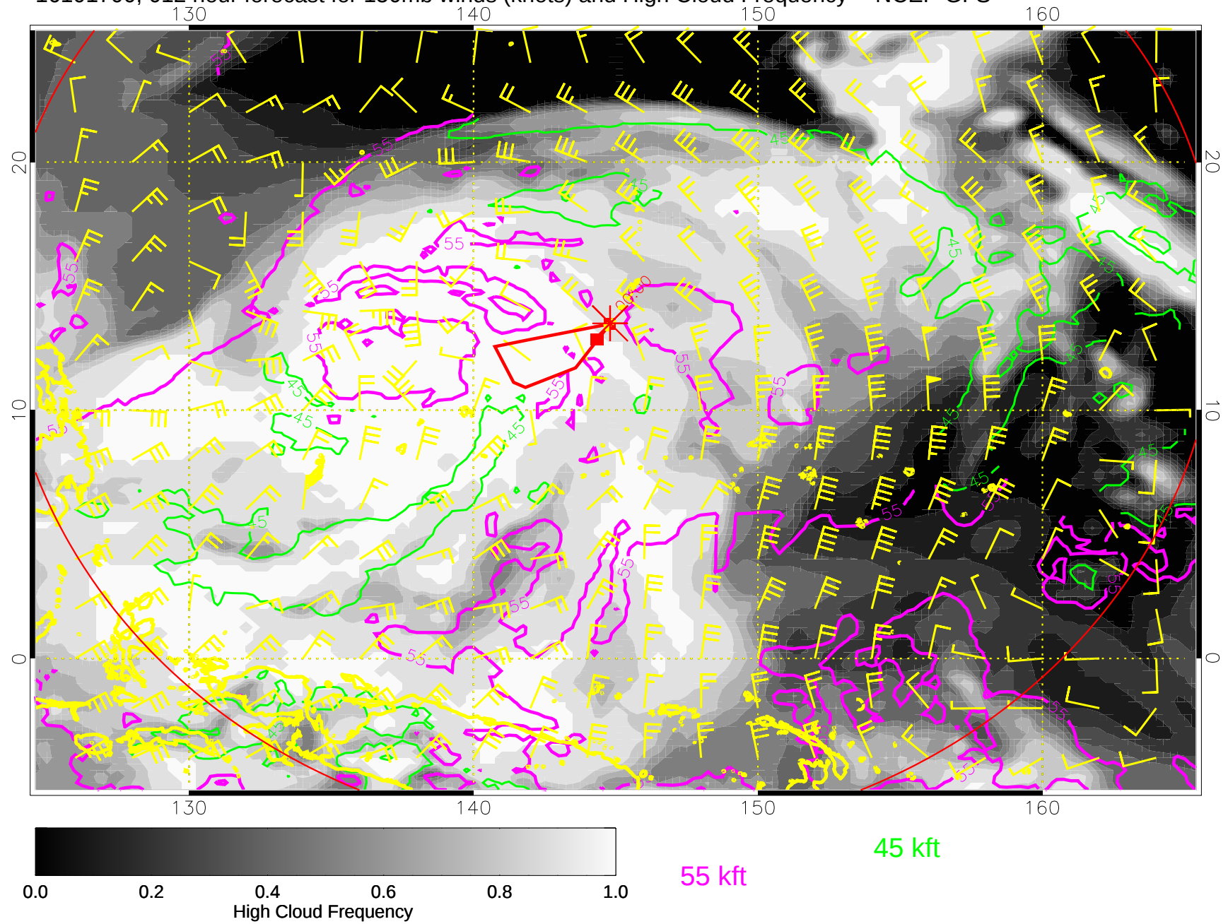
16101700, 012 hour forecast for 150mb winds (knots) and High Cloud Frequency -- NCEP GFS
