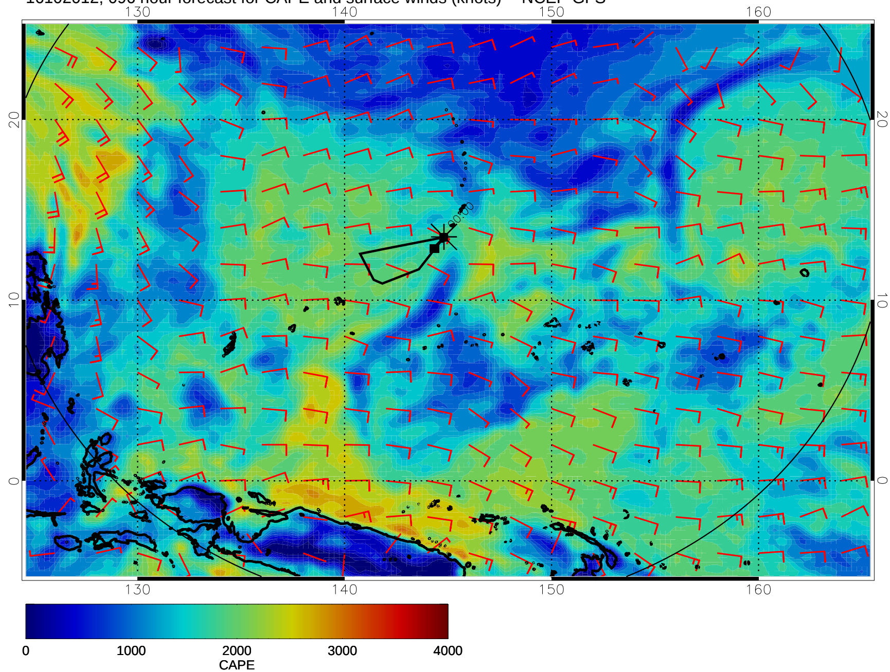
16102012, 096 hour forecast for CAPE and surface winds (knots) -- NCEP GFS
