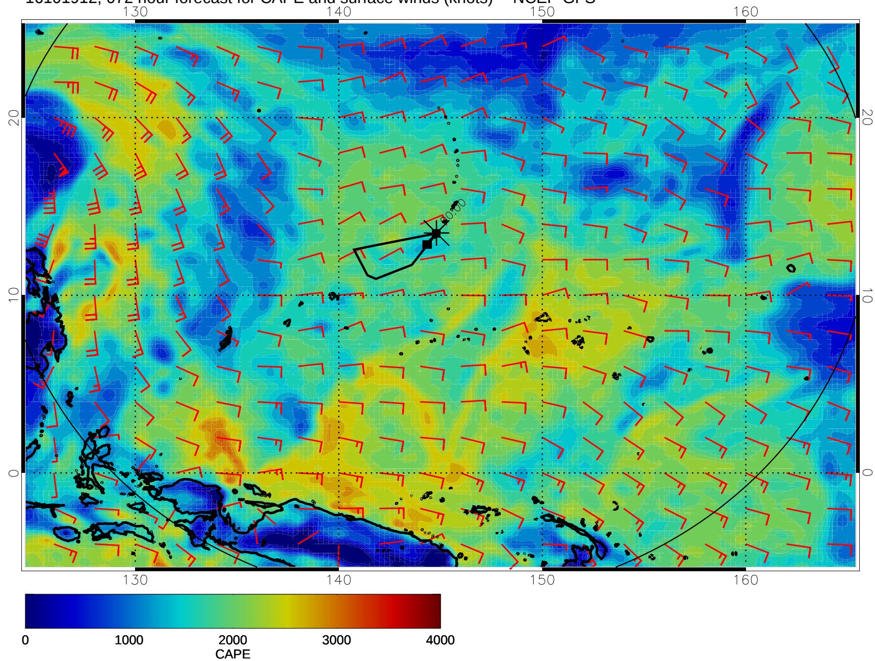
16101912, 072 hour forecast for CAPE and surface winds (knots) -- NCEP GFS
