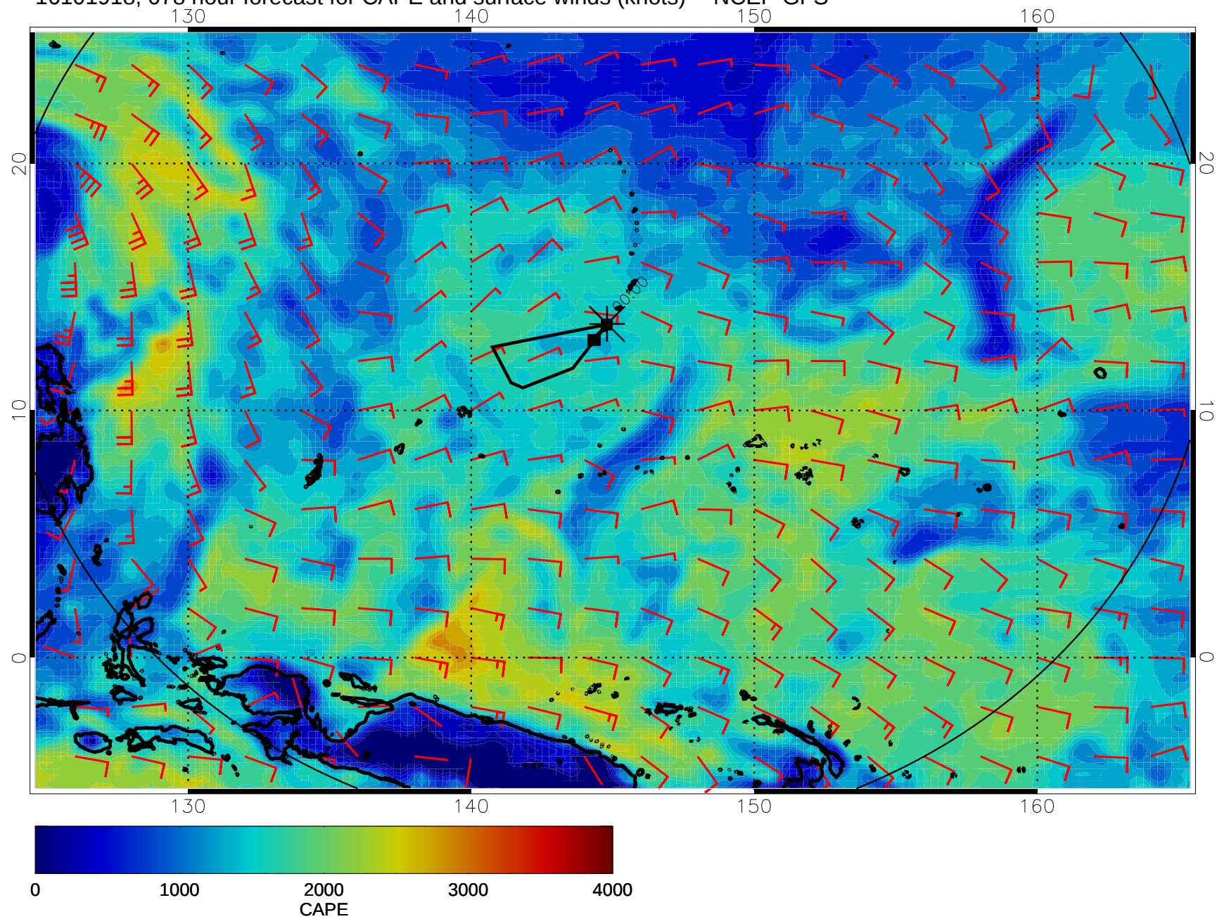
16101918, 078 hour forecast for CAPE and surface winds (knots) -- NCEP GFS
