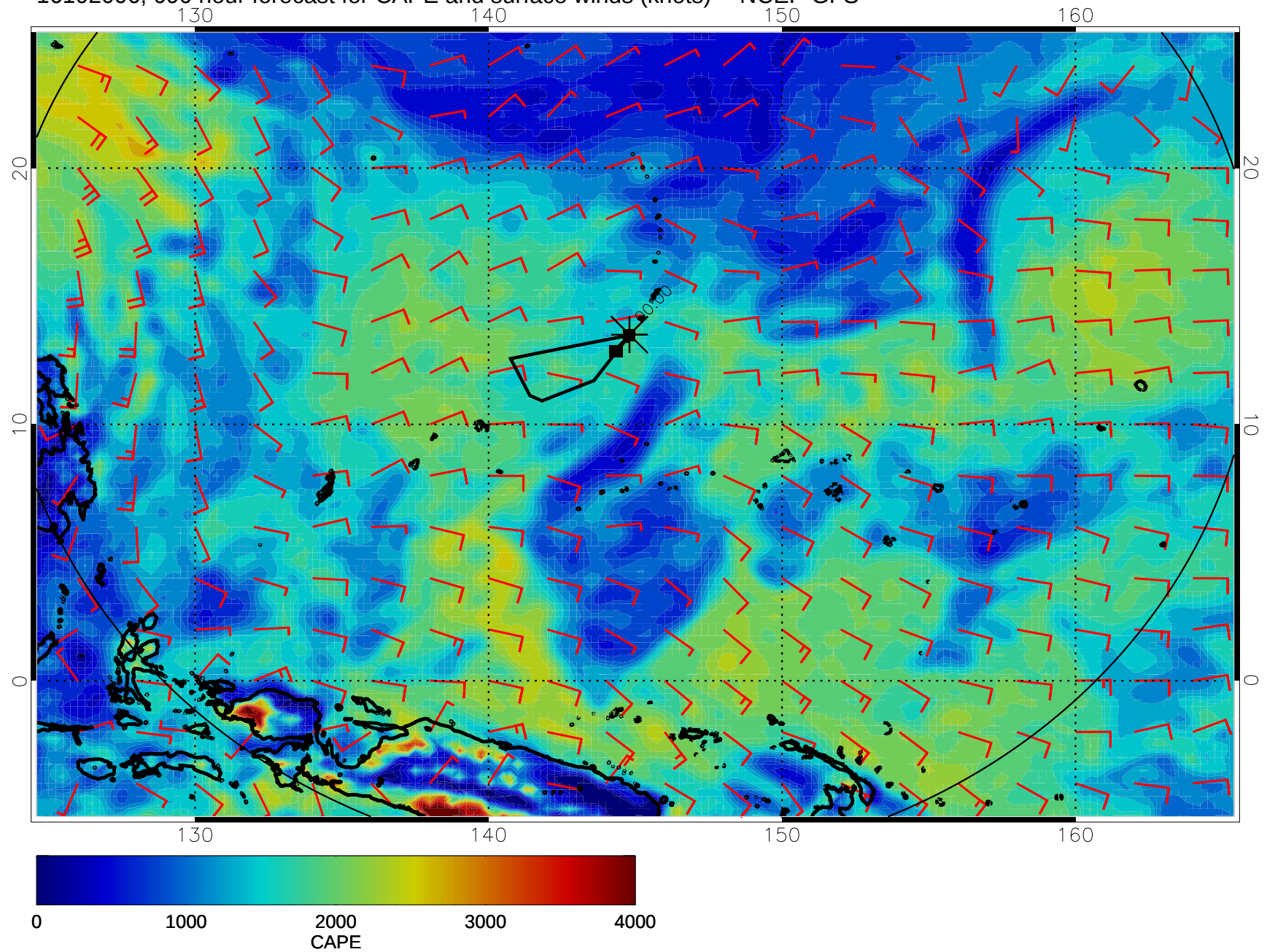
16102006, 0900 hour forecast for CAPE and surface winds (knots) -- NCEP GFS
