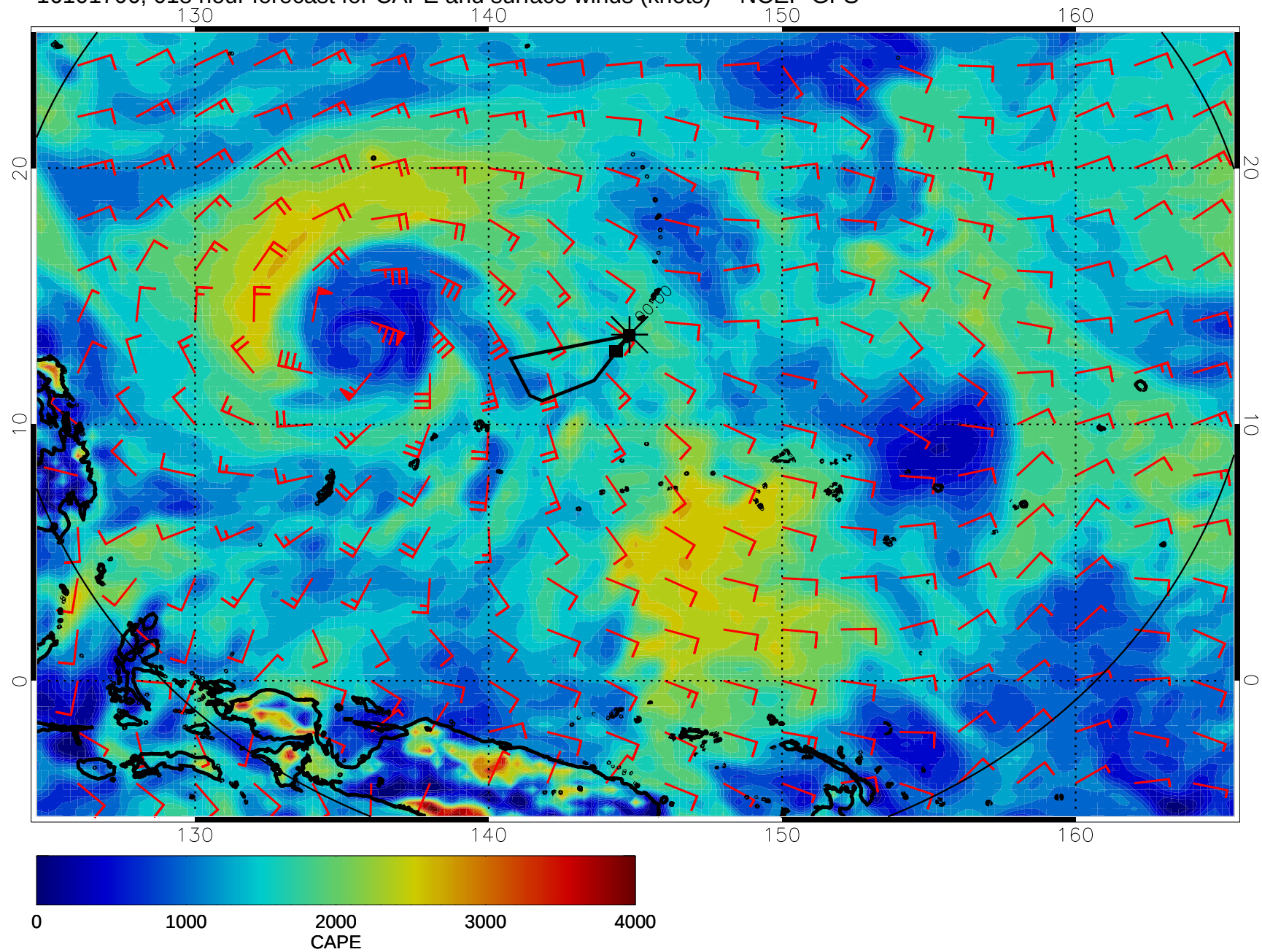
16101706, 018 hour forecast for CAPE and surface winds (knots) -- NCEP GFS
