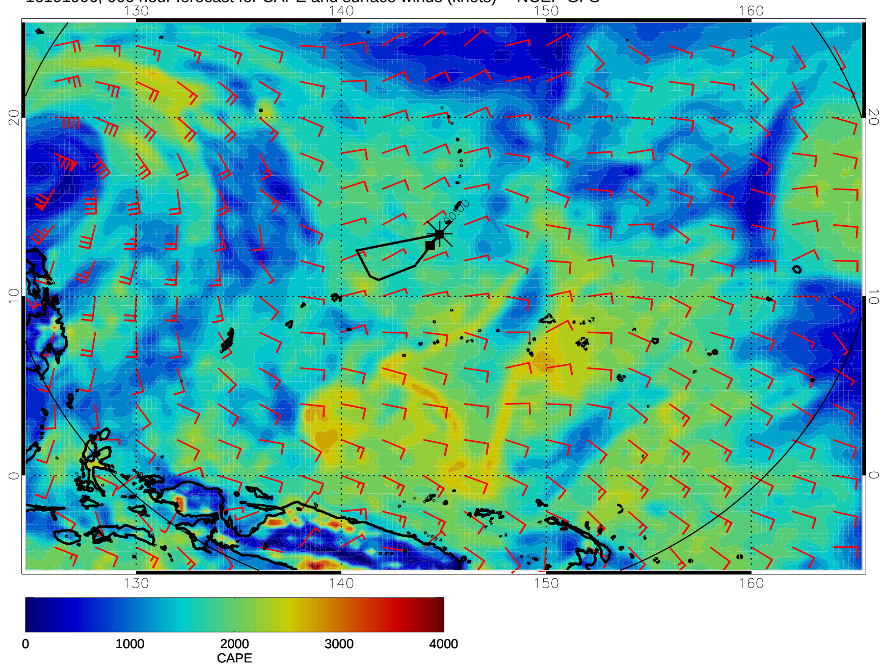
16101906, 066 hour forecast for CAPE and surface winds (knots) -- NCEP GFS
