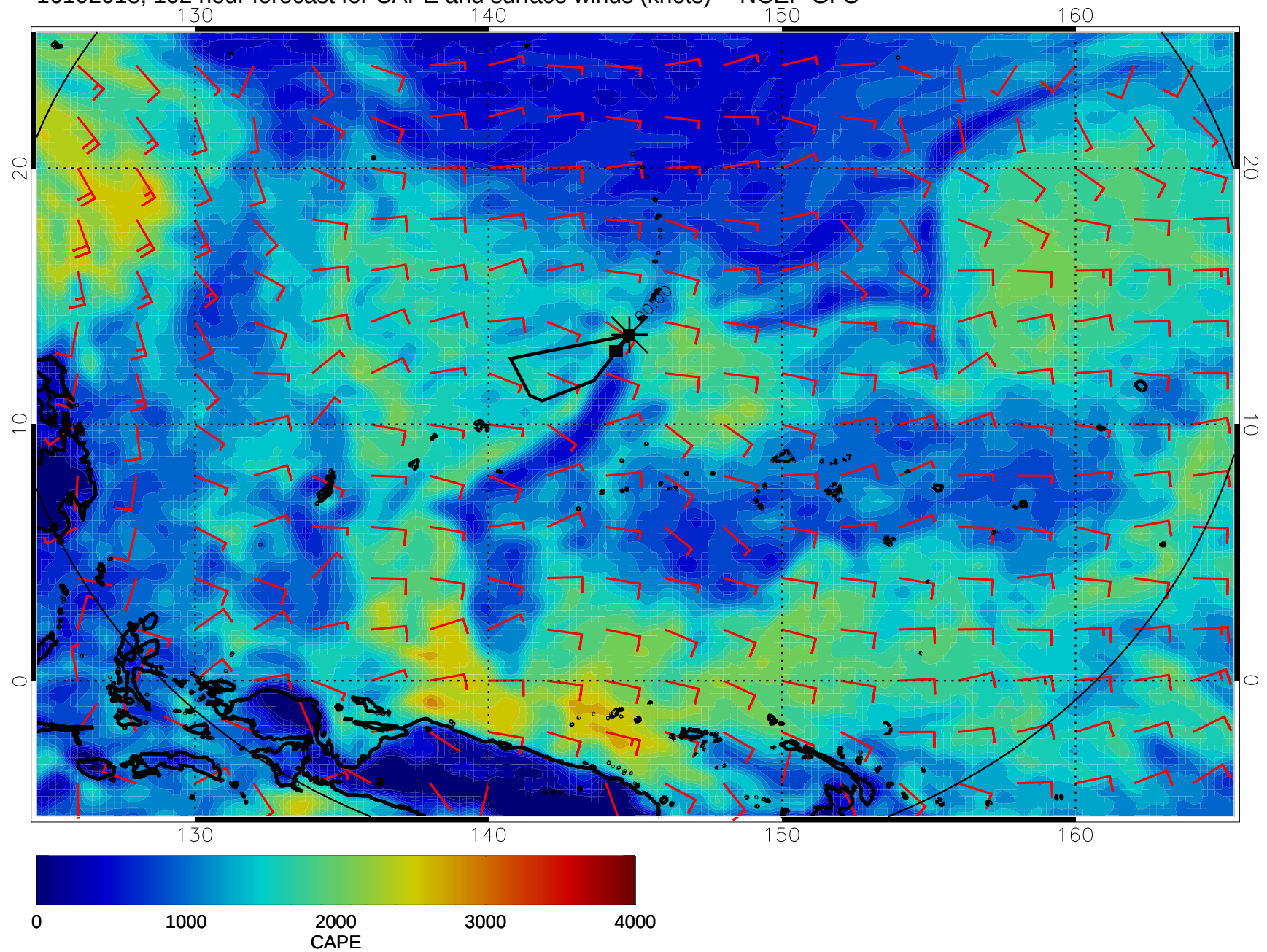
16102018, 102 hour forecast for CAPE and surface winds (knots) -- NCEP GFS
