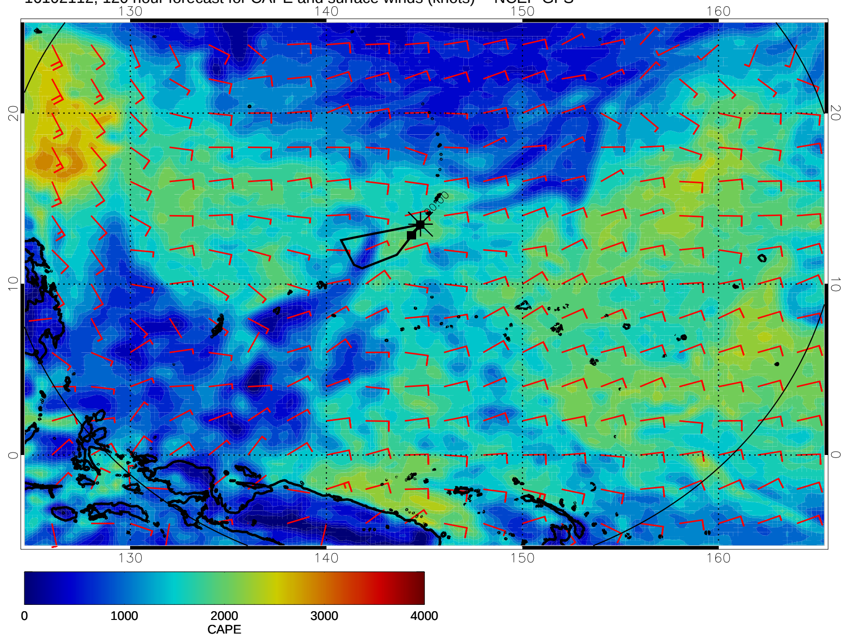
16102112, 120 hour forecast for CAPE and surface winds (knots) -- NCEP GFS
