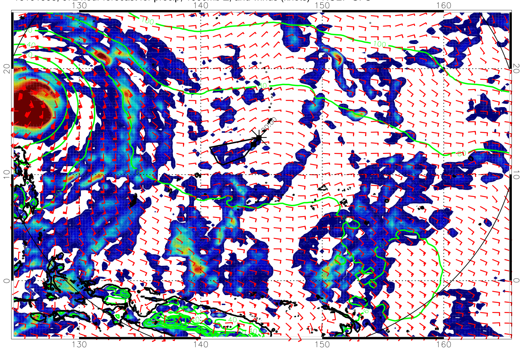
16101906, 072 hour forecast for precip, 1000mb Z, and winds (knots) -- NCEP GFS
