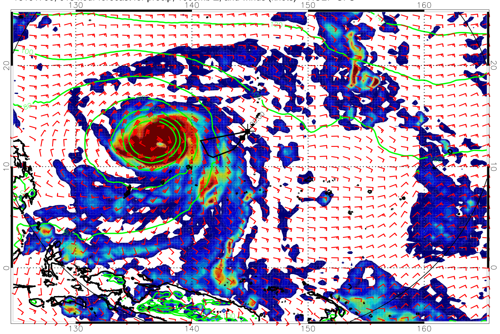
16101700, 018 hour forecast for precip, 1000mb Z, and winds (knots) -- NCEP GFS
