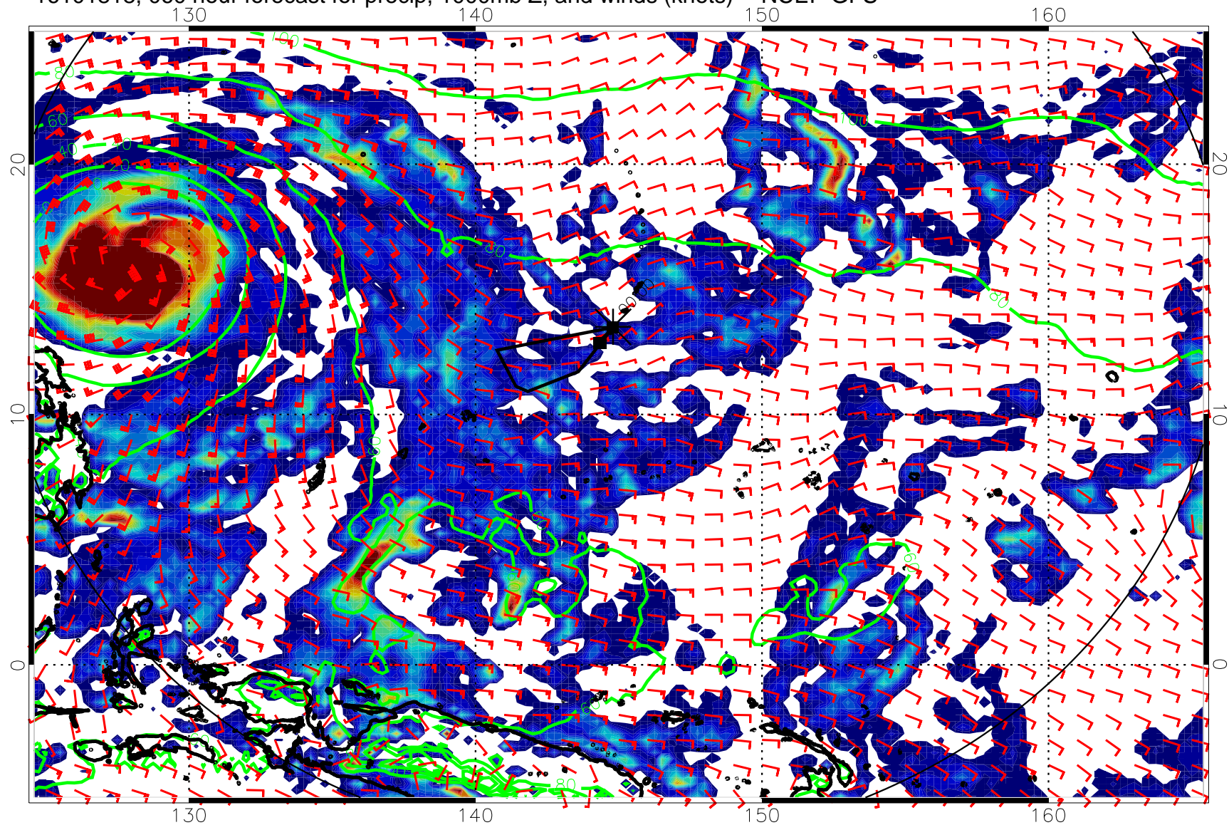
16101818, 060 hour forecast for precip, 1000mb Z, and winds (knots) -- NCEP GFS
