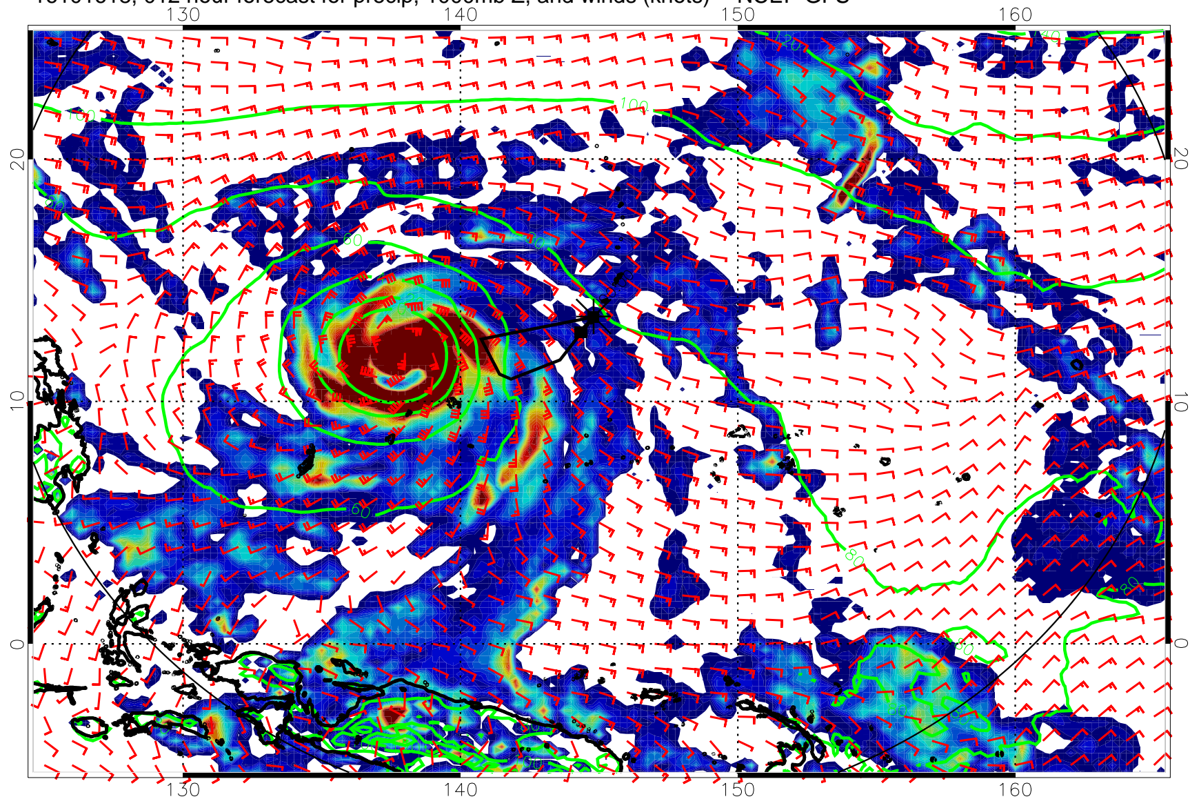
16101618, 012 hour forecast for precip, 1000mb Z, and winds (knots) -- NCEP GFS
