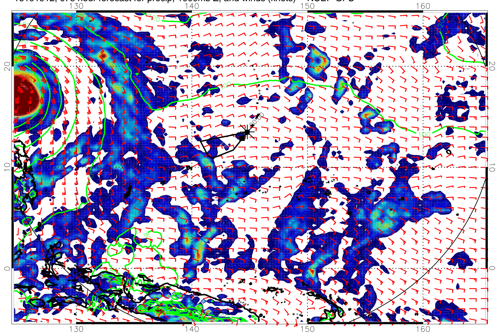
16101912, 078 hour forecast for precip, 1000mb Z, and winds (knots) -- NCEP GFS
