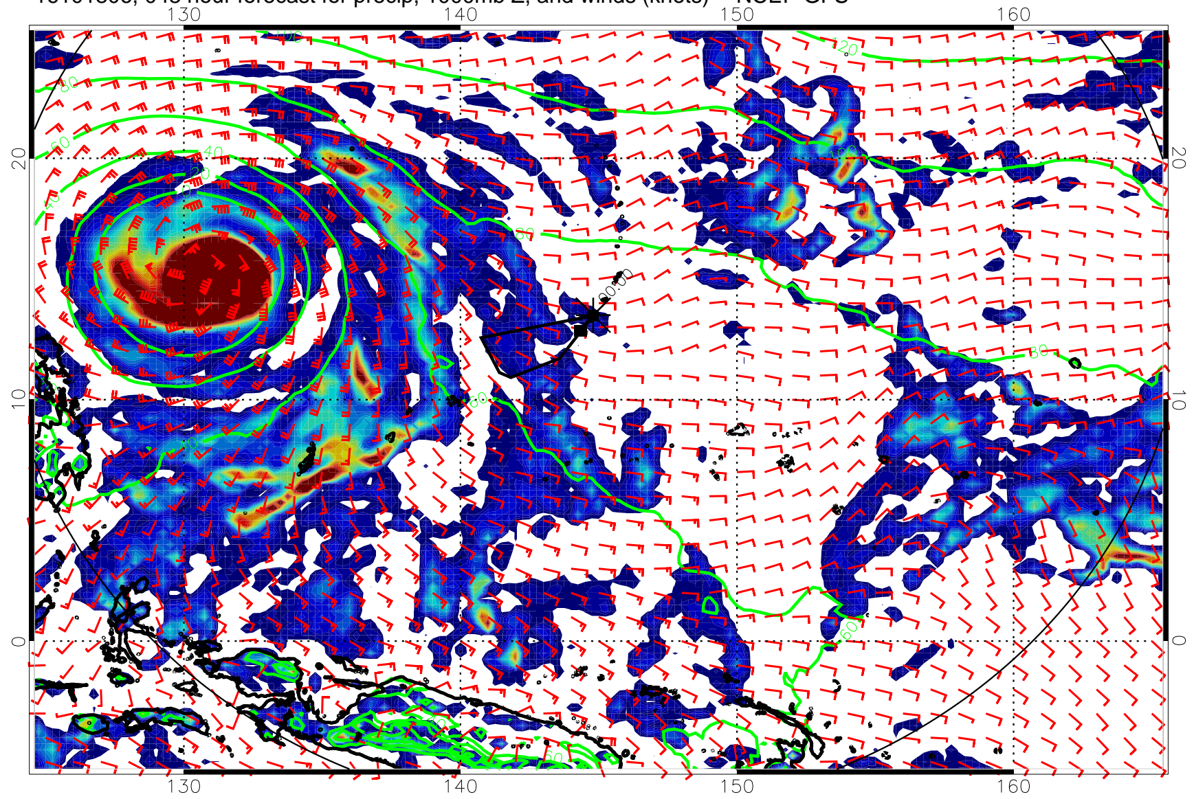
16101806, 048 hour forecast for precip, 1000mb Z, and winds (knots) -- NCEP GFS
