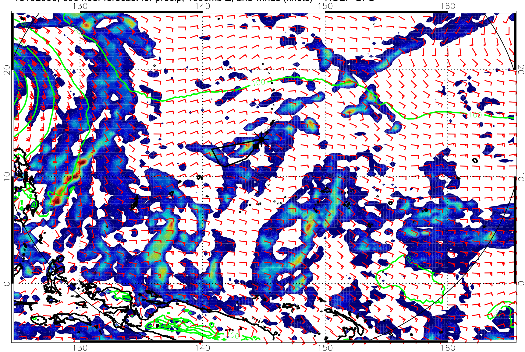
16102000, 090 hour forecast for precip, 1000mb Z, and winds (knots) -- NCEP GFS
