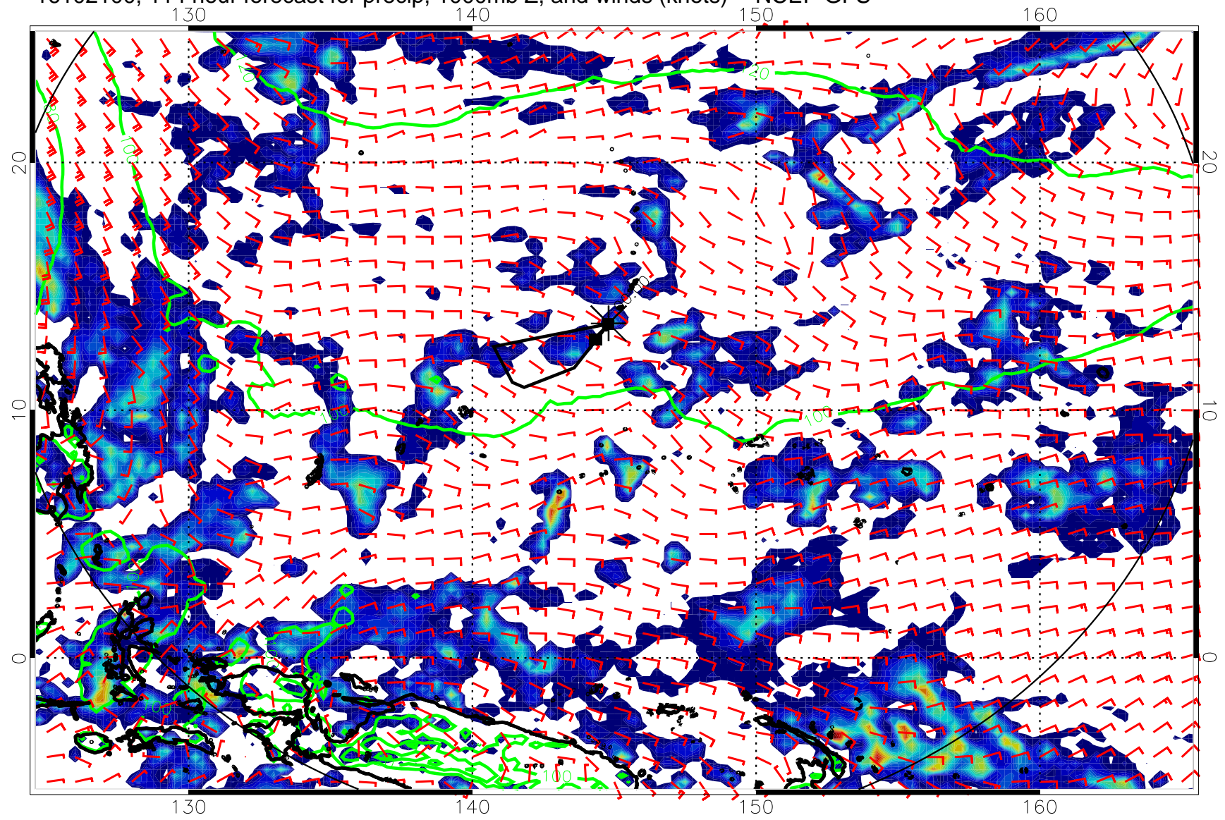
16102100, 114 hour forecast for precip, 1000mb Z, and winds (knots) -- NCEP GFS
