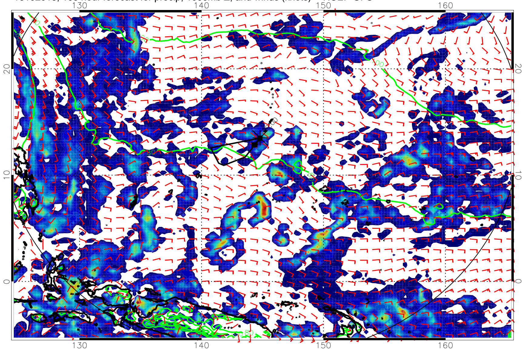
16102018, 108 hour forecast for precip, 1000mb Z, and winds (knots) -- NCEP GFS
