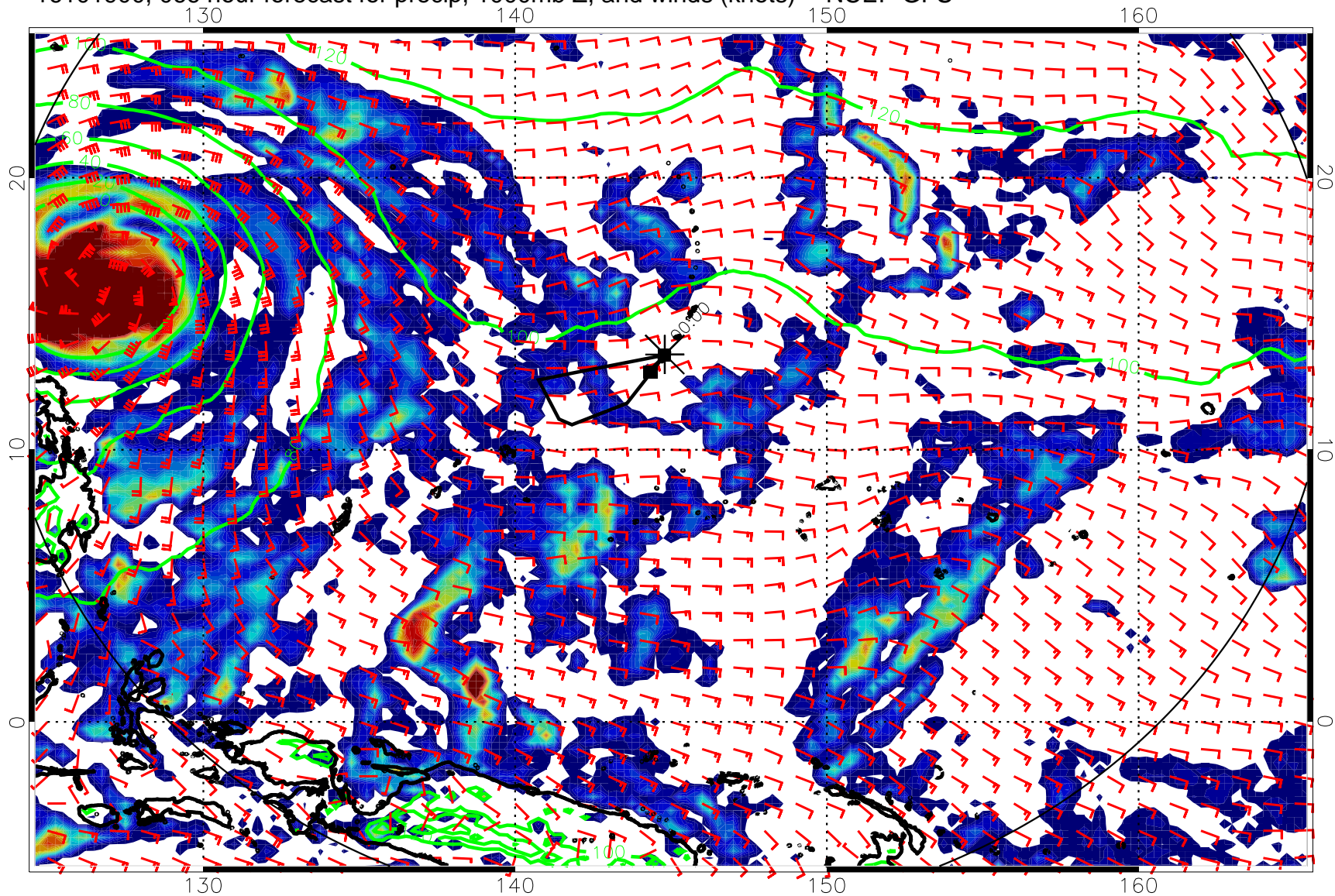
16101900, 066 hour forecast for precip, 1000mb Z, and winds (knots) -- NCEP GFS
