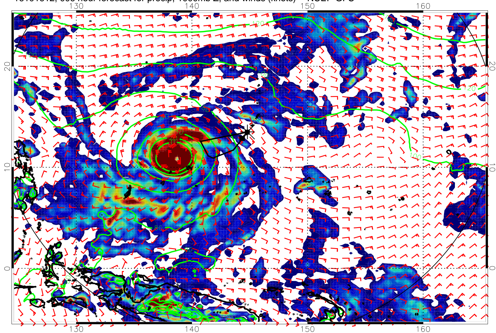
16101612, 006 hour forecast for precip, 1000mb Z, and winds (knots) -- NCEP GFS
