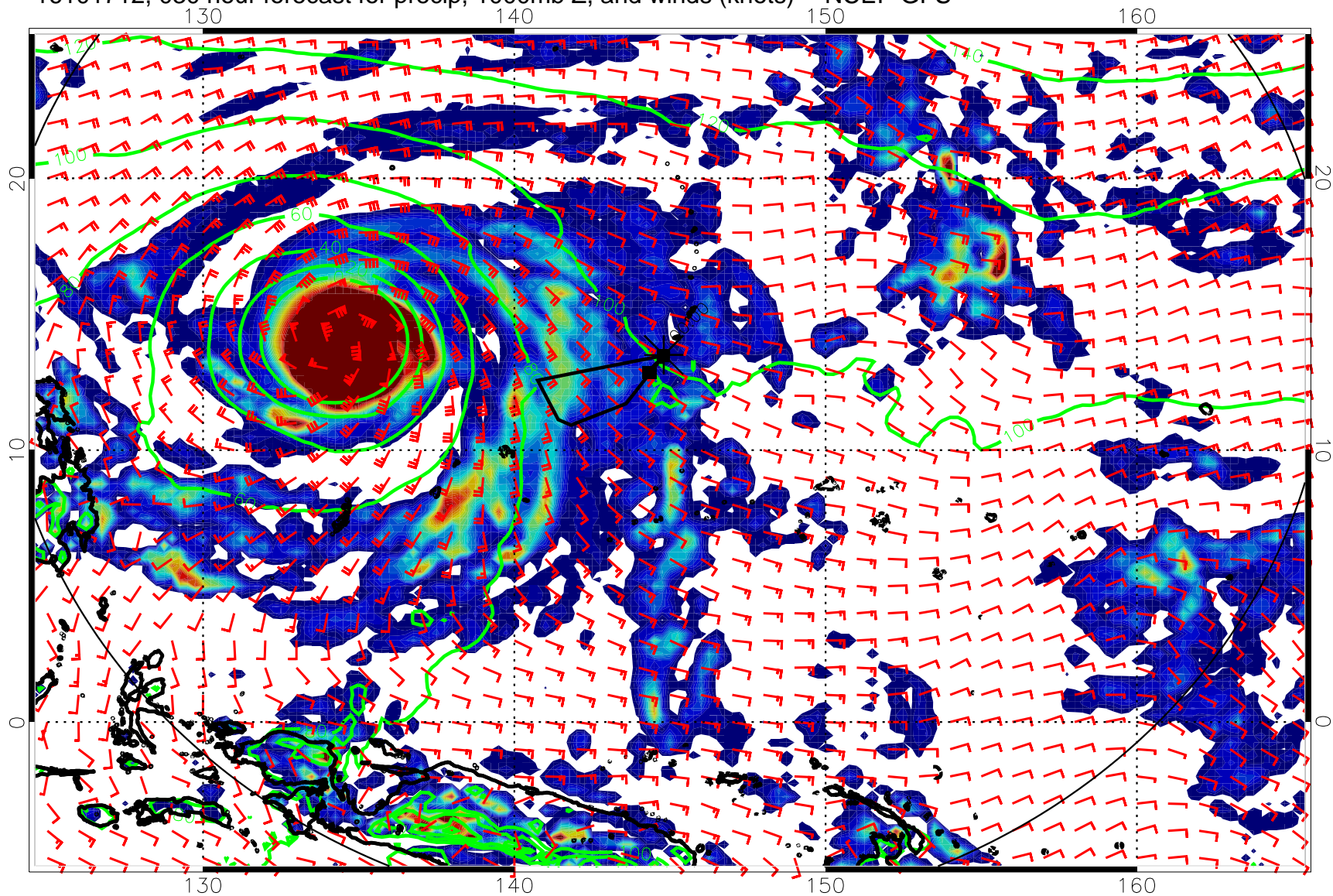
16101712, 030 hour forecast for precip, 1000mb Z, and winds (knots) -- NCEP GFS
