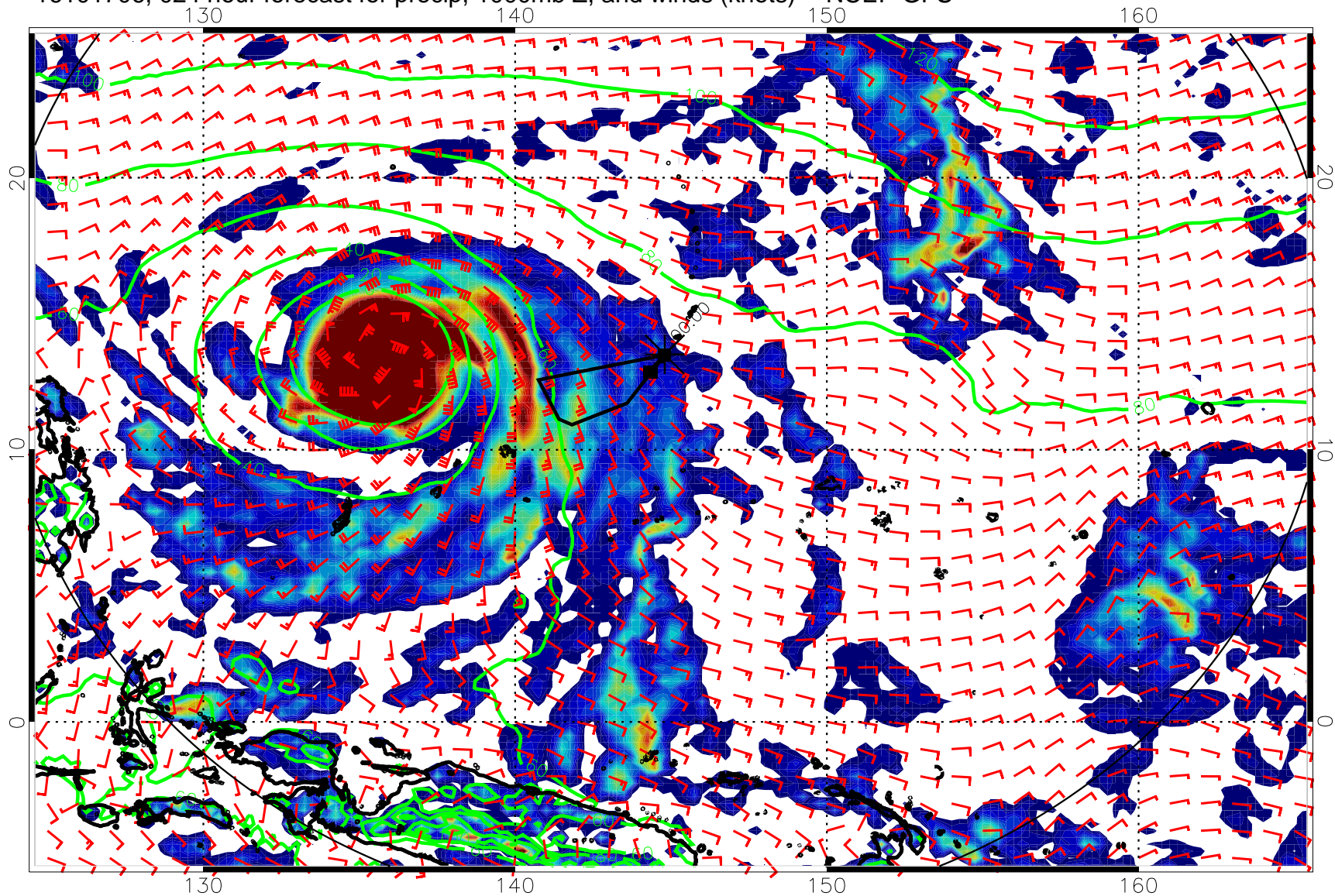
16101706, 024 hour forecast for precip, 1000mb Z, and winds (knots) -- NCEP GFS
