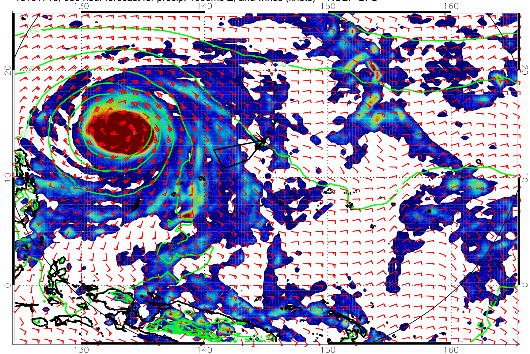
16101718, 036 hour forecast for precip, 1000mb Z, and winds (knots) -- NCEP GFS
