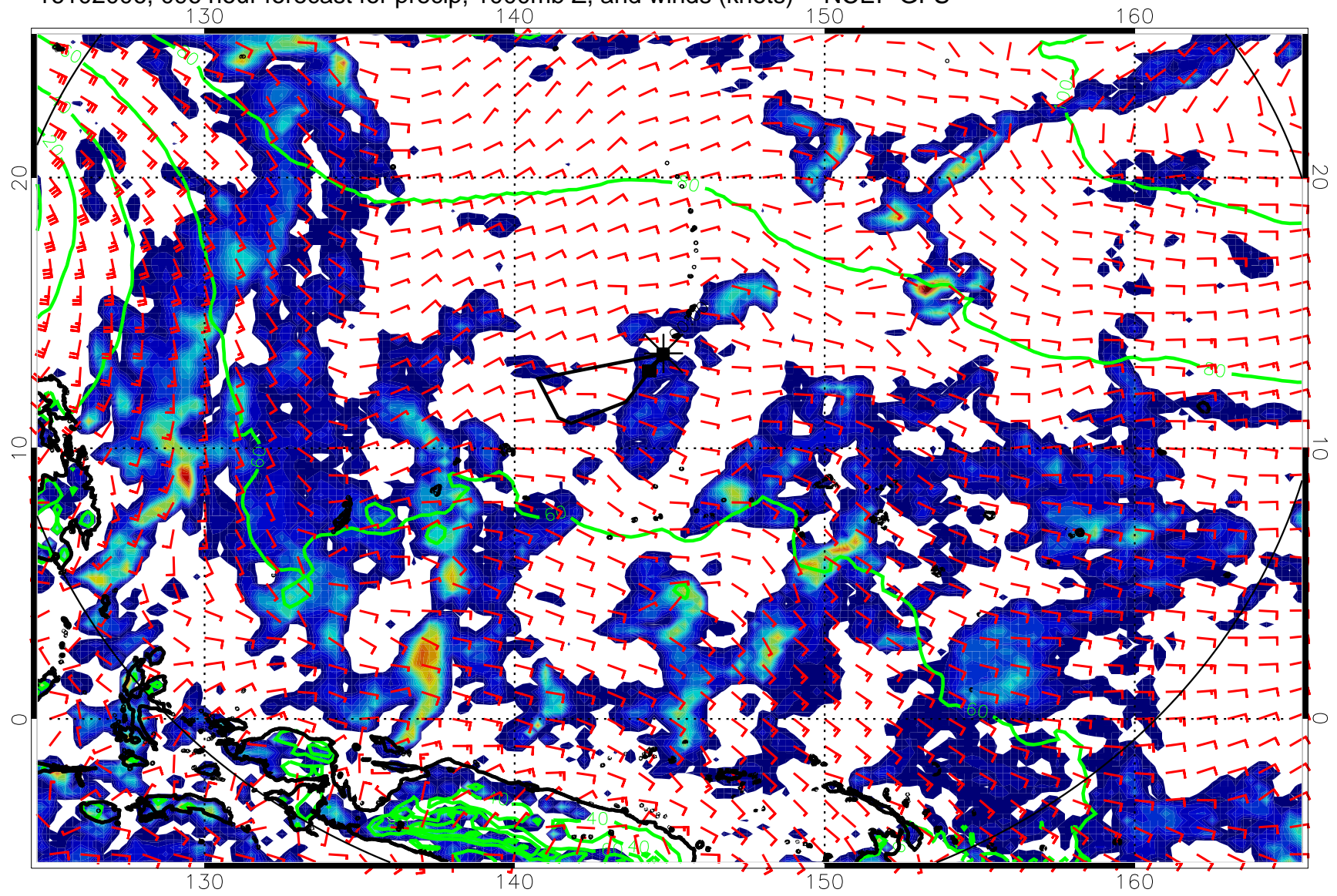
16102006, 096 hour forecast for precip, 1000mb Z, and winds (knots) -- NCEP GFS
