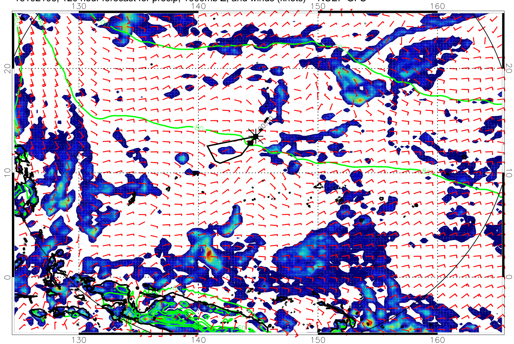
16102106, 120 hour forecast for precip, 1000mb Z, and winds (knots) -- NCEP GFS
