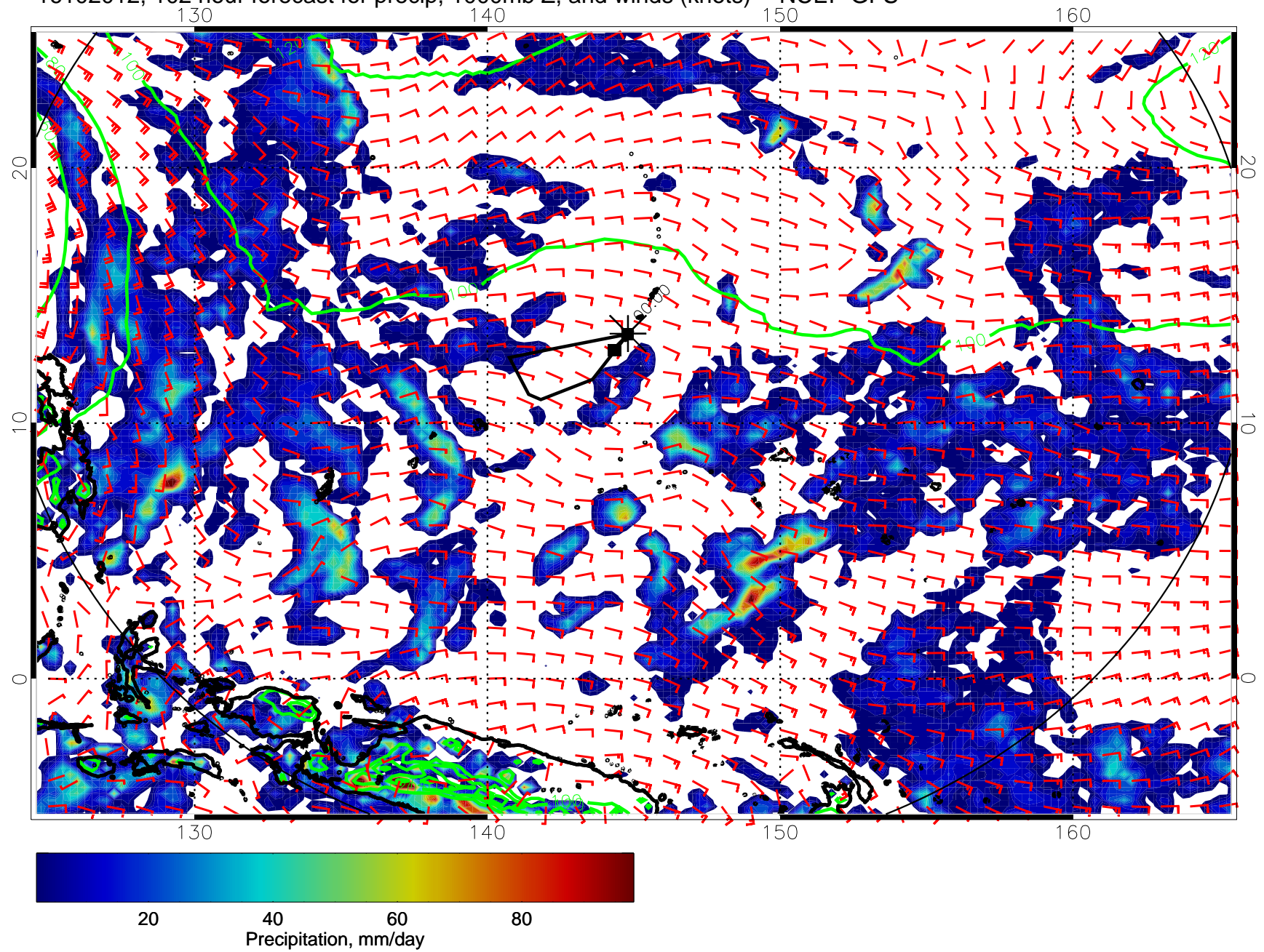
16102012, 102 hour forecast for precip, 1000mb Z, and winds (knots) -- NCEP GFS
