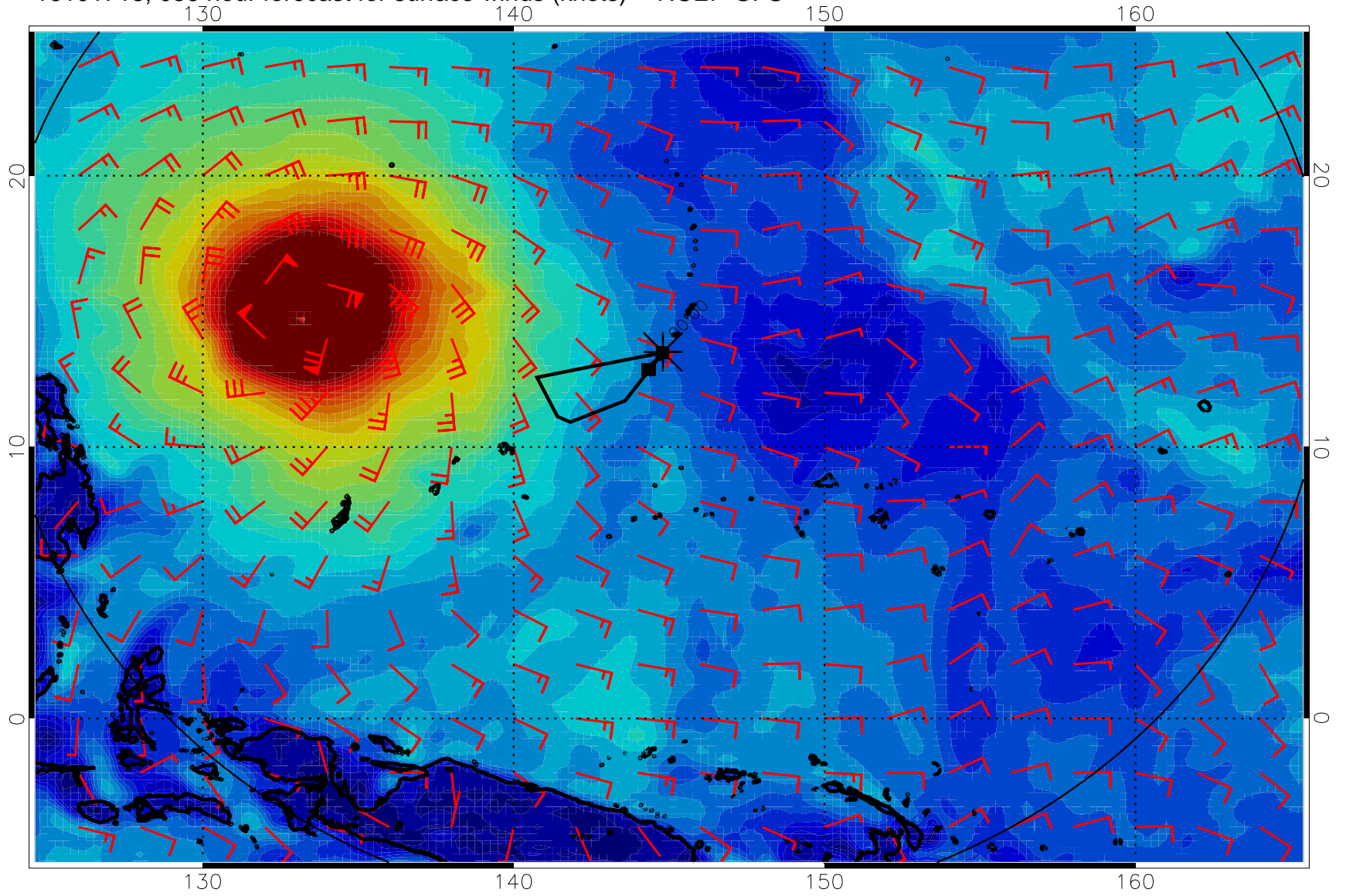
16101718, 036 hour forecast for surface winds (knots) -- NCEP GFS
