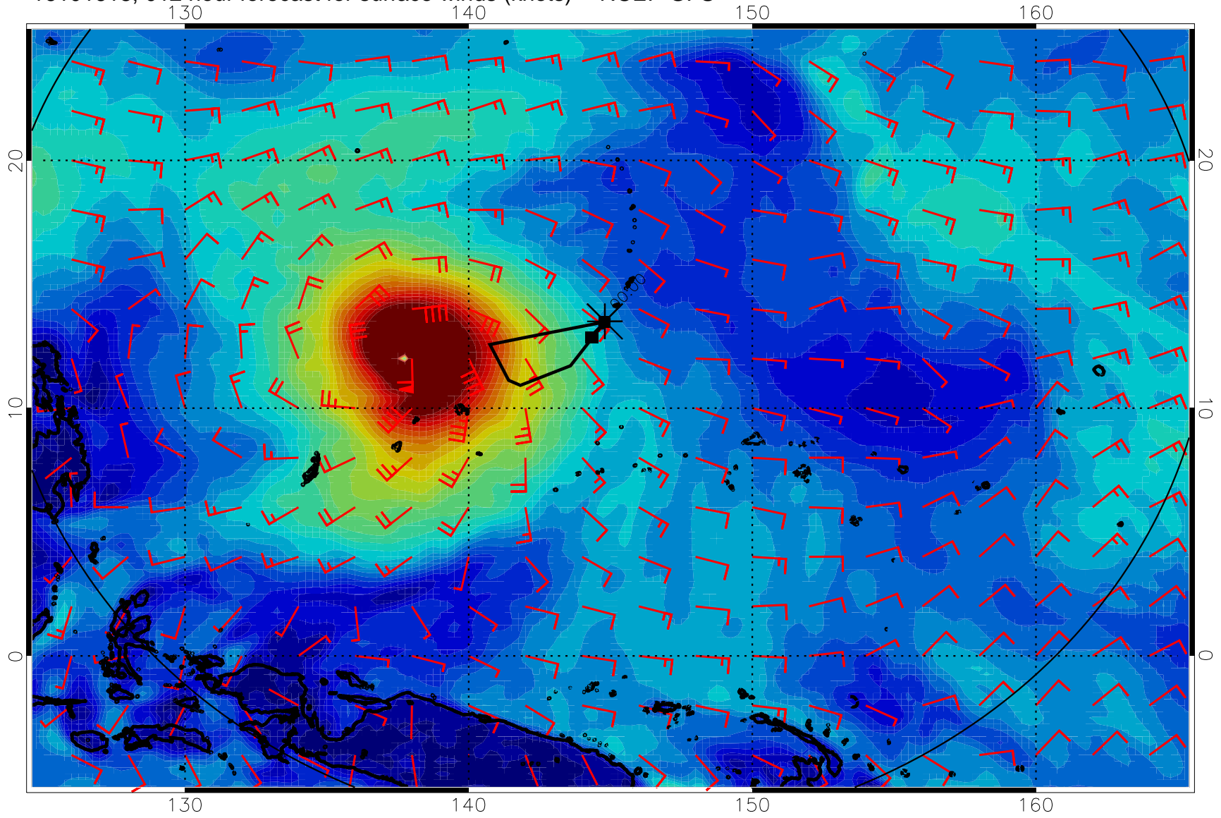
16101618, 012 hour forecast for surface winds (knots) -- NCEP GFS
