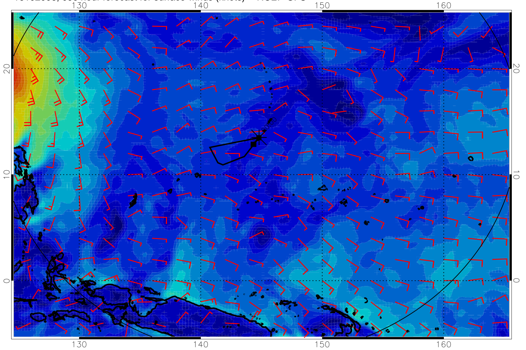
16102006, 096 hour forecast for surface winds (knots) -- NCEP GFS
