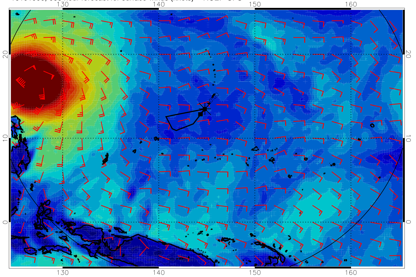
16101900, 066 hour forecast for surface winds (knots) -- NCEP GFS
