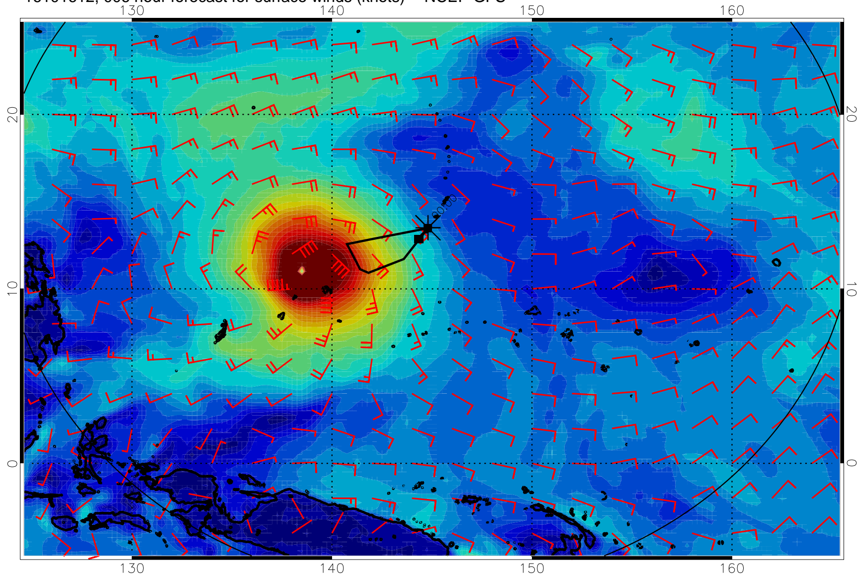
16101612, 006 hour forecast for surface winds (knots) -- NCEP GFS
