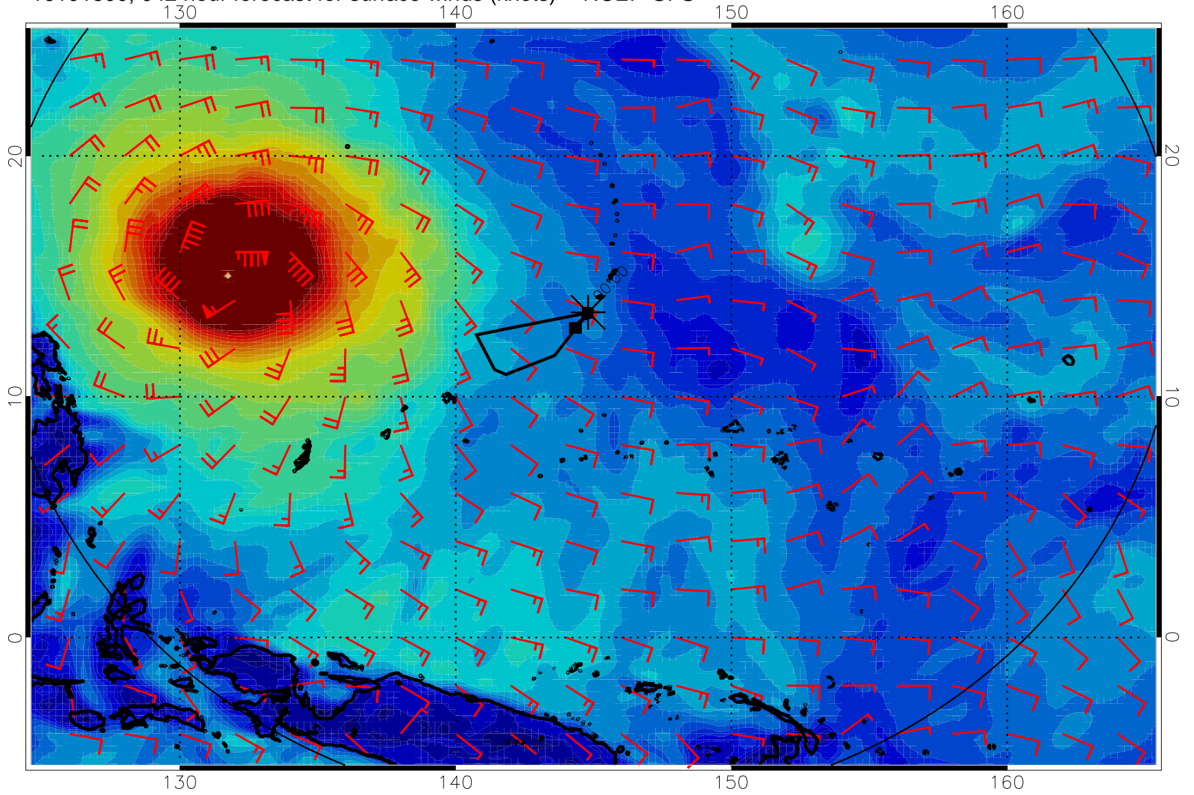
16101800, 042 hour forecast for surface winds (knots) -- NCEP GFS
