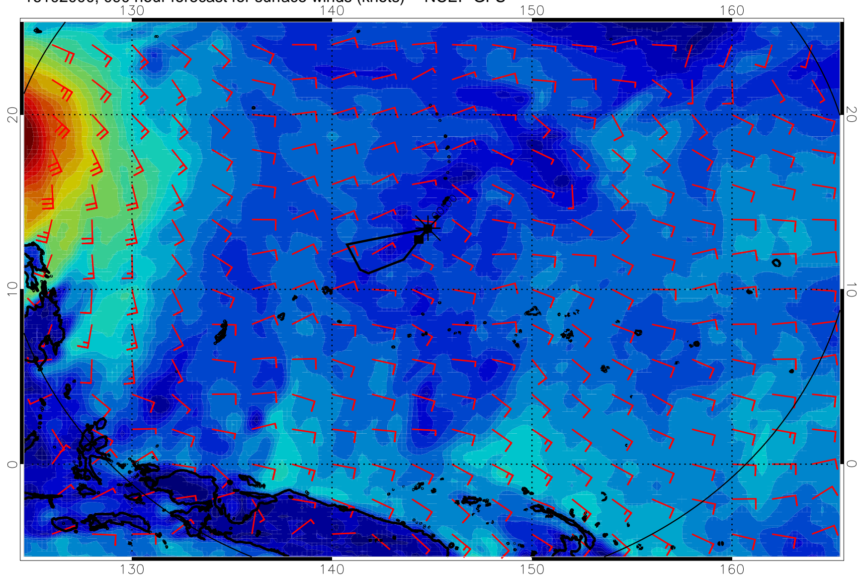
16102000, 090 hour forecast for surface winds (knots) -- NCEP GFS
