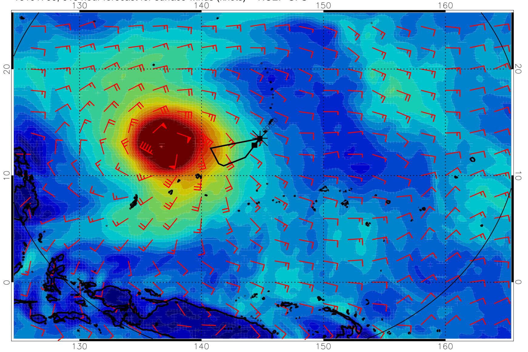
16101700, 018 hour forecast for surface winds (knots) -- NCEP GFS
