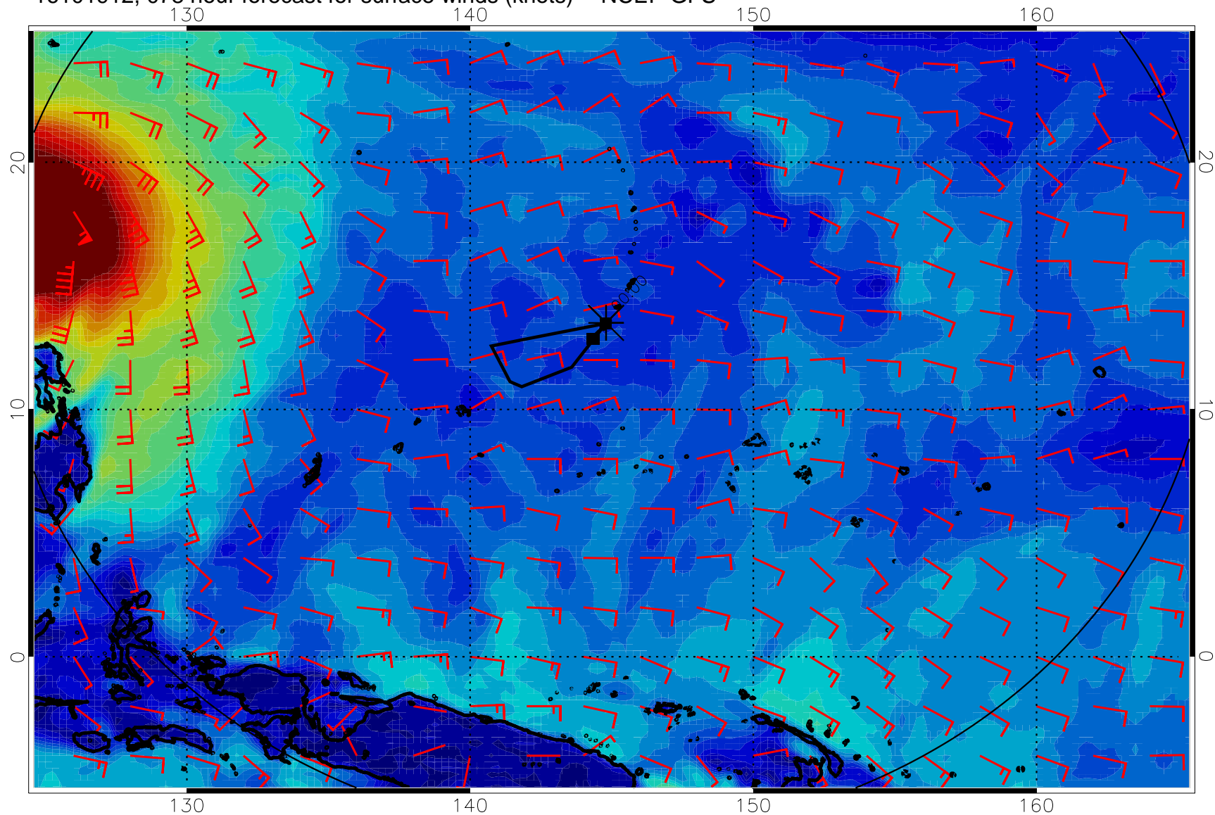
16101912, 078 hour forecast for surface winds (knots) -- NCEP GFS
