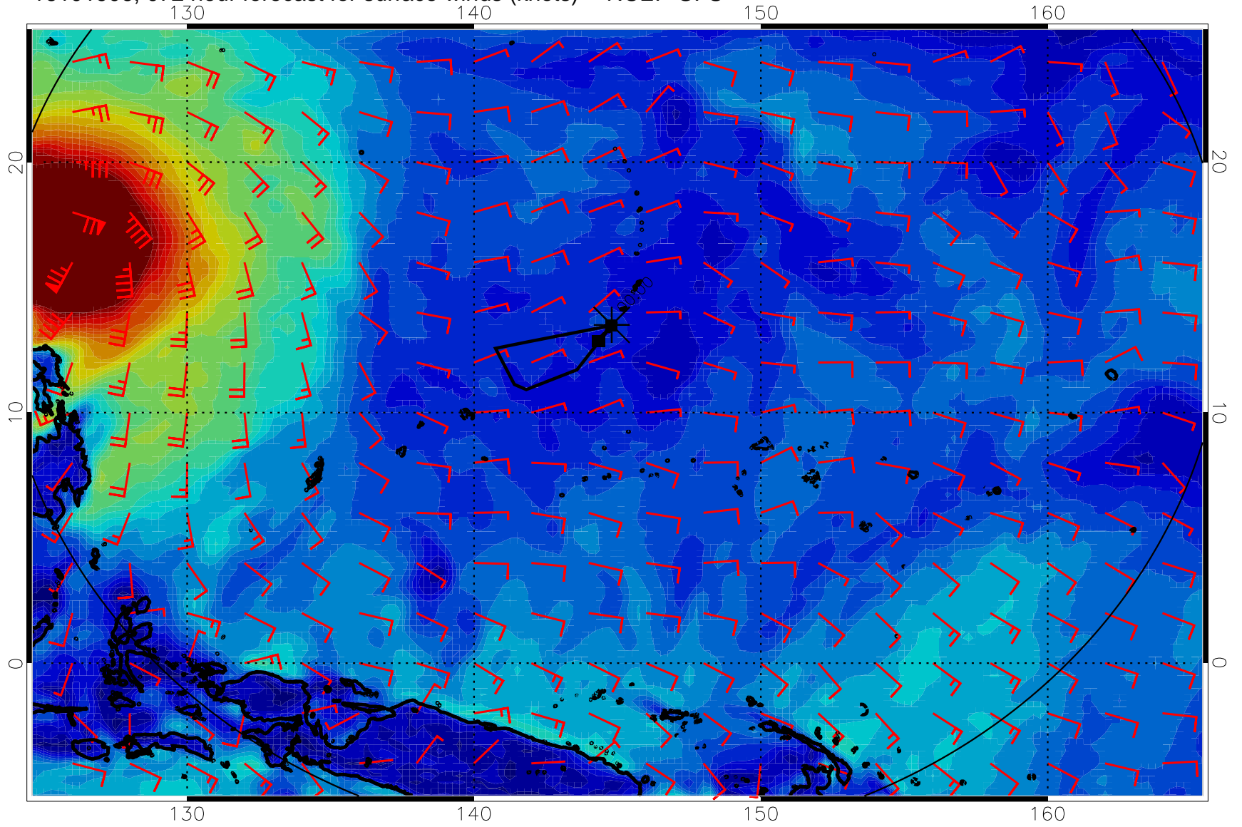
16101906, 072 hour forecast for surface winds (knots) -- NCEP GFS
