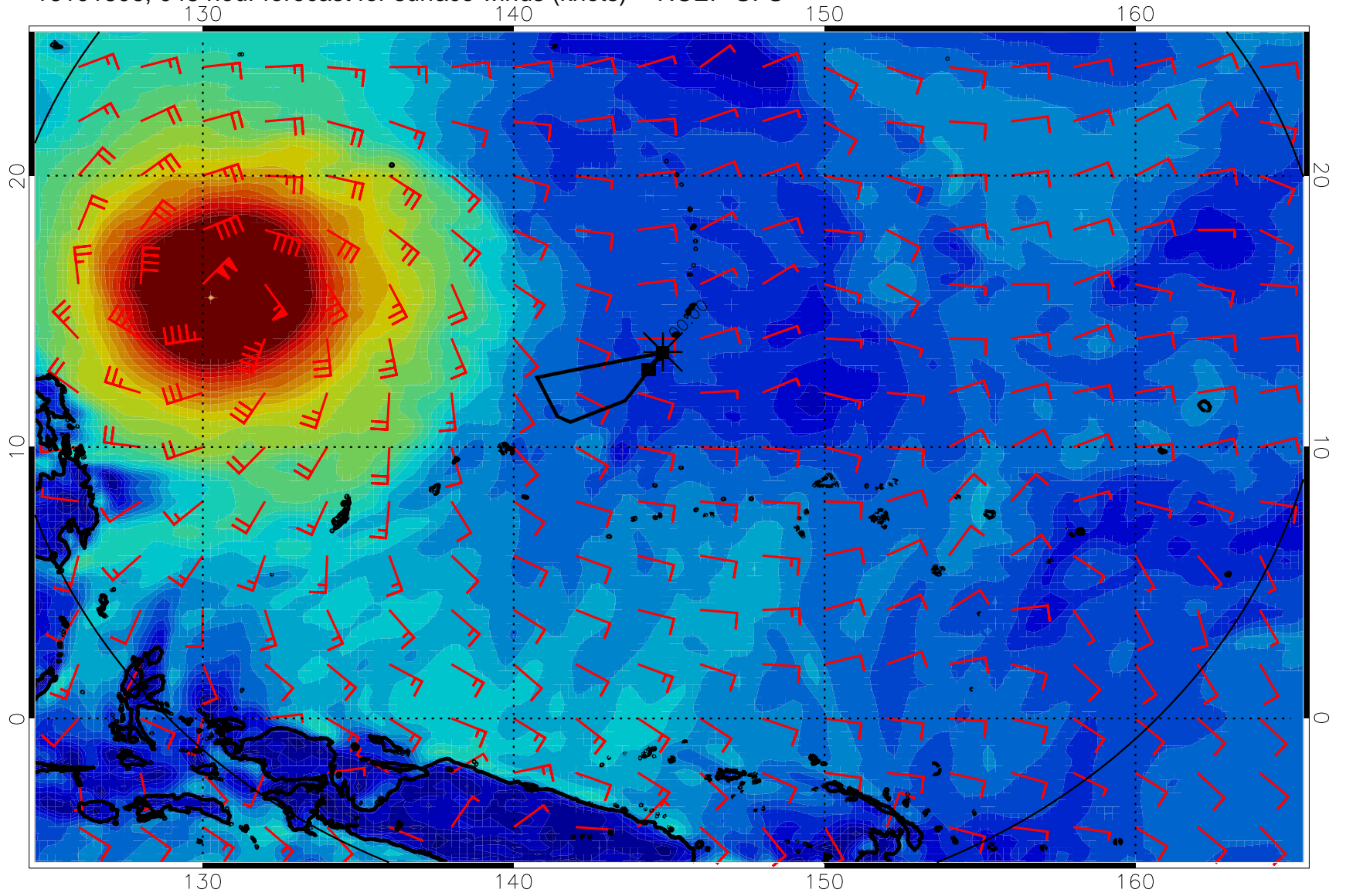
16101806, 048 hour forecast for surface winds (knots) -- NCEP GFS
