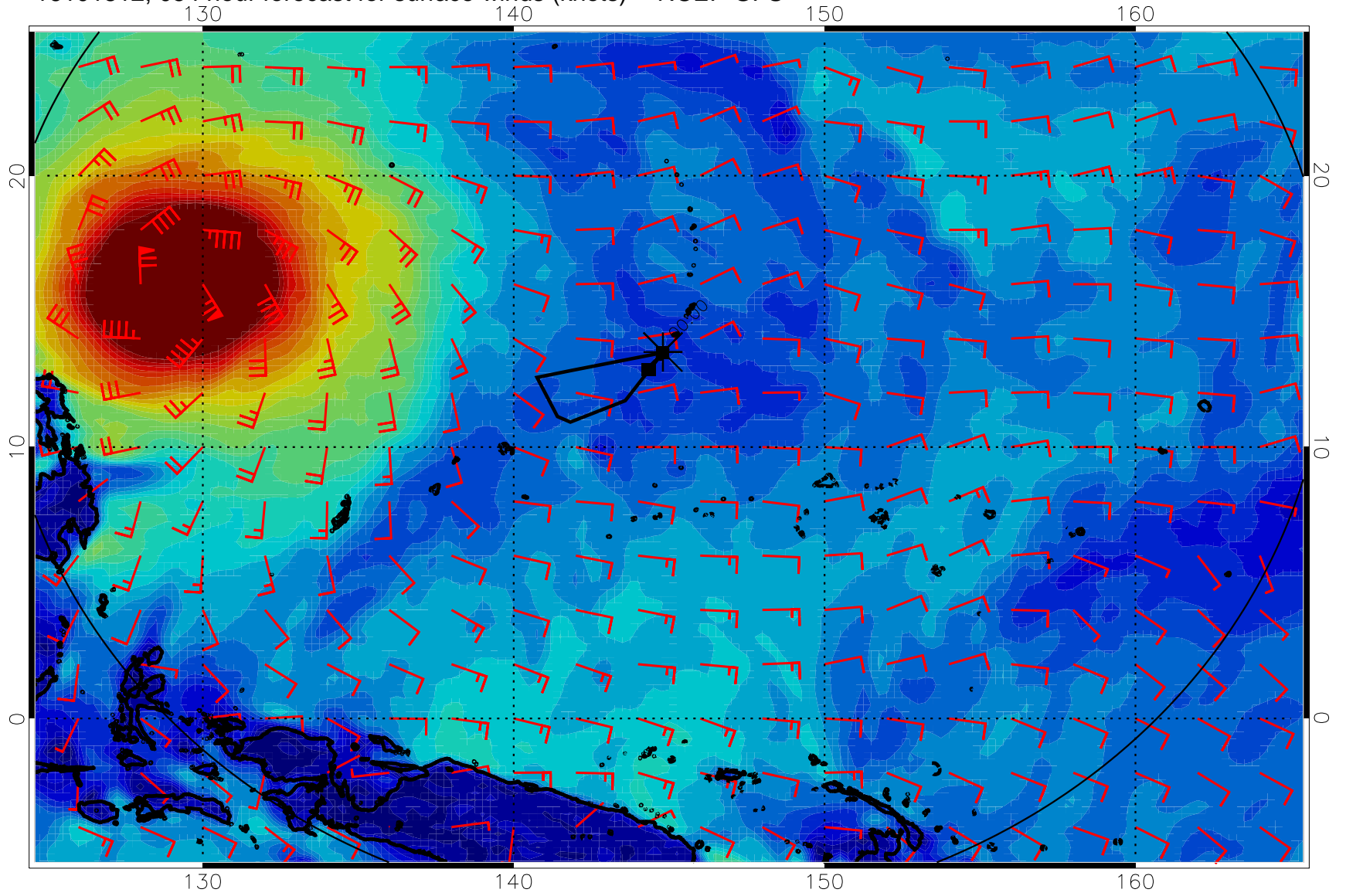
16101812, 054 hour forecast for surface winds (knots) -- NCEP GFS
