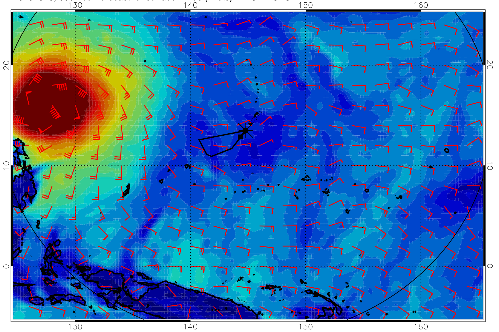
16101818, 060 hour forecast for surface winds (knots) -- NCEP GFS
