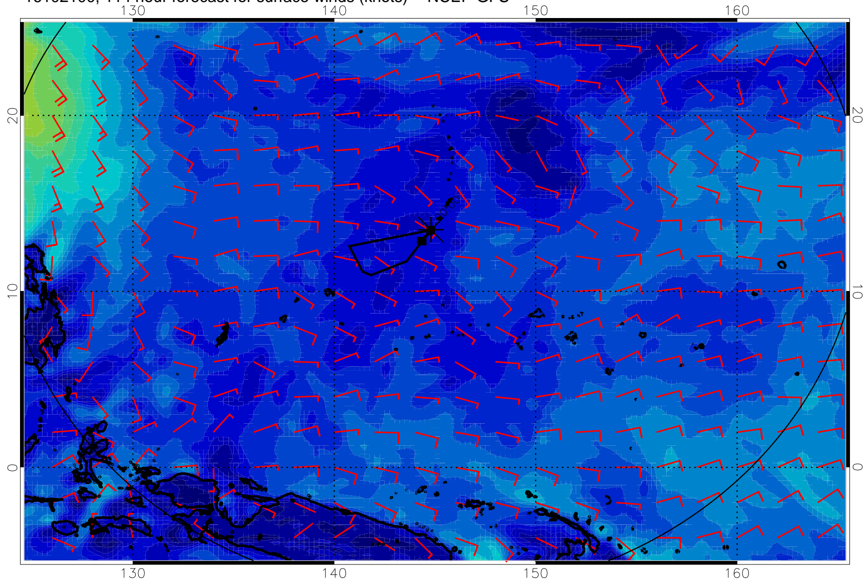
16102100, 114 hour forecast for surface winds (knots) -- NCEP GFS
