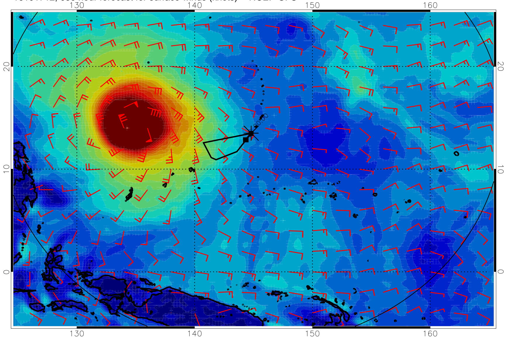
16101712, 030 hour forecast for surface winds (knots) -- NCEP GFS
