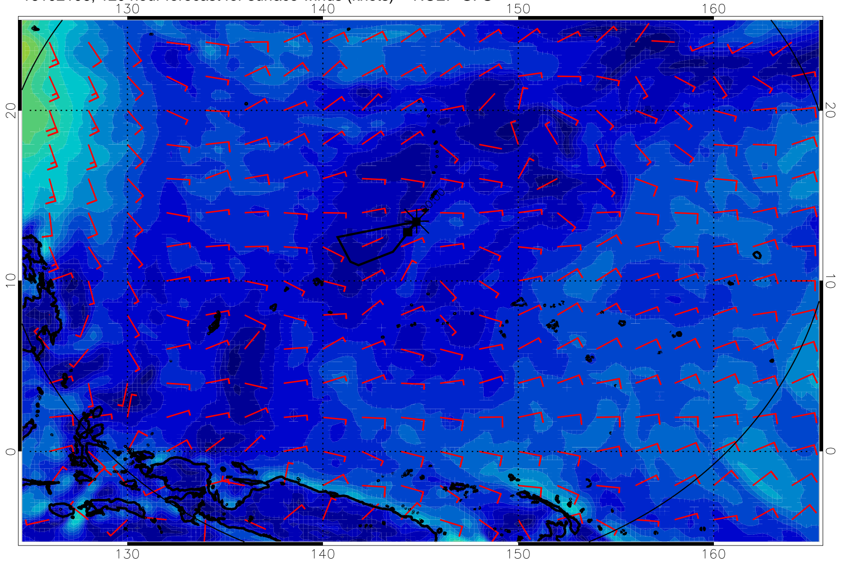
16102106, 120 hour forecast for surface winds (knots) -- NCEP GFS
