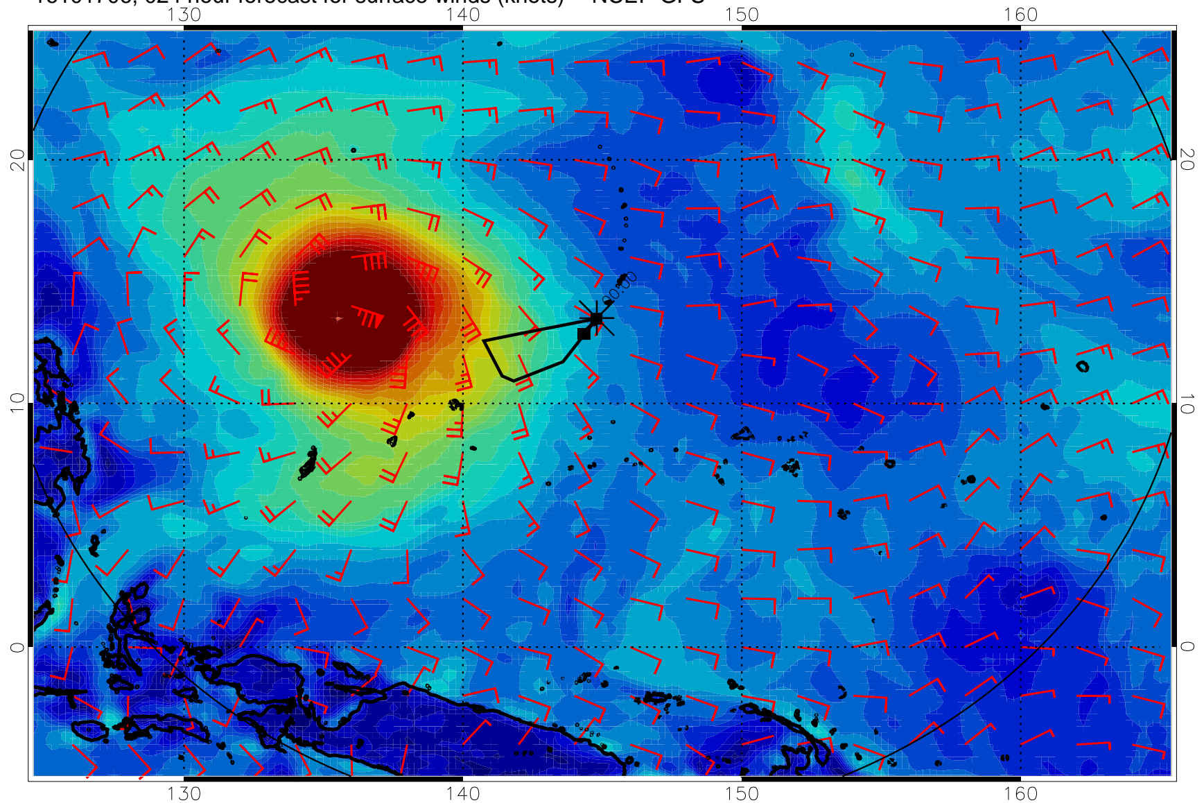
16101706, 024 hour forecast for surface winds (knots) -- NCEP GFS
