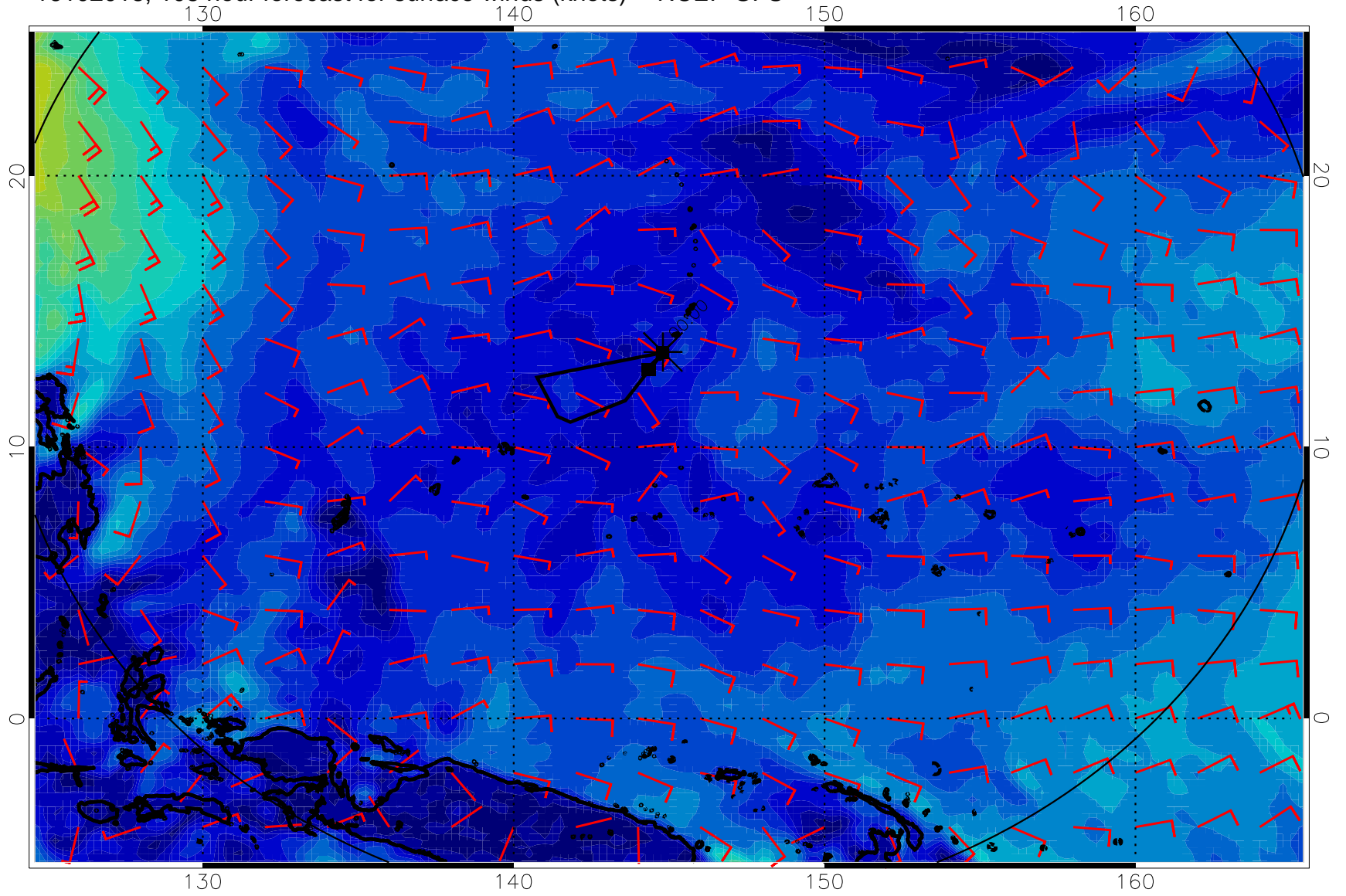
16102018, 108 hour forecast for surface winds (knots) -- NCEP GFS
