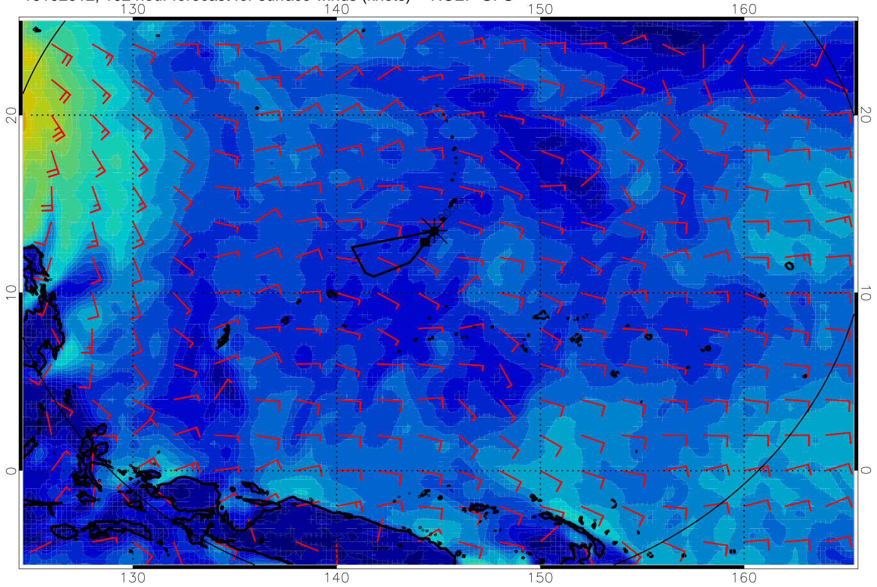
16102012, 102 hour forecast for surface winds (knots) -- NCEP GFS
