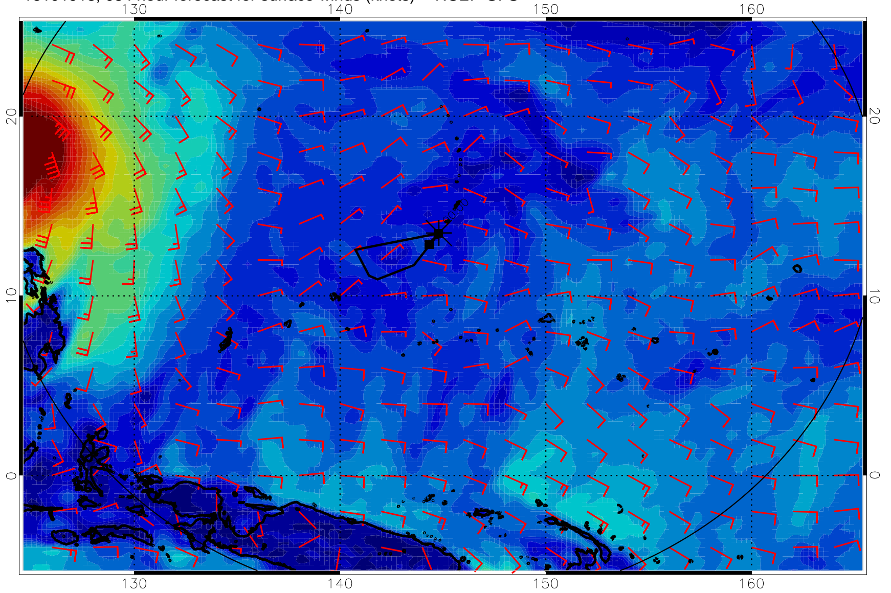
16101918, 084 hour forecast for surface winds (knots) -- NCEP GFS
