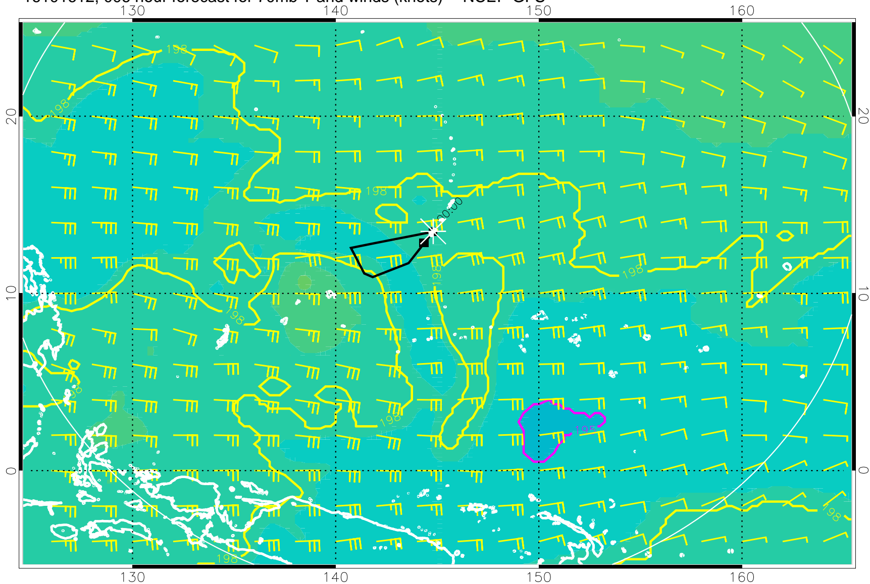
16101612, 006 hour forecast for 70mb T and winds (knots) -- NCEP GFS
