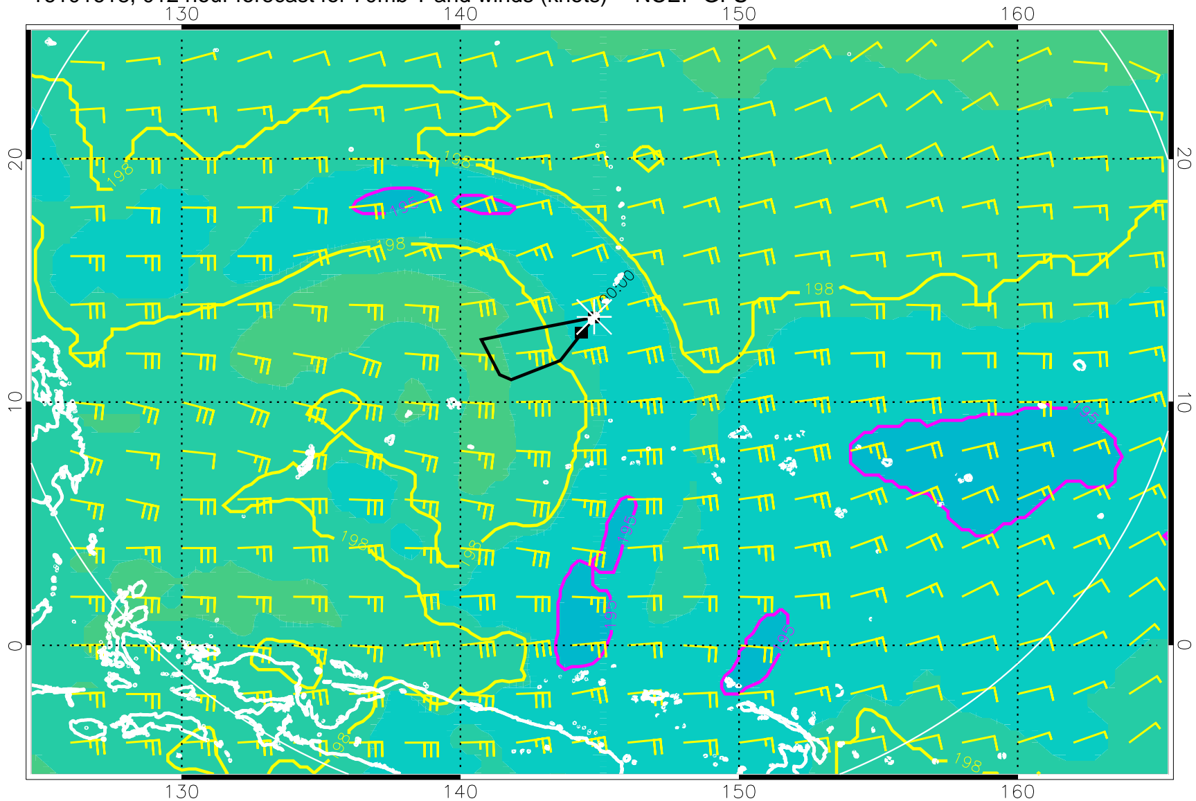
16101618, 012 hour forecast for 70mb T and winds (knots) -- NCEP GFS
