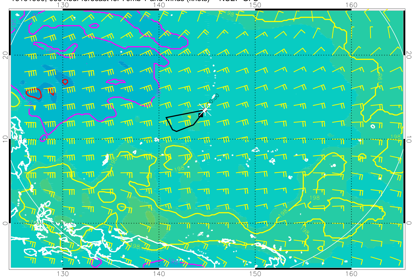
16101900, 066 hour forecast for 70mb T and winds (knots) -- NCEP GFS
