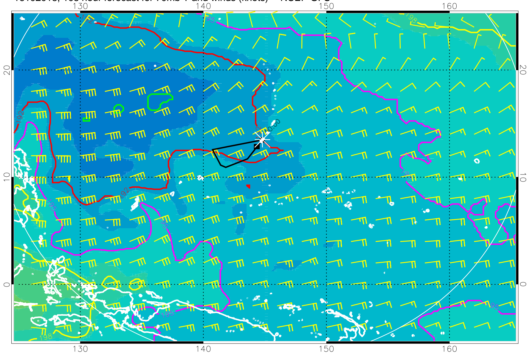
16102018, 108 hour forecast for 70mb T and winds (knots) -- NCEP GFS
