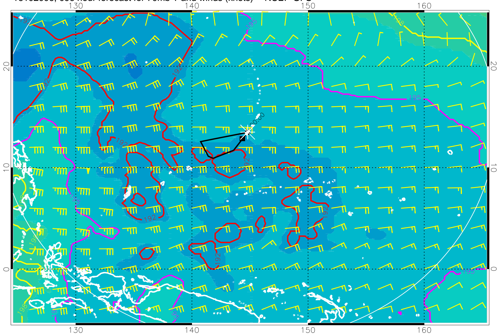
16102006, 096 hour forecast for 70mb T and winds (knots) -- NCEP GFS
