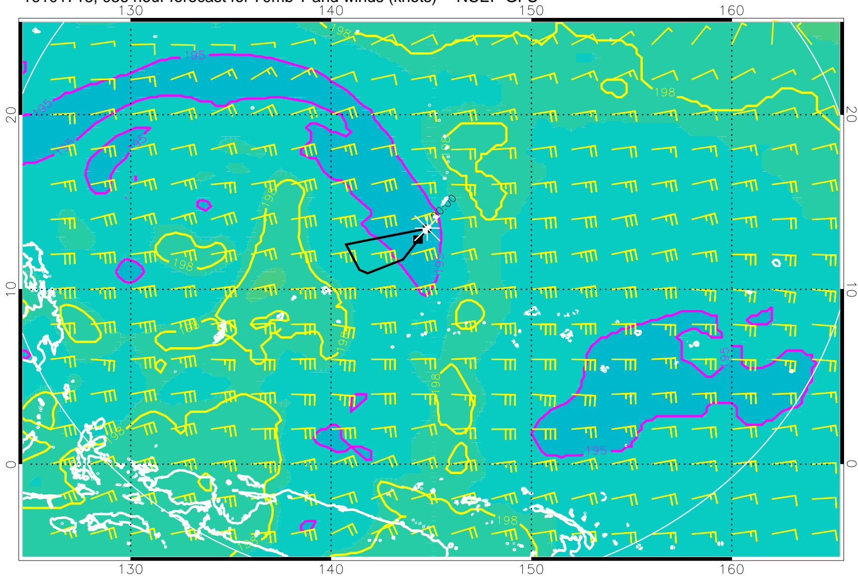
16101718, 036 hour forecast for 70mb T and winds (knots) -- NCEP GFS
