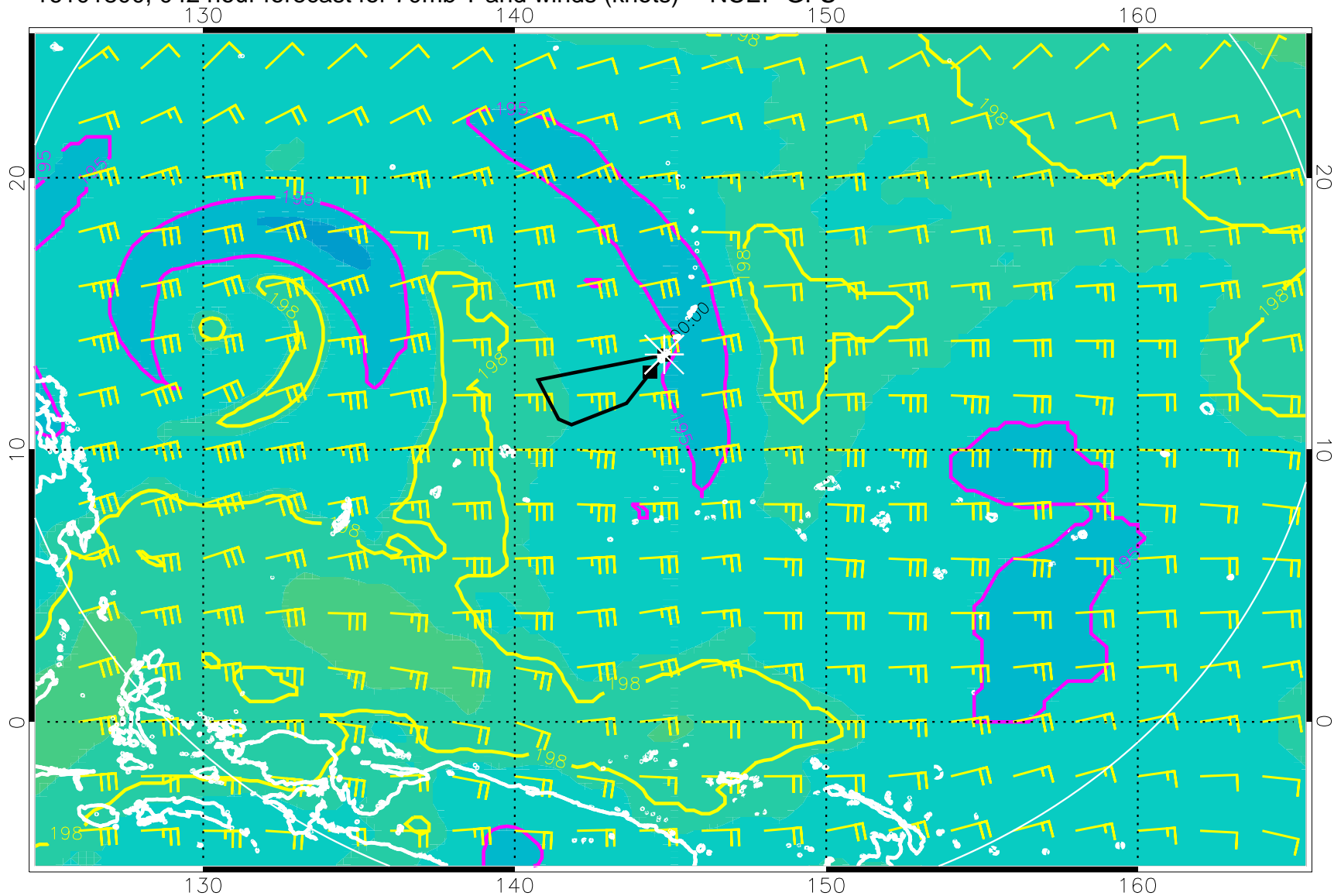
16101800, 042 hour forecast for 70mb T and winds (knots) -- NCEP GFS
