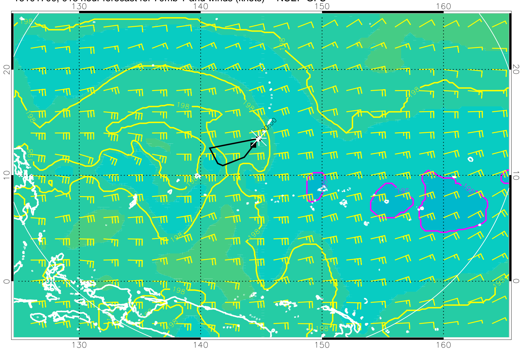
16101700, 018 hour forecast for 70mb T and winds (knots) -- NCEP GFS
