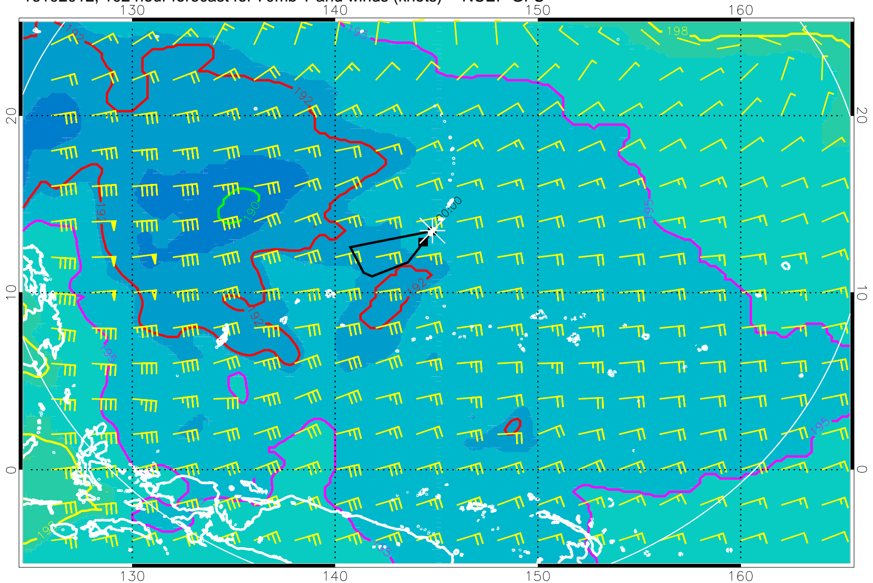
16102012, 102 hour forecast for 70mb T and winds (knots) -- NCEP GFS
