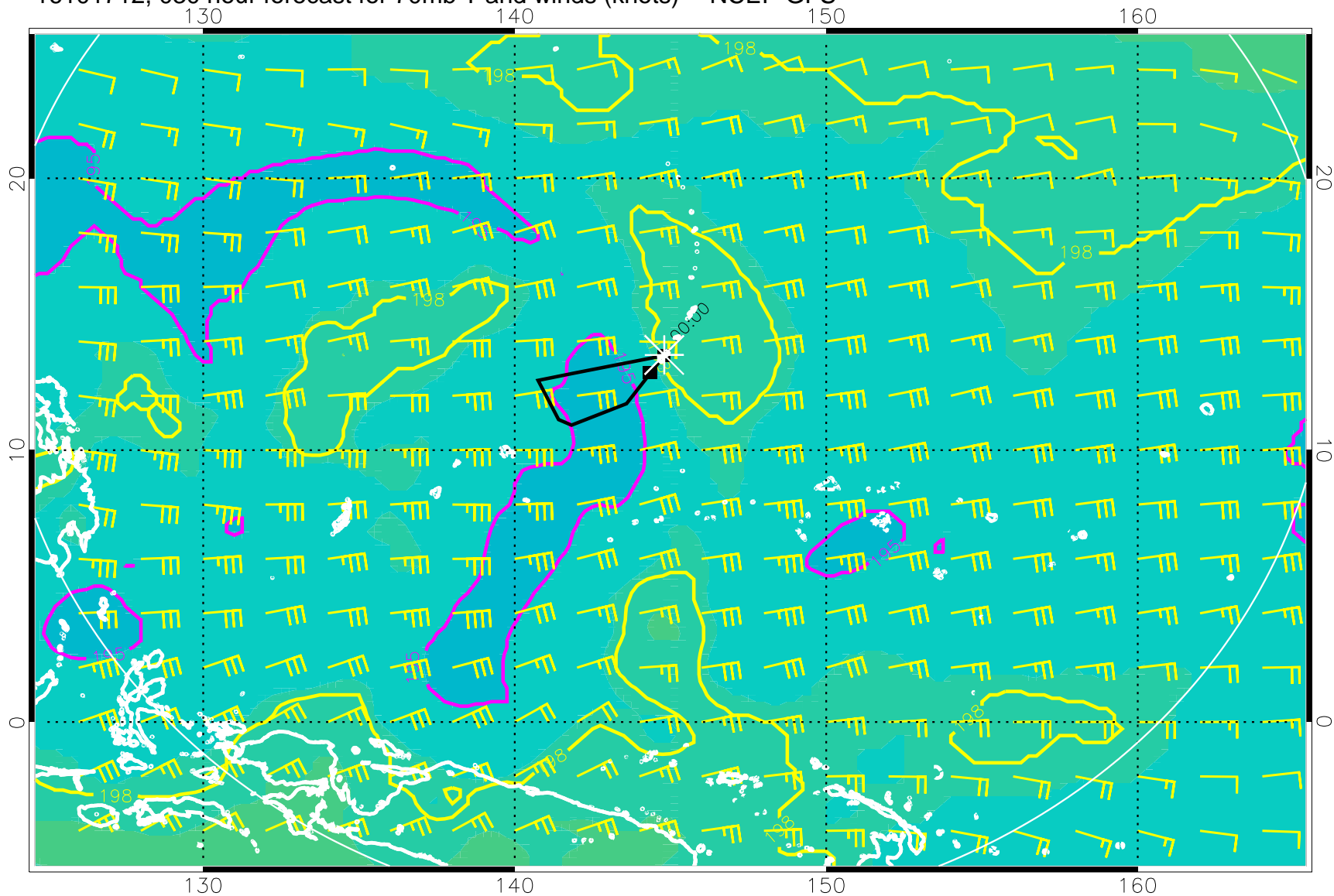
16101712, 030 hour forecast for 70mb T and winds (knots) -- NCEP GFS
