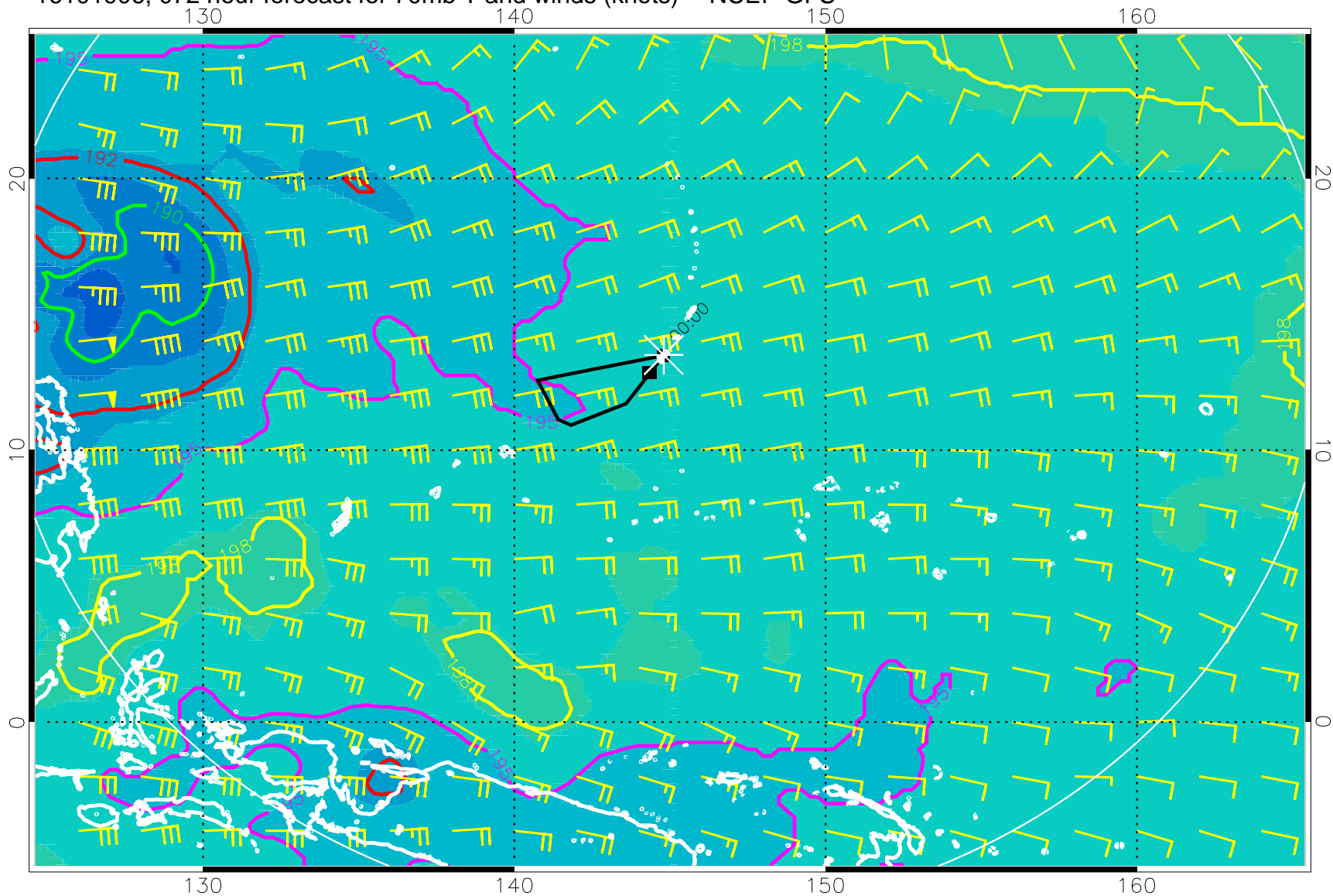
16101906, 072 hour forecast for 70mb T and winds (knots) -- NCEP GFS
