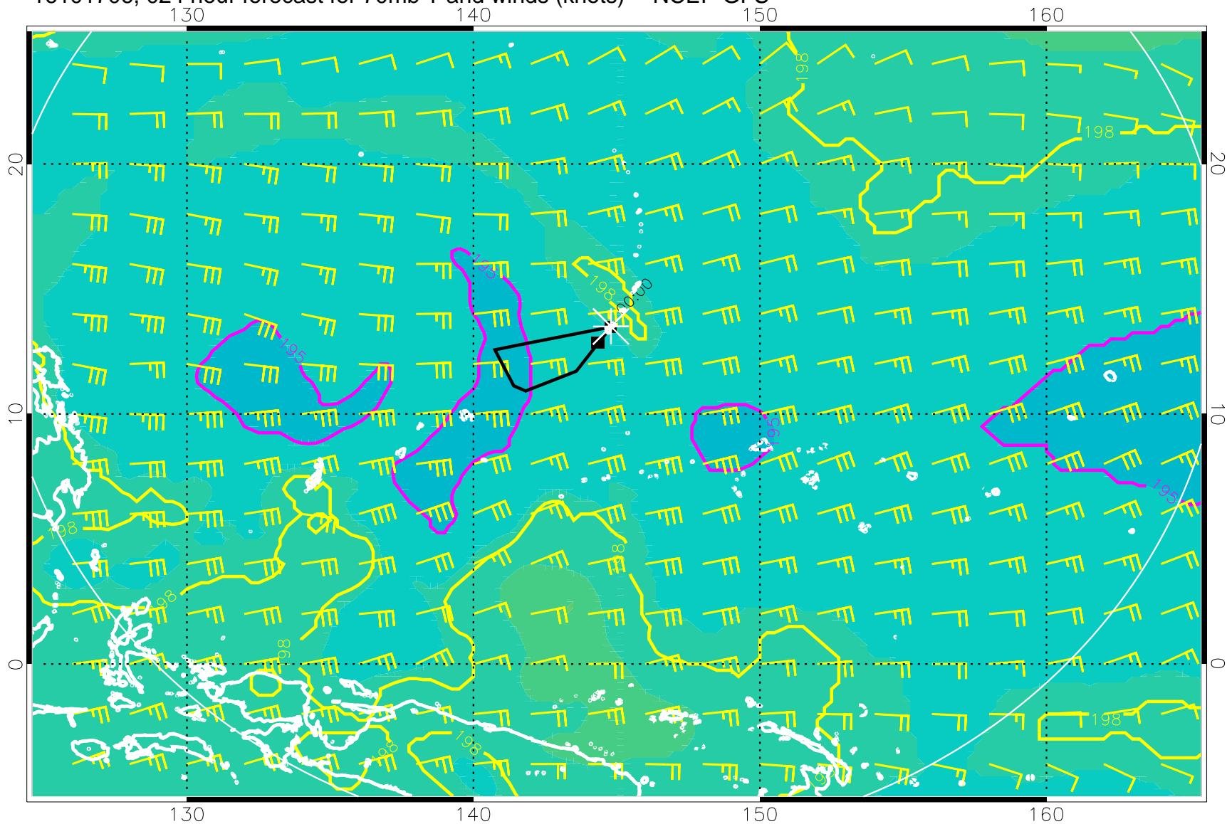
16101706, 024 hour forecast for 70mb T and winds (knots) -- NCEP GFS
