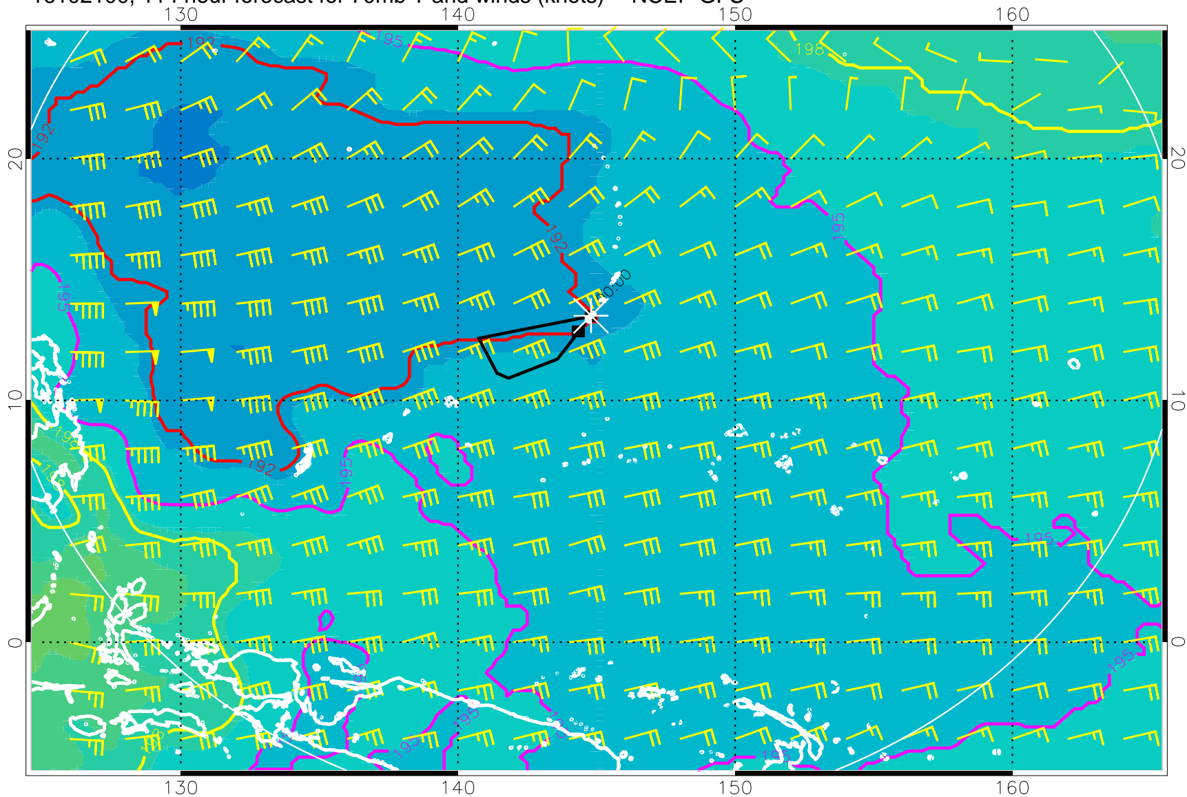
16102100, 114 hour forecast for 70mb T and winds (knots) -- NCEP GFS
