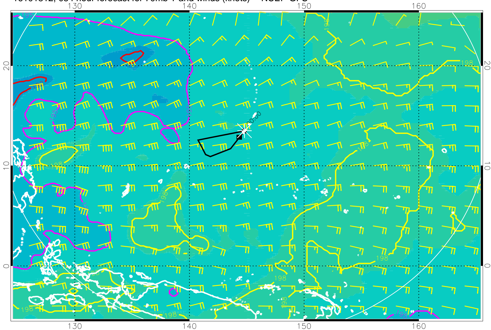
16101812, 054 hour forecast for 70mb T and winds (knots) -- NCEP GFS
