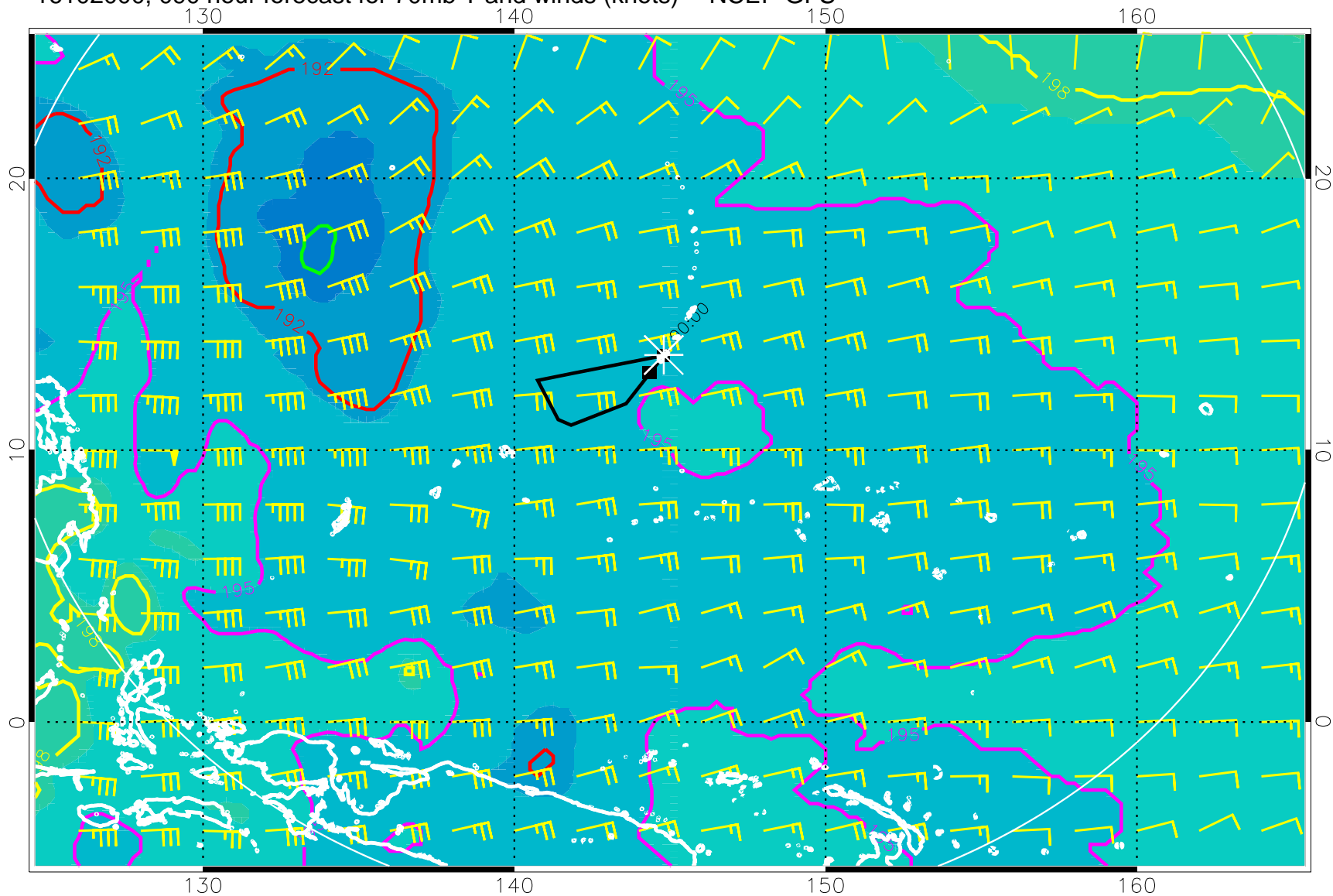
16102000, 090 hour forecast for 70mb T and winds (knots) -- NCEP GFS
