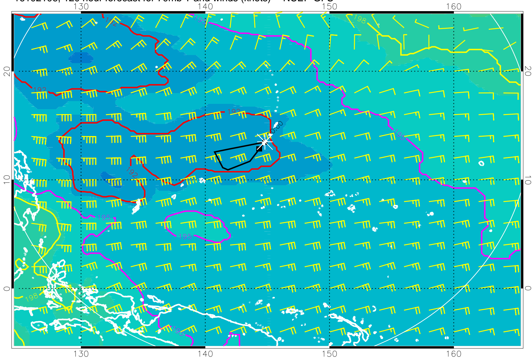
16102106, 120 hour forecast for 70mb T and winds (knots) -- NCEP GFS
