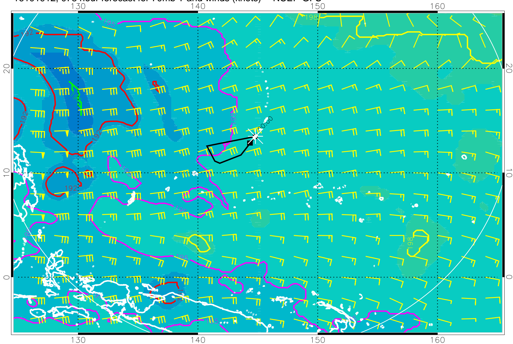
16101912, 078 hour forecast for 70mb T and winds (knots) -- NCEP GFS
