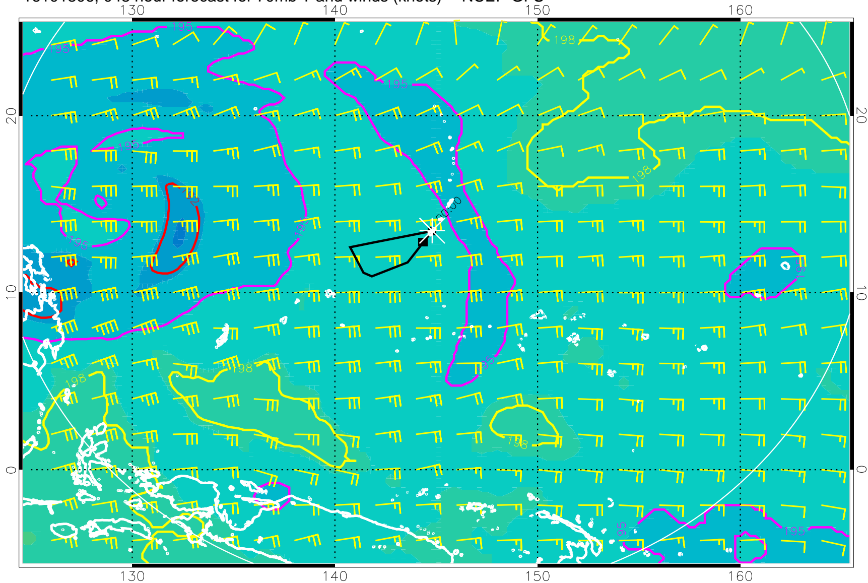
16101806, 048 hour forecast for 70mb T and winds (knots) -- NCEP GFS
