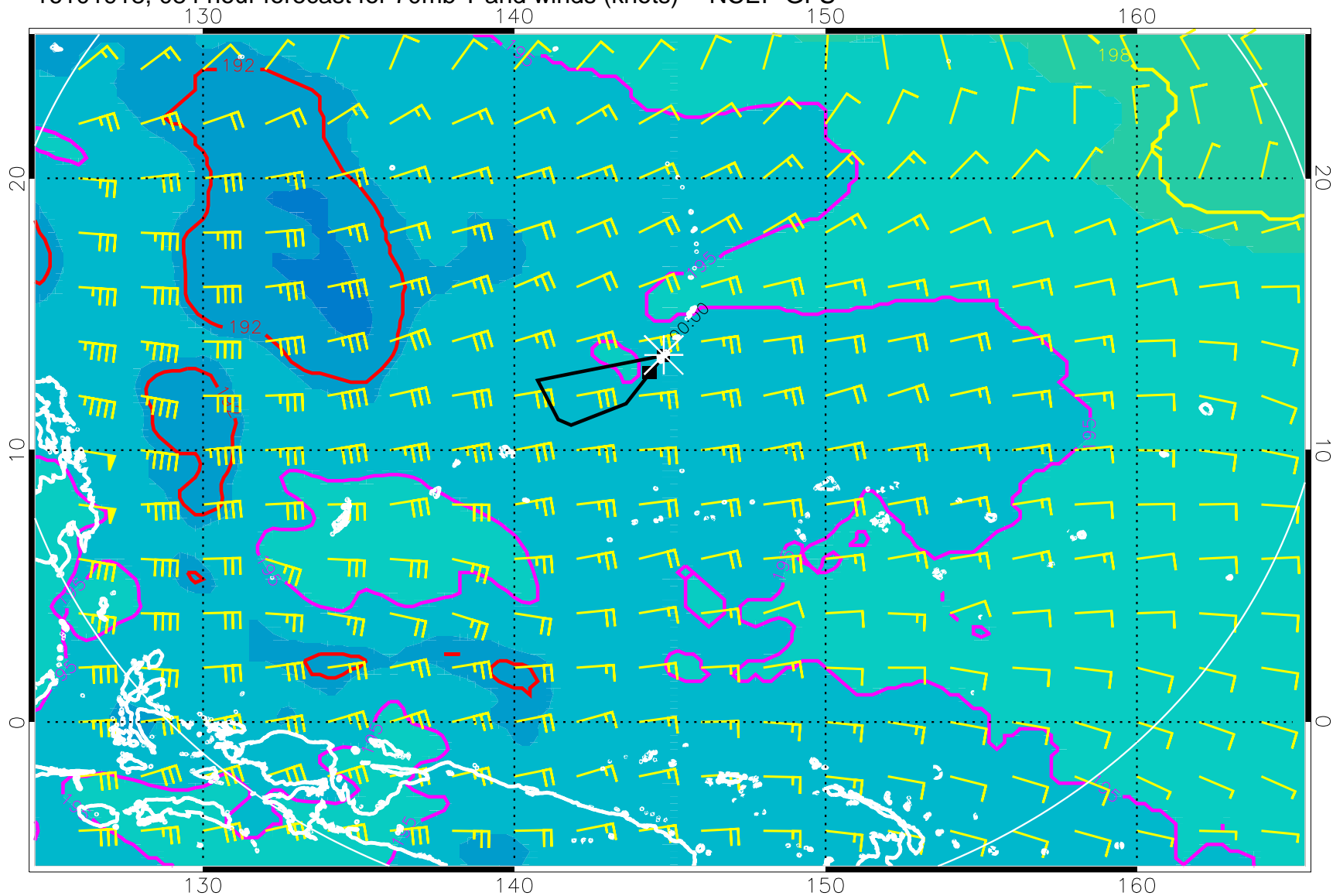
16101918, 084 hour forecast for 70mb T and winds (knots) -- NCEP GFS
