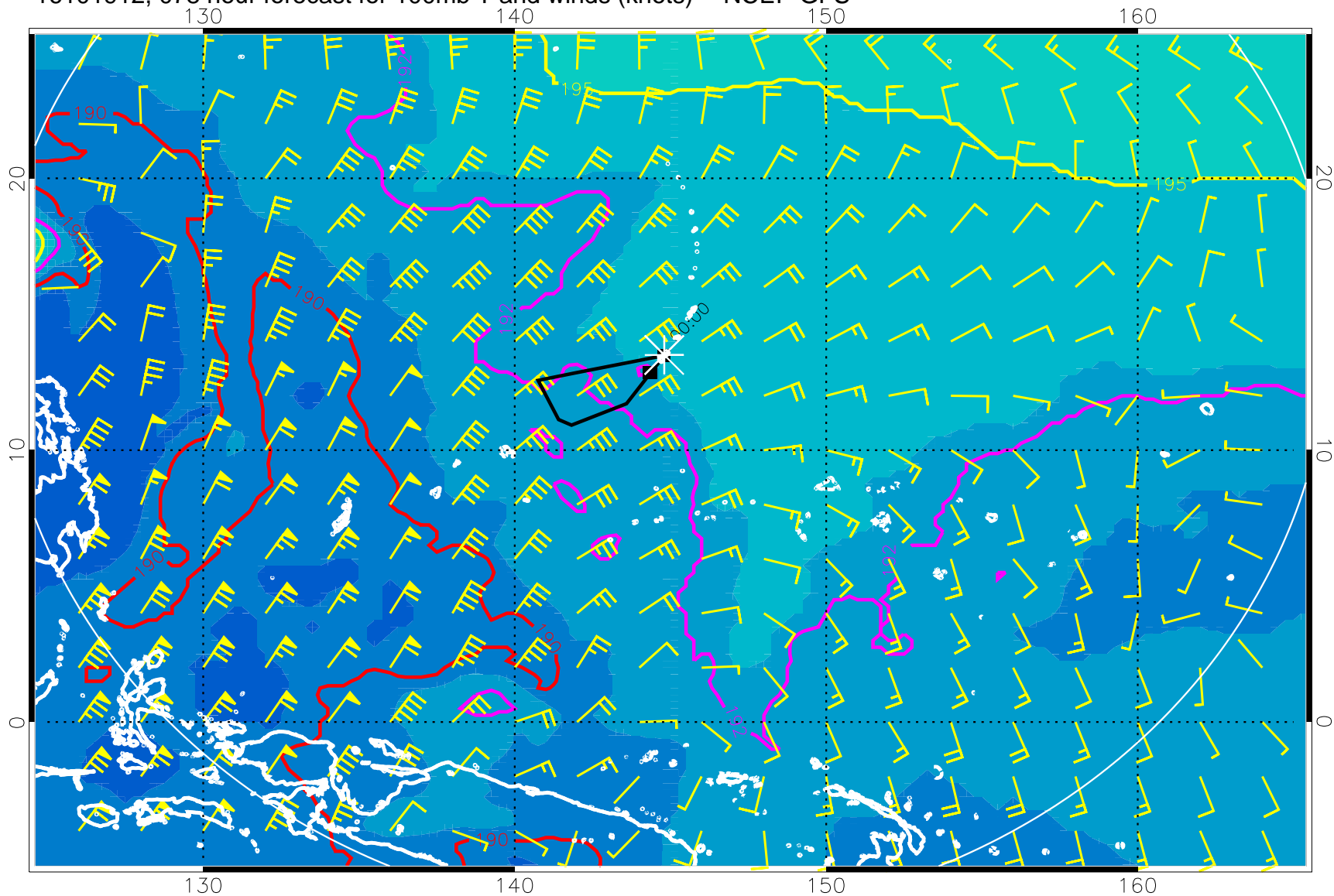
16101912, 078 hour forecast for 100mb T and winds (knots) -- NCEP GFS
