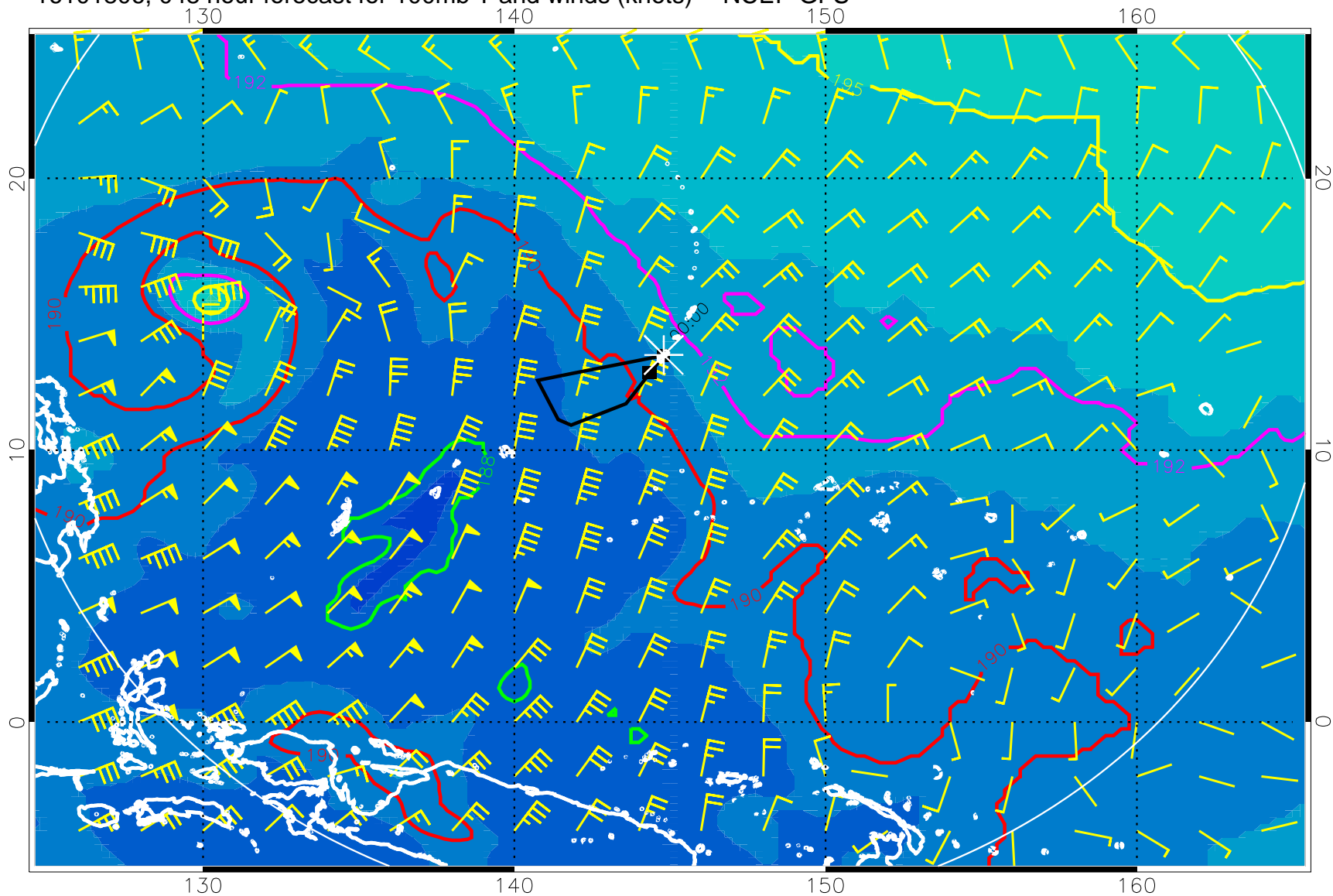
16101806, 048 hour forecast for 100mb T and winds (knots) -- NCEP GFS
