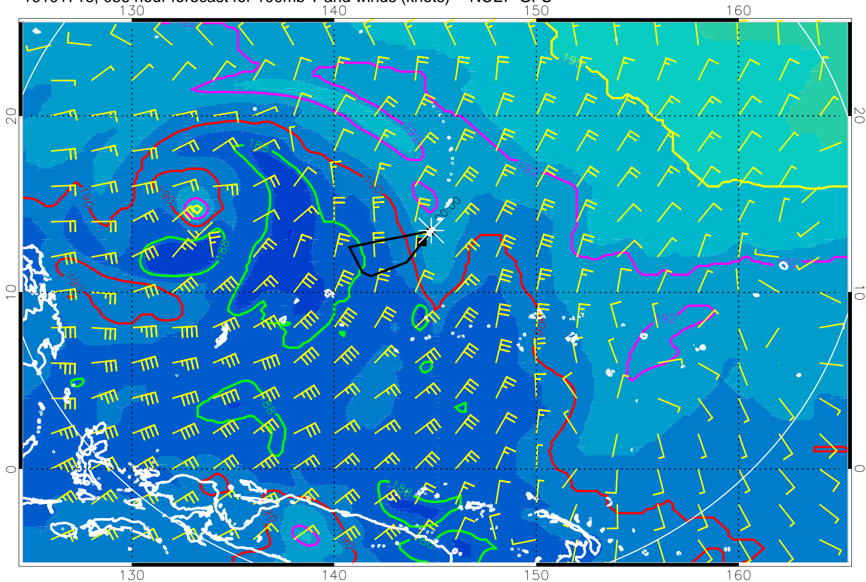
16101718, 036 hour forecast for 100mb T and winds (knots) -- NCEP GFS
