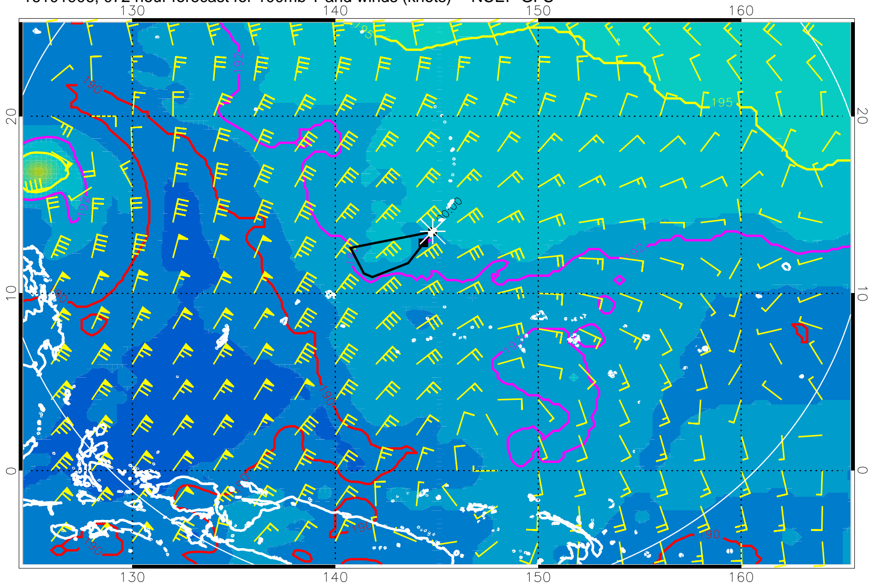
16101906, 072 hour forecast for 100mb T and winds (knots) -- NCEP GFS
