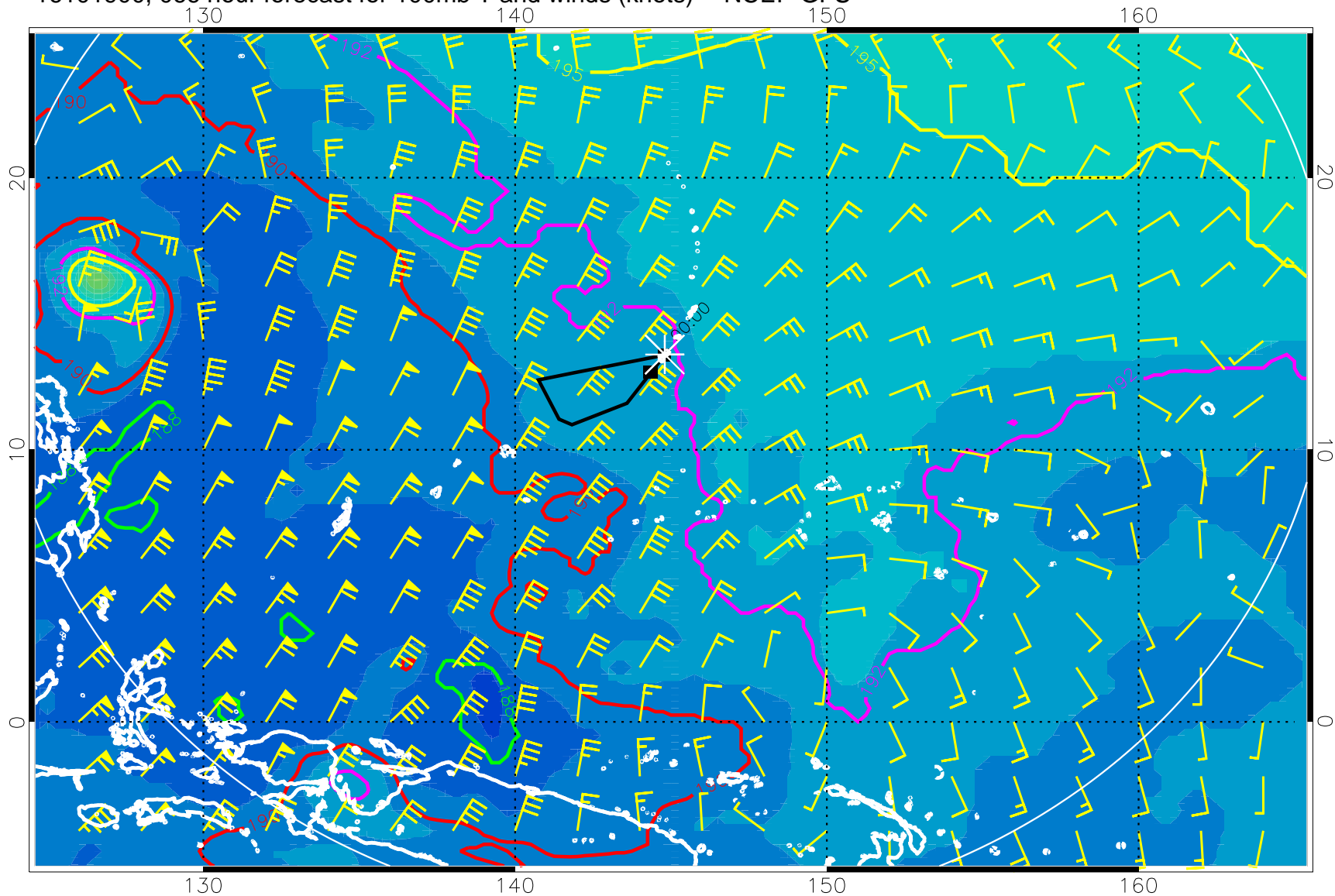
16101900, 066 hour forecast for 100mb T and winds (knots) -- NCEP GFS
