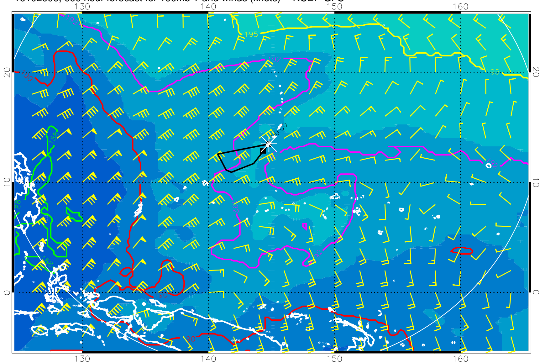
16102000, 090 hour forecast for 100mb T and winds (knots) -- NCEP GFS
