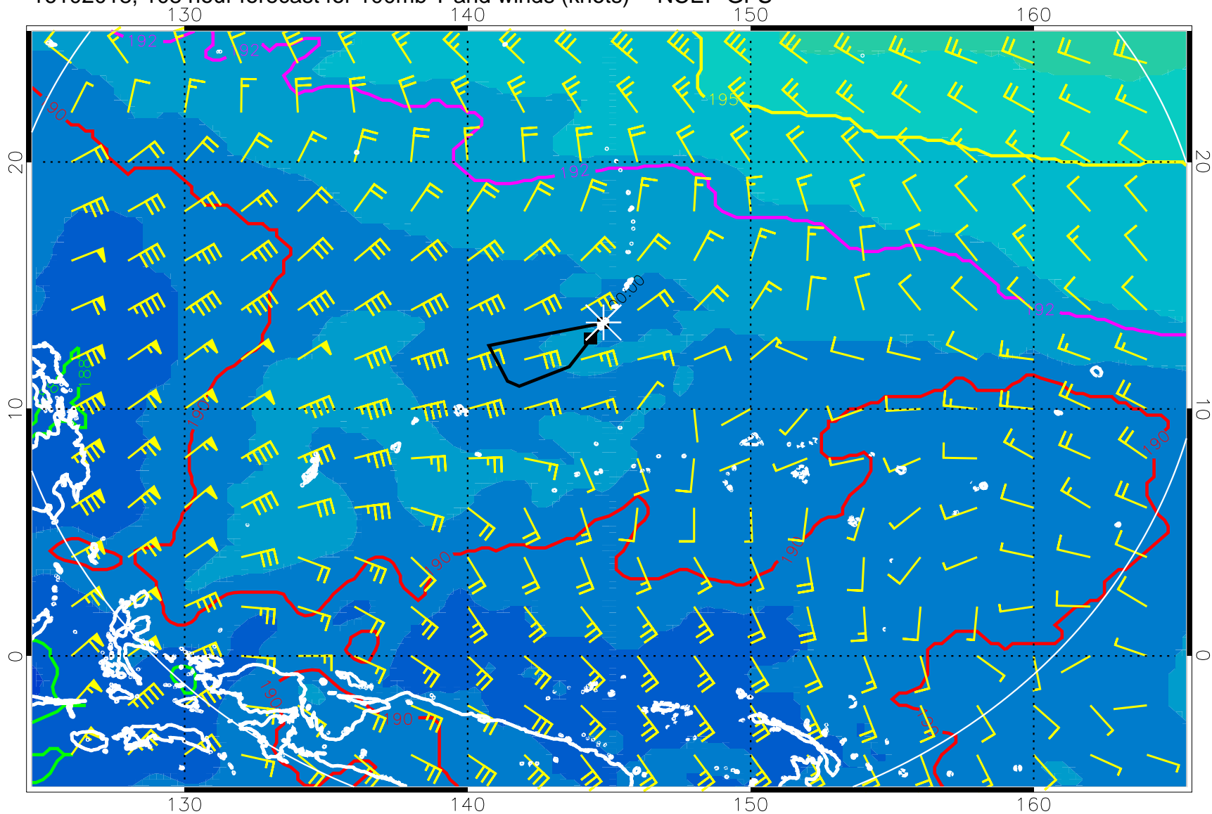
16102018, 108 hour forecast for 100mb T and winds (knots) -- NCEP GFS
