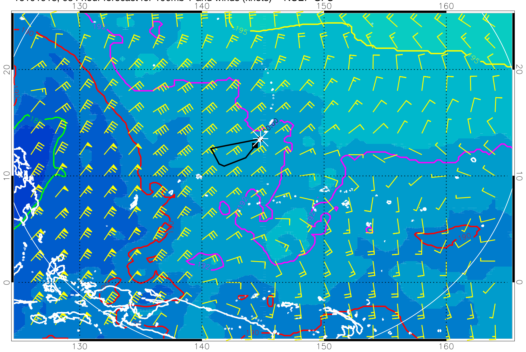
16101918, 084 hour forecast for 100mb T and winds (knots) -- NCEP GFS
