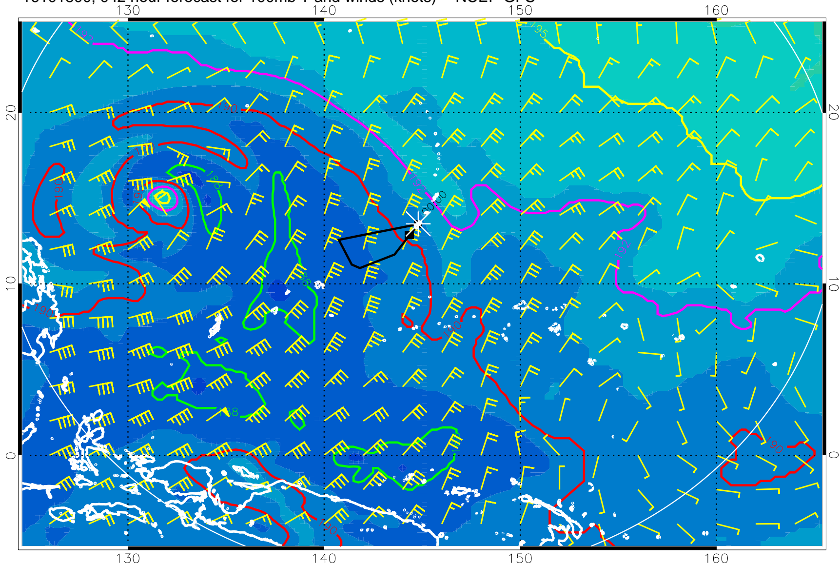
16101800, 042 hour forecast for 100mb T and winds (knots) -- NCEP GFS
