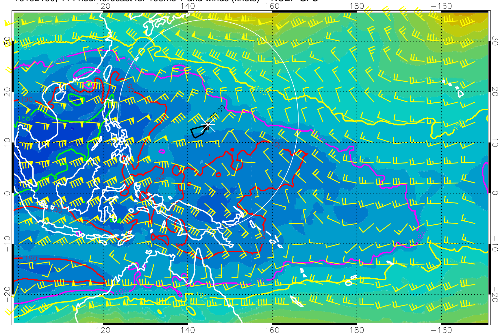
16102100, 114 hour forecast for 100mb T and winds (knots) -- NCEP GFS
