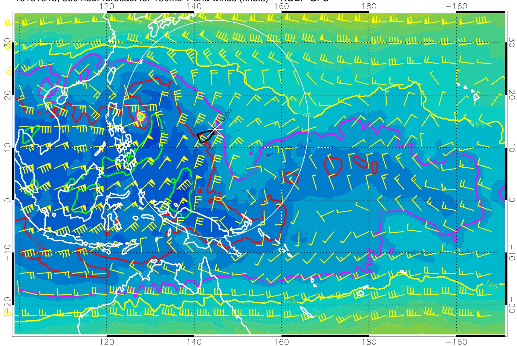
16101818, 060 hour forecast for 100mb T and winds (knots) -- NCEP GFS
