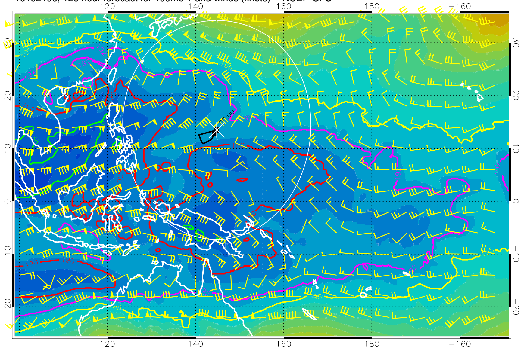
16102106, 120 hour forecast for 100mb T and winds (knots) -- NCEP GFS
