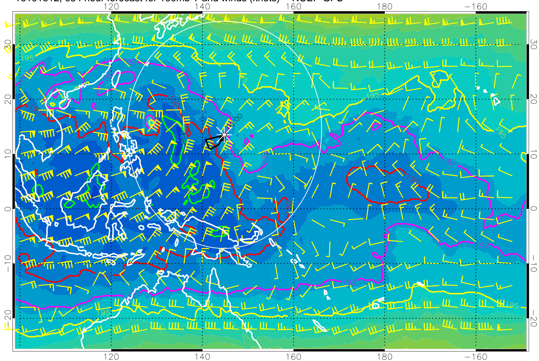
16101812, 054 hour forecast for 100mb T and winds (knots) -- NCEP GFS
