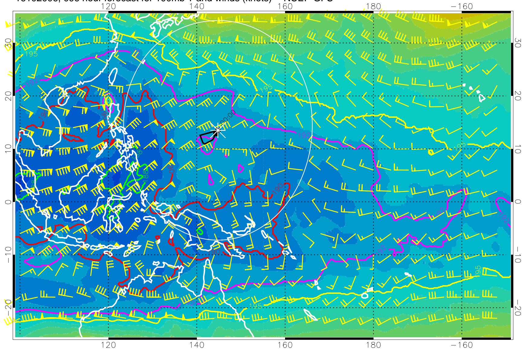
16102006, 096 hour forecast for 100mb T and winds (knots) -- NCEP GFS
