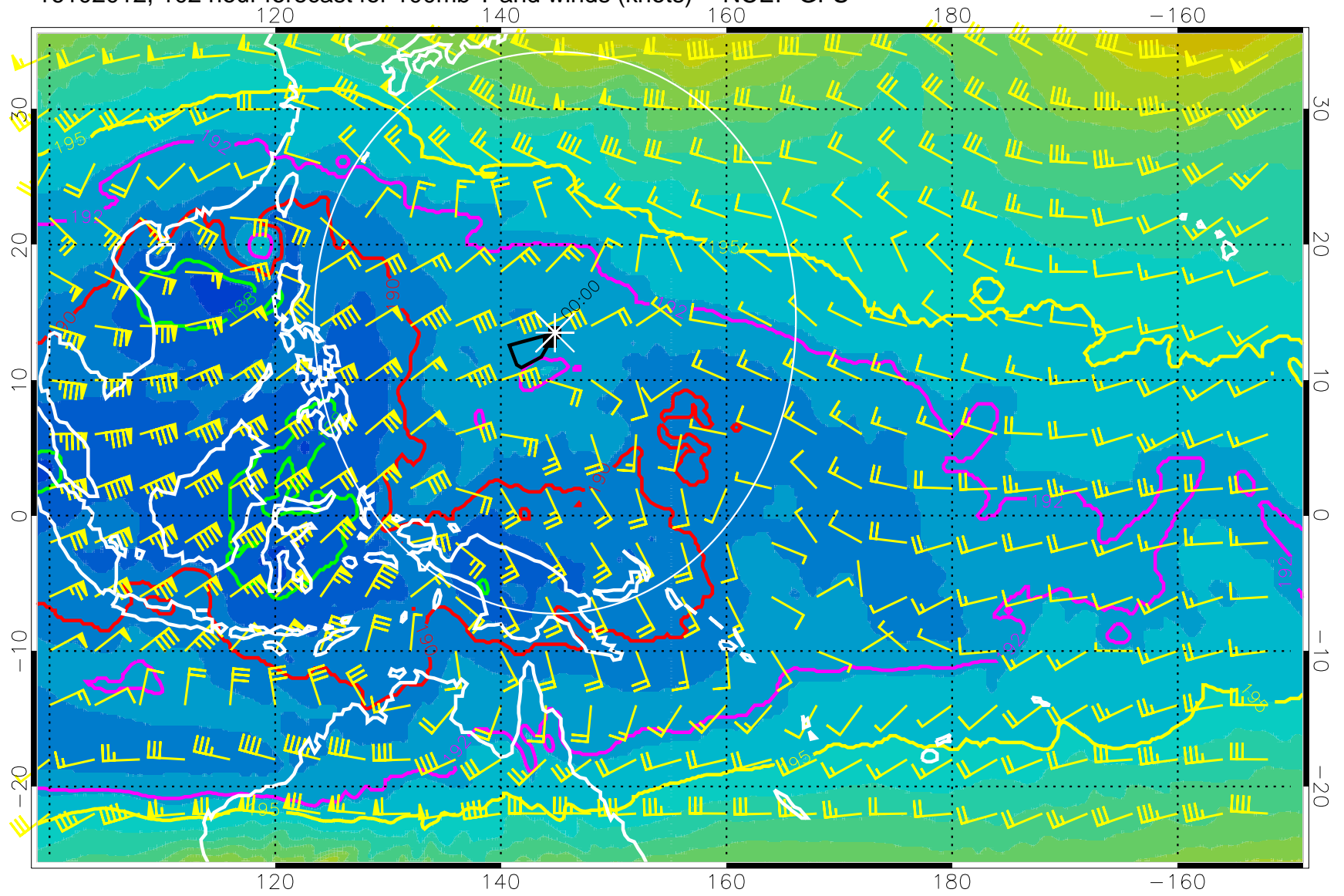
16102012, 102 hour forecast for 100mb T and winds (knots) -- NCEP GFS
