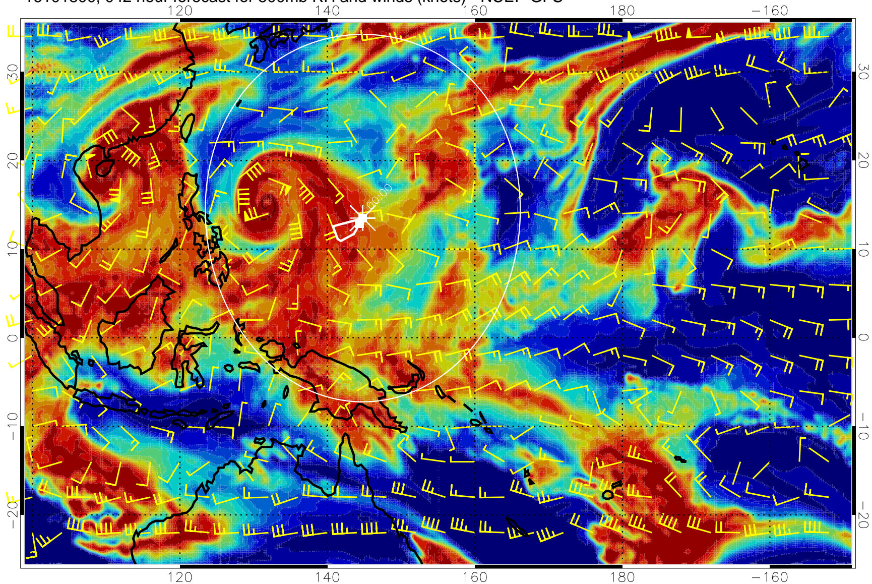
16101800, 042 hour forecast for 500mb RH and winds (knots) - NCEP GFS
