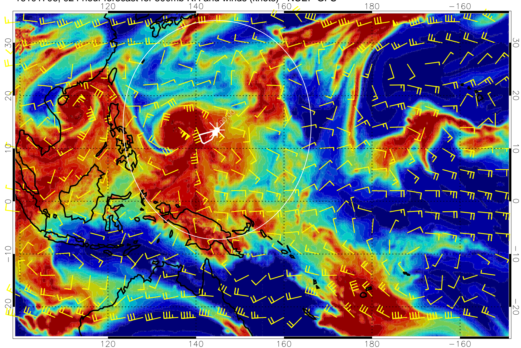
16101706, 024 hour forecast for 500mb RH and winds (knots) - NCEP GFS
