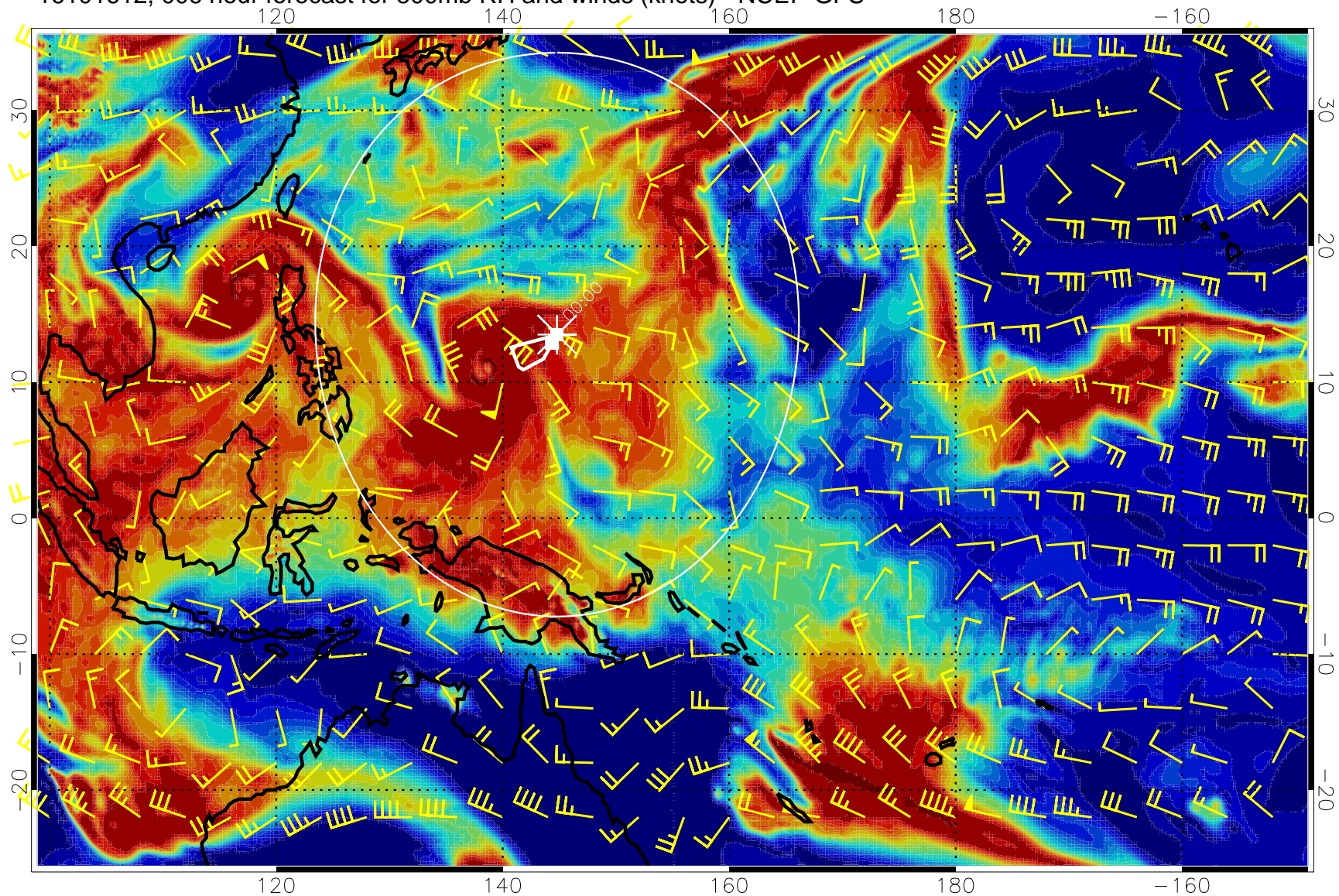
16101612, 006 hour forecast for 500mb RH and winds (knots) - NCEP GFS
