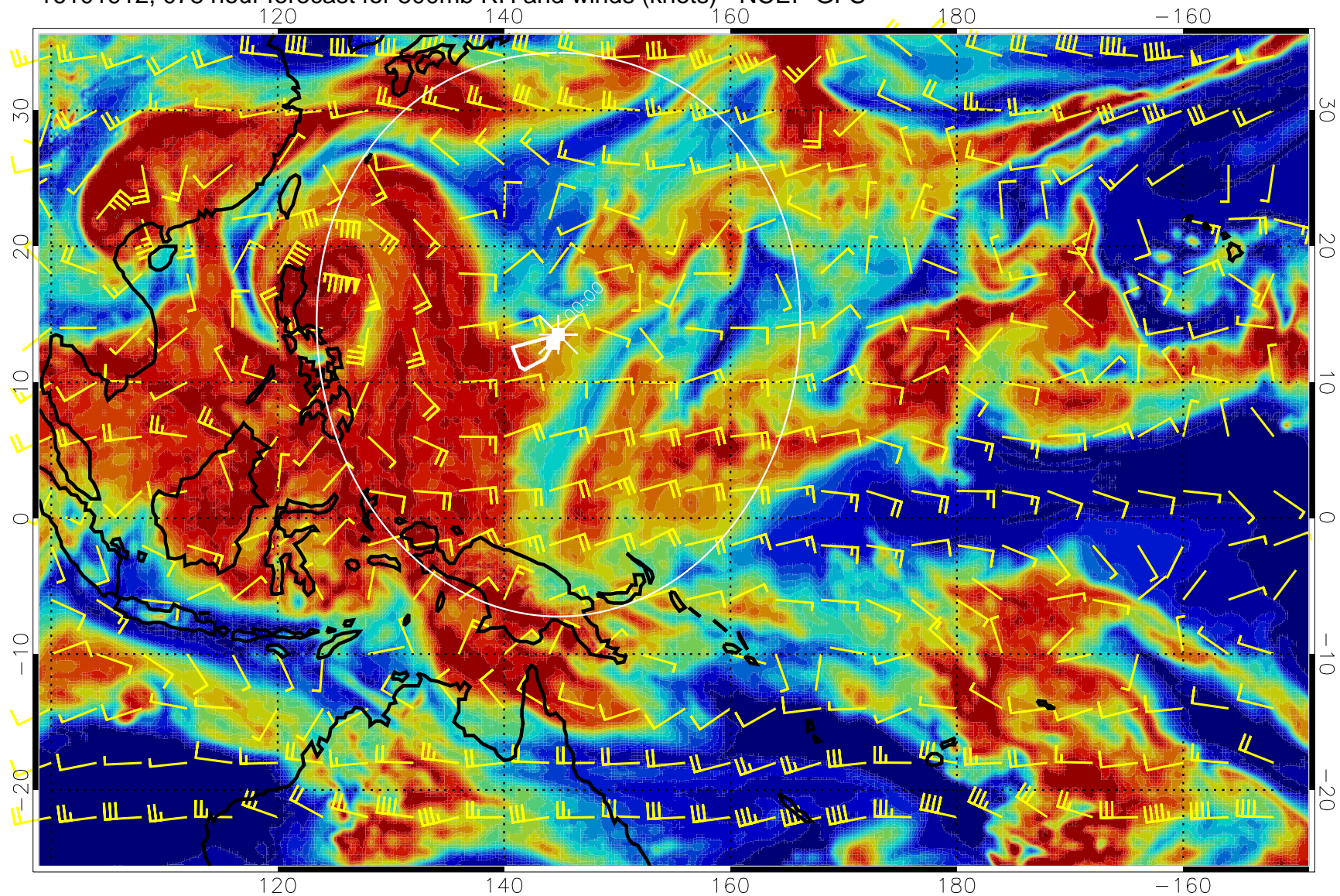
16101912, 078 hour forecast for 500mb RH and winds (knots) - NCEP GFS
