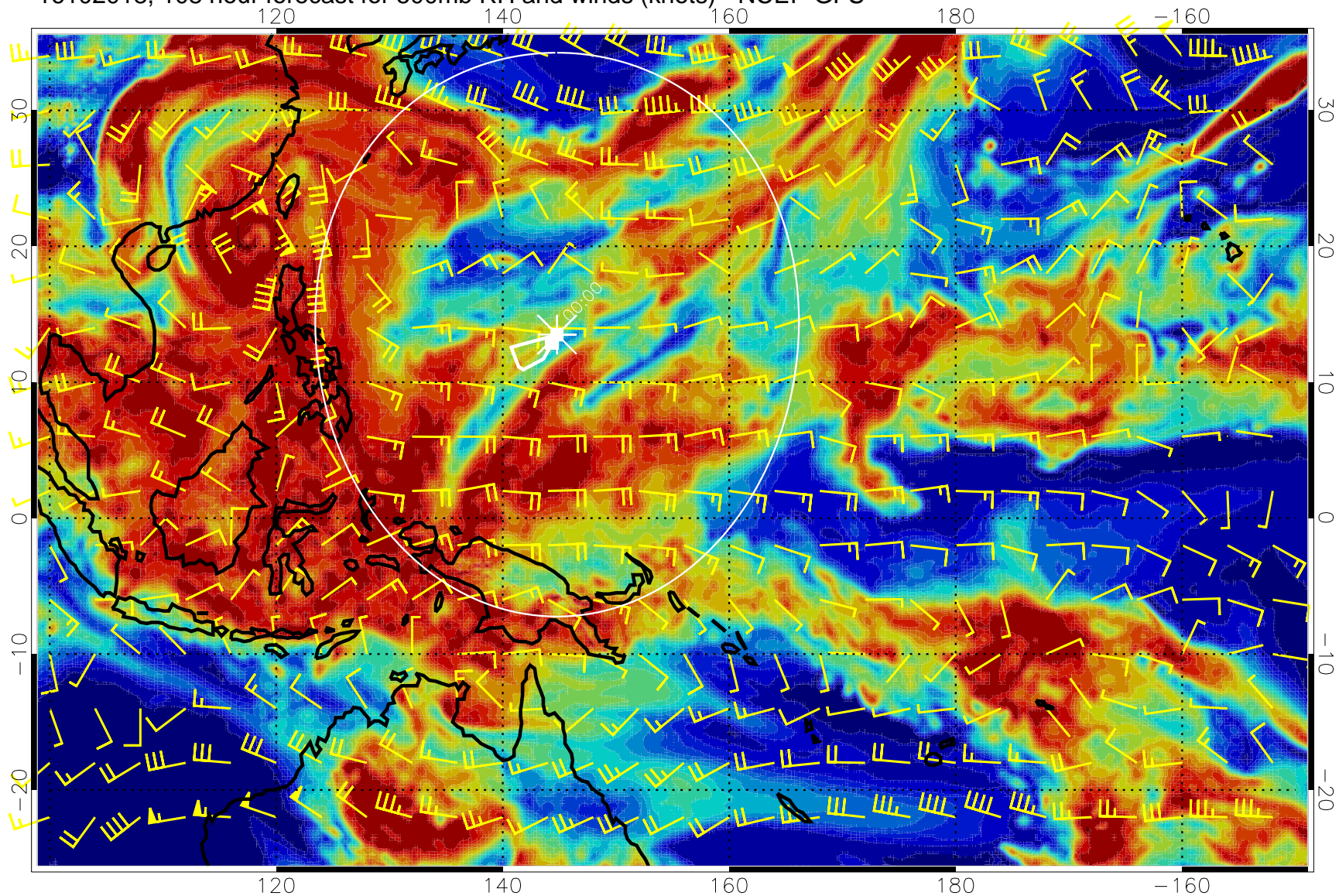
16102018, 108 hour forecast for 500mb RH and winds (knots) - NCEP GFS
