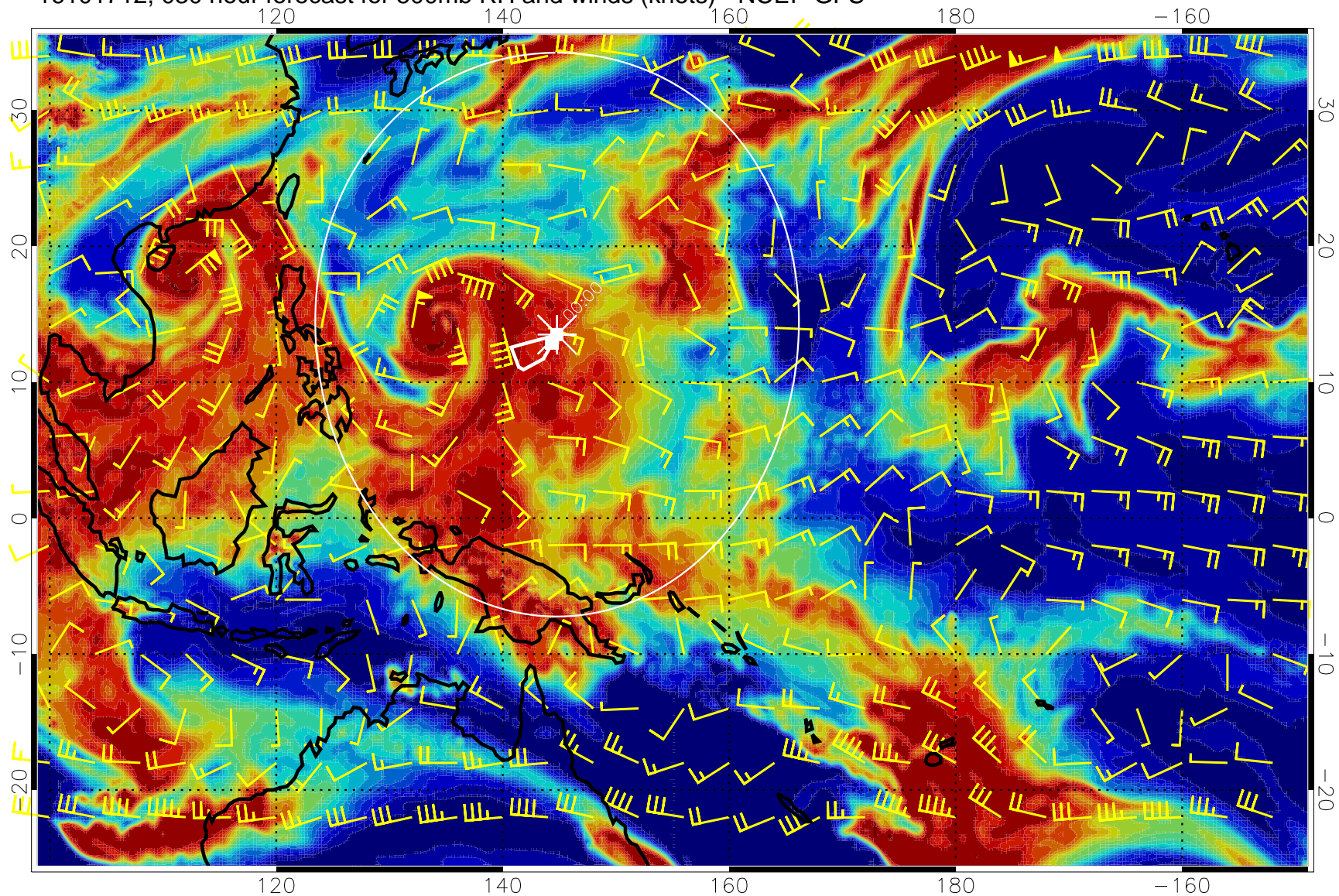
16101712, 030 hour forecast for 500mb RH and winds (knots) - NCEP GFS
