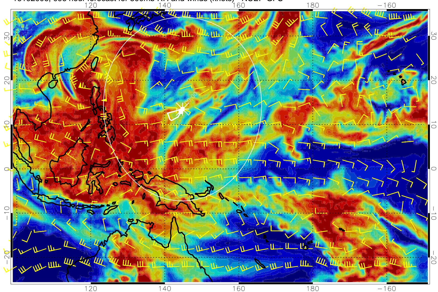
16102006, 096 hour forecast for 500mb RH and winds (knots) - NCEP GFS
