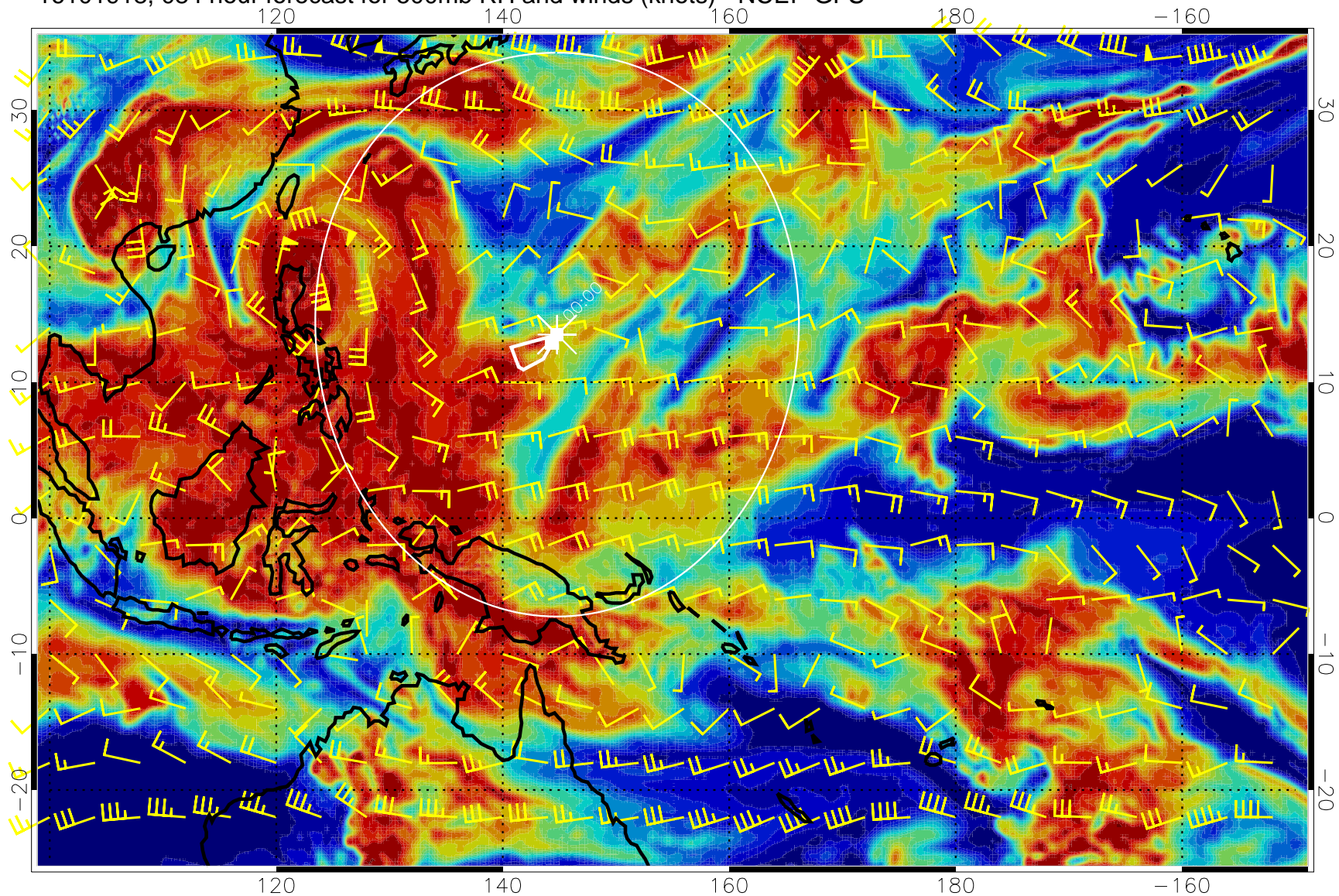
16101918, 084 hour forecast for 500mb RH and winds (knots) - NCEP GFS
