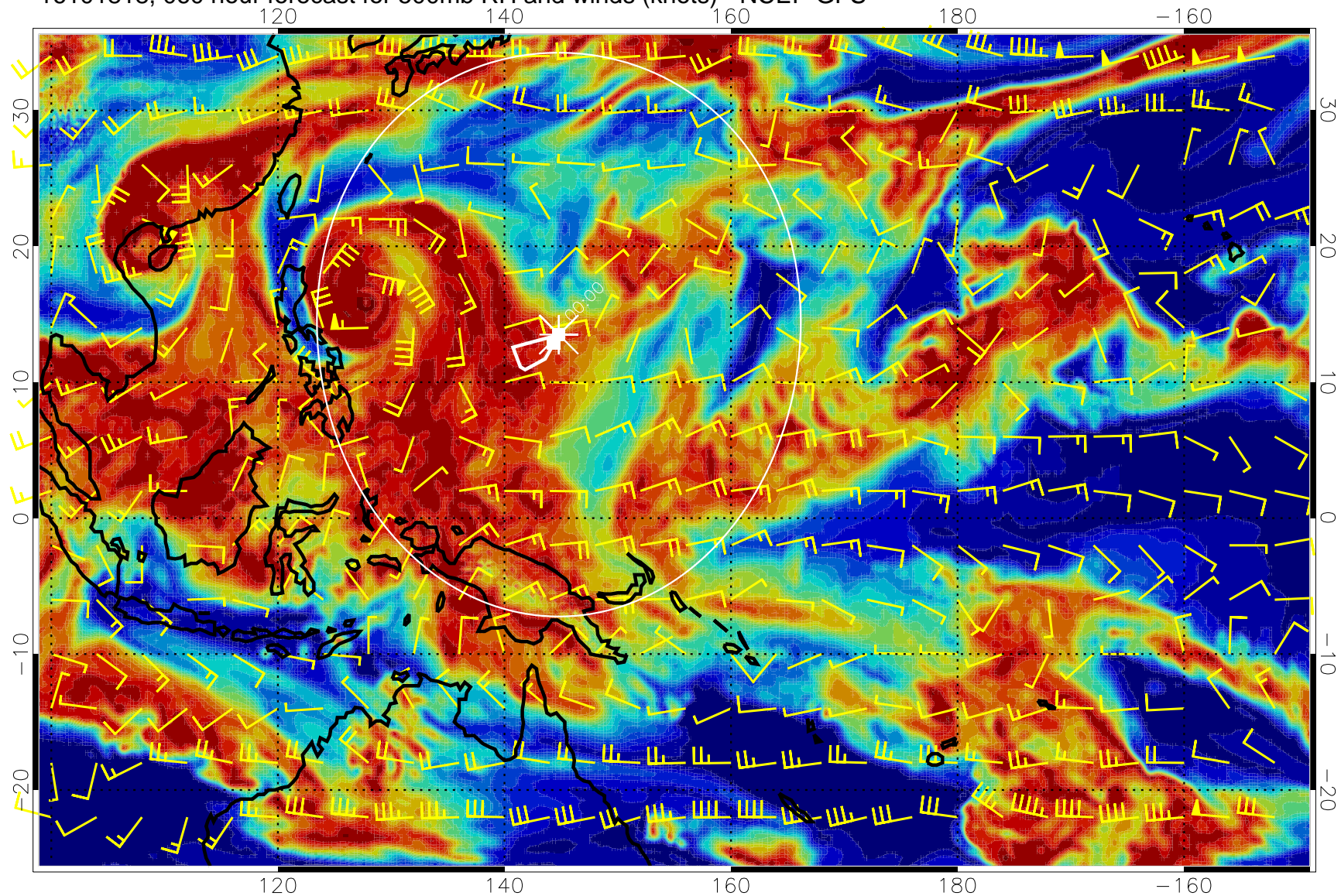
16101818, 060 hour forecast for 500mb RH and winds (knots) - NCEP GFS
