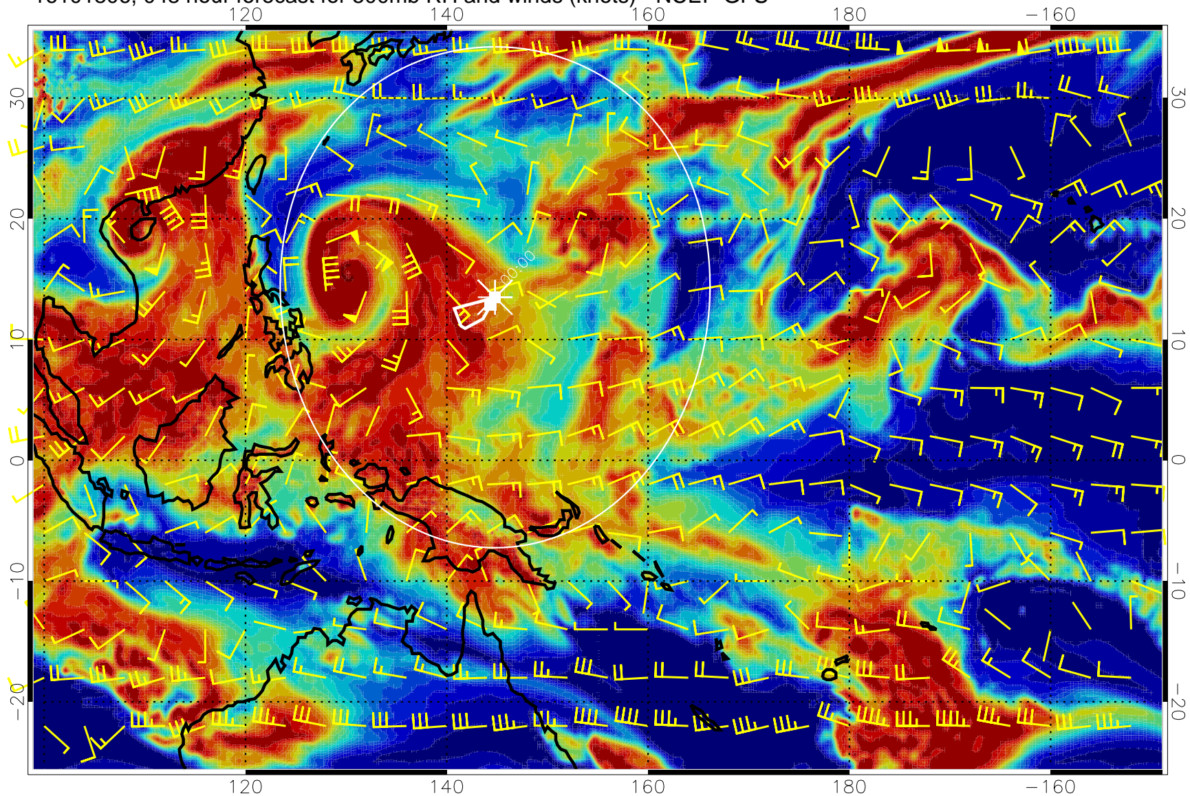
16101806, 048 hour forecast for 500mb RH and winds (knots) - NCEP GFS
