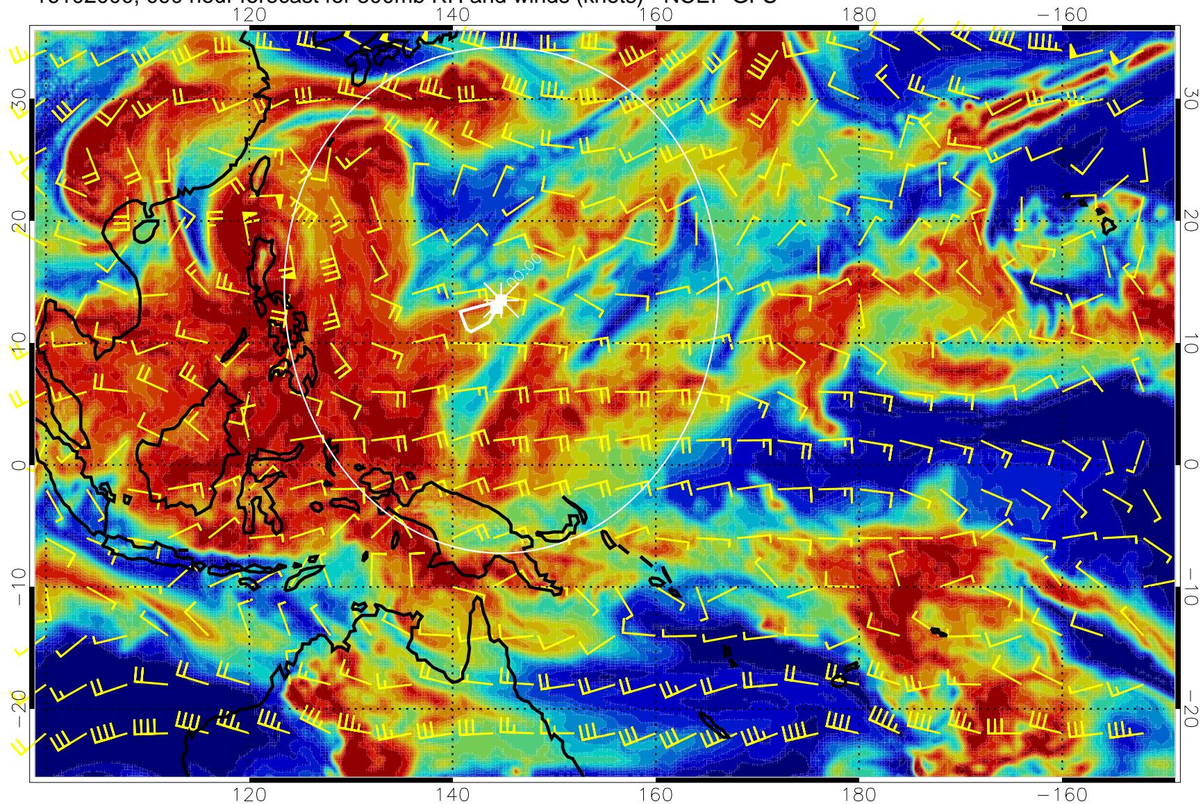
16102000, 090 hour forecast for 500mb RH and winds (knots) - NCEP GFS
