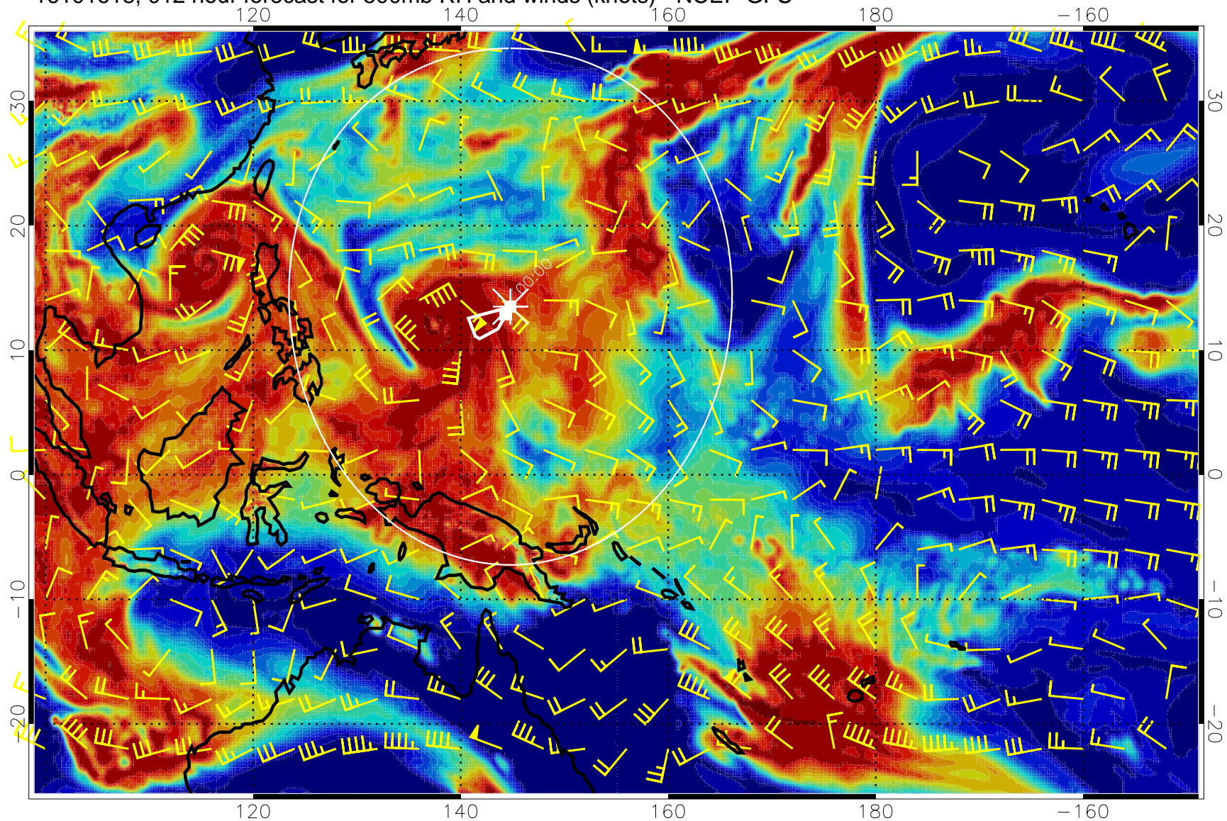
16101618, 012 hour forecast for 500mb RH and winds (knots) - NCEP GFS
