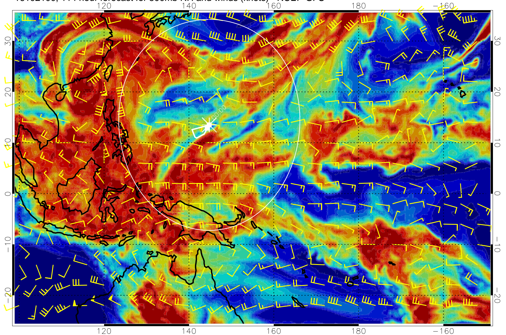
16102100, 114 hour forecast for 500mb RH and winds (knots) - NCEP GFS
