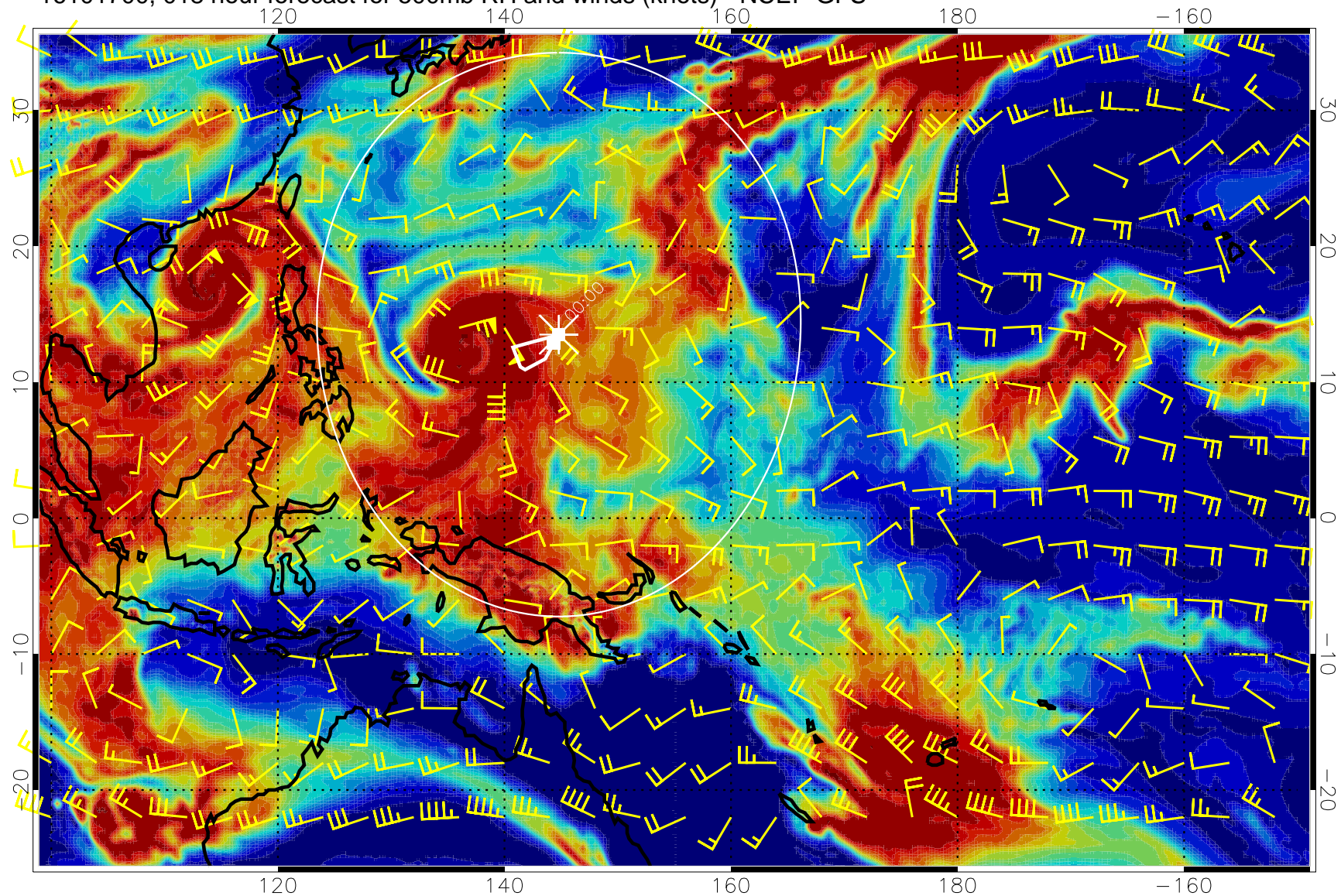
16101700, 018 hour forecast for 500mb RH and winds (knots) - NCEP GFS
