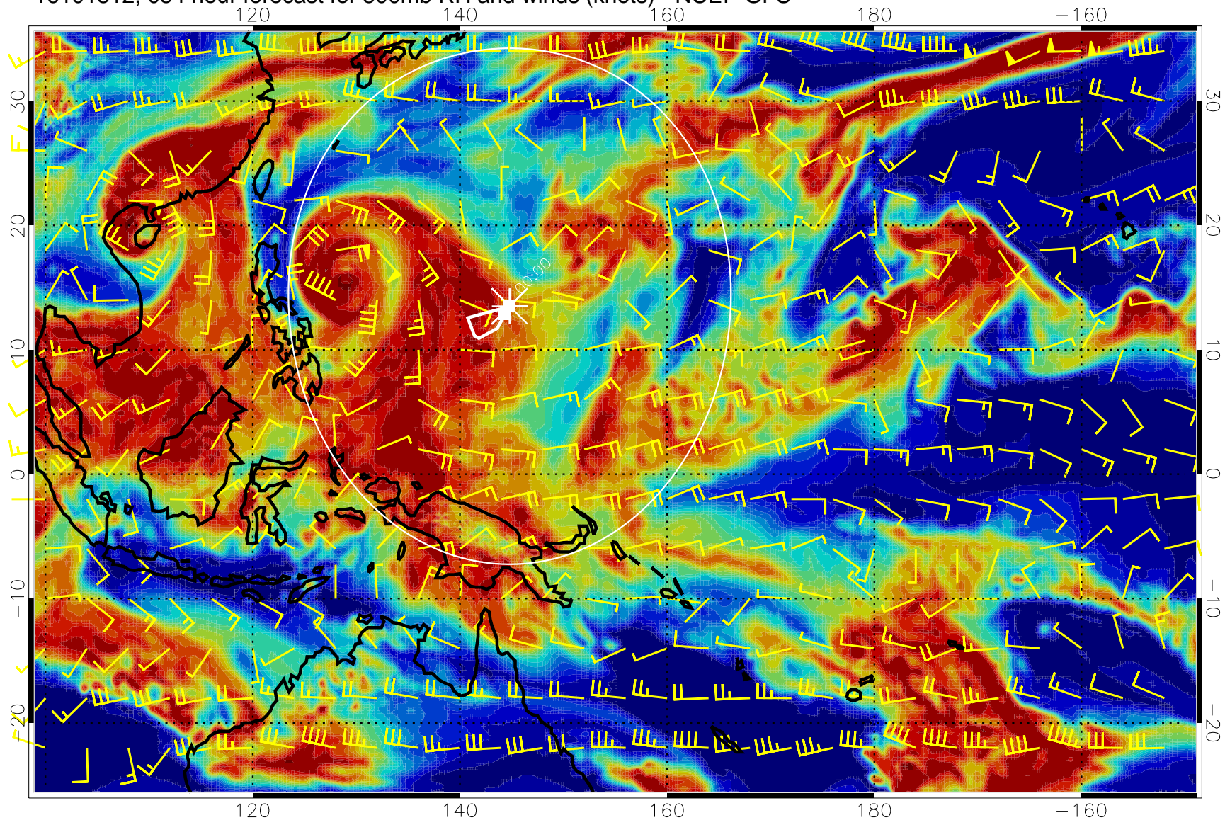
16101812, 054 hour forecast for 500mb RH and winds (knots) - NCEP GFS
