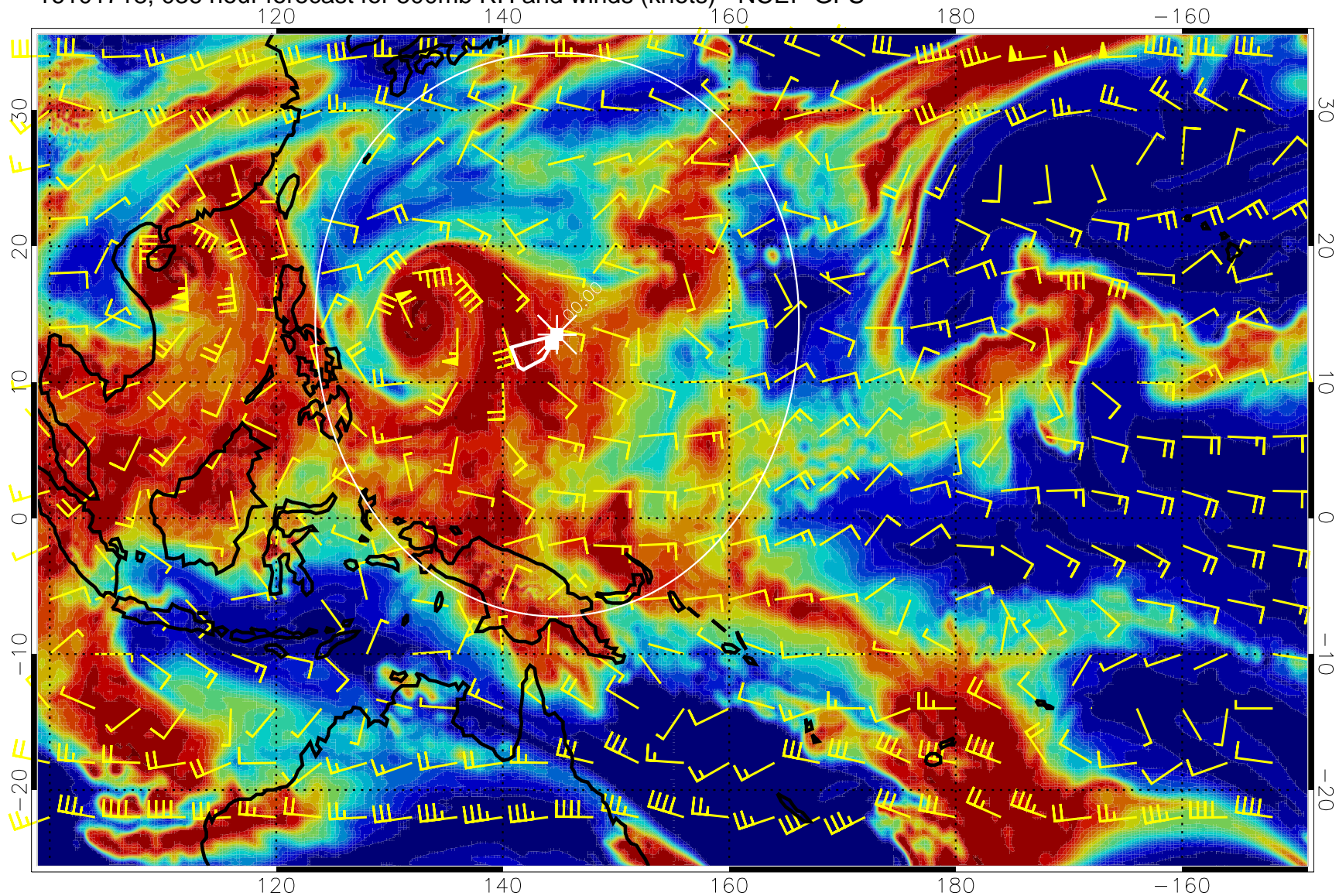
16101718, 036 hour forecast for 500mb RH and winds (knots) - NCEP GFS
