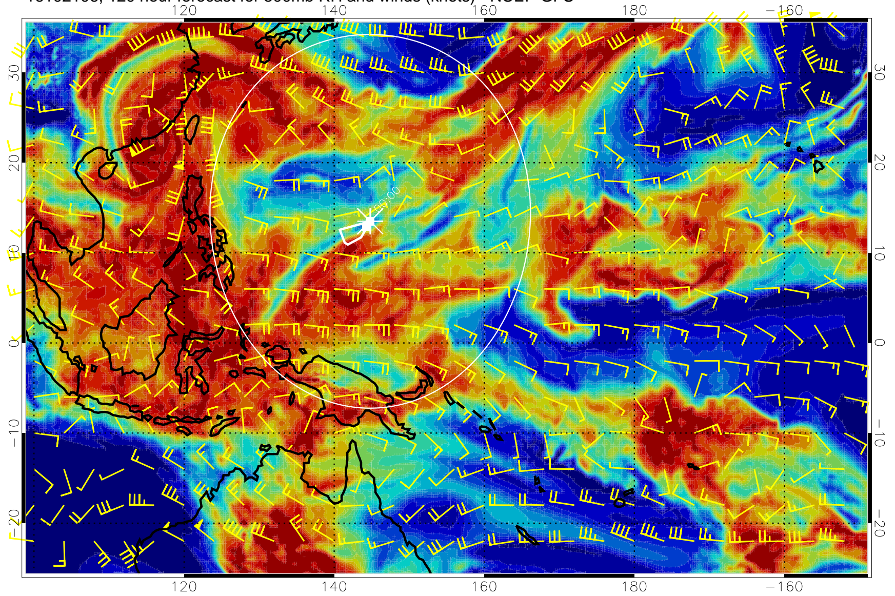
16102106, 120 hour forecast for 500mb RH and winds (knots) - NCEP GFS
