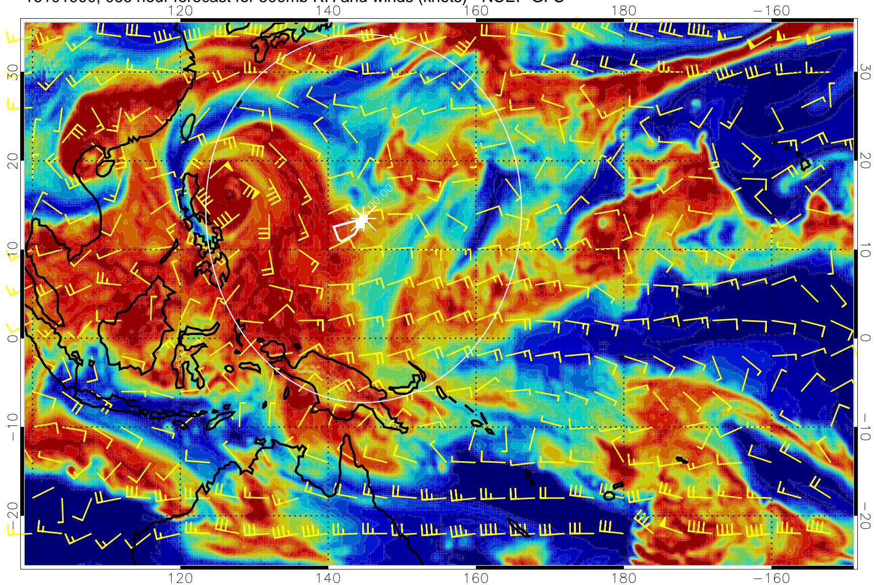
16101900, 066 hour forecast for 500mb RH and winds (knots) - NCEP GFS
