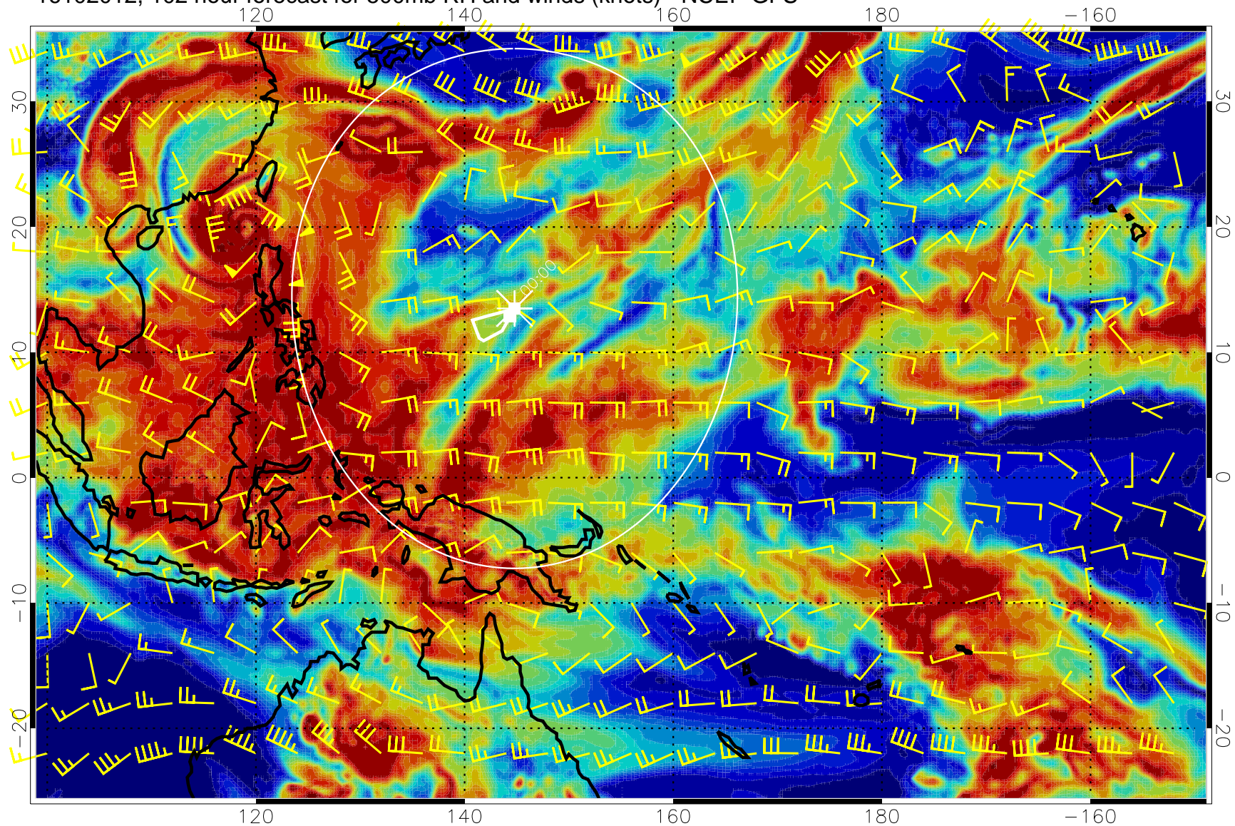
16102012, 102 hour forecast for 500mb RH and winds (knots) - NCEP GFS
