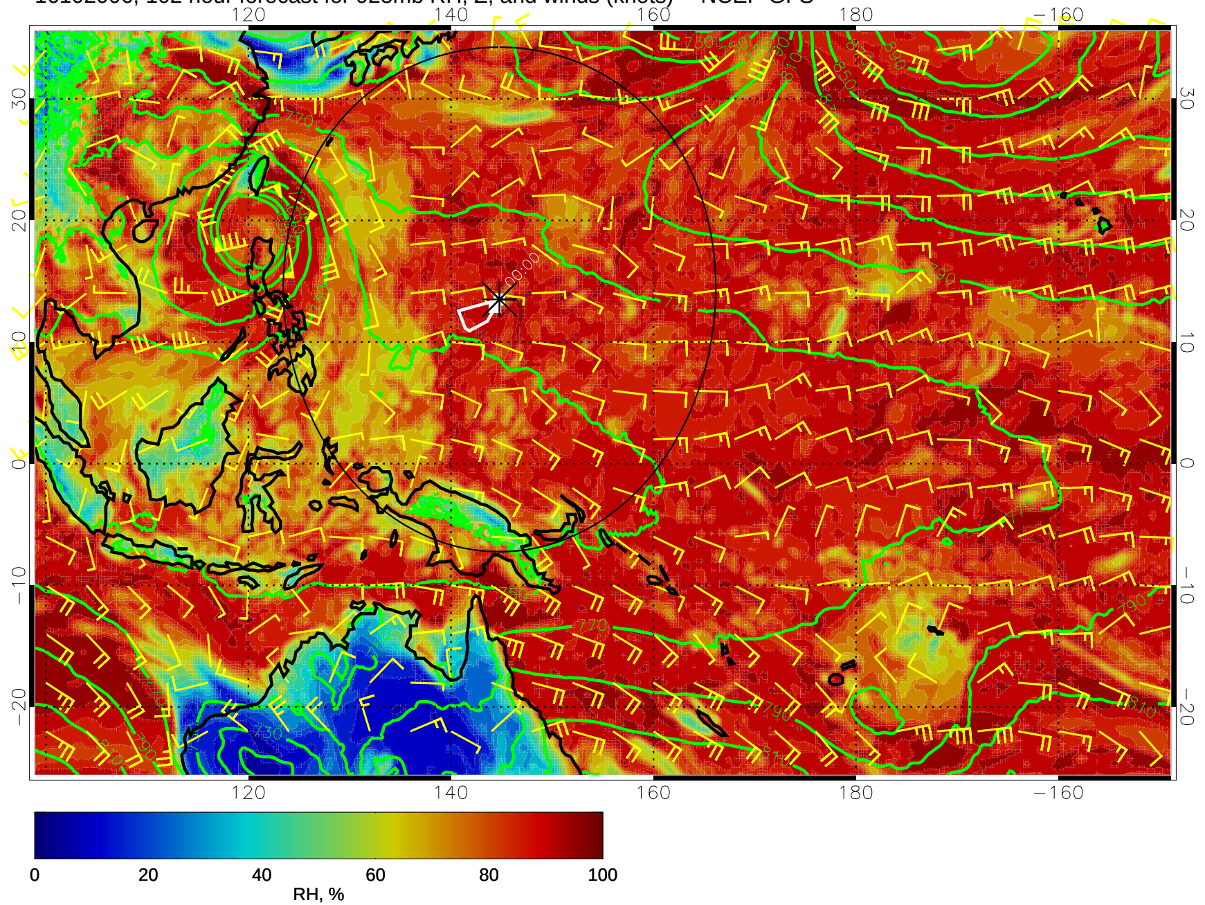
16102006, 102 hour forecast for 925mb RH, Z, and winds (knots) -- NCEP GFS
