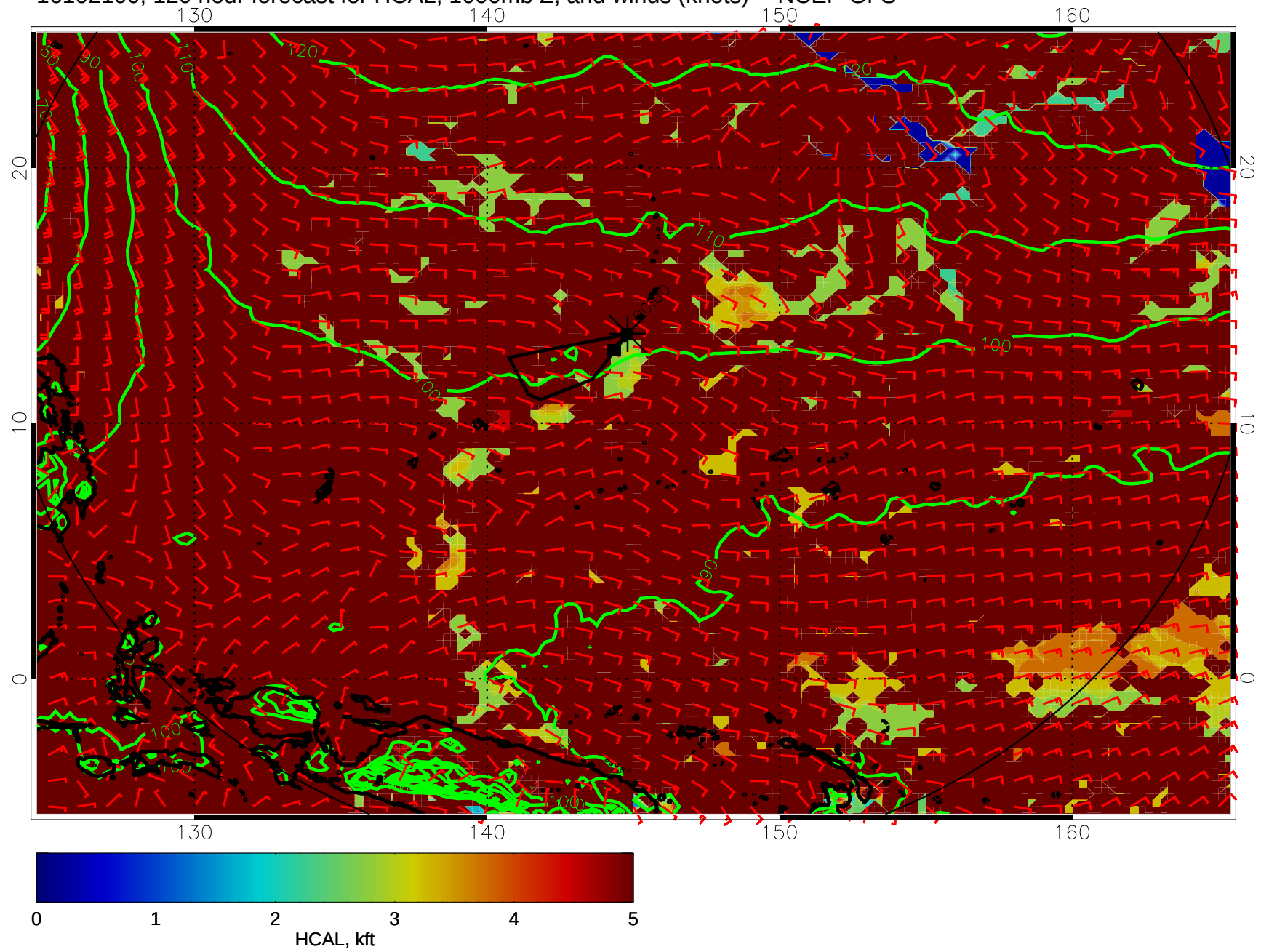
16102100, 120 hour forecast for HCAL, 1000mb Z, and winds (knots) -- NCEP GFS
