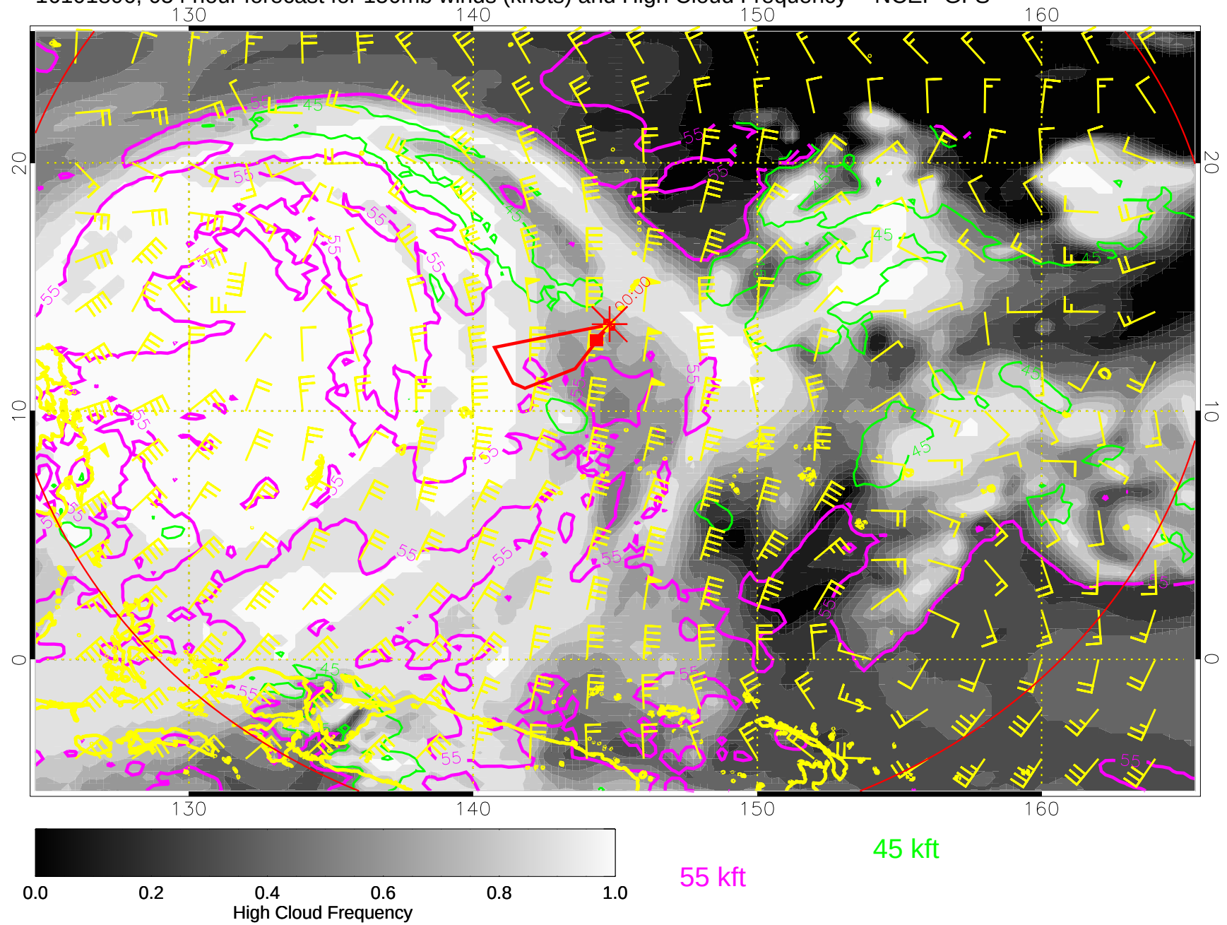
16101806, 054 hour forecast for 150mb winds (knots) and High Cloud Frequency -- NCEP GFS
