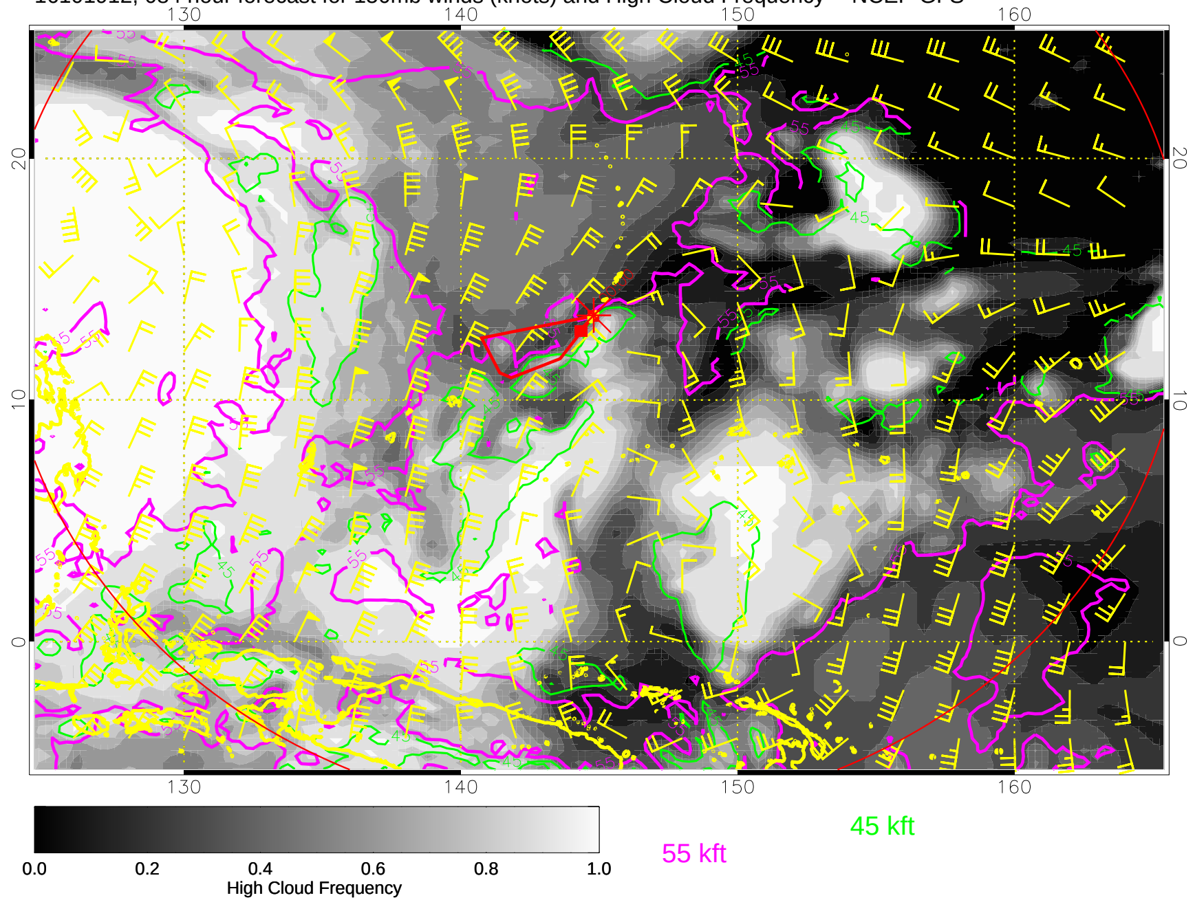
16101912, 084 hour forecast for 150mb winds (knots) and High Cloud Frequency -- NCEP GFS
