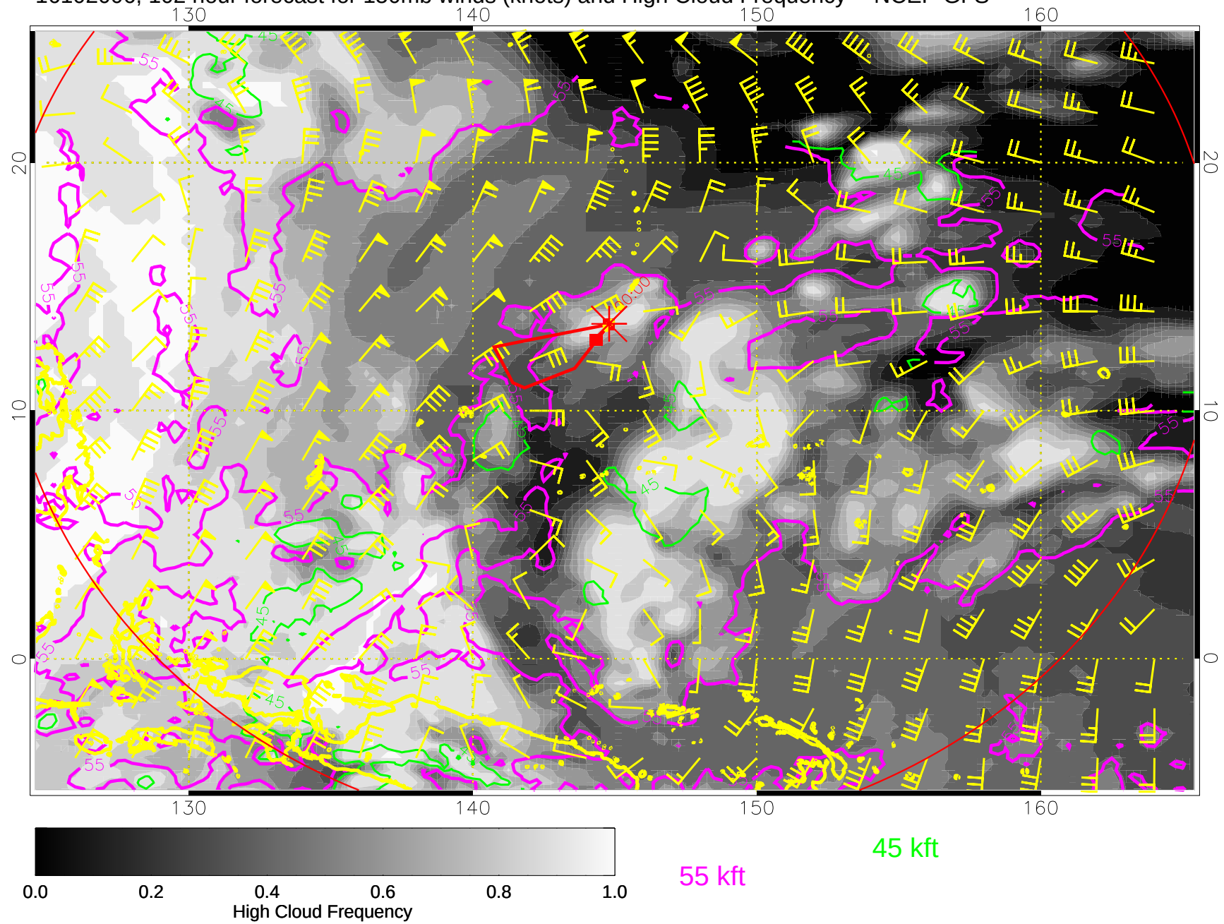
16102006, 102 hour forecast for 150mb winds (knots) and High Cloud Frequency -- NCEP GFS
