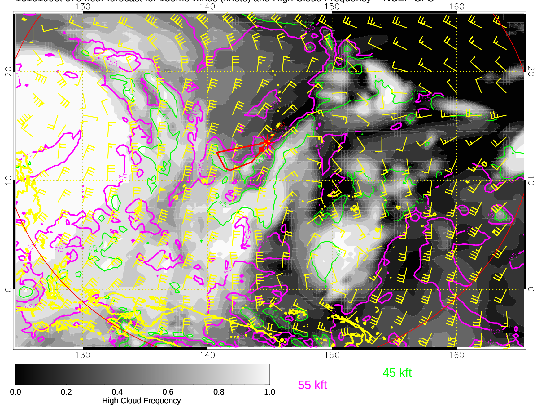
16101906, 078 hour forecast for 150mb winds (knots) and High Cloud Frequency -- NCEP GFS
