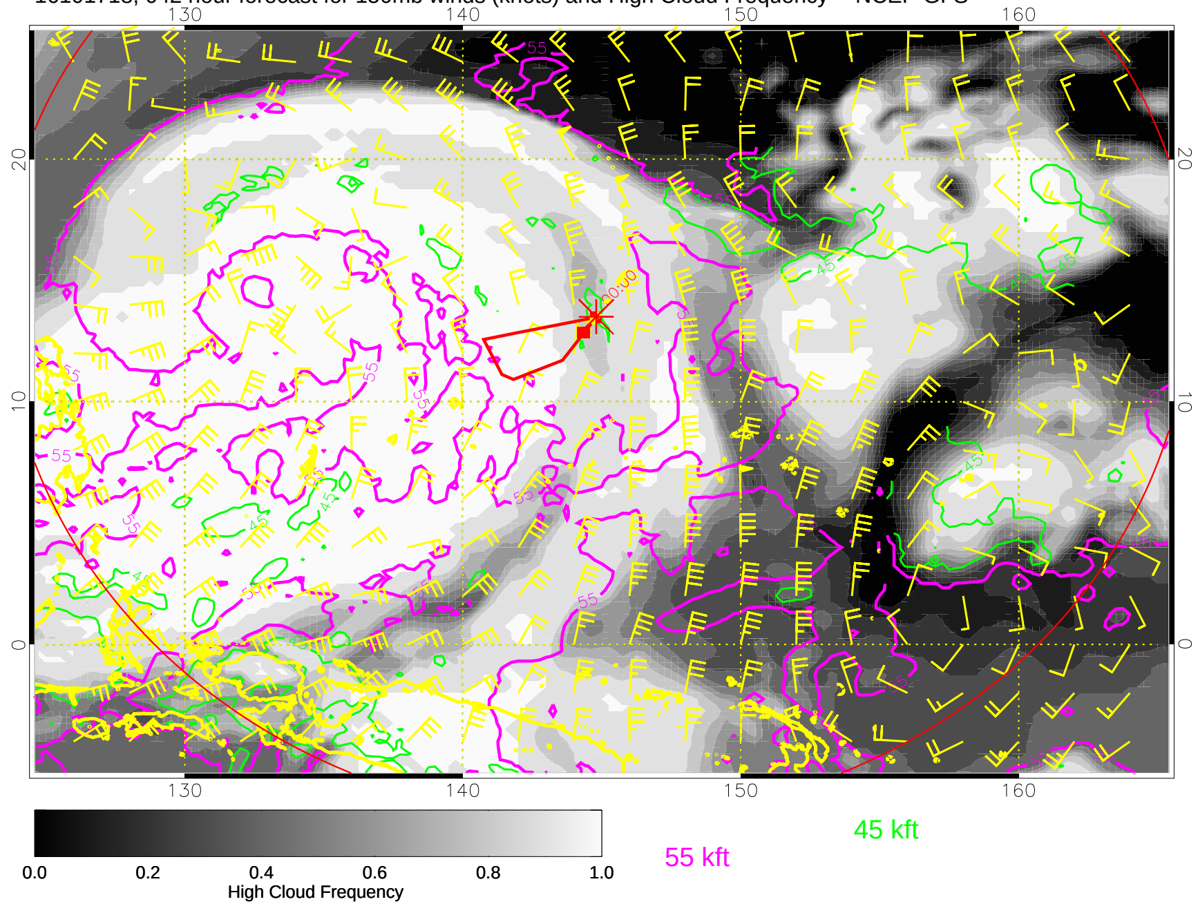
16101718, 04Z hour forecast for 150mb winds (knots) and High Cloud Frequency -- NCEP GFS
