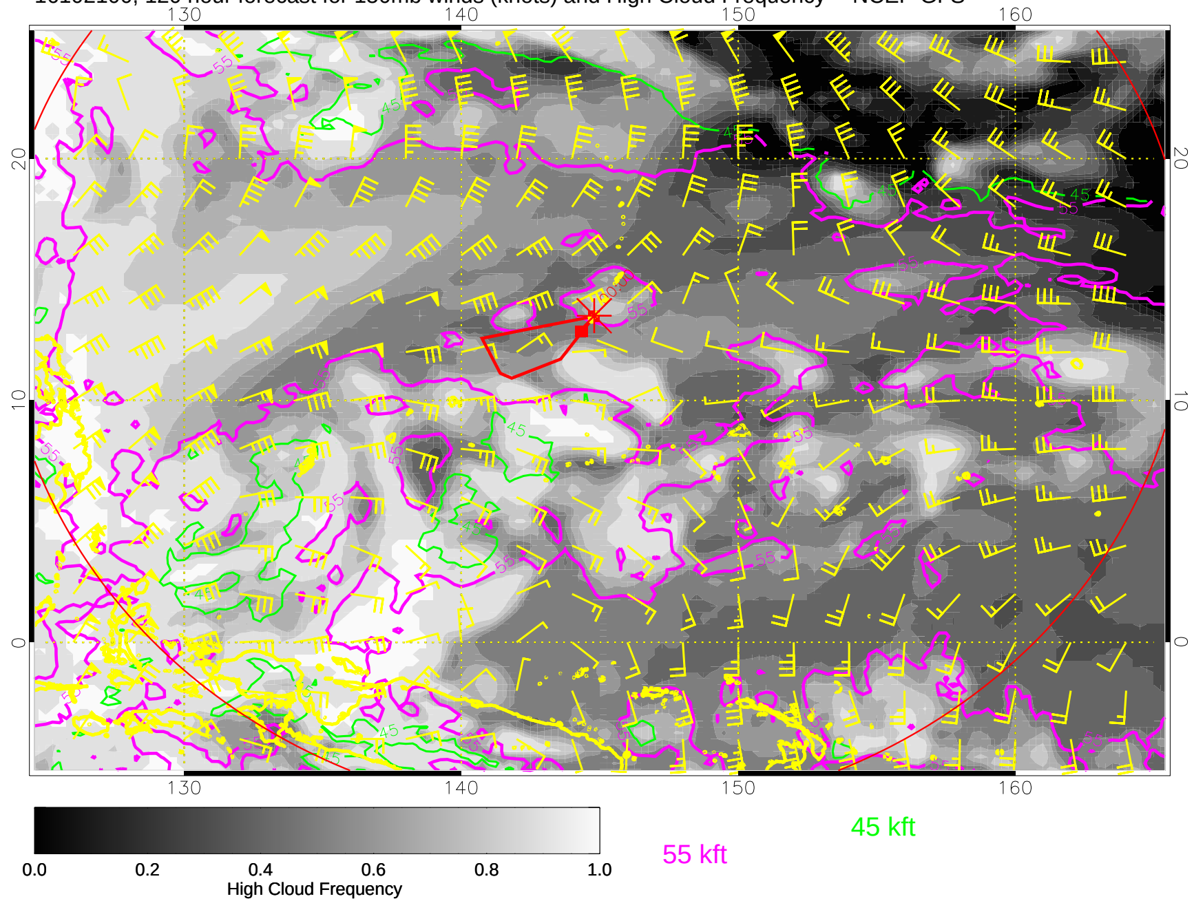
16102100, 120 hour forecast for 150mb winds (knots) and High Cloud Frequency -- NCEP GFS
