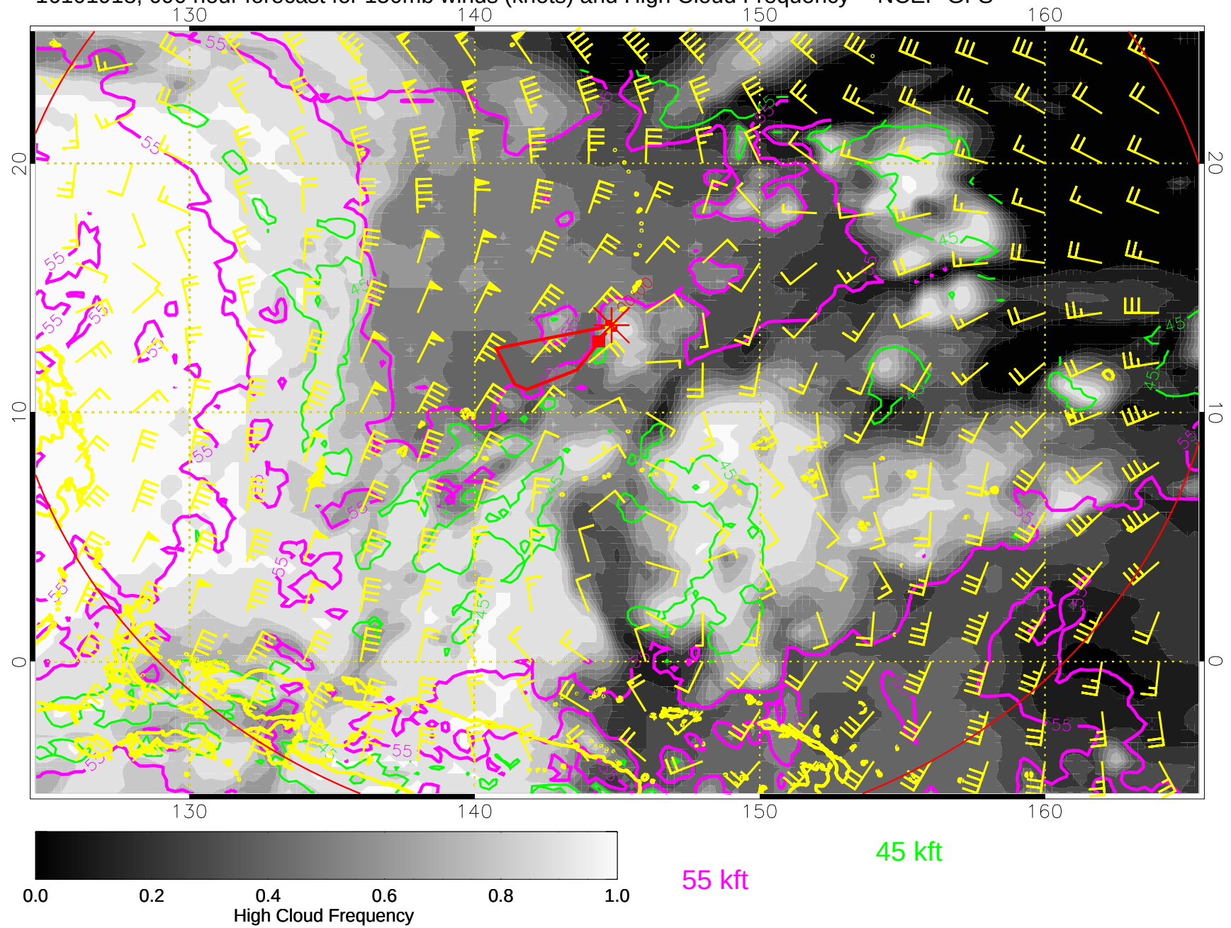
16101918, 090 hour forecast for 150mb winds (knots) and High Cloud Frequency -- NCEP GFS
