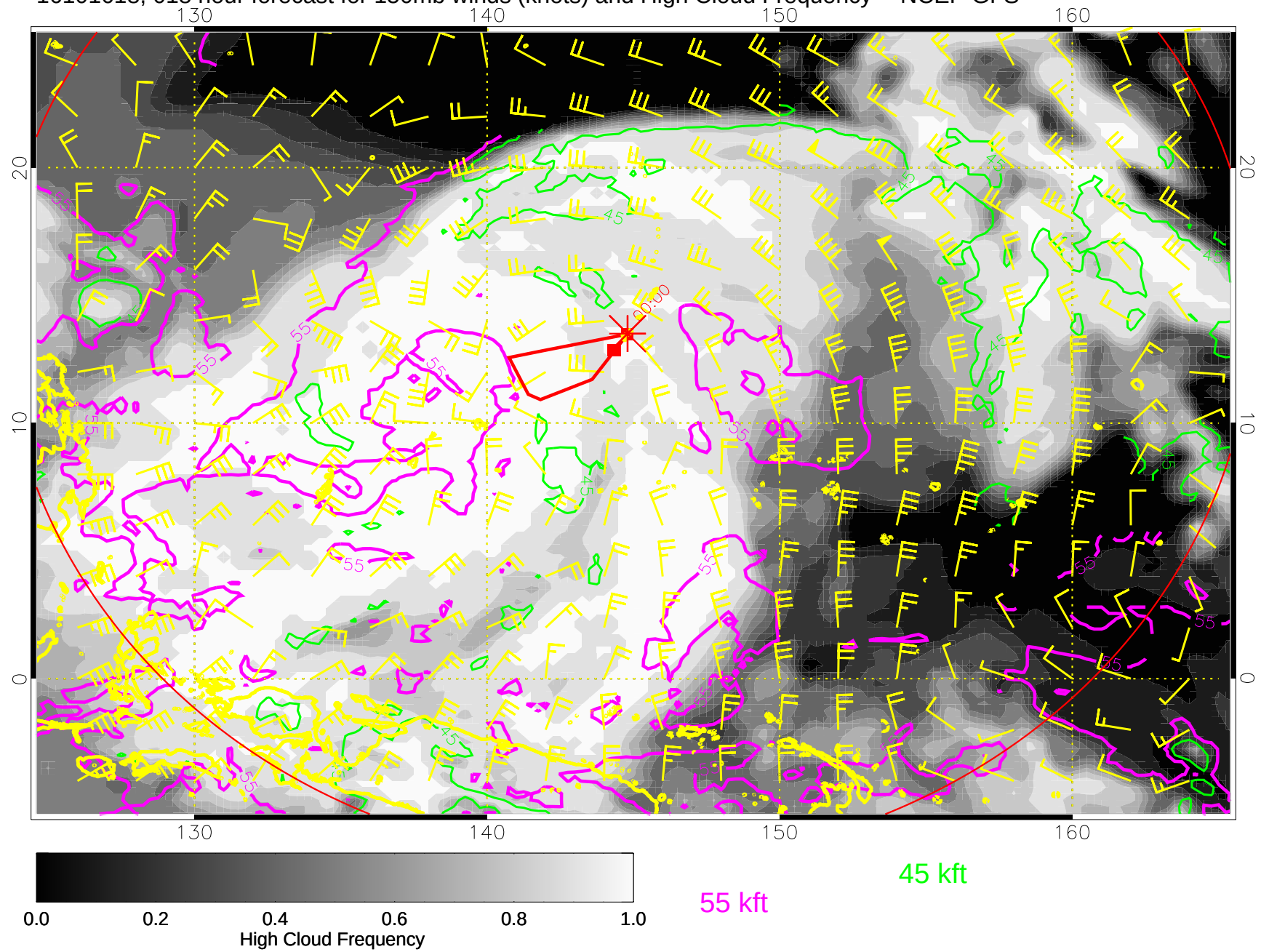
16101618, 018 hour forecast for 150mb winds (knots) and High Cloud Frequency -- NCEP GFS
