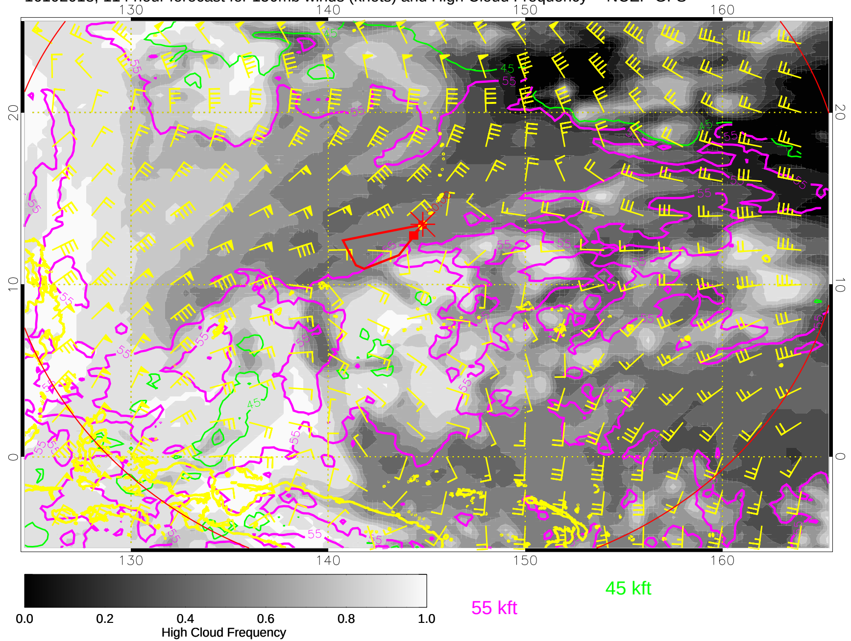
16102018, 114 hour forecast for 150mb winds (knots) and High Cloud Frequency -- NCEP GFS
