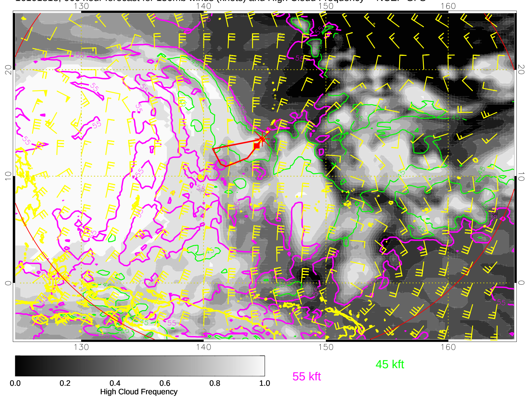
16101818, 066 hour forecast for 150mb winds (knots) and High Cloud Frequency -- NCEP GFS
