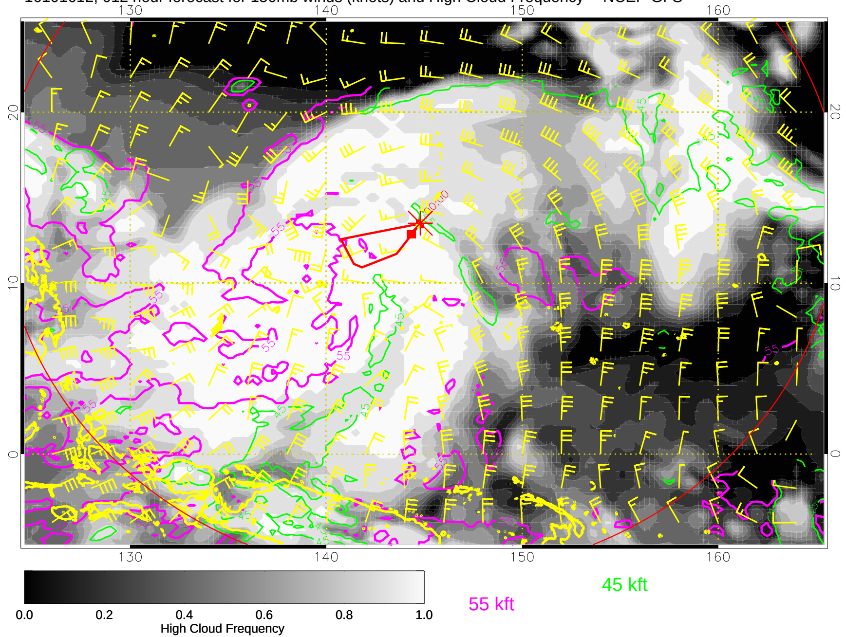
16101612, 012 hour forecast for 150mb winds (knots) and High Cloud Frequency -- NCEP GFS
