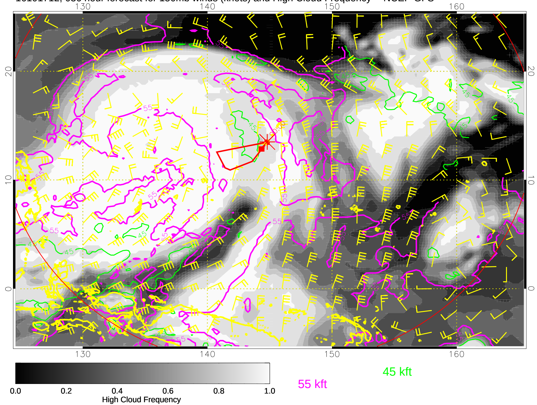
16101712, 036 hour forecast for 150mb winds (knots) and High Cloud Frequency -- NCEP GFS
