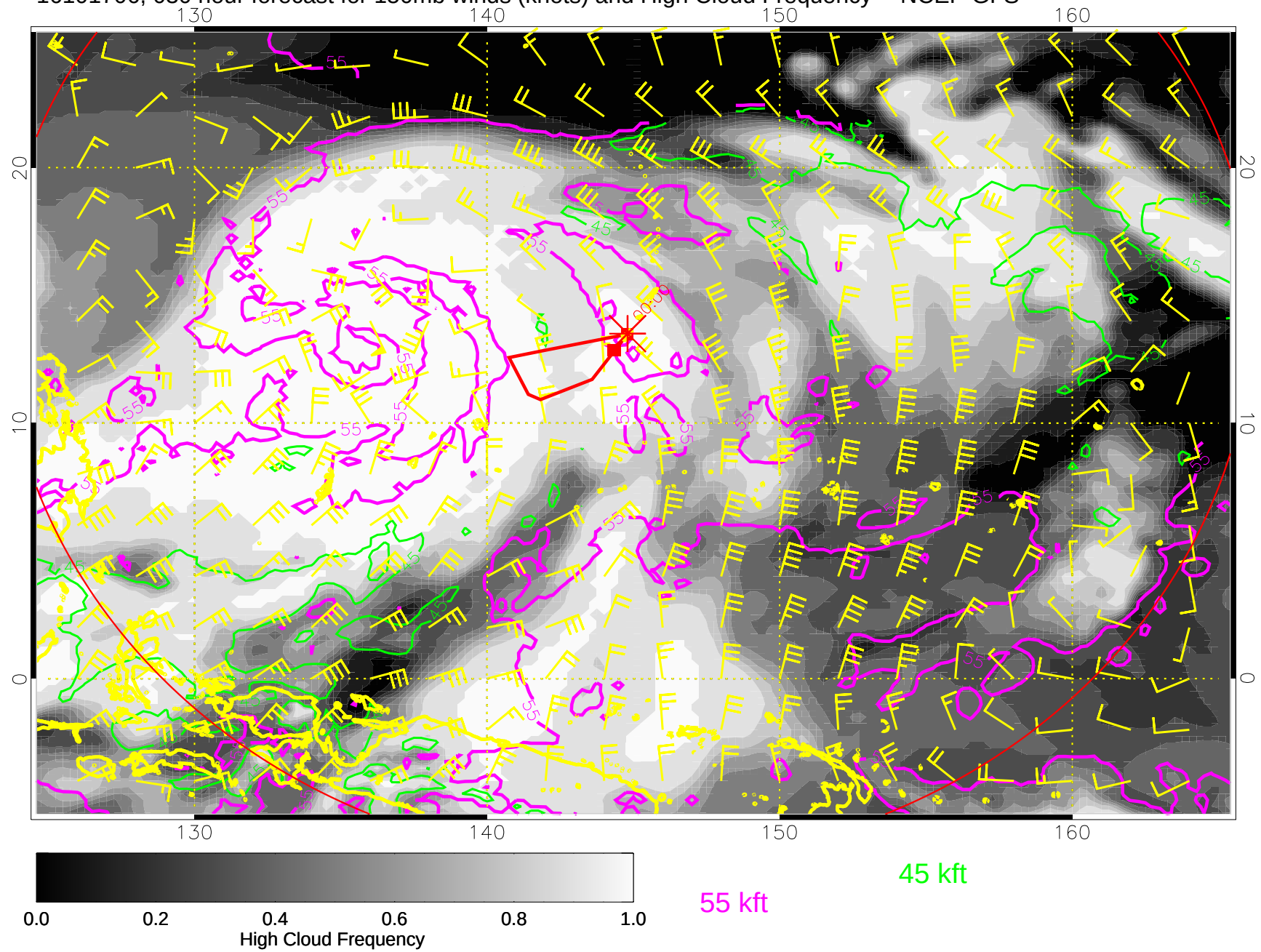
16101706, 030 hour forecast for 150mb winds (knots) and High Cloud Frequency -- NCEP GFS
