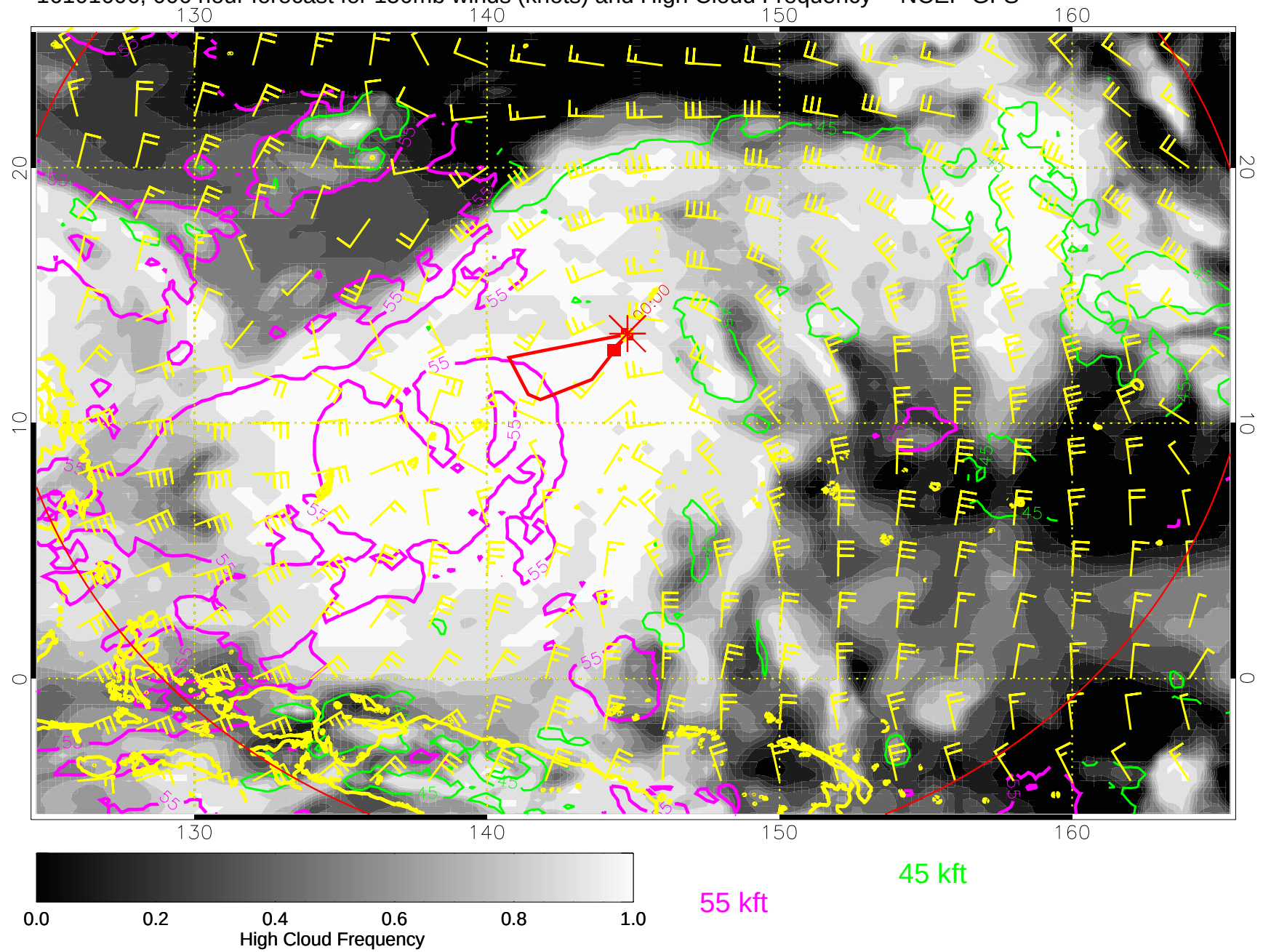
16101606, 006 hour forecast for 150mb winds (knots) and High Cloud Frequency -- NCEP GFS
