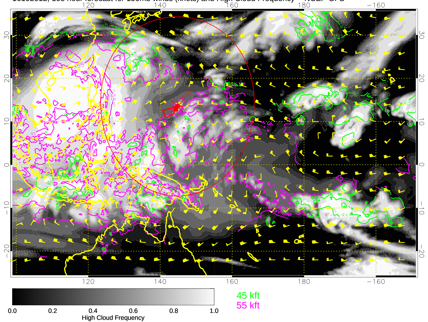
16102012, 108 hour forecast for 150mb winds (knots) and High Cloud Frequency -- NCEP GFS
