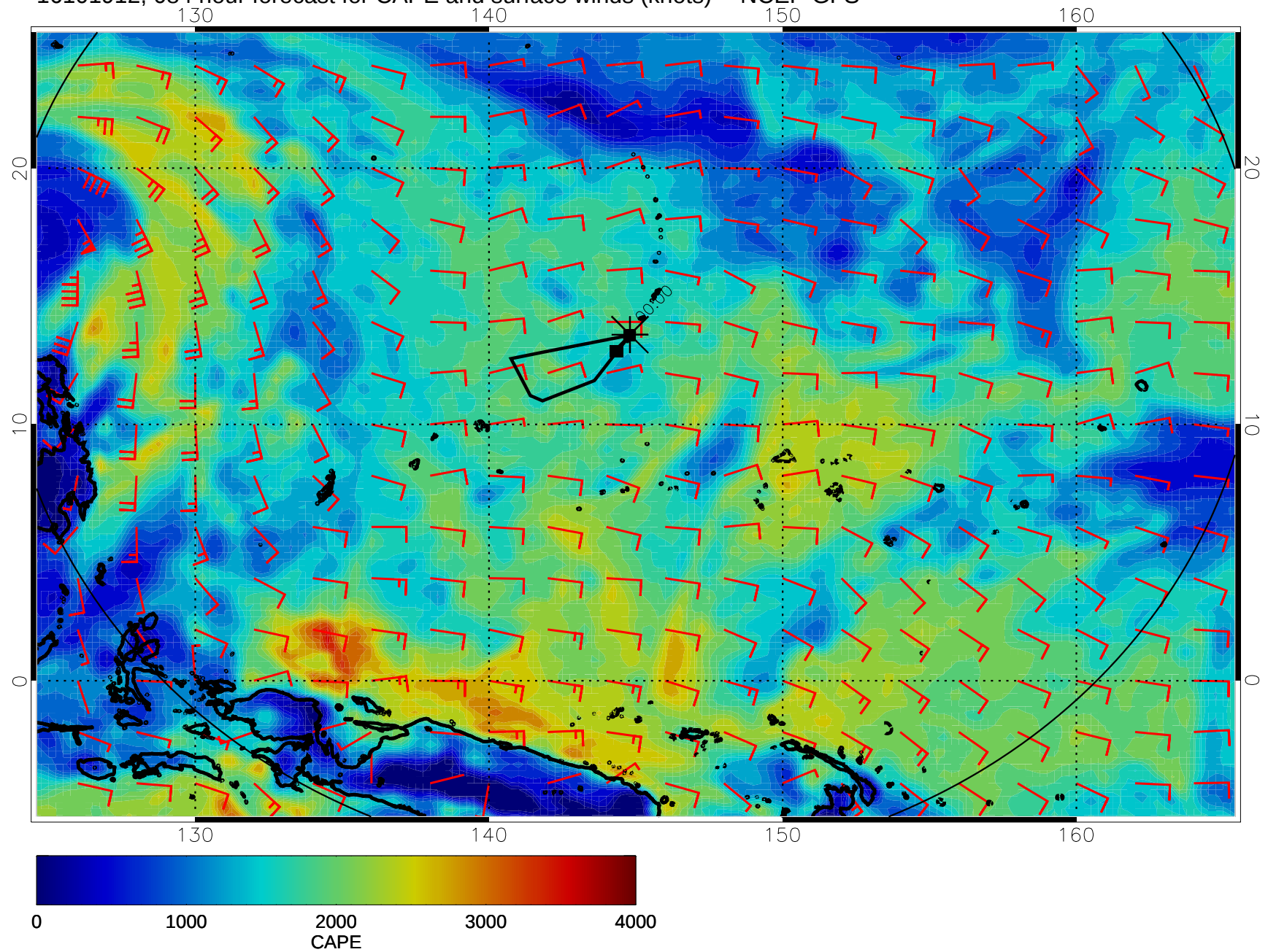
16101912, 084 hour forecast for CAPE and surface winds (knots) -- NCEP GFS
