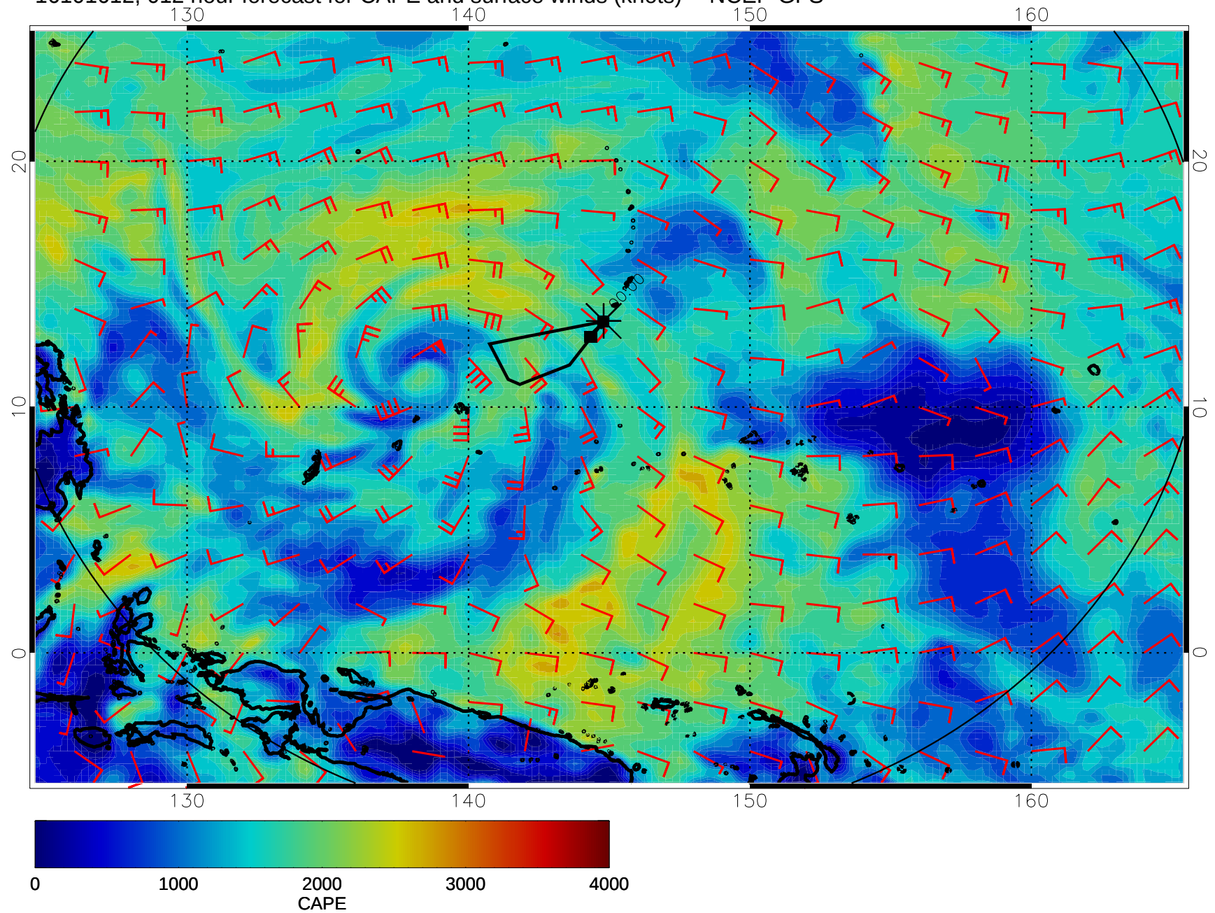
16101612, 012 hour forecast for CAPE and surface winds (knots) -- NCEP GFS
