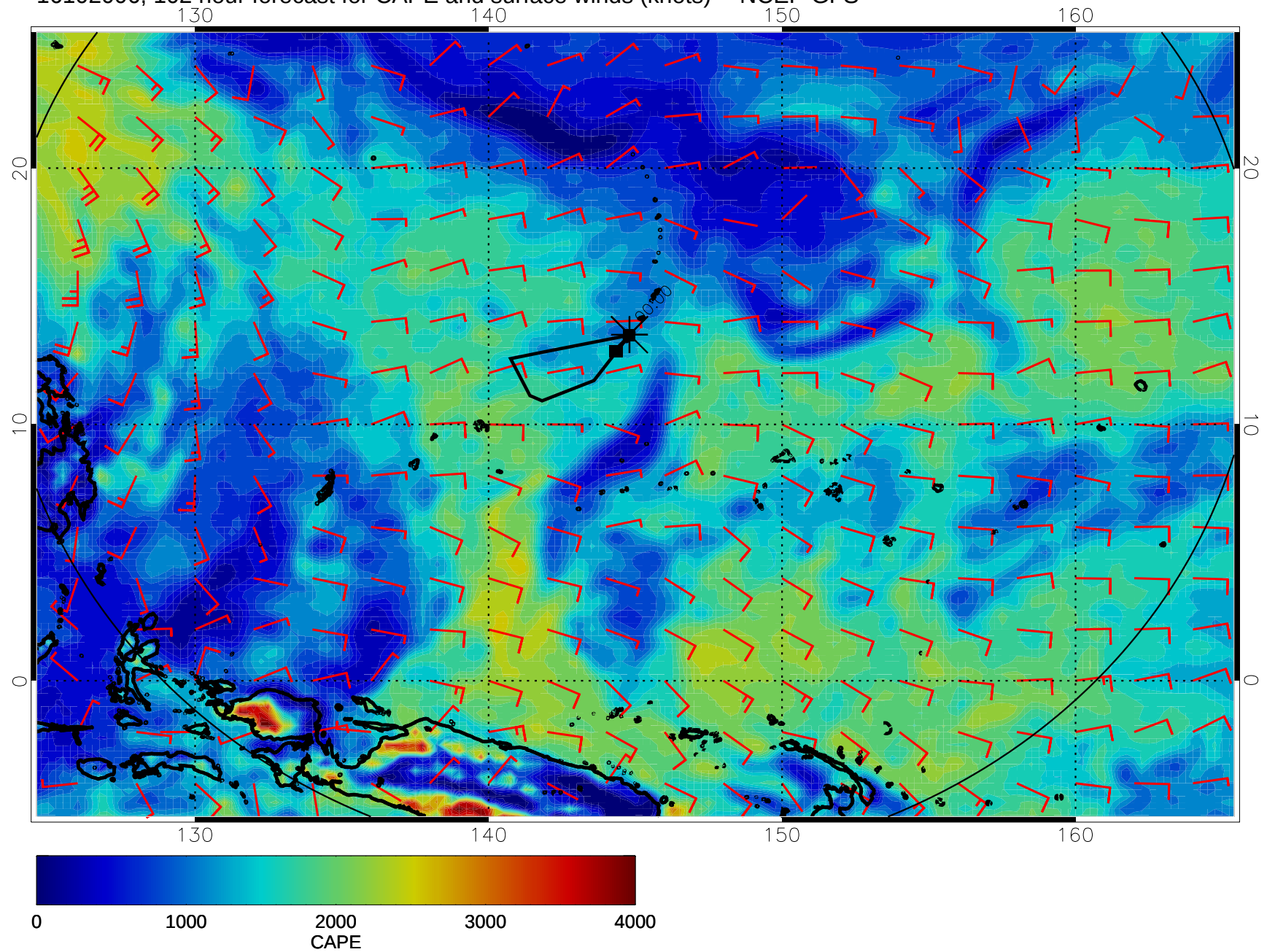
16102006, 102 hour forecast for CAPE and surface winds (knots) -- NCEP GFS
