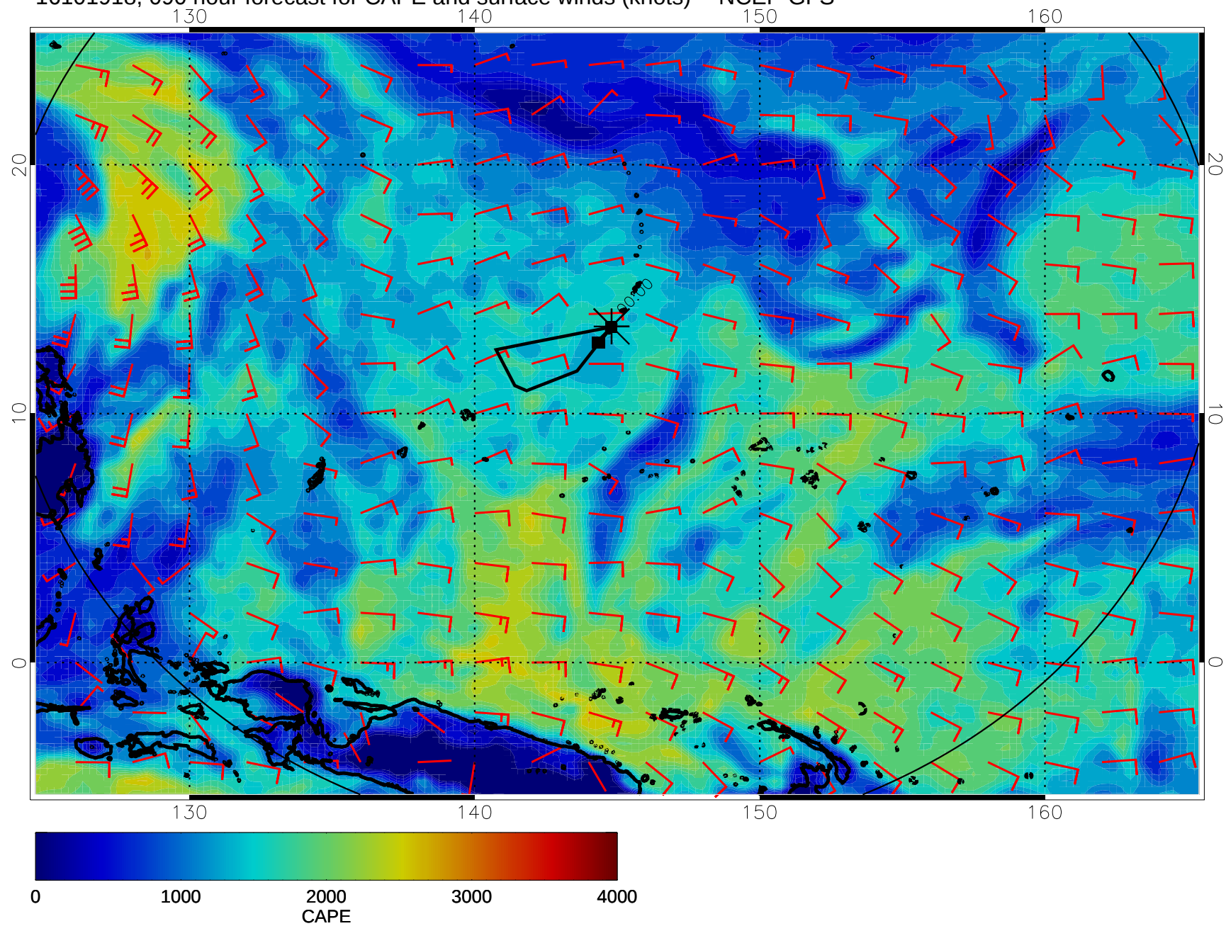
16101918, 0900 hour forecast for CAPE and surface winds (knots) -- NCEP GFS
