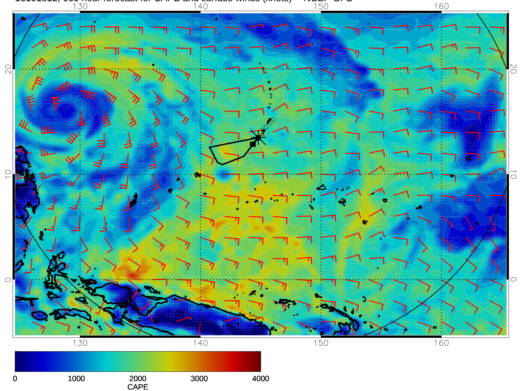
16101812, 060 hour forecast for CAPE and surface winds (knots) -- NCEP GFS
