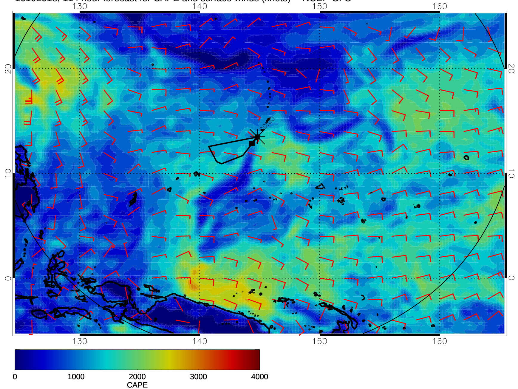
16102018, 114 hour forecast for CAPE and surface winds (knots) -- NCEP GFS
