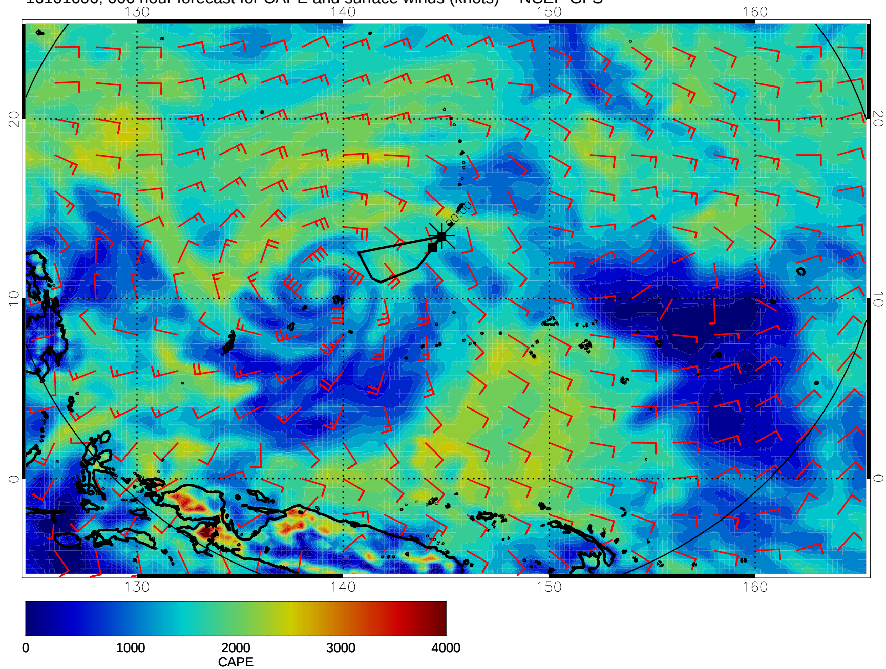
16101606, 006 hour forecast for CAPE and surface winds (knots) -- NCEP GFS
