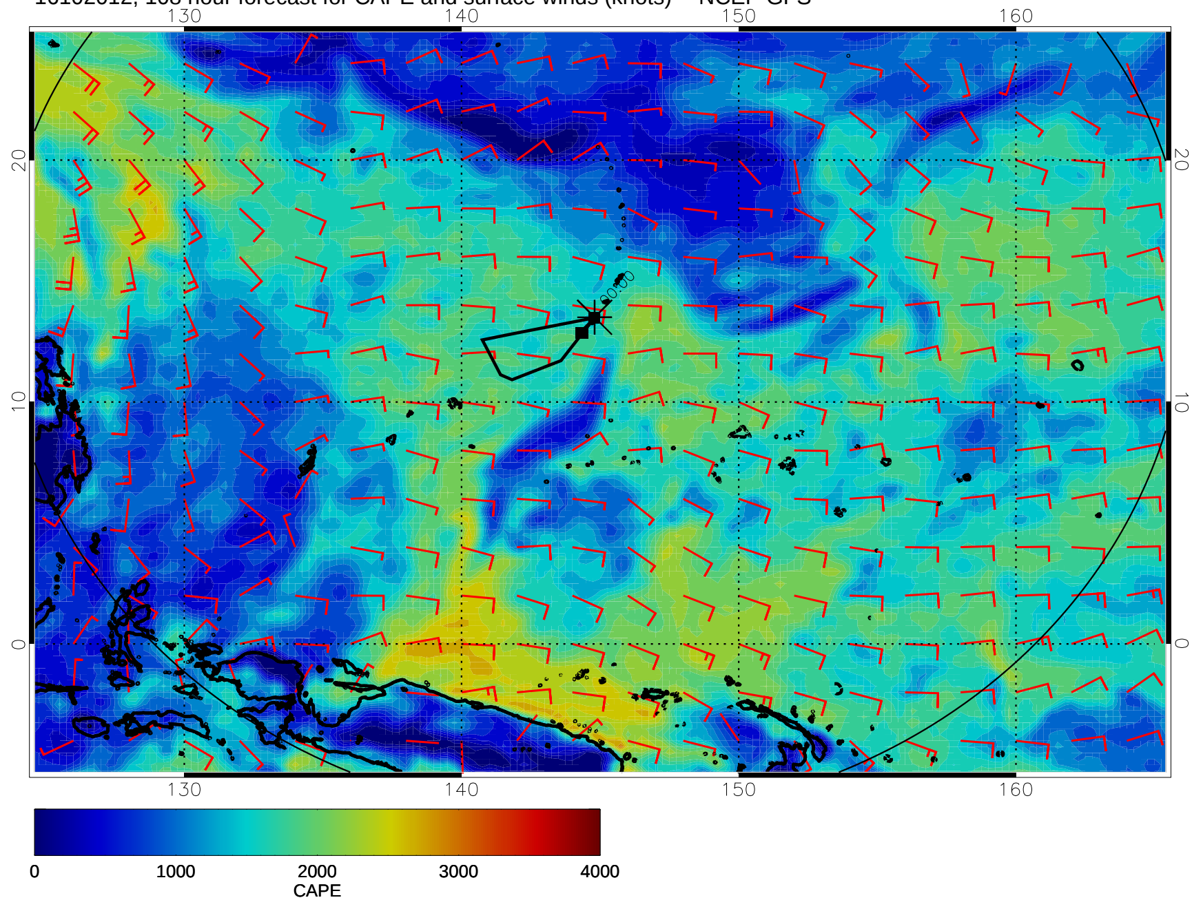
16102012, 108 hour forecast for CAPE and surface winds (knots) -- NCEP GFS
