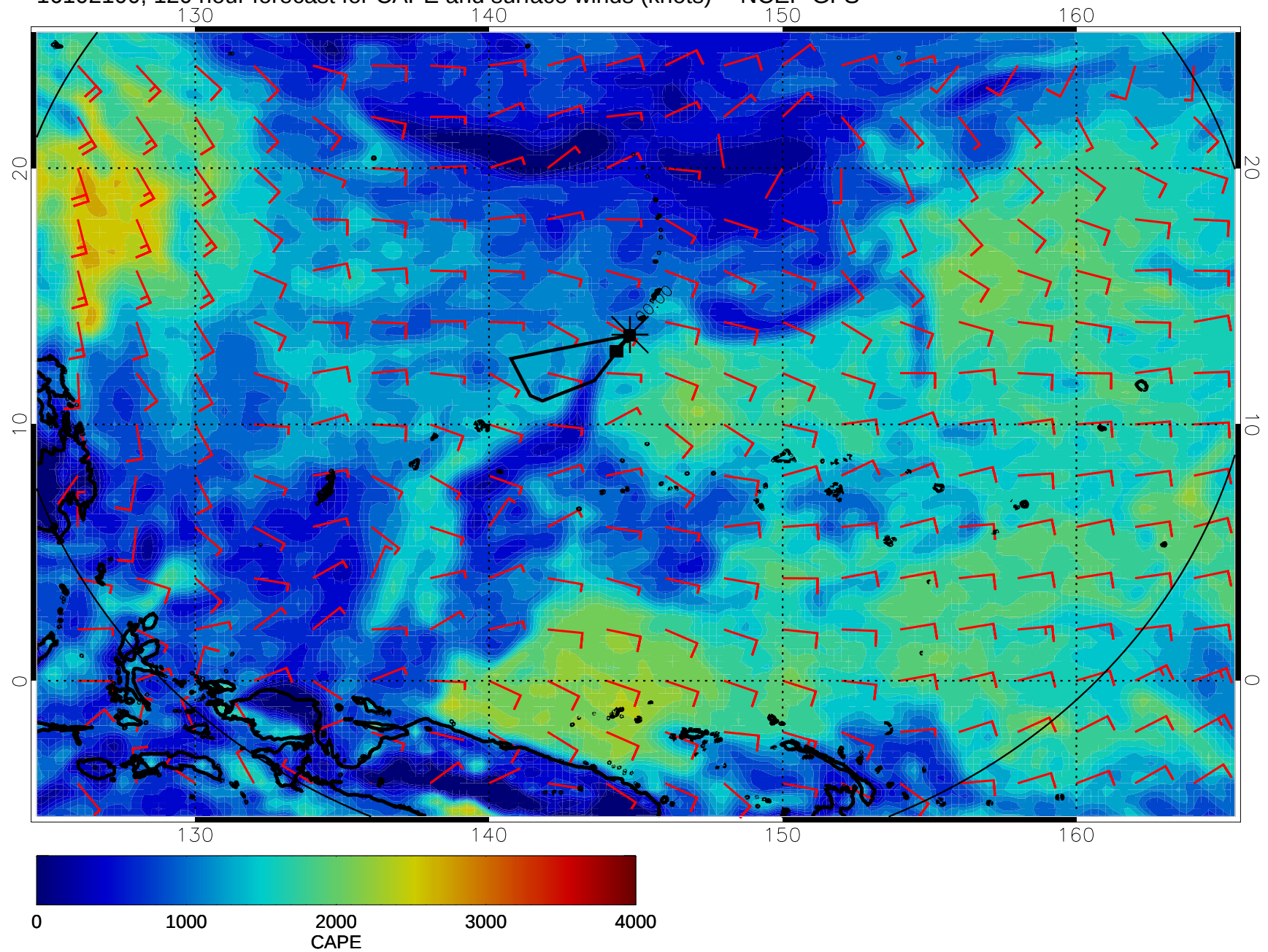
16102100, 120 hour forecast for CAPE and surface winds (knots) -- NCEP GFS
