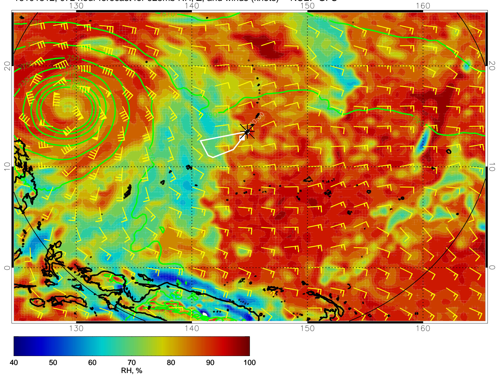
16101812, 072 hour forecast for 925mb RH, Z, and winds (knots) -- NCEP GFS
