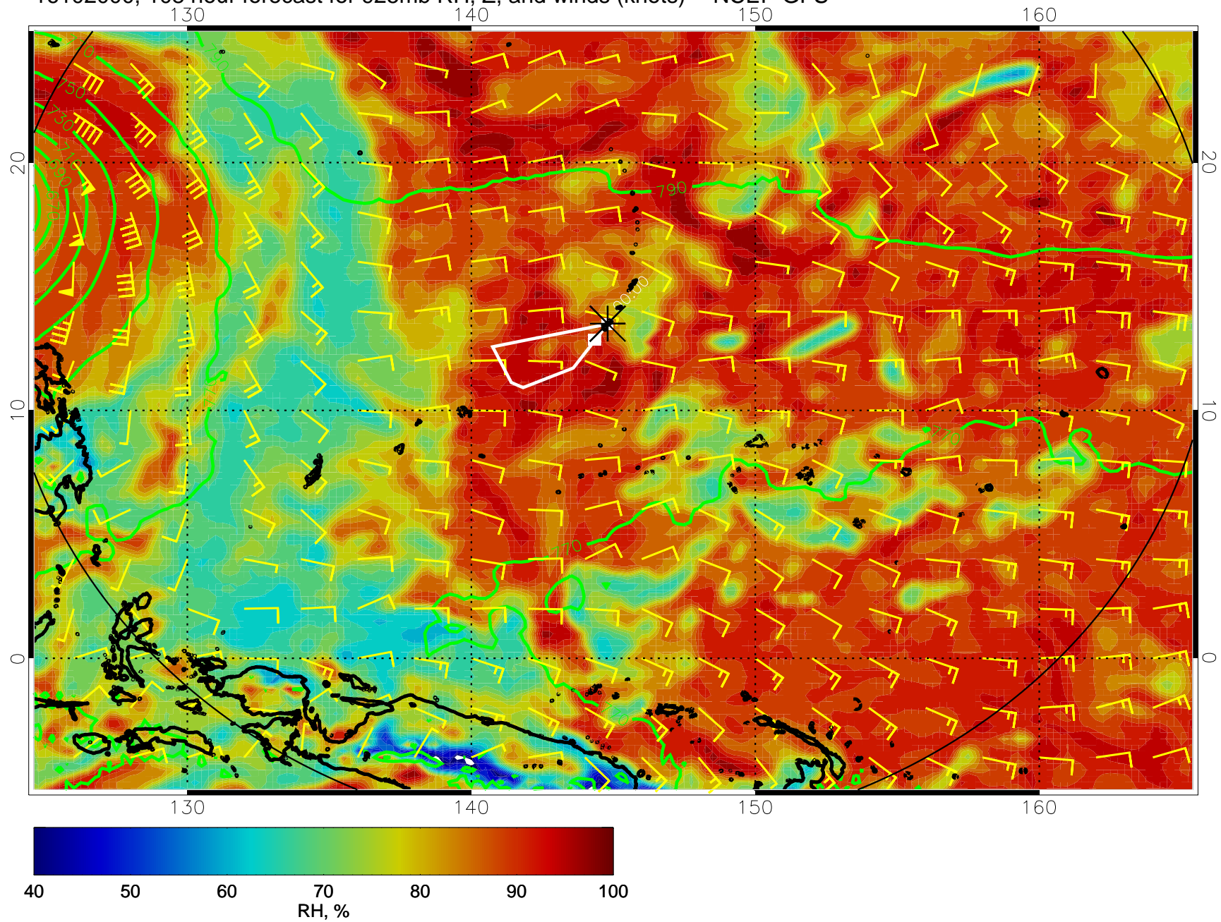
16102000, 108 hour forecast for 925mb RH, Z, and winds (knots) -- NCEP GFS
