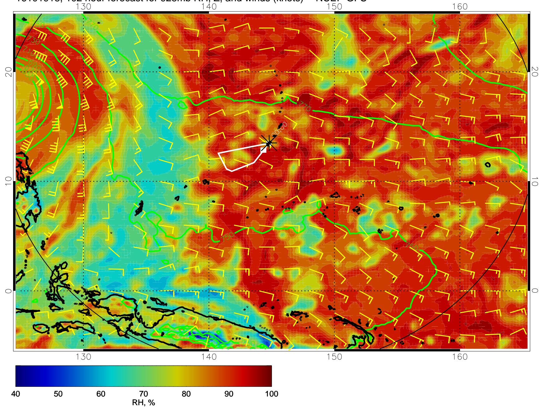
16101918, 102 hour forecast for 925mb RH, Z, and winds (knots) -- NCEP GFS
