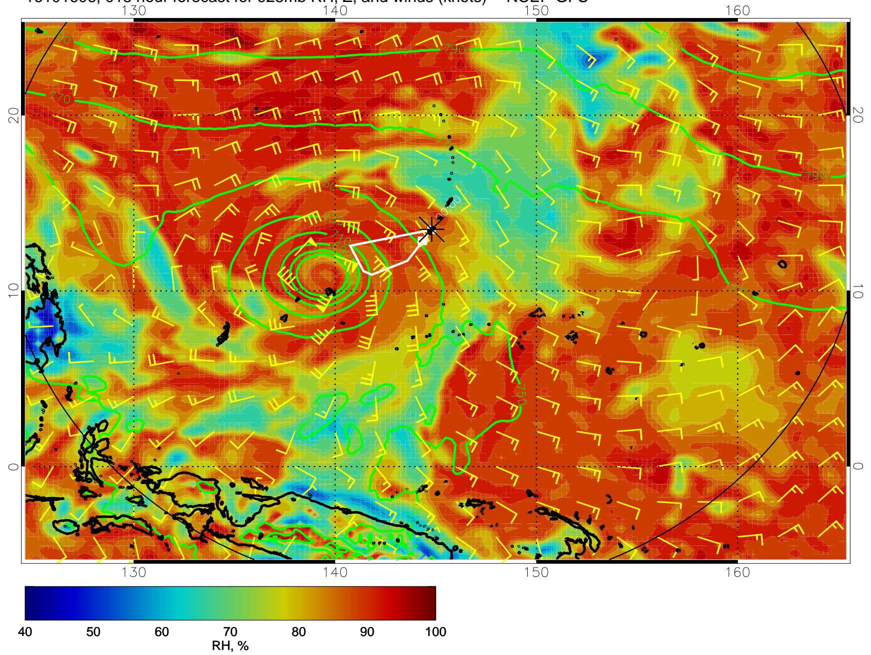
16101606, 018 hour forecast for 925mb RH, Z, and winds (knots) -- NCEP GFS
