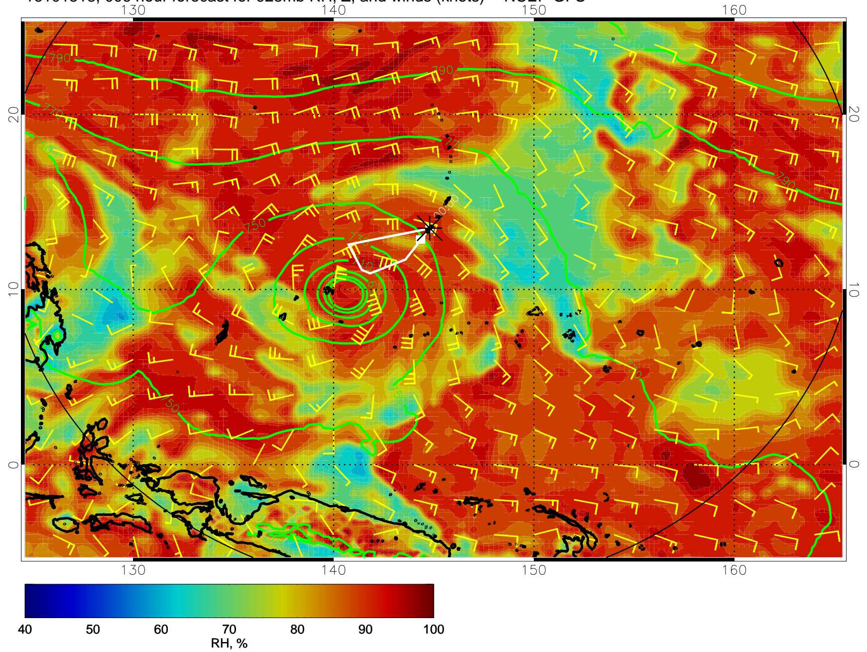
16101518, 006 hour forecast for 925mb RH, Z, and winds (knots) -- NCEP GFS
