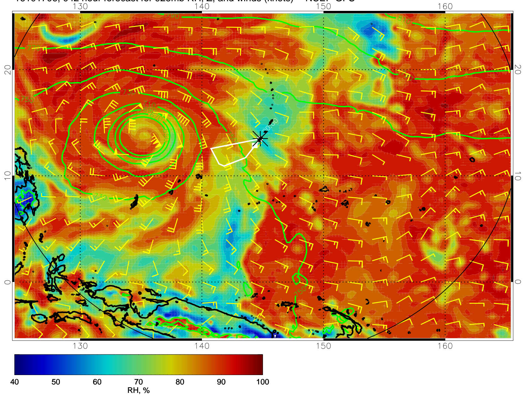
16101706, 042 hour forecast for 925mb RH, Z, and winds (knots) -- NCEP GFS
