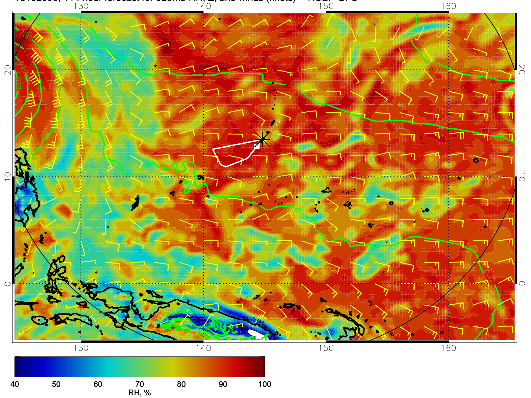
16102006, 114 hour forecast for 925mb RH, Z, and winds (knots) -- NCEP GFS
