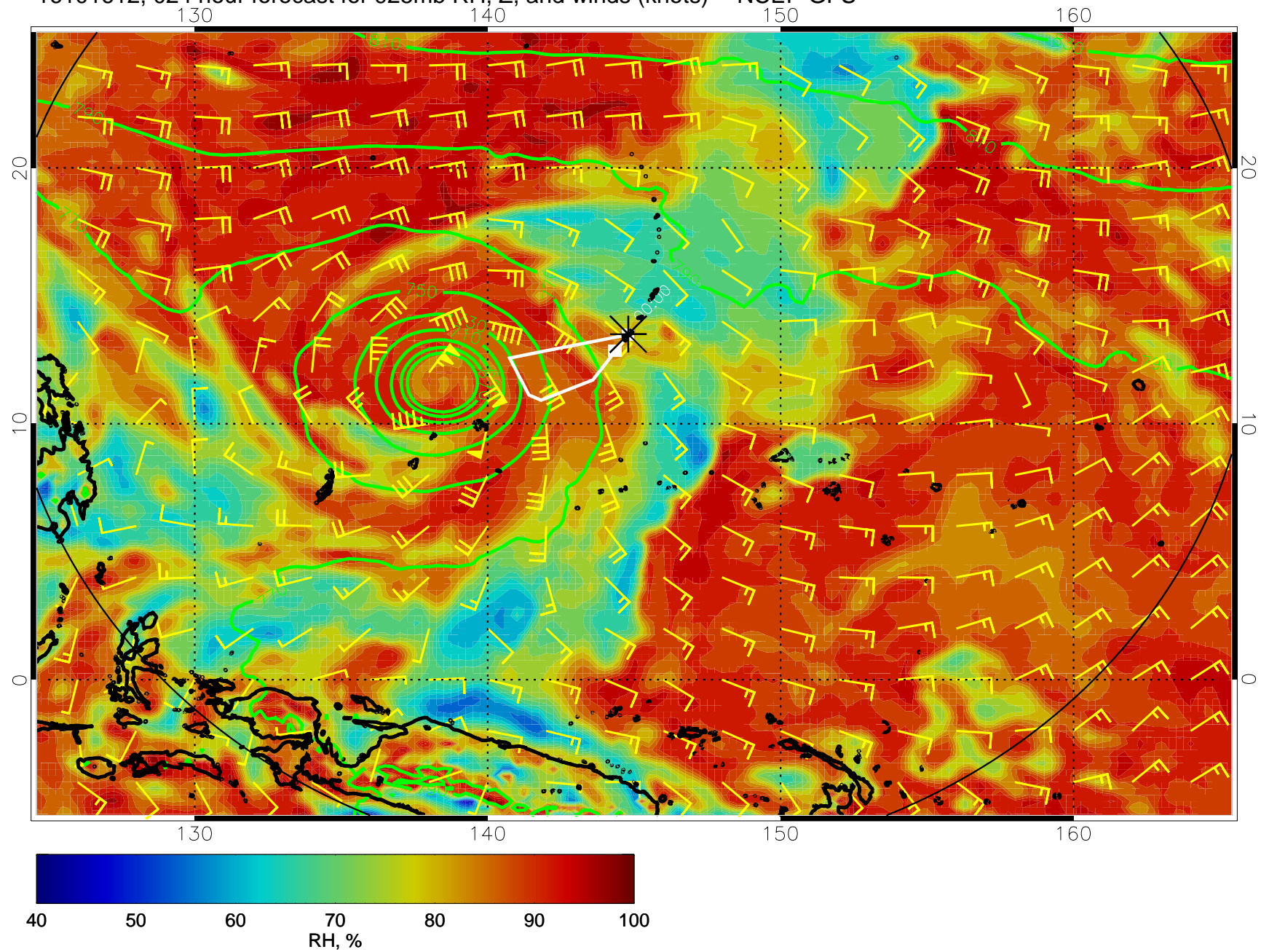
16101612, 024 hour forecast for 925mb RH, Z, and winds (knots) -- NCEP GFS
