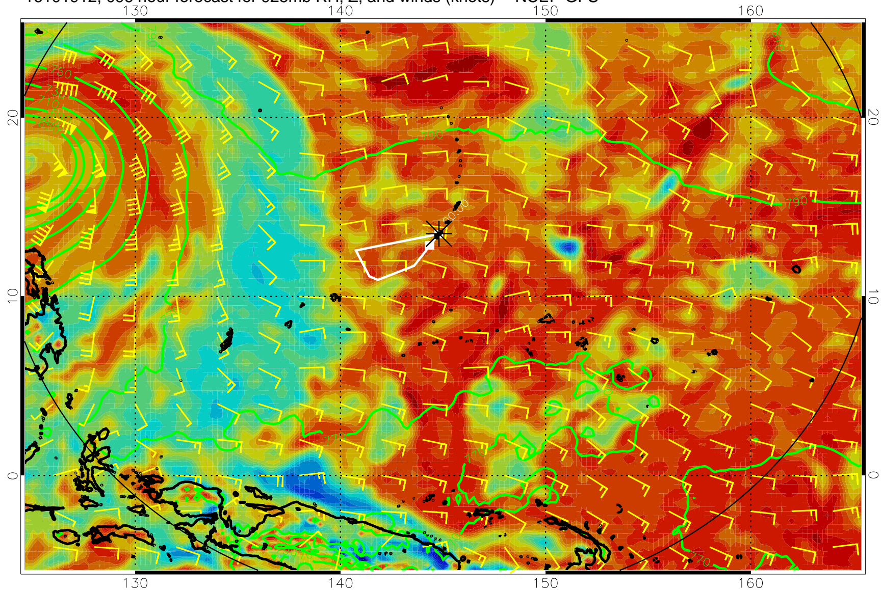
16101912, 096 hour forecast for 925mb RH, Z, and winds (knots) -- NCEP GFS
