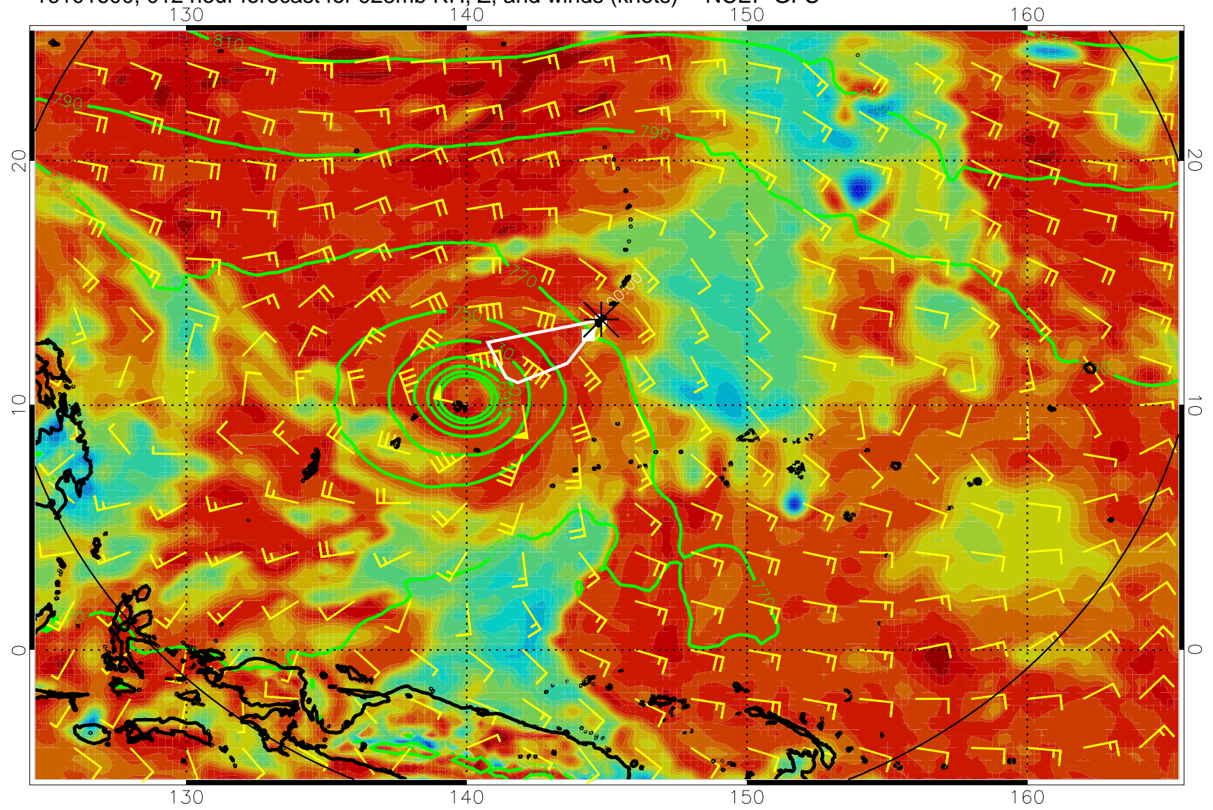
16101600, 012 hour forecast for 925mb RH, Z, and winds (knots) -- NCEP GFS
