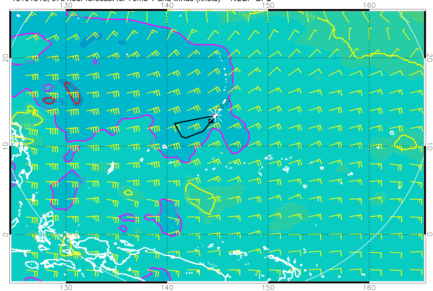
16101818, 078 hour forecast for 70mb T and winds (knots) -- NCEP GFS
