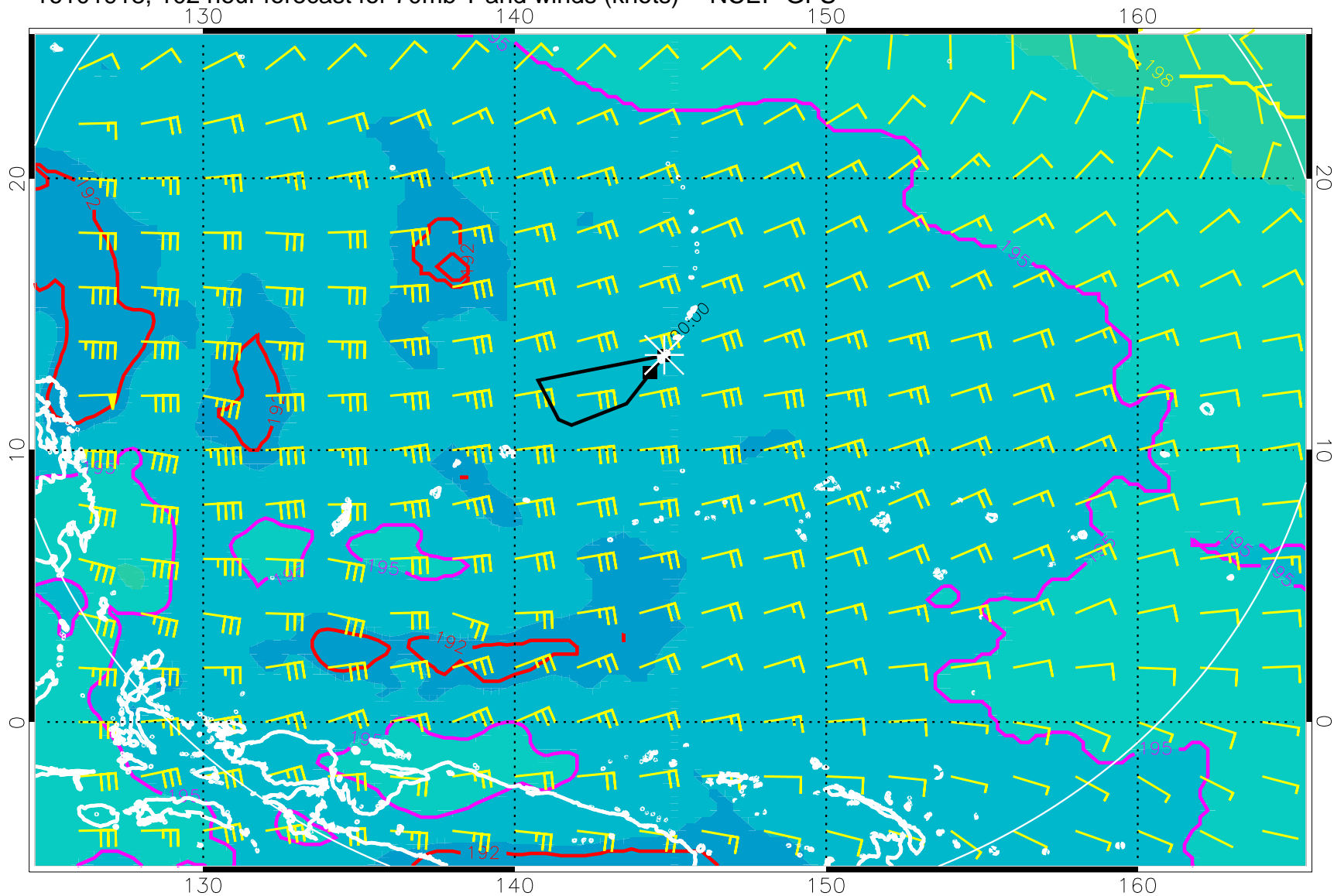
16101918, 102 hour forecast for 70mb T and winds (knots) -- NCEP GFS
