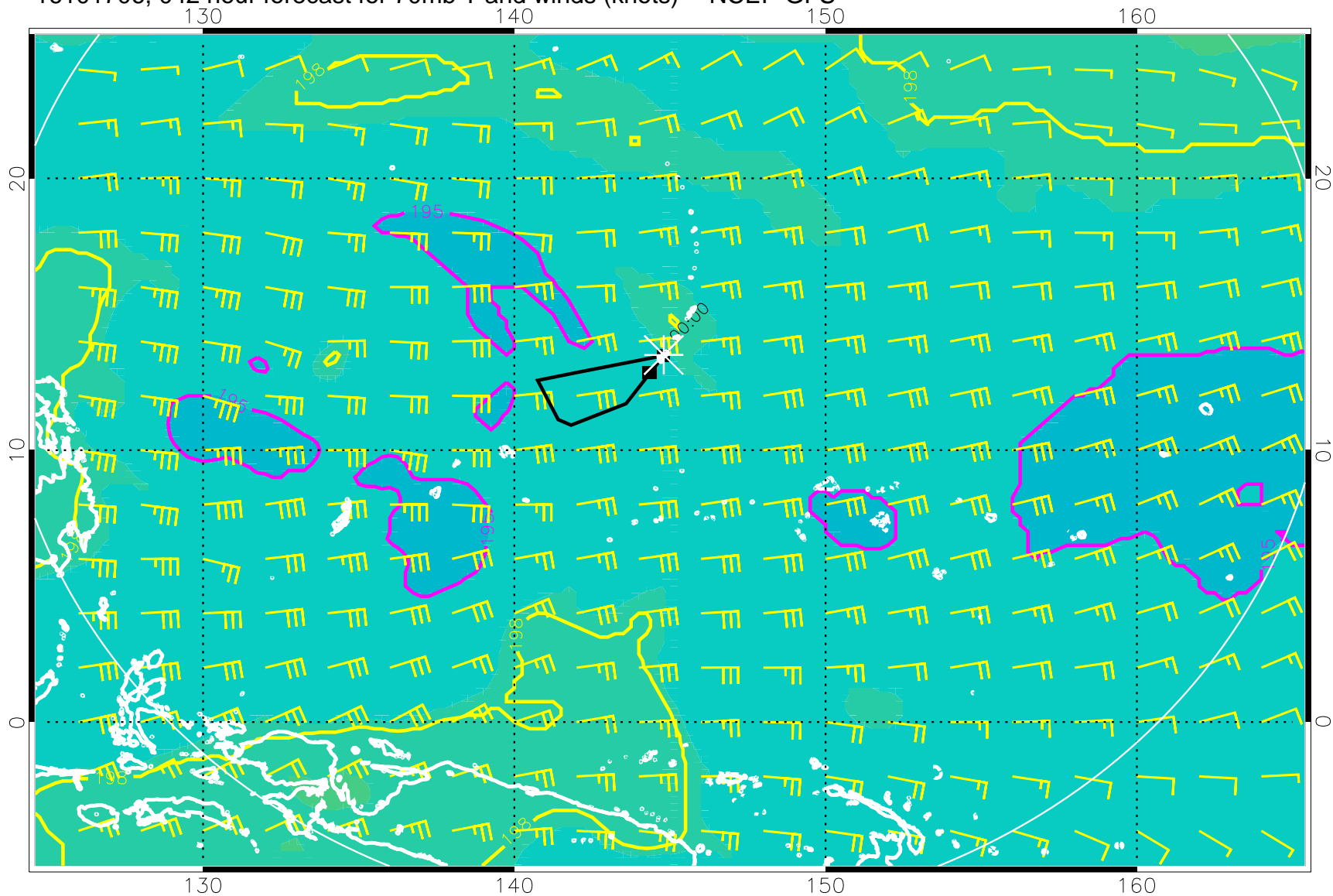
16101706, 042 hour forecast for 70mb T and winds (knots) -- NCEP GFS
