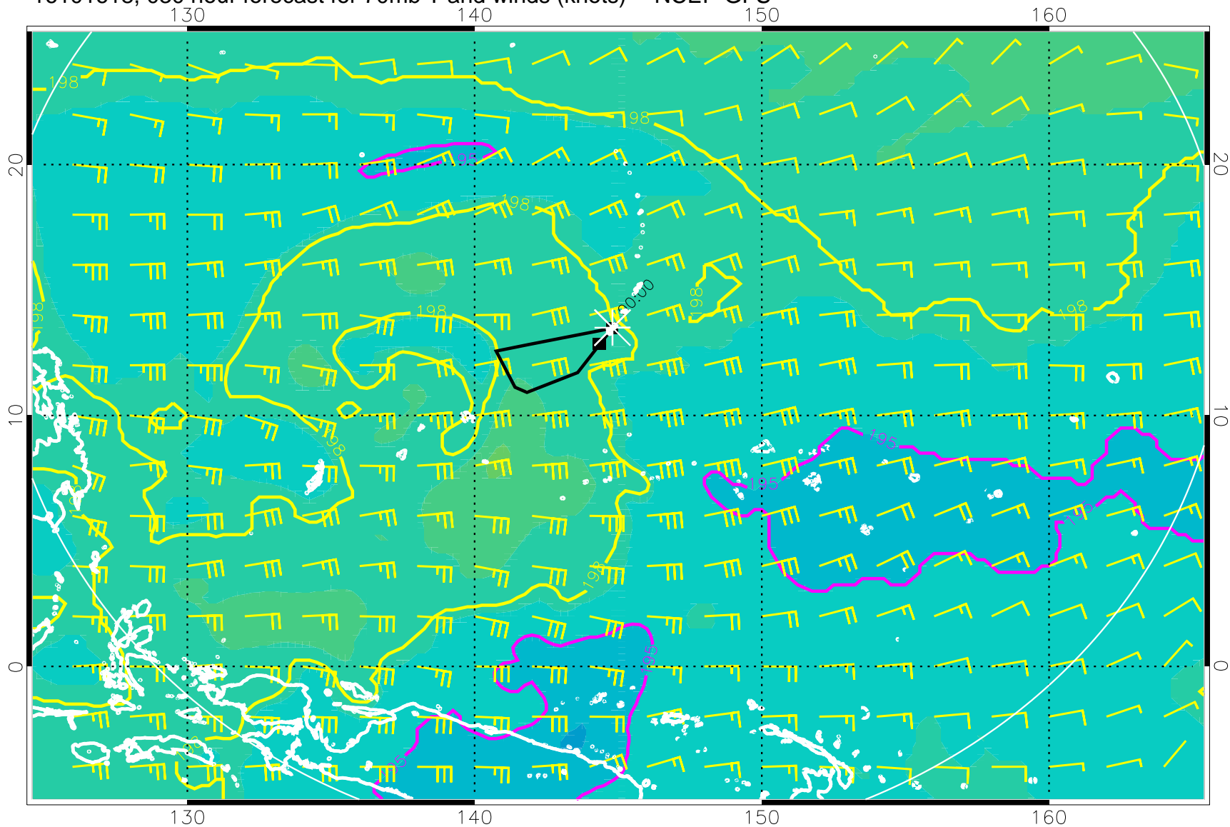
16101618, 0300 hour forecast for 70mb T and winds (knots) -- NCEP GFS
