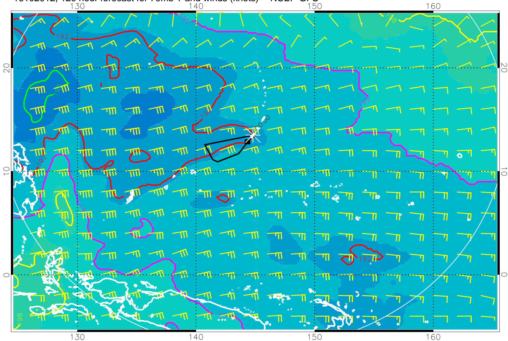
16102012, 120 hour forecast for 70mb T and winds (knots) -- NCEP GFS
