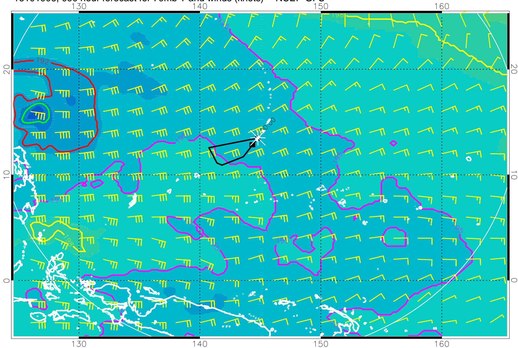
16101906, 090 hour forecast for 70mb T and winds (knots) -- NCEP GFS
