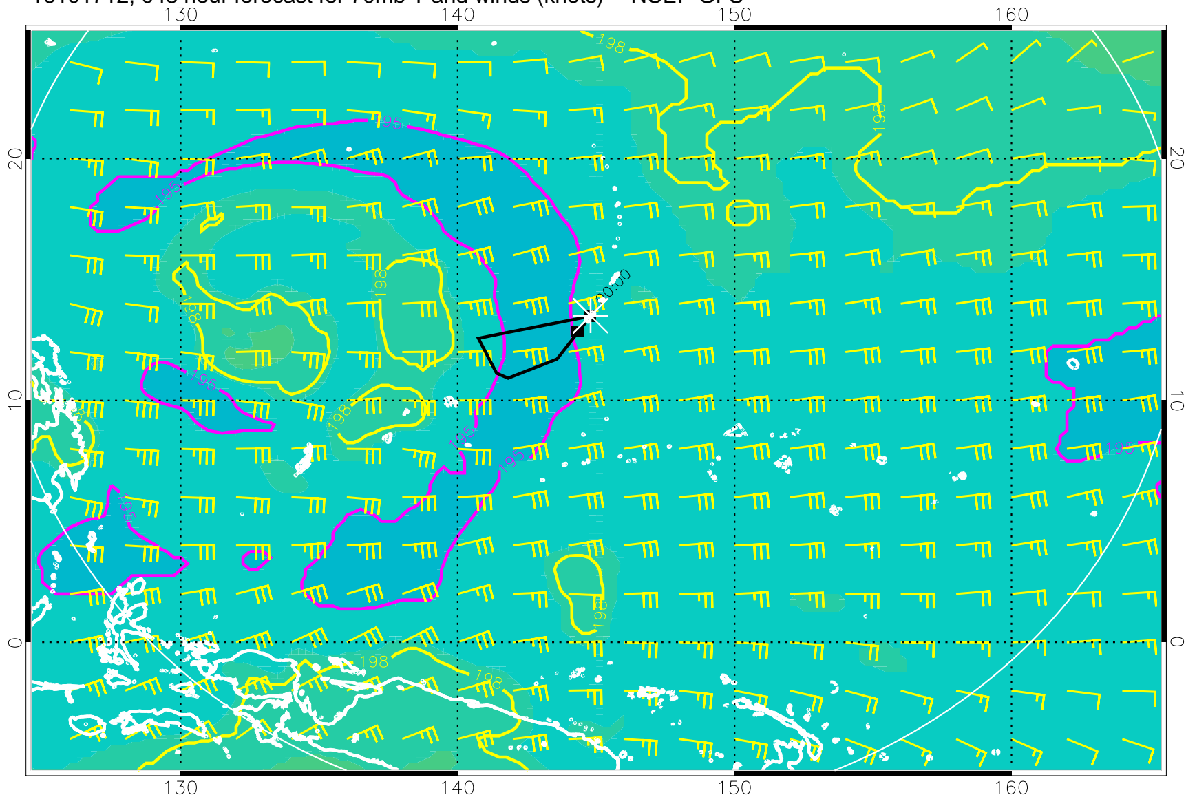
16101712, 048 hour forecast for 70mb T and winds (knots) -- NCEP GFS
