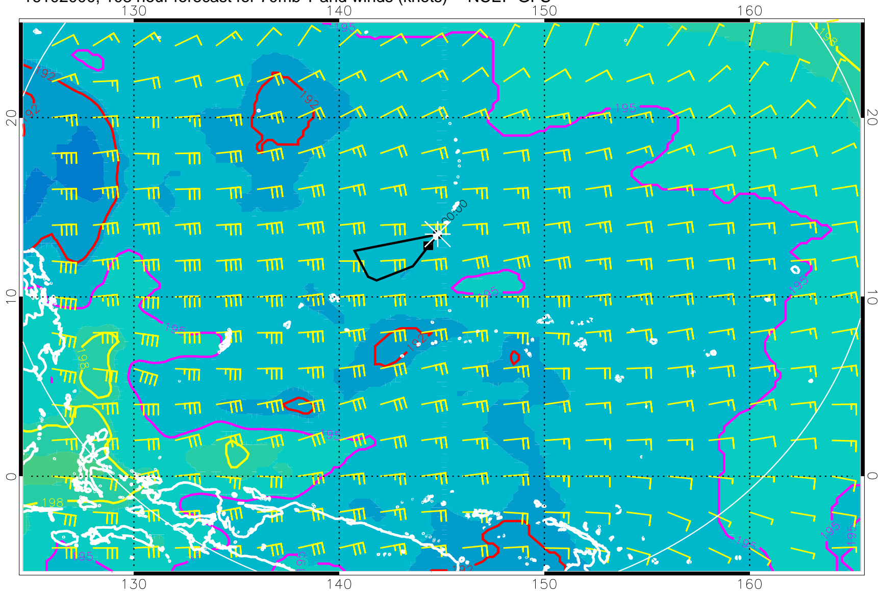
16102000, 108 hour forecast for 70mb T and winds (knots) -- NCEP GFS
