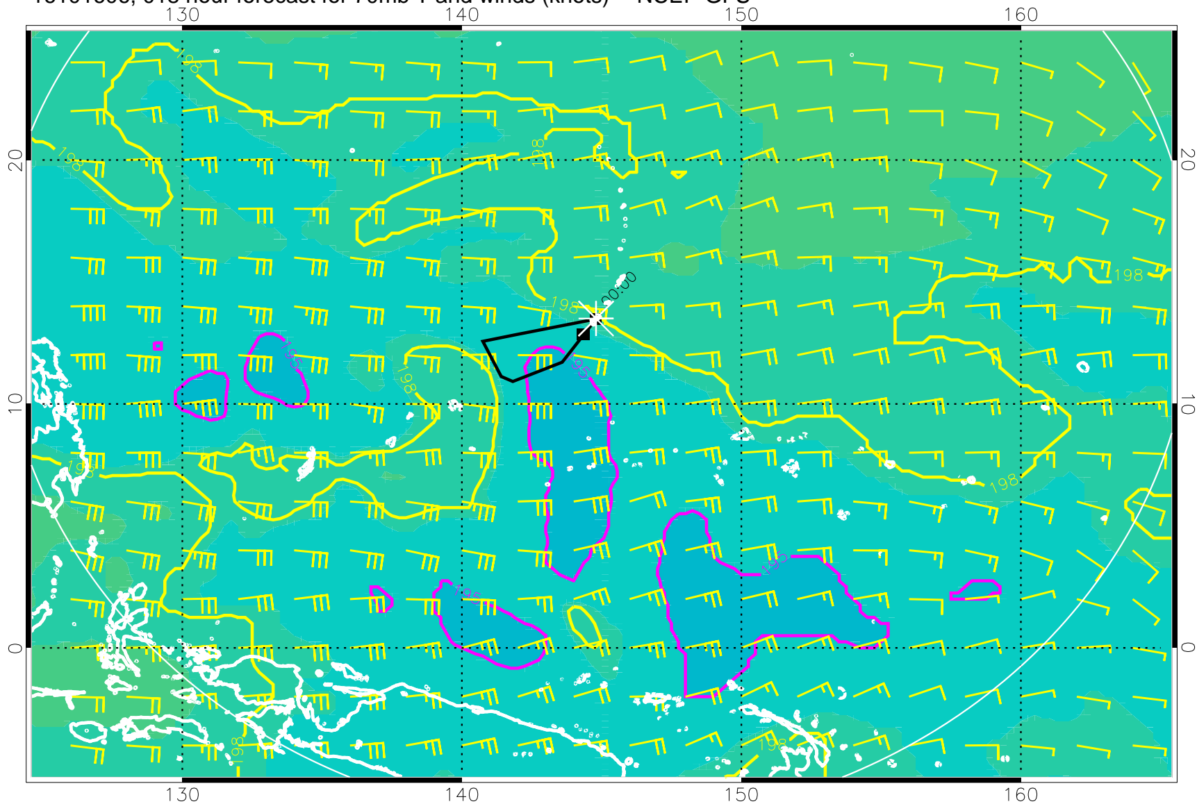
16101606, 018 hour forecast for 70mb T and winds (knots) -- NCEP GFS
