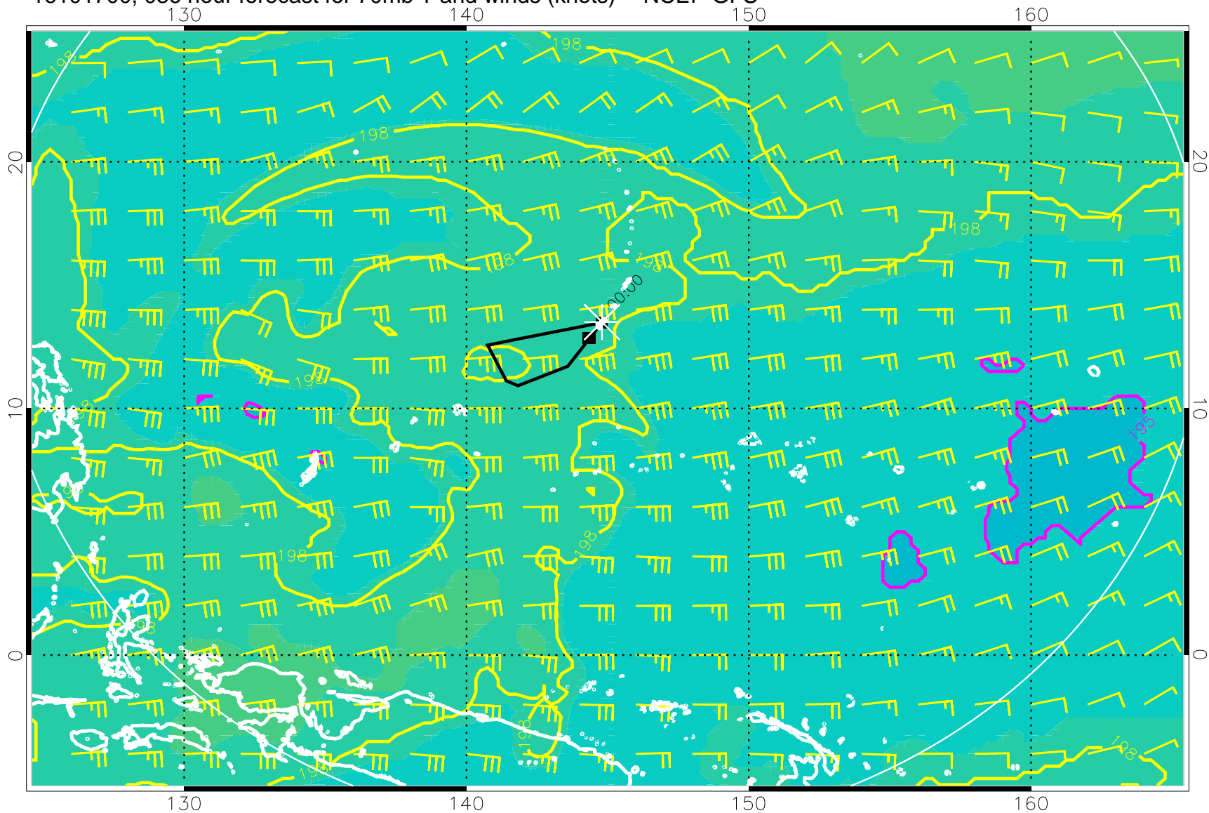
16101700, 036 hour forecast for 70mb T and winds (knots) -- NCEP GFS
