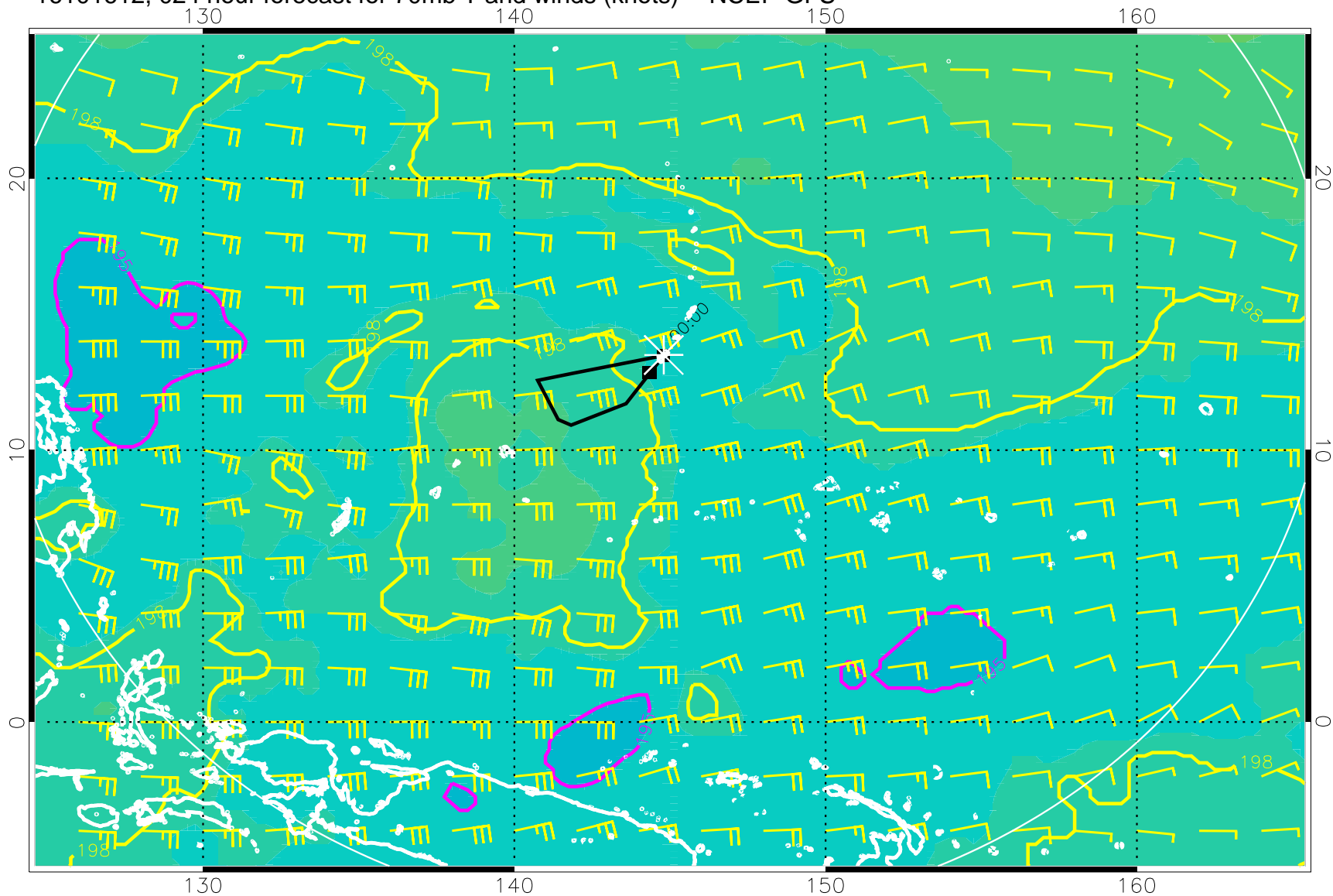
16101612, 024 hour forecast for 70mb T and winds (knots) -- NCEP GFS
