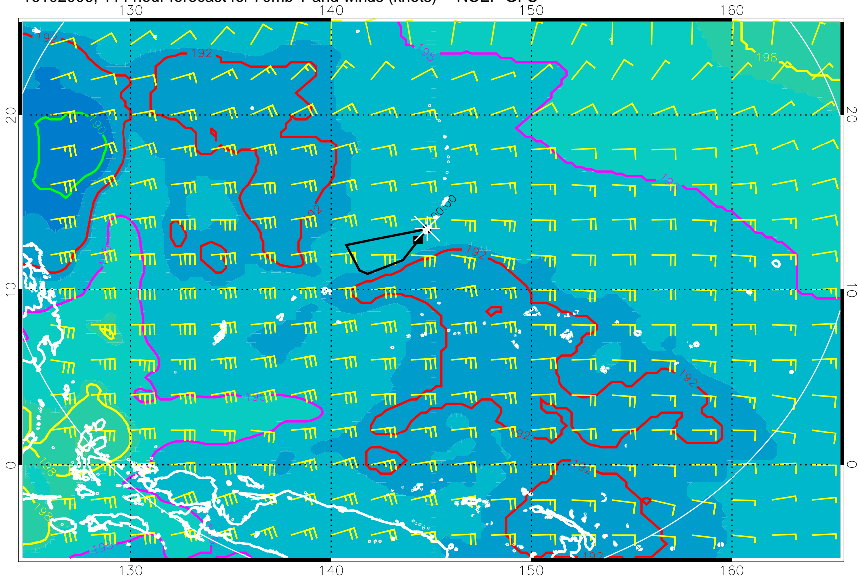
16102006, 114 hour forecast for 70mb T and winds (knots) -- NCEP GFS
