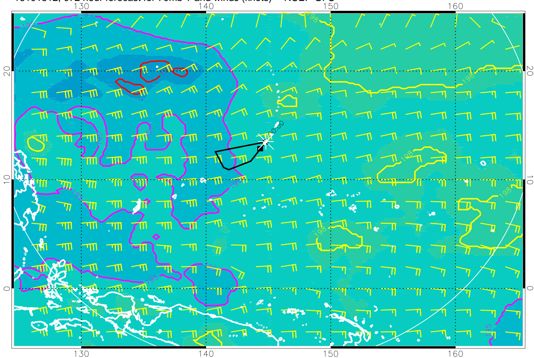
16101812, 072 hour forecast for 70mb T and winds (knots) -- NCEP GFS
