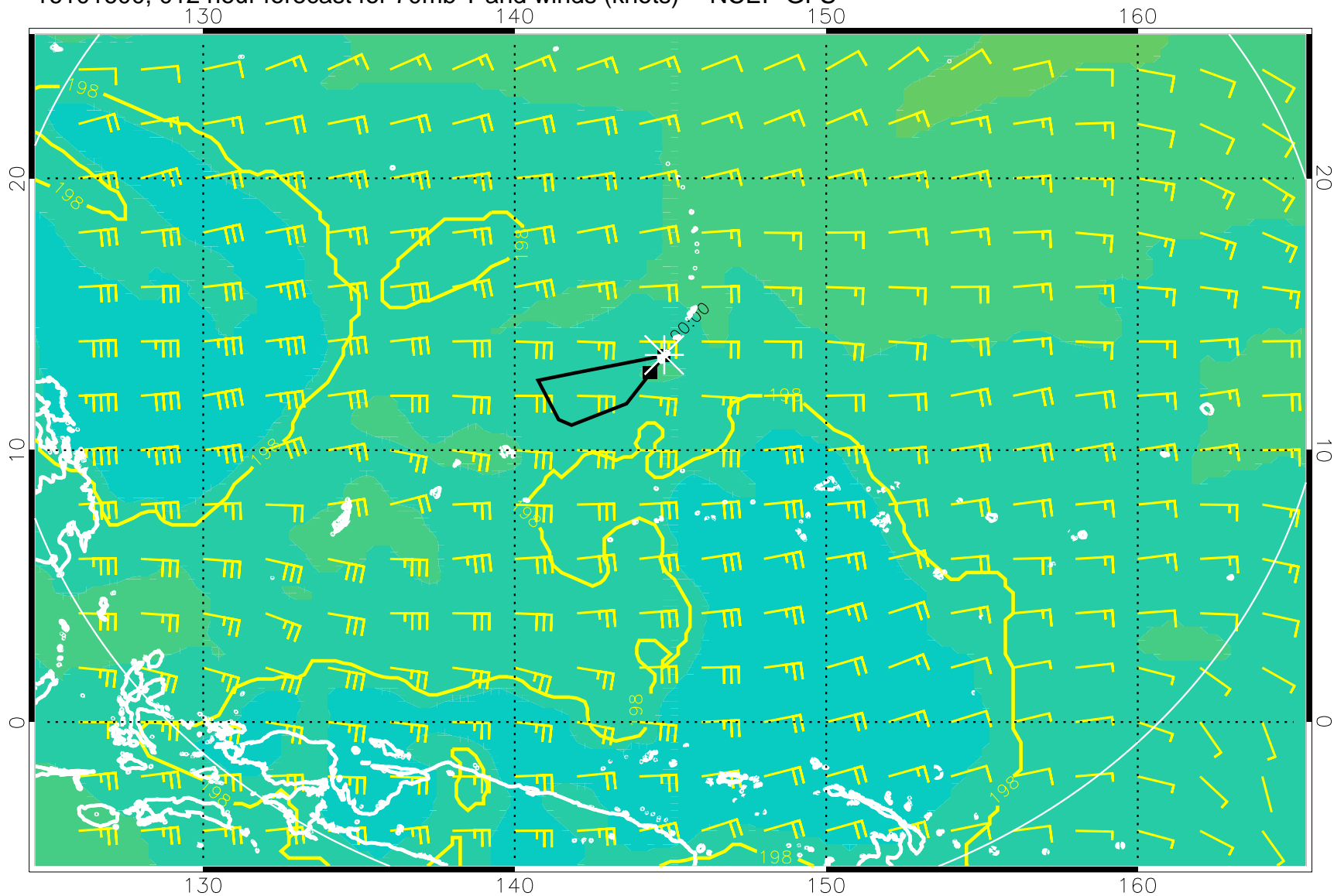
16101600, 012 hour forecast for 70mb T and winds (knots) -- NCEP GFS
