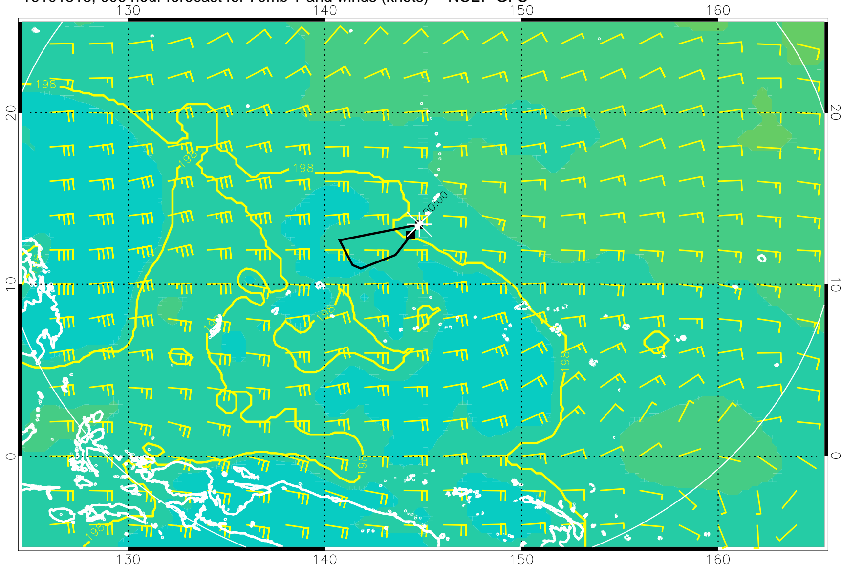
16101518, 006 hour forecast for 70mb T and winds (knots) -- NCEP GFS
