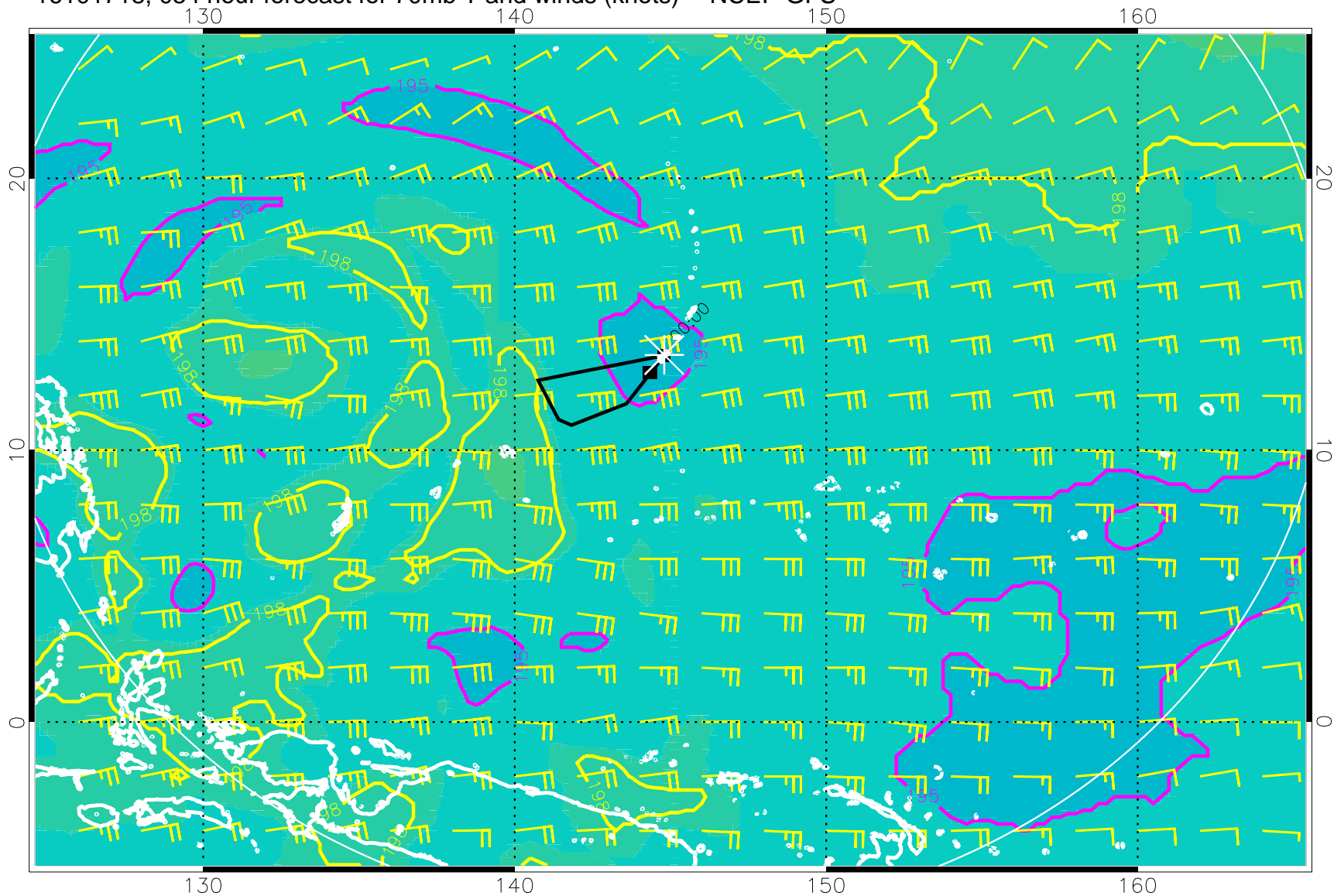
16101718, 054 hour forecast for 70mb T and winds (knots) -- NCEP GFS
