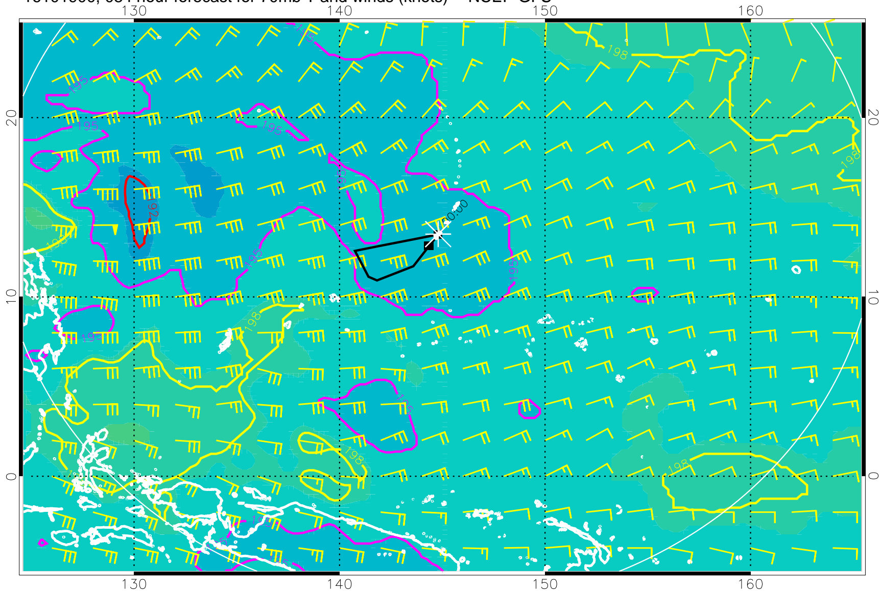
16101900, 084 hour forecast for 70mb T and winds (knots) -- NCEP GFS
