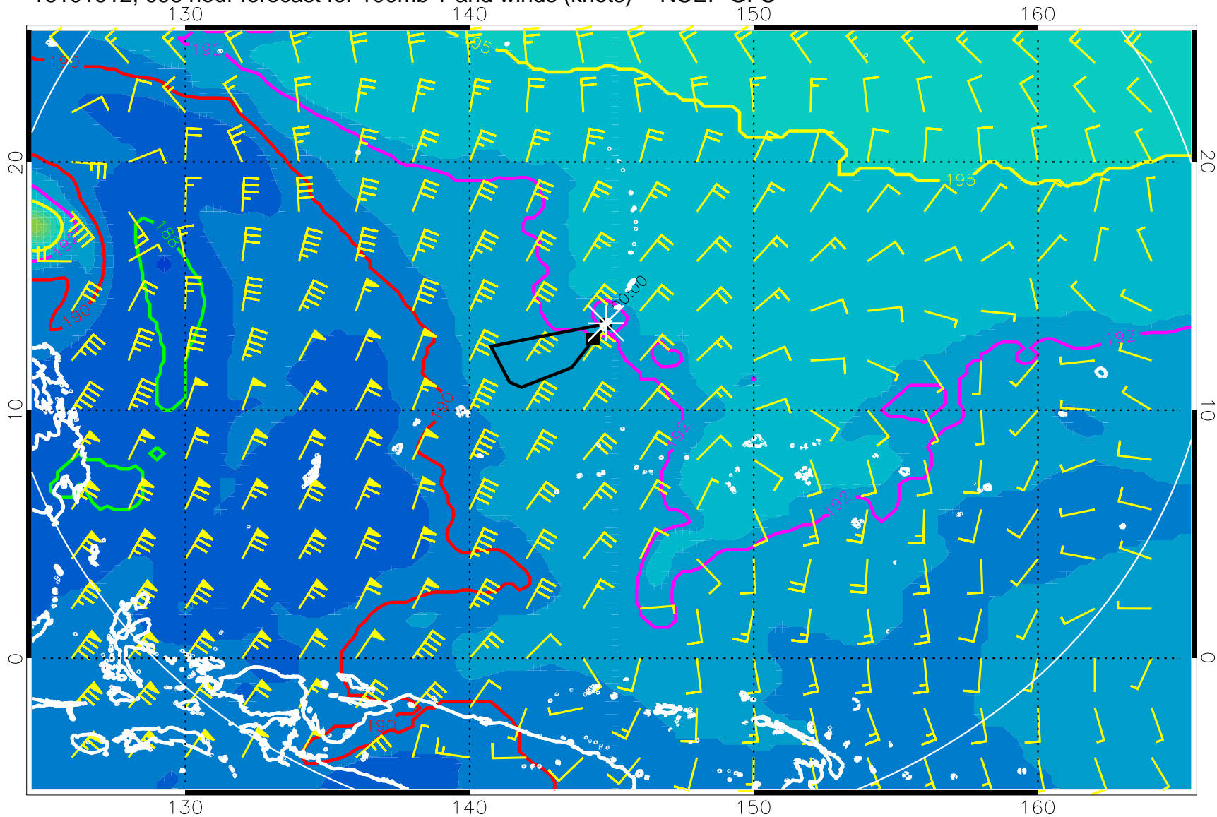
16101912, 096 hour forecast for 100mb T and winds (knots) -- NCEP GFS
