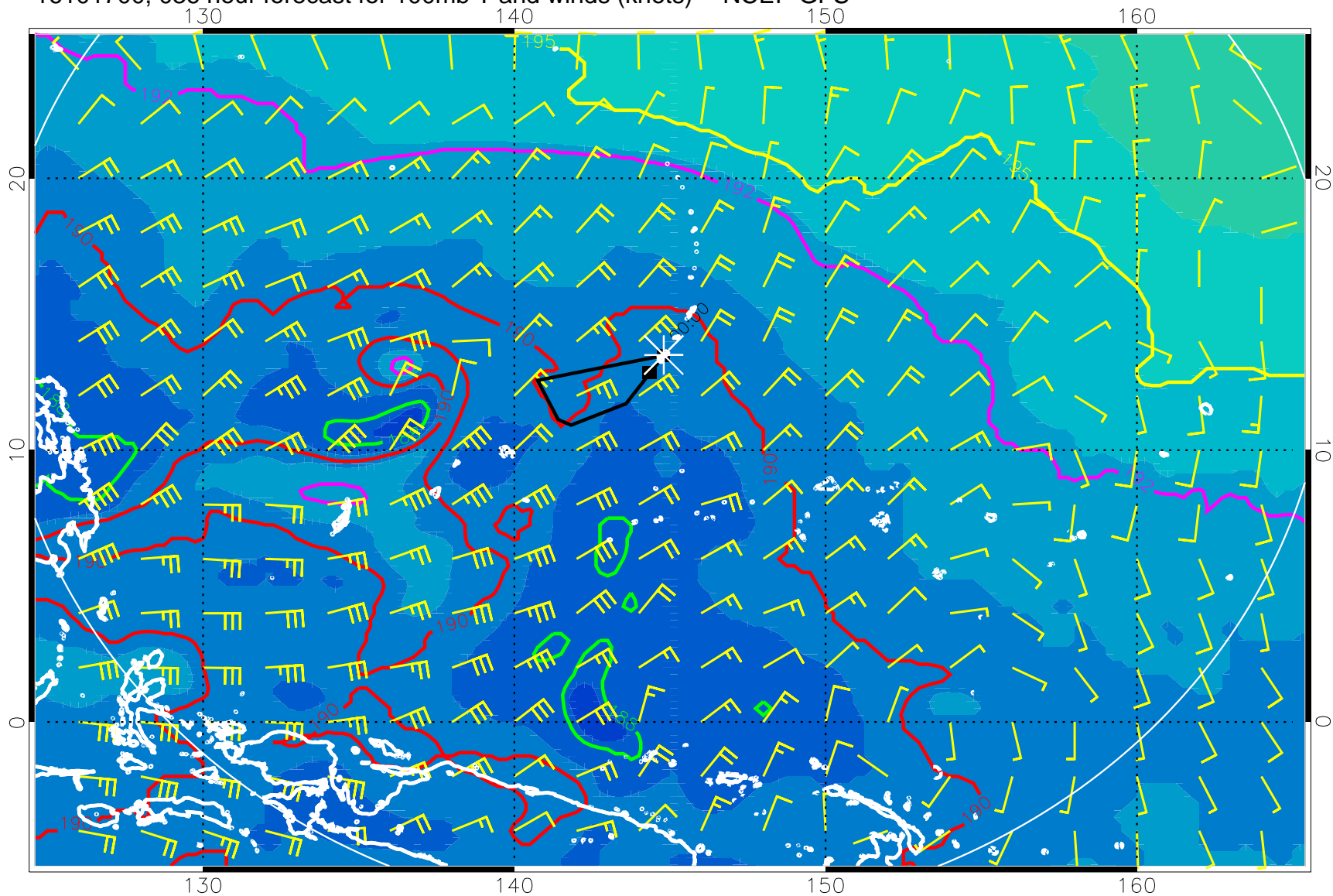
16101700, 036 hour forecast for 100mb T and winds (knots) -- NCEP GFS
