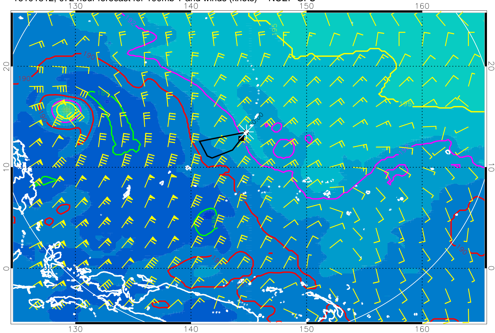
16101812, 072 hour forecast for 100mb T and winds (knots) -- NCEP GFS
