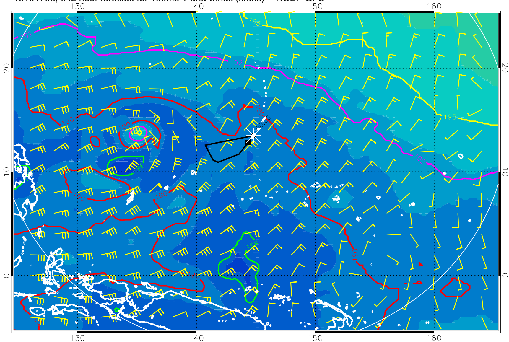
16101706, 042 hour forecast for 100mb T and winds (knots) -- NCEP GFS
