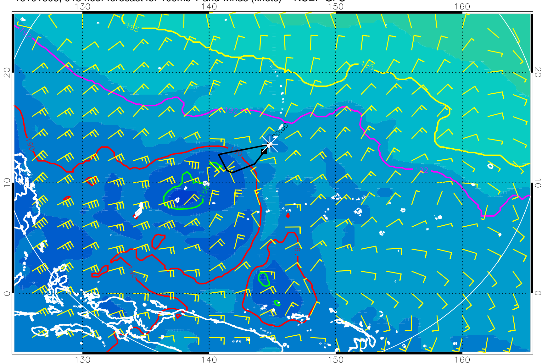
16101606, 018 hour forecast for 100mb T and winds (knots) -- NCEP GFS
