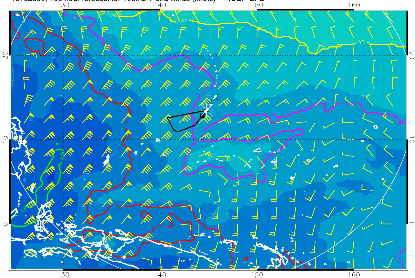
16102000, 108 hour forecast for 100mb T and winds (knots) -- NCEP GFS
