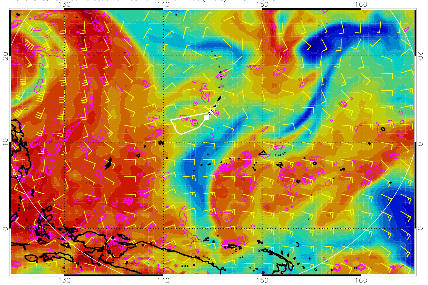
16101918, 102 hour forecast for 700mb RH and winds (knots) -- NCEP GFS
