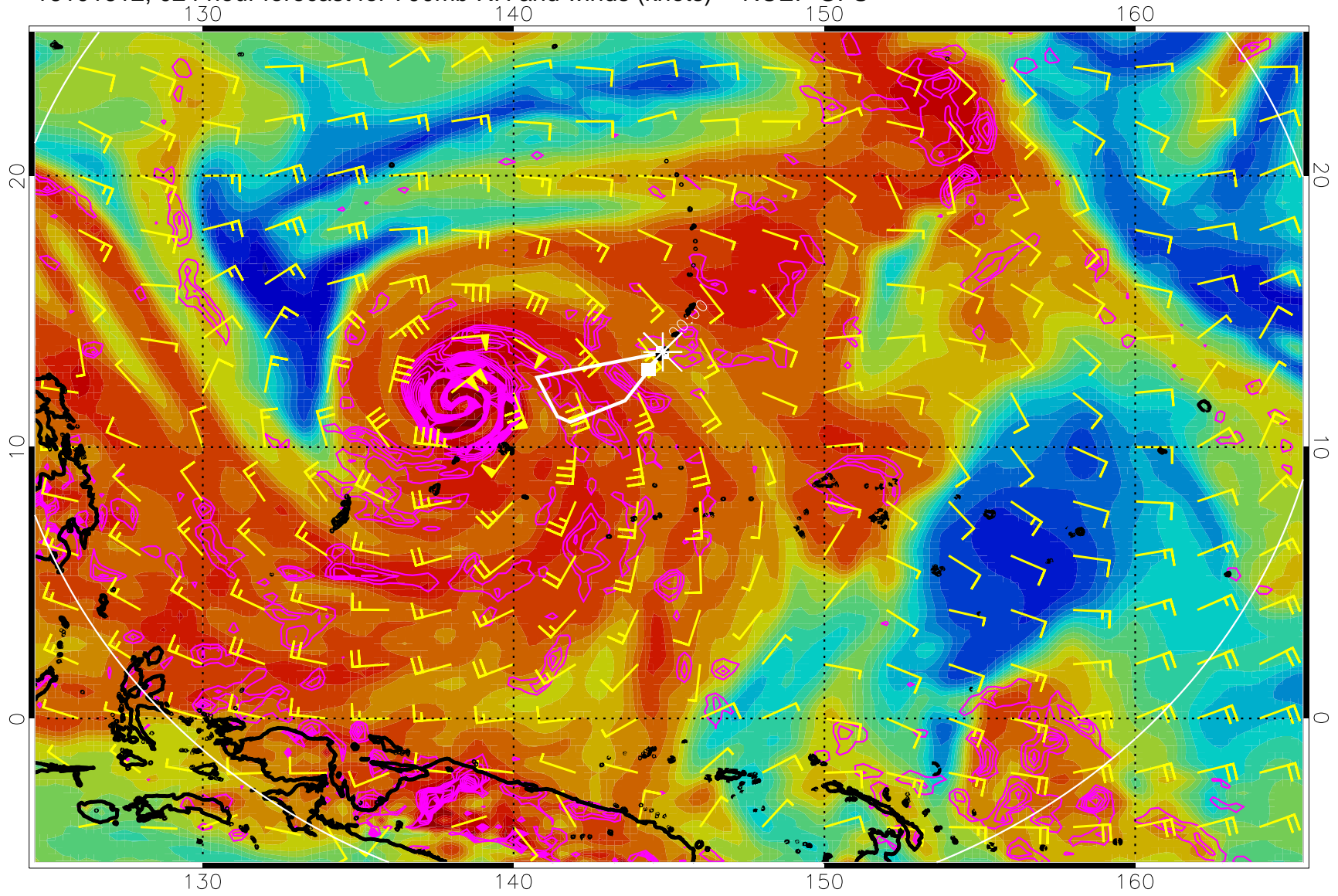
16101612, 024 hour forecast for 700mb RH and winds (knots) -- NCEP GFS
