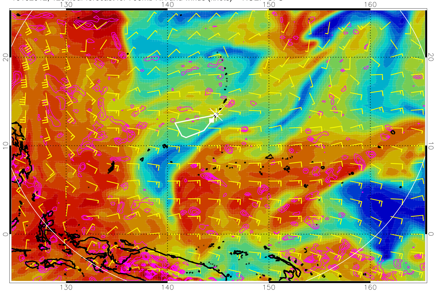
16102012, 120 hour forecast for 700mb RH and winds (knots) -- NCEP GFS
