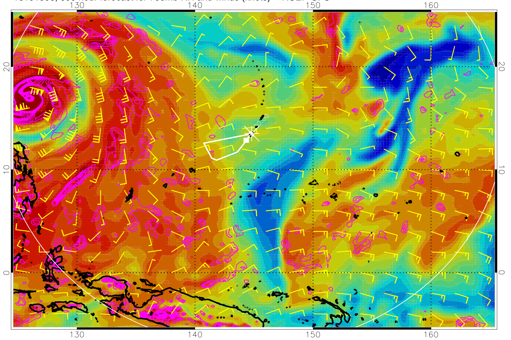
16101906, 090 hour forecast for 700mb RH and winds (knots) -- NCEP GFS
