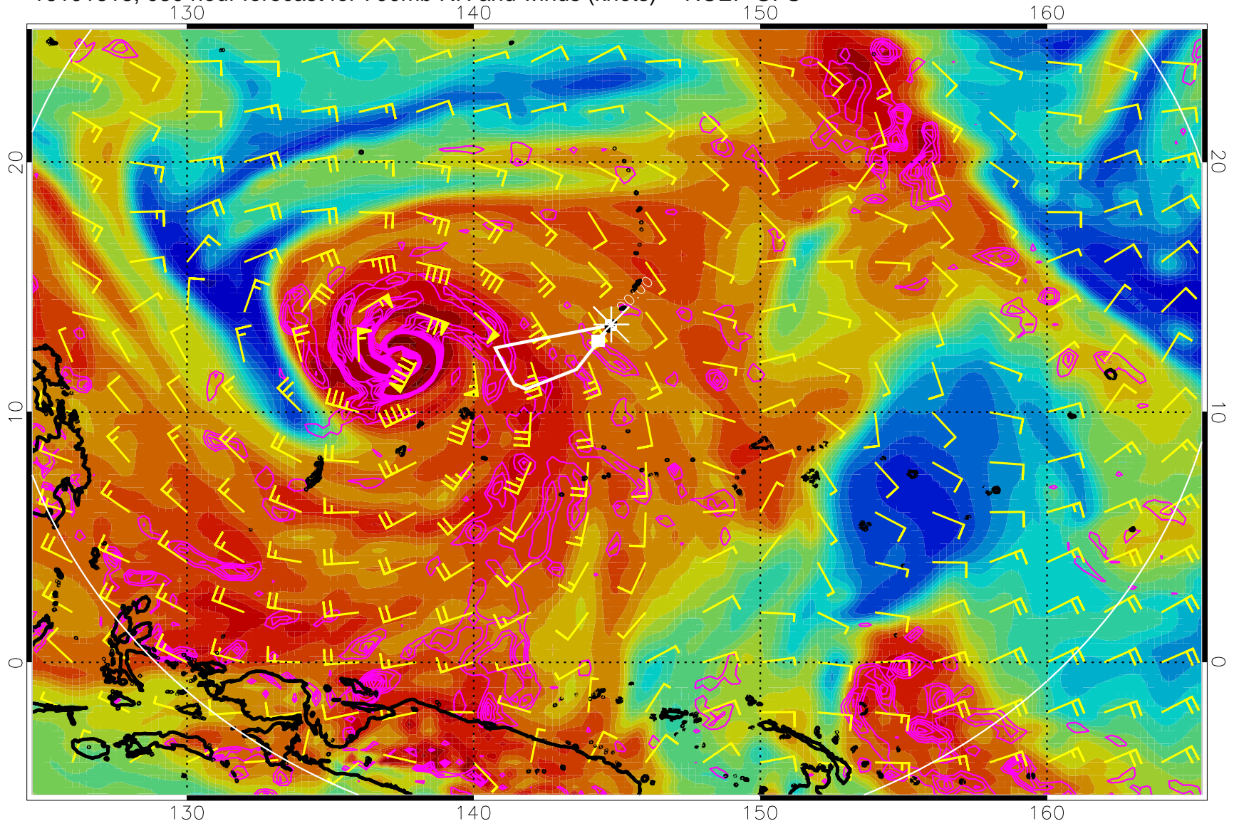
16101618, 030 hour forecast for 700mb RH and winds (knots) -- NCEP GFS
