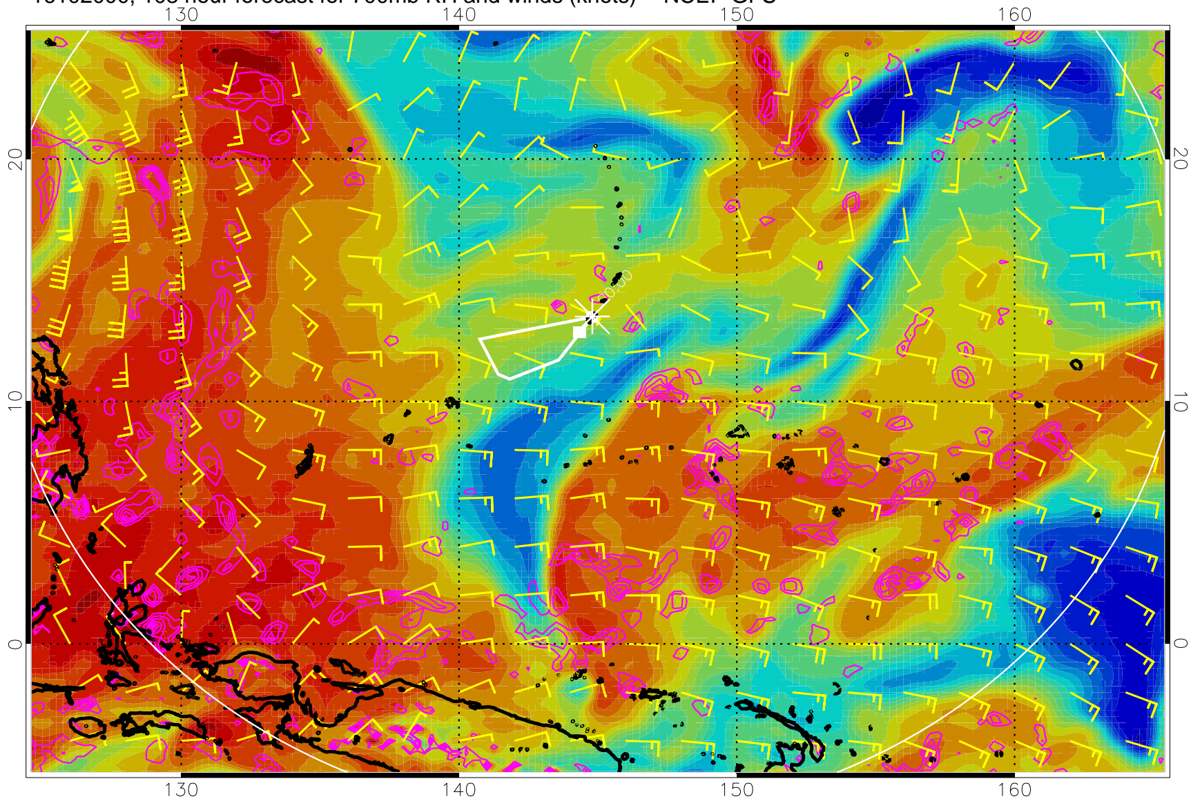
16102000, 108 hour forecast for 700mb RH and winds (knots) -- NCEP GFS
