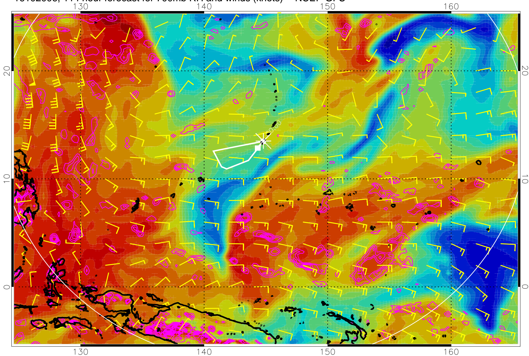
16102006, 114 hour forecast for 700mb RH and winds (knots) -- NCEP GFS
