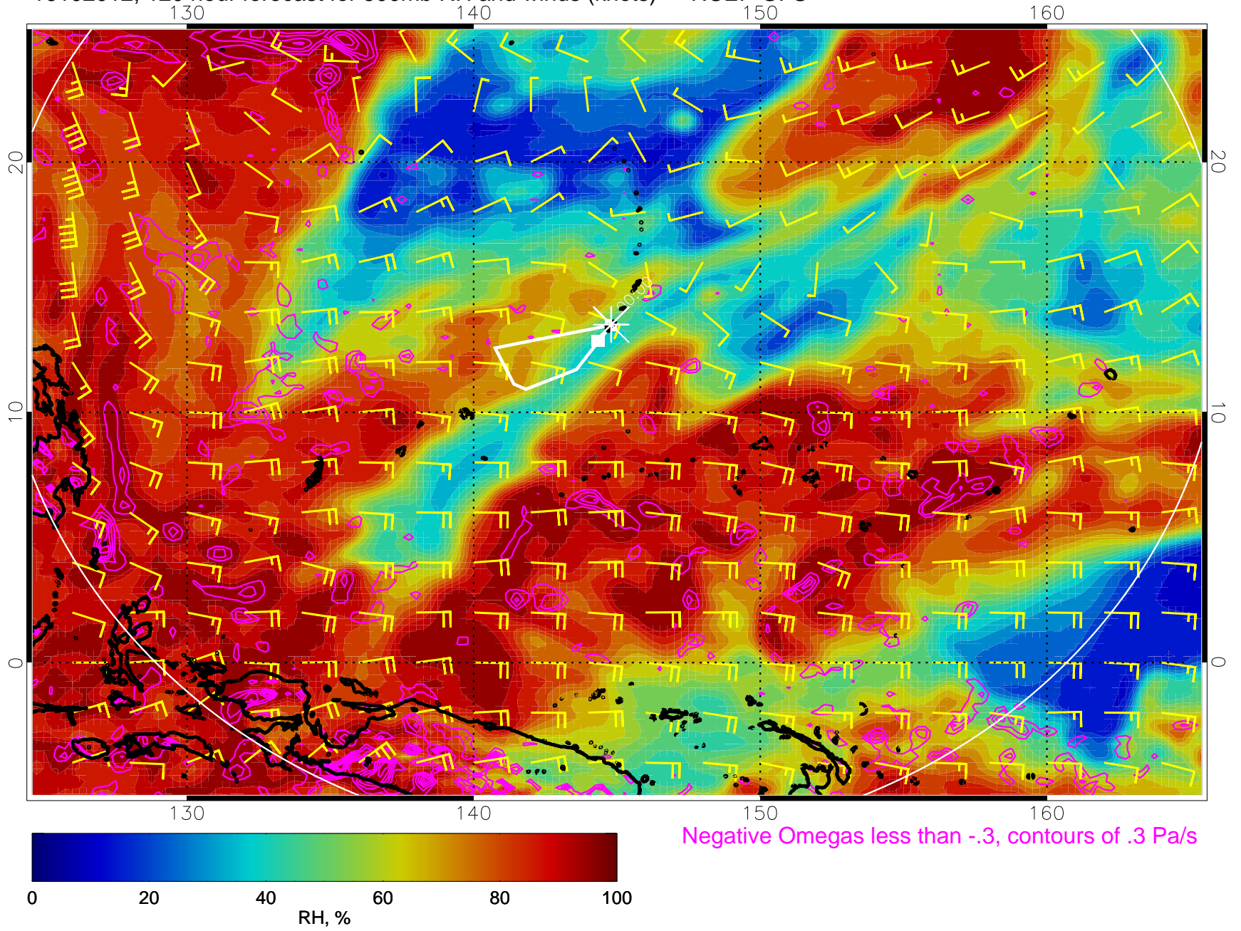
16102012, 120 hour forecast for 500mb RH and winds (knots) -- NCEP GFS
