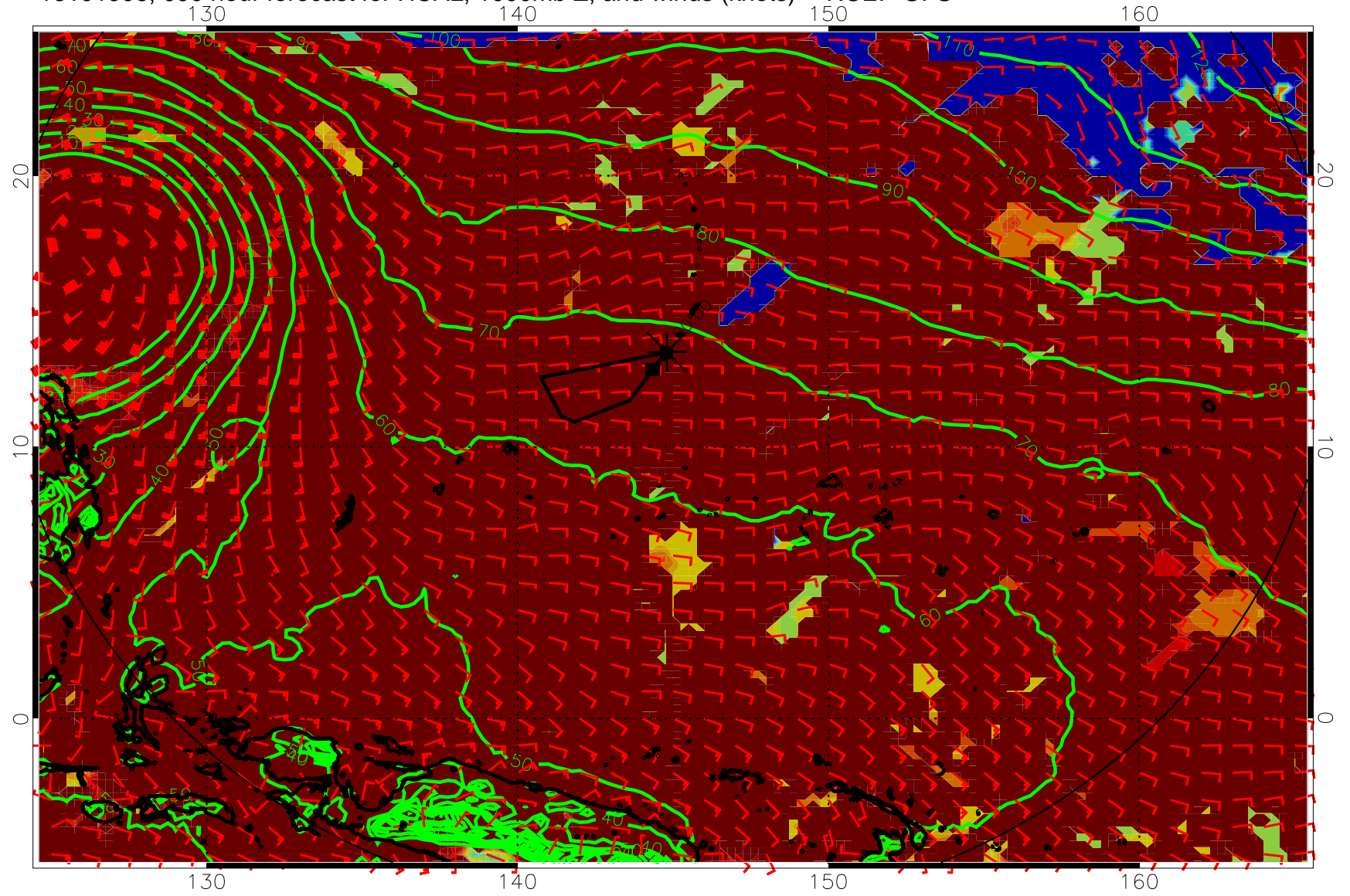
16101906, 090 hour forecast for HCAL, 1000mb Z, and winds (knots) -- NCEP GFS
