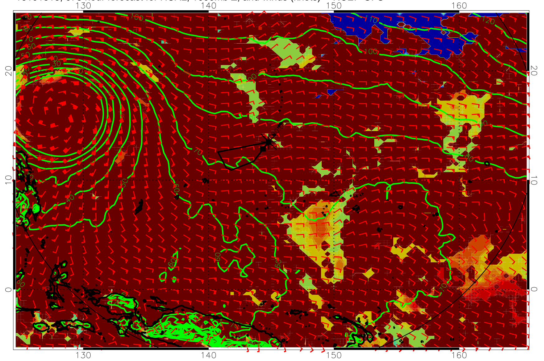
16101818, 078 hour forecast for HCAL, 1000mb Z, and winds (knots) -- NCEP GFS
