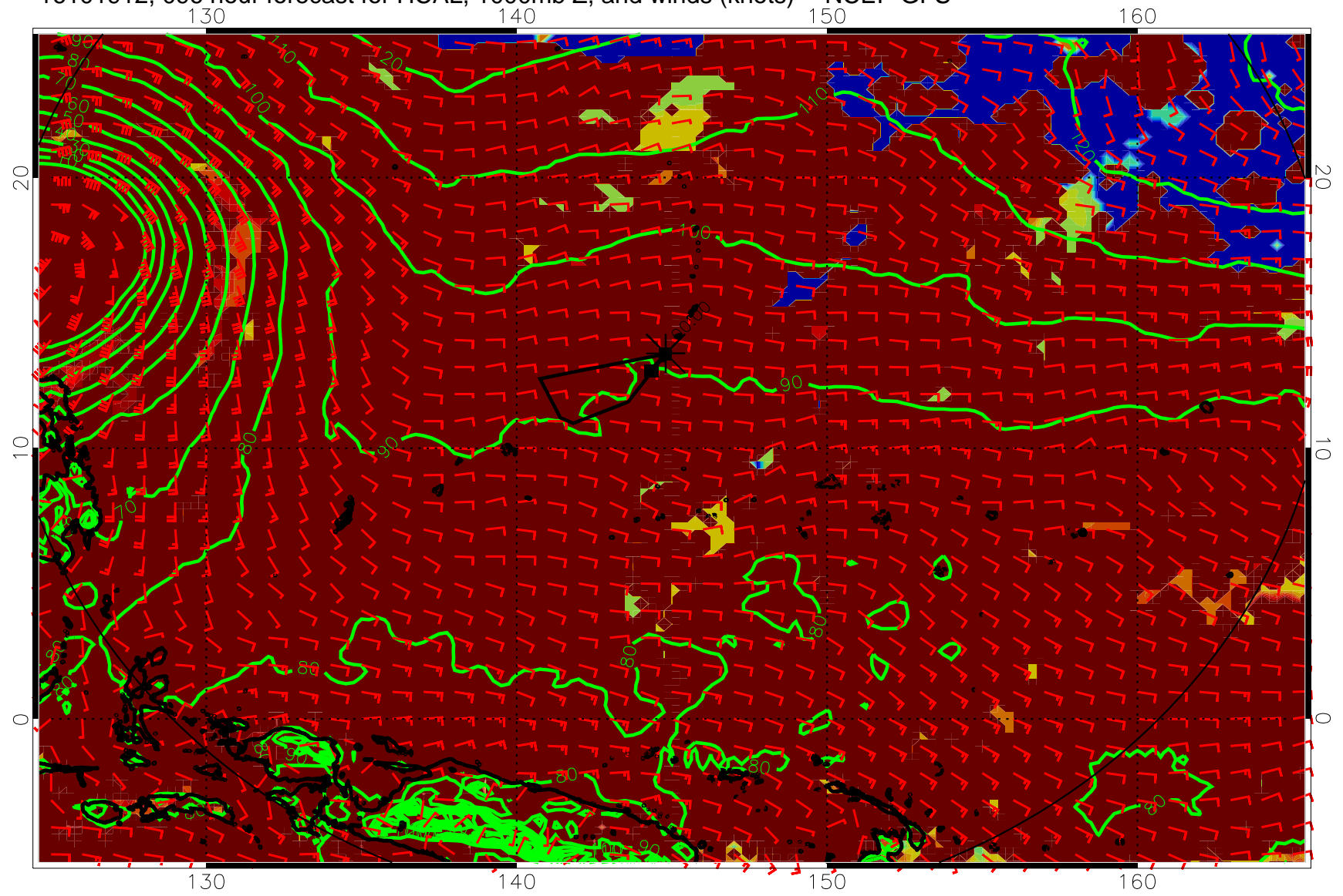
16101912, 096 hour forecast for HCAL, 1000mb Z, and winds (knots) -- NCEP GFS
