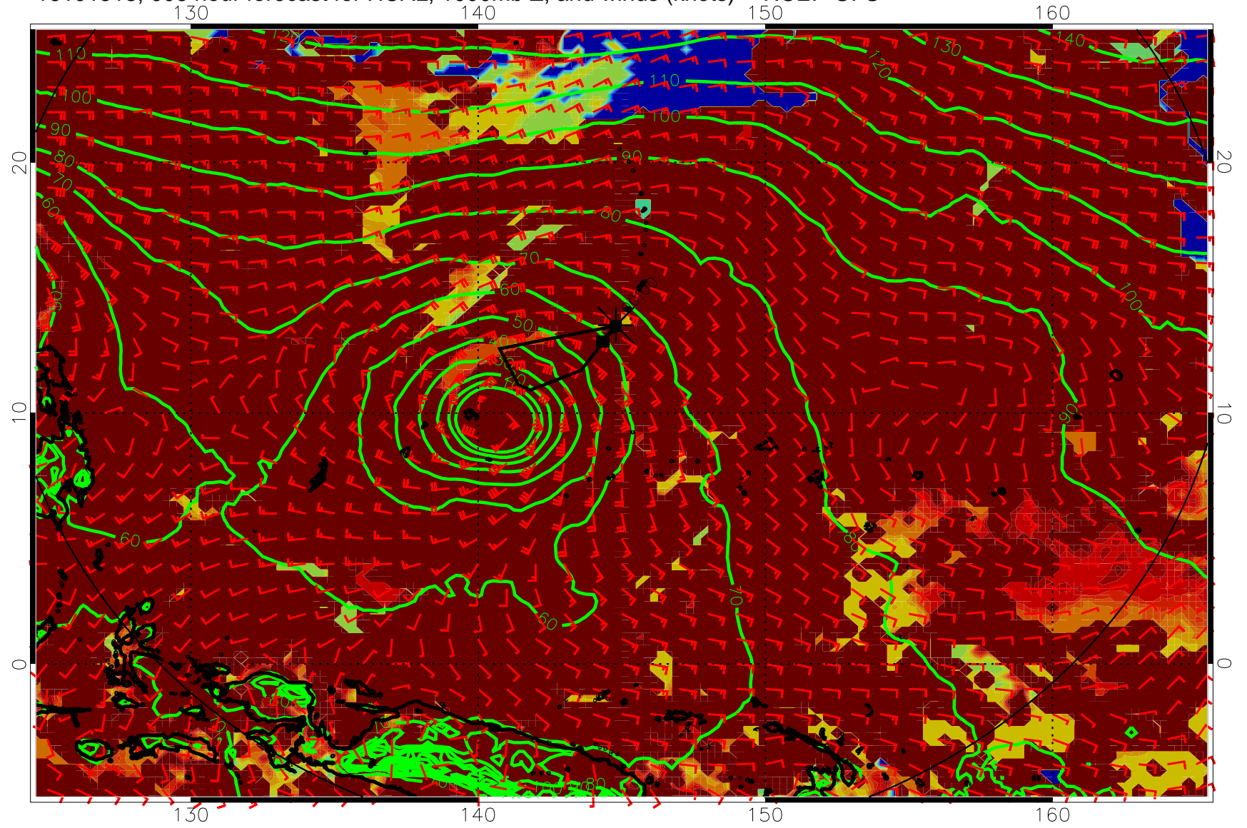
16101518, 006 hour forecast for HCAL, 1000mb Z, and winds (knots) -- NCEP GFS
