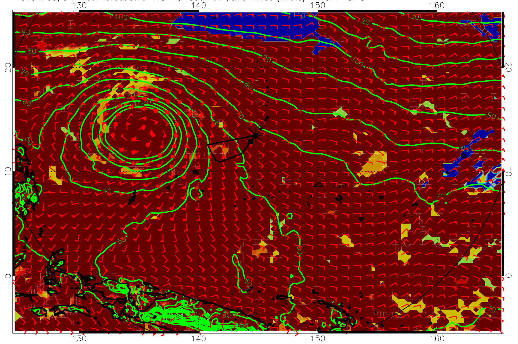
16101706, 04Z hour forecast for HCAL, 1000mb Z, and winds (knots) -- NCEP GFS
