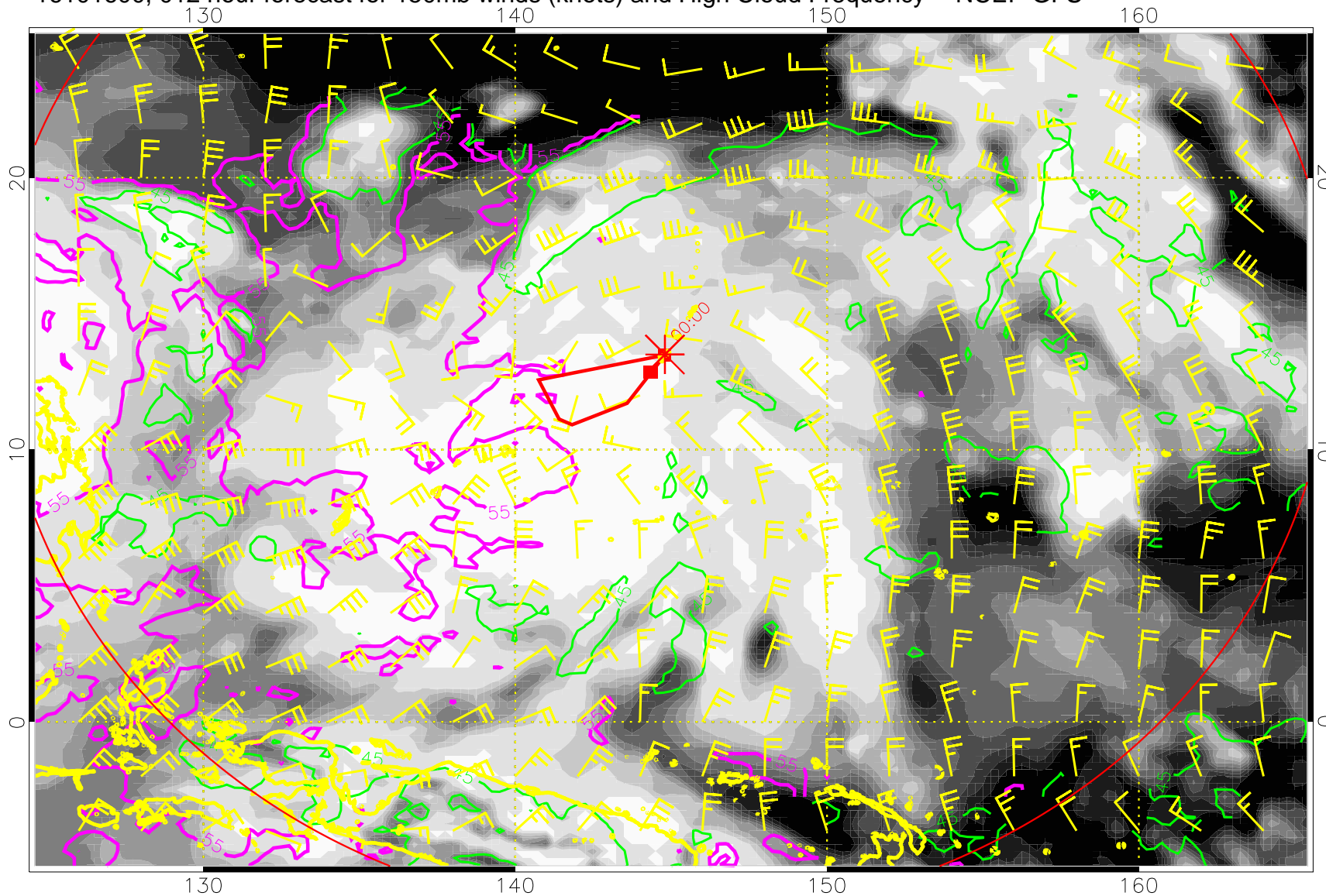
16101600, 012 hour forecast for 150mb winds (knots) and High Cloud Frequency -- NCEP GFS
