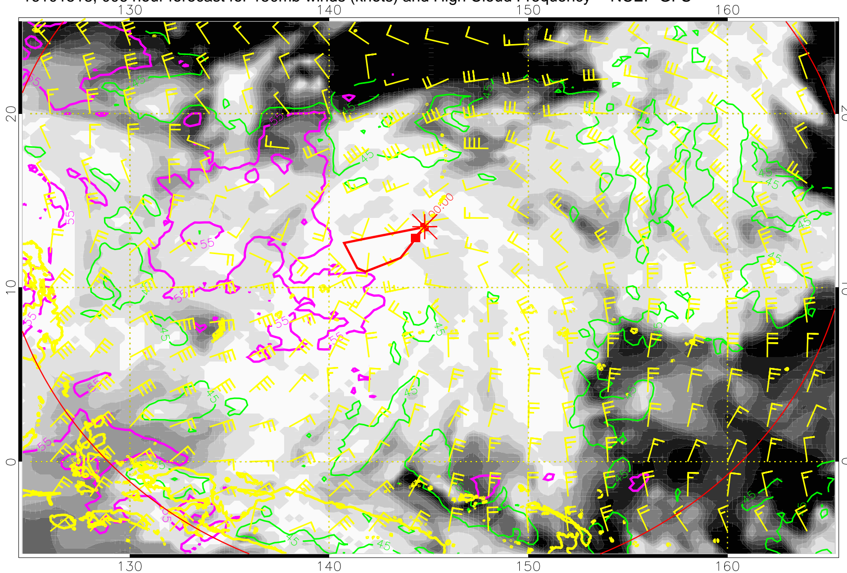
16101518, 006 hour forecast for 150mb winds (knots) and High Cloud Frequency -- NCEP GFS
