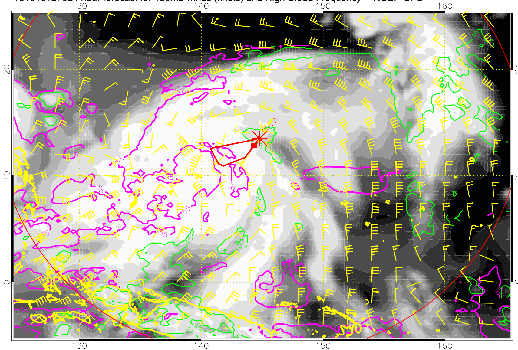
16101612, 024 hour forecast for 150mb winds (knots) and High Cloud Frequency -- NCEP GFS
