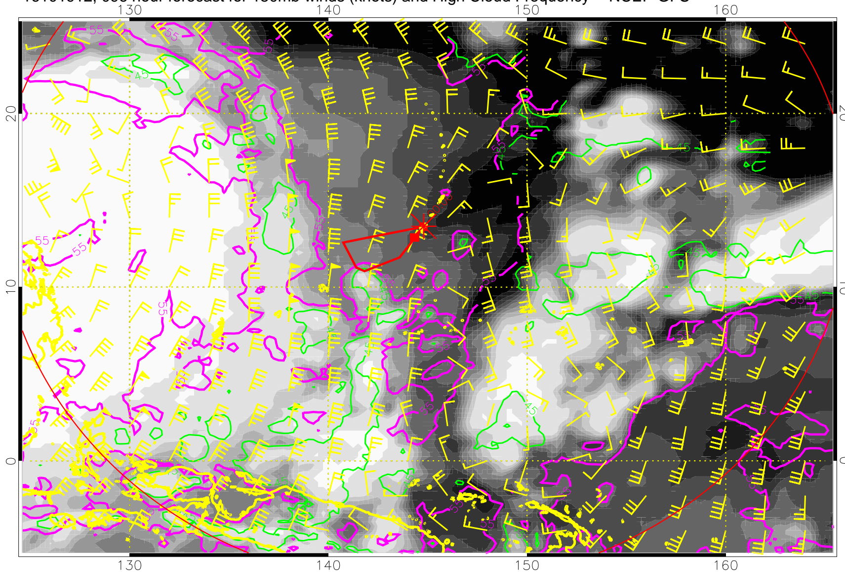
16101912, 096 hour forecast for 150mb winds (knots) and High Cloud Frequency -- NCEP GFS
