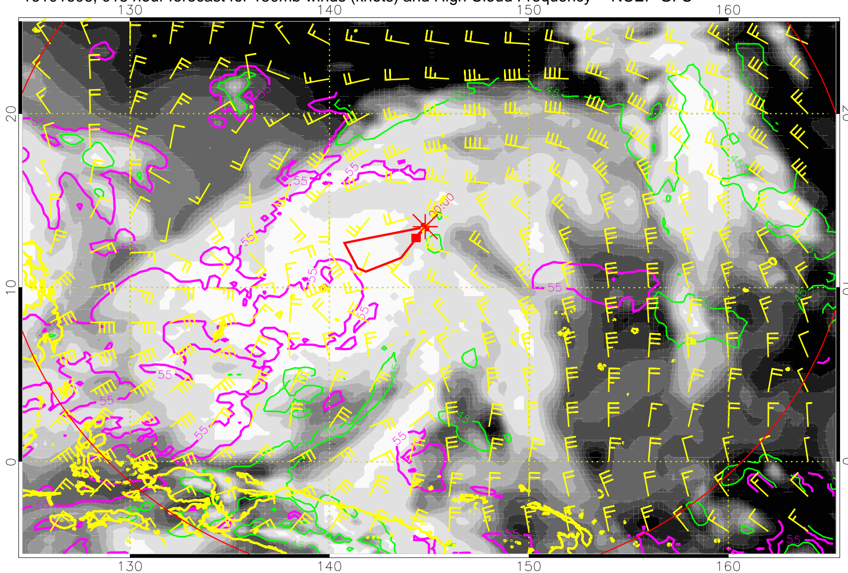
16101606, 018 hour forecast for 150mb winds (knots) and High Cloud Frequency -- NCEP GFS
