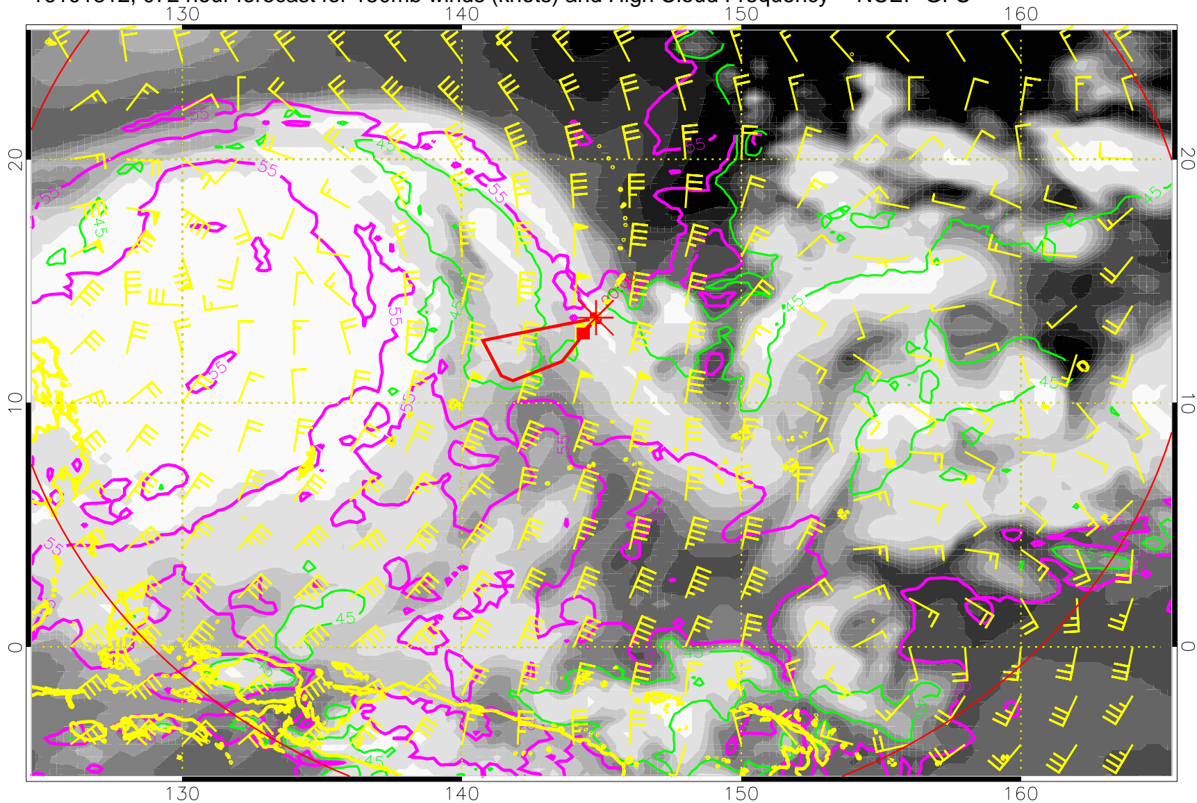
16101812, 072 hour forecast for 150mb winds (knots) and High Cloud Frequency -- NCEP GFS
