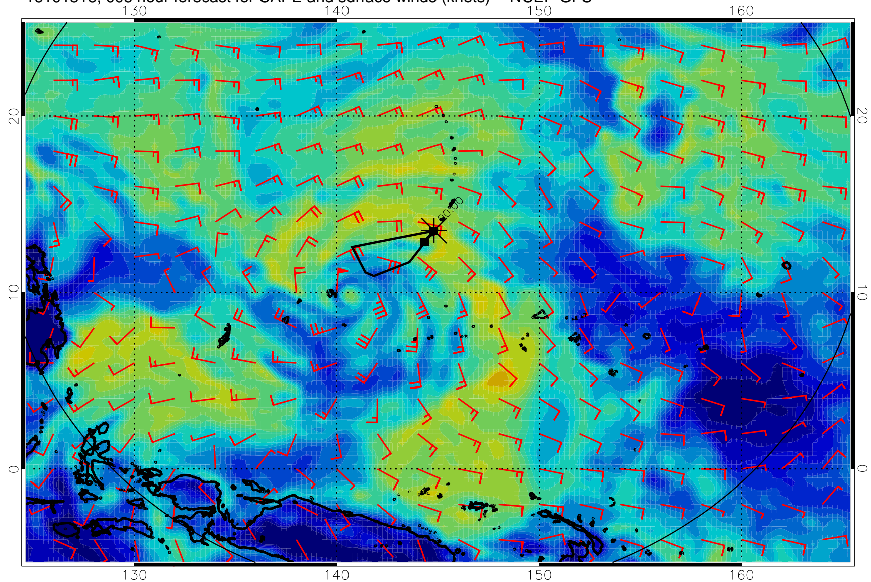
16101518, 006 hour forecast for CAPE and surface winds (knots) -- NCEP GFS
