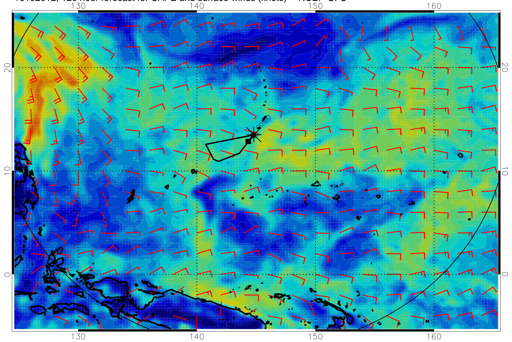
16102012, 120 hour forecast for CAPE and surface winds (knots) -- NCEP GFS
