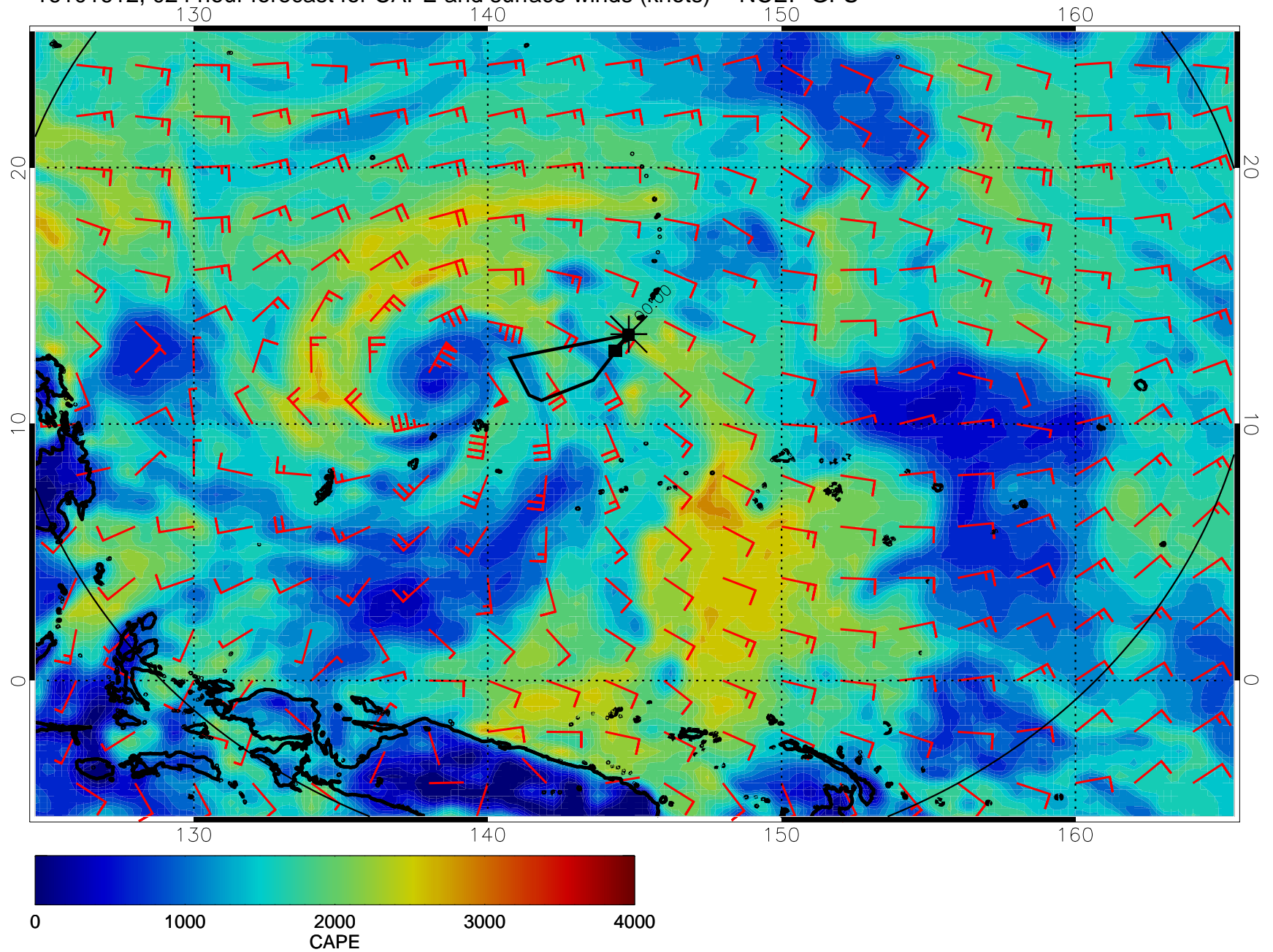
16101612, 024 hour forecast for CAPE and surface winds (knots) -- NCEP GFS
