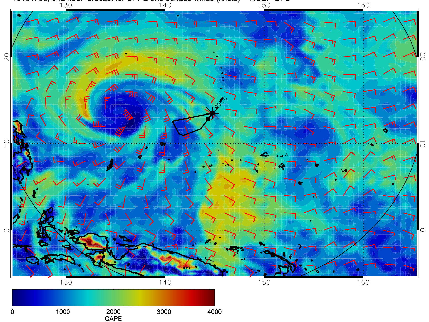
16101706, 042 hour forecast for CAPE and surface winds (knots) -- NCEP GFS
