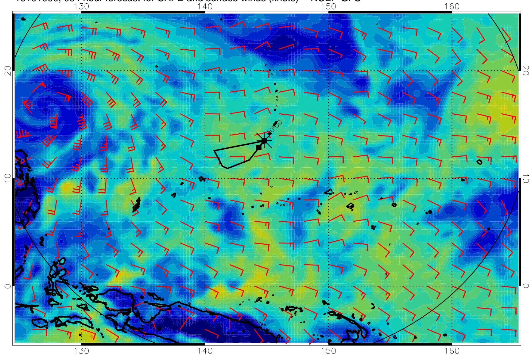
16101900, 084 hour forecast for CAPE and surface winds (knots) -- NCEP GFS
