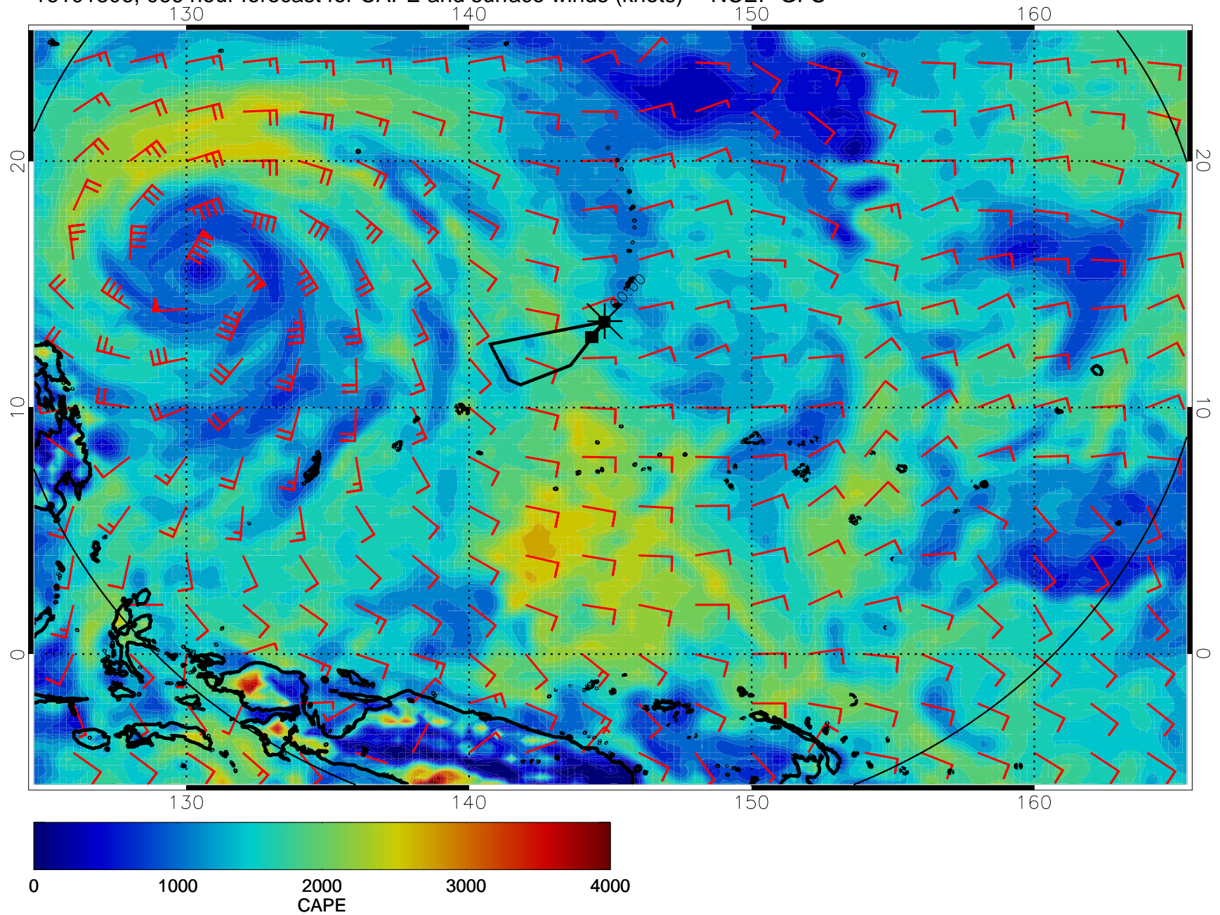
16101806, 066 hour forecast for CAPE and surface winds (knots) -- NCEP GFS
