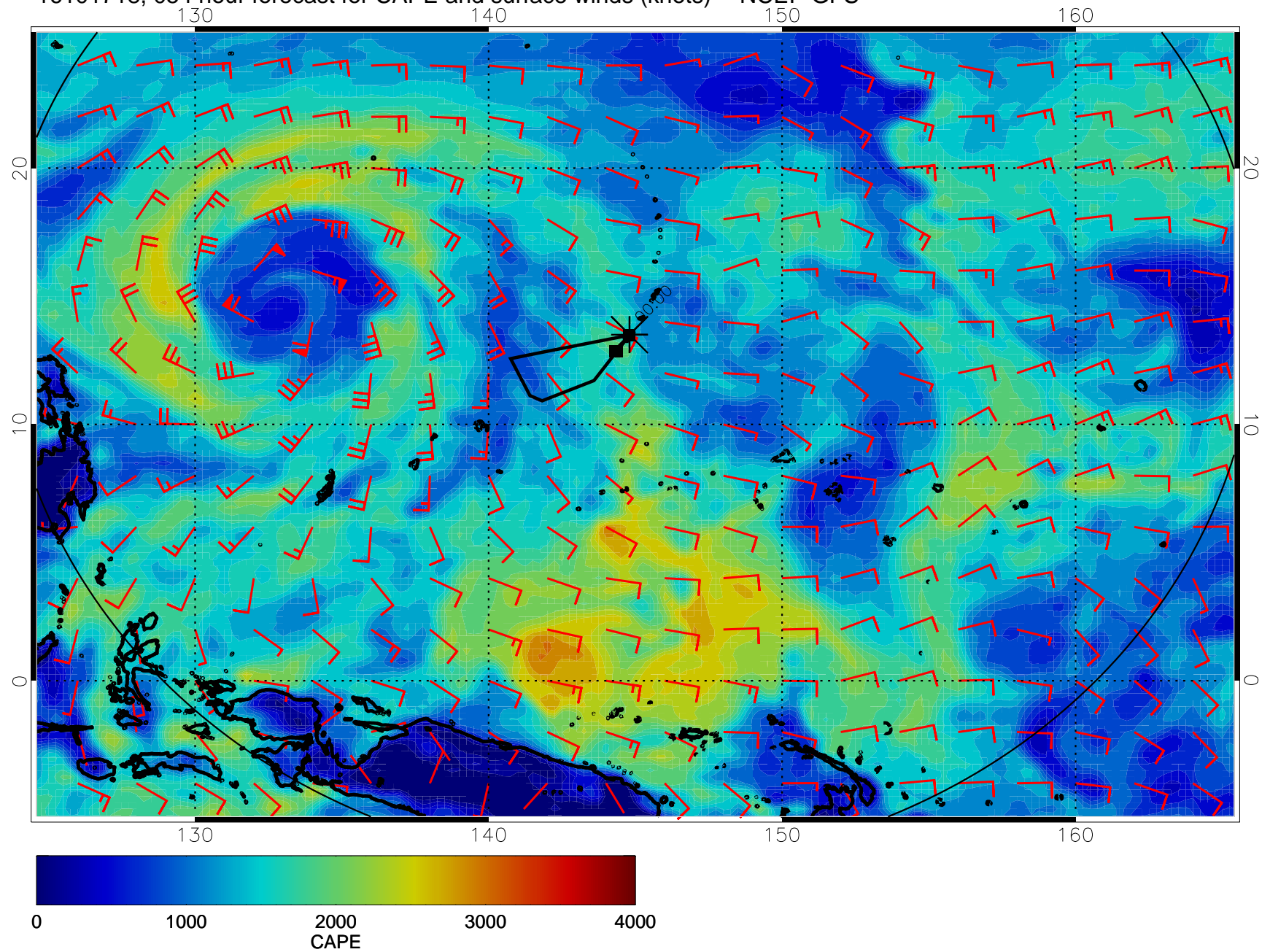
16101718, 054 hour forecast for CAPE and surface winds (knots) -- NCEP GFS
