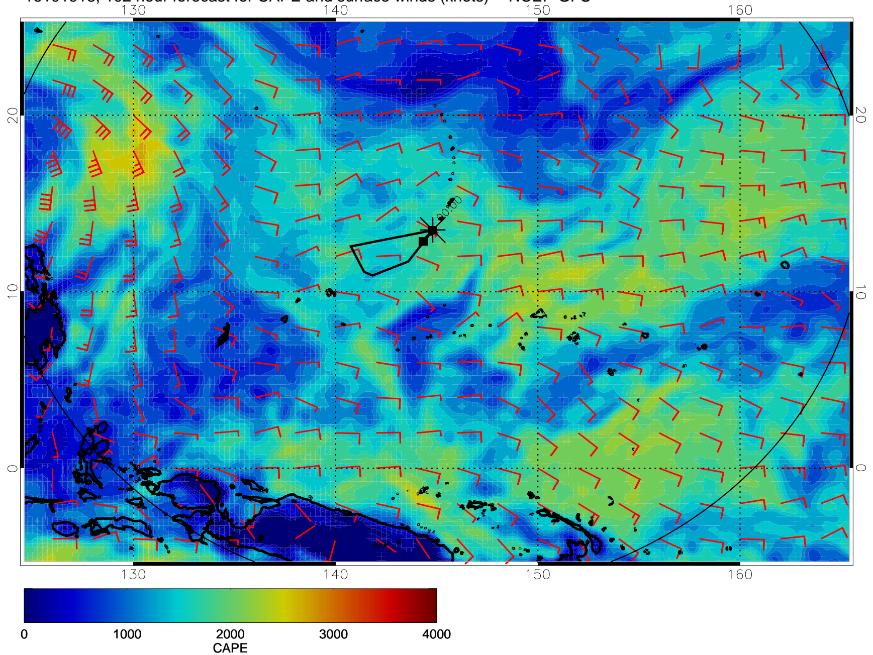
16101918, 102 hour forecast for CAPE and surface winds (knots) -- NCEP GFS
