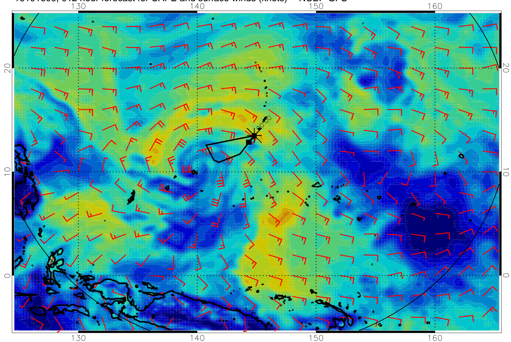
16101600, 012 hour forecast for CAPE and surface winds (knots) -- NCEP GFS
