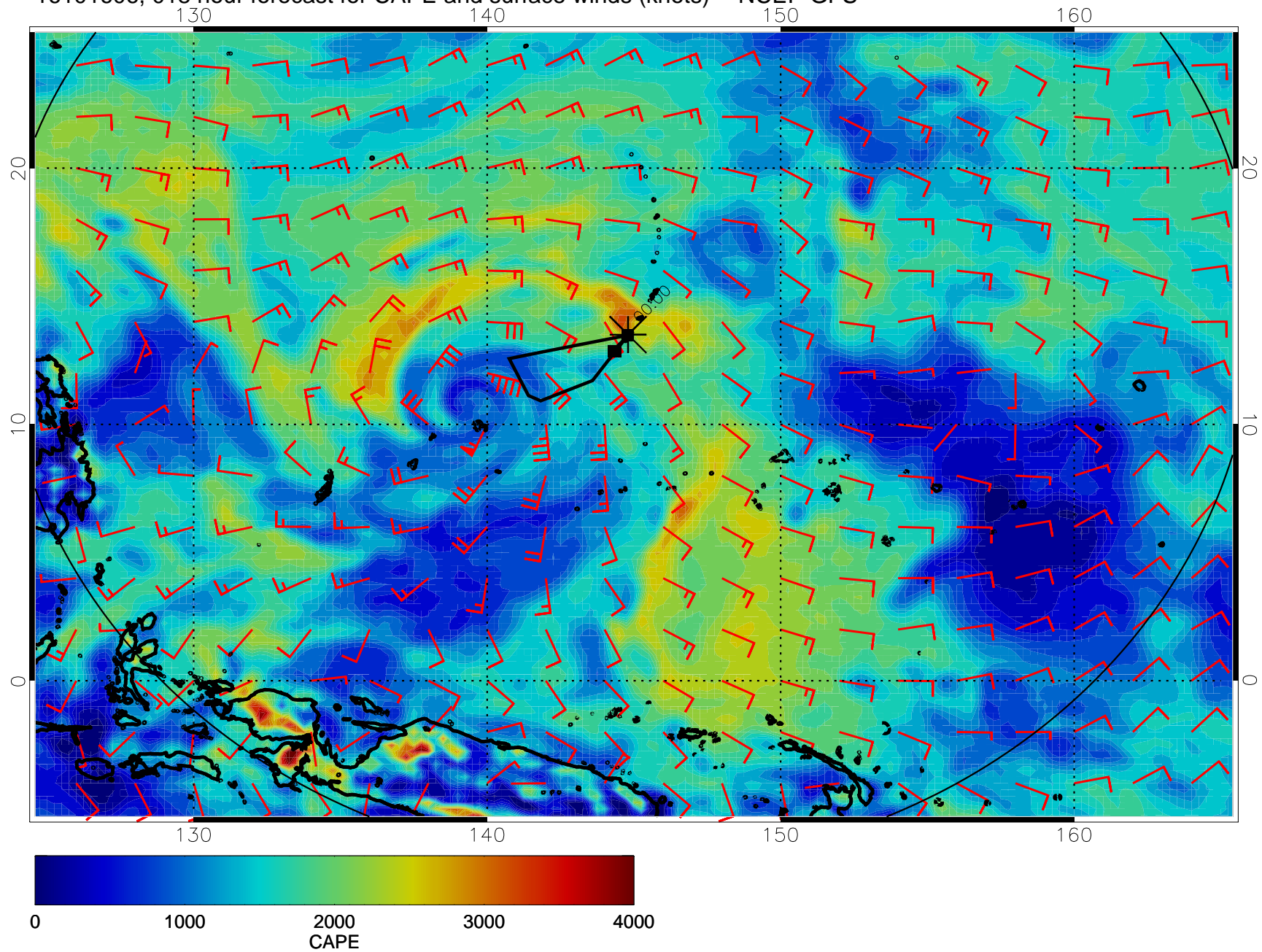
16101606, 018 hour forecast for CAPE and surface winds (knots) -- NCEP GFS
