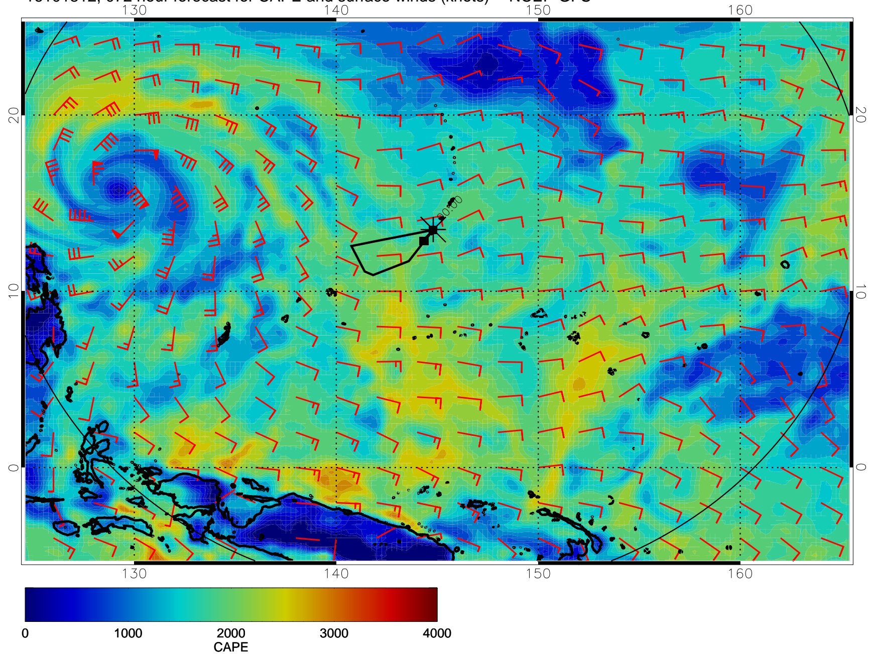
16101812, 072 hour forecast for CAPE and surface winds (knots) -- NCEP GFS
