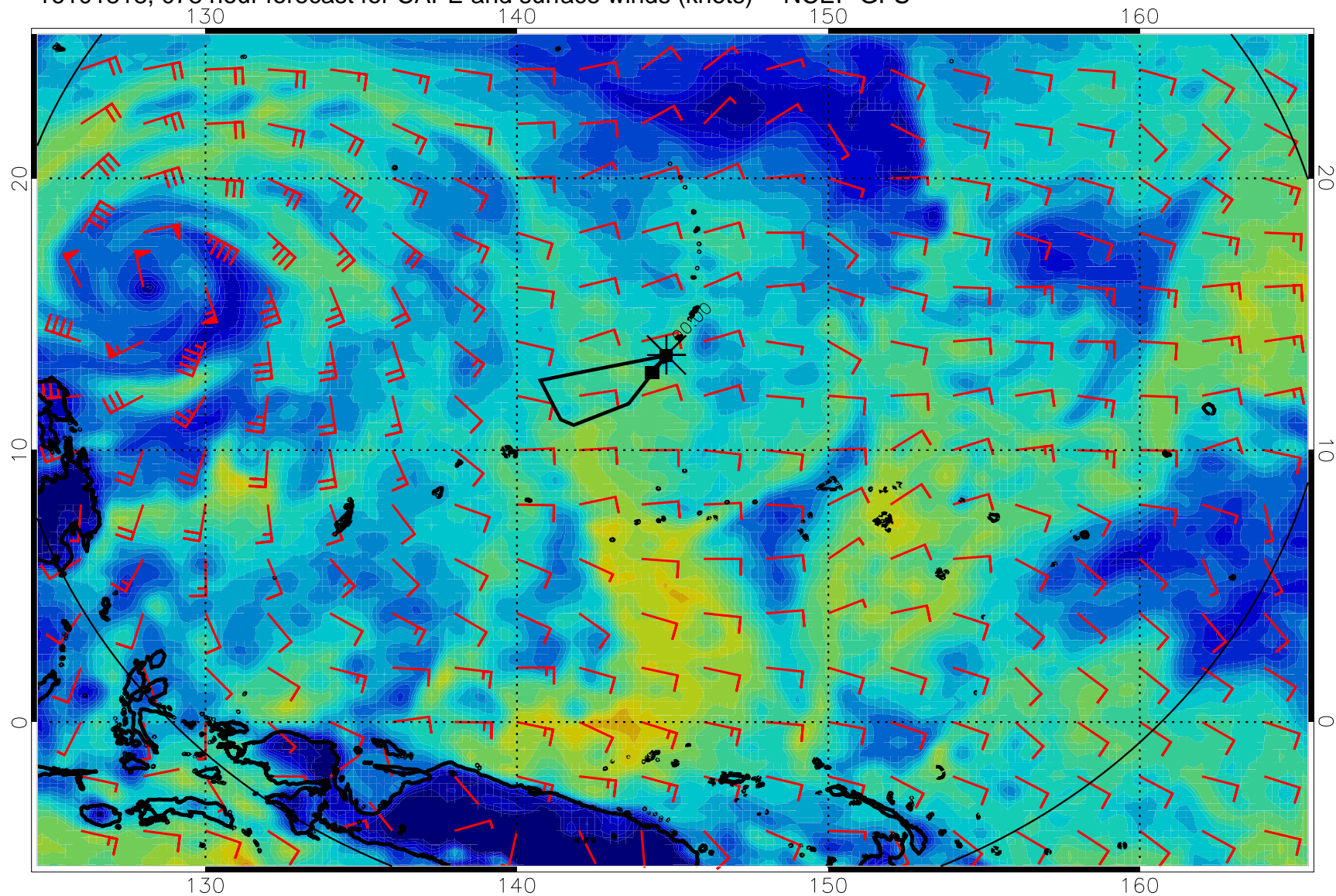
16101818, 078 hour forecast for CAPE and surface winds (knots) -- NCEP GFS
