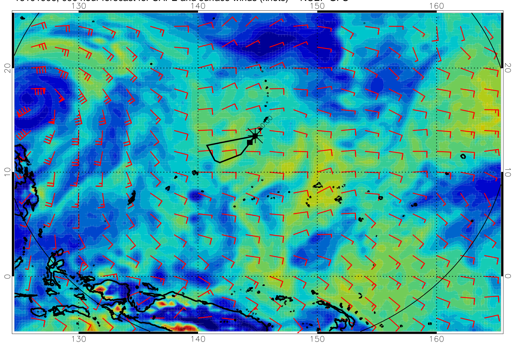
16101906, 090 hour forecast for CAPE and surface winds (knots) -- NCEP GFS
