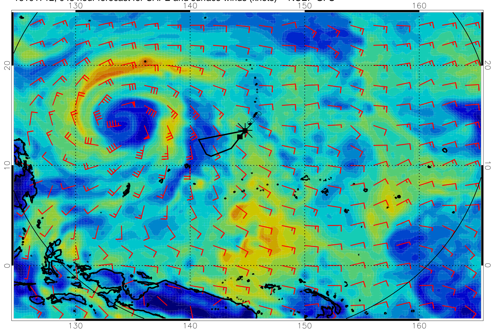
16101712, 048 hour forecast for CAPE and surface winds (knots) -- NCEP GFS
