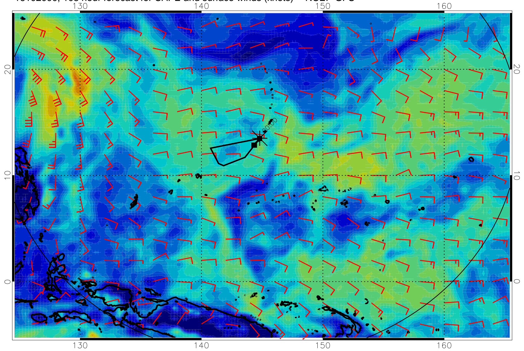
16102000, 108 hour forecast for CAPE and surface winds (knots) -- NCEP GFS
