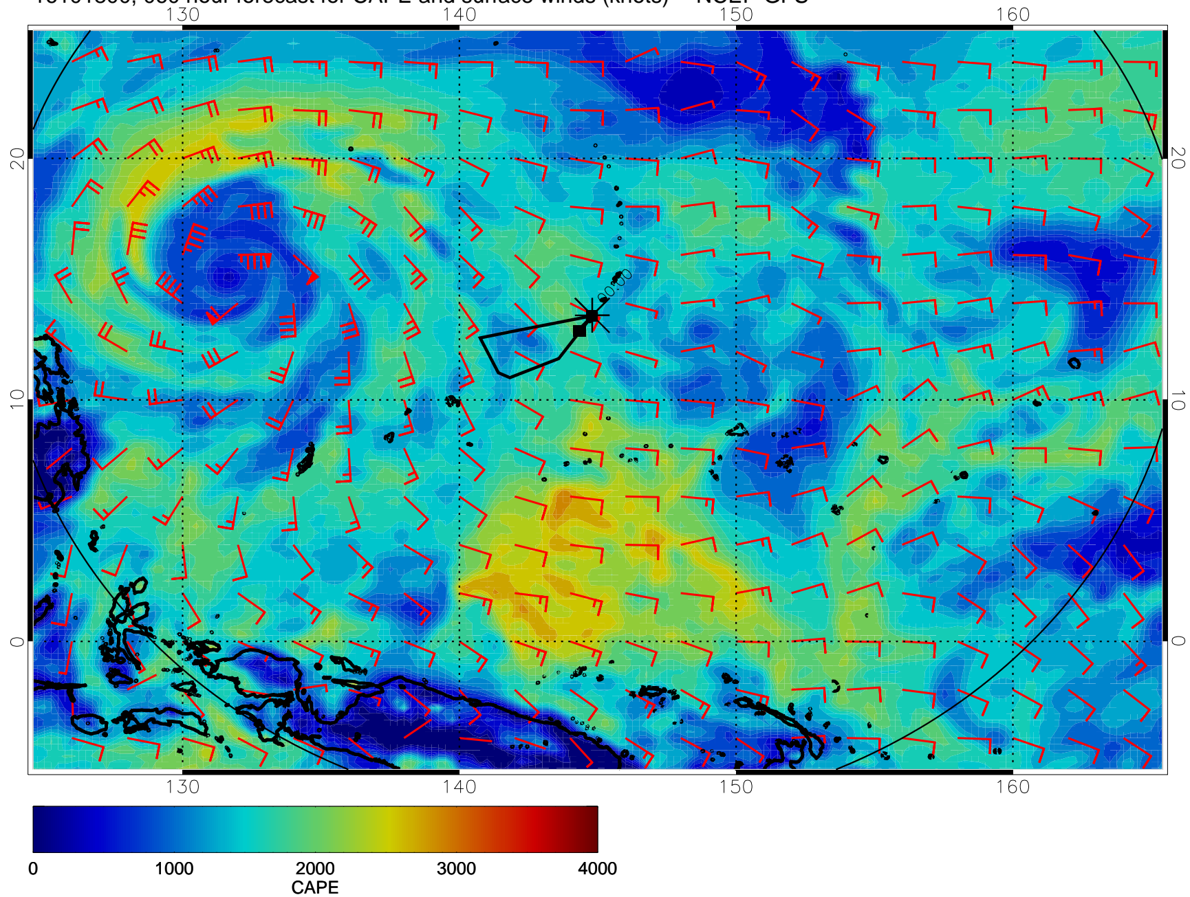
16101800, 060 hour forecast for CAPE and surface winds (knots) -- NCEP GFS
