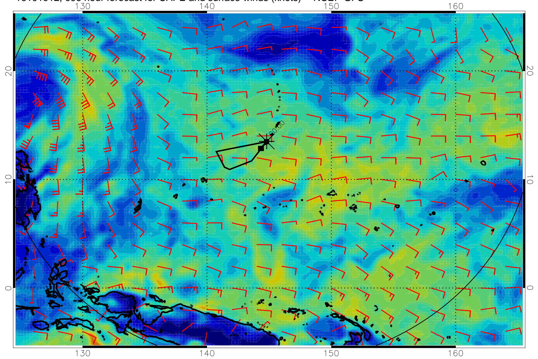
16101912, 096 hour forecast for CAPE and surface winds (knots) -- NCEP GFS
