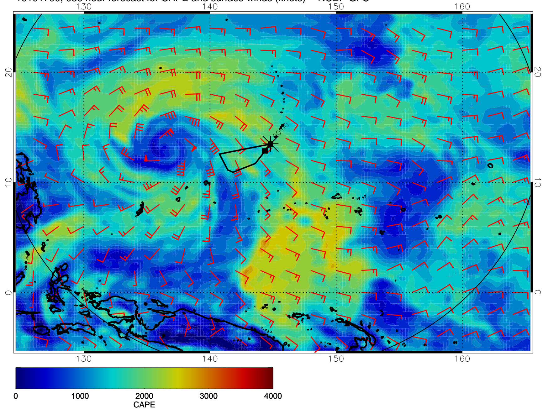
16101700, 036 hour forecast for CAPE and surface winds (knots) -- NCEP GFS
