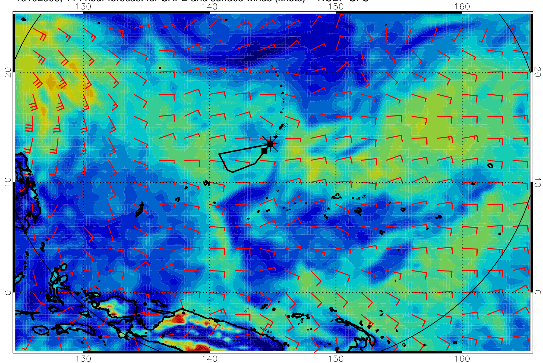
16102006, 114 hour forecast for CAPE and surface winds (knots) -- NCEP GFS
