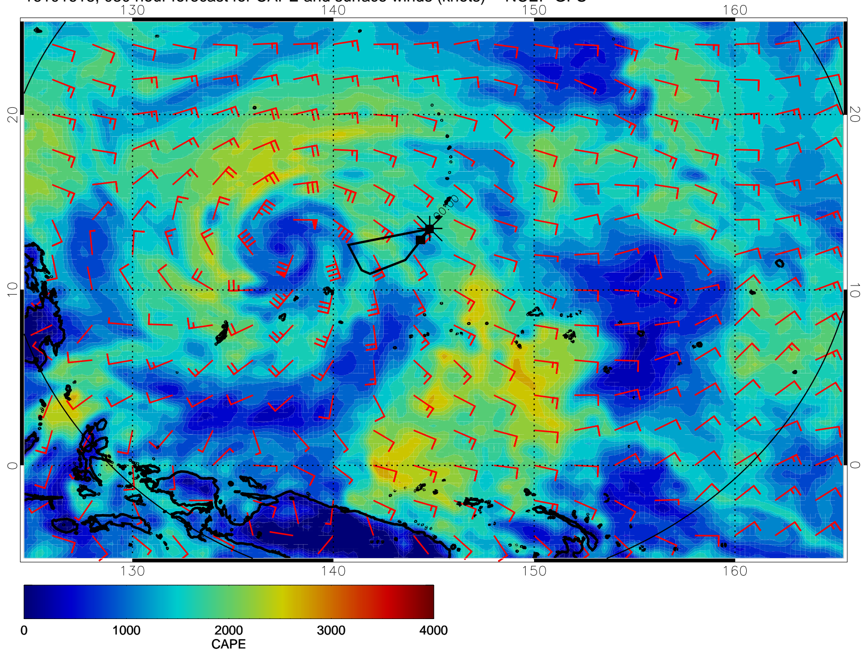
16101618, 030 hour forecast for CAPE and surface winds (knots) -- NCEP GFS
