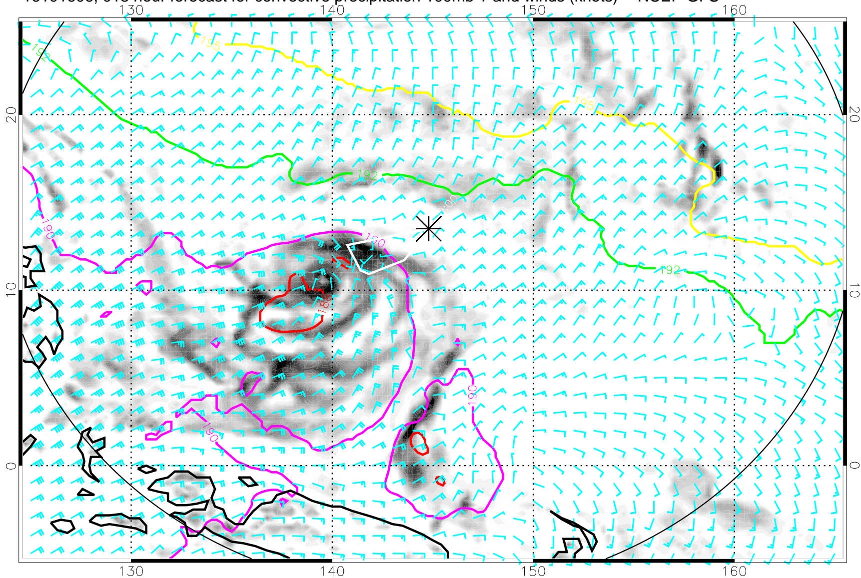
16101606, 018 hour forecast for convective precipitation 100mb T and winds (knots) -- NCEP GFS
