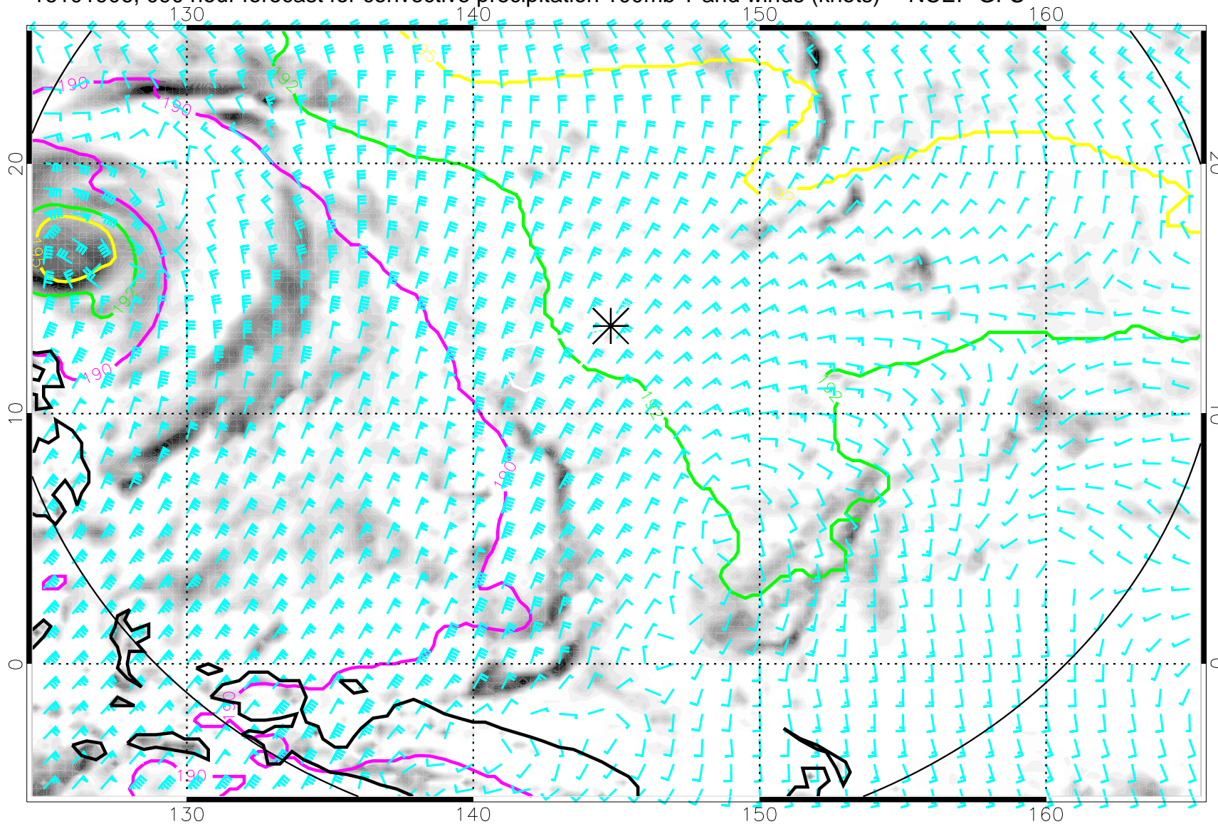
16101906, 090 hour forecast for convective precipitation 100mb T and winds (knots) -- NCEP GFS
