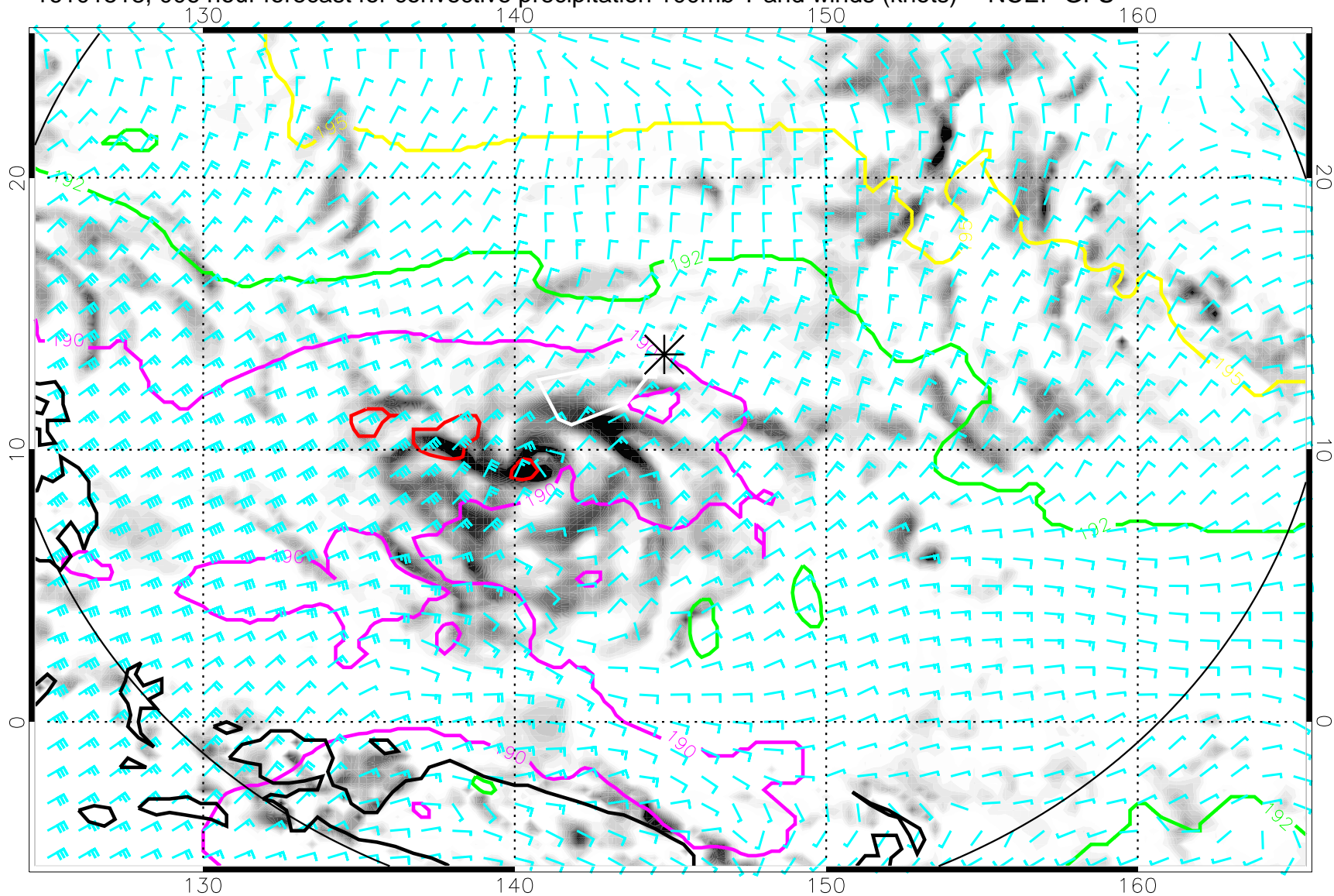
16101518, 006 hour forecast for convective precipitation 100mb T and winds (knots) -- NCEP GFS
