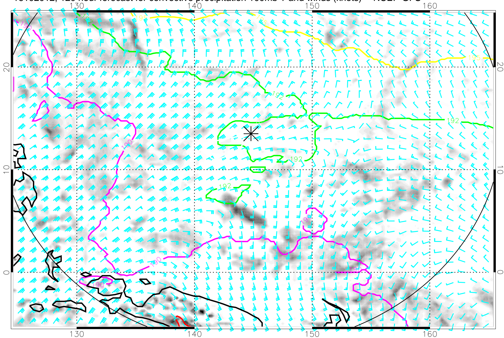
16102012, 120 hour forecast for convective precipitation 100mb T and winds (knots) -- NCEP GFS
