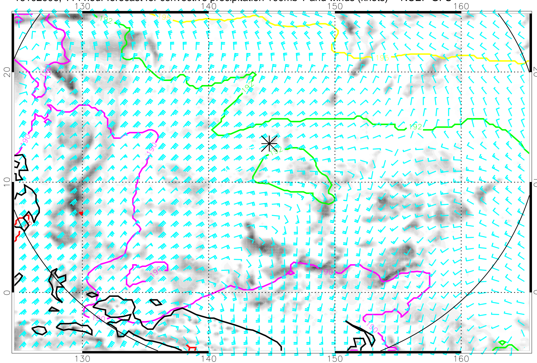
16102006, 114 hour forecast for convective precipitation 100mb T and winds (knots) -- NCEP GFS
