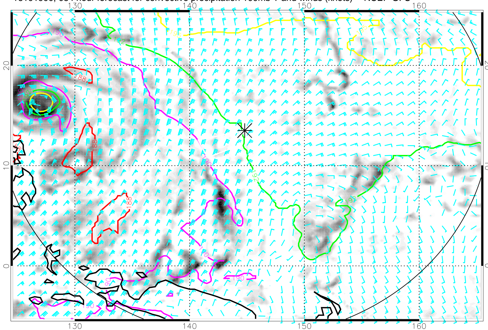
16101900, 084 hour forecast for convective precipitation 100mb T and winds (knots) -- NCEP GFS
