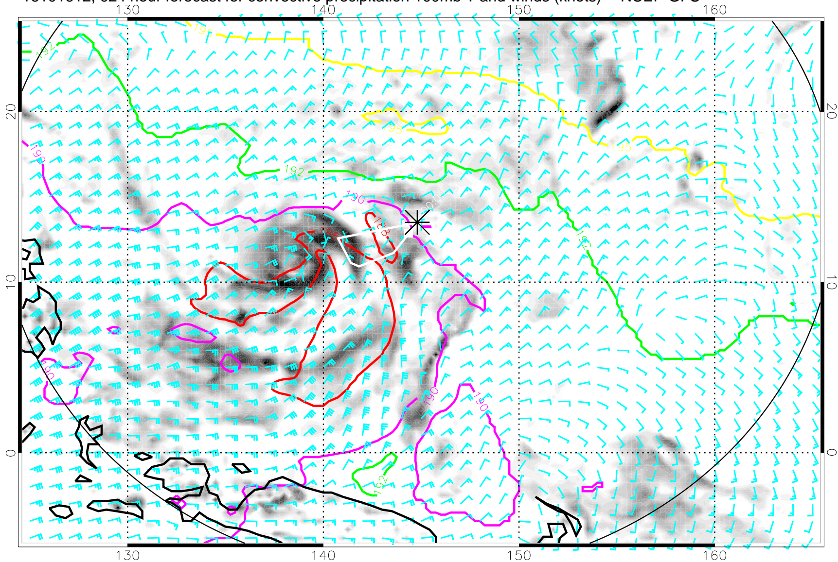
16101612, 024 hour forecast for convective precipitation 100mb T and winds (knots) -- NCEP GFS
