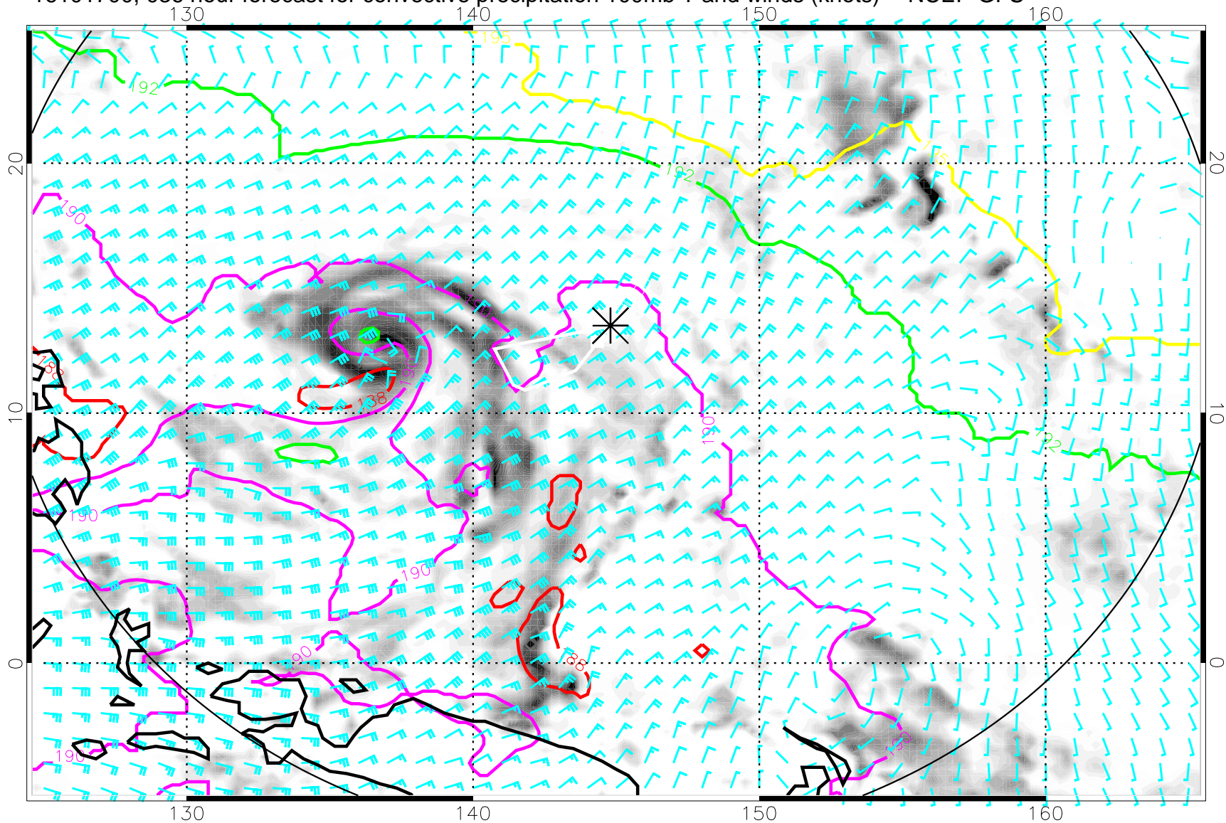
16101700, 036 hour forecast for convective precipitation 100mb T and winds (knots) -- NCEP GFS
