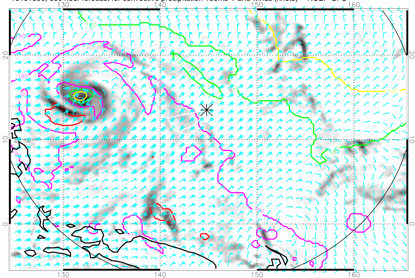
16101800, 060 hour forecast for convective precipitation 100mb T and winds (knots) -- NCEP GFS
