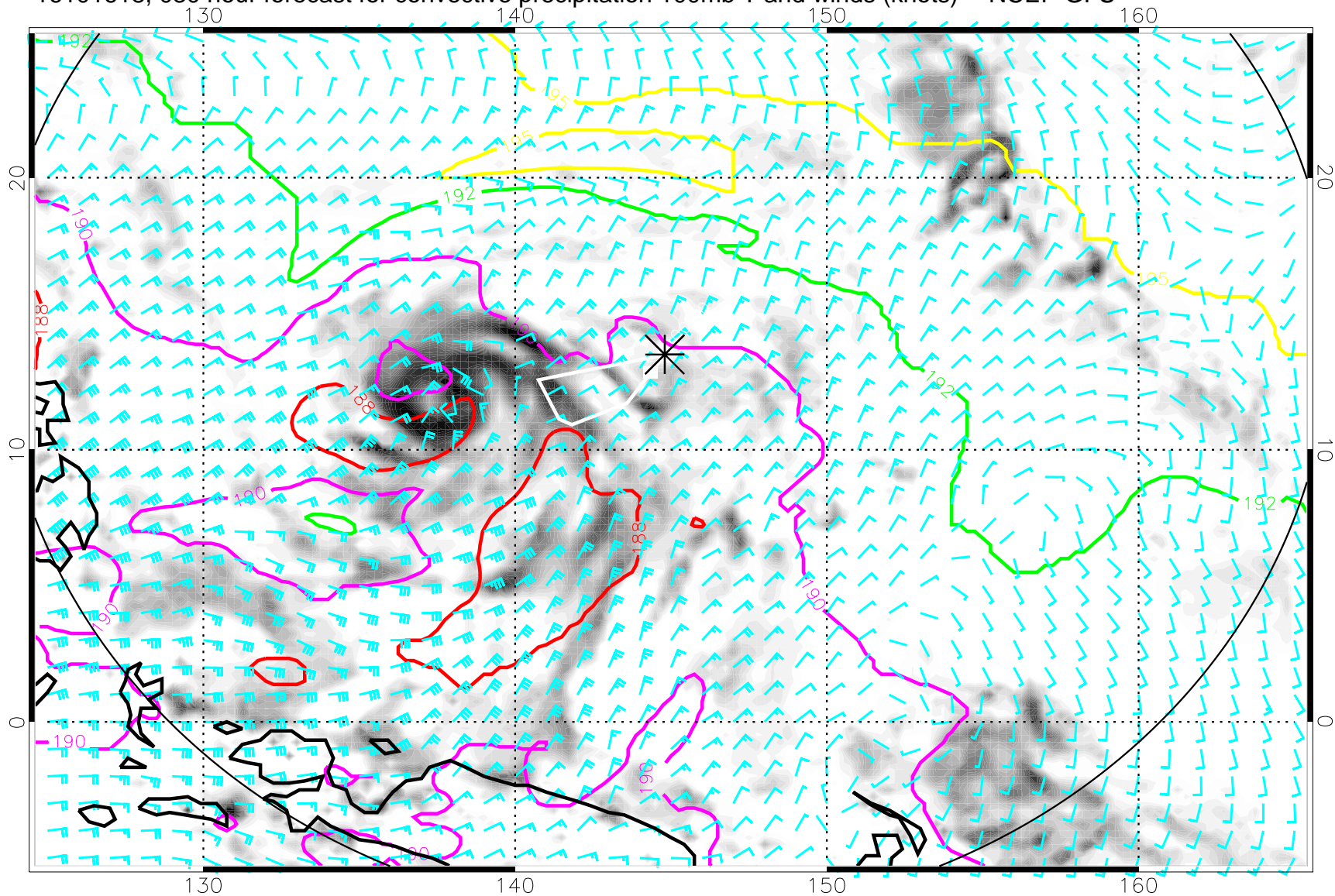
16101618, 030 hour forecast for convective precipitation 100mb T and winds (knots) -- NCEP GFS
