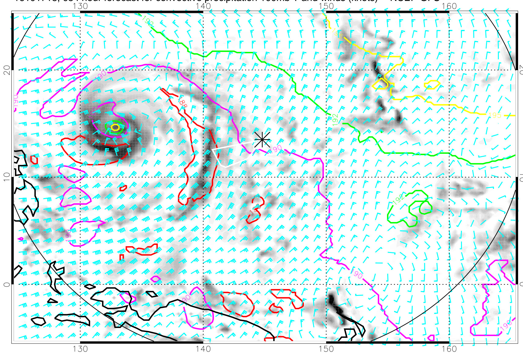
16101718, 054 hour forecast for convective precipitation 100mb T and winds (knots) -- NCEP GFS
