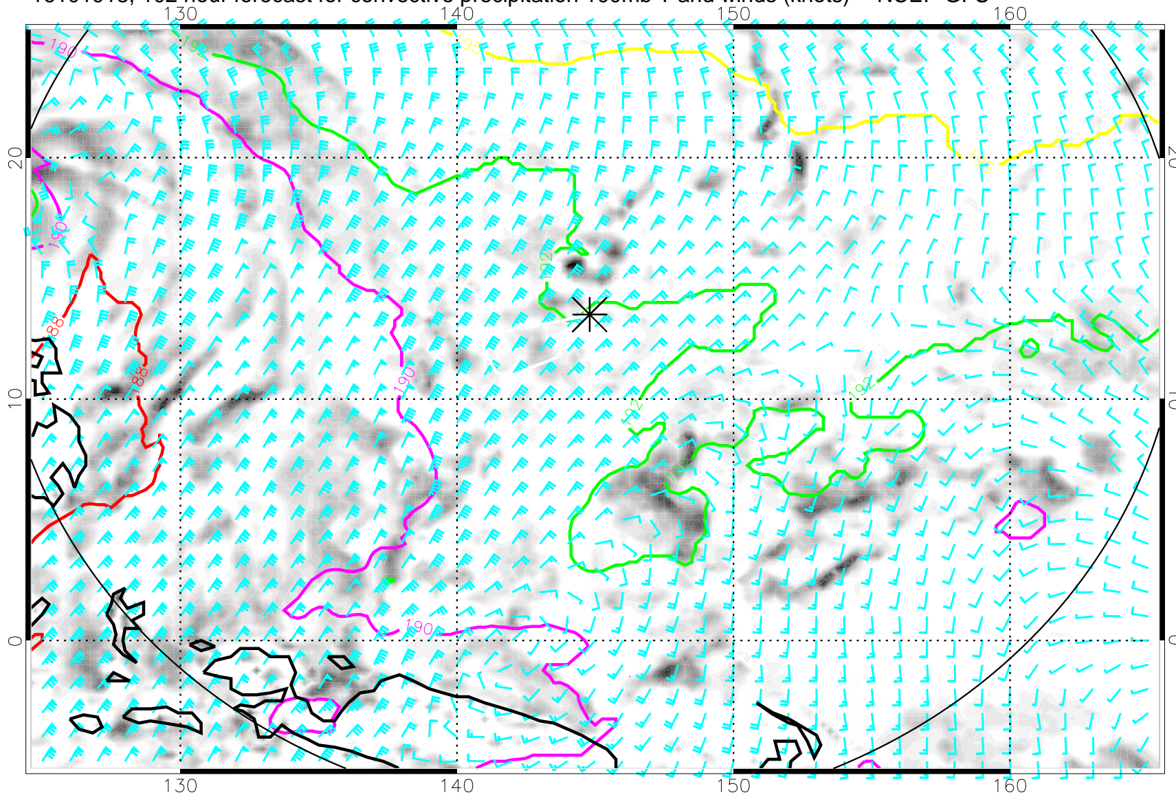
16101918, 102 hour forecast for convective precipitation 100mb T and winds (knots) -- NCEP GFS
