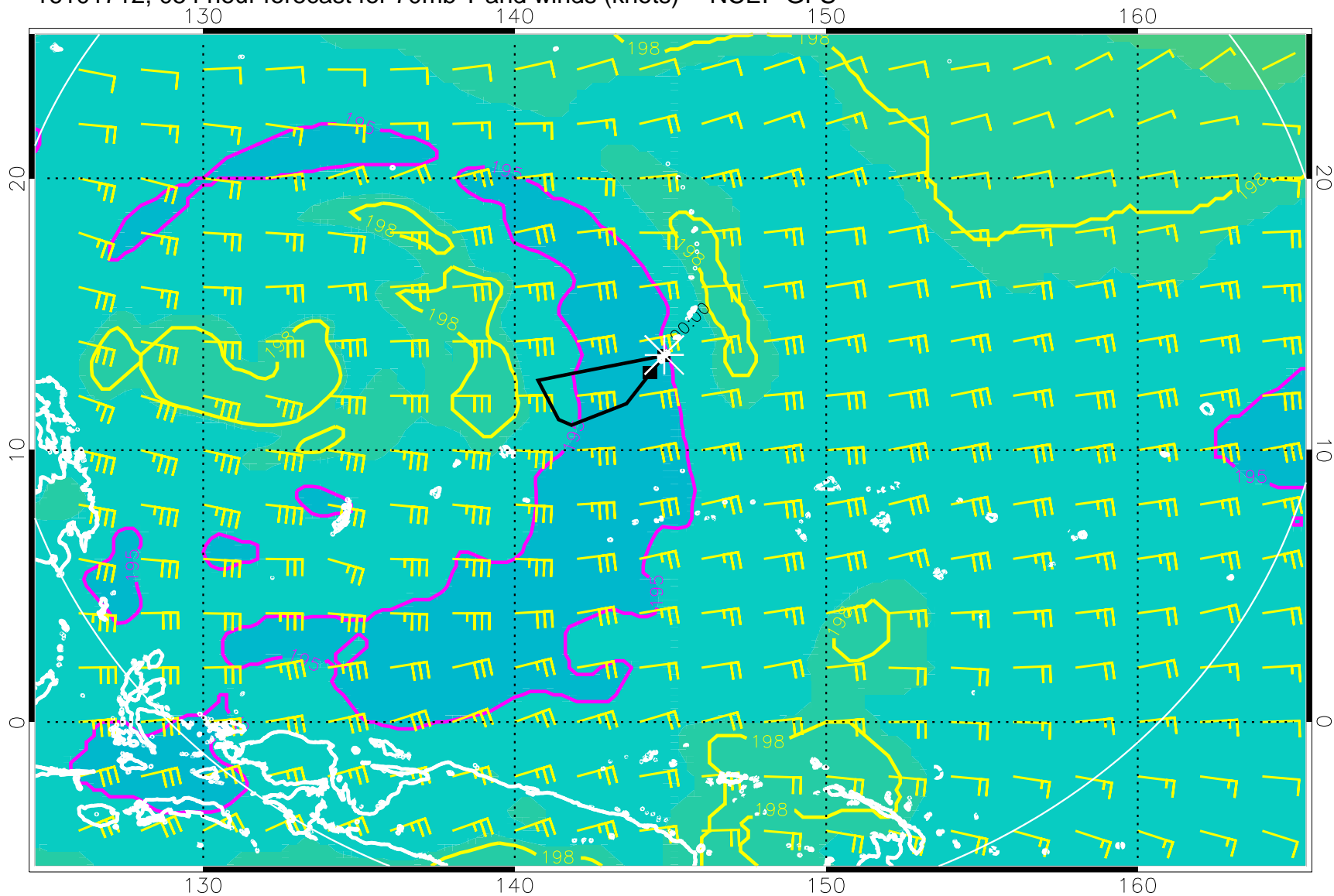
16101712, 054 hour forecast for 70mb T and winds (knots) -- NCEP GFS
