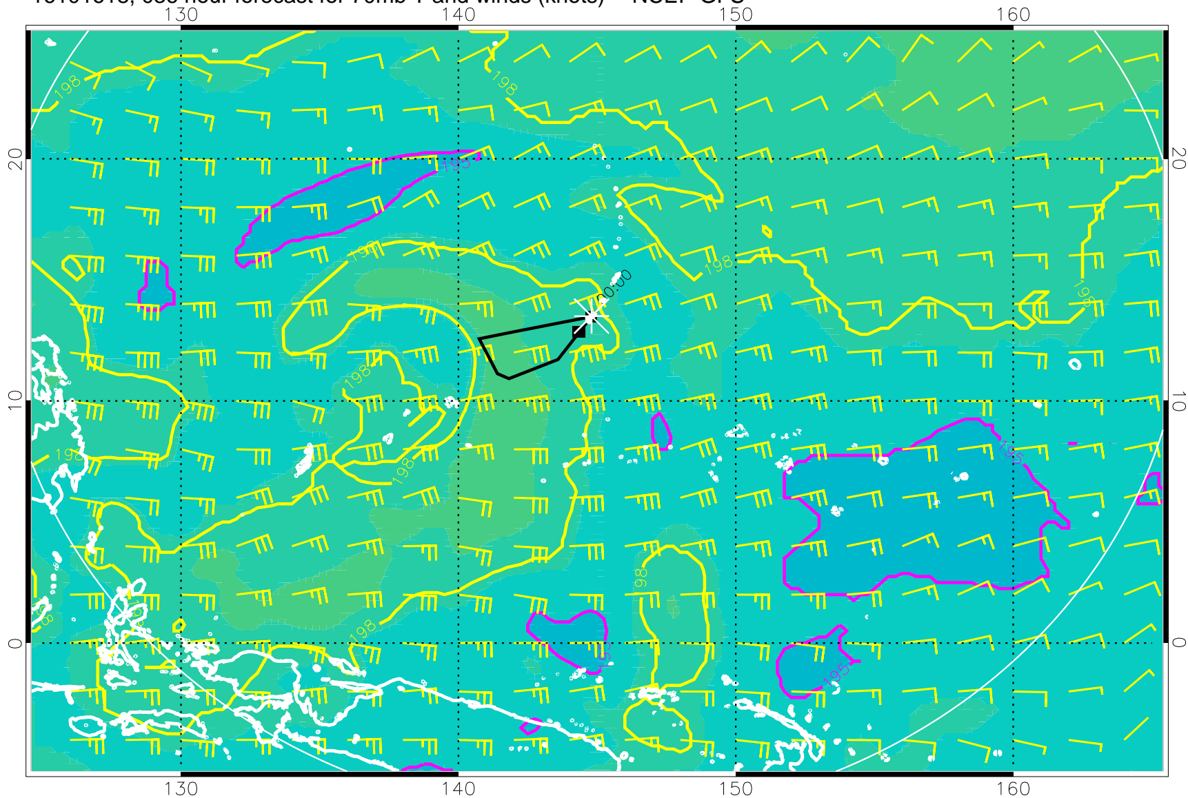
16101618, 036 hour forecast for 70mb T and winds (knots) -- NCEP GFS
