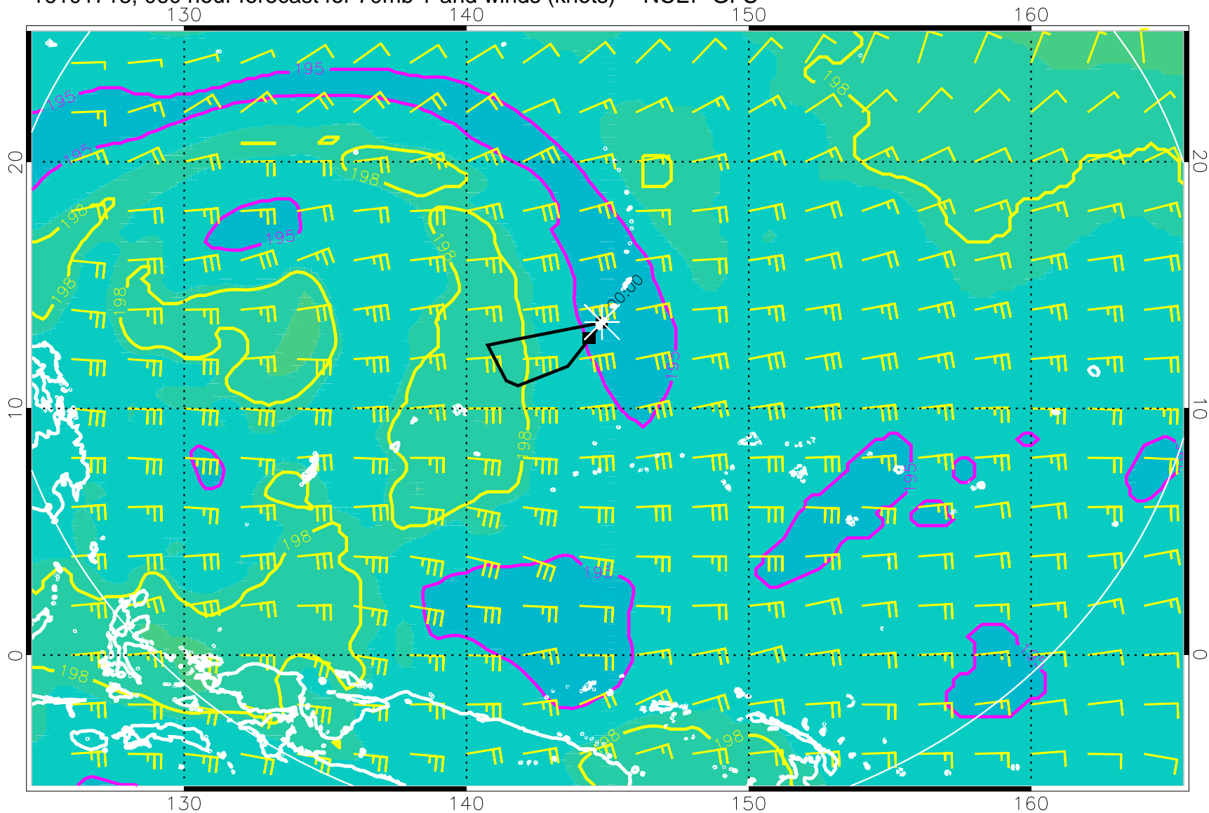
16101718, 060 hour forecast for 70mb T and winds (knots) -- NCEP GFS
