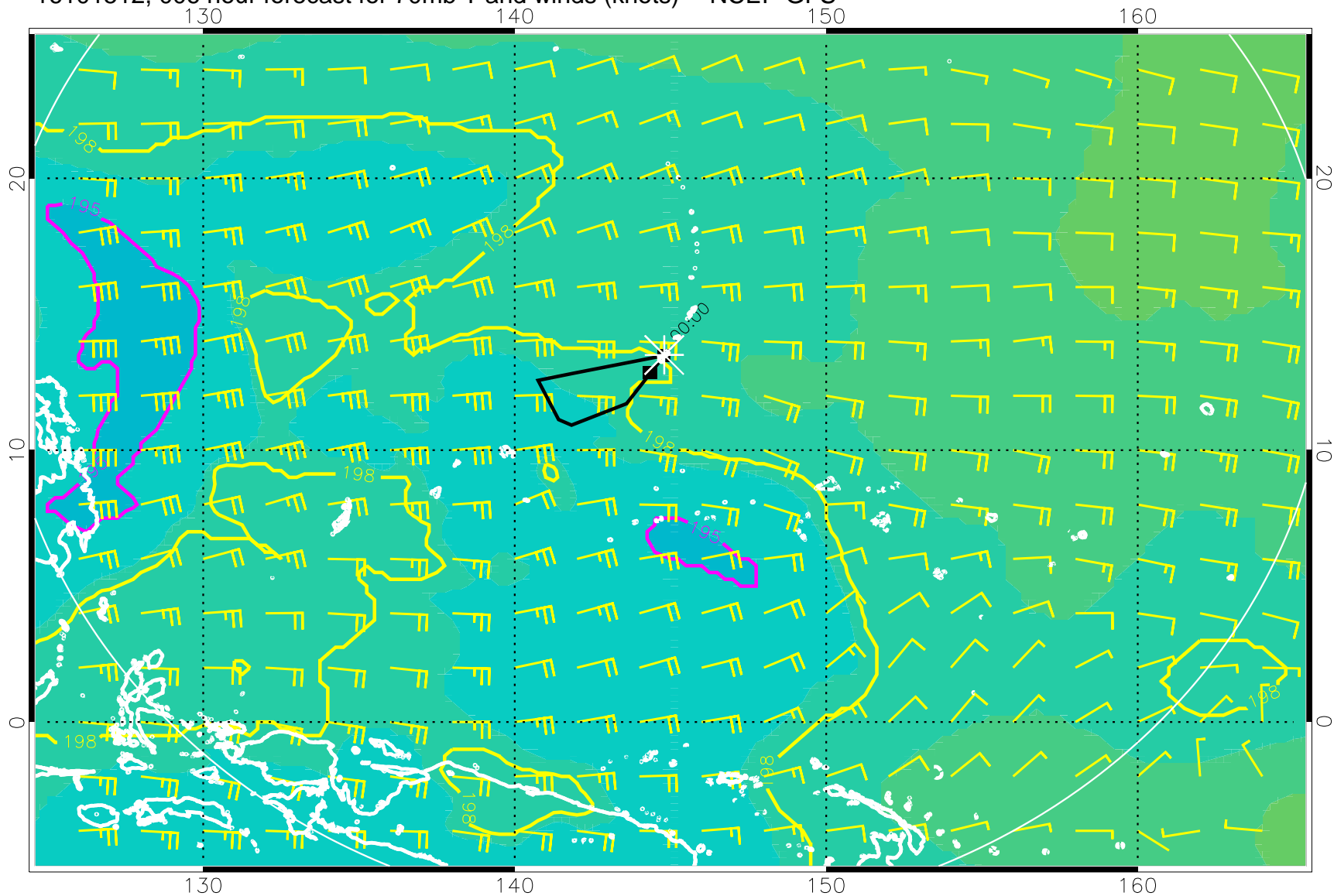
16101512, 006 hour forecast for 70mb T and winds (knots) -- NCEP GFS
