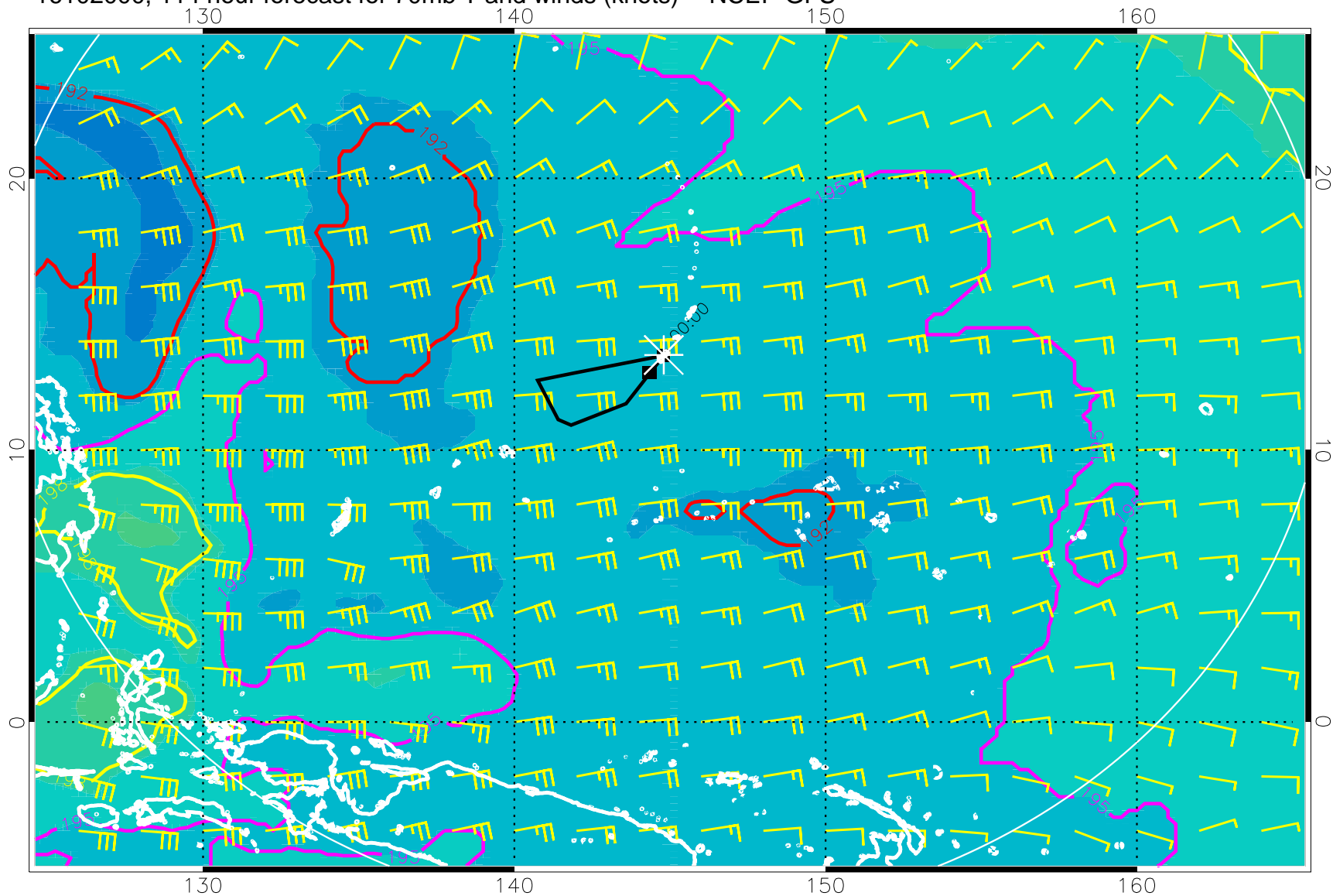
16102000, 114 hour forecast for 70mb T and winds (knots) -- NCEP GFS
