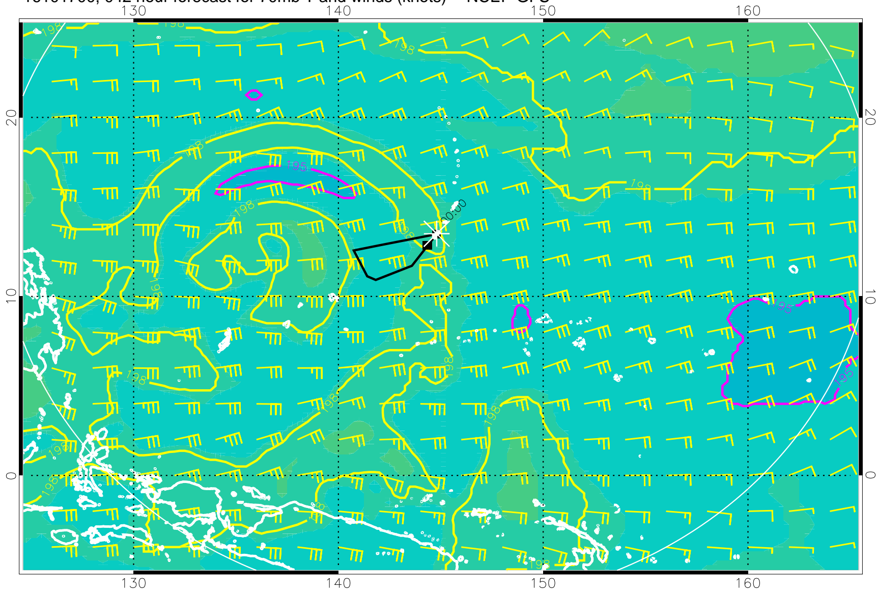
16101700, 042 hour forecast for 70mb T and winds (knots) -- NCEP GFS
