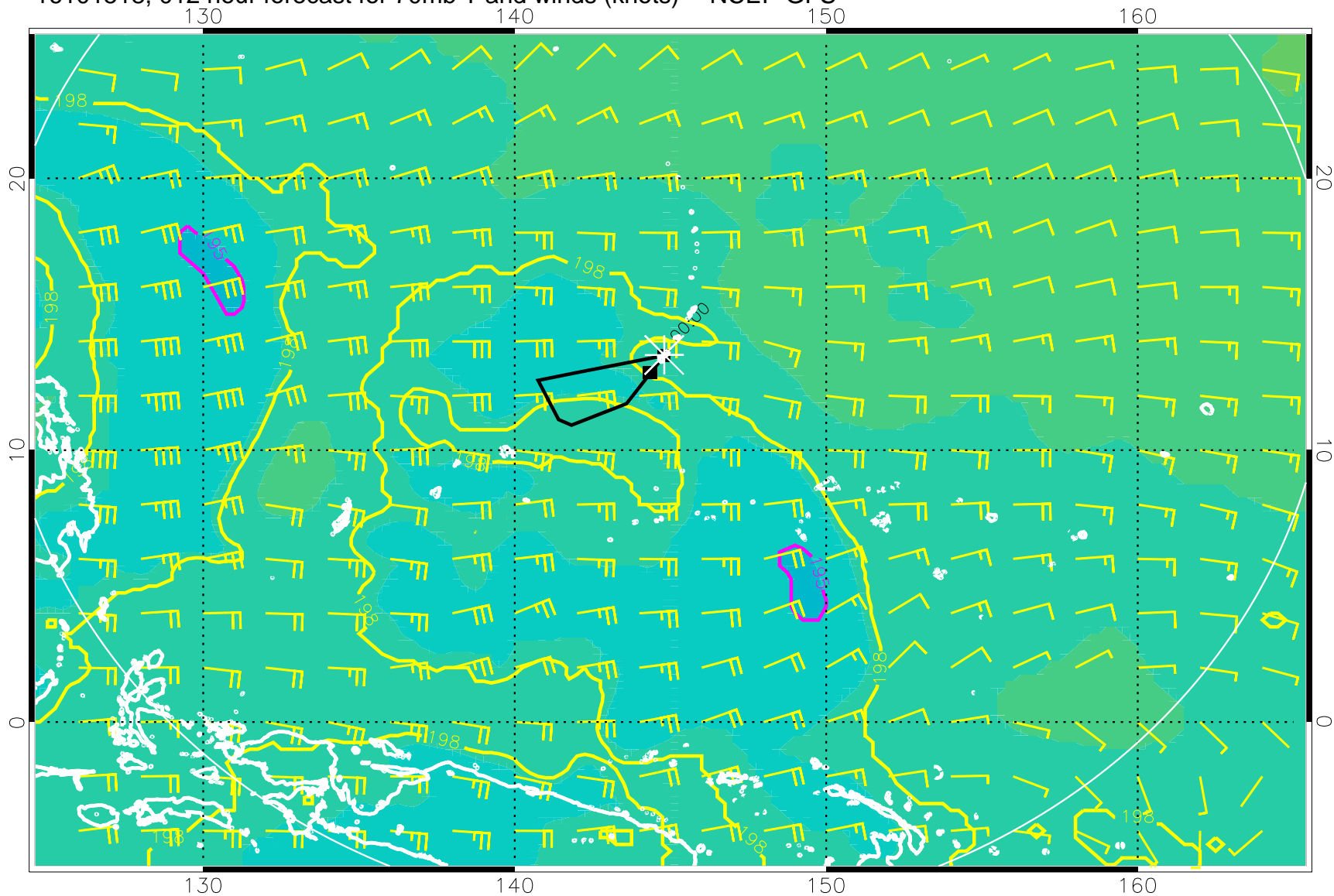
16101518, 012 hour forecast for 70mb T and winds (knots) -- NCEP GFS
