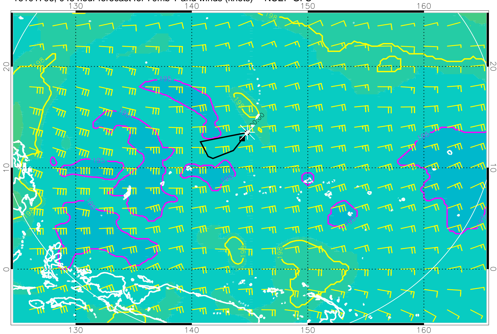
16101706, 048 hour forecast for 70mb T and winds (knots) -- NCEP GFS
