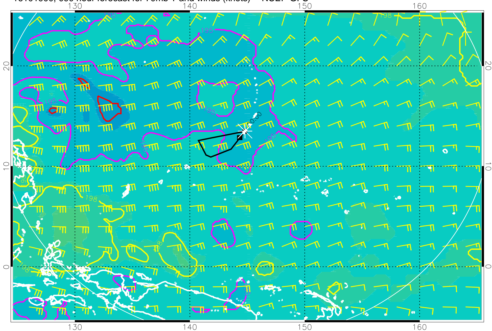
16101900, 090 hour forecast for 70mb T and winds (knots) -- NCEP GFS
