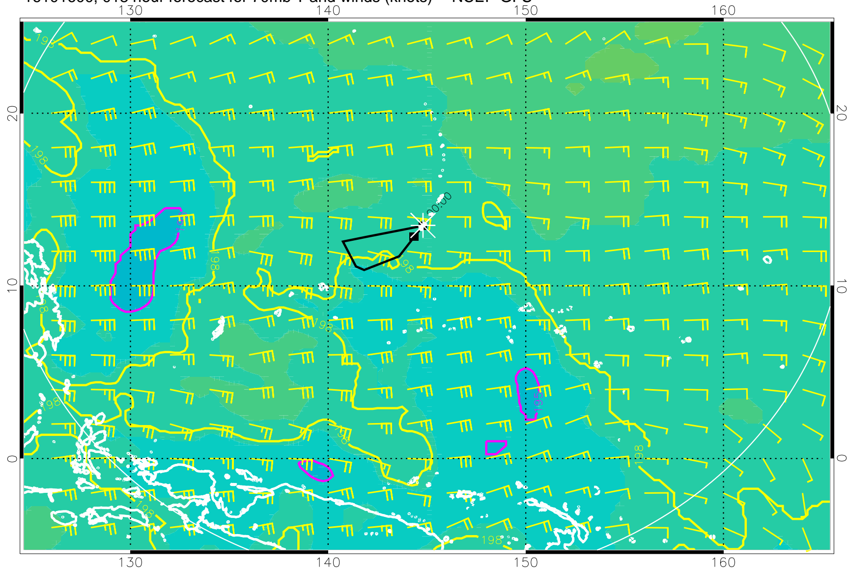
16101600, 018 hour forecast for 70mb T and winds (knots) -- NCEP GFS
