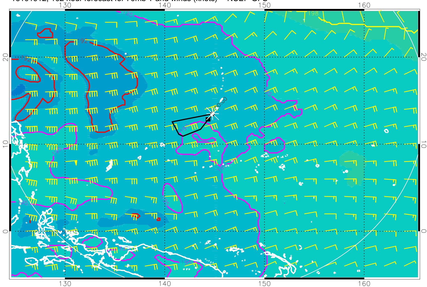
16101912, 102 hour forecast for 70mb T and winds (knots) -- NCEP GFS
