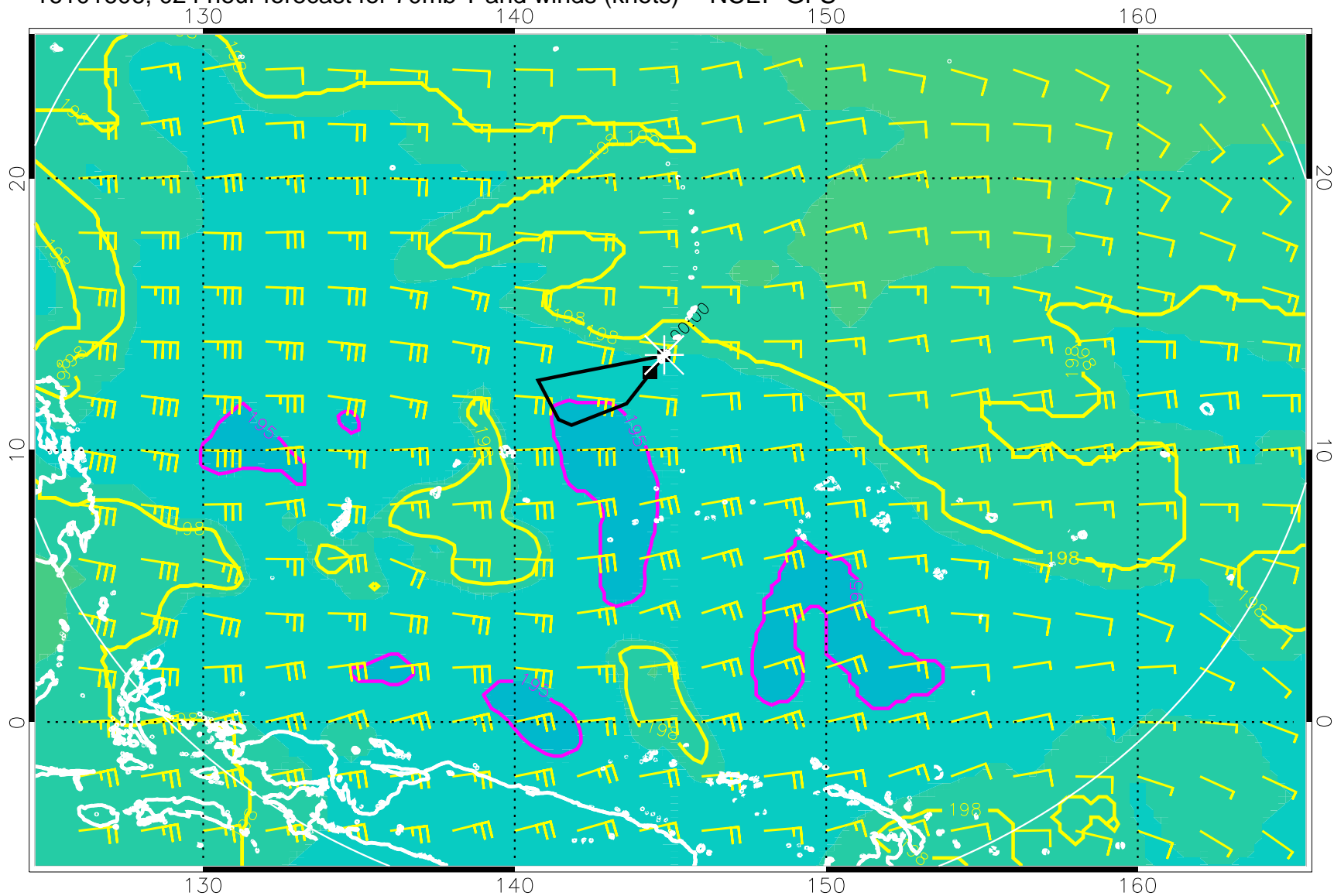
16101606, 024 hour forecast for 70mb T and winds (knots) -- NCEP GFS
