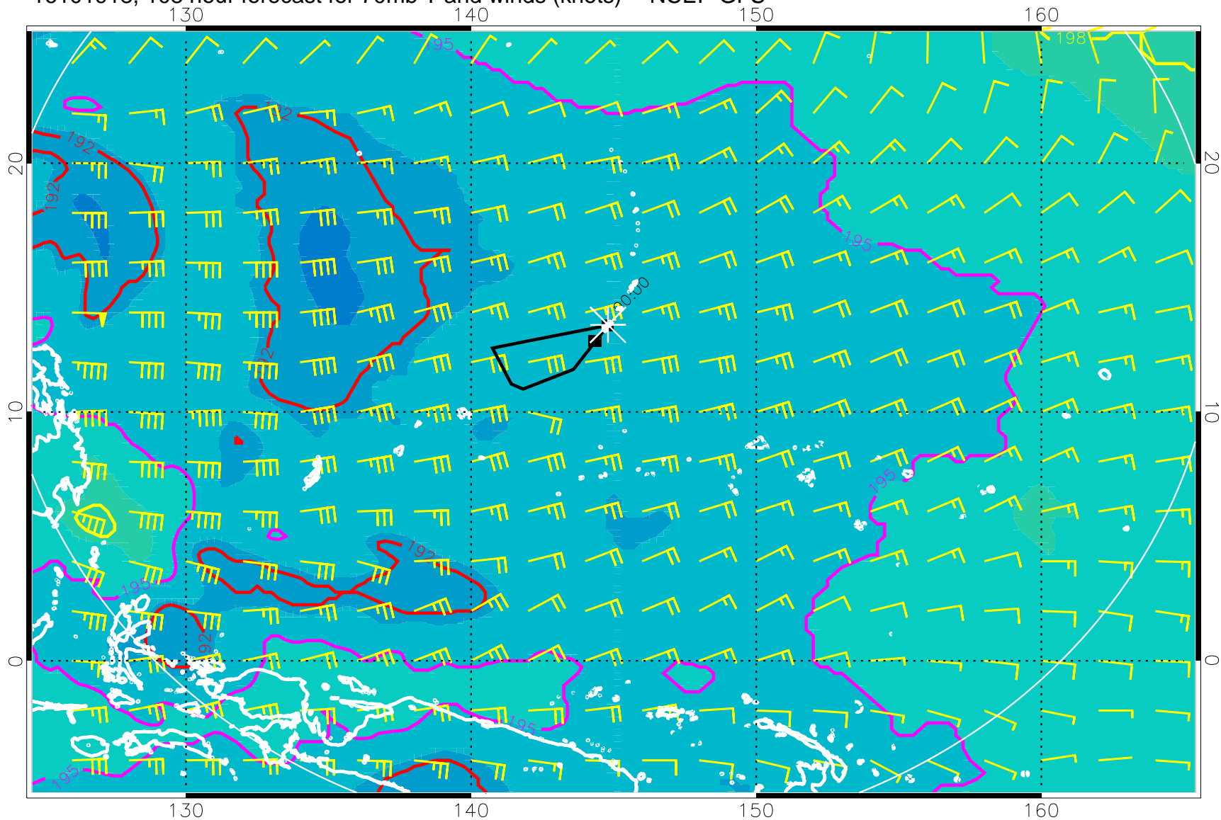
16101918, 108 hour forecast for 70mb T and winds (knots) -- NCEP GFS
