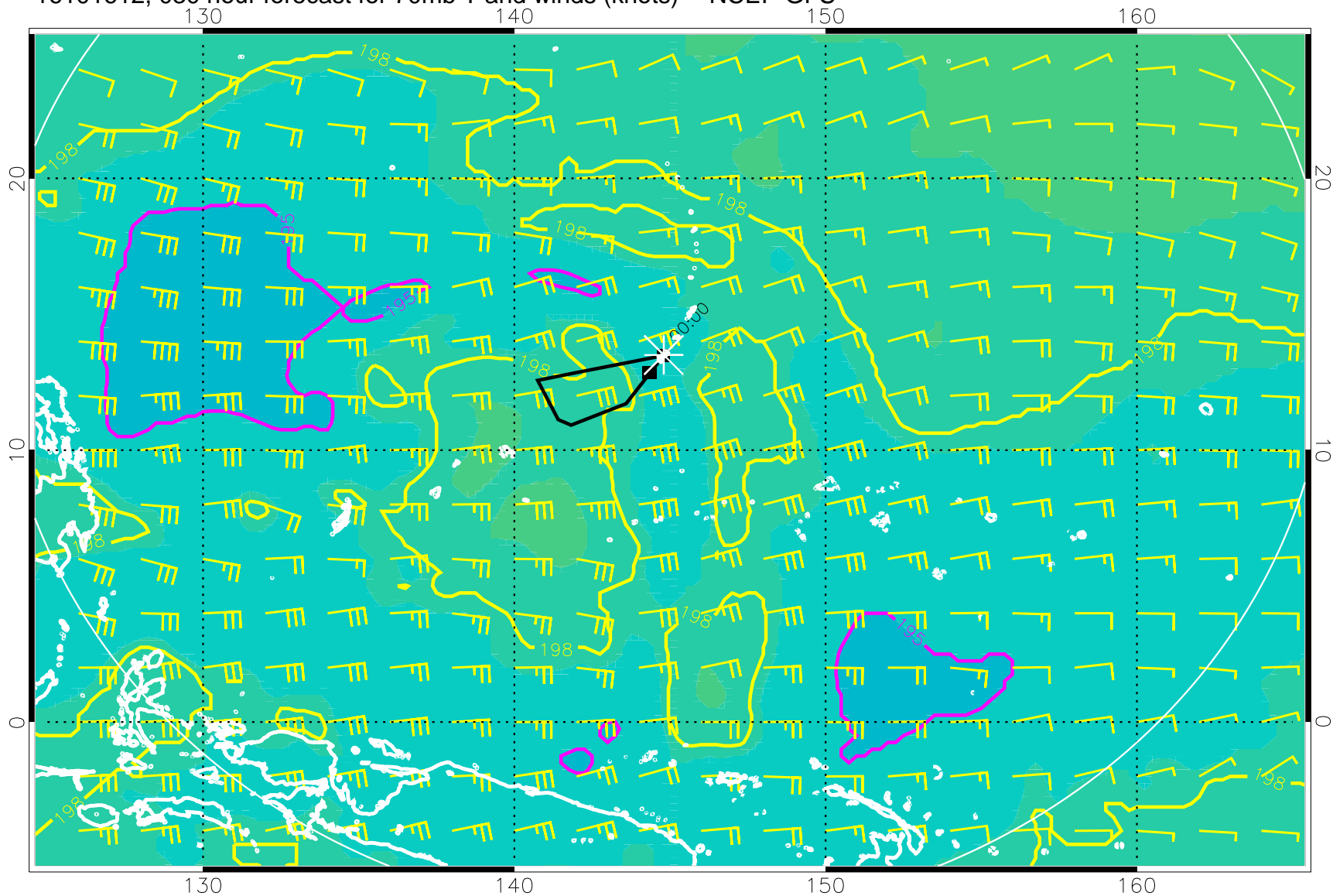
16101612, 0300 hour forecast for 70mb T and winds (knots) -- NCEP GFS
