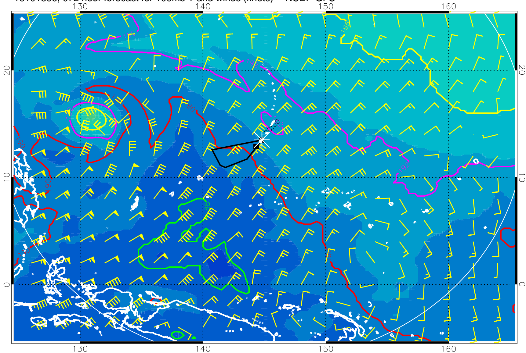
16101806, 072 hour forecast for 100mb T and winds (knots) -- NCEP GFS
