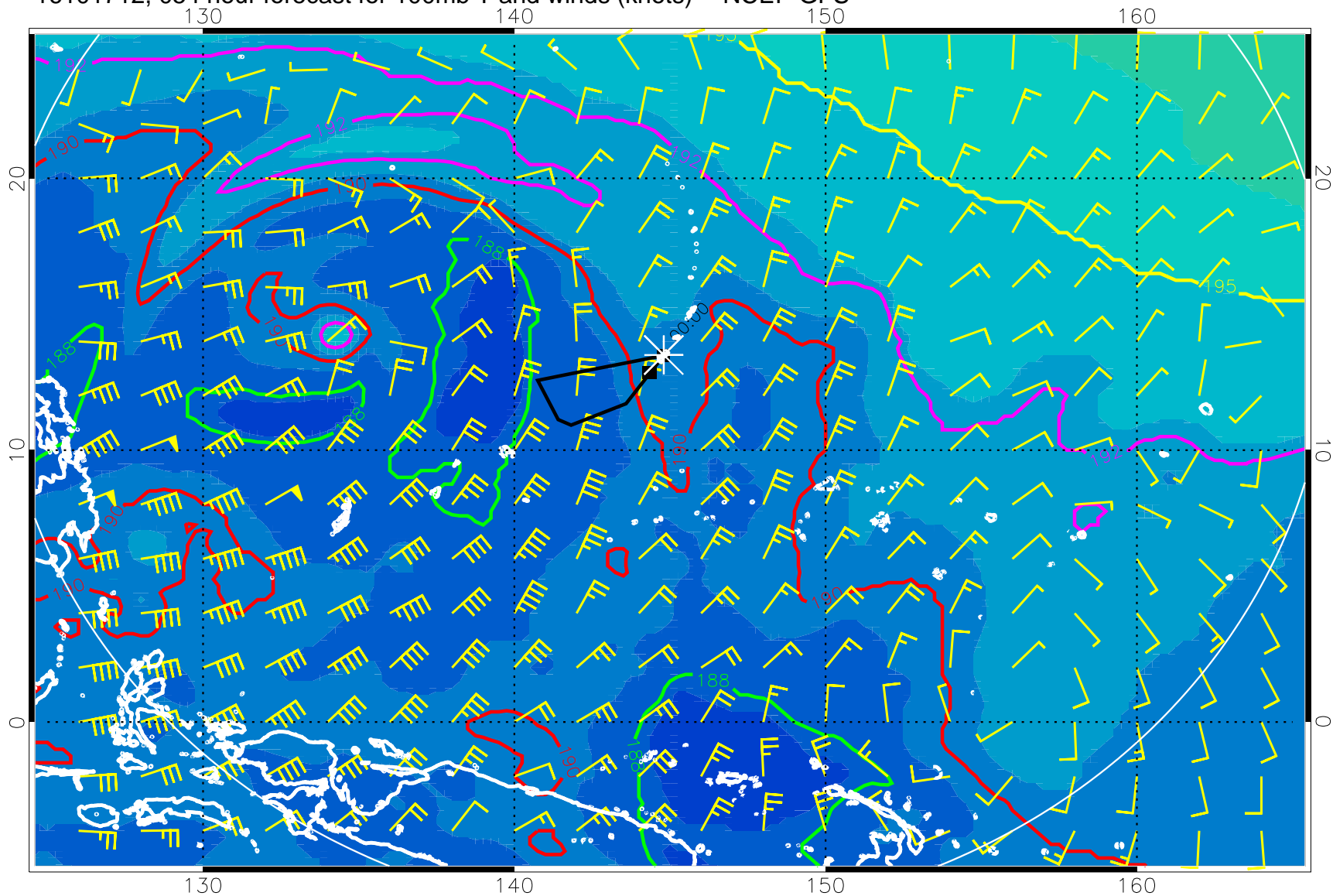
16101712, 054 hour forecast for 100mb T and winds (knots) -- NCEP GFS
