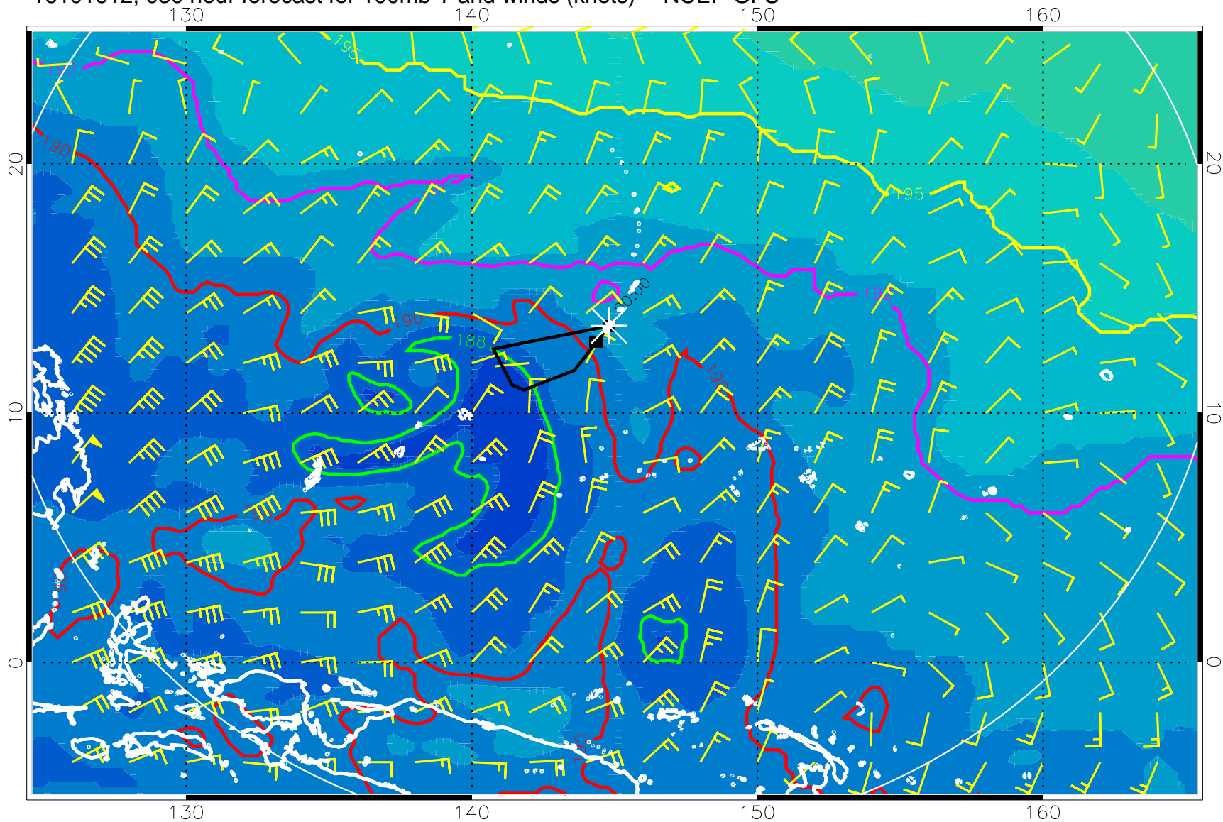
16101612, 0300 hour forecast for 100mb T and winds (knots) -- NCEP GFS
