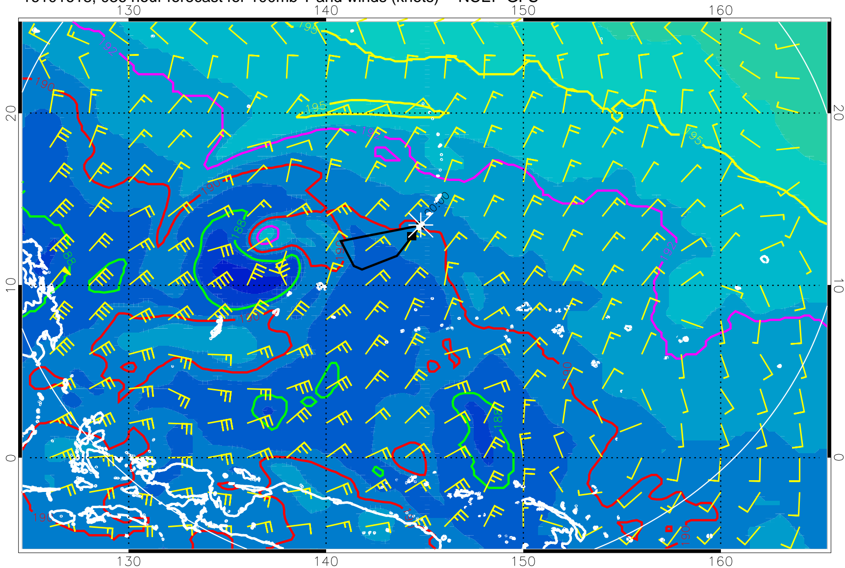
16101618, 036 hour forecast for 100mb T and winds (knots) -- NCEP GFS
