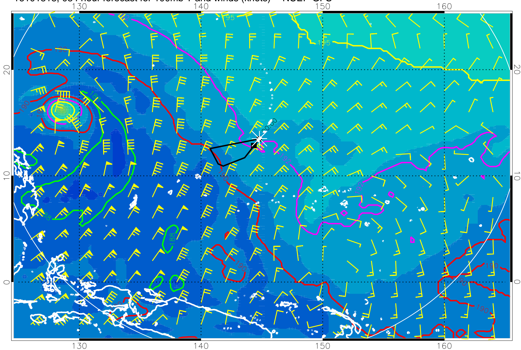
16101818, 084 hour forecast for 100mb T and winds (knots) -- NCEP GFS
