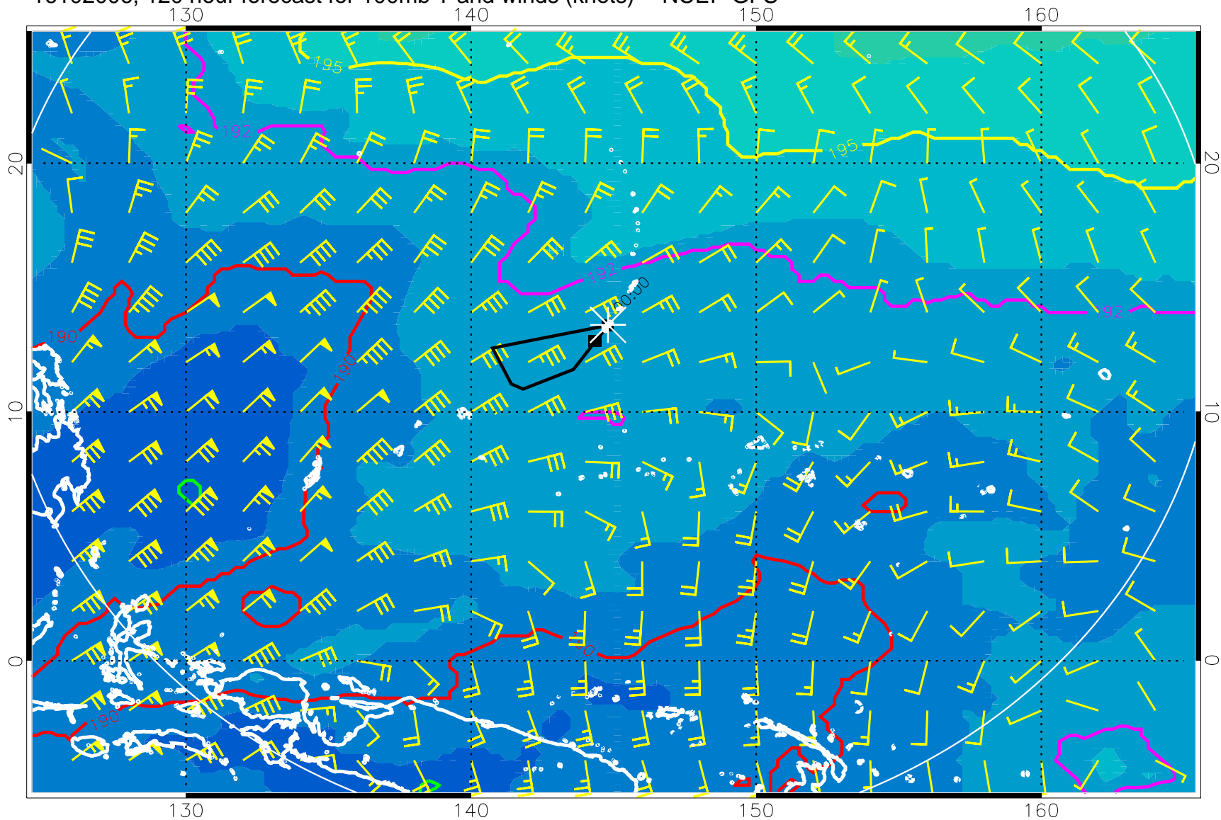
16102006, 120 hour forecast for 100mb T and winds (knots) -- NCEP GFS
