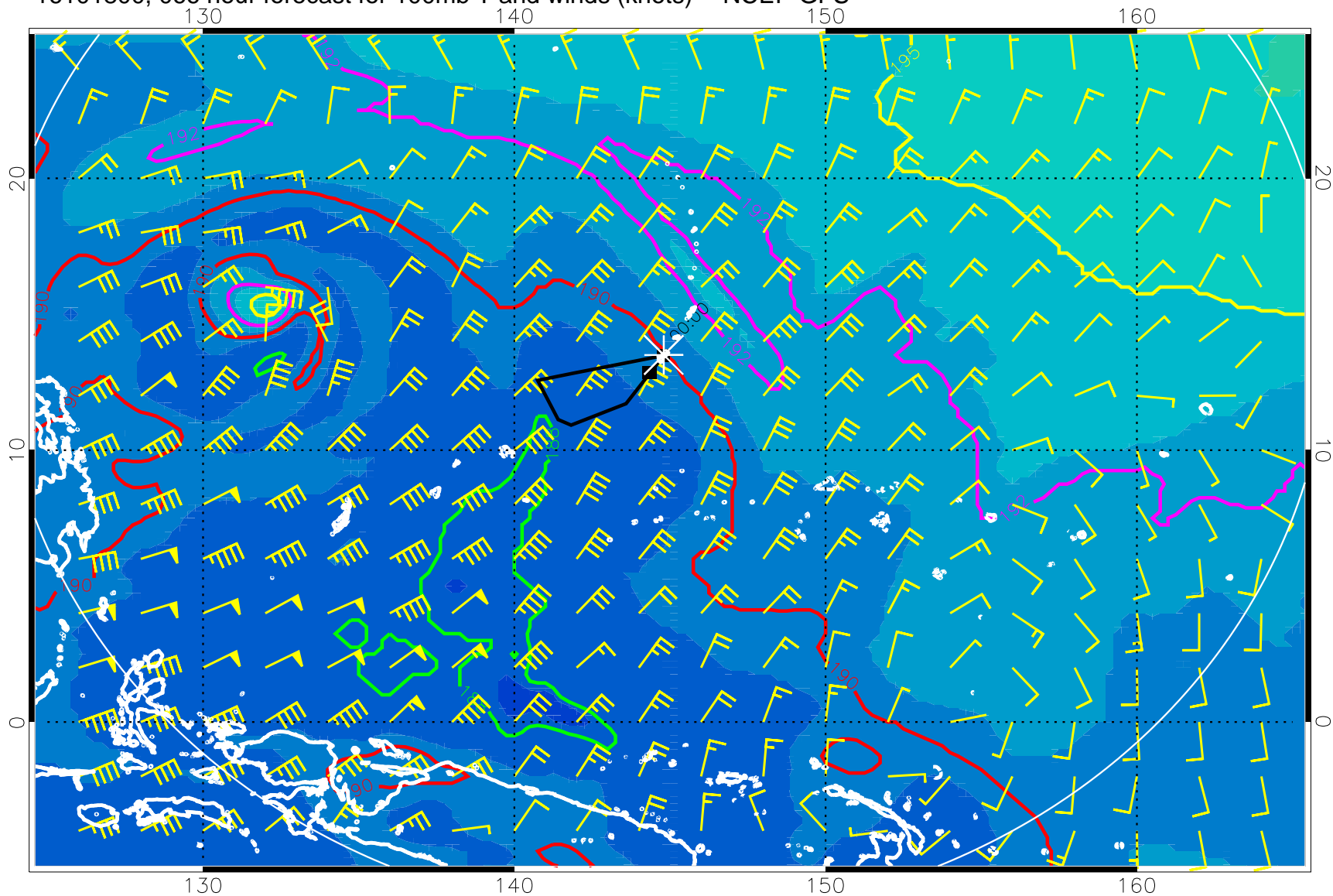
16101800, 066 hour forecast for 100mb T and winds (knots) -- NCEP GFS
