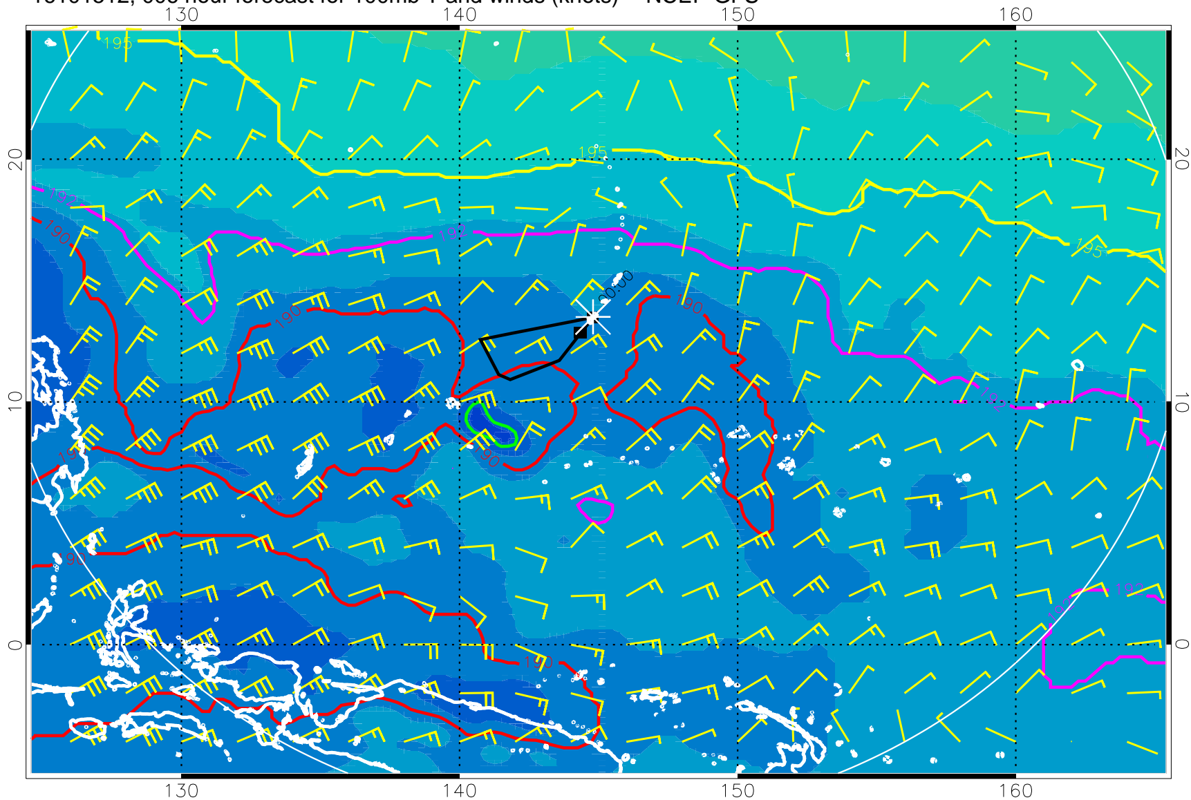
16101512, 006 hour forecast for 100mb T and winds (knots) -- NCEP GFS
