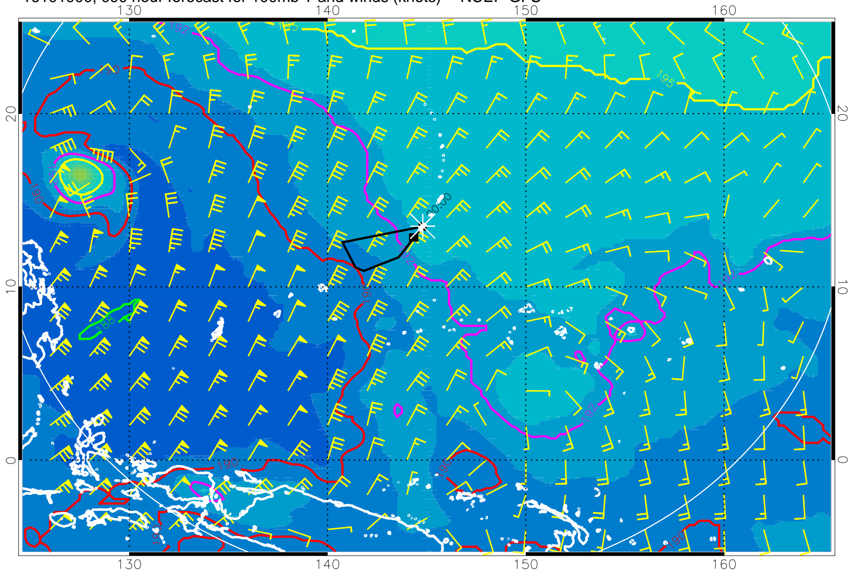
16101900, 090 hour forecast for 100mb T and winds (knots) -- NCEP GFS
