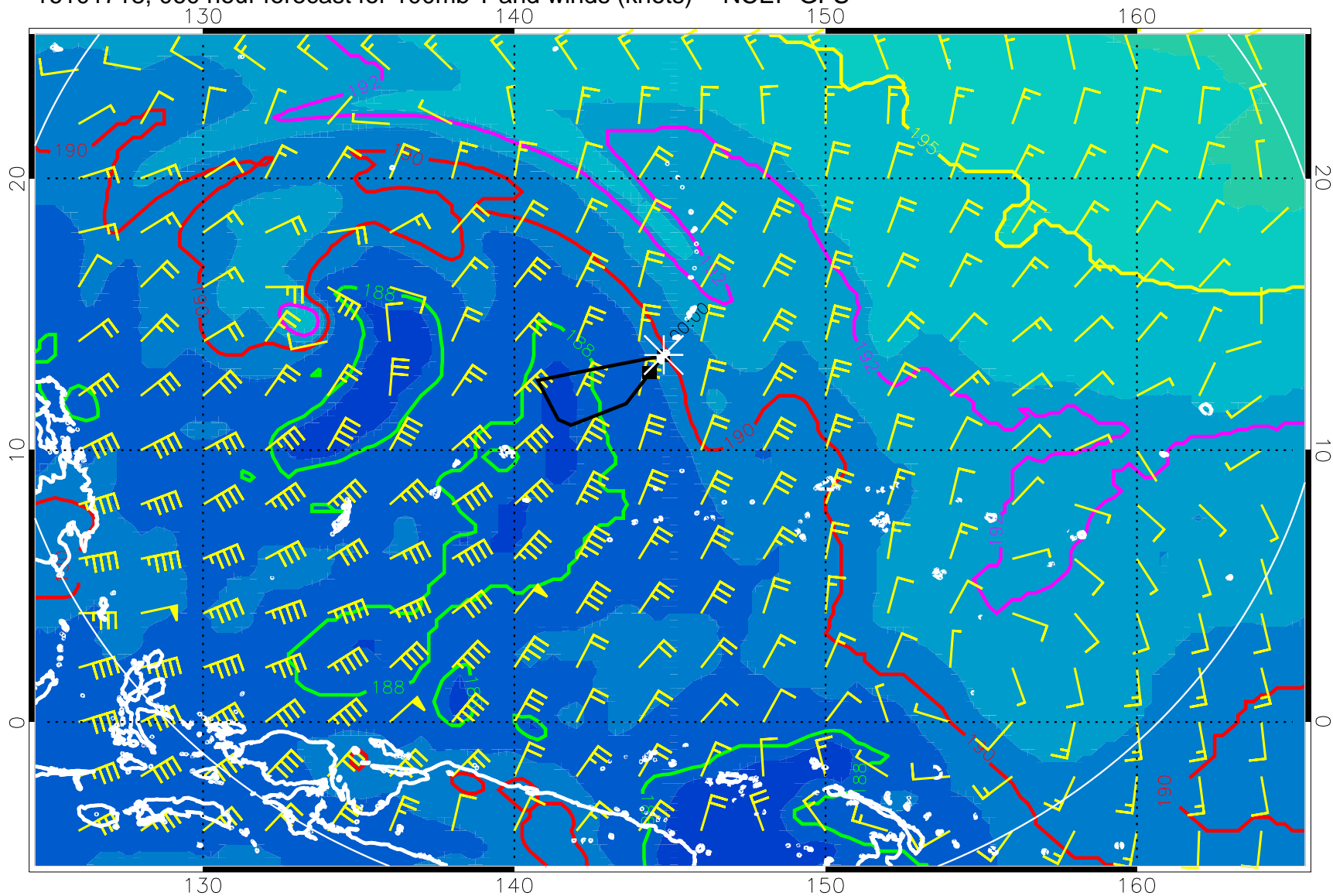
16101718, 060 hour forecast for 100mb T and winds (knots) -- NCEP GFS
