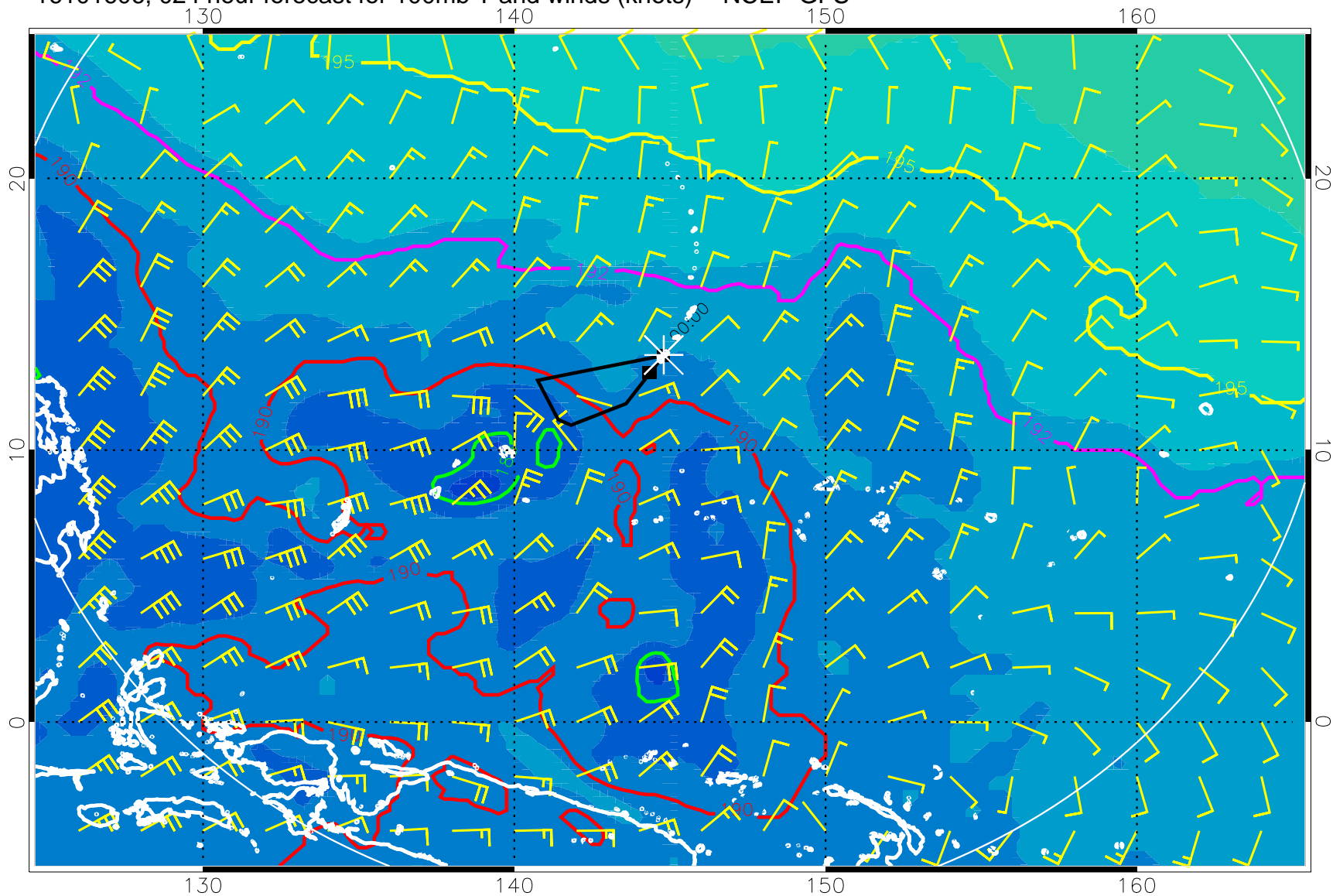
16101606, 024 hour forecast for 100mb T and winds (knots) -- NCEP GFS
