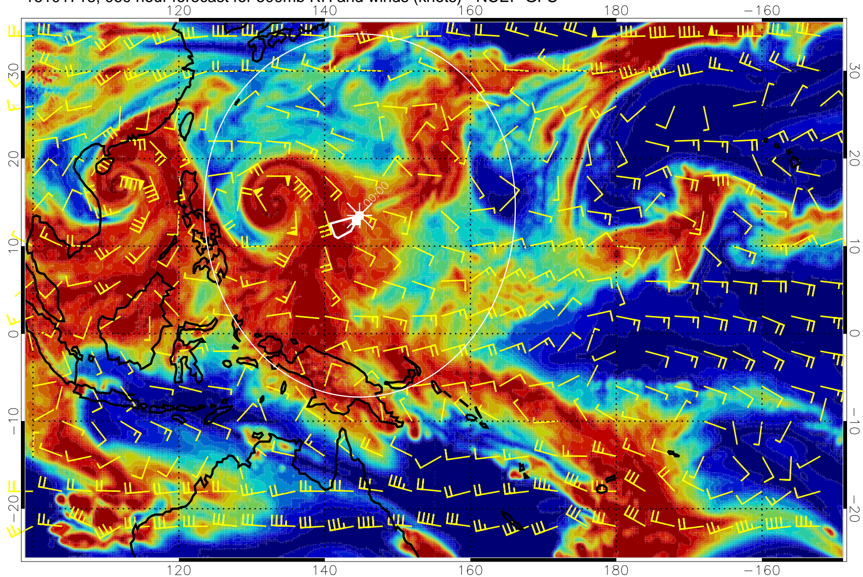
16101718, 060 hour forecast for 500mb RH and winds (knots) - NCEP GFS
