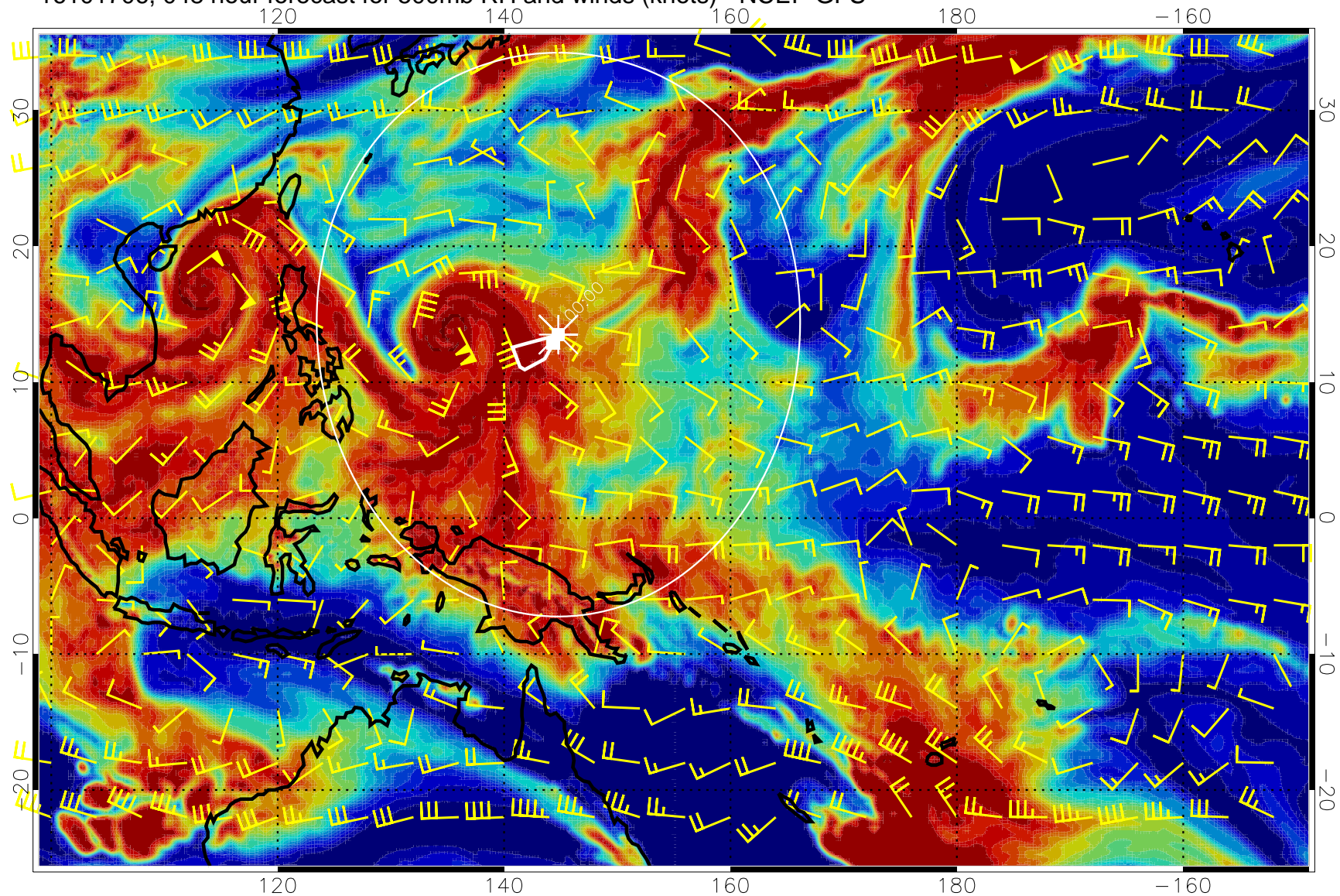
16101706, 048 hour forecast for 500mb RH and winds (knots) - NCEP GFS
