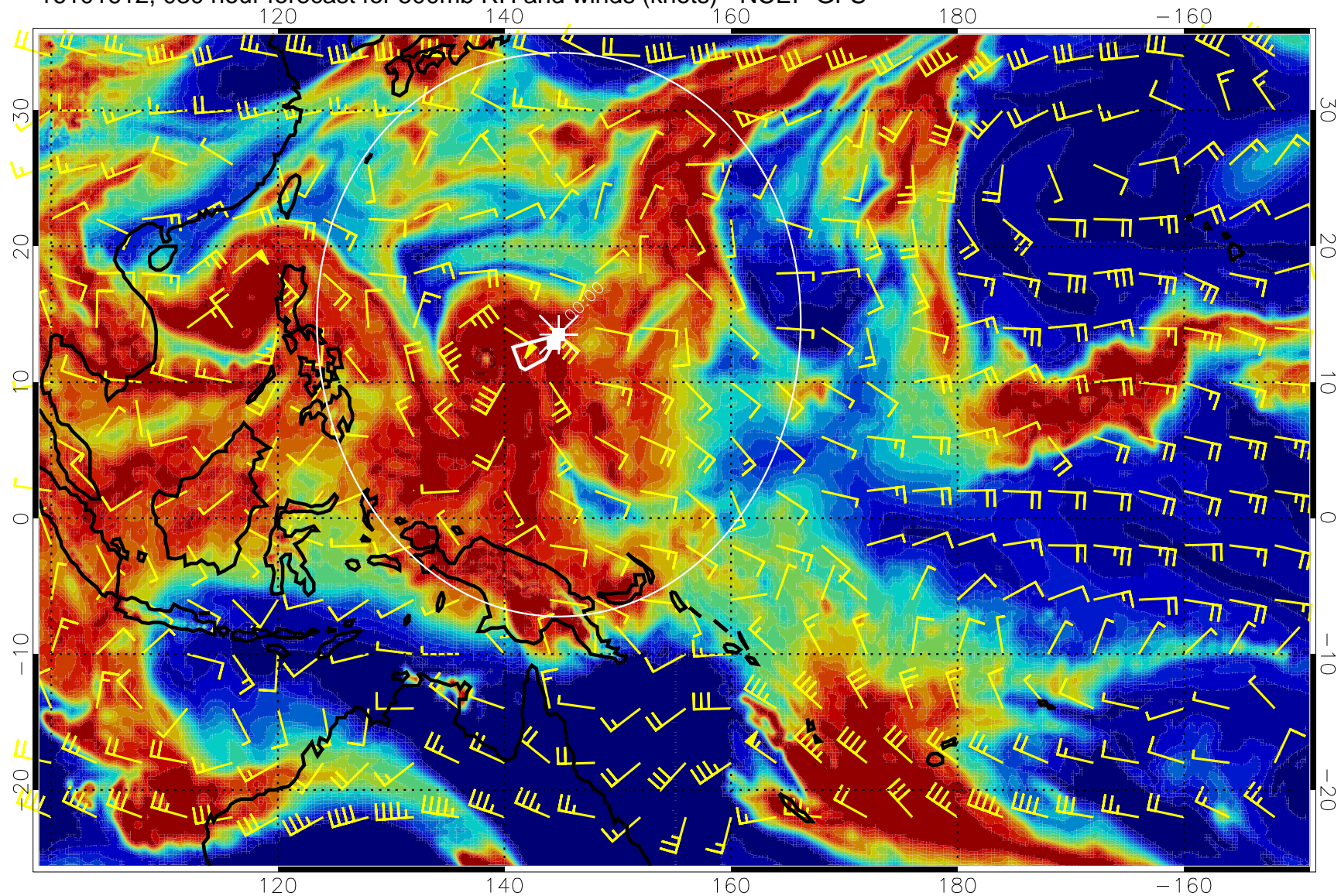
16101612, 030 hour forecast for 500mb RH and winds (knots) - NCEP GFS
