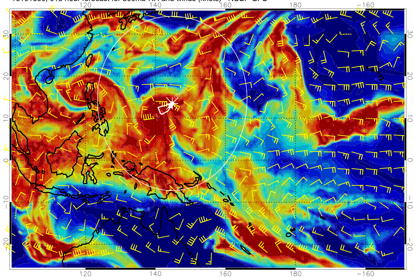
16101600, 018 hour forecast for 500mb RH and winds (knots) - NCEP GFS
