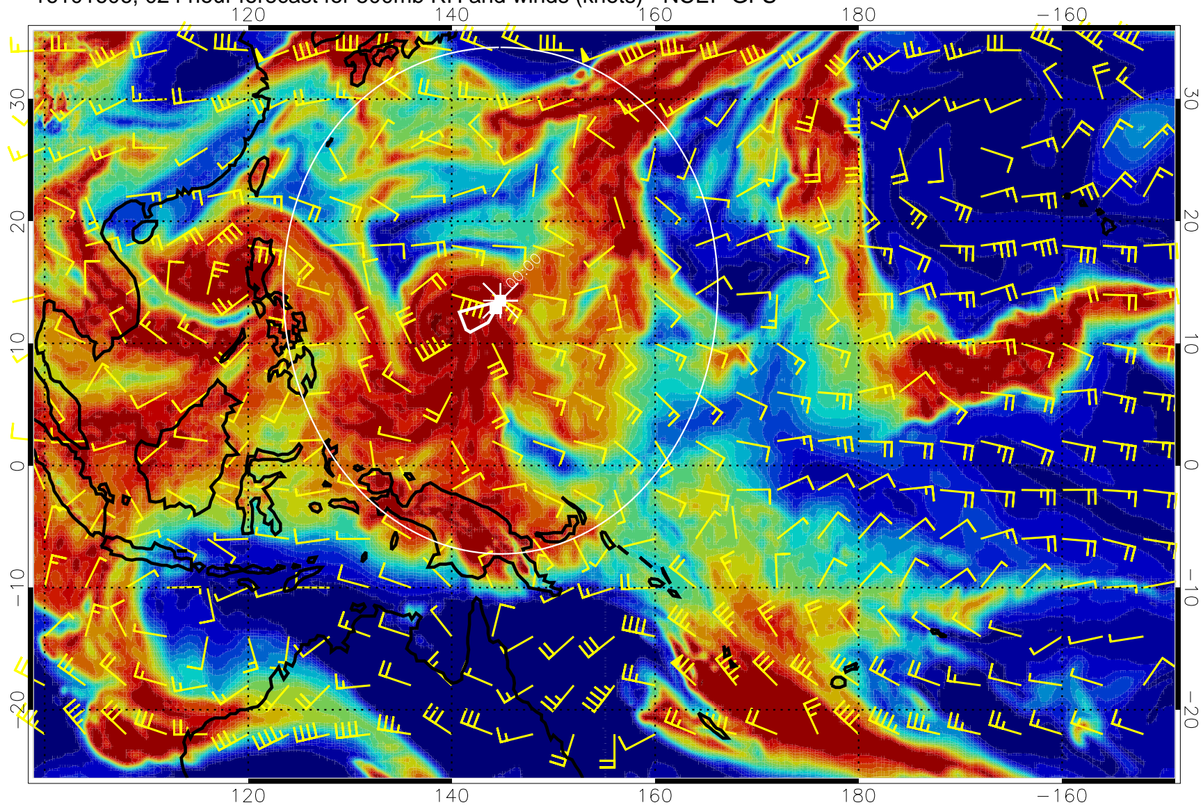
16101606, 024 hour forecast for 500mb RH and winds (knots) - NCEP GFS
