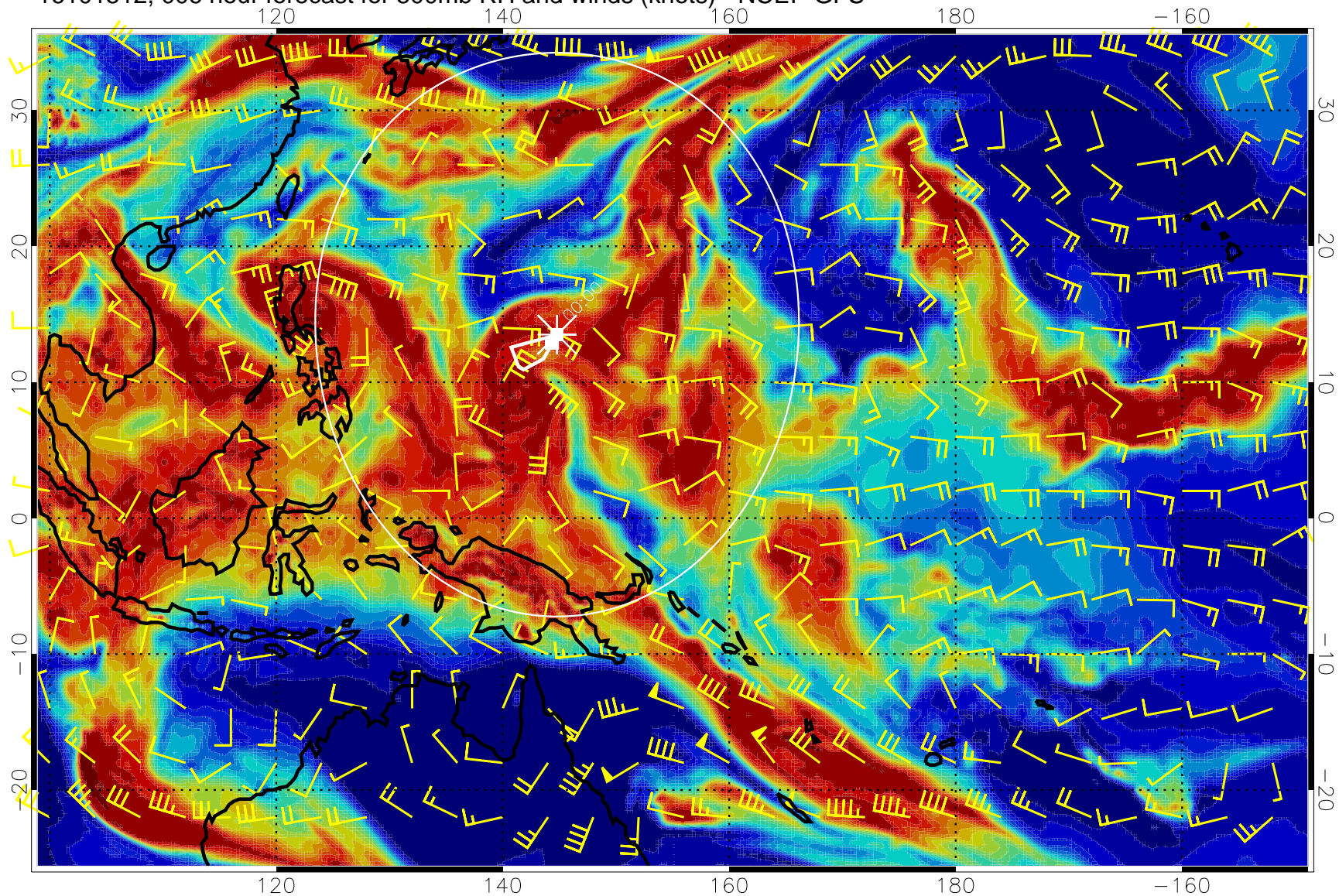
16101512, 006 hour forecast for 500mb RH and winds (knots) - NCEP GFS
