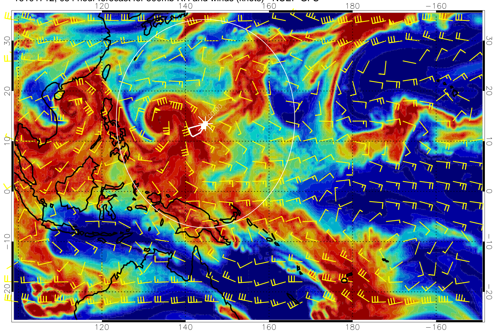
16101712, 054 hour forecast for 500mb RH and winds (knots) - NCEP GFS
