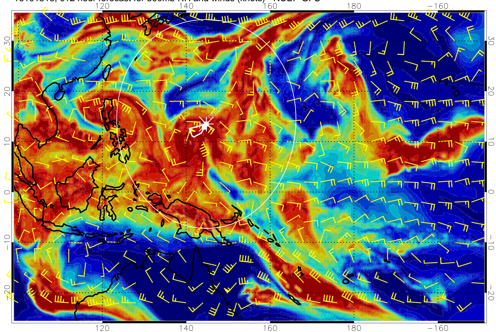
16101518, 012 hour forecast for 500mb RH and winds (knots) - NCEP GFS
