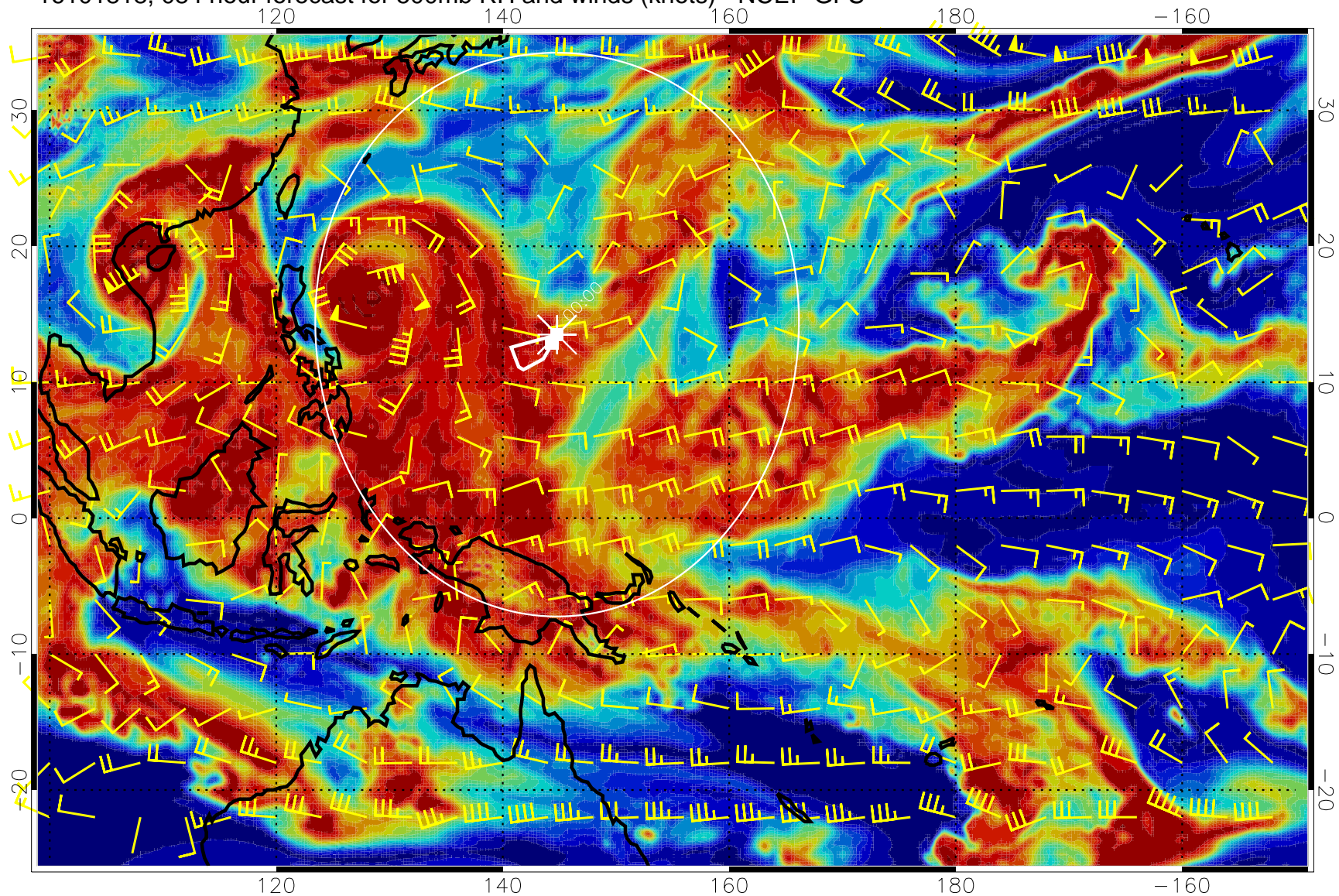
16101818, 084 hour forecast for 500mb RH and winds (knots) - NCEP GFS
