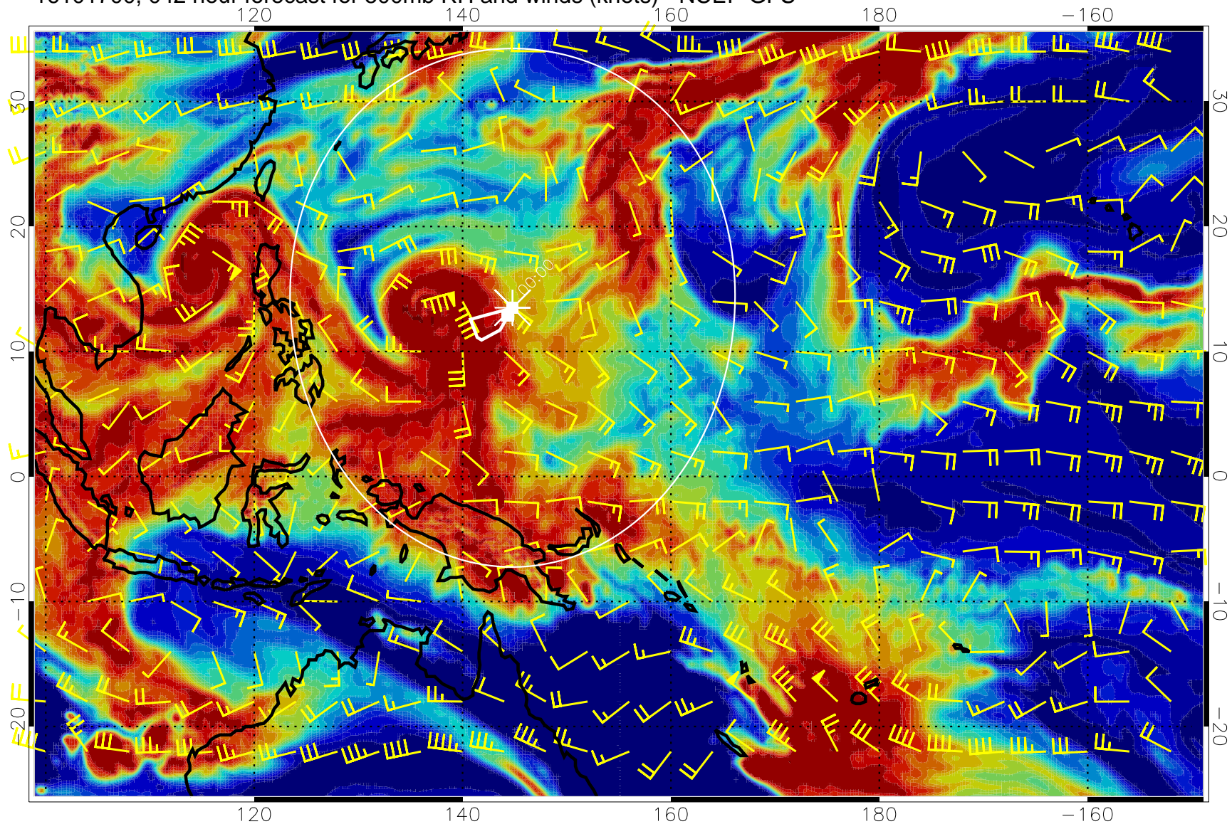
16101700, 042 hour forecast for 500mb RH and winds (knots) - NCEP GFS
