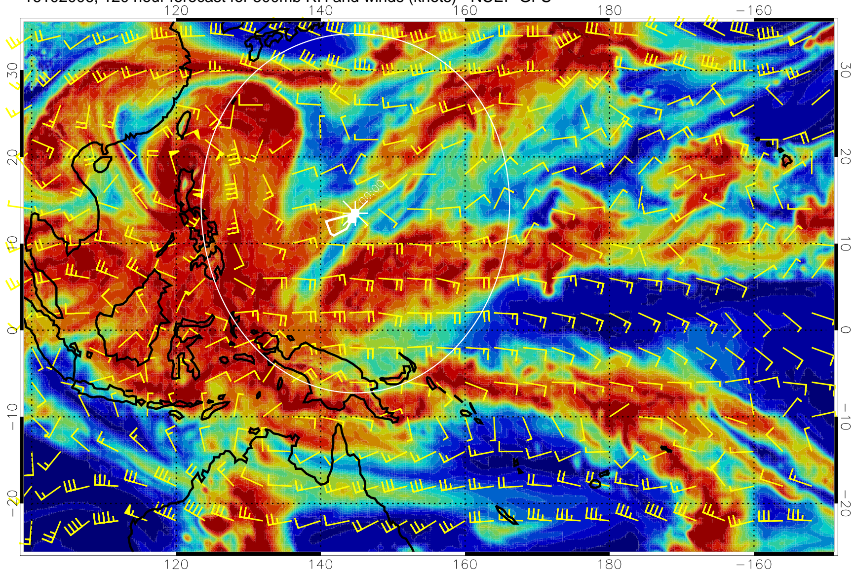
16102006, 120 hour forecast for 500mb RH and winds (knots) - NCEP GFS
