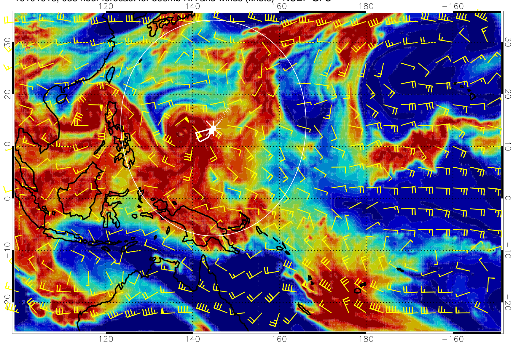
16101618, 036 hour forecast for 500mb RH and winds (knots) - NCEP GFS
