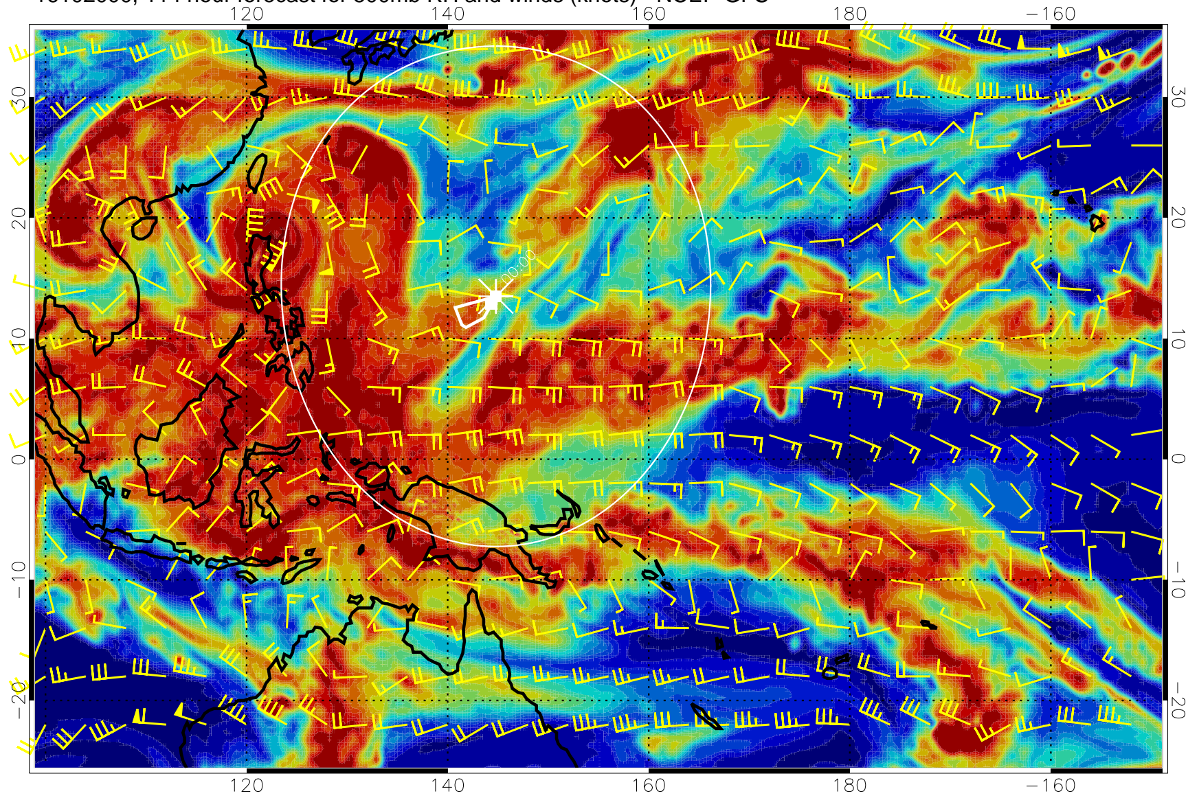
16102000, 114 hour forecast for 500mb RH and winds (knots) - NCEP GFS
