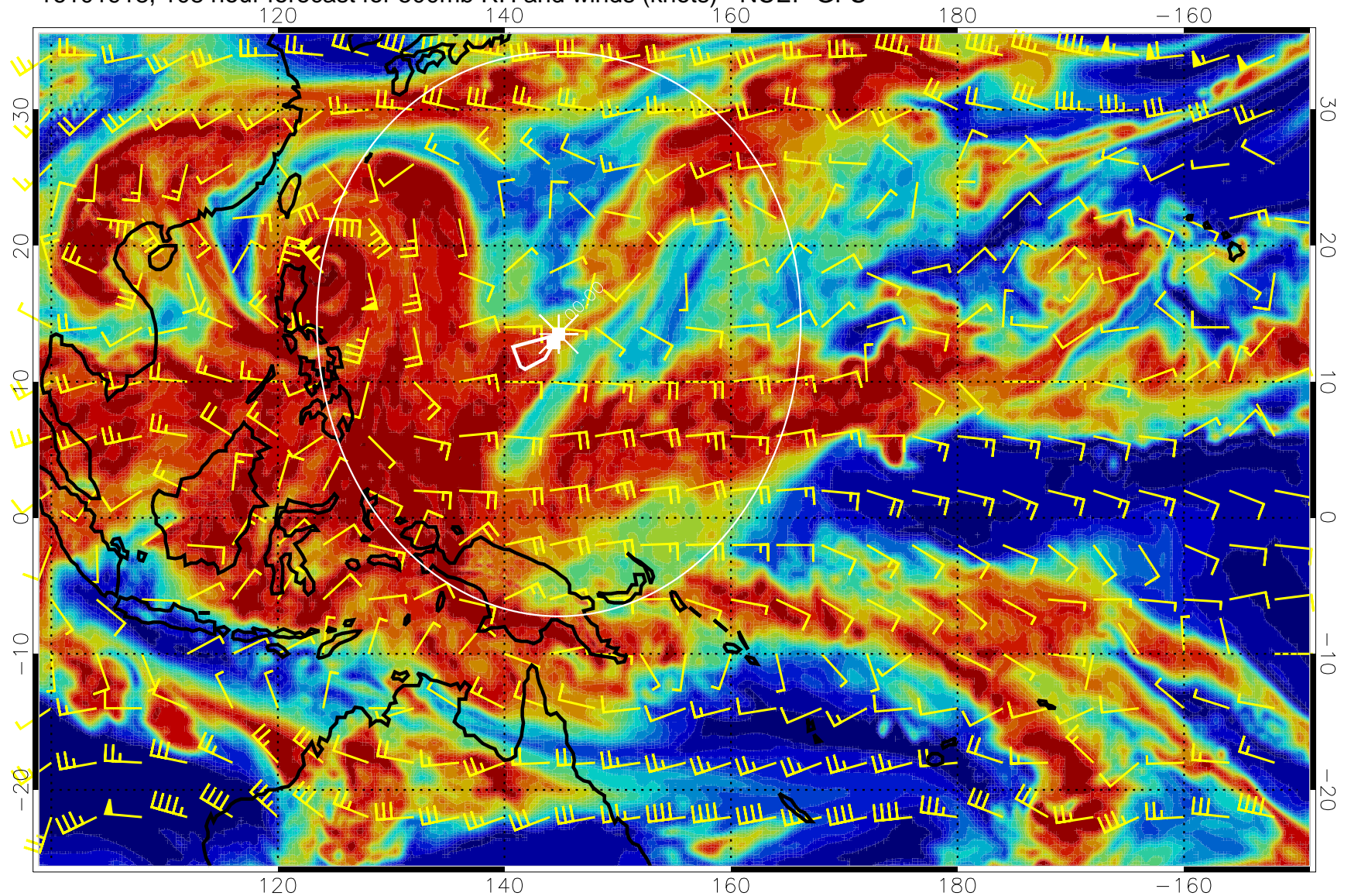
16101918, 108 hour forecast for 500mb RH and winds (knots) - NCEP GFS
