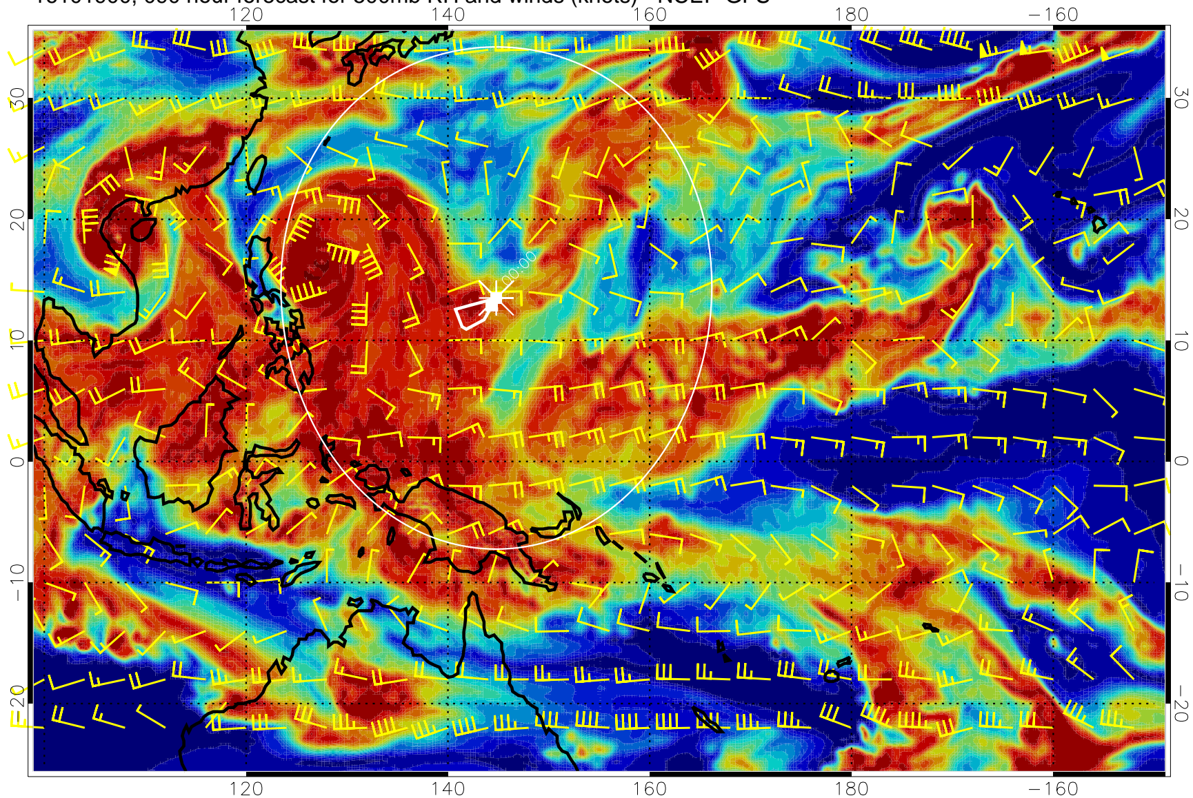
16101900, 090 hour forecast for 500mb RH and winds (knots) - NCEP GFS
