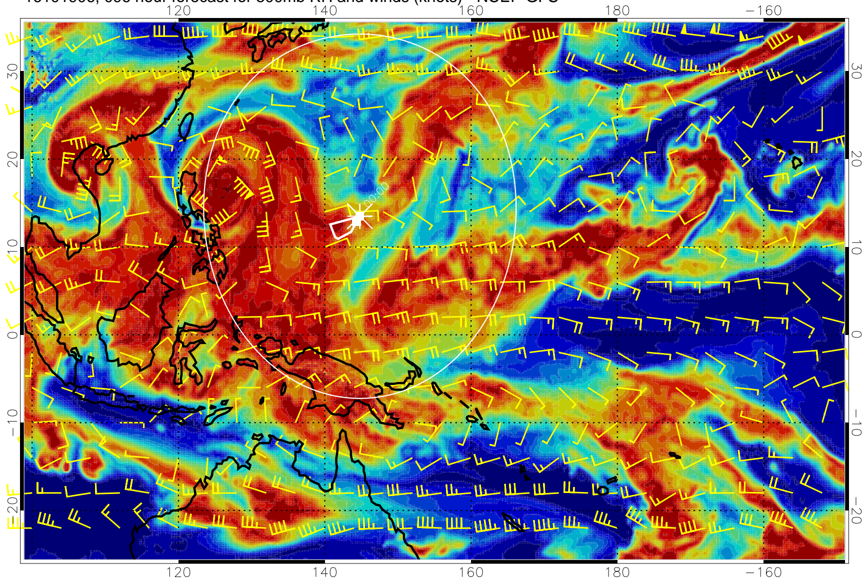
16101906, 096 hour forecast for 500mb RH and winds (knots) - NCEP GFS
