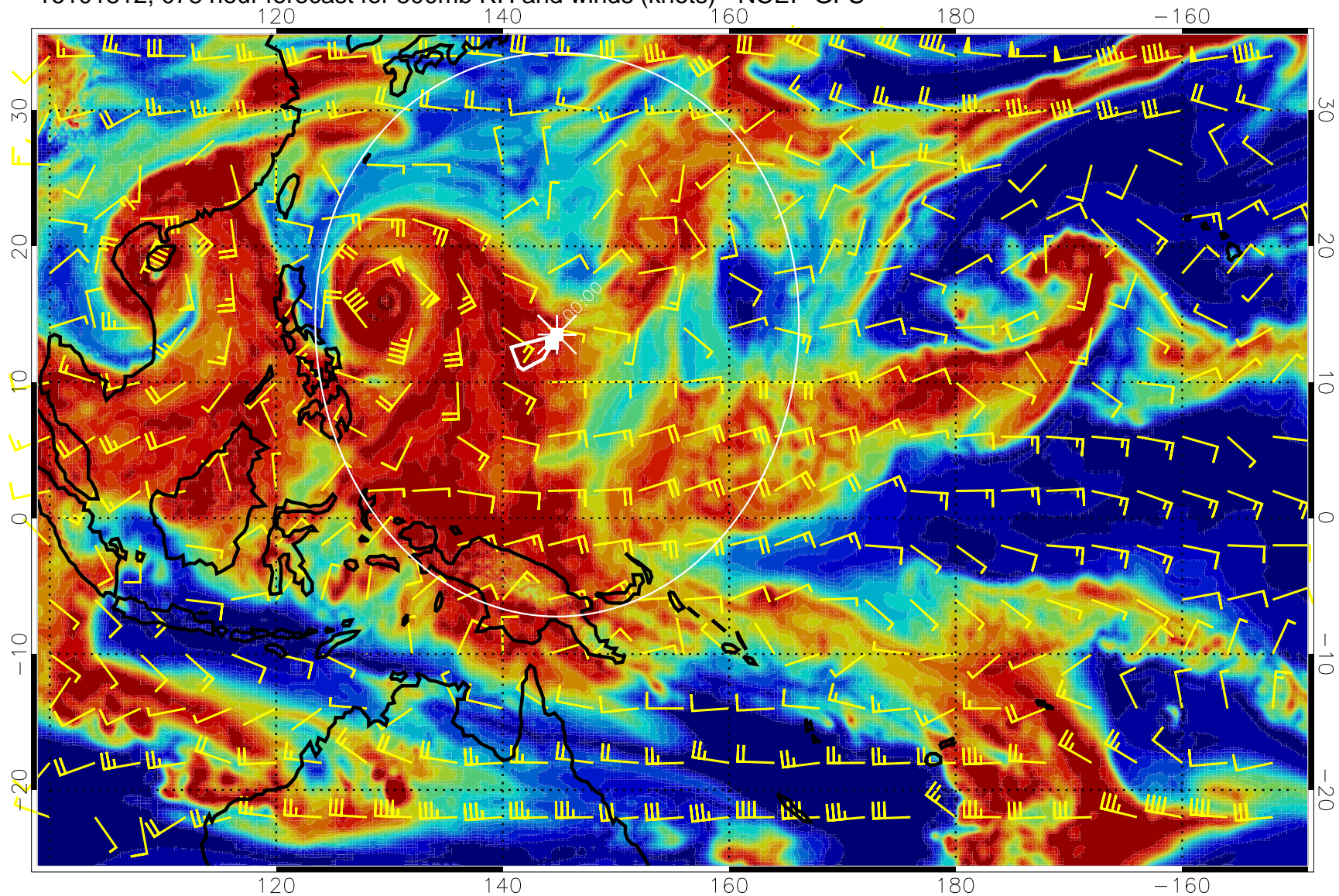
16101812, 078 hour forecast for 500mb RH and winds (knots) - NCEP GFS
