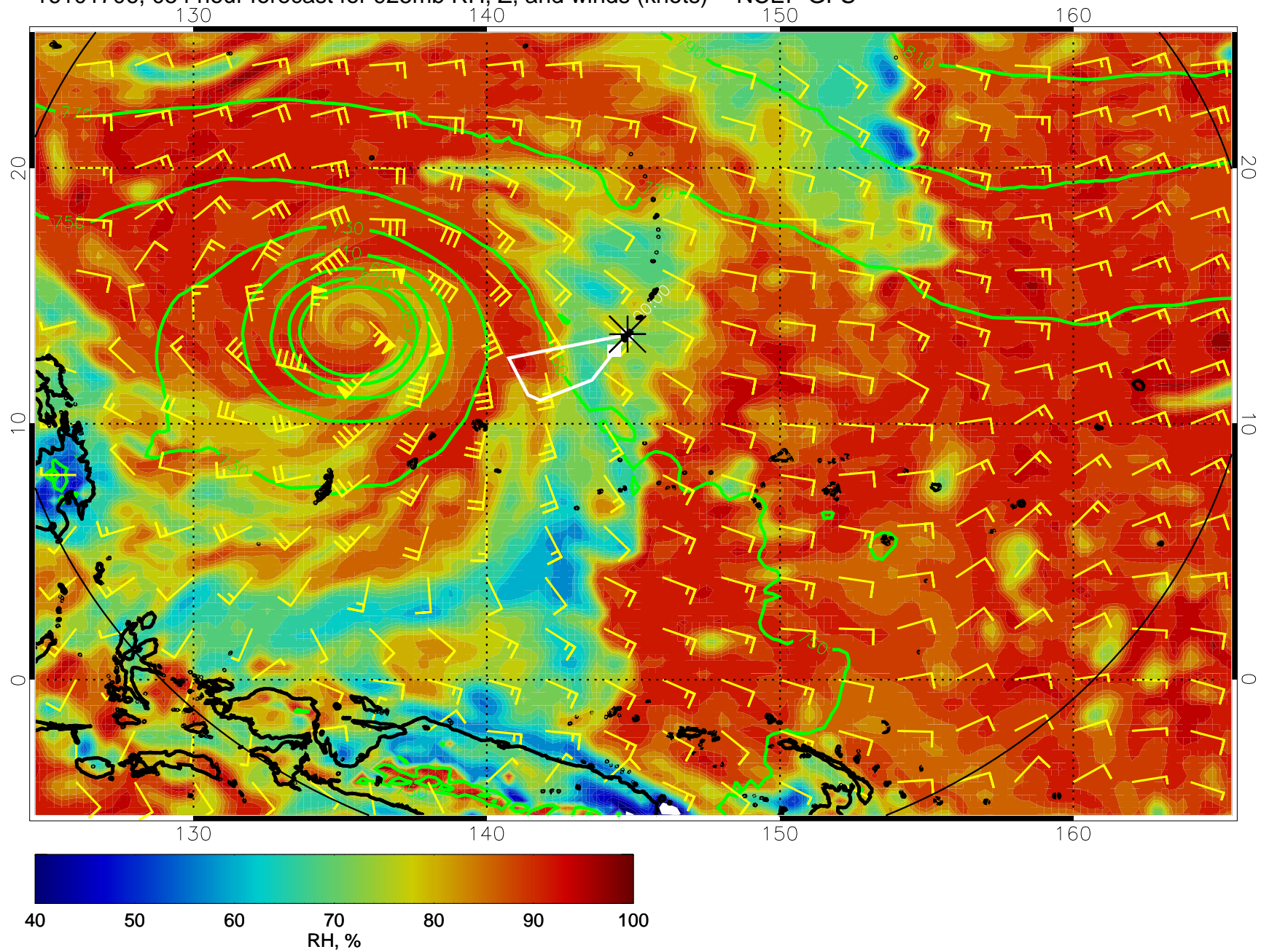
16101706, 054 hour forecast for 925mb RH, Z, and winds (knots) -- NCEP GFS
