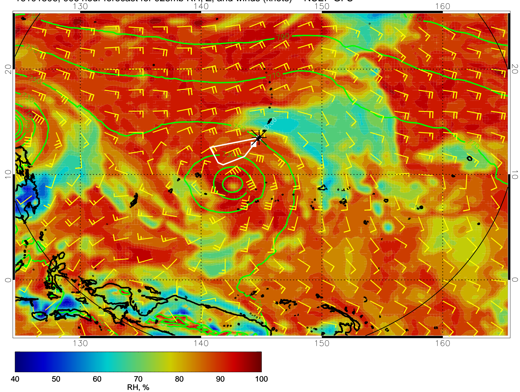
16101506, 006 hour forecast for 925mb RH, Z, and winds (knots) -- NCEP GFS
