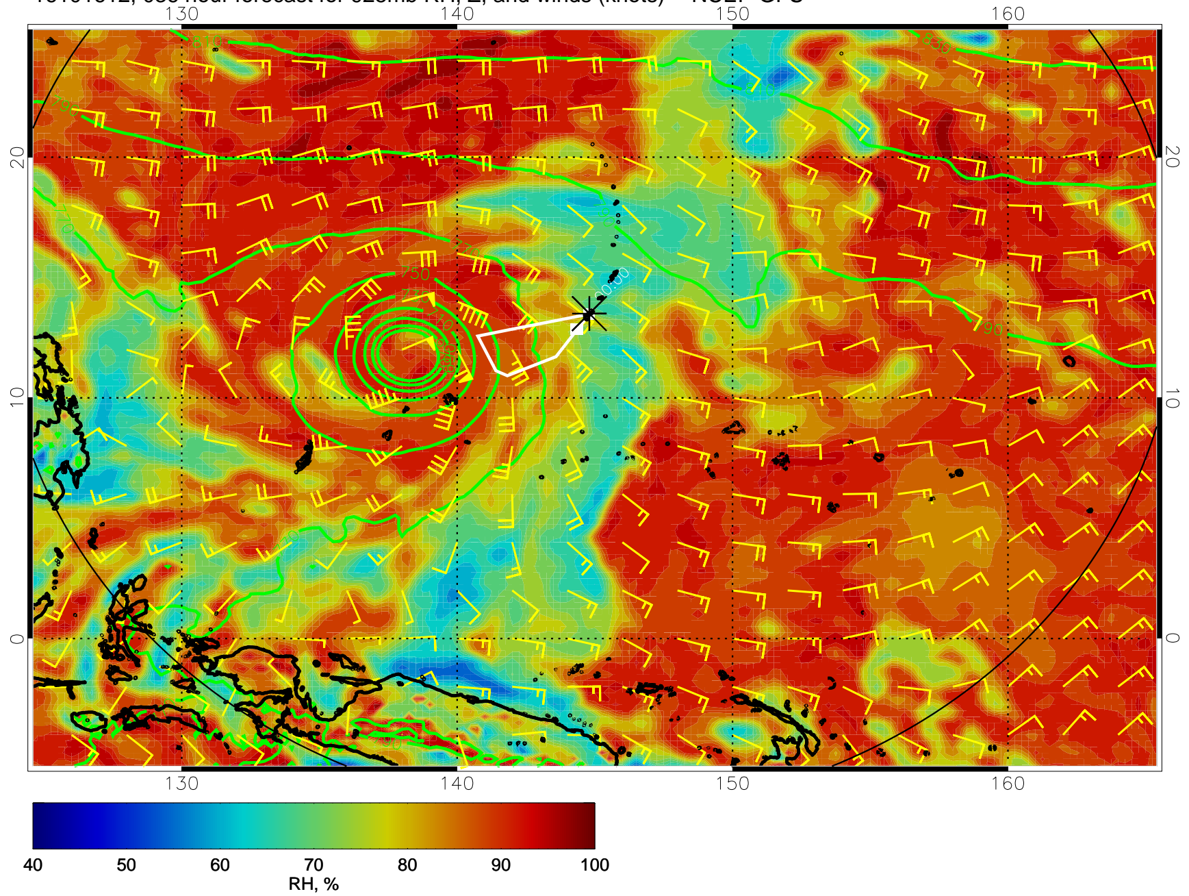
16101612, 036 hour forecast for 925mb RH, Z, and winds (knots) -- NCEP GFS
