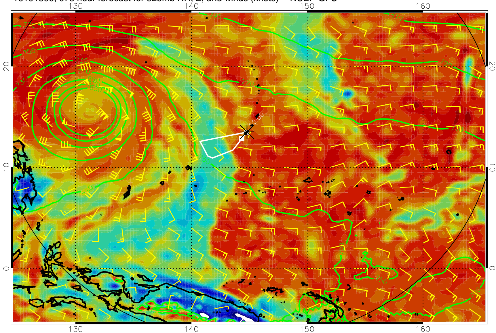
16101806, 078 hour forecast for 925mb RH, Z, and winds (knots) -- NCEP GFS
