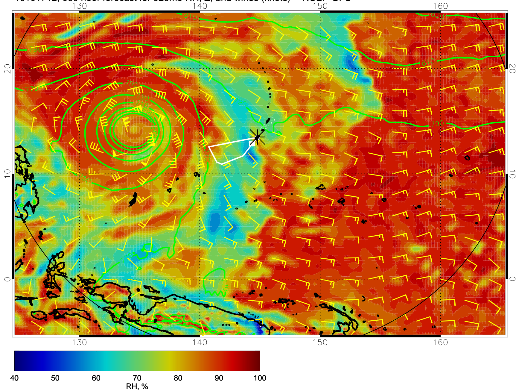
16101712, 060 hour forecast for 925mb RH, Z, and winds (knots) -- NCEP GFS
