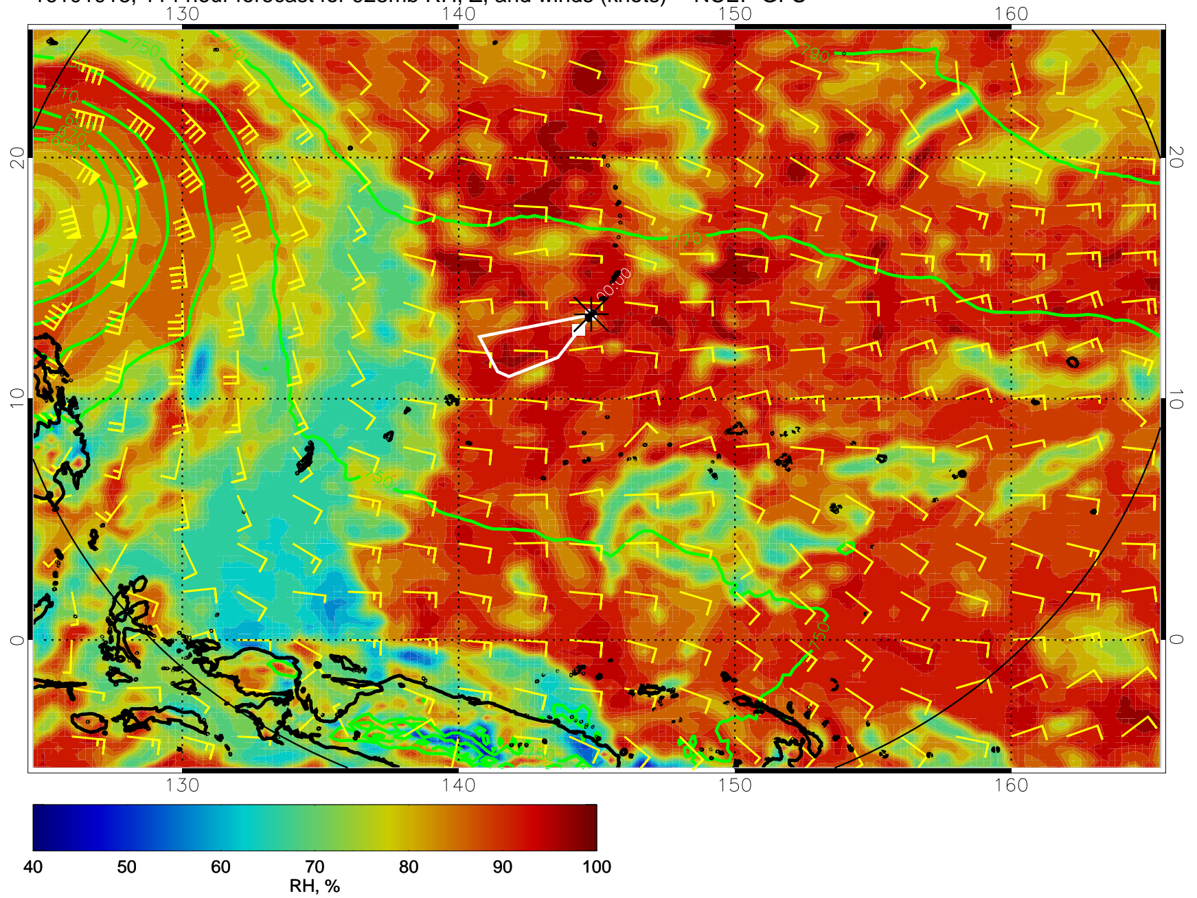
16101918, 114 hour forecast for 925mb RH, Z, and winds (knots) -- NCEP GFS
