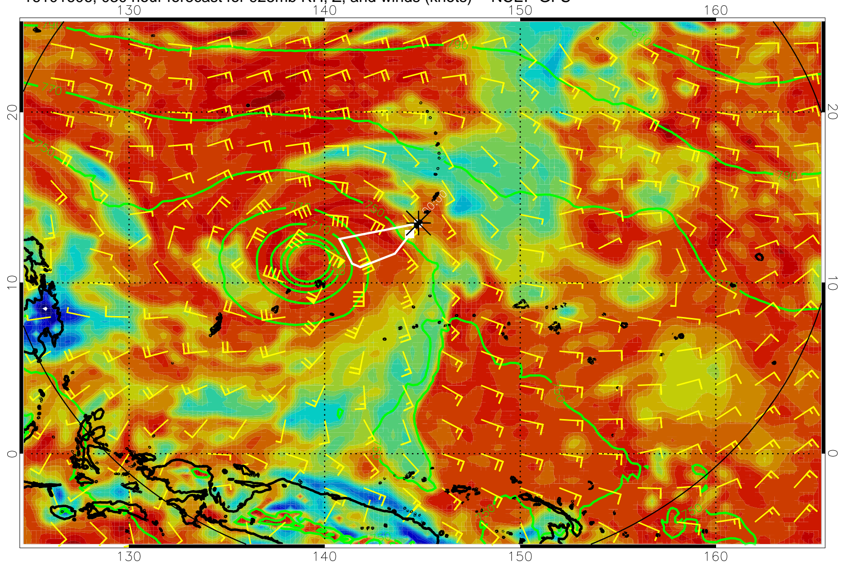
16101606, 030 hour forecast for 925mb RH, Z, and winds (knots) -- NCEP GFS
