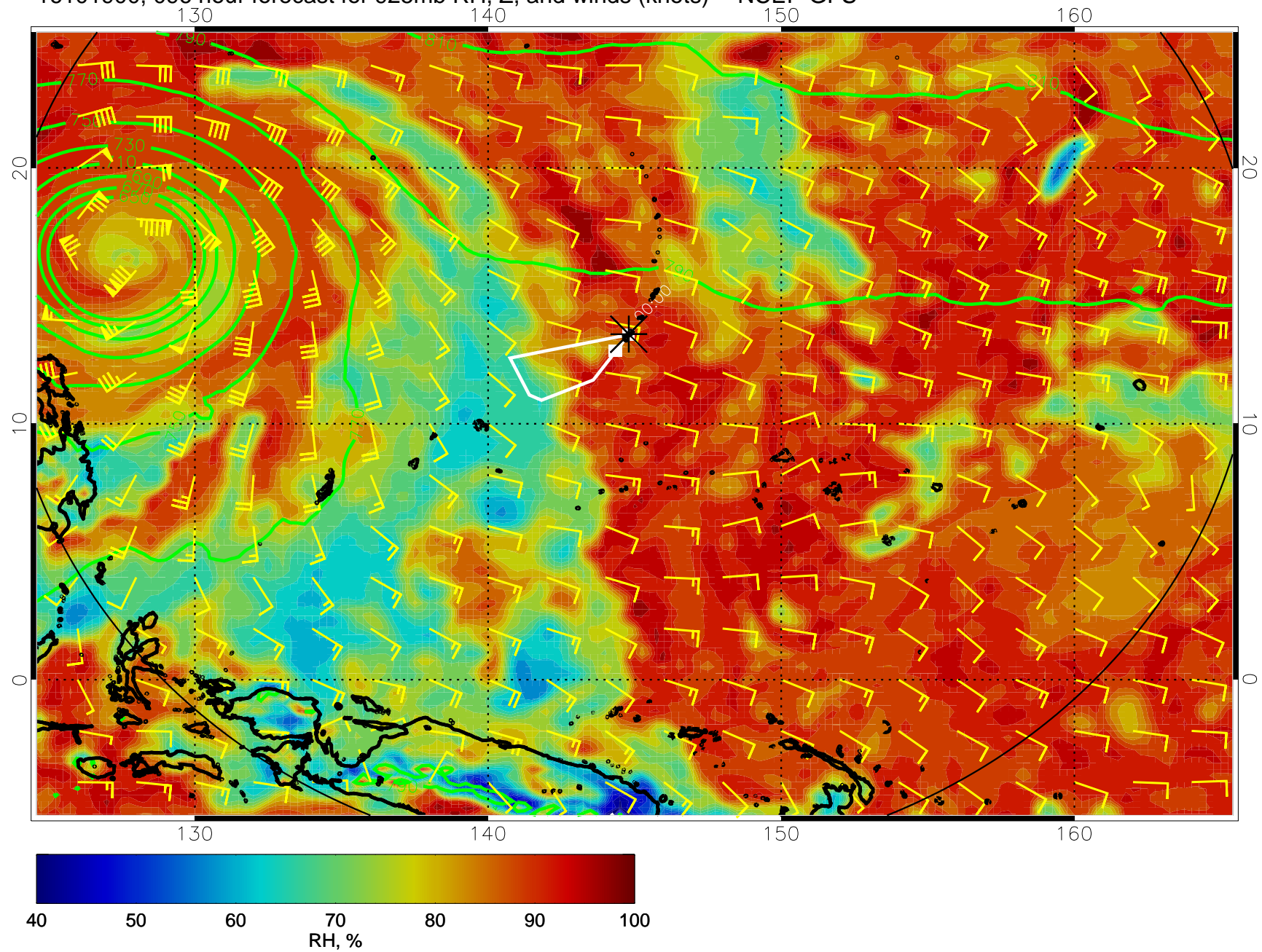
16101900, 096 hour forecast for 925mb RH, Z, and winds (knots) -- NCEP GFS
