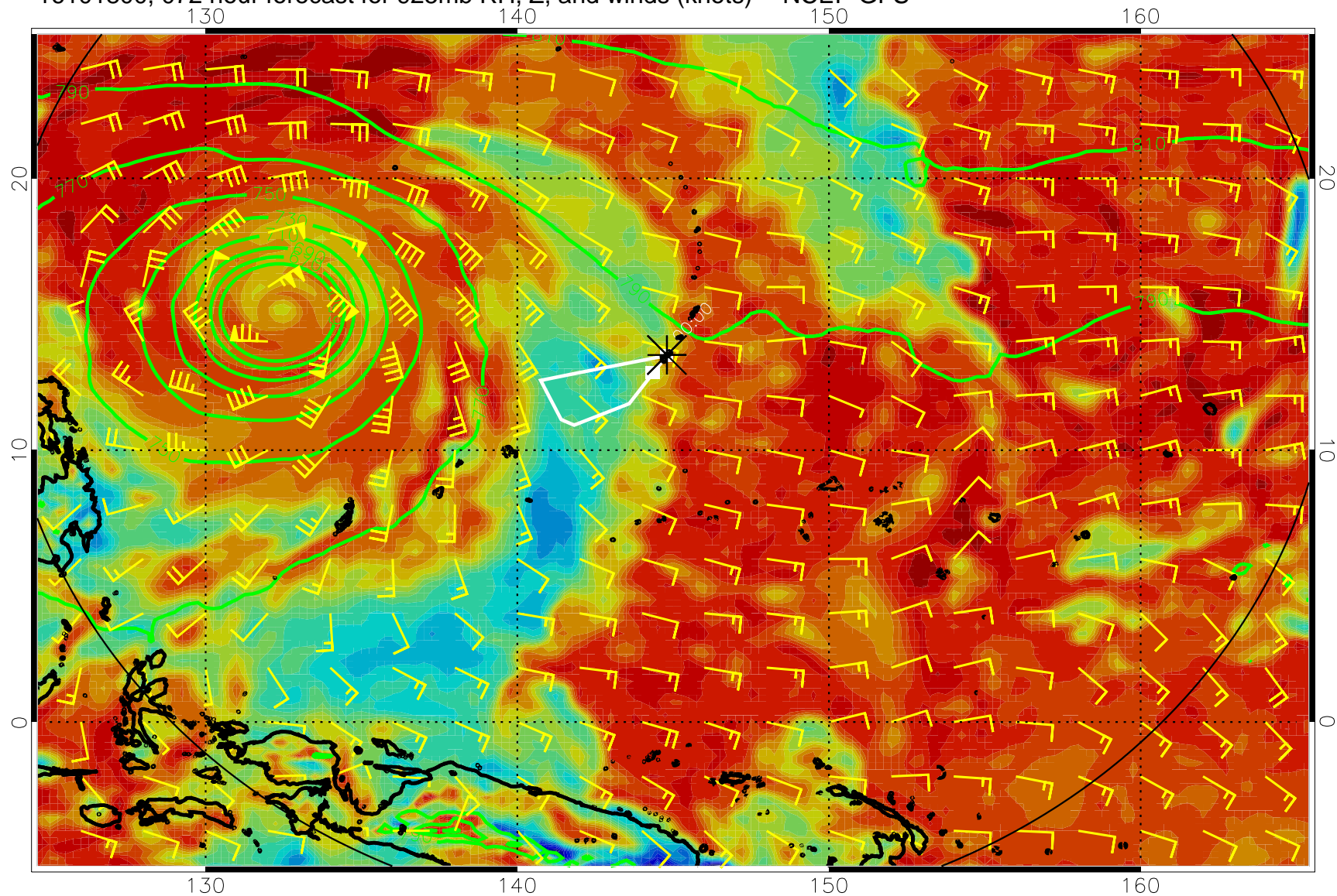
16101800, 072 hour forecast for 925mb RH, Z, and winds (knots) -- NCEP GFS
