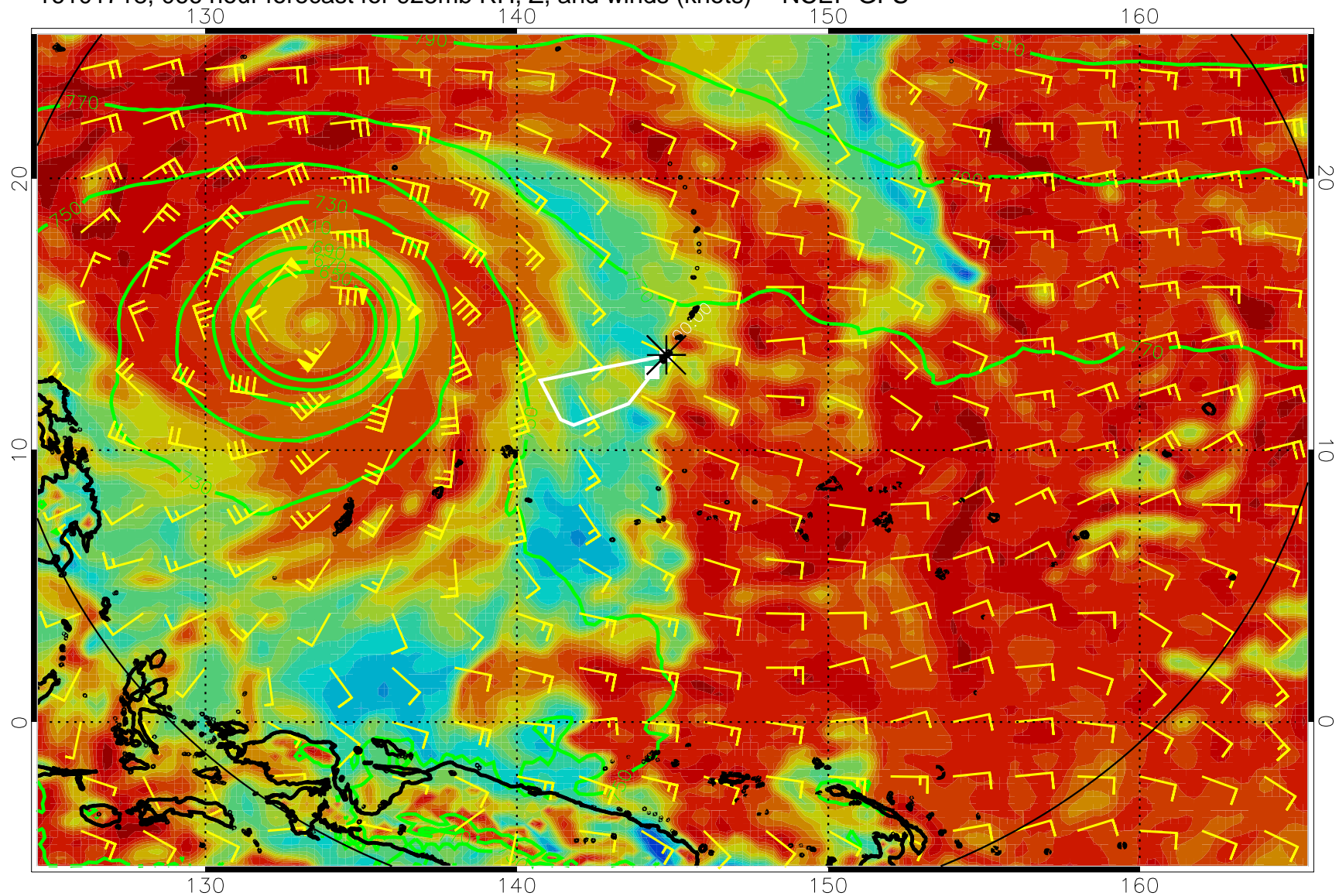
16101718, 066 hour forecast for 925mb RH, Z, and winds (knots) -- NCEP GFS
