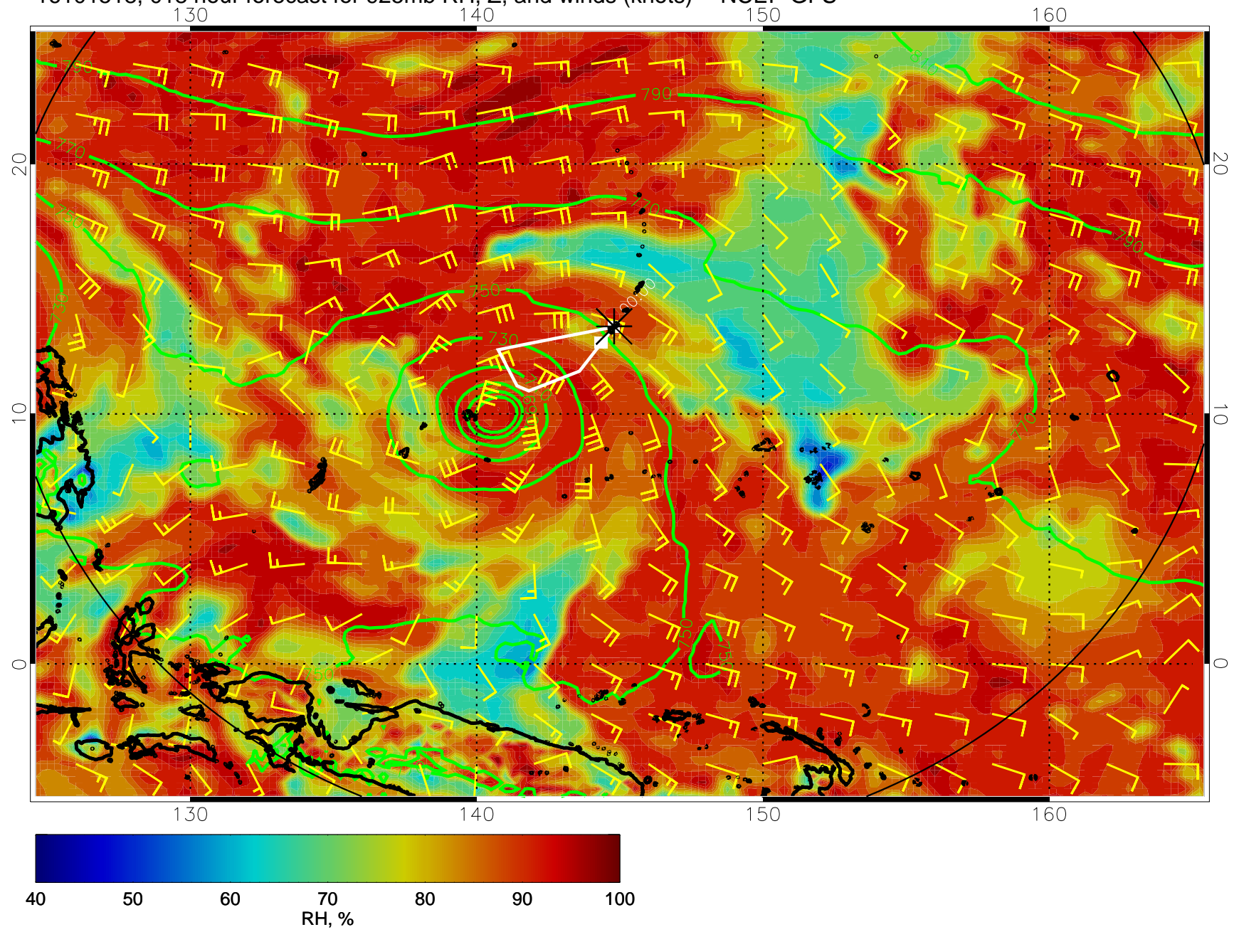
16101518, 018 hour forecast for 925mb RH, Z, and winds (knots) -- NCEP GFS
