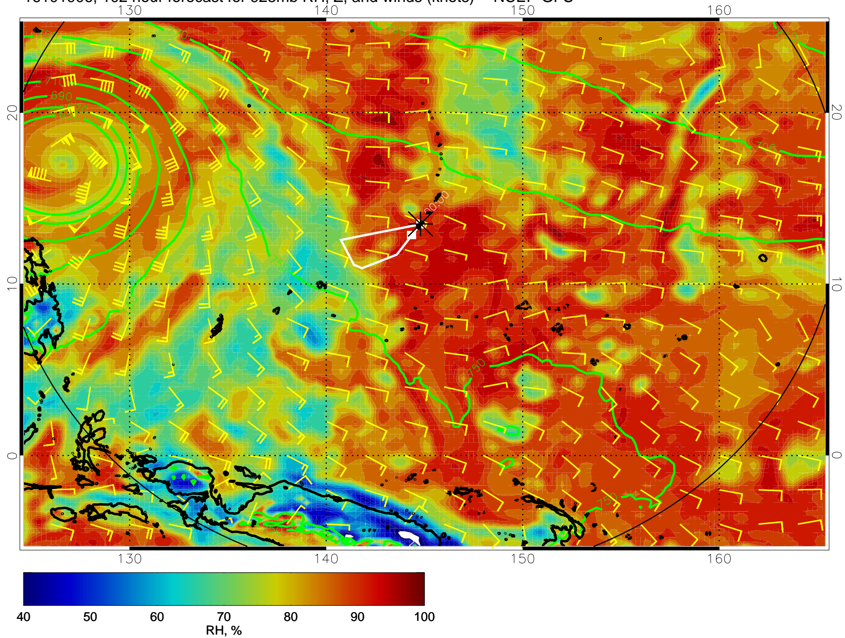
16101906, 102 hour forecast for 925mb RH, Z, and winds (knots) -- NCEP GFS
