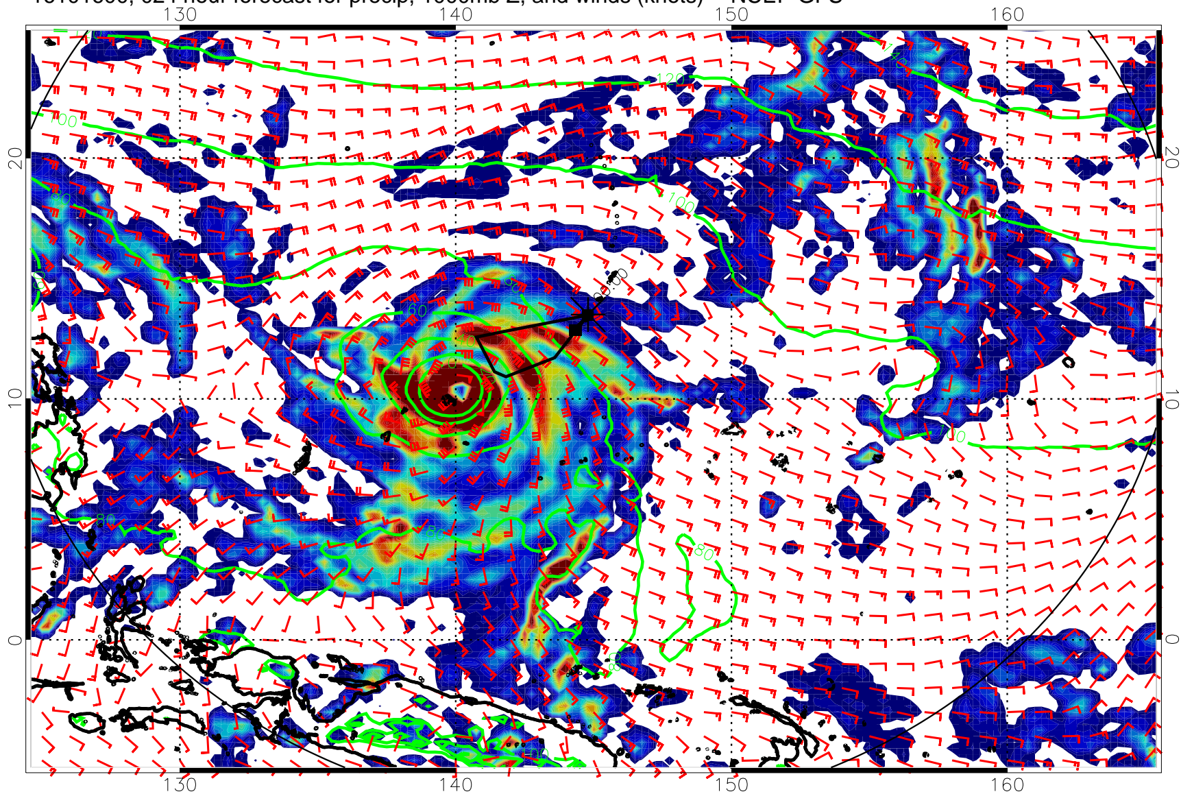
16101600, 024 hour forecast for precip, 1000mb Z, and winds (knots) -- NCEP GFS
