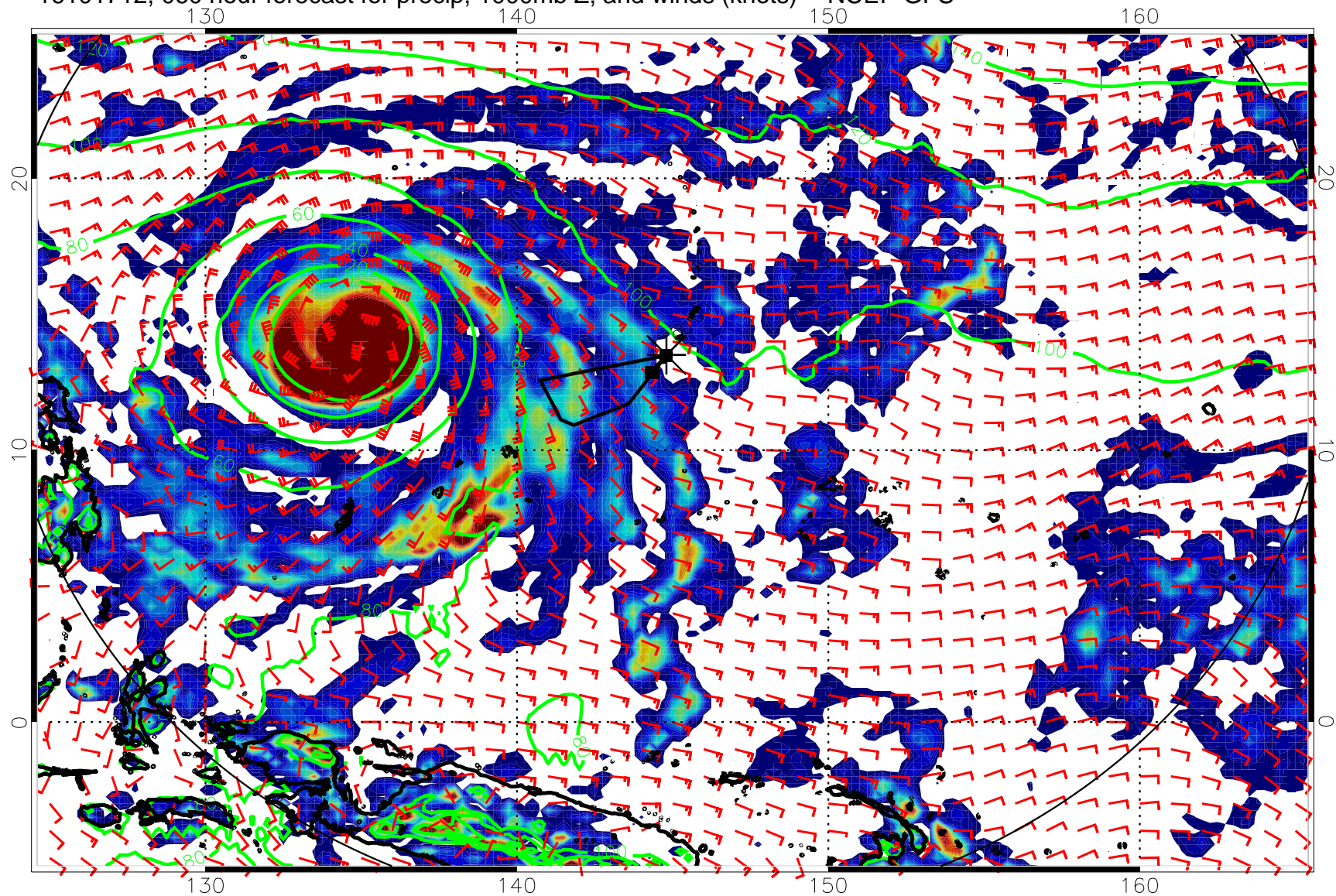
16101712, 060 hour forecast for precip, 1000mb Z, and winds (knots) -- NCEP GFS
