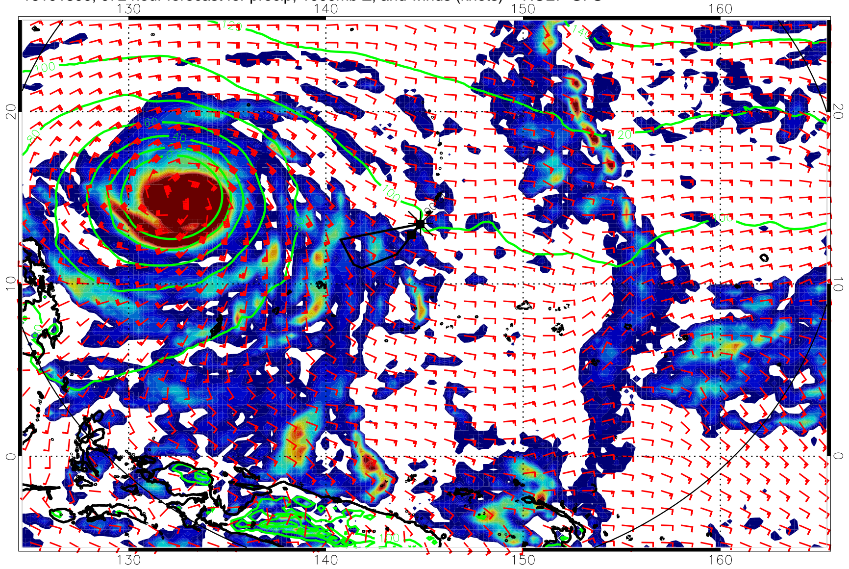
16101800, 072 hour forecast for precip, 1000mb Z, and winds (knots) -- NCEP GFS
