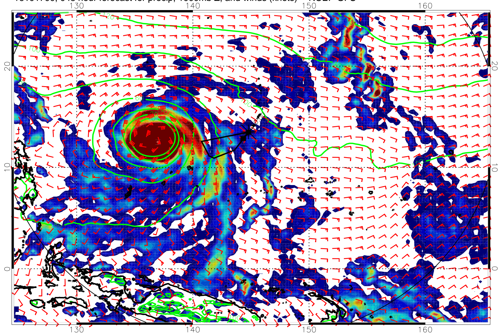
16101700, 048 hour forecast for precip, 1000mb Z, and winds (knots) -- NCEP GFS
