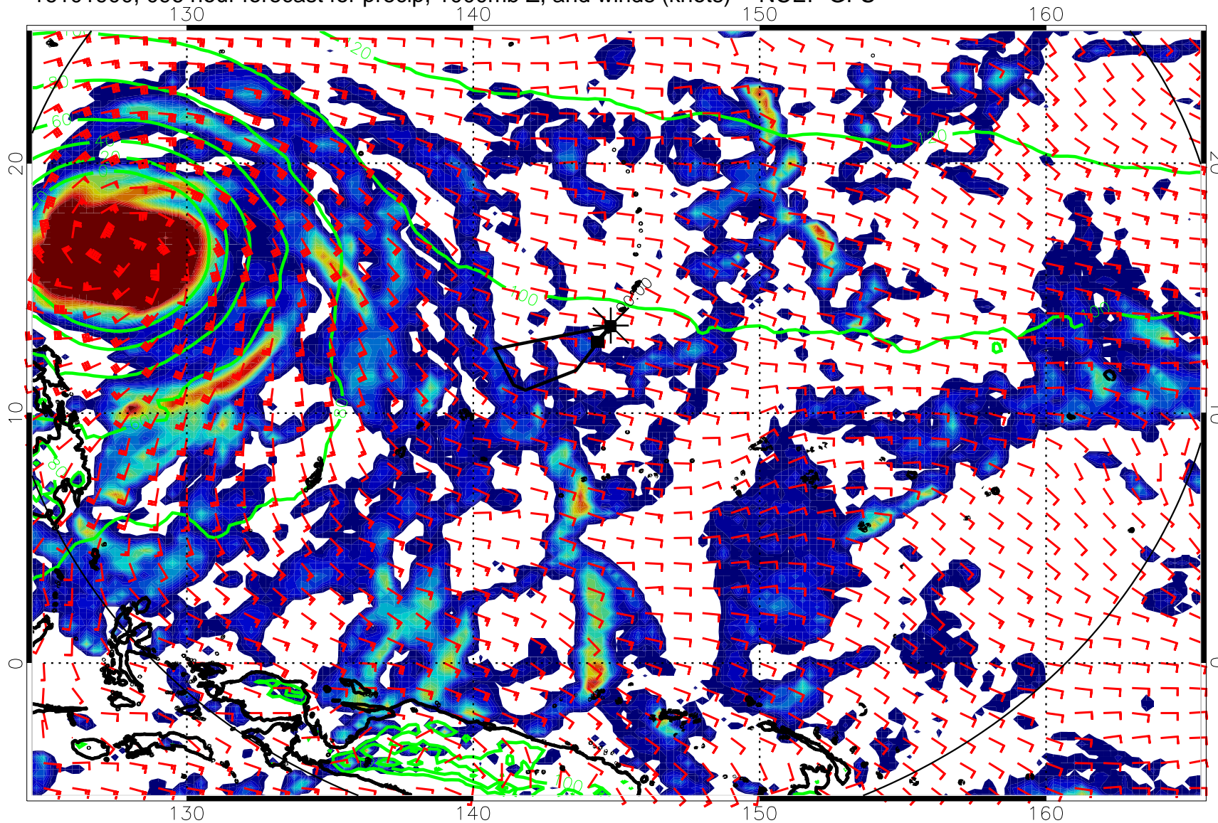
16101900, 096 hour forecast for precip, 1000mb Z, and winds (knots) -- NCEP GFS
