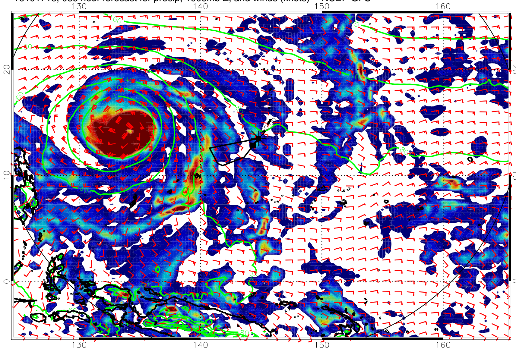
16101718, 066 hour forecast for precip, 1000mb Z, and winds (knots) -- NCEP GFS
