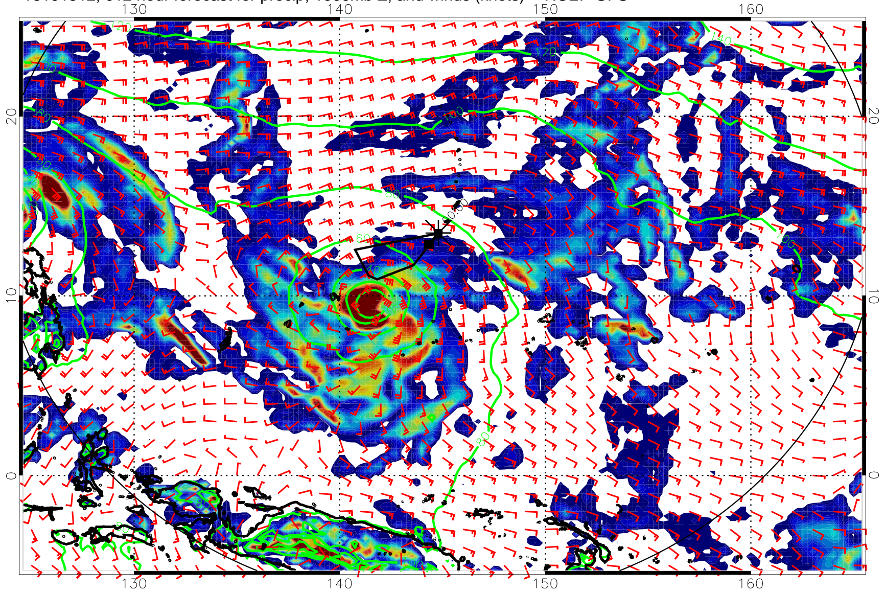
16101512, 012 hour forecast for precip, 1000mb Z, and winds (knots) -- NCEP GFS
