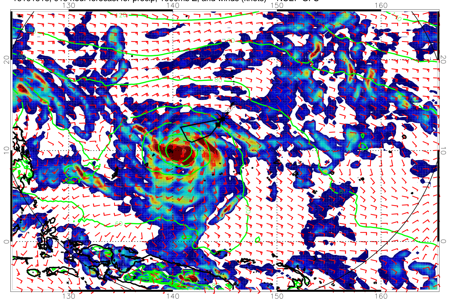
16101518, 018 hour forecast for precip, 1000mb Z, and winds (knots) -- NCEP GFS
