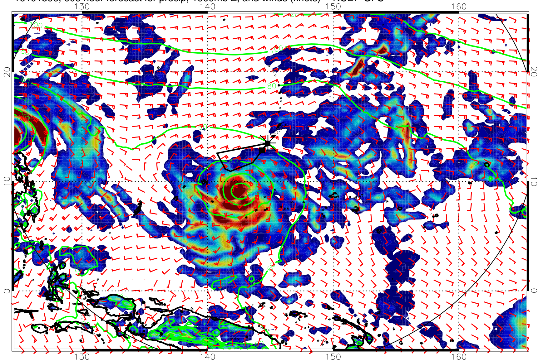
16101506, 006 hour forecast for precip, 1000mb Z, and winds (knots) -- NCEP GFS
