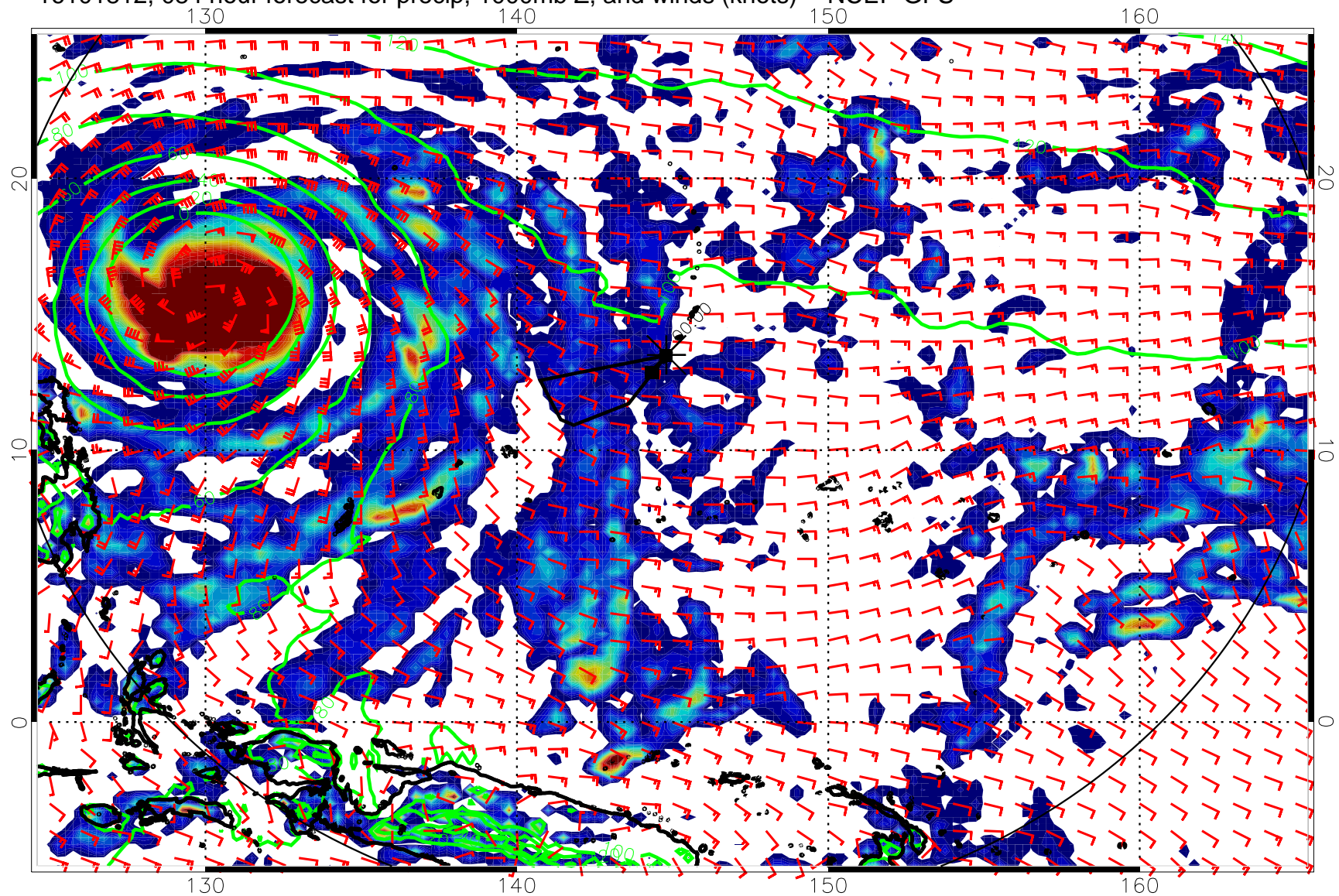
16101812, 084 hour forecast for precip, 1000mb Z, and winds (knots) -- NCEP GFS
