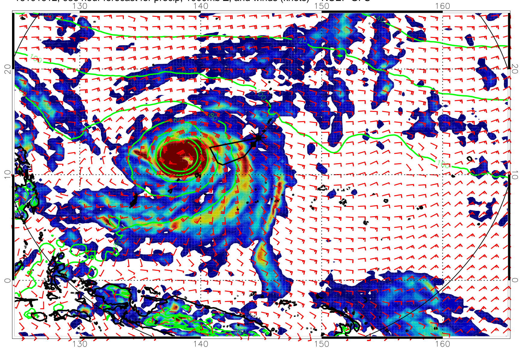
16101612, 036 hour forecast for precip, 1000mb Z, and winds (knots) -- NCEP GFS
