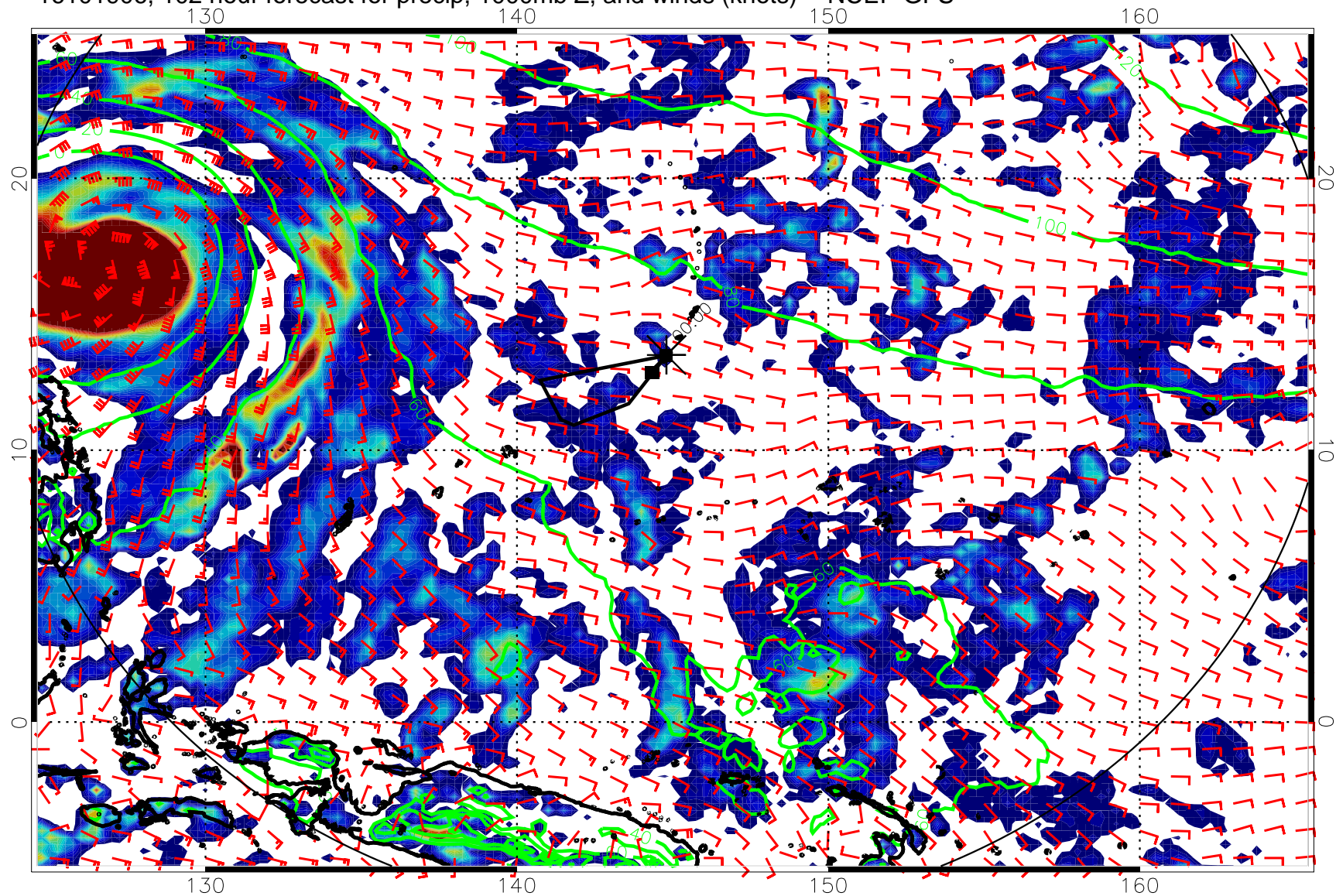
16101906, 102 hour forecast for precip, 1000mb Z, and winds (knots) -- NCEP GFS
