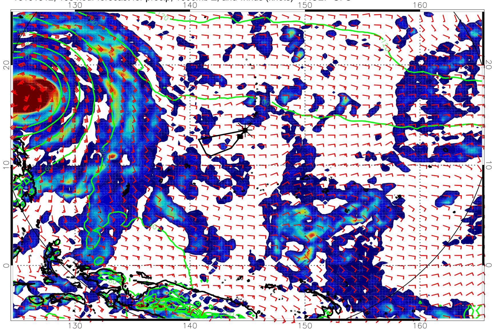
16101912, 108 hour forecast for precip, 1000mb Z, and winds (knots) -- NCEP GFS
