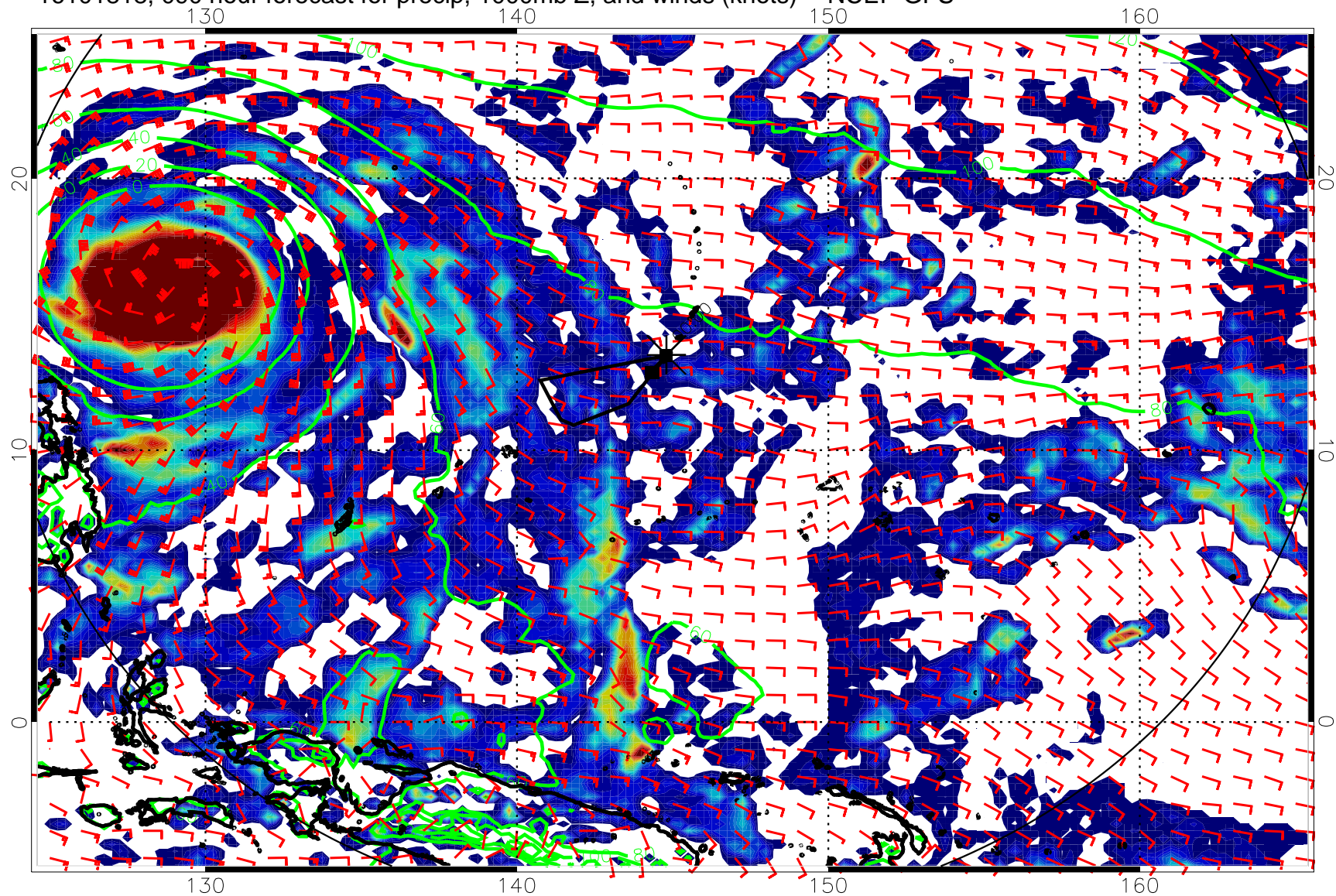
16101818, 090 hour forecast for precip, 1000mb Z, and winds (knots) -- NCEP GFS
