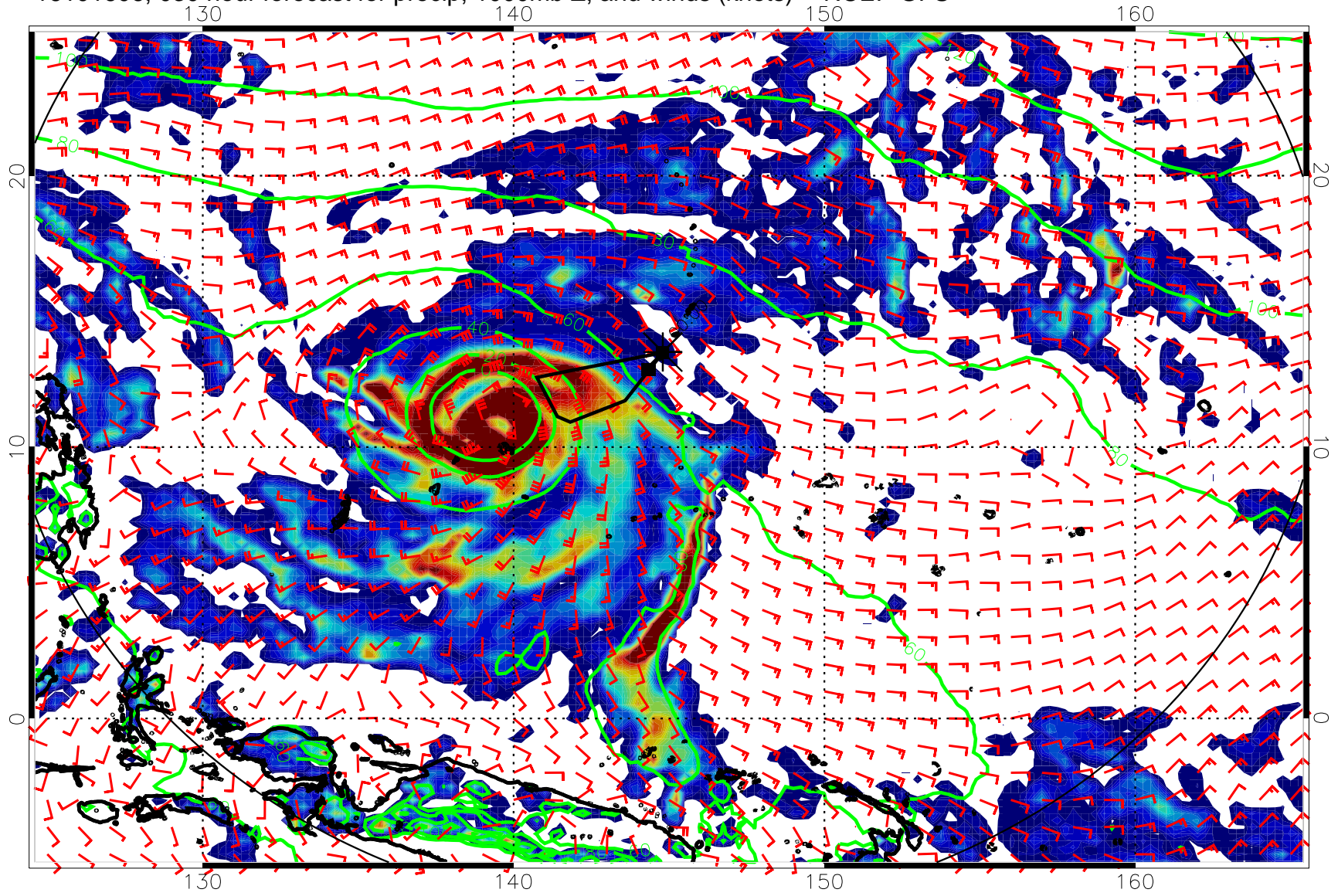
16101606, 030 hour forecast for precip, 1000mb Z, and winds (knots) -- NCEP GFS
