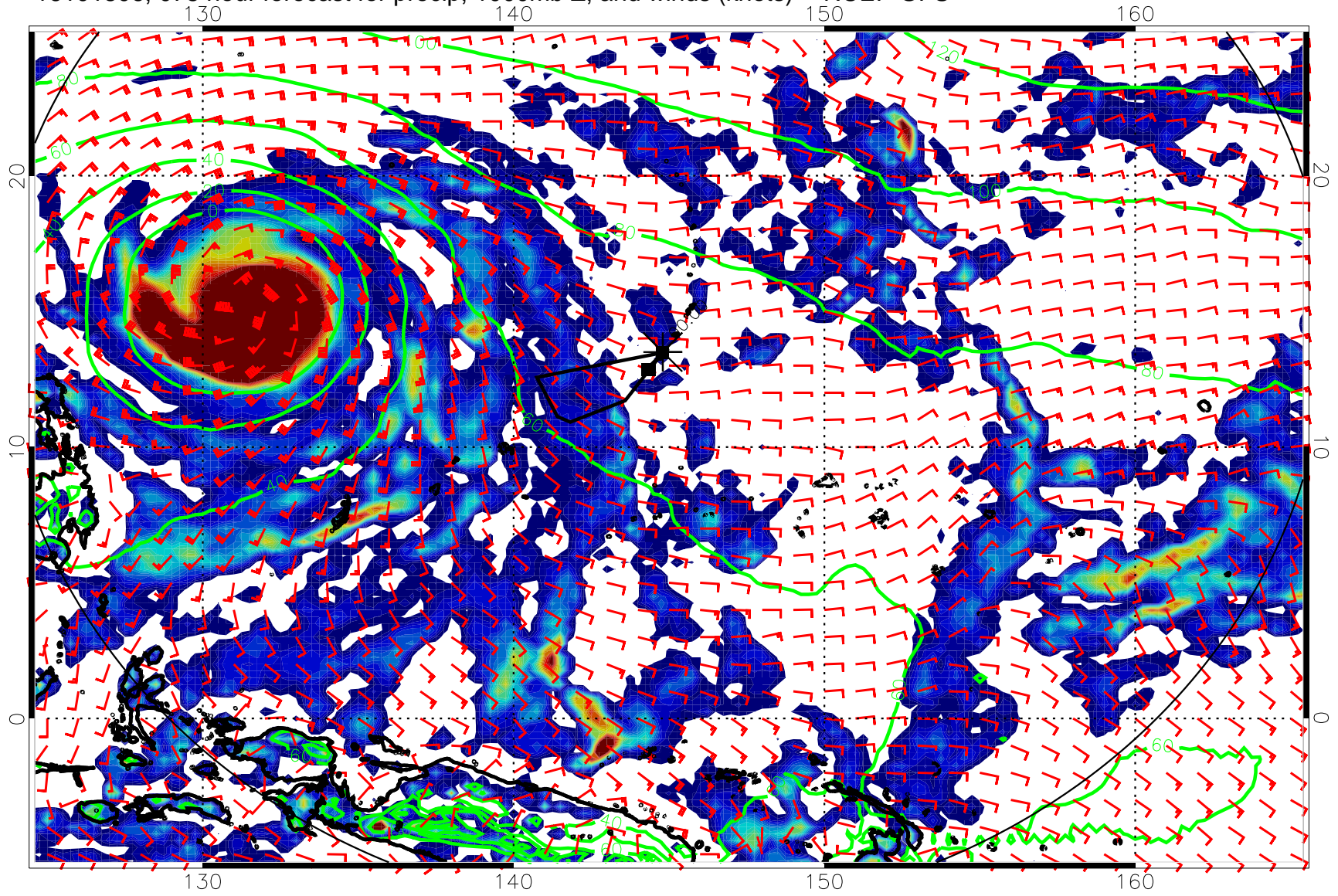
16101806, 078 hour forecast for precip, 1000mb Z, and winds (knots) -- NCEP GFS
