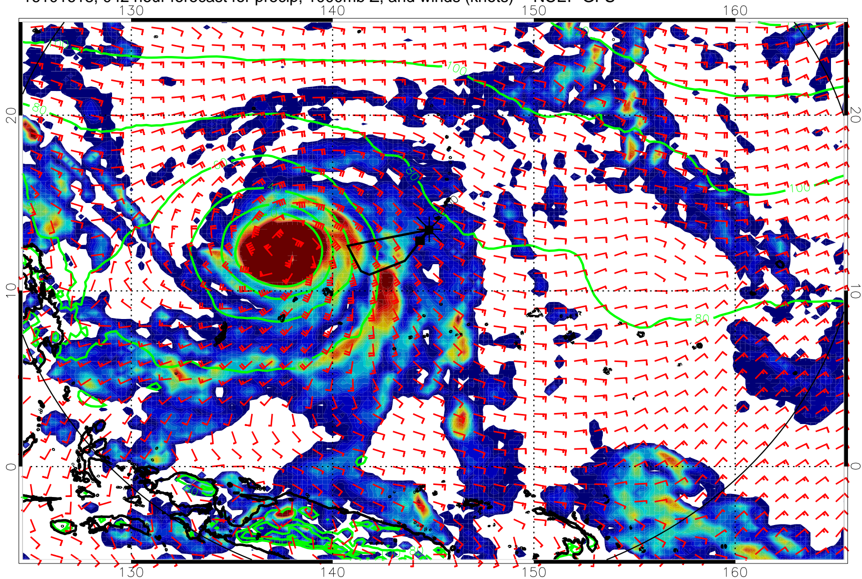
16101618, 042 hour forecast for precip, 1000mb Z, and winds (knots) -- NCEP GFS
