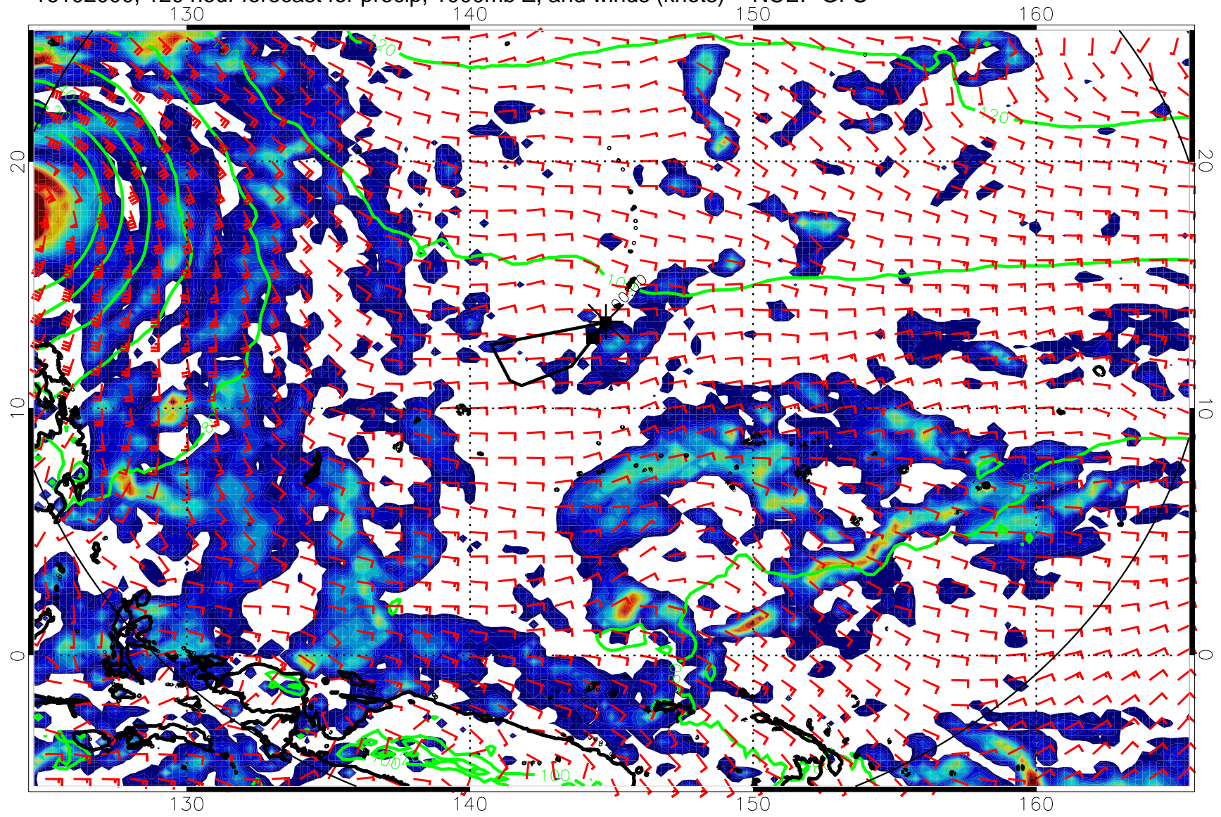
16102000, 120 hour forecast for precip, 1000mb Z, and winds (knots) -- NCEP GFS
