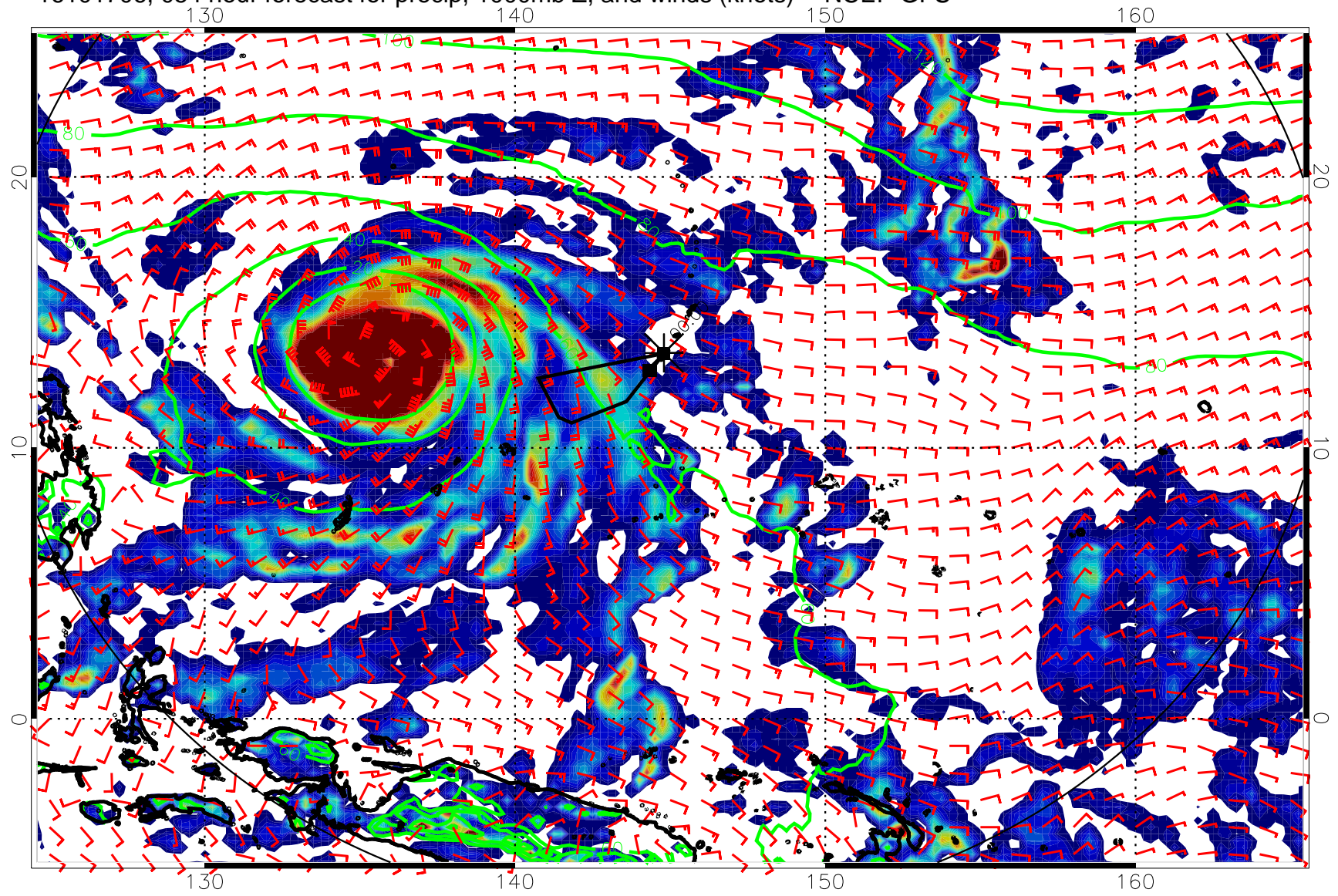
16101706, 054 hour forecast for precip, 1000mb Z, and winds (knots) -- NCEP GFS
