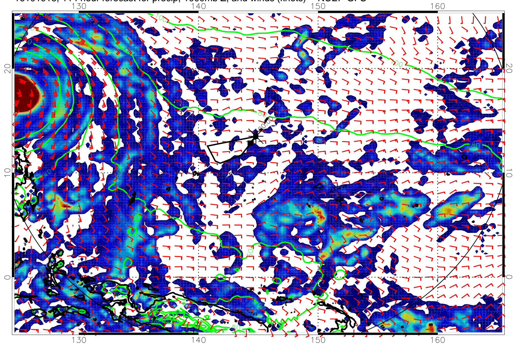
16101918, 114 hour forecast for precip, 1000mb Z, and winds (knots) -- NCEP GFS
