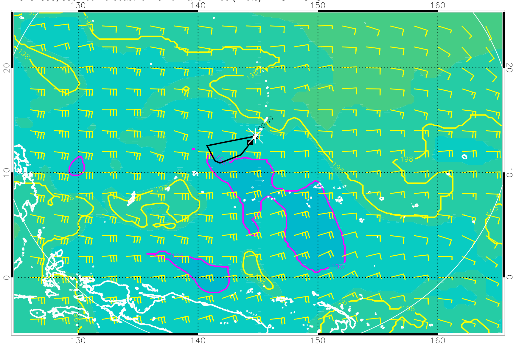
16101606, 030 hour forecast for 70mb T and winds (knots) -- NCEP GFS
