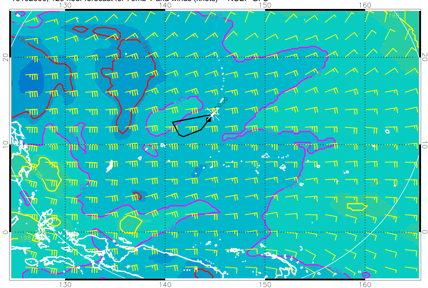
16102000, 120 hour forecast for 70mb T and winds (knots) -- NCEP GFS
