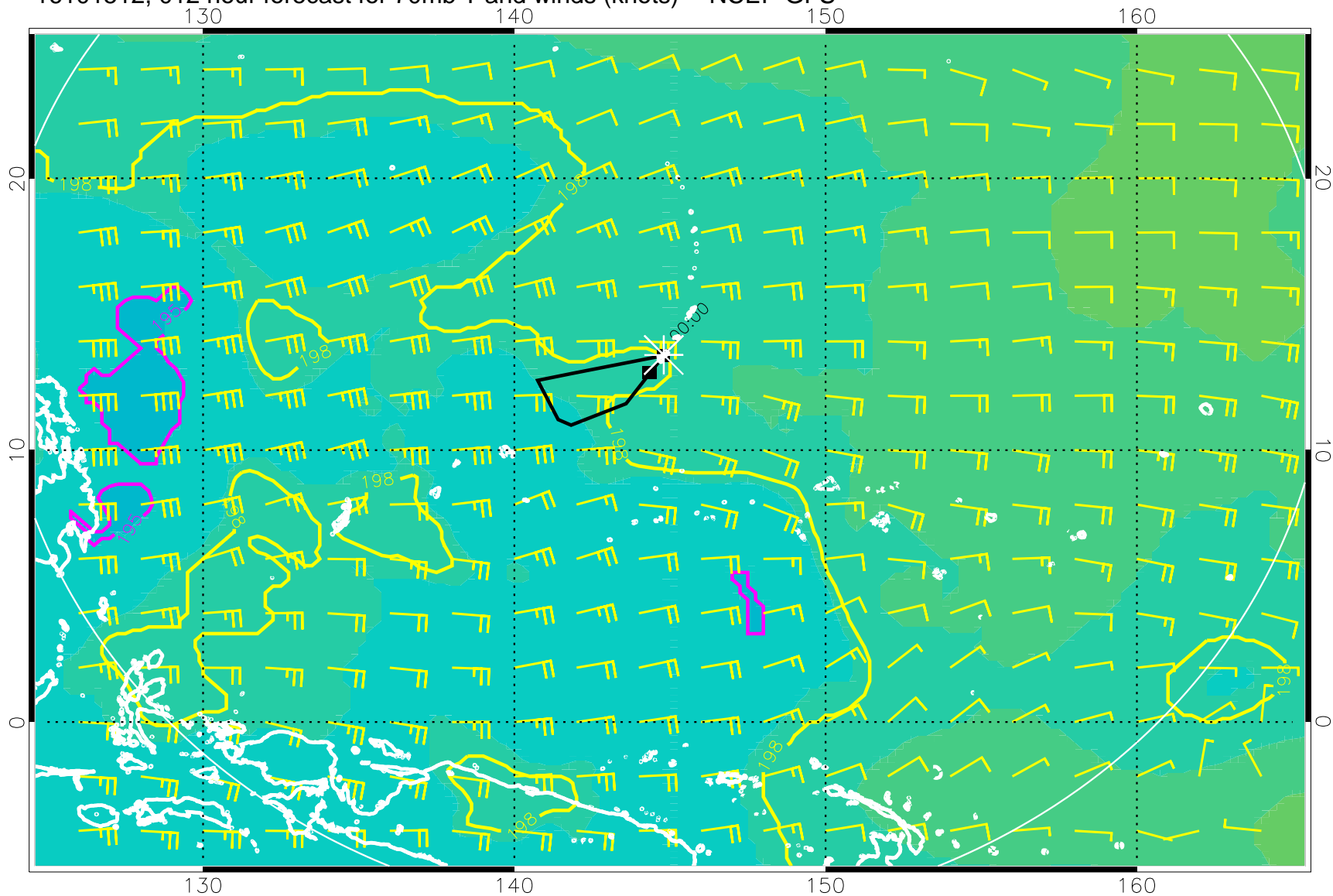
16101512, 012 hour forecast for 70mb T and winds (knots) -- NCEP GFS
