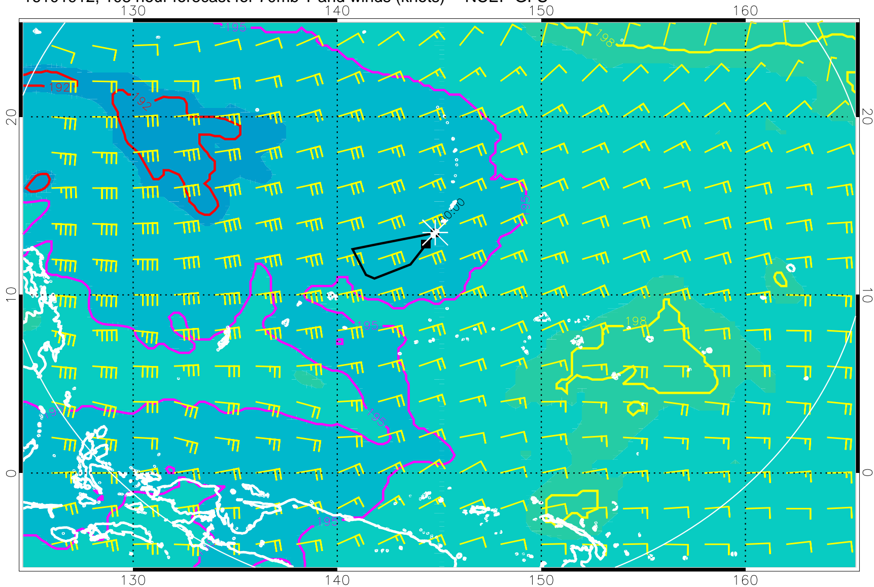
16101912, 108 hour forecast for 70mb T and winds (knots) -- NCEP GFS
