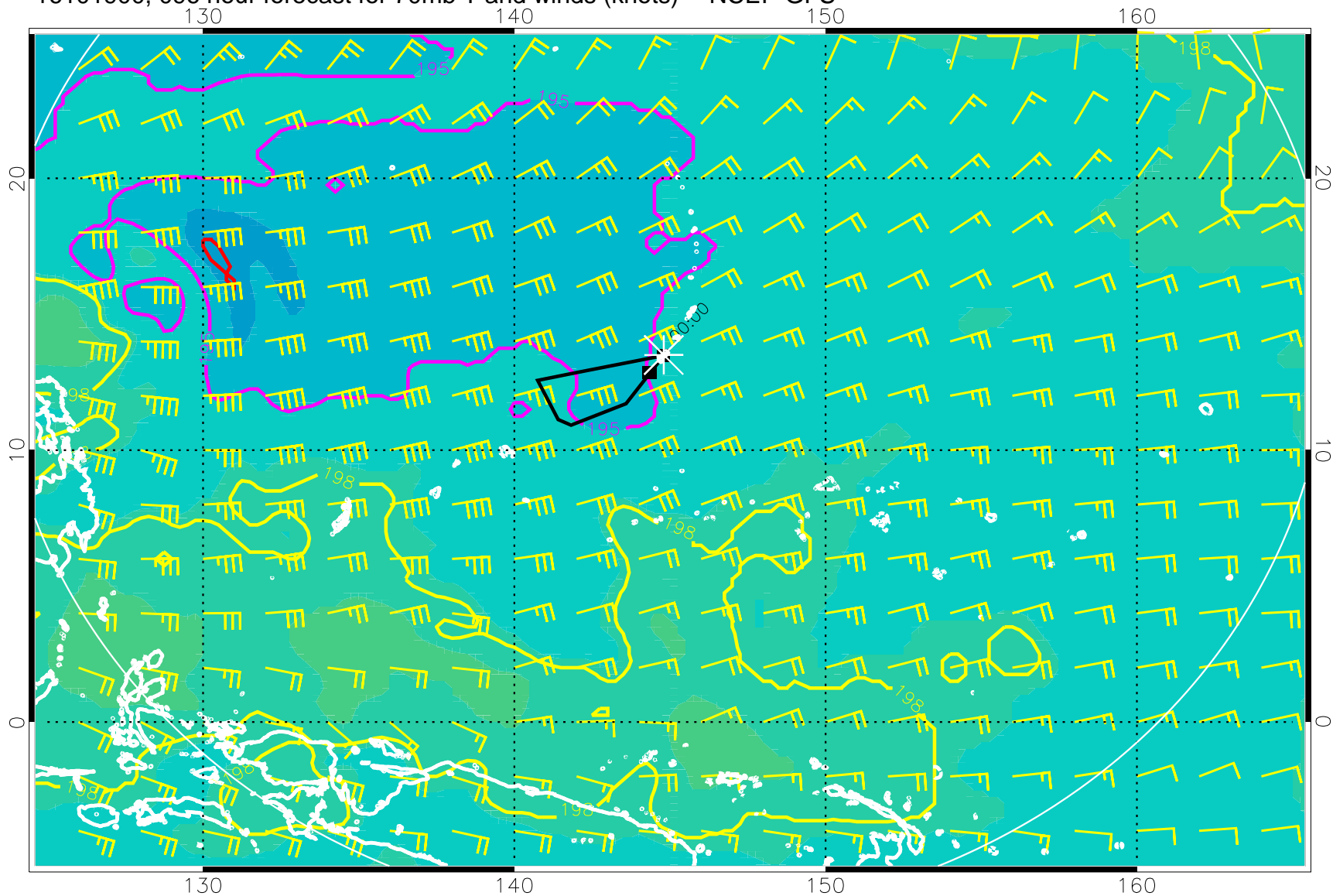
16101900, 096 hour forecast for 70mb T and winds (knots) -- NCEP GFS
