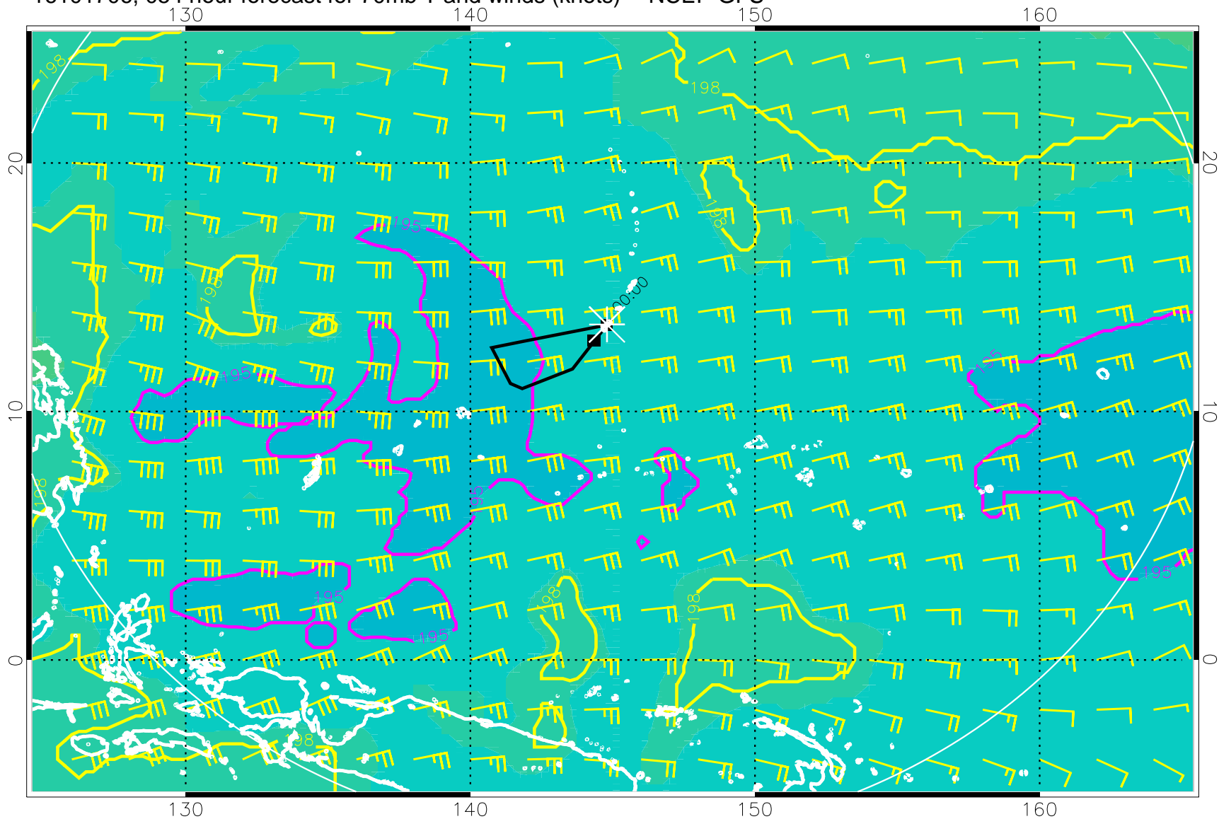
16101706, 054 hour forecast for 70mb T and winds (knots) -- NCEP GFS
