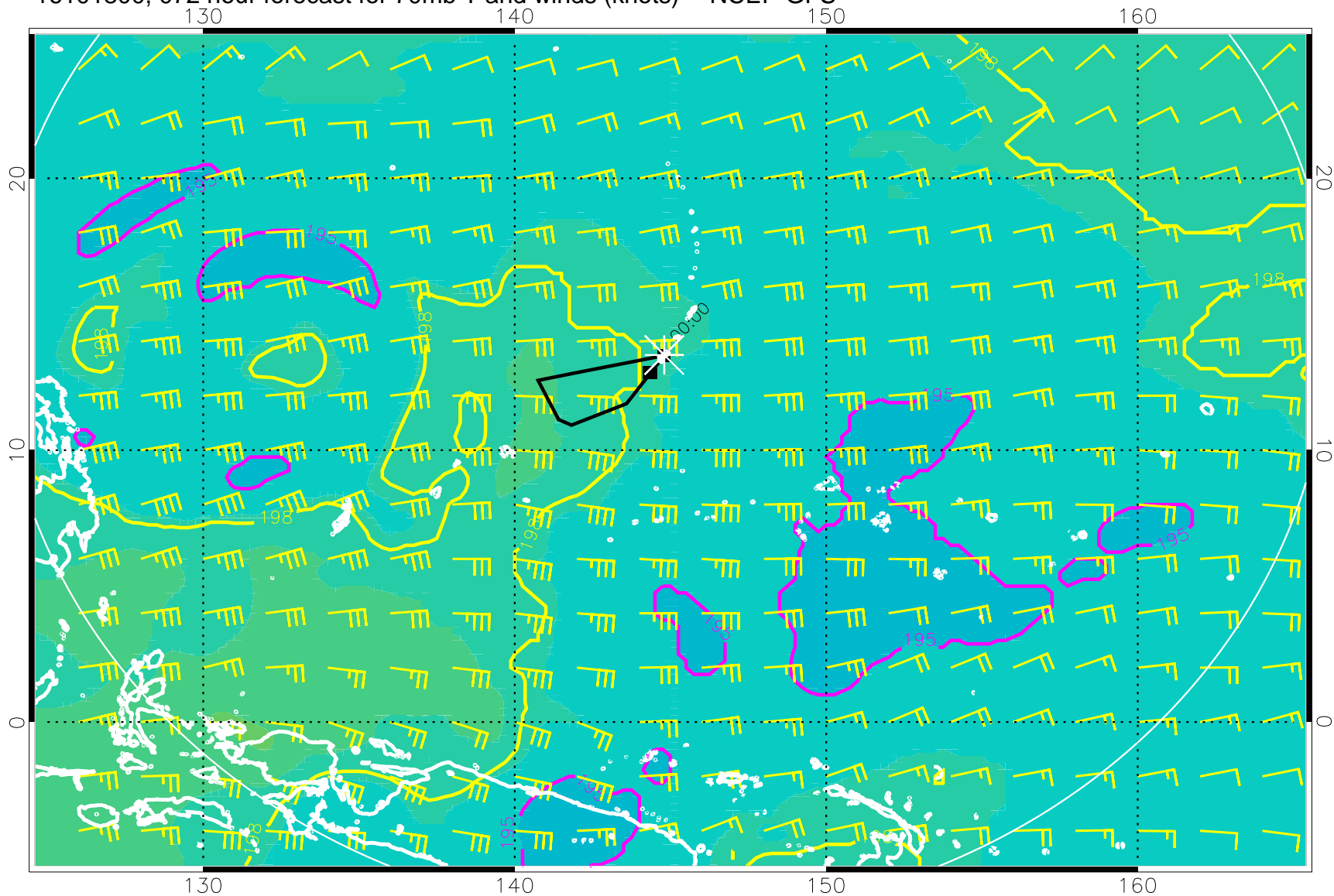
16101800, 072 hour forecast for 70mb T and winds (knots) -- NCEP GFS
