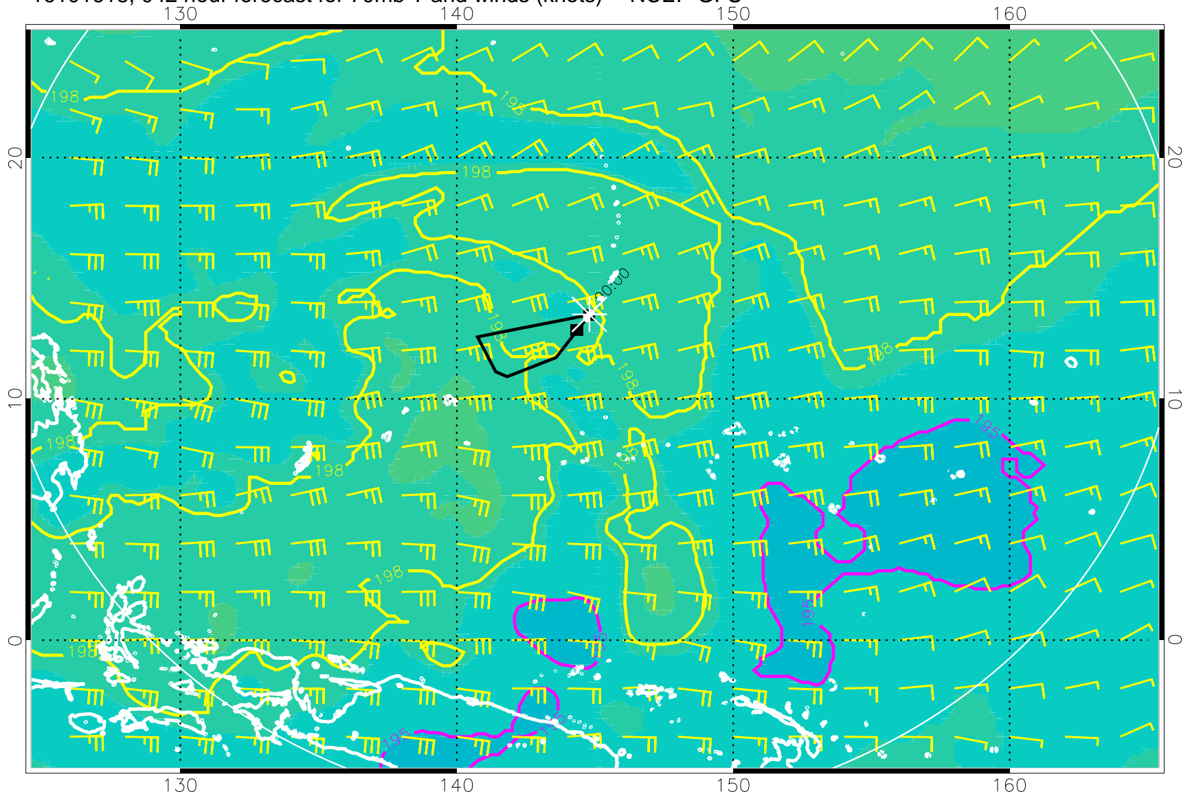
16101618, 042 hour forecast for 70mb T and winds (knots) -- NCEP GFS
