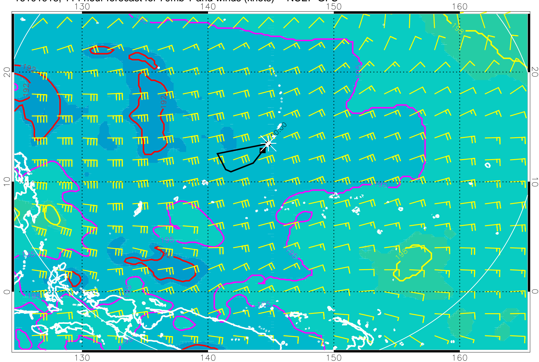
16101918, 114 hour forecast for 70mb T and winds (knots) -- NCEP GFS
