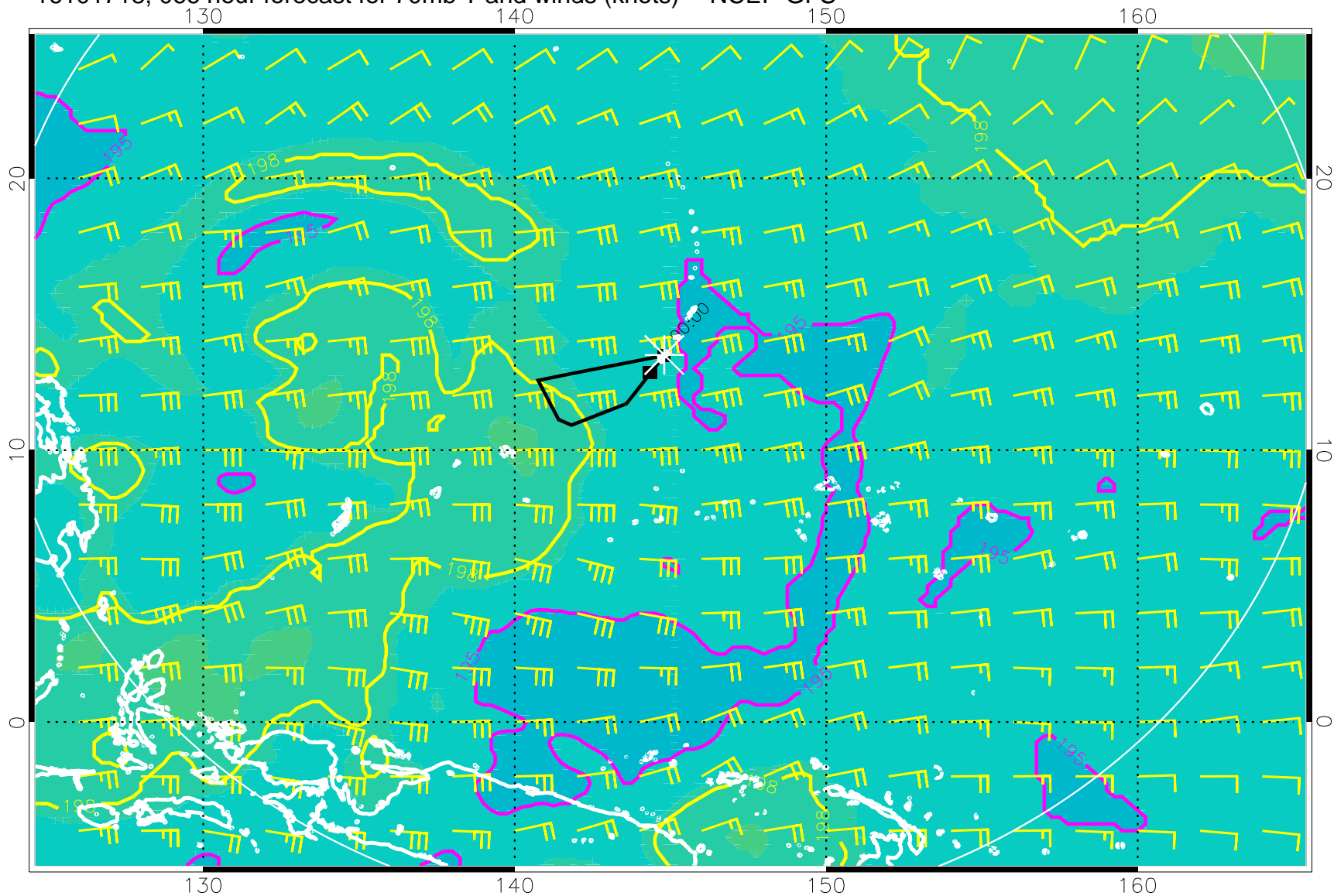
16101718, 066 hour forecast for 70mb T and winds (knots) -- NCEP GFS
