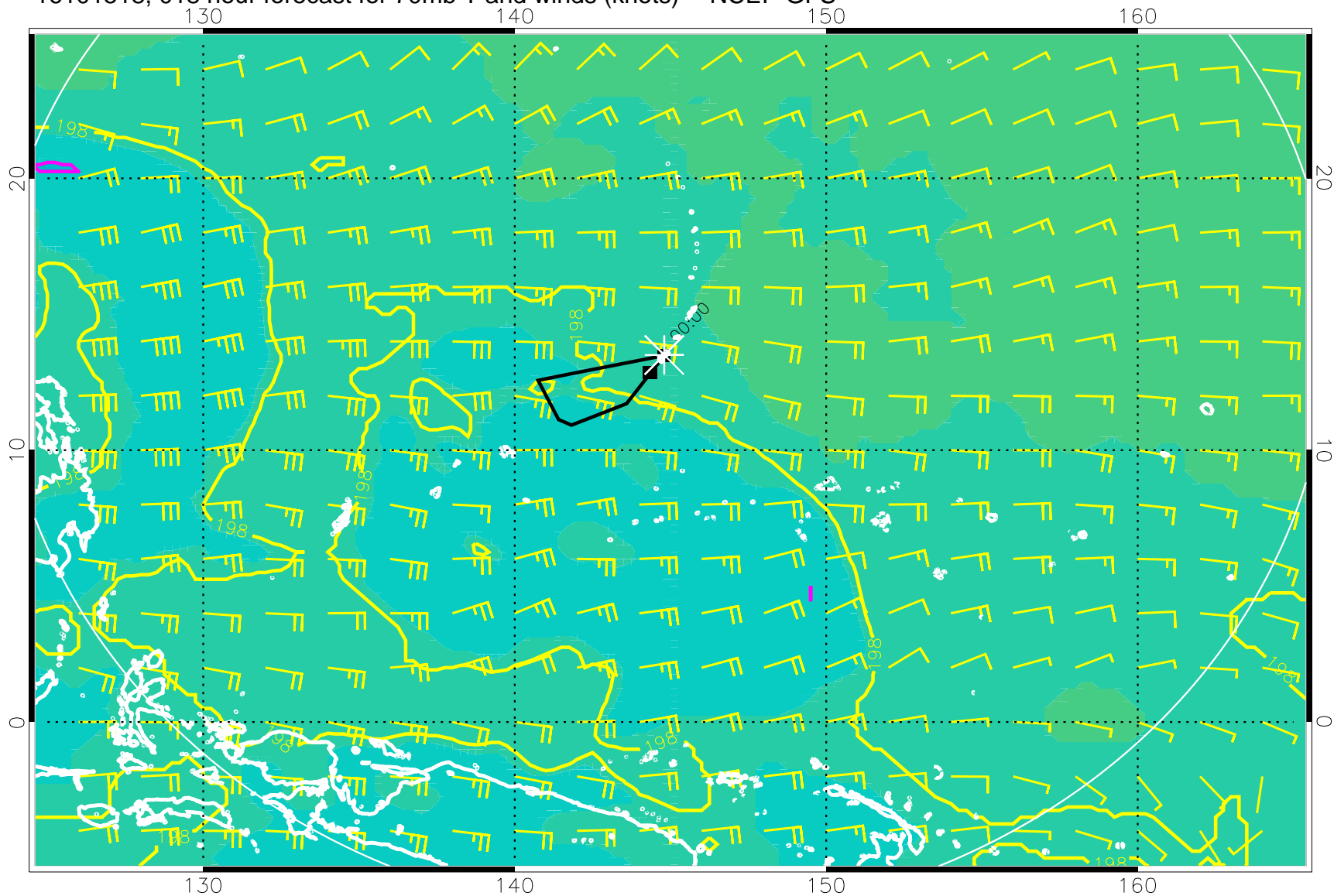
16101518, 018 hour forecast for 70mb T and winds (knots) -- NCEP GFS
