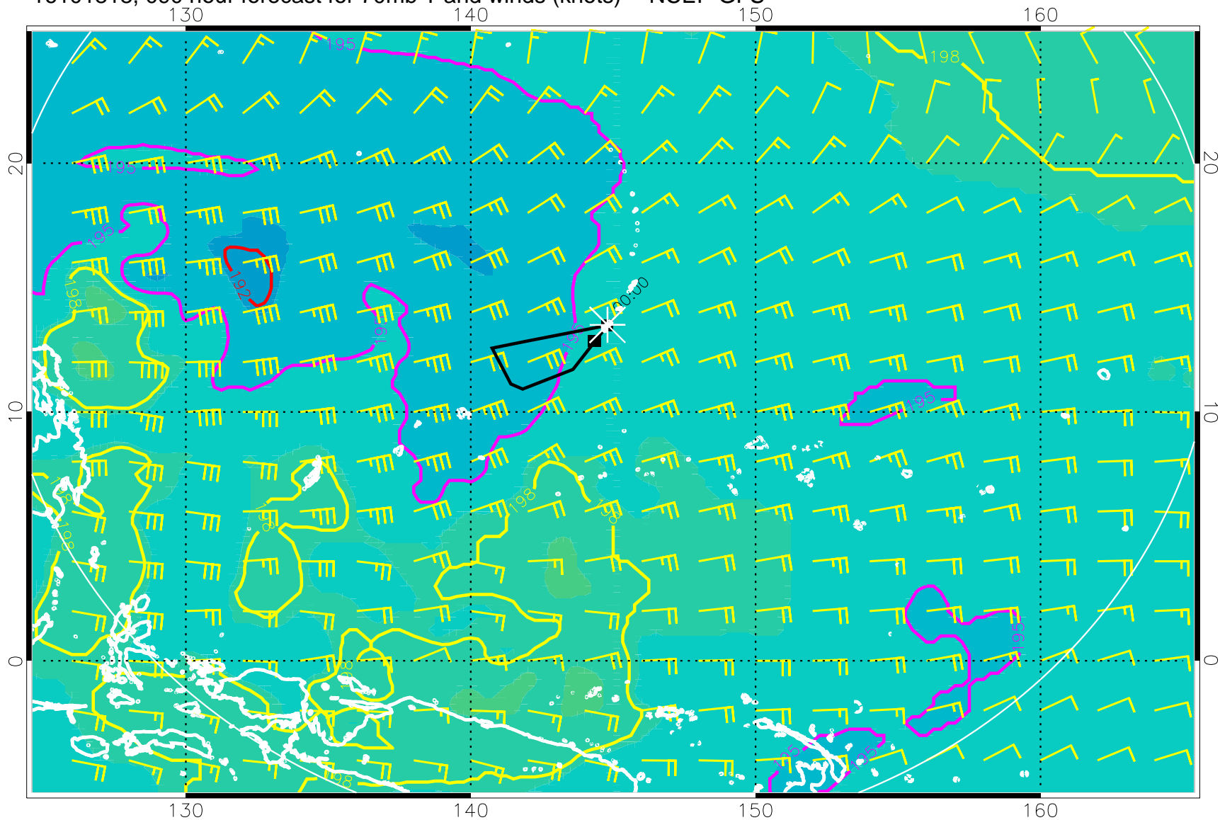
16101818, 090 hour forecast for 70mb T and winds (knots) -- NCEP GFS
