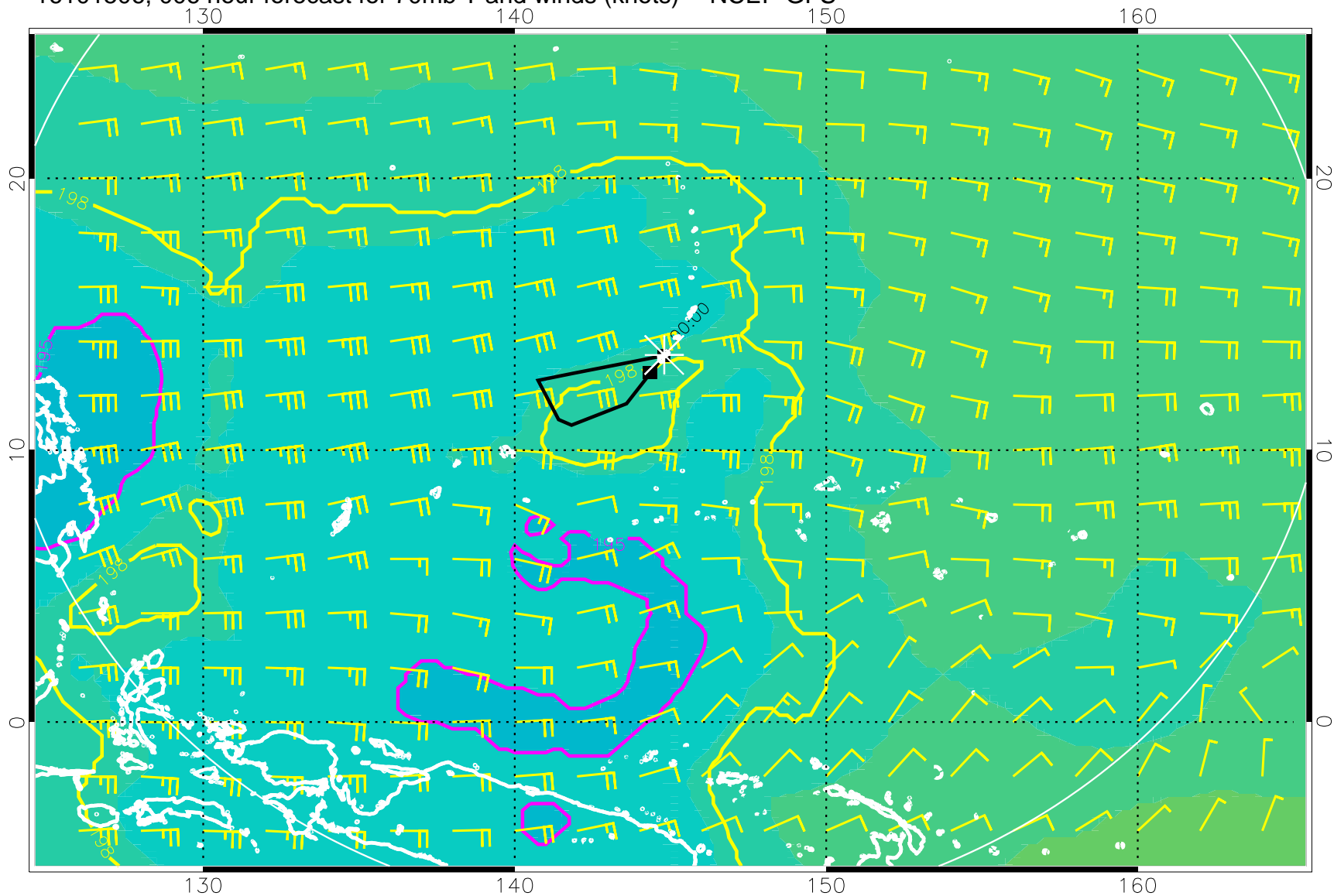
16101506, 006 hour forecast for 70mb T and winds (knots) -- NCEP GFS
