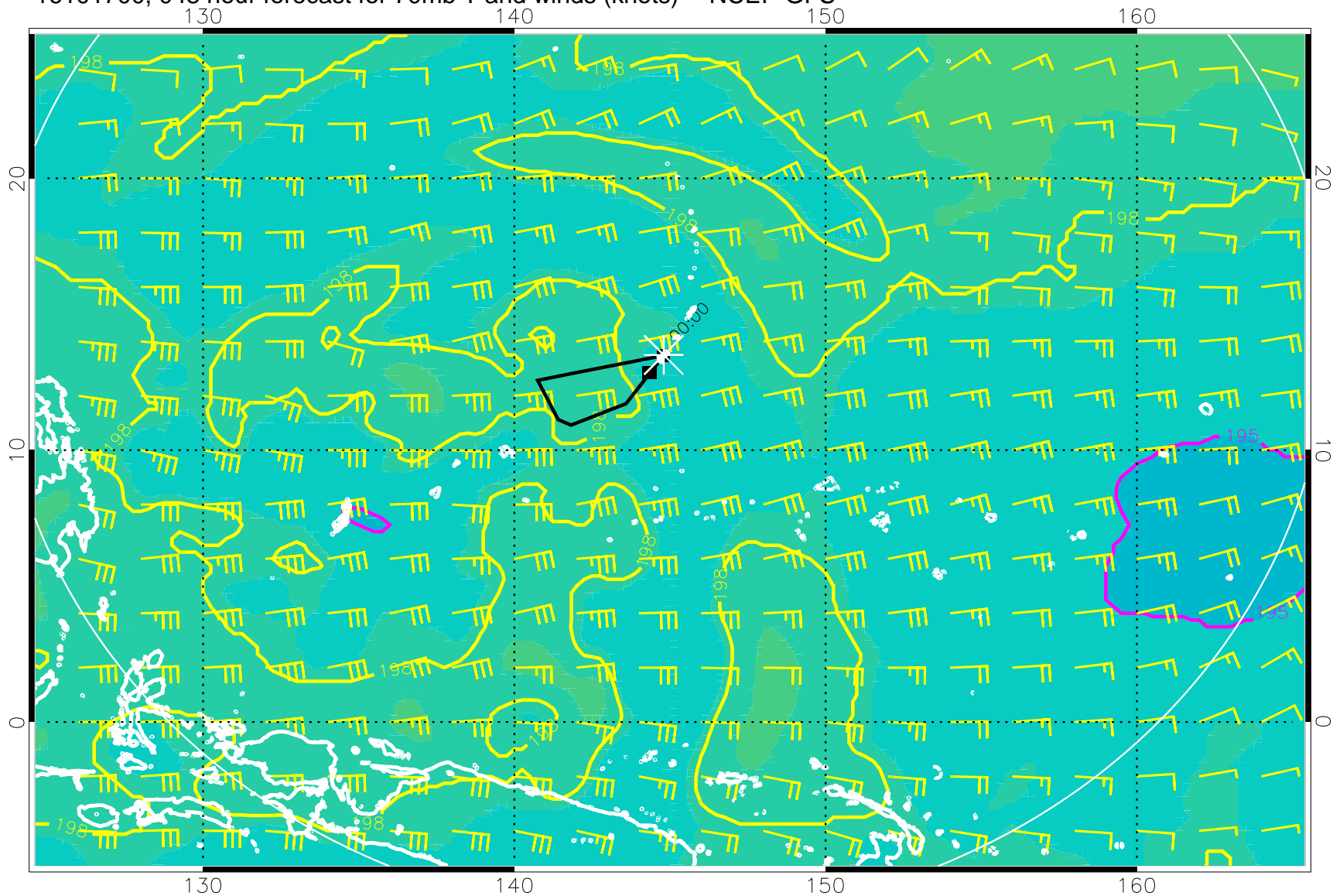
16101700, 048 hour forecast for 70mb T and winds (knots) -- NCEP GFS
