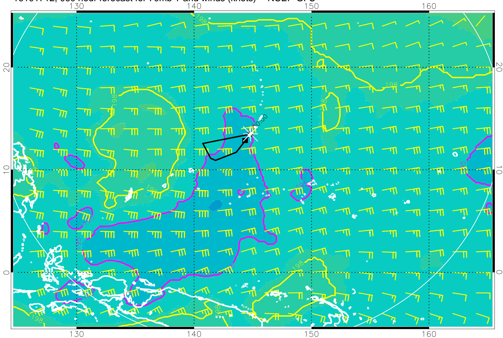
16101712, 060 hour forecast for 70mb T and winds (knots) -- NCEP GFS
