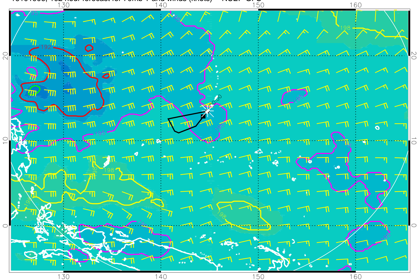
16101906, 102 hour forecast for 70mb T and winds (knots) -- NCEP GFS
