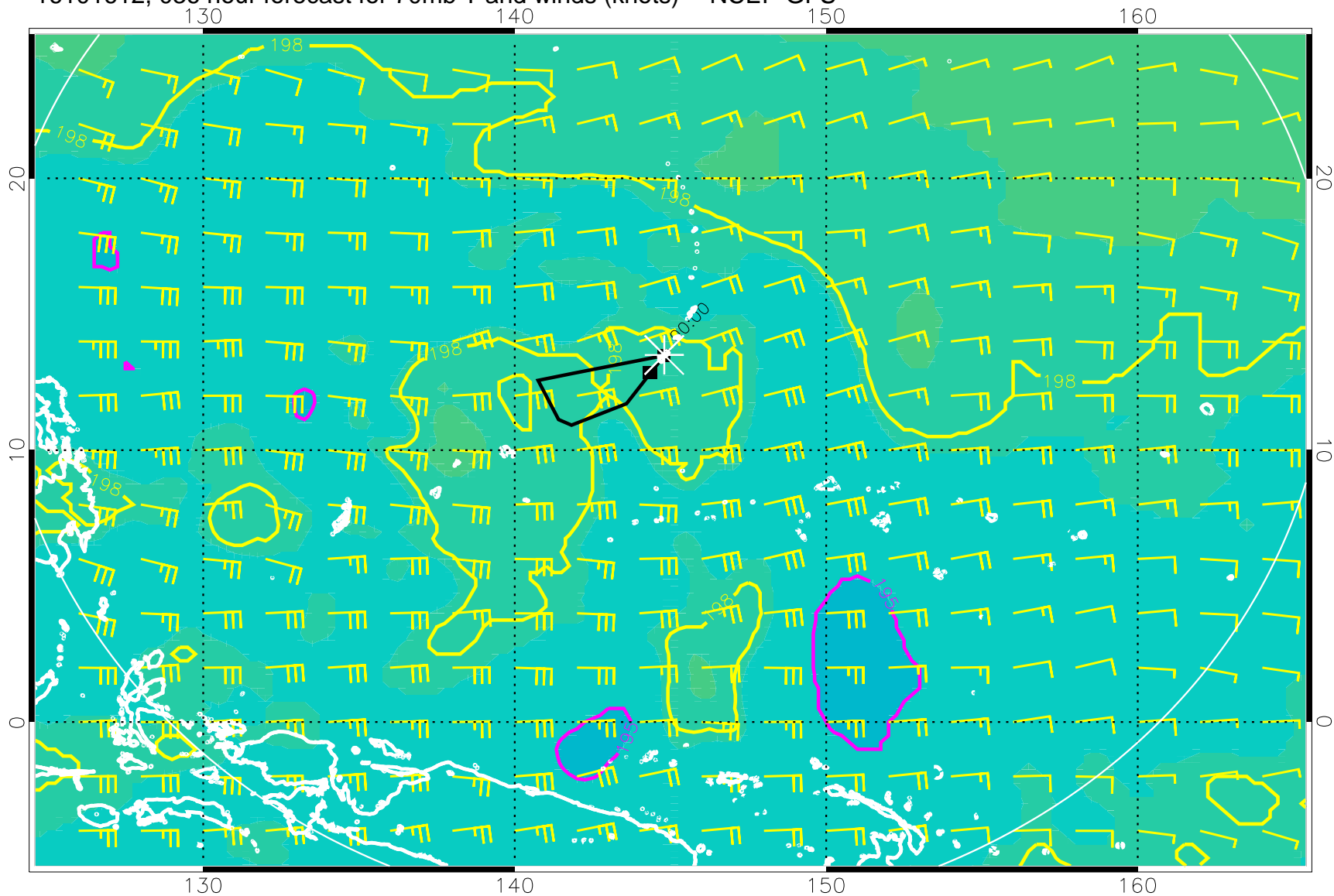
16101612, 036 hour forecast for 70mb T and winds (knots) -- NCEP GFS
