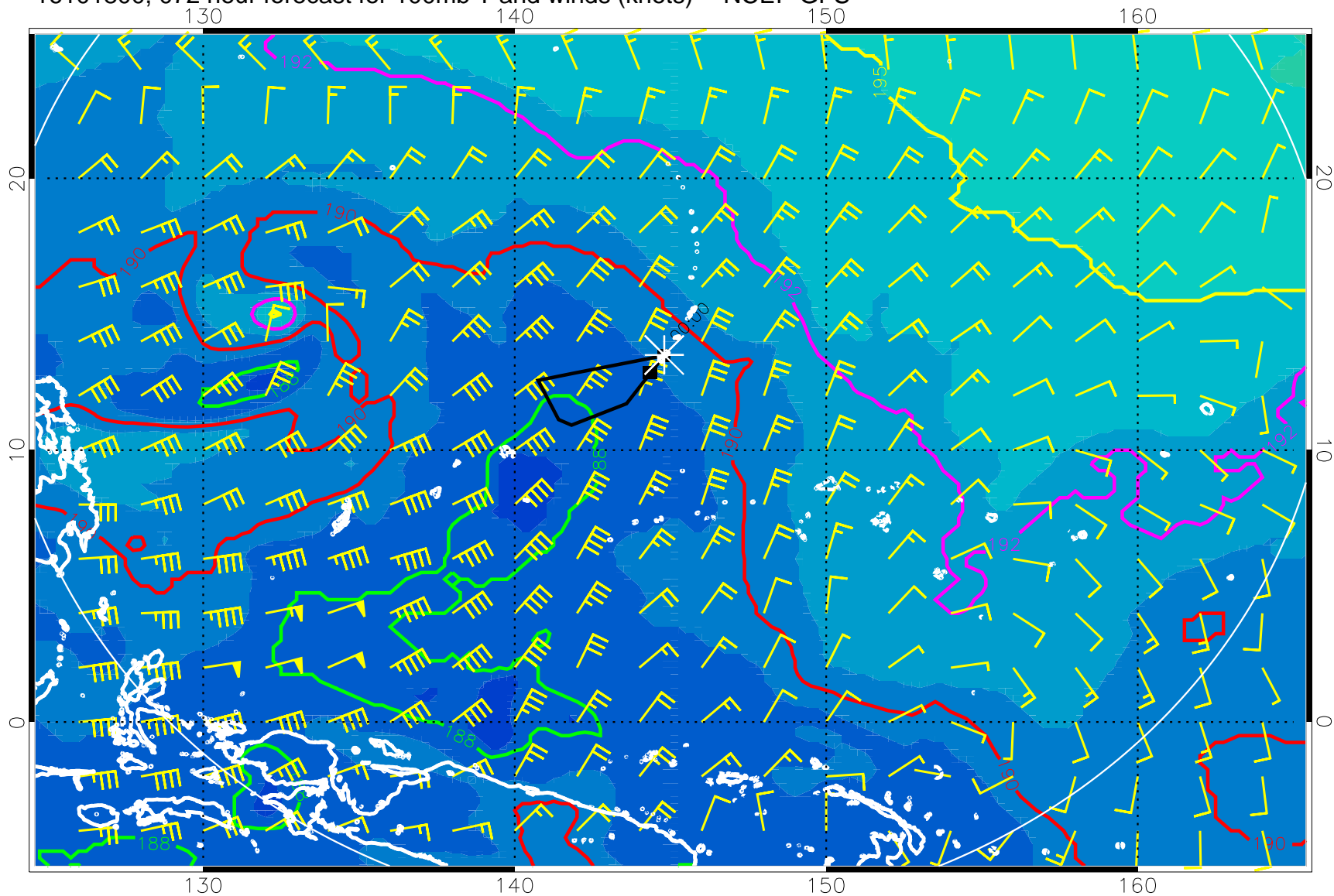
16101800, 072 hour forecast for 100mb T and winds (knots) -- NCEP GFS
