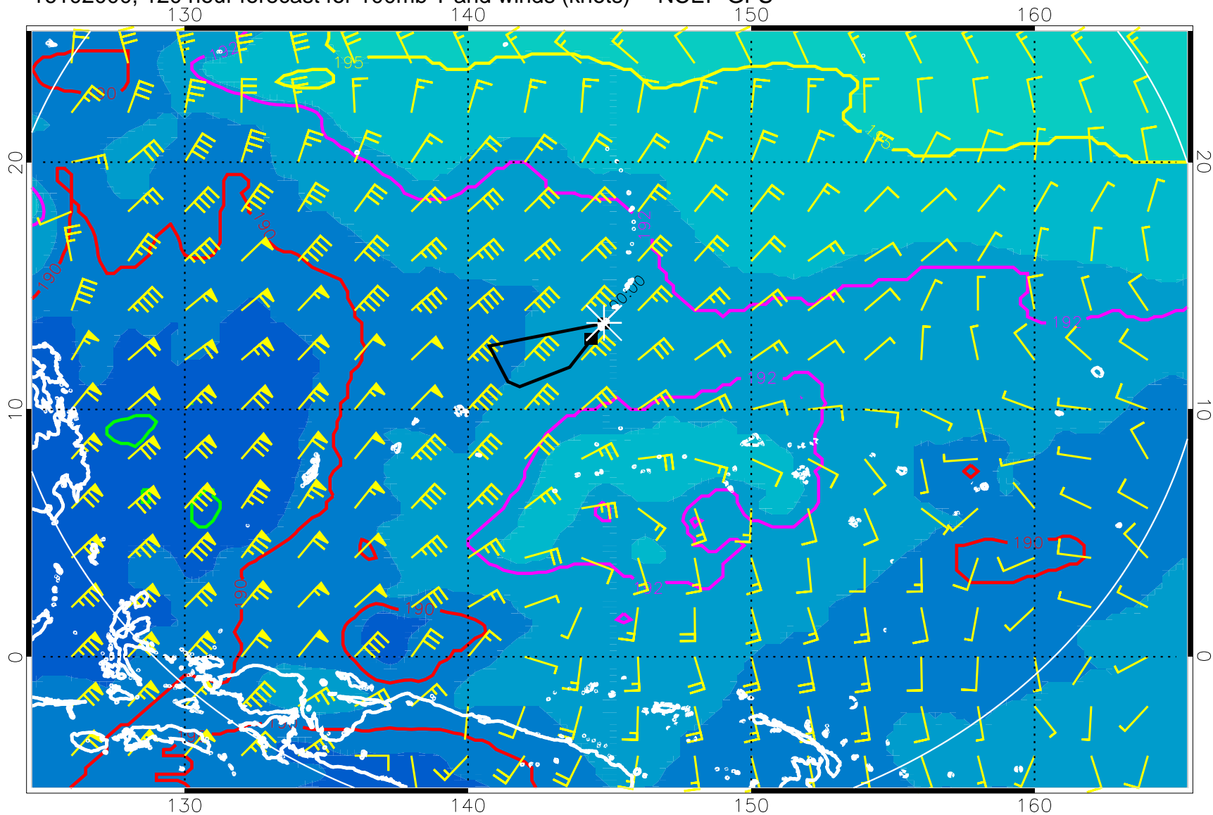
16102000, 120 hour forecast for 100mb T and winds (knots) -- NCEP GFS
