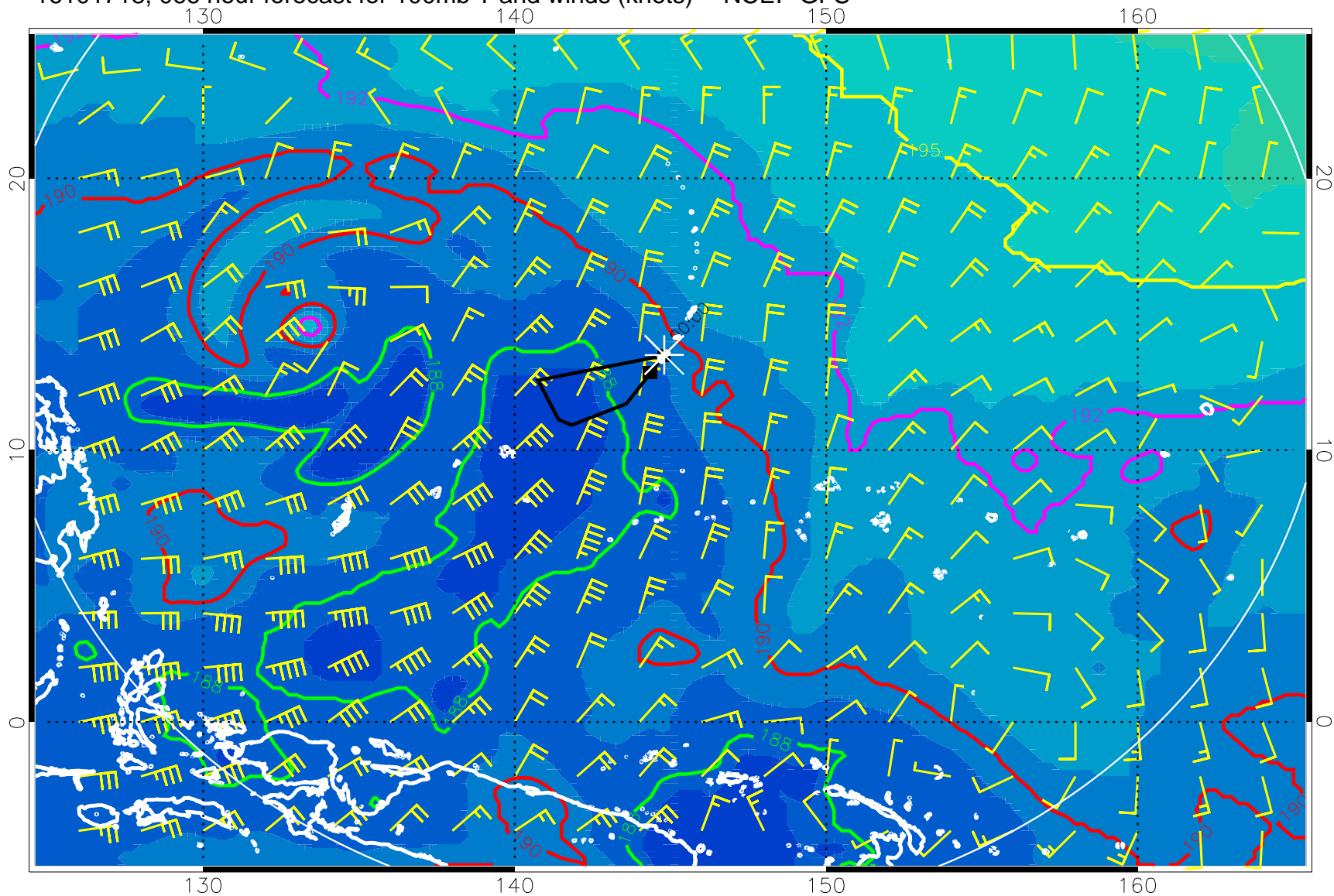
16101718, 066 hour forecast for 100mb T and winds (knots) -- NCEP GFS
