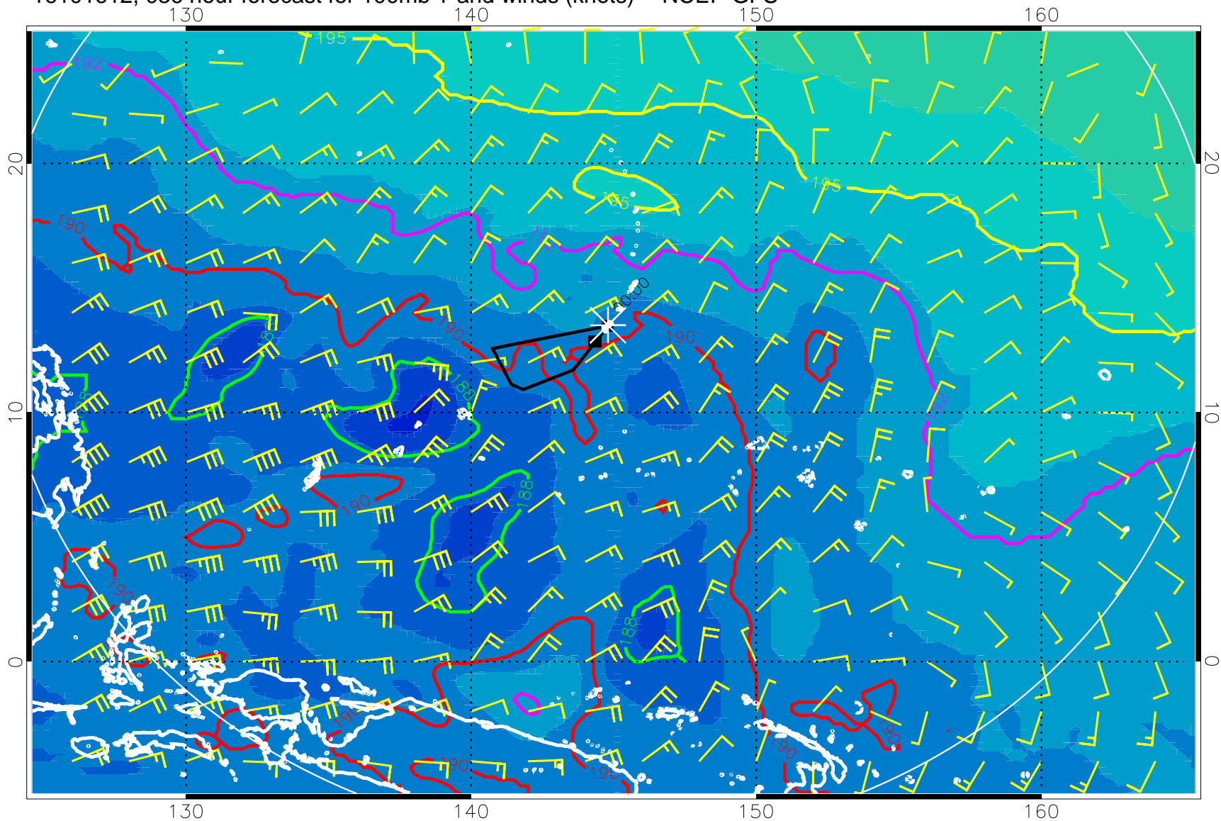
16101612, 036 hour forecast for 100mb T and winds (knots) -- NCEP GFS
