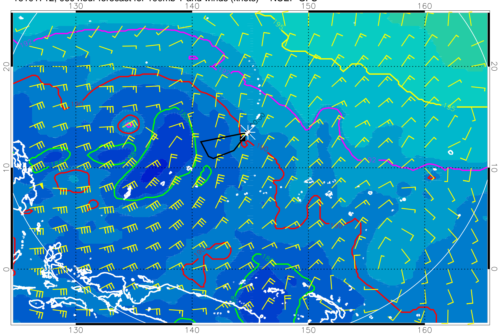
16101712, 060 hour forecast for 100mb T and winds (knots) -- NCEP GFS
