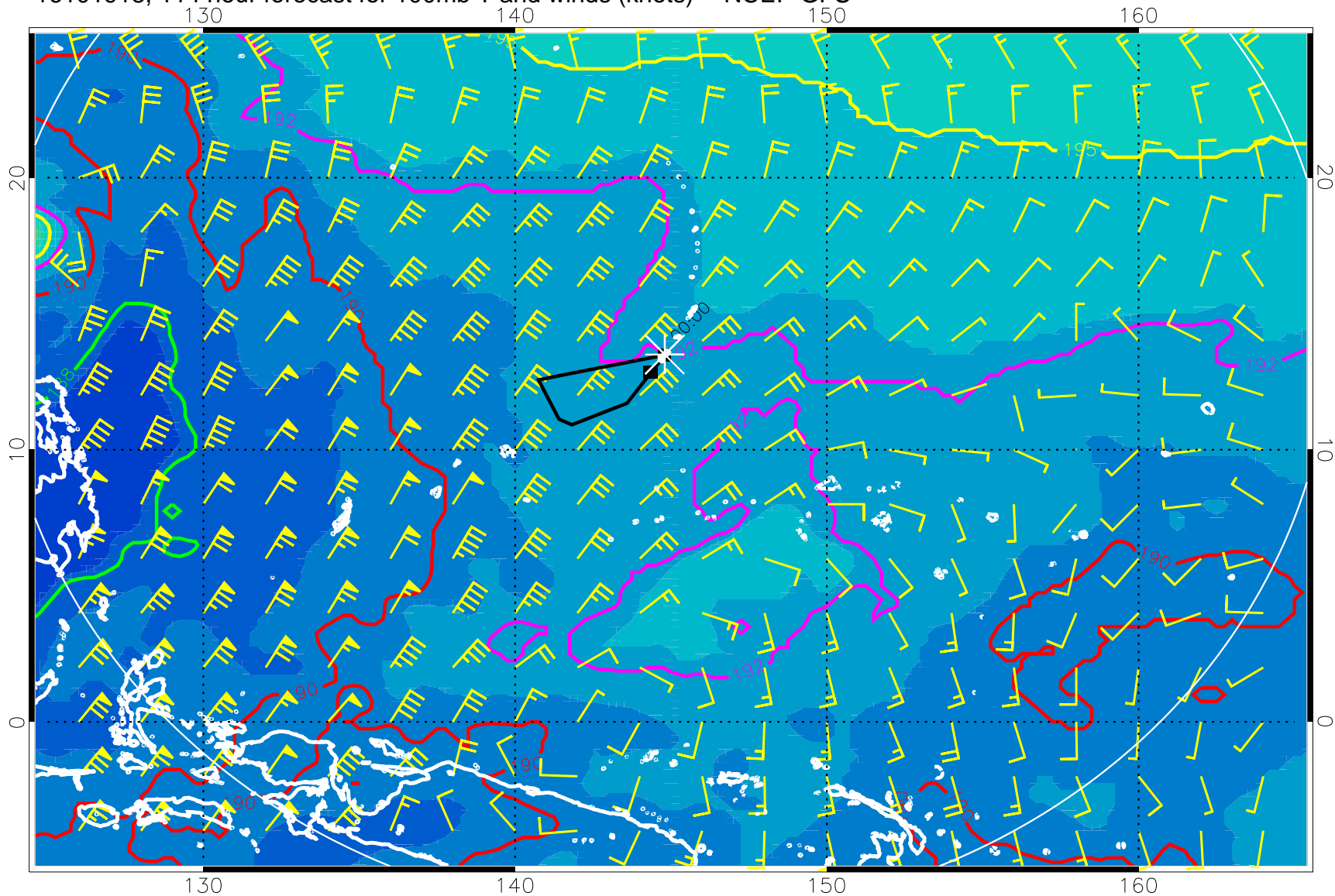
16101918, 114 hour forecast for 100mb T and winds (knots) -- NCEP GFS
