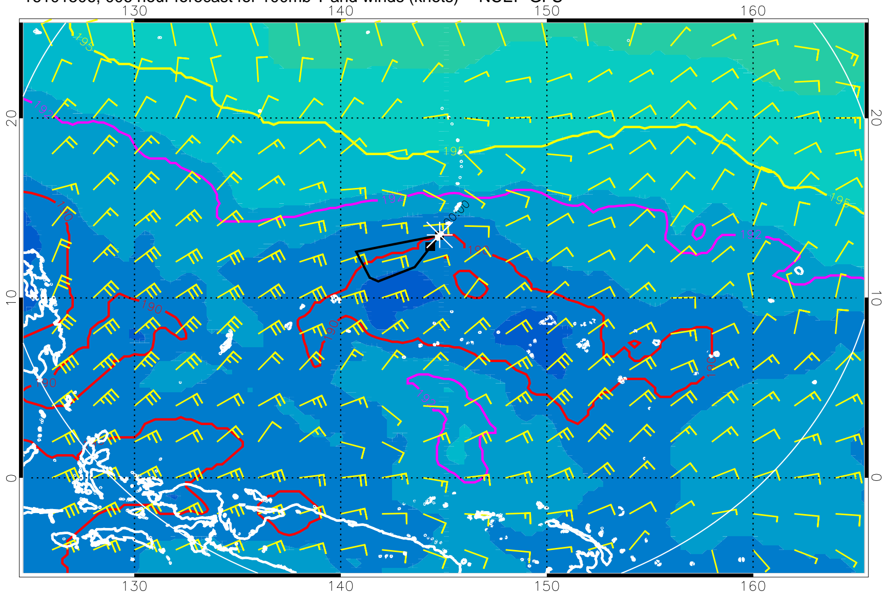
16101506, 006 hour forecast for 100mb T and winds (knots) -- NCEP GFS
