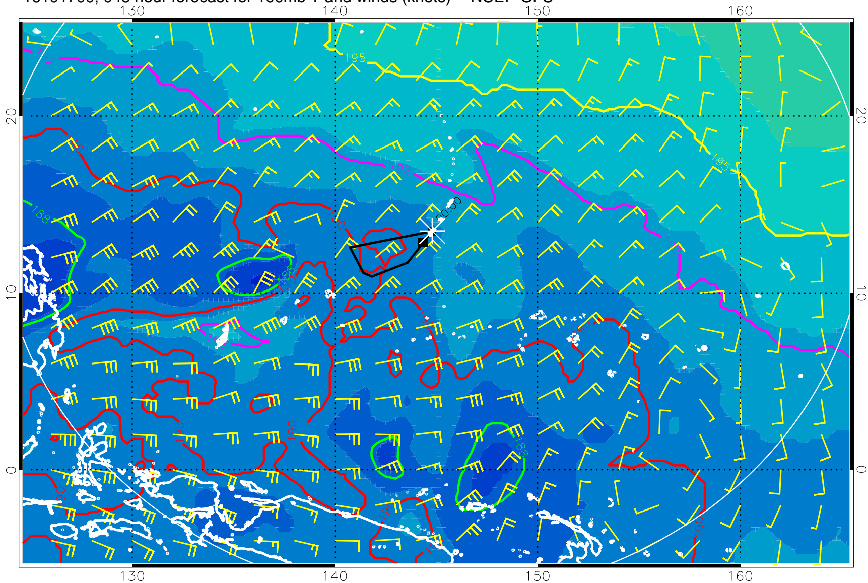
16101700, 048 hour forecast for 100mb T and winds (knots) -- NCEP GFS
