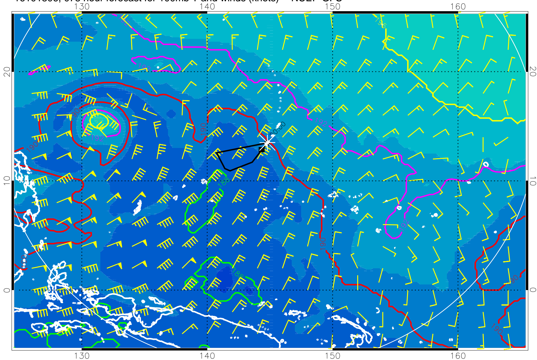
16101806, 078 hour forecast for 100mb T and winds (knots) -- NCEP GFS
