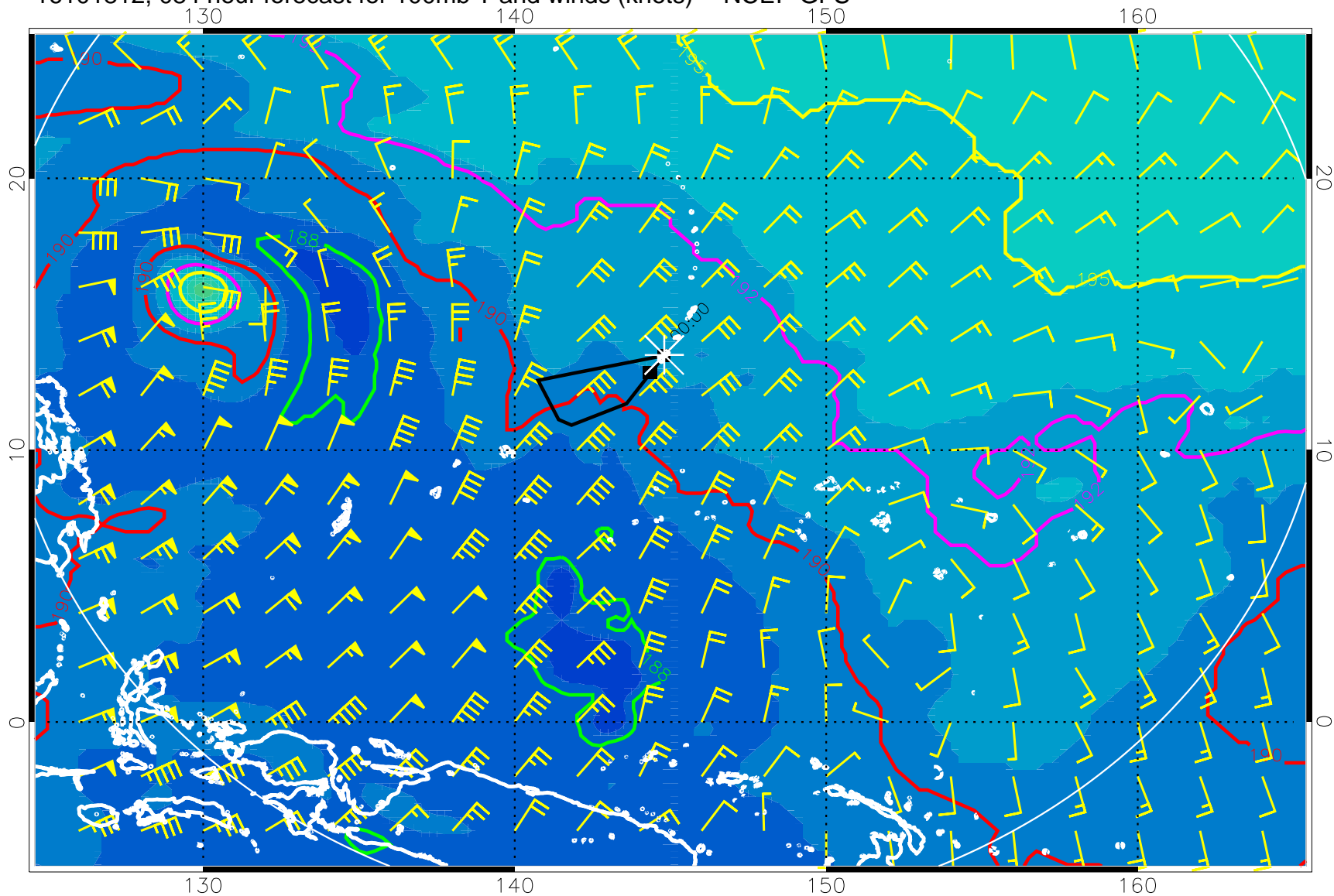
16101812, 084 hour forecast for 100mb T and winds (knots) -- NCEP GFS
