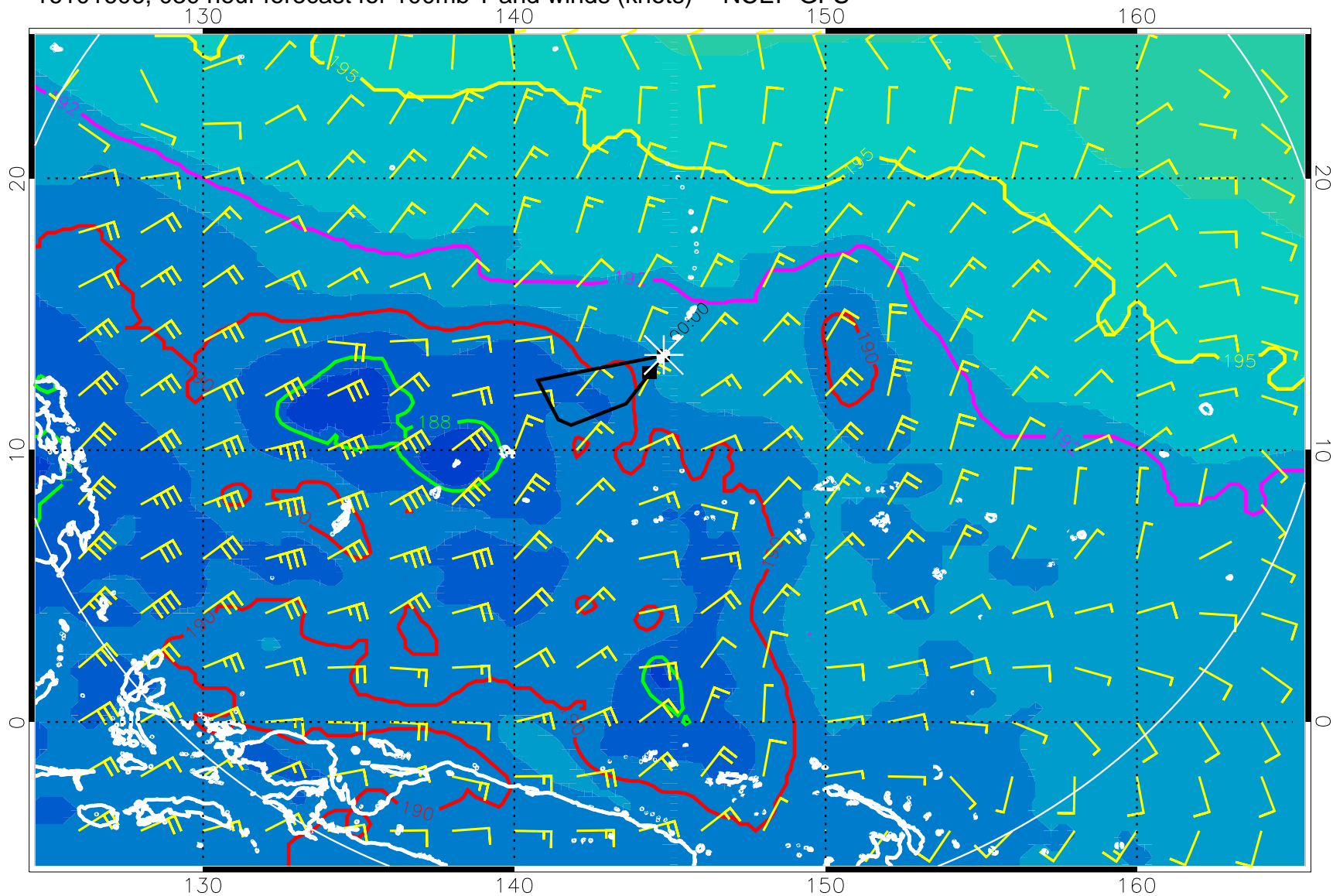
16101606, 030 hour forecast for 100mb T and winds (knots) -- NCEP GFS
