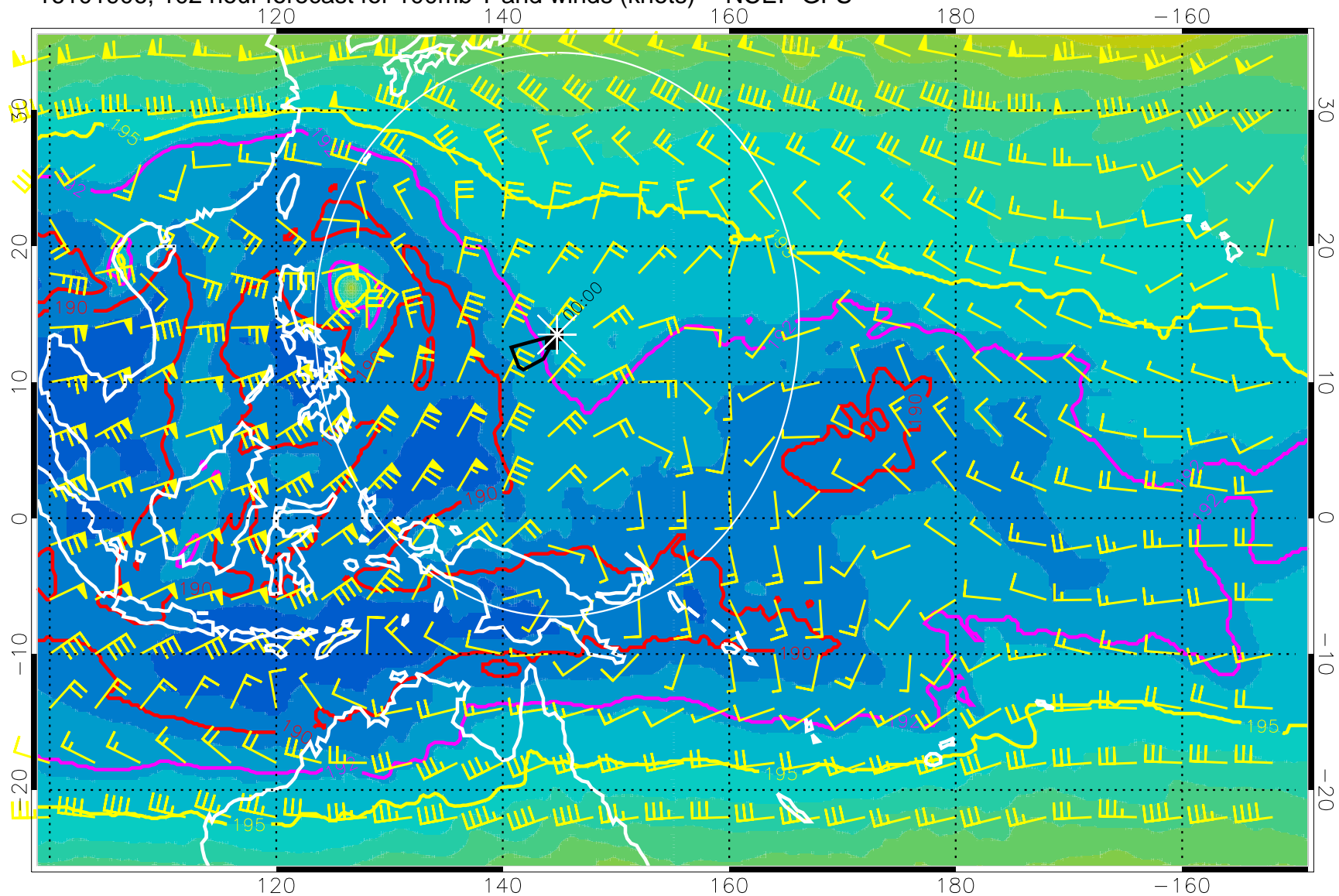
16101906, 102 hour forecast for 100mb T and winds (knots) -- NCEP GFS
