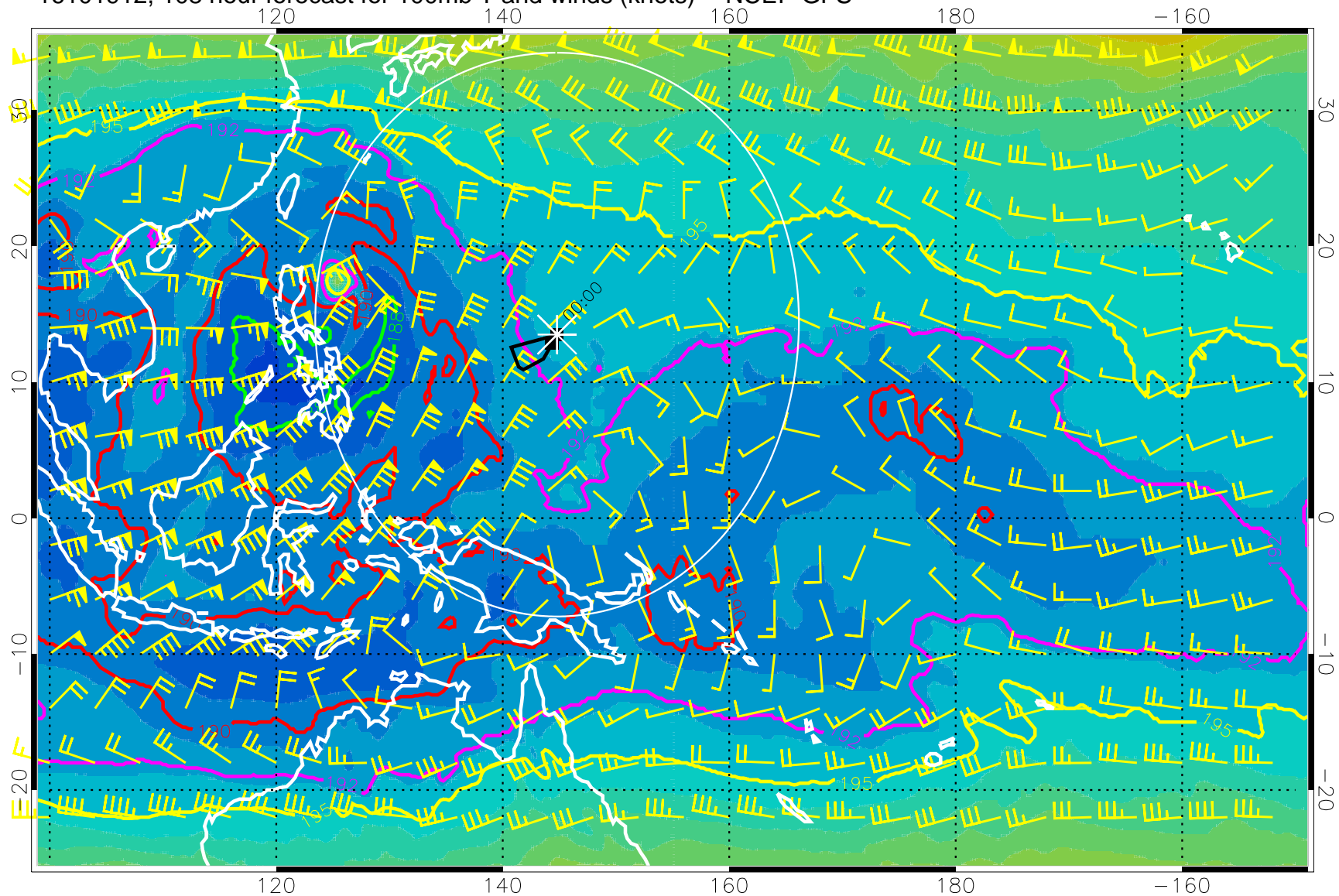
16101912, 108 hour forecast for 100mb T and winds (knots) -- NCEP GFS
