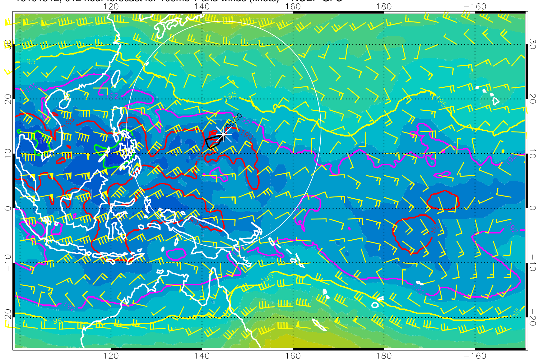
16101512, 012 hour forecast for 100mb T and winds (knots) -- NCEP GFS
