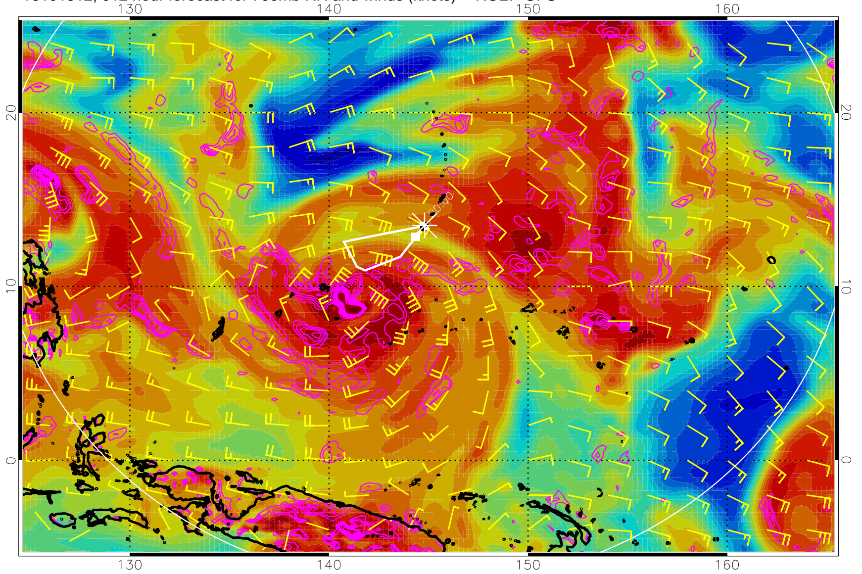
16101512, 012 hour forecast for 700mb RH and winds (knots) -- NCEP GFS
