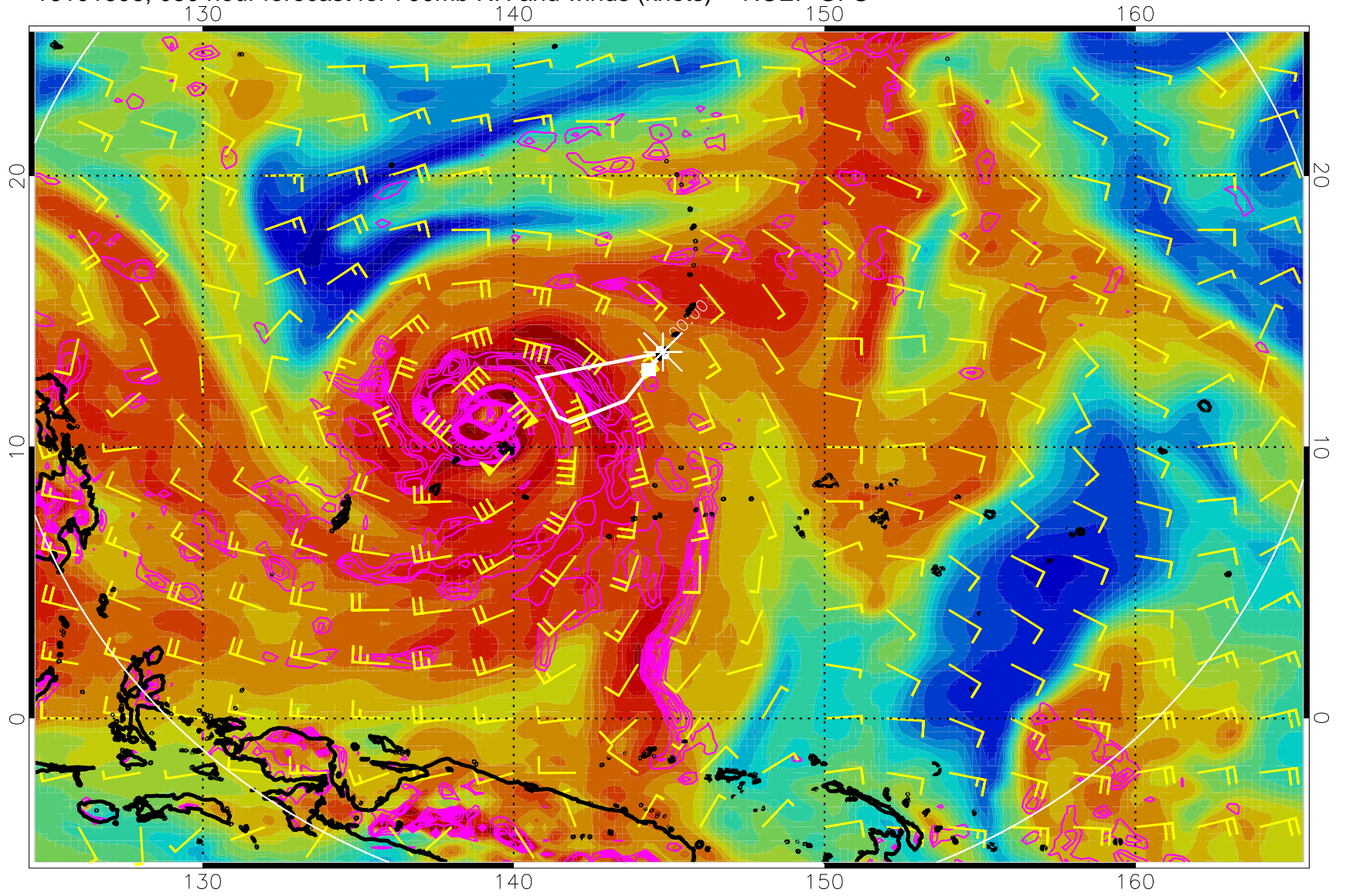
16101606, 030 hour forecast for 700mb RH and winds (knots) -- NCEP GFS
