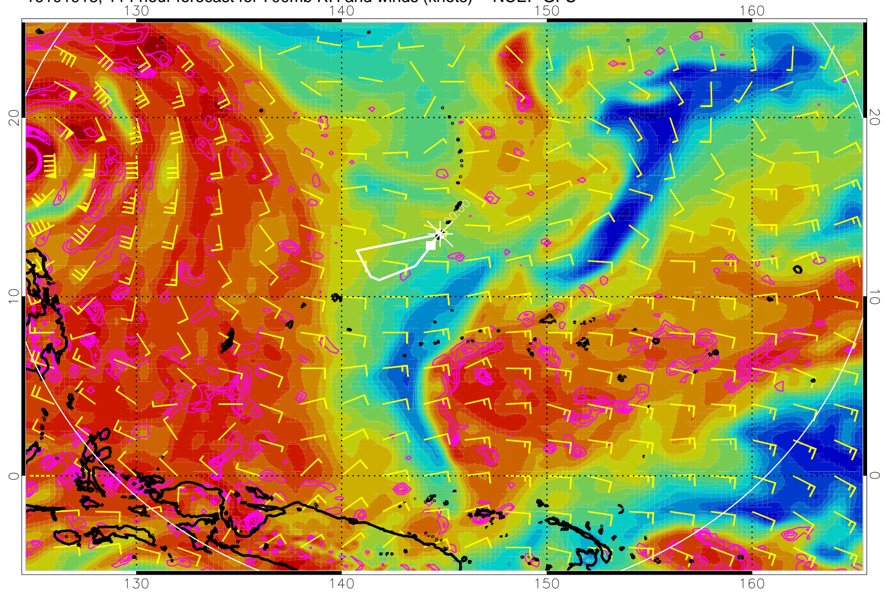
16101918, 114 hour forecast for 700mb RH and winds (knots) -- NCEP GFS
