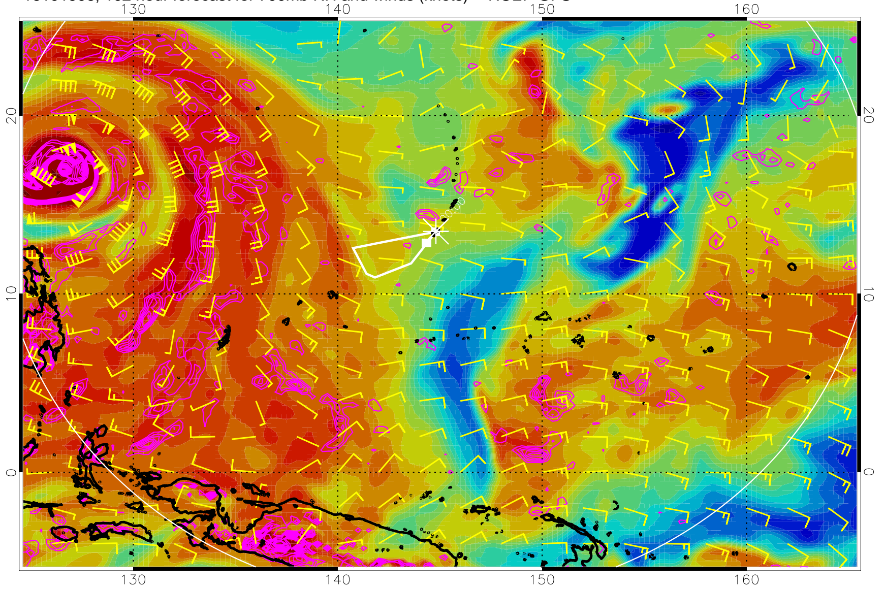
16101906, 102 hour forecast for 700mb RH and winds (knots) -- NCEP GFS
