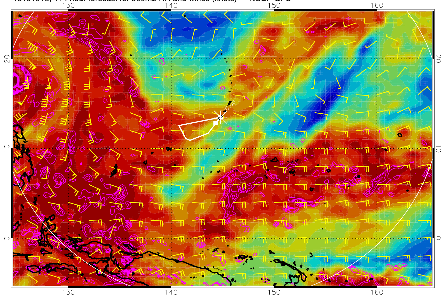
16101918, 114 hour forecast for 500mb RH and winds (knots) -- NCEP GFS
