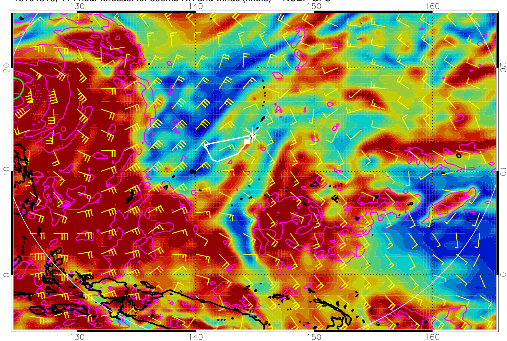
16101918, 114 hour forecast for 300mb RH and winds (knots) -- NCEP GFS
