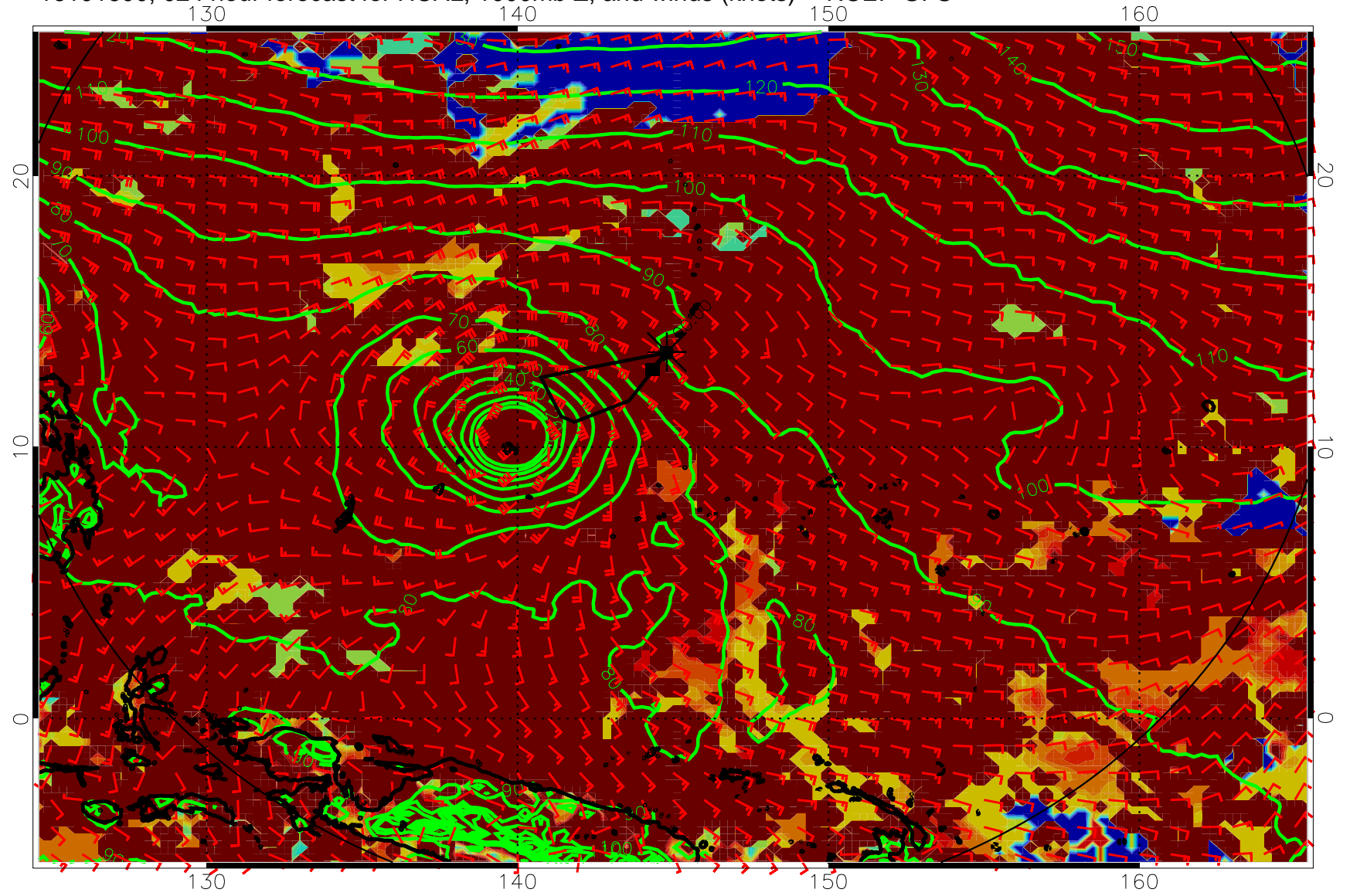
16101600, 024 hour forecast for HCAL, 1000mb Z, and winds (knots) -- NCEP GFS
