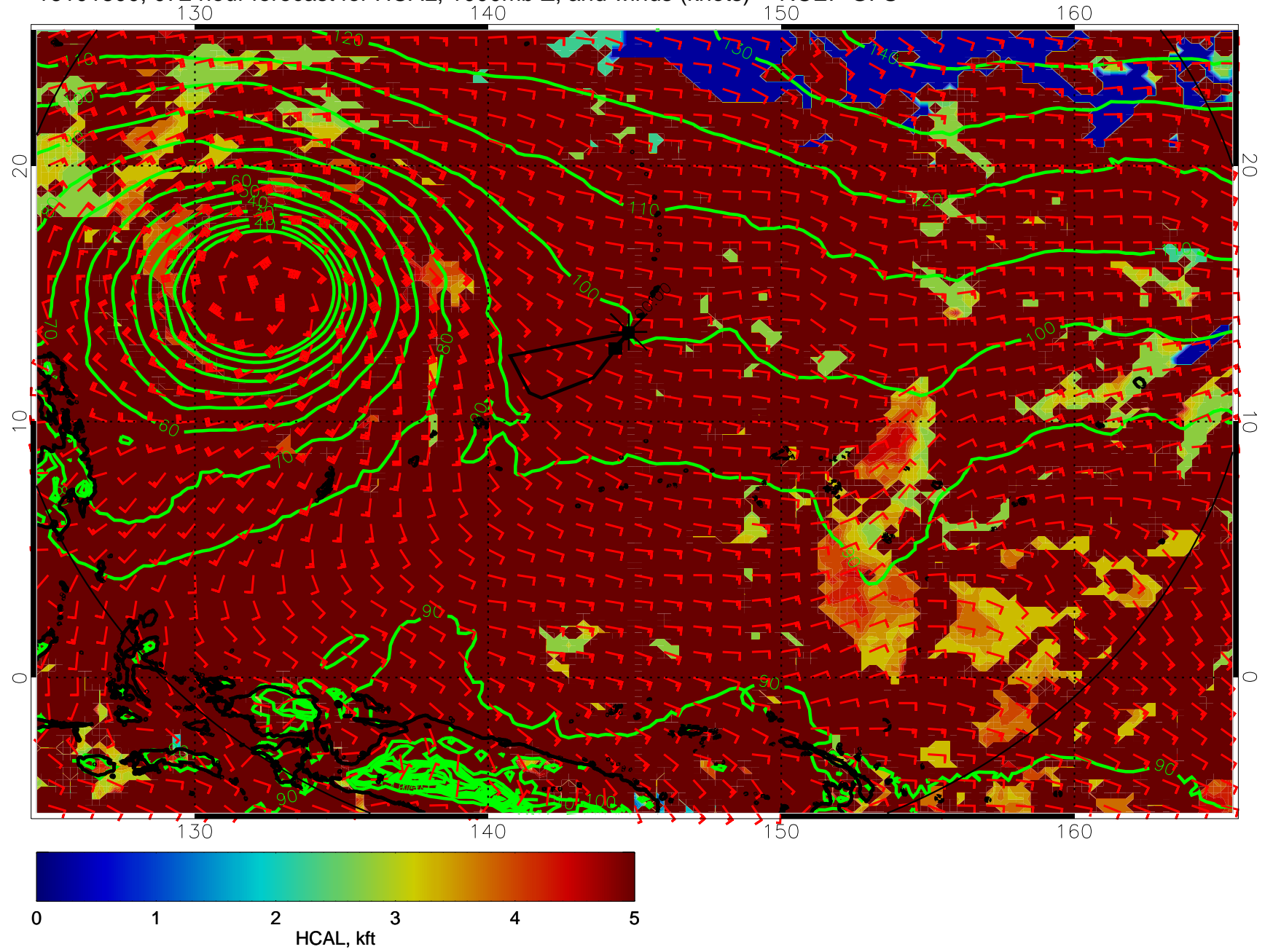
16101800, 072 hour forecast for HCAL, 1000mb Z, and winds (knots) -- NCEP GFS
