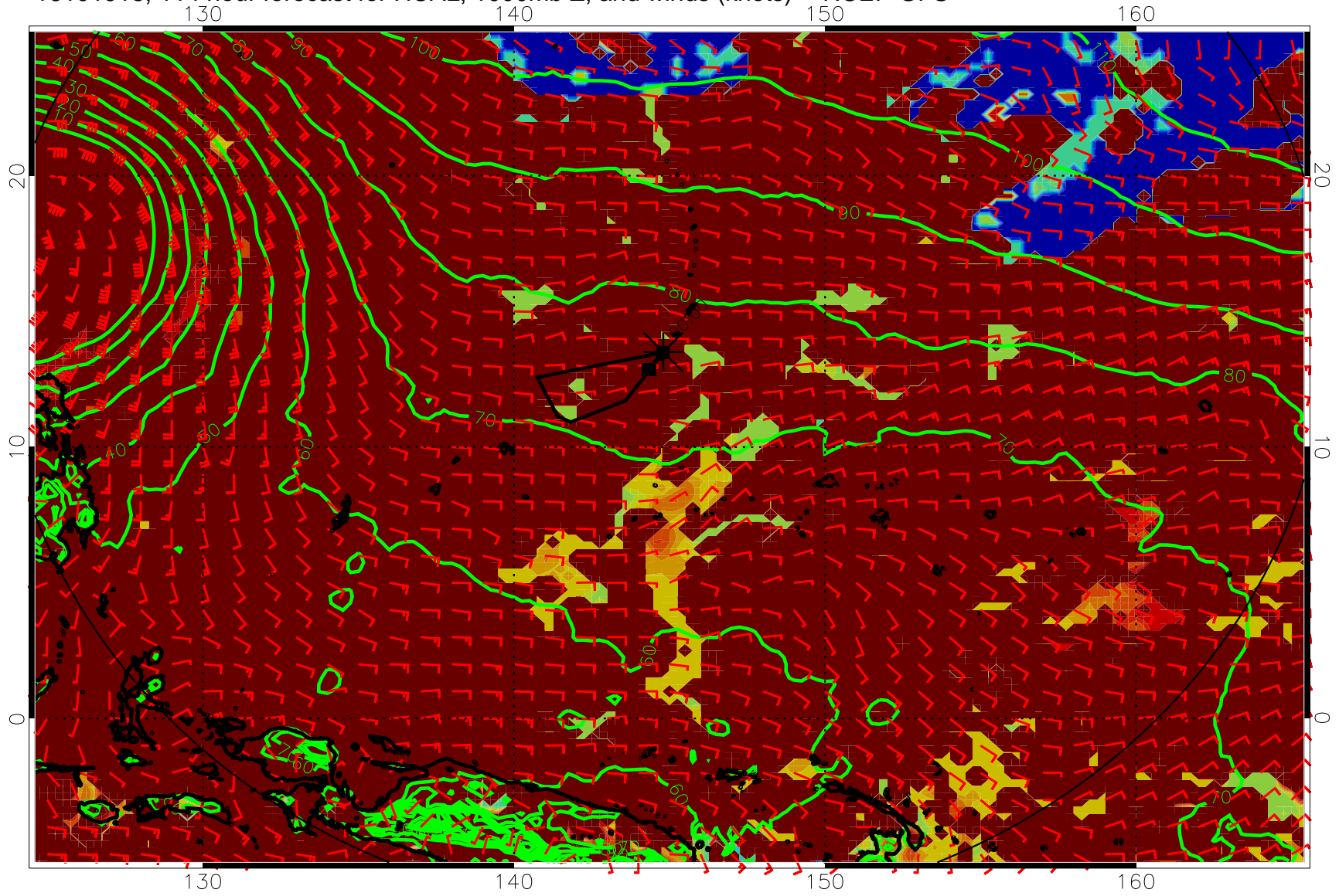
16101918, 114 hour forecast for HCAL, 1000mb Z, and winds (knots) -- NCEP GFS
