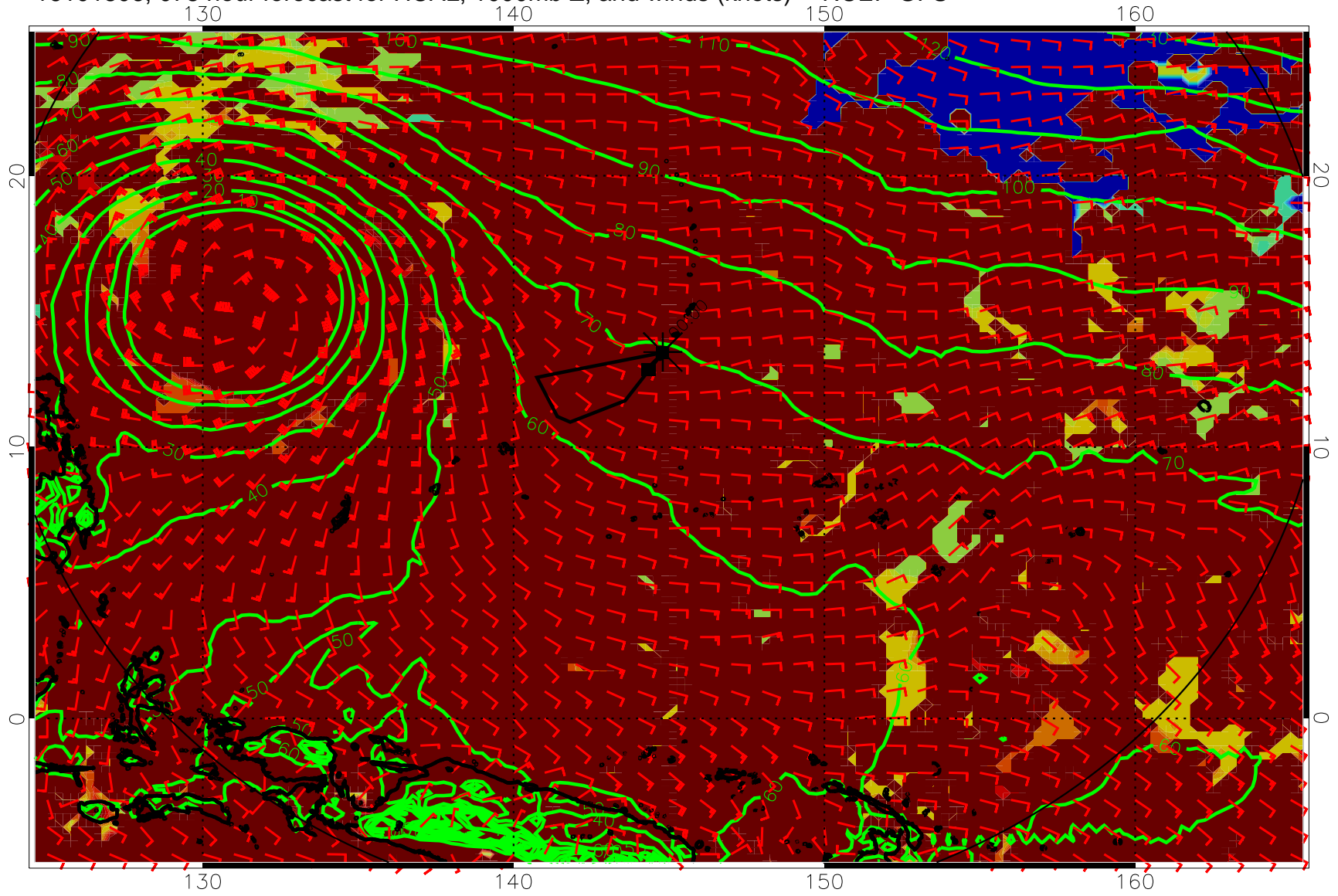
16101806, 078 hour forecast for HCAL, 1000mb Z, and winds (knots) -- NCEP GFS
