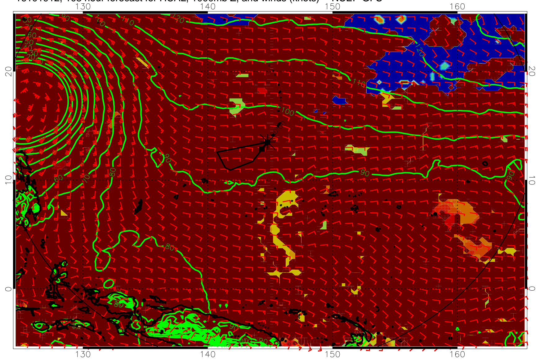
16101912, 108 hour forecast for HCAL, 1000mb Z, and winds (knots) -- NCEP GFS
