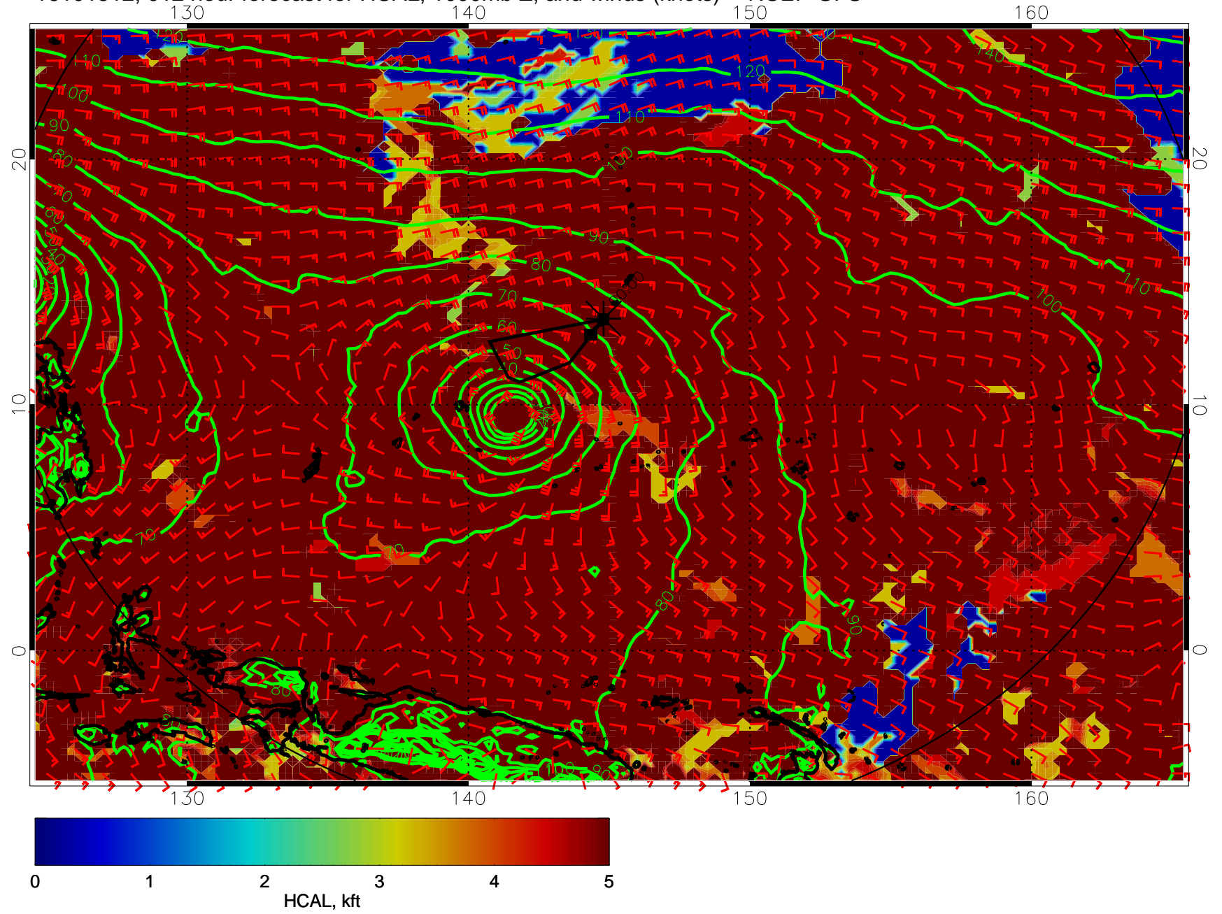
16101512, 012 hour forecast for HCAL, 1000mb Z, and winds (knots) -- NCEP GFS
