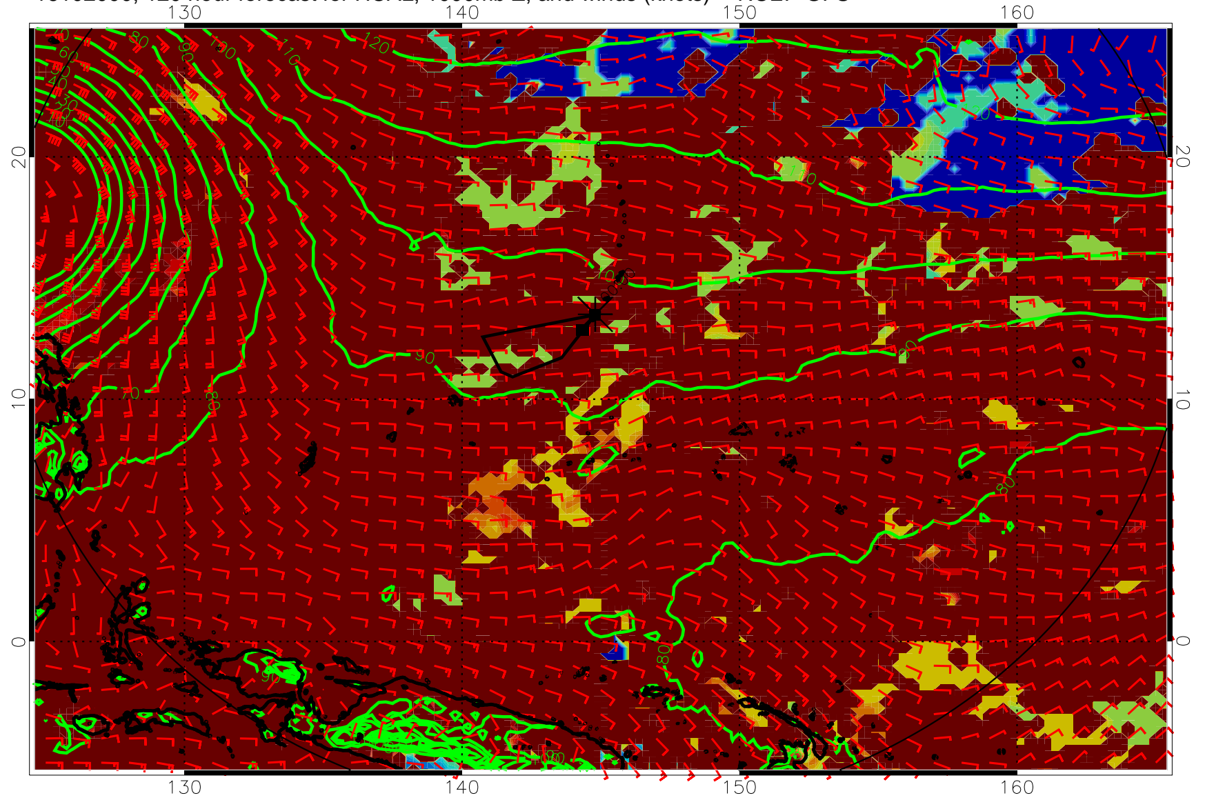
16102000, 120 hour forecast for HCAL, 1000mb Z, and winds (knots) -- NCEP GFS
