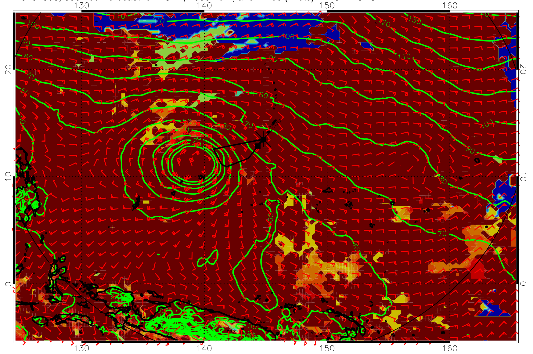
16101606, 030 hour forecast for HCAL, 1000mb Z, and winds (knots) -- NCEP GFS
