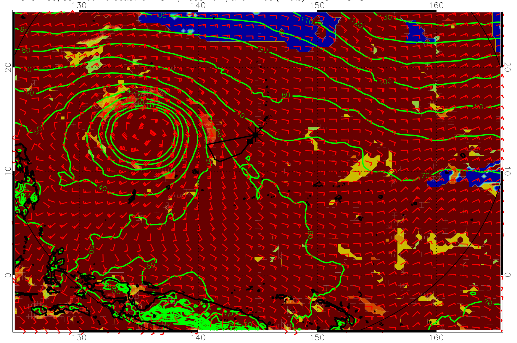
16101706, 054 hour forecast for HCAL, 1000mb Z, and winds (knots) -- NCEP GFS
