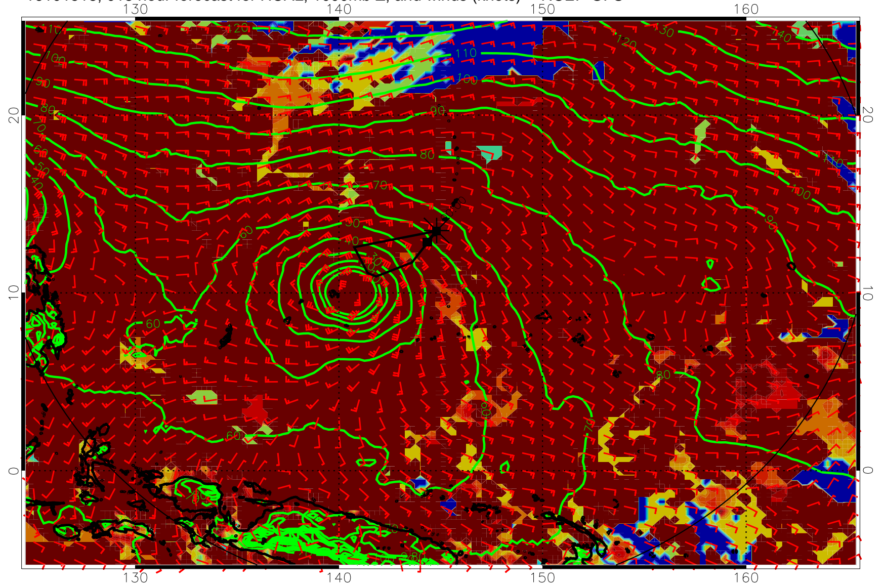
16101518, 018 hour forecast for HCAL, 1000mb Z, and winds (knots) -- NCEP GFS
