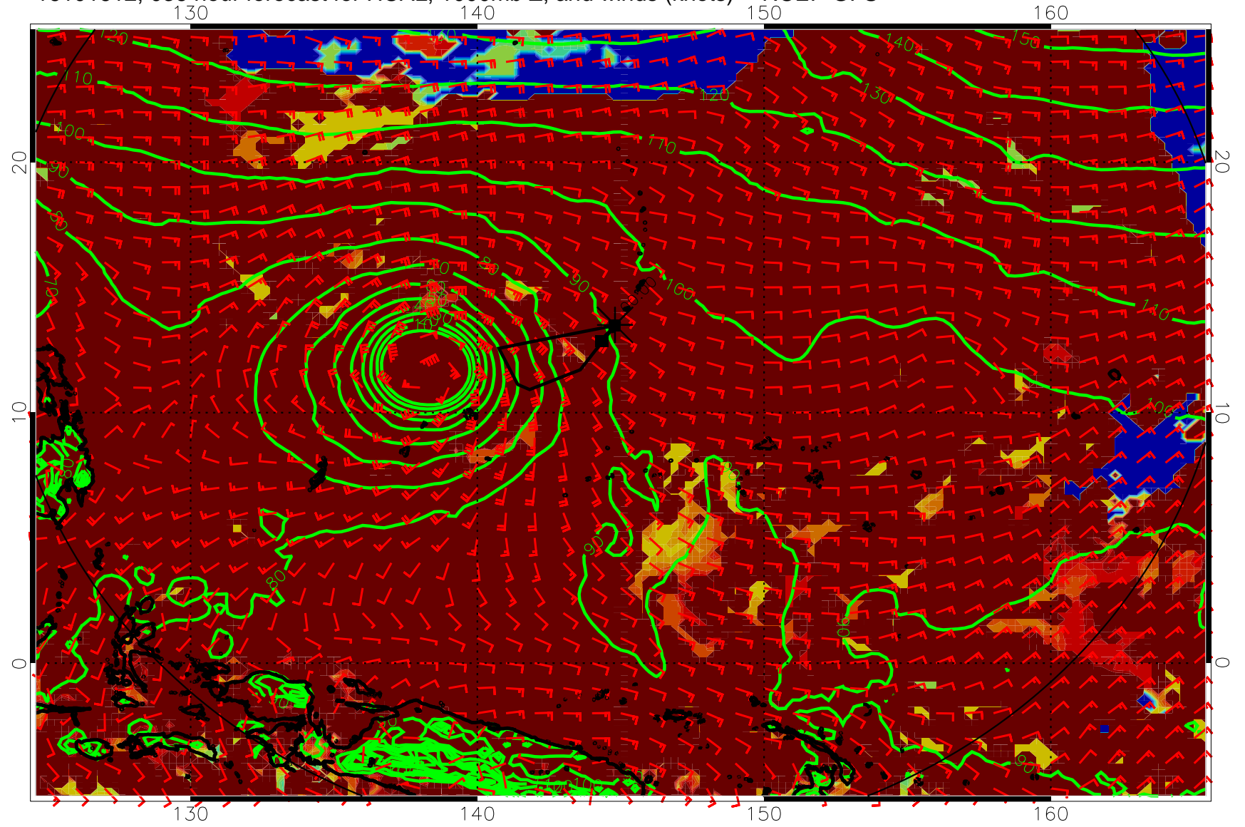
16101612, 036 hour forecast for HCAL, 1000mb Z, and winds (knots) -- NCEP GFS
