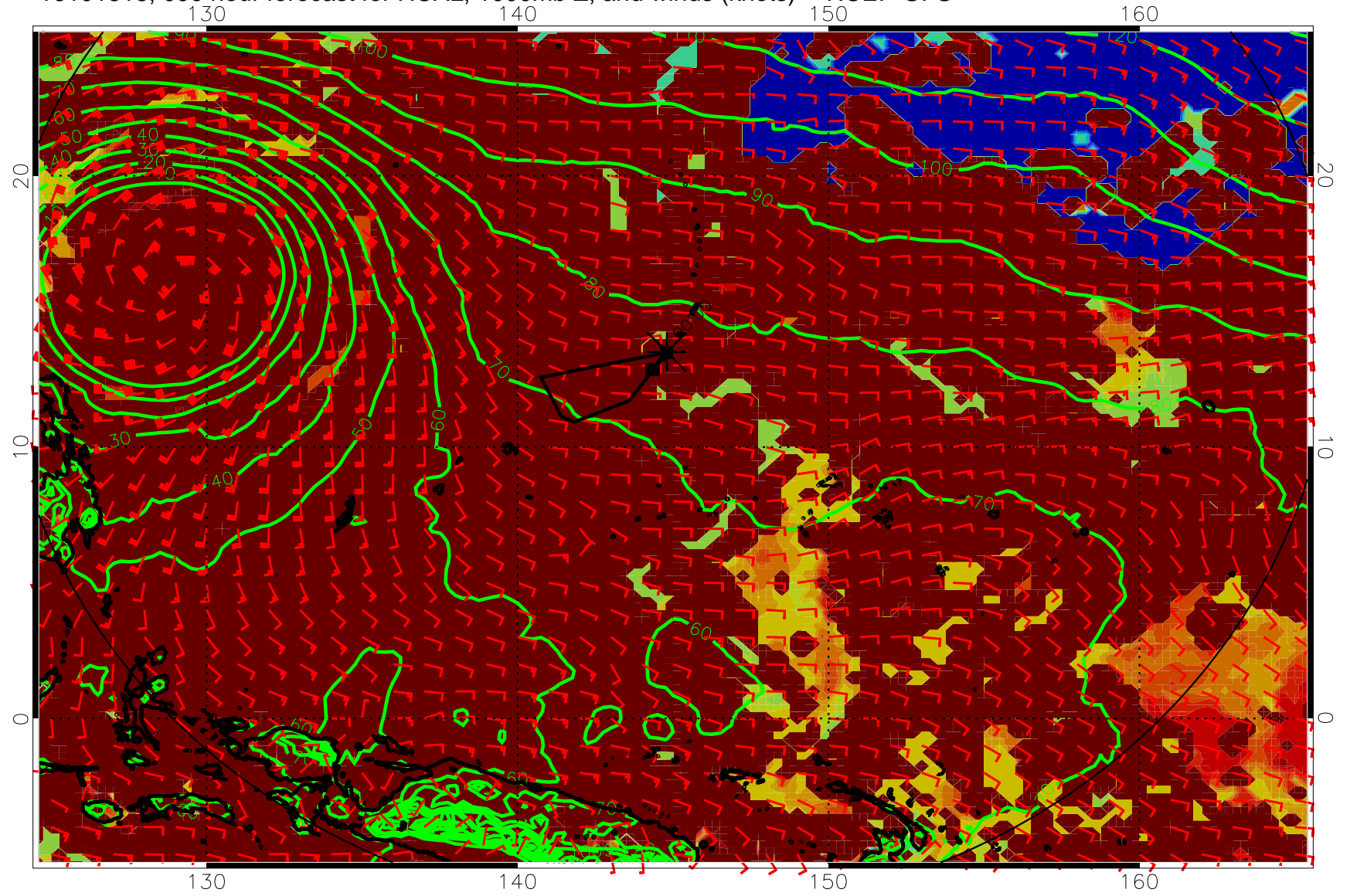
16101818, 090 hour forecast for HCAL, 1000mb Z, and winds (knots) -- NCEP GFS
