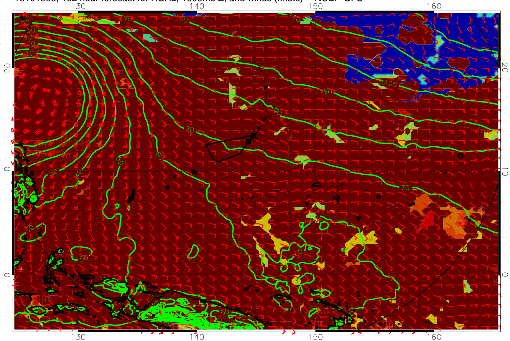
16101906, 102 hour forecast for HCAL, 1000mb Z, and winds (knots) -- NCEP GFS
