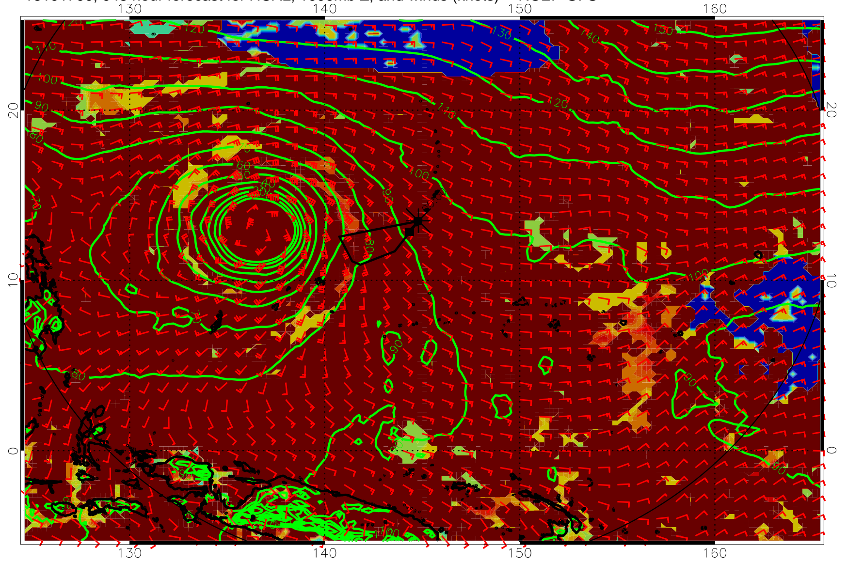
16101700, 048 hour forecast for HCAL, 1000mb Z, and winds (knots) -- NCEP GFS
