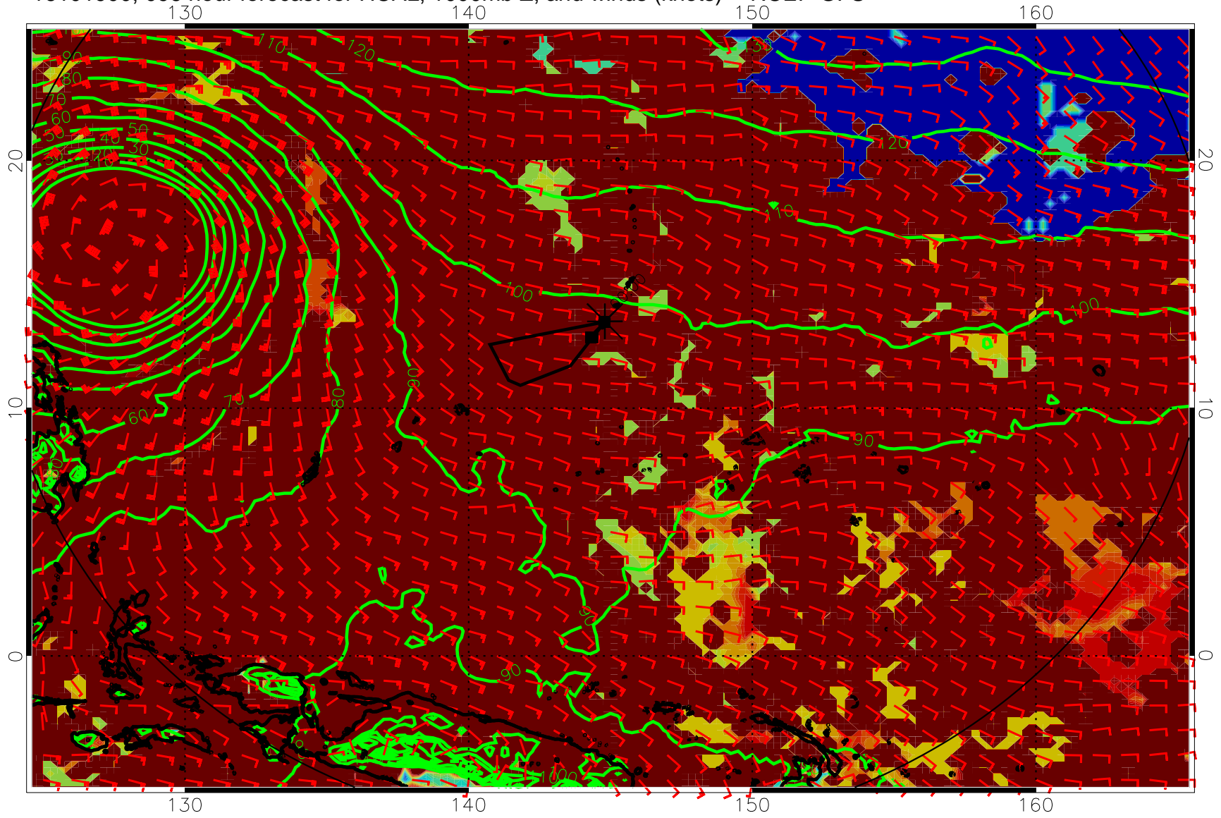
16101900, 096 hour forecast for HCAL, 1000mb Z, and winds (knots) -- NCEP GFS
