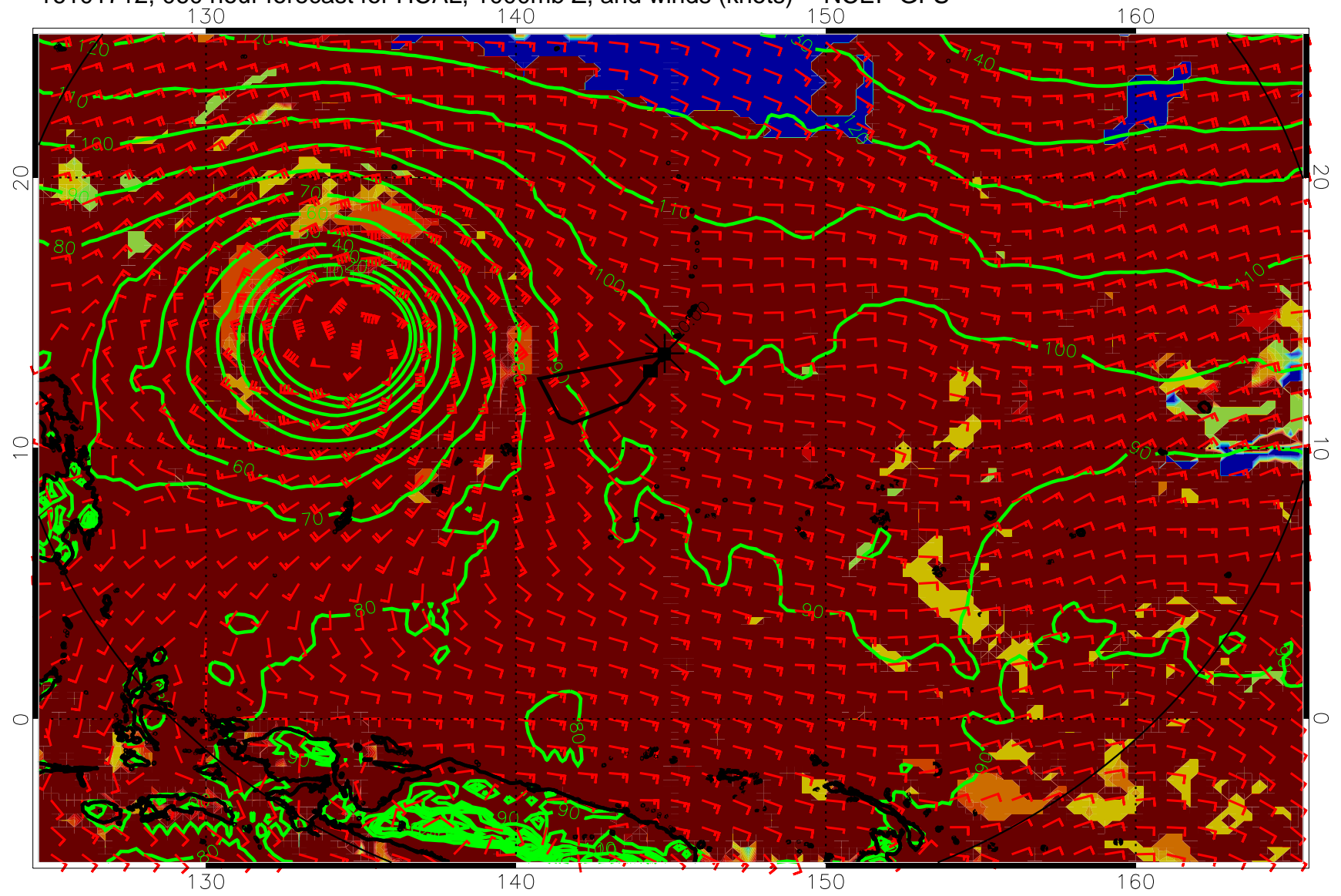
16101712, 060 hour forecast for HCAL, 1000mb Z, and winds (knots) -- NCEP GFS
