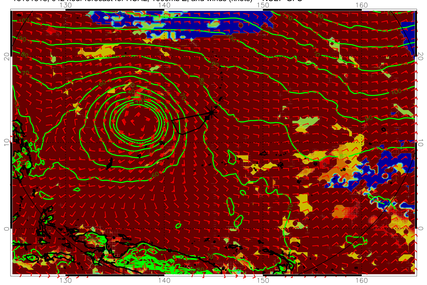
16101618, 042 hour forecast for HCAL, 1000mb Z, and winds (knots) -- NCEP GFS
