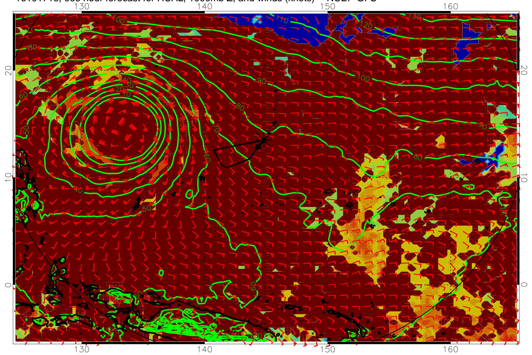
16101718, 066 hour forecast for HCAL, 1000mb Z, and winds (knots) -- NCEP GFS
