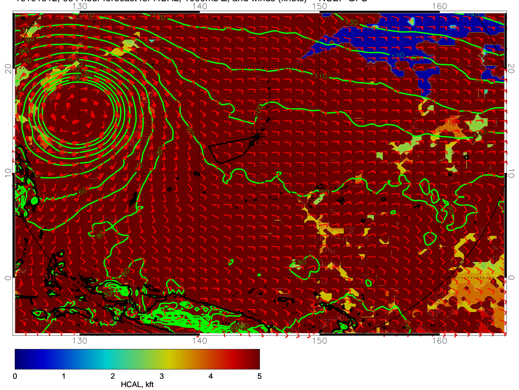
16101812, 084 hour forecast for HCAL, 1000mb Z, and winds (knots) -- NCEP GFS
