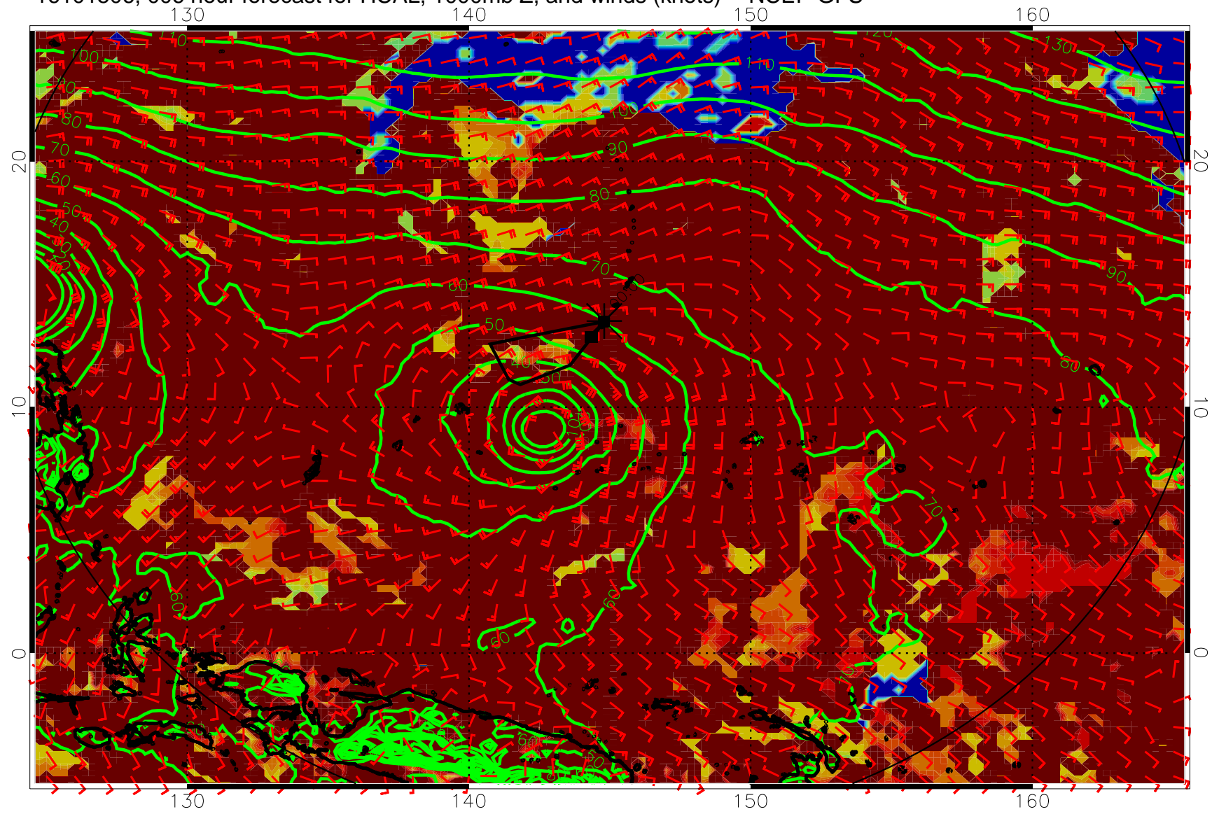
16101506, 006 hour forecast for HCAL, 1000mb Z, and winds (knots) -- NCEP GFS
