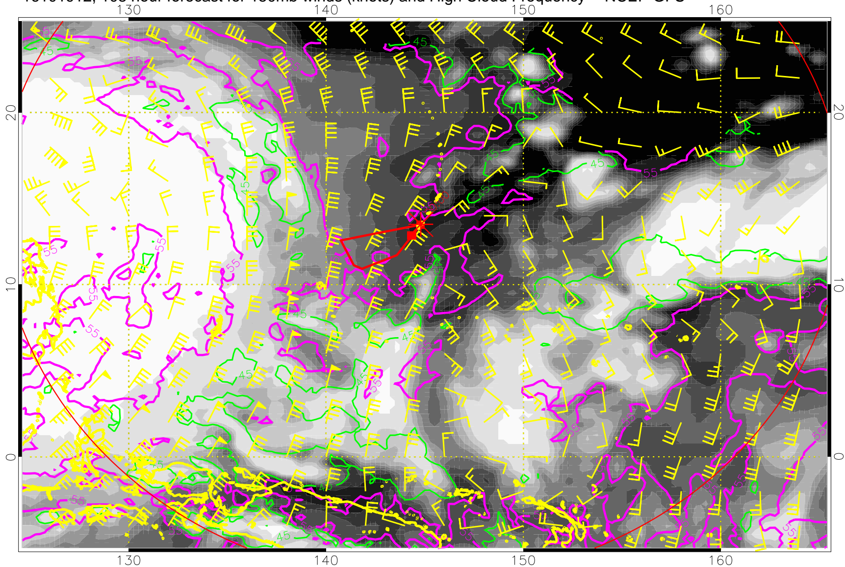
16101912, 108 hour forecast for 150mb winds (knots) and High Cloud Frequency -- NCEP GFS
