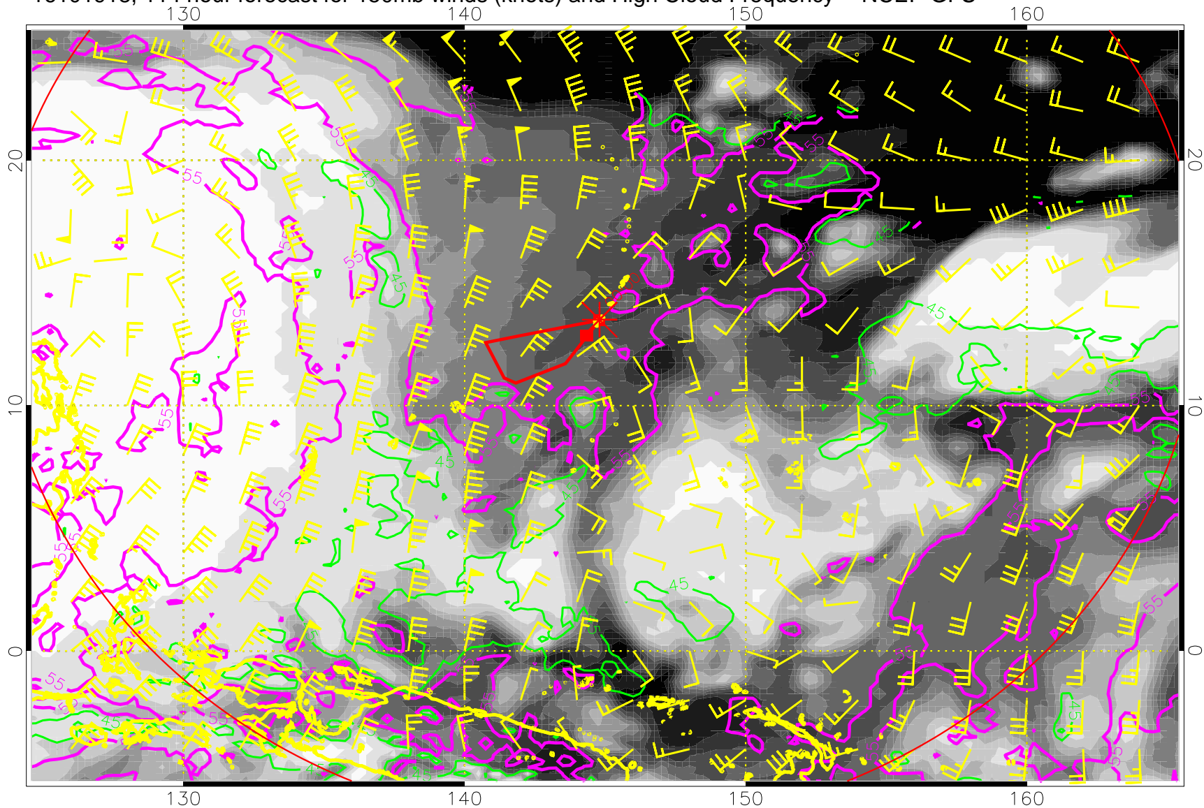
16101918, 114 hour forecast for 150mb winds (knots) and High Cloud Frequency -- NCEP GFS
