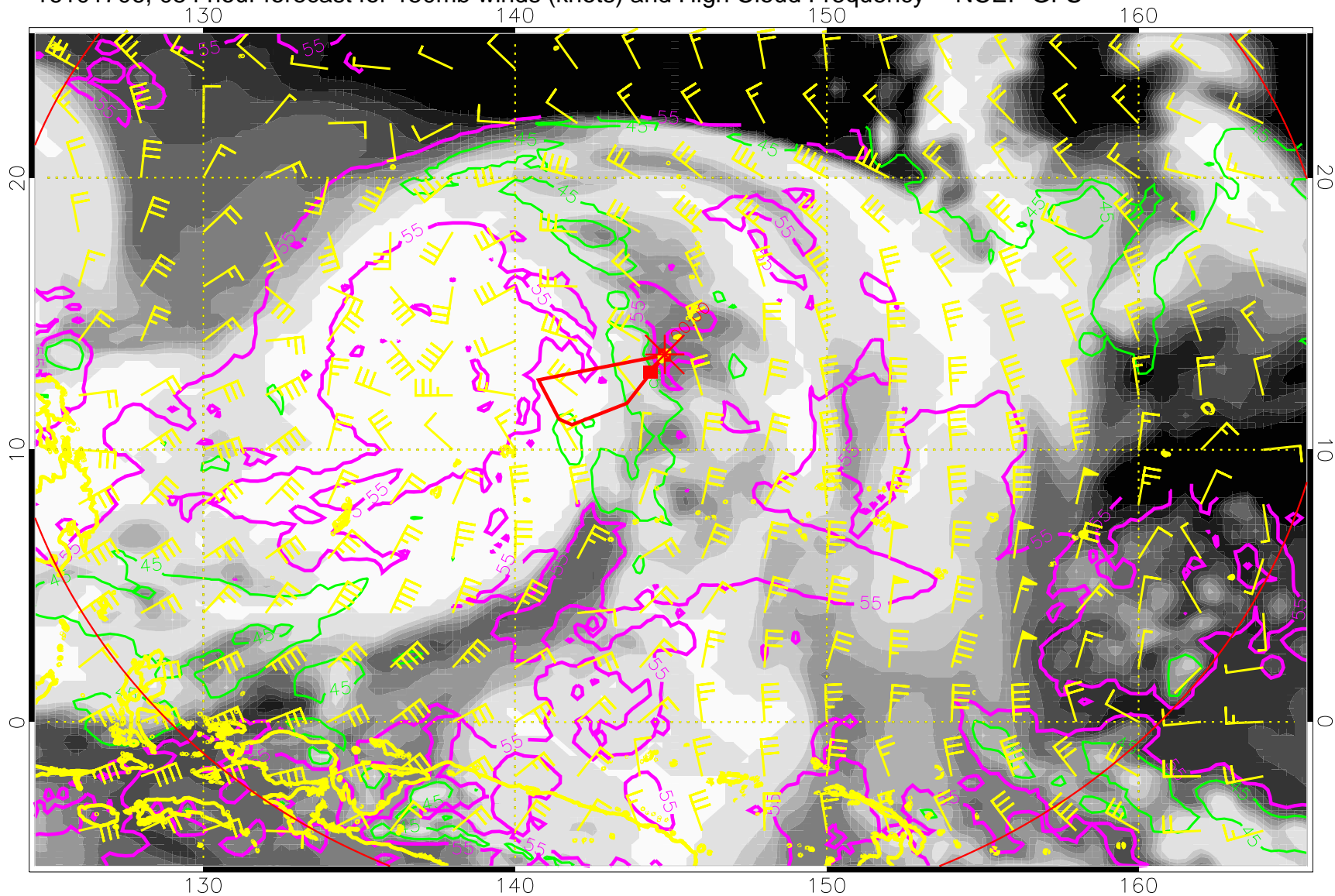
16101706, 054 hour forecast for 150mb winds (knots) and High Cloud Frequency -- NCEP GFS
