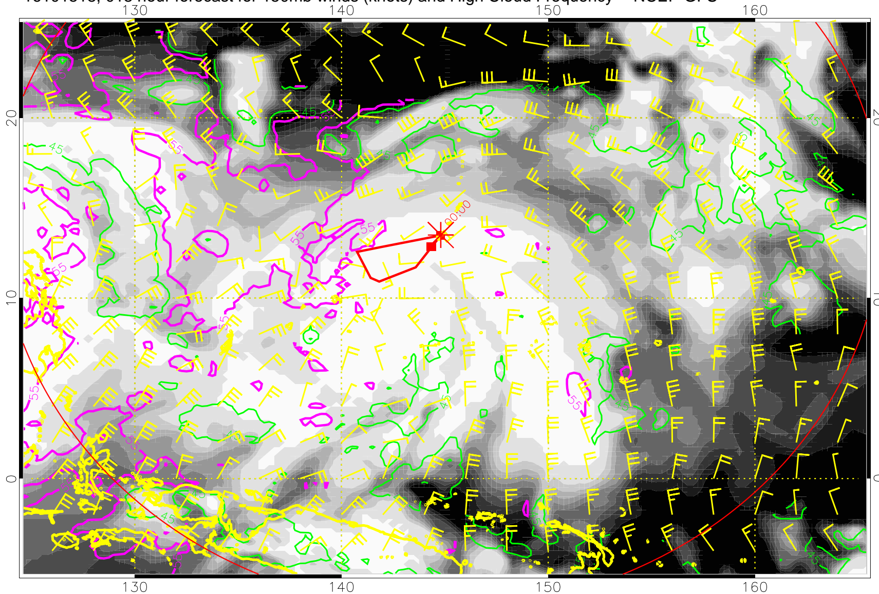
16101518, 018 hour forecast for 150mb winds (knots) and High Cloud Frequency -- NCEP GFS
