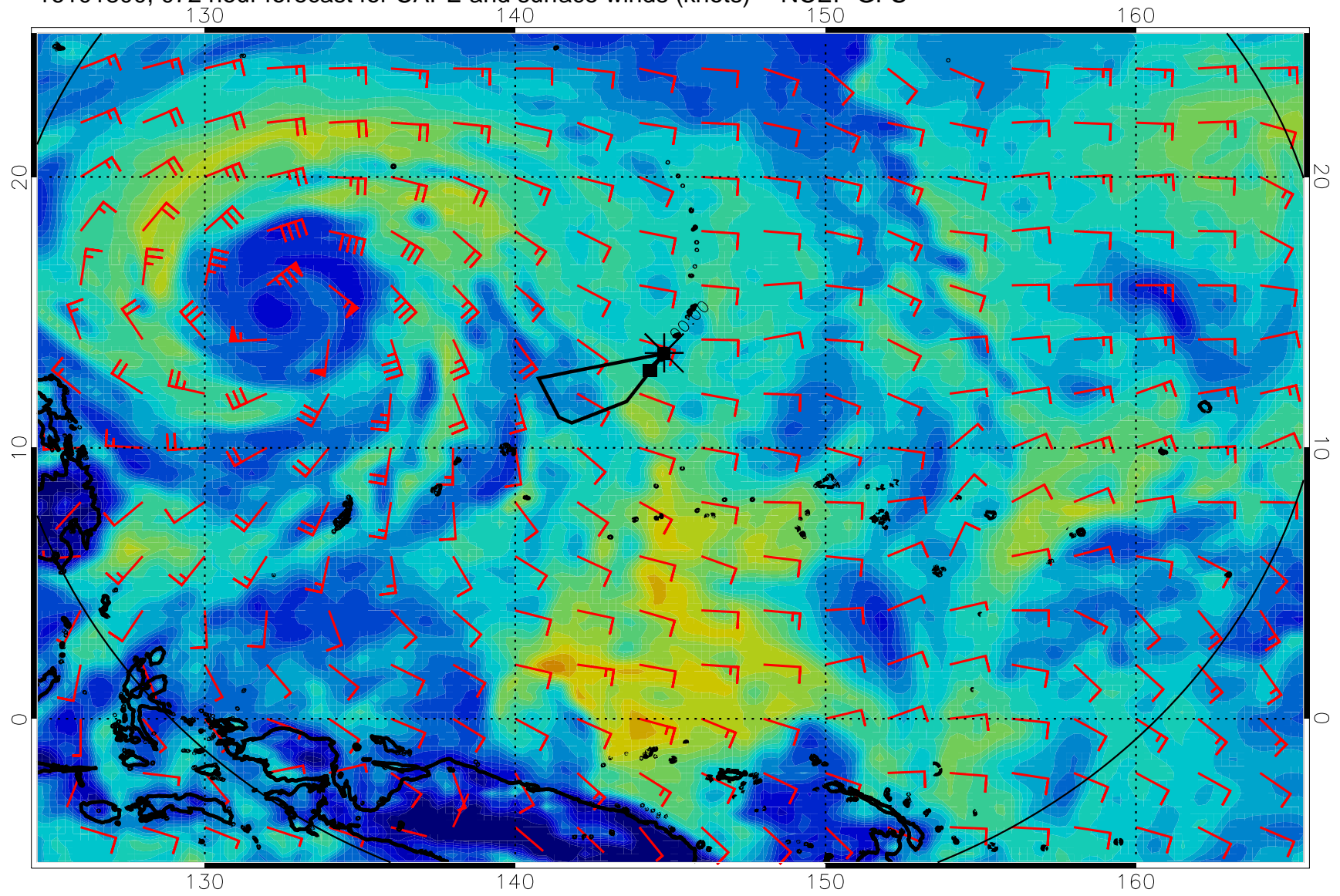
16101800, 072 hour forecast for CAPE and surface winds (knots) -- NCEP GFS
