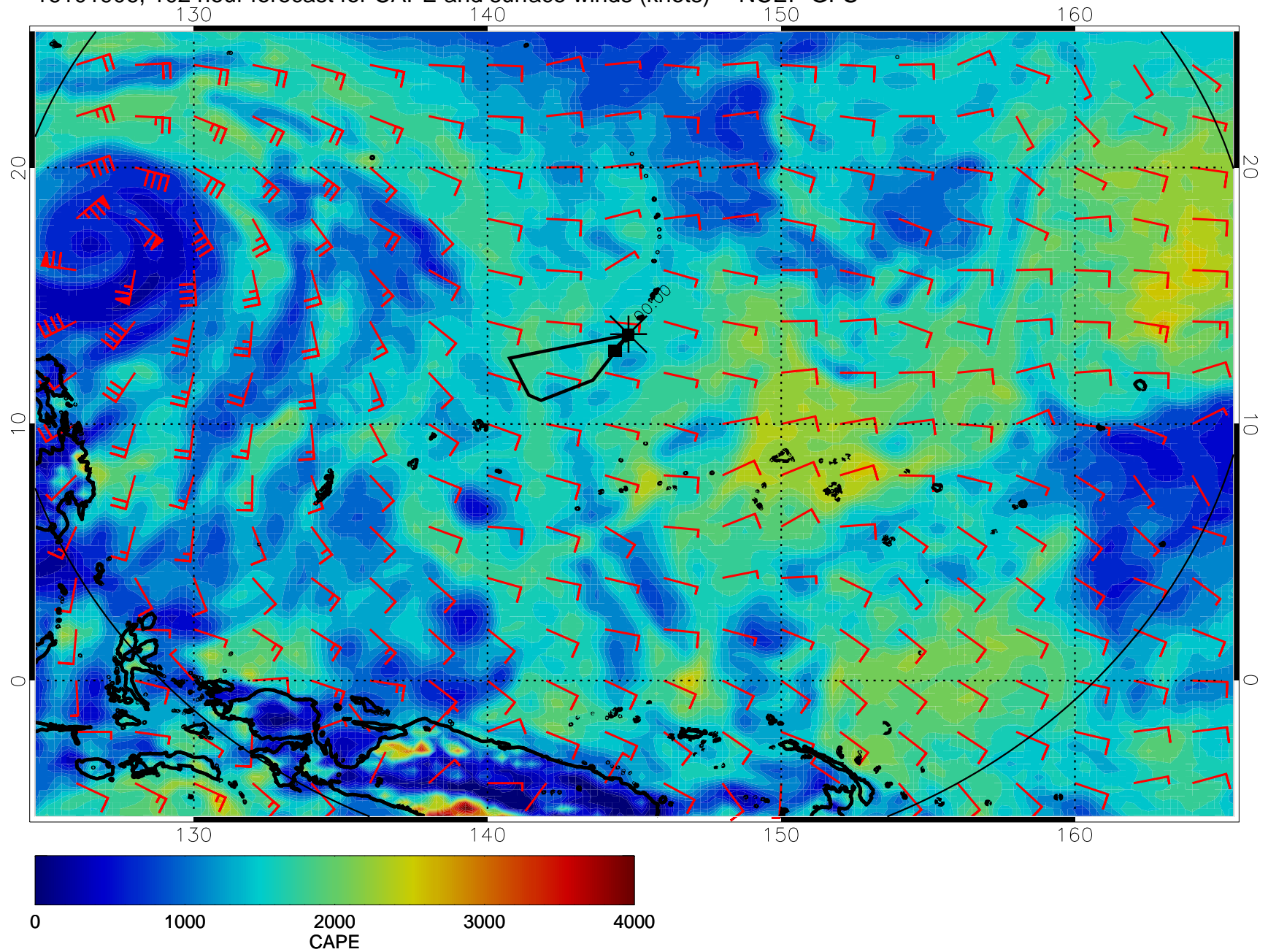
16101906, 102 hour forecast for CAPE and surface winds (knots) -- NCEP GFS
