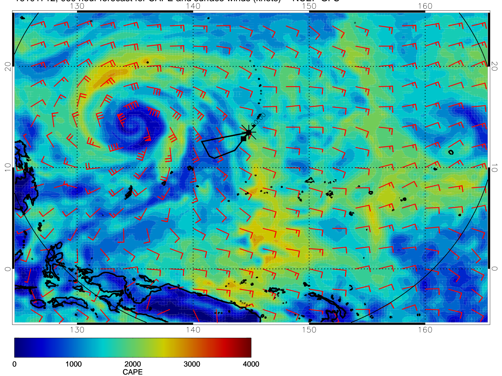
16101712, 060 hour forecast for CAPE and surface winds (knots) -- NCEP GFS
