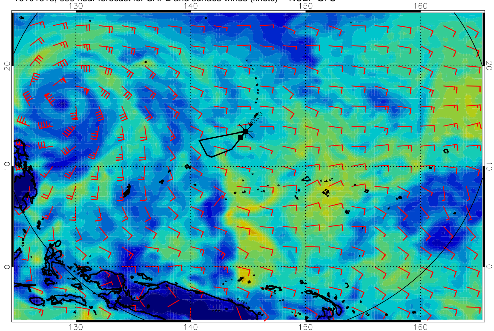
16101818, 090 hour forecast for CAPE and surface winds (knots) -- NCEP GFS
