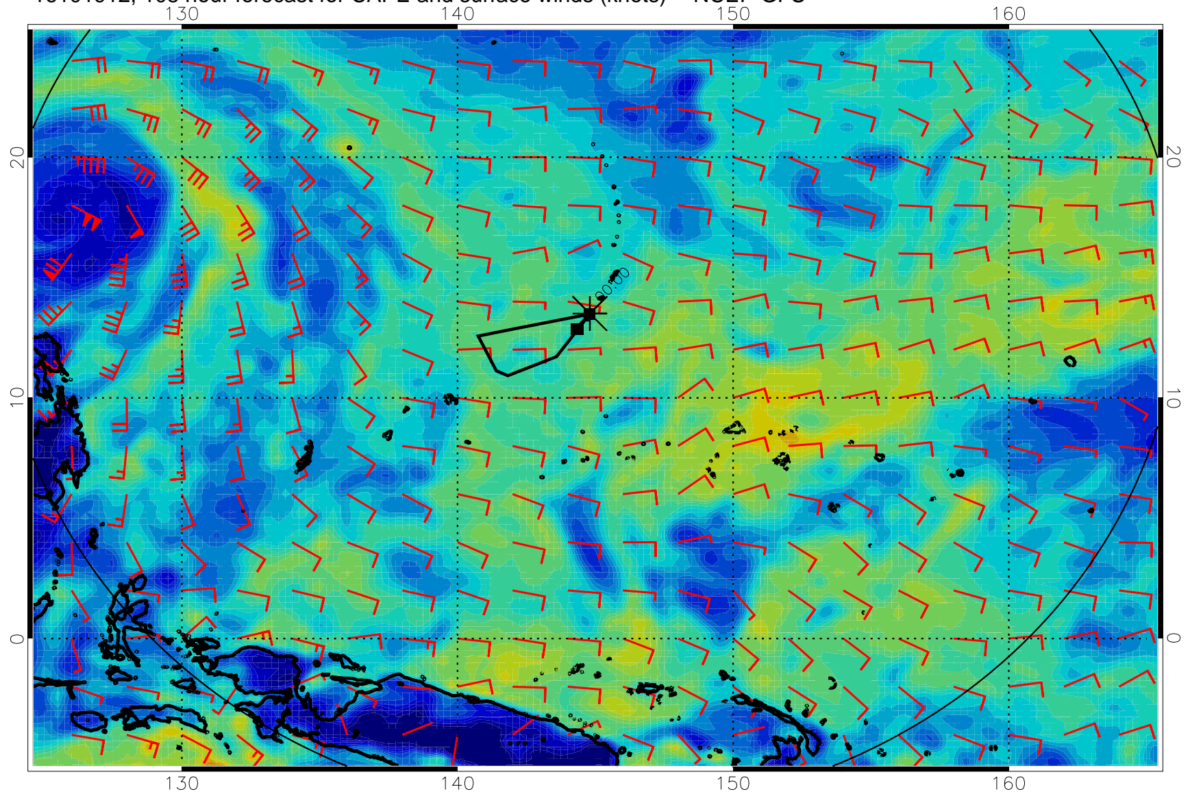
16101912, 108 hour forecast for CAPE and surface winds (knots) -- NCEP GFS
