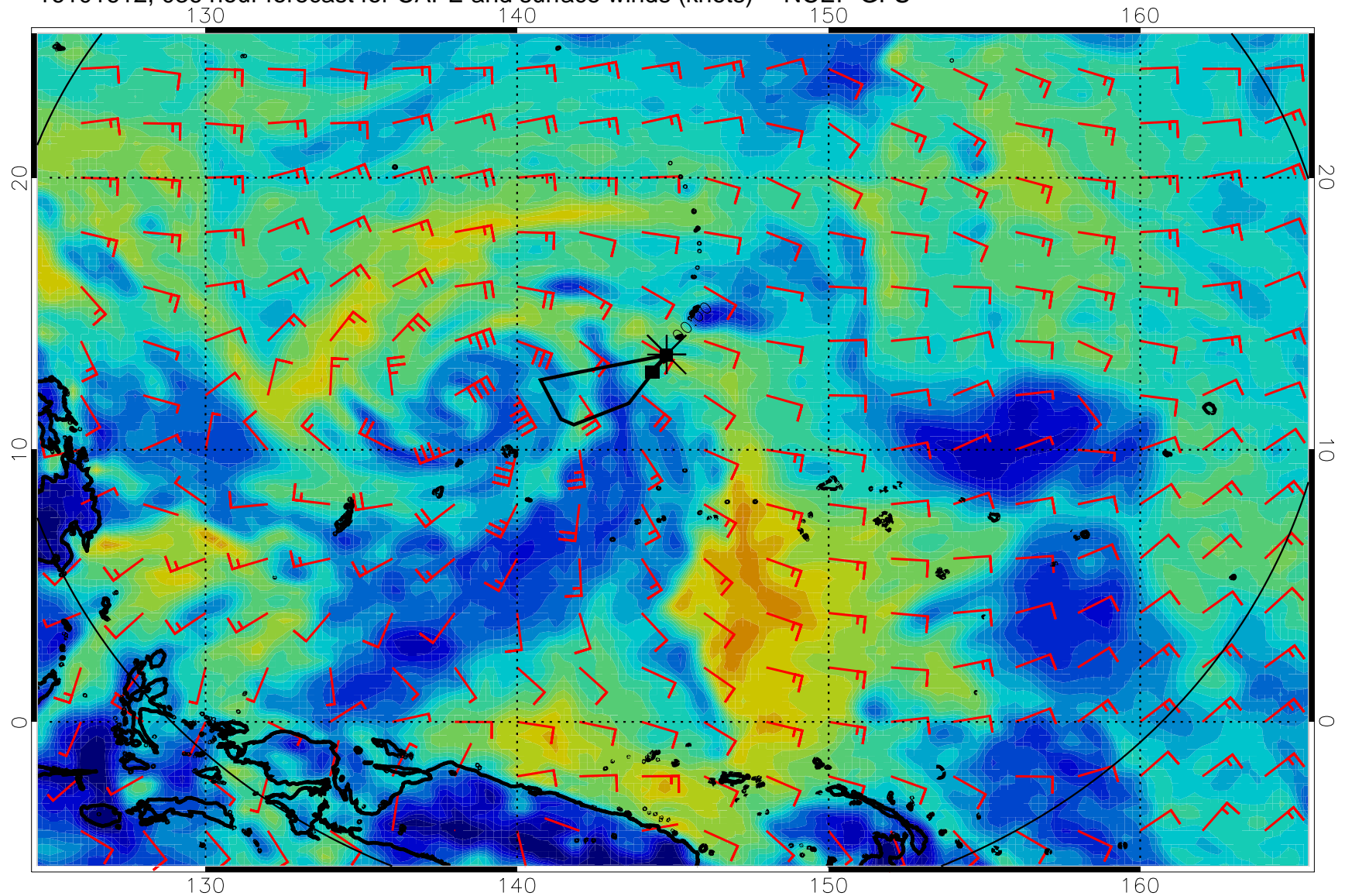
16101612, 036 hour forecast for CAPE and surface winds (knots) -- NCEP GFS
