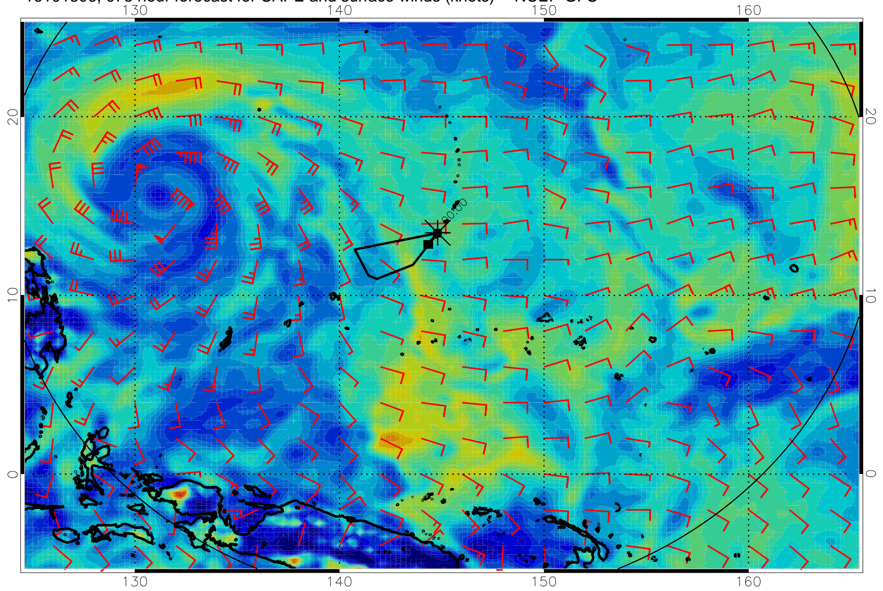
16101806, 078 hour forecast for CAPE and surface winds (knots) -- NCEP GFS
