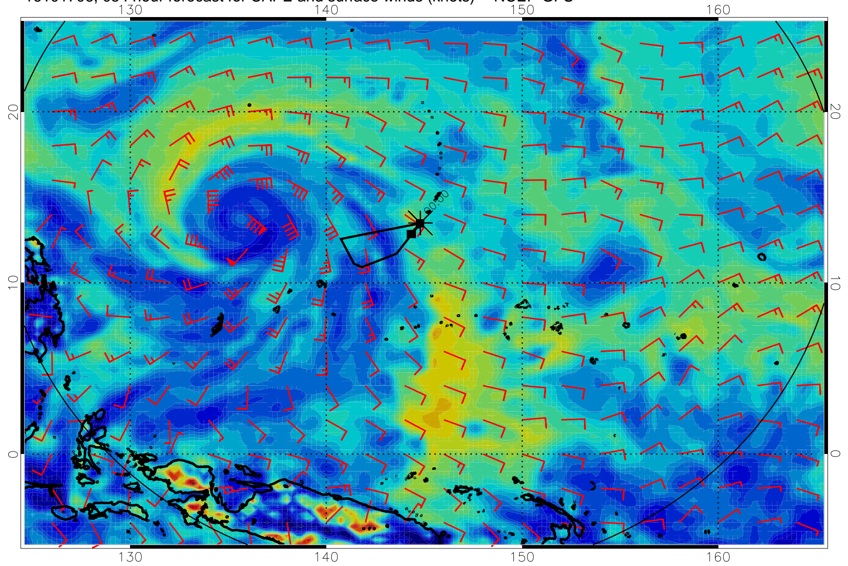
16101706, 054 hour forecast for CAPE and surface winds (knots) -- NCEP GFS
