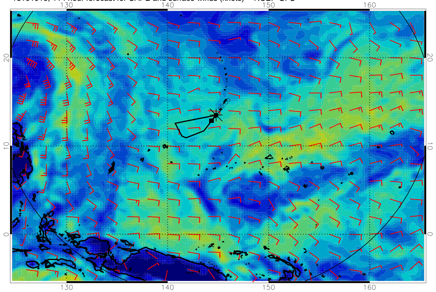
16101918, 114 hour forecast for CAPE and surface winds (knots) -- NCEP GFS
