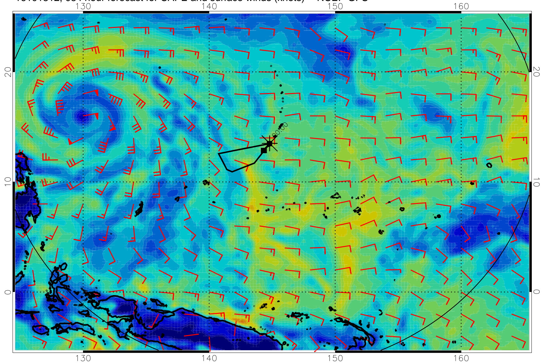
16101812, 084 hour forecast for CAPE and surface winds (knots) -- NCEP GFS
