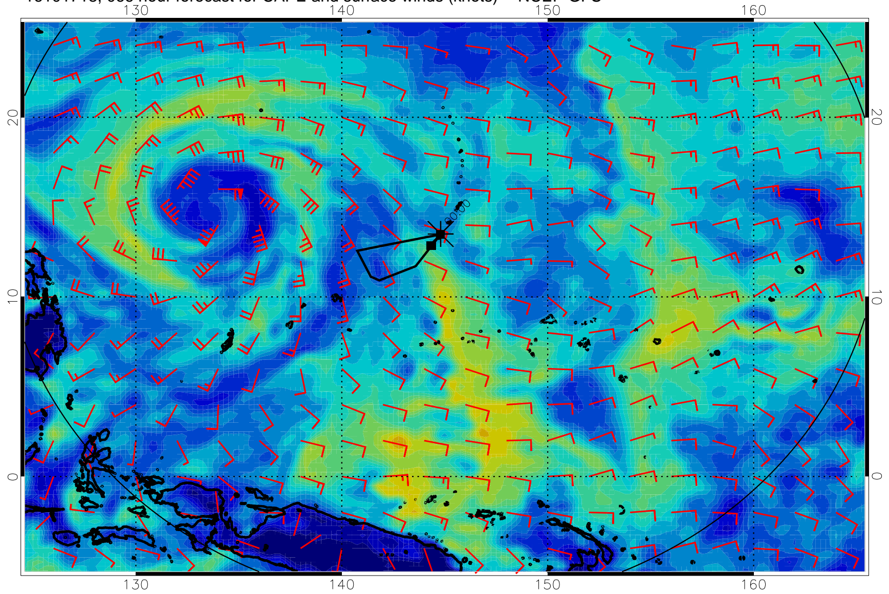
16101718, 066 hour forecast for CAPE and surface winds (knots) -- NCEP GFS
