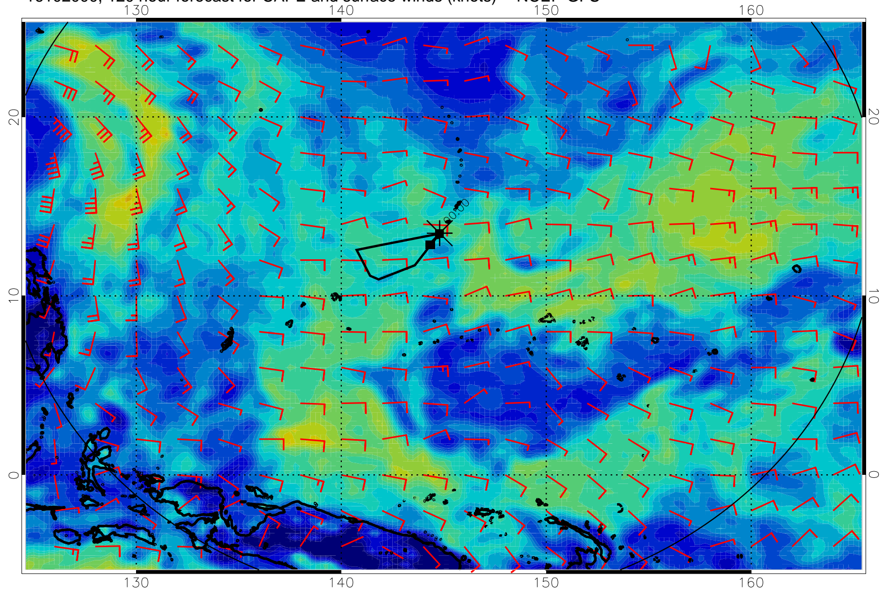
16102000, 120 hour forecast for CAPE and surface winds (knots) -- NCEP GFS
