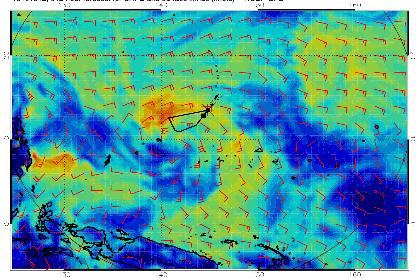
16101512, 012 hour forecast for CAPE and surface winds (knots) -- NCEP GFS
