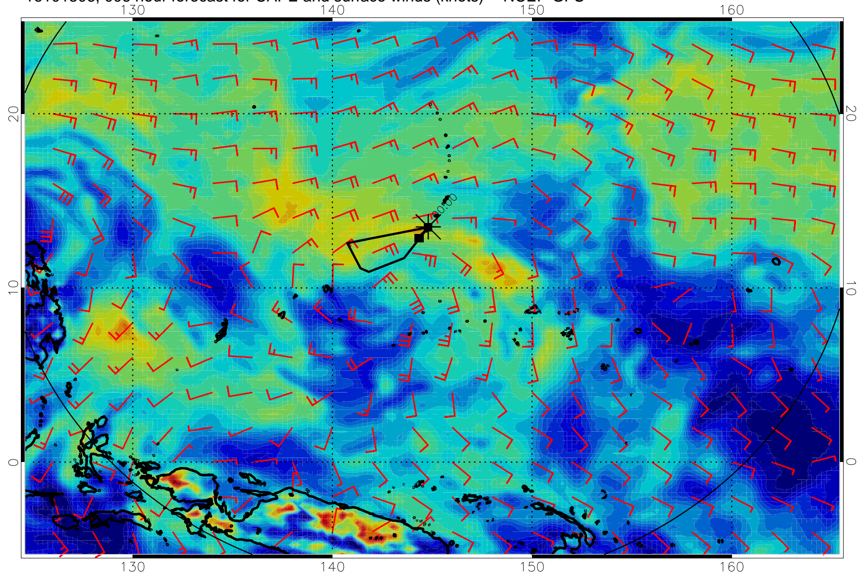
16101506, 006 hour forecast for CAPE and surface winds (knots) -- NCEP GFS
