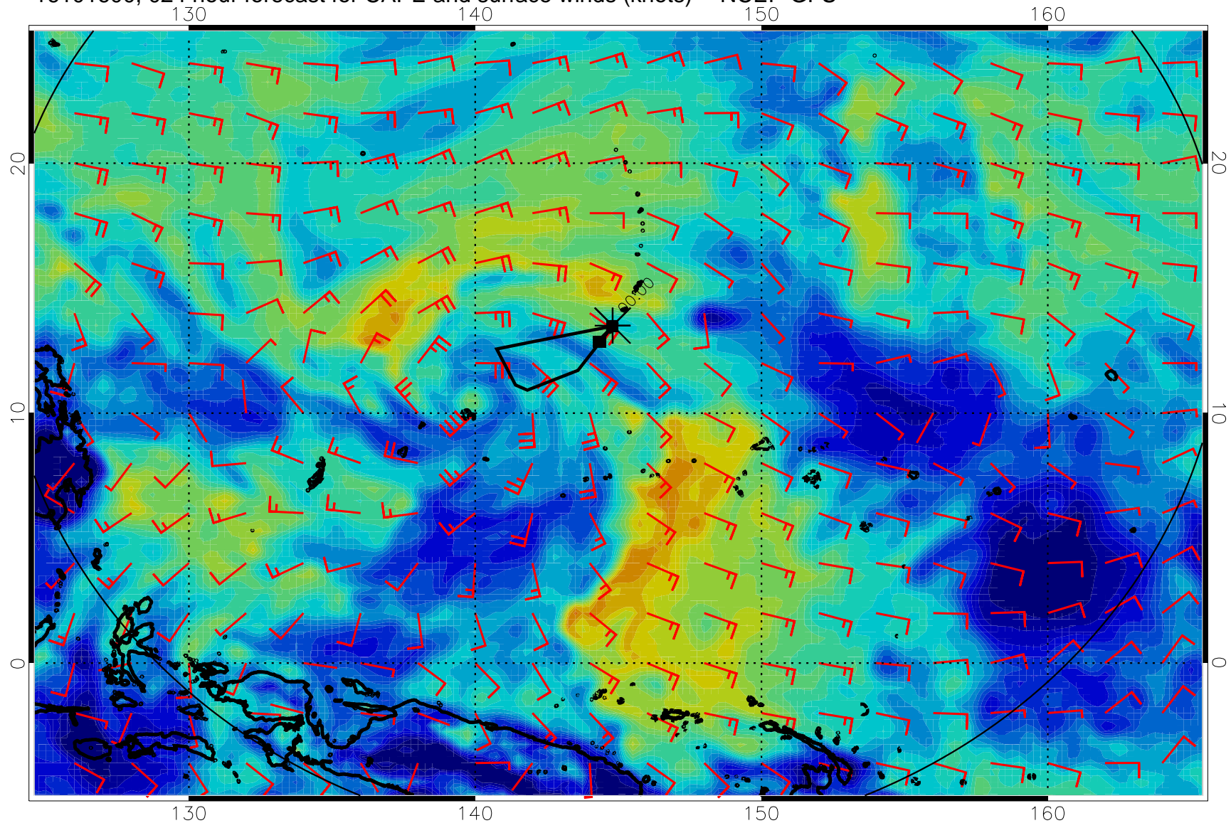
16101600, 024 hour forecast for CAPE and surface winds (knots) -- NCEP GFS
