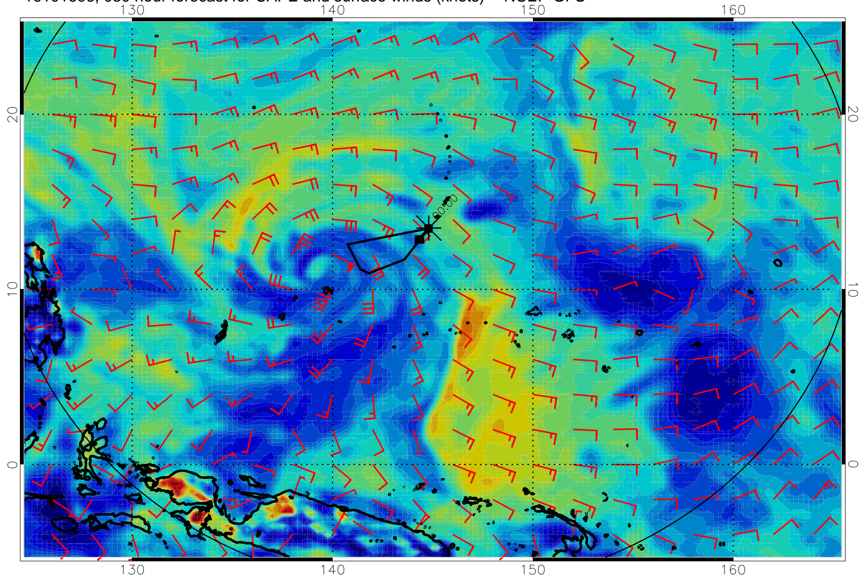
16101606, 030 hour forecast for CAPE and surface winds (knots) -- NCEP GFS
