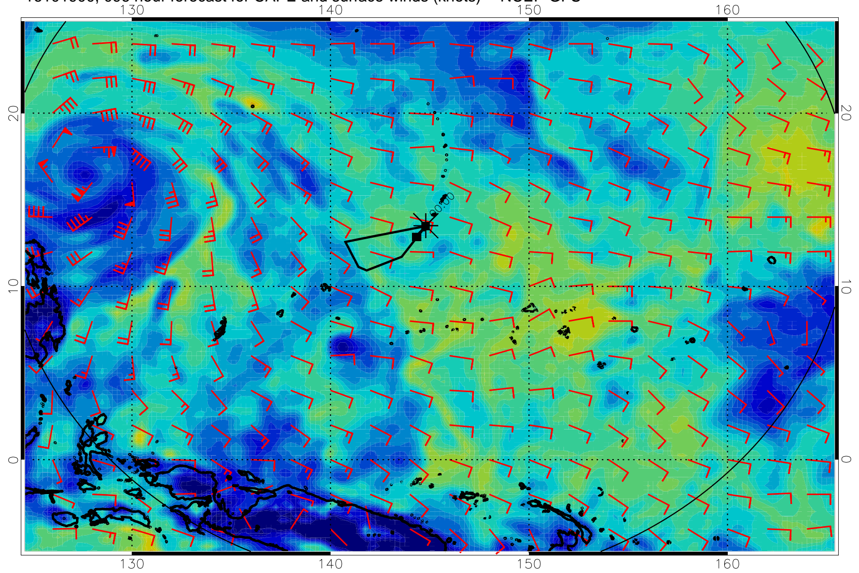
16101900, 096 hour forecast for CAPE and surface winds (knots) -- NCEP GFS
