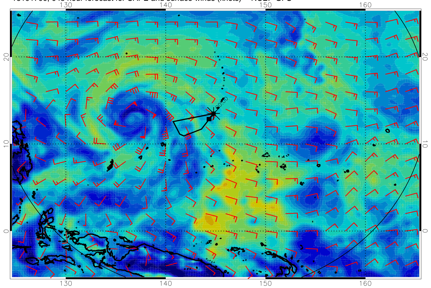
16101700, 048 hour forecast for CAPE and surface winds (knots) -- NCEP GFS
