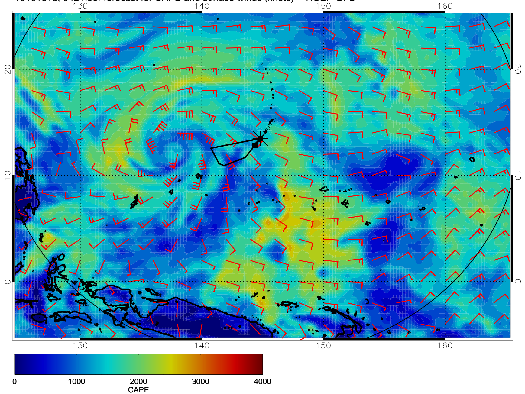
16101618, 042 hour forecast for CAPE and surface winds (knots) -- NCEP GFS
