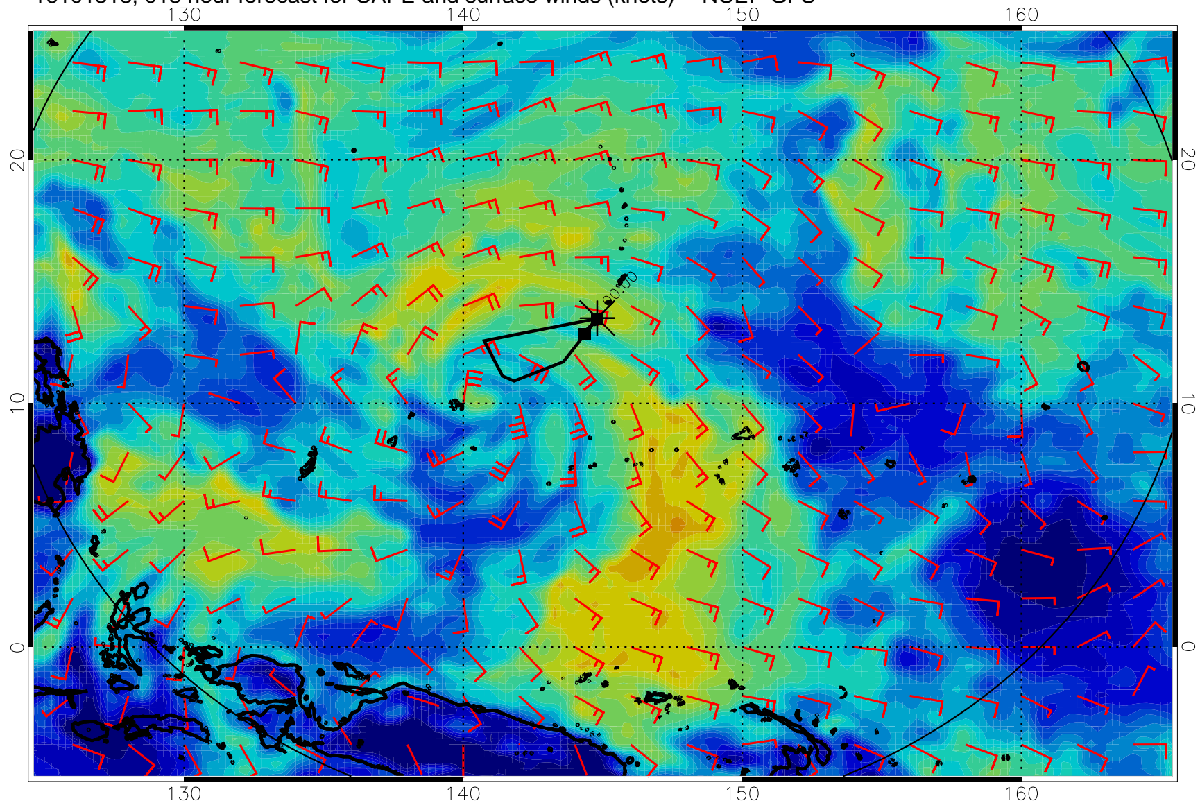
16101518, 018 hour forecast for CAPE and surface winds (knots) -- NCEP GFS
