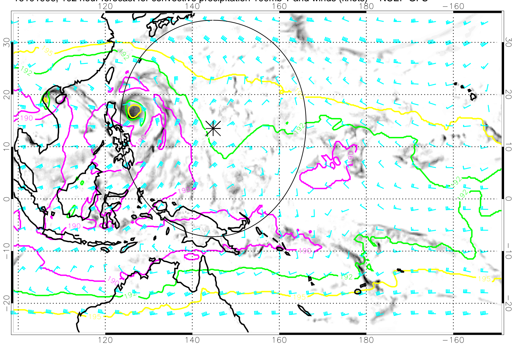
16101906, 102 hour forecast for convective precipitation 100mb T and winds (knots) -- NCEP GFS
